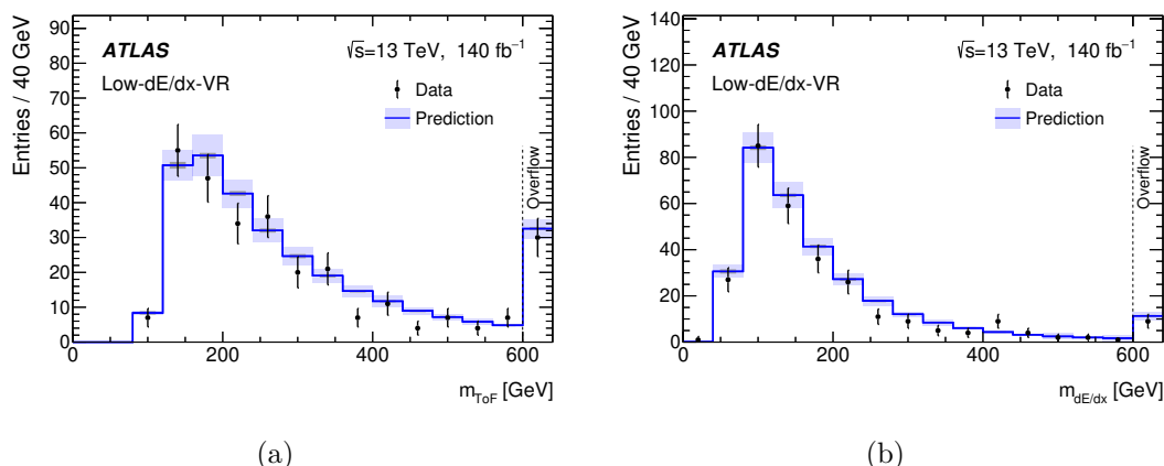
Figure 5. Comparison of predicted (a) m_{\text{ToF}} and (b) m_{dE/dx} background to data in the low- dE/dx validation region. The statistical and systematic uncertainty in the predicted background is calculated as indicated in section 5.5 and shown as a coloured band. The histogram overflow is added into the rightmost bin.
