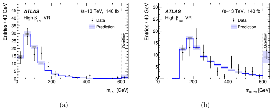
Figure 6. Comparison of predicted (a) m_{\text{ToF}} and (b) m_{dE/dx} background to data in the high- \beta_{\text{ToF}} validation region. The statistical and systematic uncertainty in the predicted background is calculated as indicated in section 5.5 and shown as a coloured band. The histogram overflow is added into the rightmost bin.
