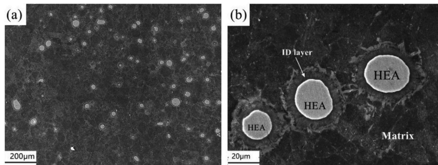
Fig. 15. Microstructure of CoCrFeMnNi HEA-particles reinforced 2024 Al-matrix composites showing SEM images at (a) low magnification; (b) high magnification [47]. Cullled with permission from Elsevier.
