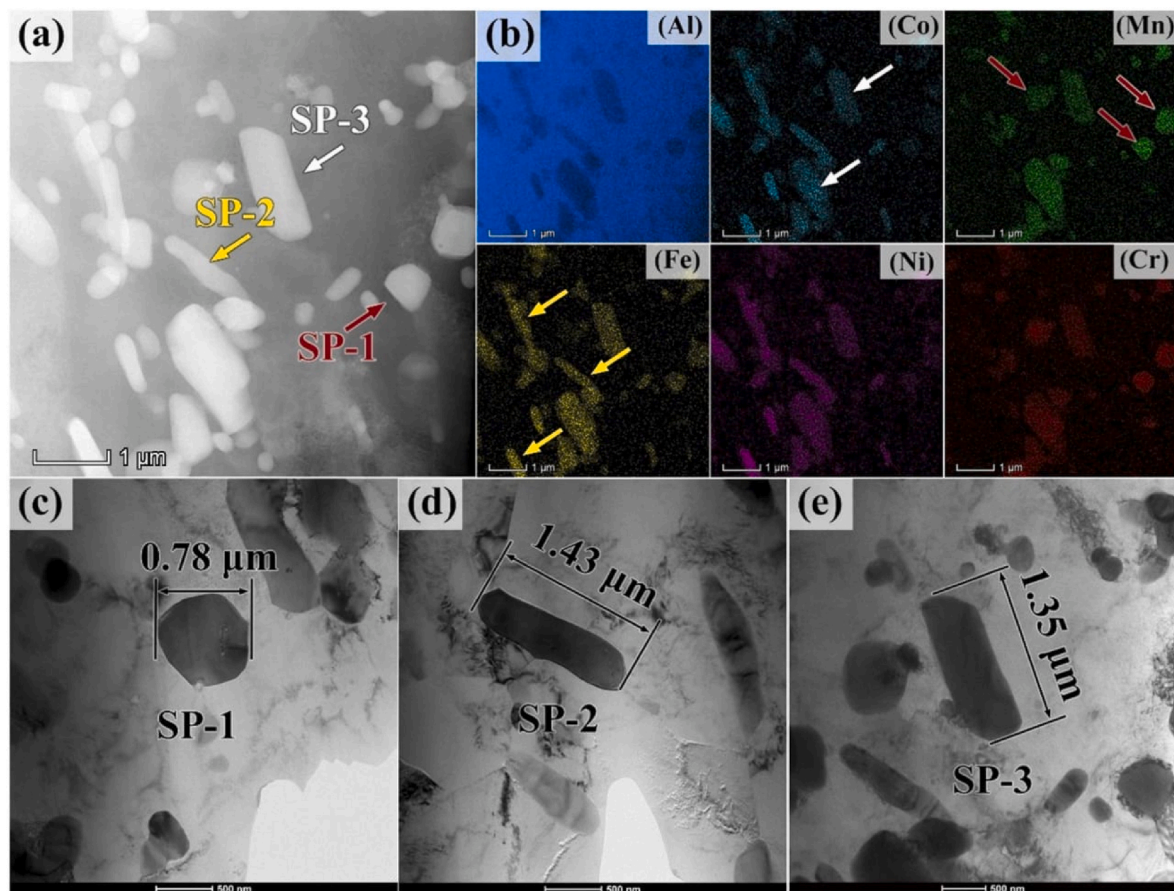
Fig. 19. TEM images and element mapping results of the sample S3: (a) the dark-field image of the TEM foil, (b) the corresponding element mapping results of (a), and (c–e) the magnification micrographs of the formed second phases [88]. Culled with permission from Elsevier.
