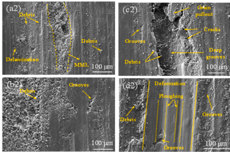
Fig. 22. Wear track topography for the different HEAp at a fixed applied load of 30 kN and sliding velocity of 70 mm/s for (a2) AA2219, (b2) 1.5 wt%, (c2) 3.0 wt% and (d2) 5.0 wt% high entropy alloy particle/Al matrix composites (MML – mechanically mixed layer) [102] culled with permission from Elsevier.
