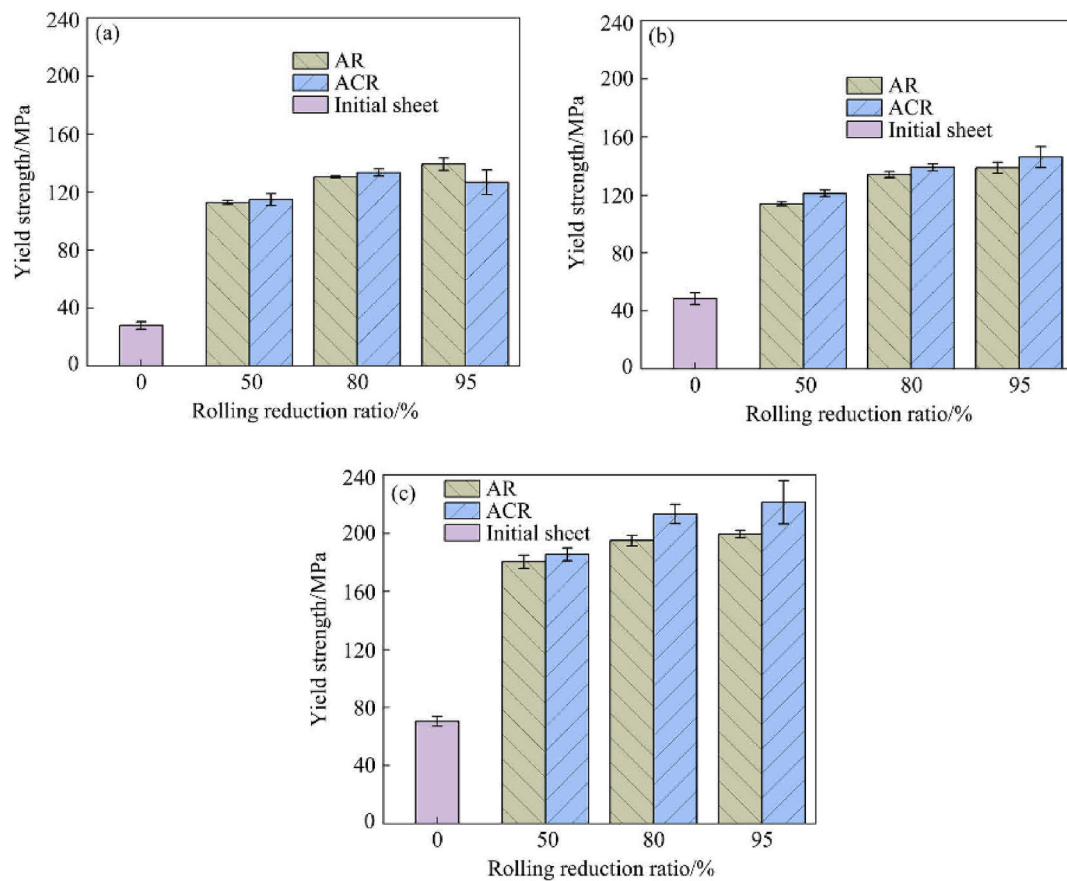
Fig. 11. Yield strength of the initial sheet (as-cast), AR, and ACR samples for: (a) 0 wt% HEAP; (b) 1 wt% HEAP; (c) 3 wt% HEAP [73]. Cullled with permission from Elsevier.
