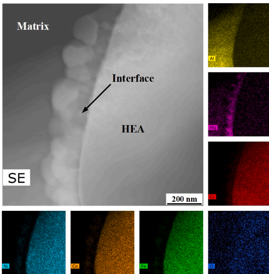
Fig. 9. Transmission electron microscopy image of the HEA/Al-matrix interface and live mapping of the constituent elements [39]. Culled with permission from Elsevier.
