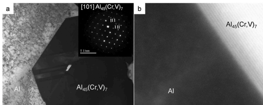
Fig. 7. Results of scanning/transmission electron microscopy (STEM/TEM) for 3 wt% HEA particle reinforced Al-matrix. (a) Bright-field TEM image and the diffraction pattern along [101] zone axis of \text{Al}_{45}(\text{Cr,V})_7 diffusion layer. (b) STEM image of the \text{Al}_{45}(\text{Cr,V})_7 HEA reinforcement/Al-matrix interface [63]. Culled with permission from Elsevier.
