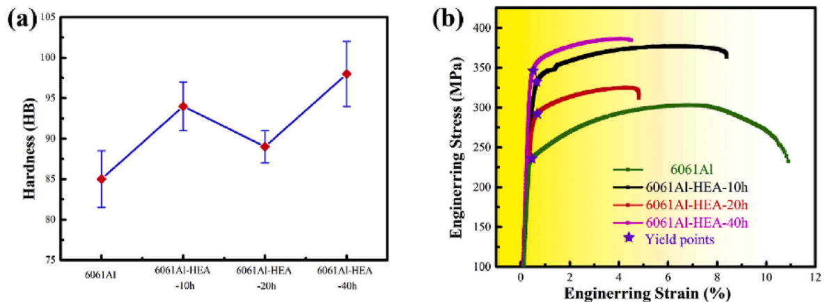
Fig. 17. The effect of milling time on the (a) hardness and (b) yield strength of the HEA/6061Al composites [37]. Cullled with permission from Elsevier.
