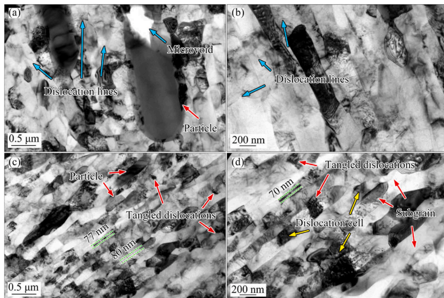
Fig. 12. TEM images of 3 wt% HEA-particles reinforced AMCs with 95% rolling reduction via AR (a, b) and ACR (c, d) processes [73]. Cullled with permission from Elsevier.
