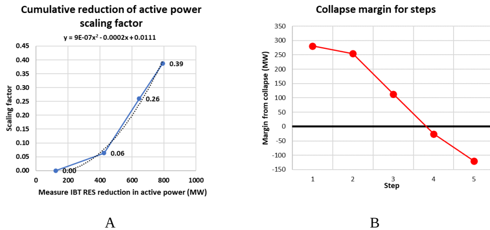
Figure 67 – Cumulative reduction of active-power export scaling factor and collapse margin for steps 1-4
