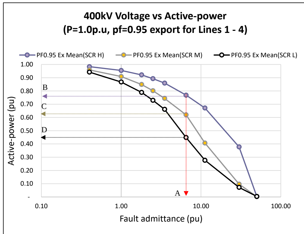
Figure 29 – Impact of active-power export reduction for varied fault admittance for high, medium and low system strengths for various initial conditions of active-power and reactive-power
