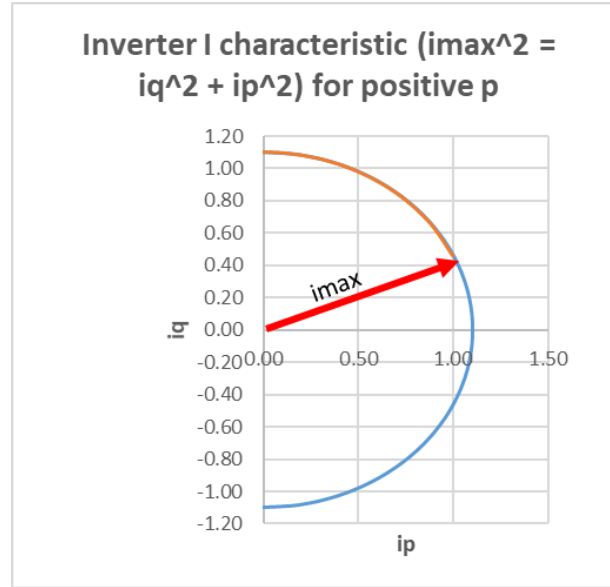
Figure 22 - Inverter Current (I) characteristic (active and reactive current)
