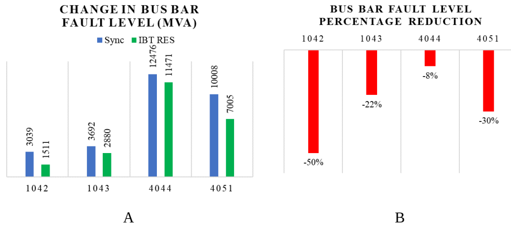
Figure 51 – Fault level comparison for the synchronous scenario and for the IBT RES scenario
