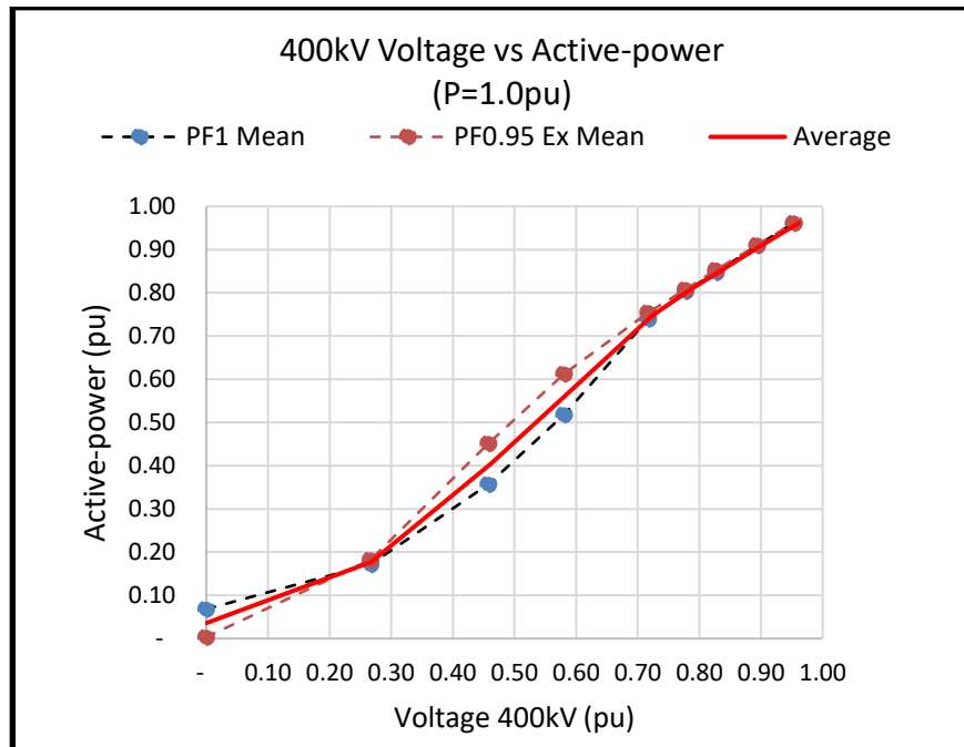
Figure 33 – Average Tx busbar voltage vs active-power export reduction for active-power output 1p.u.
