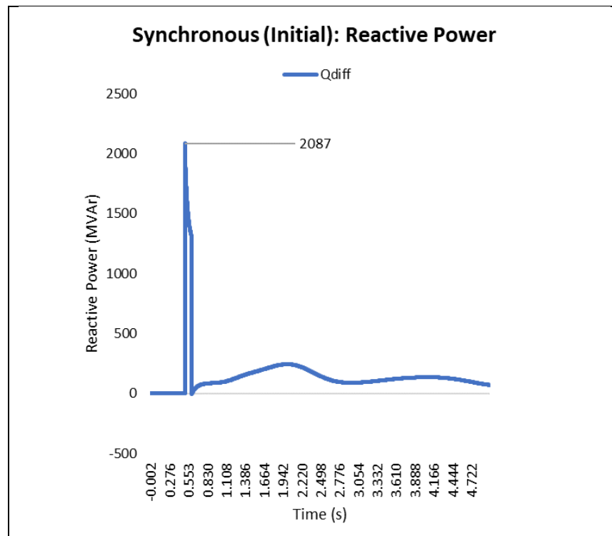
Figure 71 – Synchronous scenario reactive-power response.
