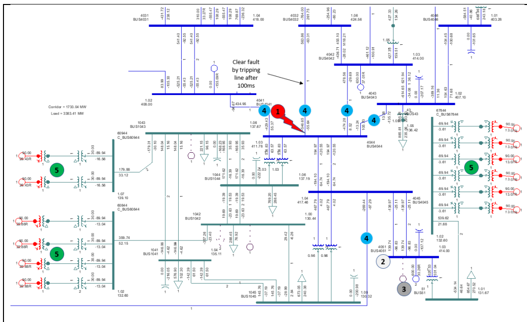
Figure 53 – IBT RES Scenario: Initial steady-state conditions and load flow results
