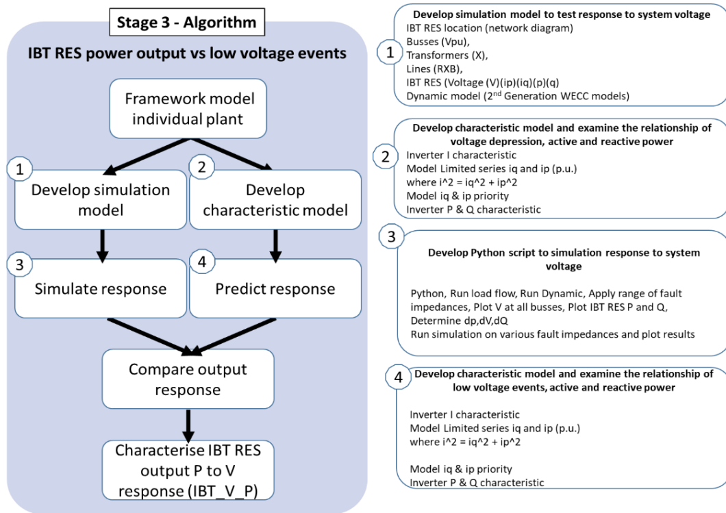
Figure 20 – IBT RES active-power vs LVRT procedure
