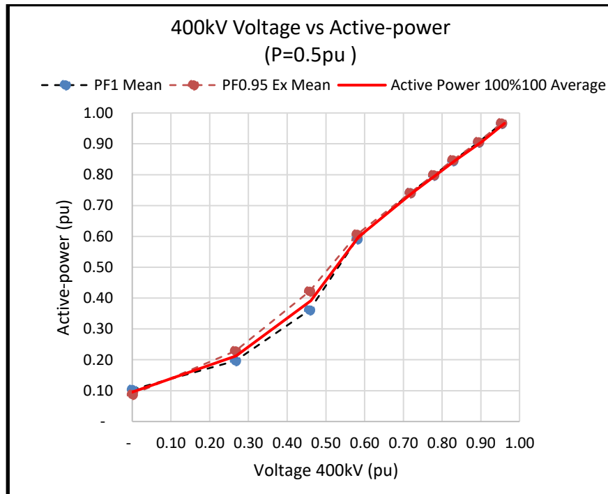
Figure 34 – Average Tx voltage versus active-power export reduction for initial active-power export of 0.5pu
