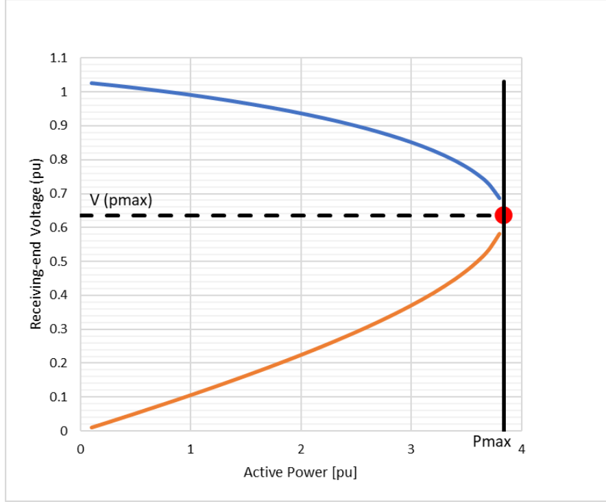
Figure 5 – Voltage stability analysis: P-V curve
