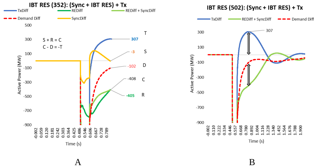
Figure 73 – IBT RES active-power response
