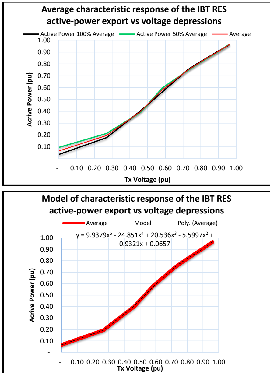
Figure 35 - Average characteristic response of 1pu and 0.5pu initial IBT RES active-power export curves to determine the Tx voltage vs active-power export characteristic model
