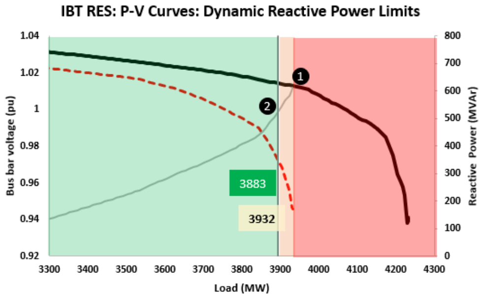
Figure 46 – IBT RES scenario: P-V steady-state analysis with 5% reactive-power safety margin and limit
