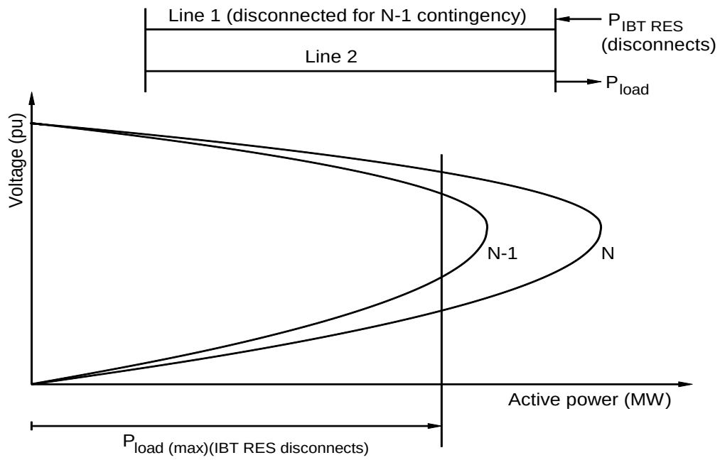
Figure 10 – IBT RES present but disconnects during the network contingency
