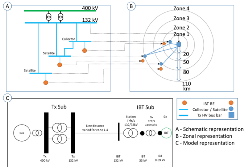
Figure 18 – Simulation model
