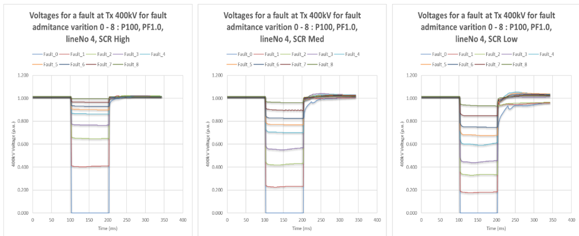
Figure 27 – Transmission voltage depression for high, medium and low system strength
