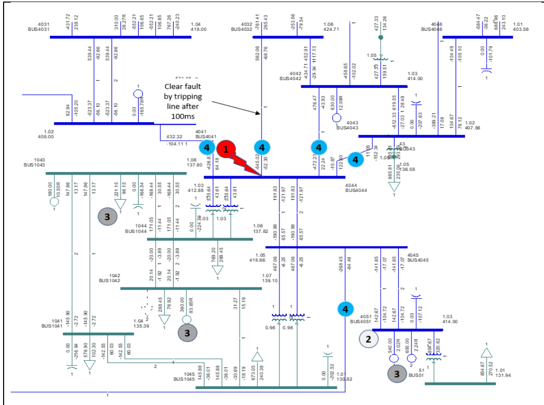
Figure 52 – Synchronous Scenario: Initial steady-state conditions and load flow results
