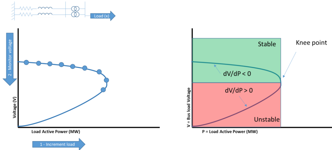
Figure 6 – Classical P-V curves and classical voltage stability definitions
