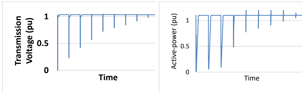
Figure 26 - Nine faults with different fault admittance values causing different Tx busbar voltage dip depths (left) and different IBT RES active-power exports (right)
