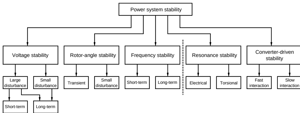
Figure 3 – Revised power system stability classification [PES-TR77]
