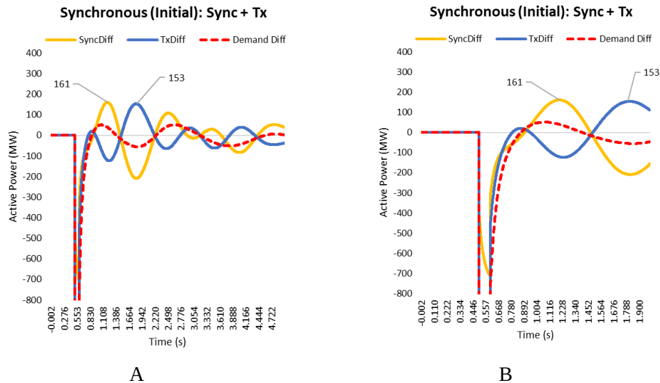
Figure 58 – Synchronous scenario: active-power response
