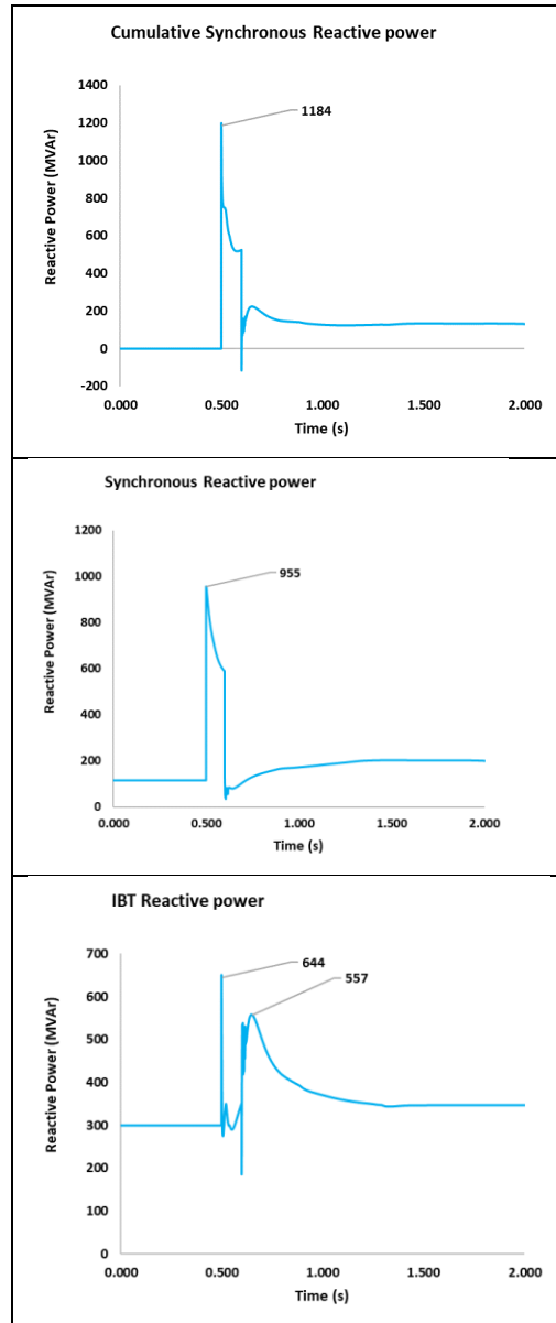
Figure 74 – IBT RES scenario reactive-power response
