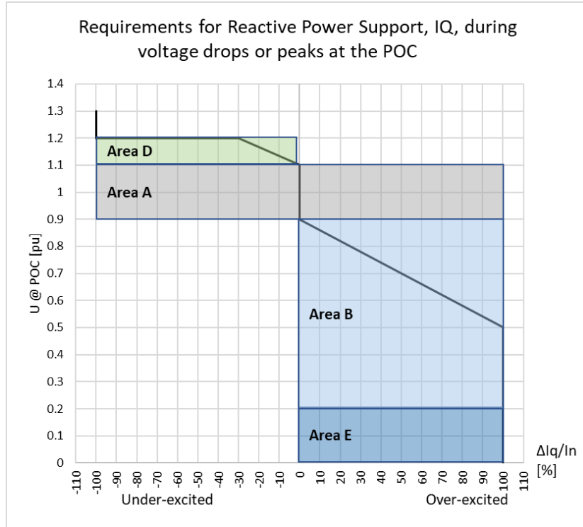
Figure 14 – SAGCRPP requirements for reactive-current export \Delta I_q/I_n , during low-voltage and high-voltage events at the POC [37]
