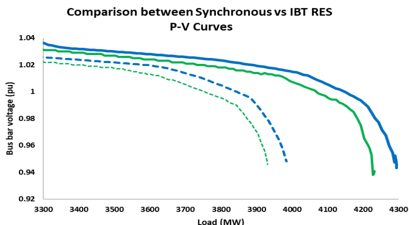
Figure 49 - P-V curve comparison of the synchronous scenario (blue) and of the IBT RES scenario (green) for the base network (solid lines) and worst contingency (dashed lines)
