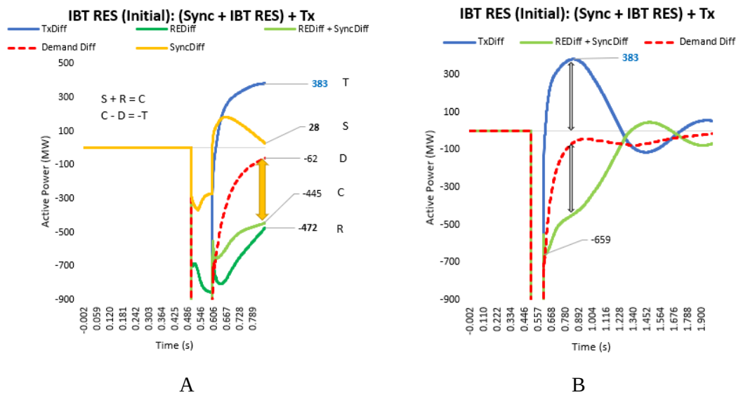
Figure 62 – IBT RES scenario active-power responses (using an accurate network model)
