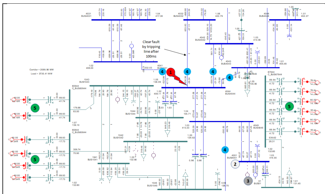
Figure 64 – IBT RES scenario: Network P-V limits and load flow
