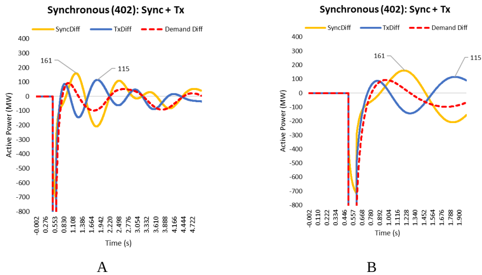
Figure 70 – Synchronous scenario active-power disturbance.
