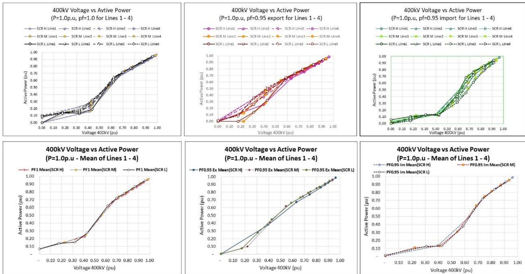
Figure 31 – Active-power export reduction for varied system strengths: high, medium and low for various fixed reactive-power initial conditions.
