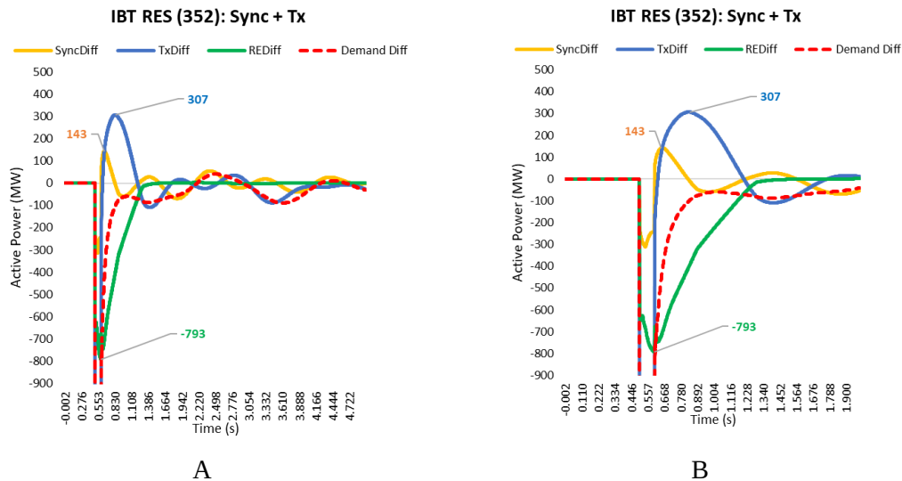
Figure 72 – IBT RES scenario active-power response
