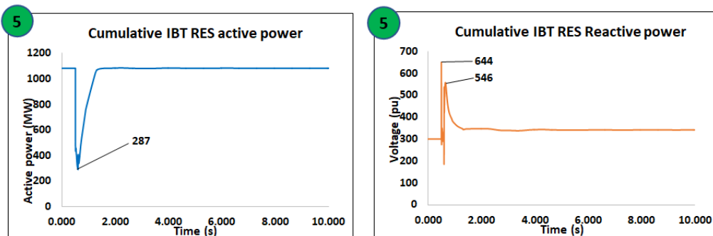
Figure 69 – IBT RES scenario: IBT RES active-power and reactive-power
