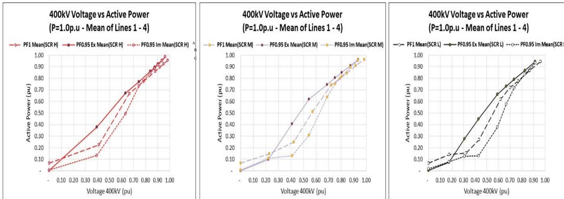
Figure 30 – Active-power export reduction for varied fault admittances for high, medium and low system strengths for various initial conditions.
