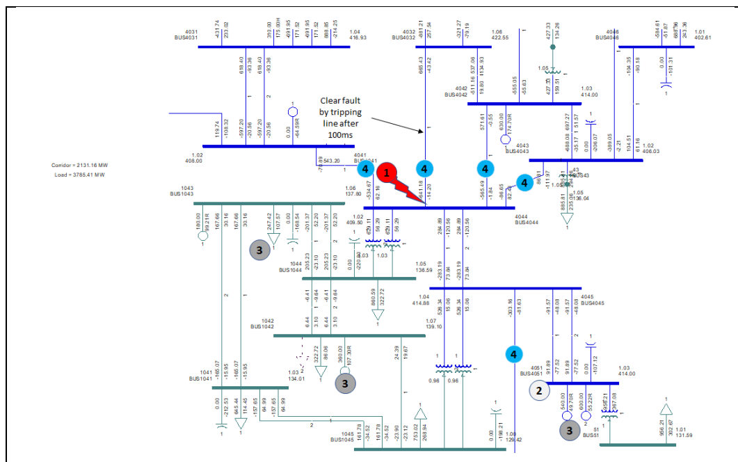
Figure 63 – Synchronous scenario: Network P-V limits condition and load flow
