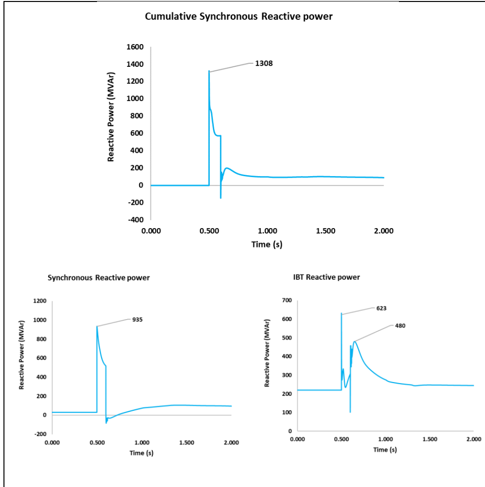
Figure 61 – IBT RES scenario: reactive-power response.
