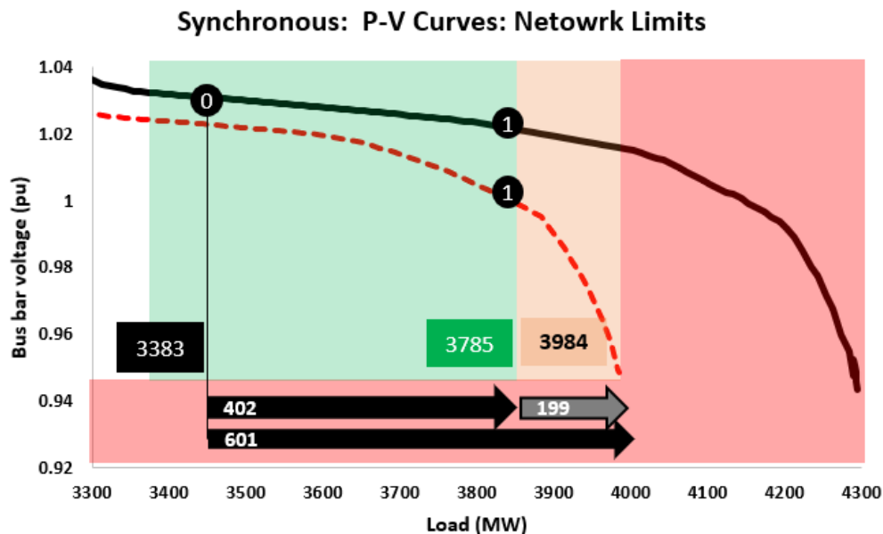
Figure 42 – Synchronous scenario: P-V steady-state analysis for Tx margin (still safe for limiting network contingency) and network limit (voltage collapse for worst network contingencies)
