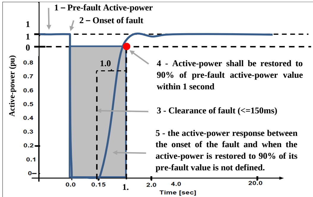
Figure 15 – Post-fault active-power ramp up
