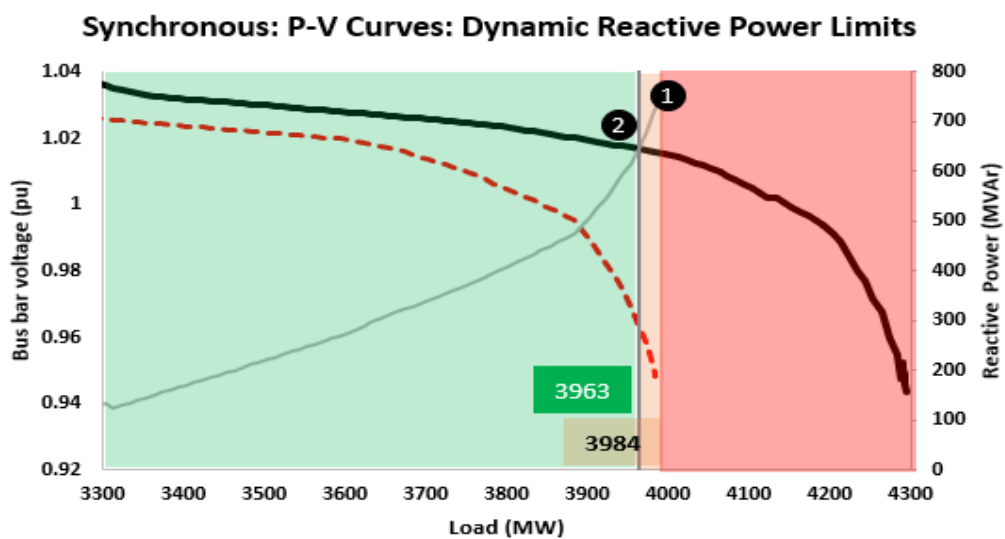
Figure 41 – Synchronous scenario: P-V steady-state analysis with 5% reactive-power safety margin and limit
