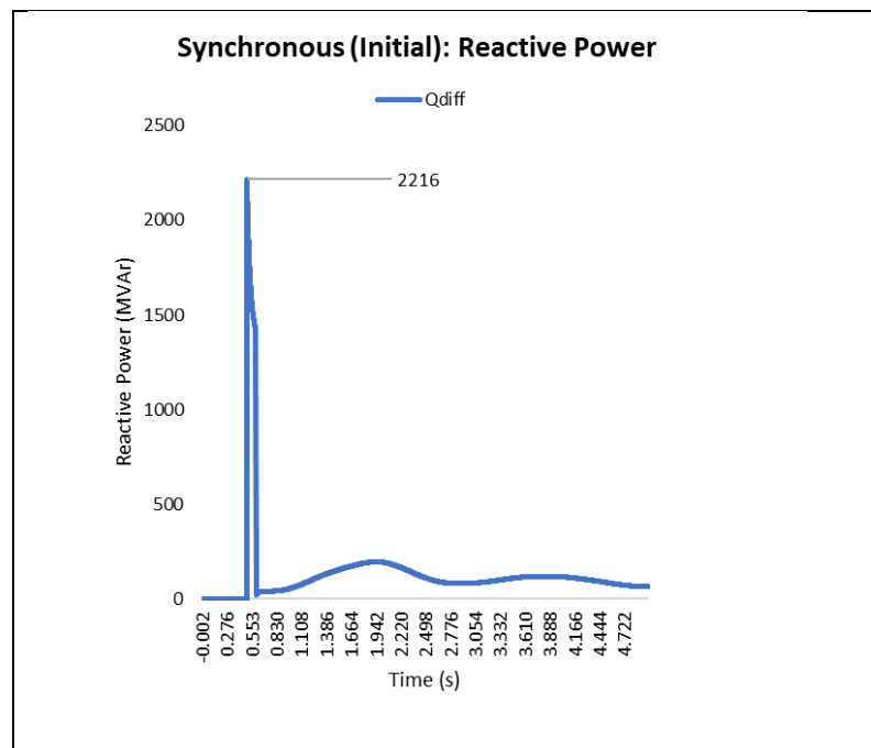
Figure 59 – Synchronous scenario: reactive-power response.
