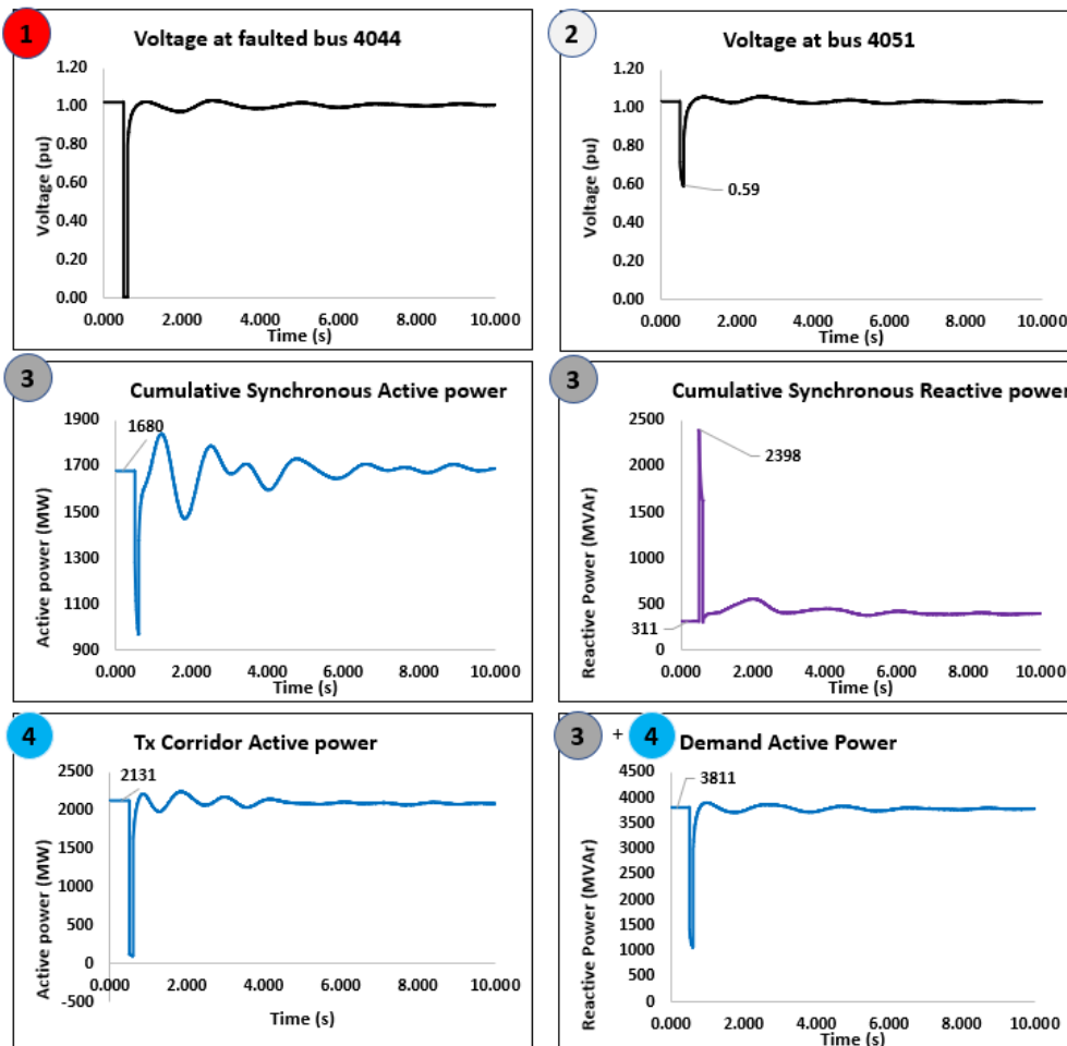
Figure 65 – Synchronous scenario: P-V network results
