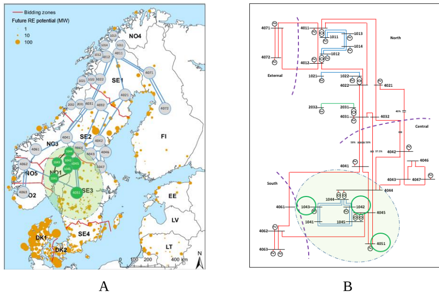
Figure 37 – Cigre Nordic voltage collapse test network
