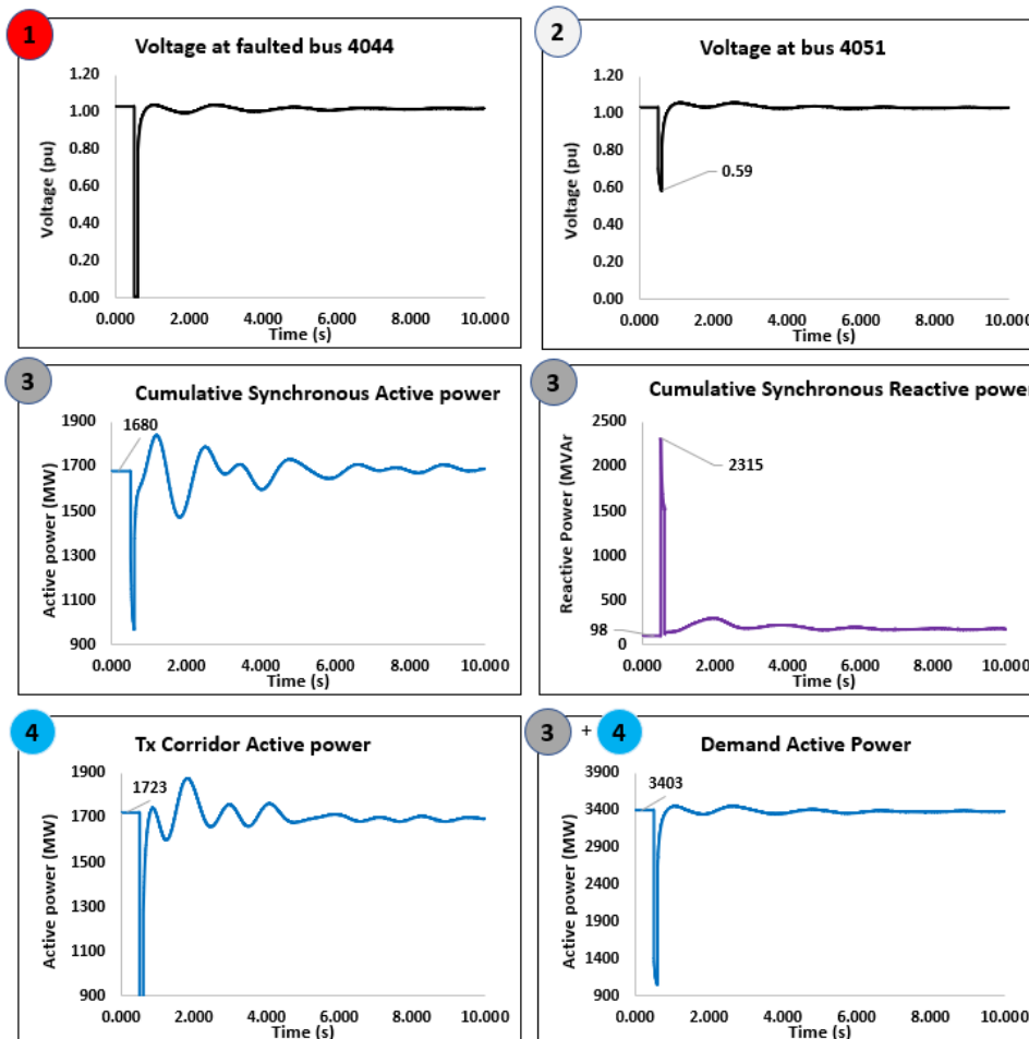
Figure 54 – Synchronous scenario
