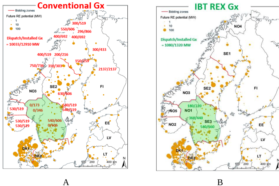
Figure 44 – IBT RES scenario: Synchronous (MW) and IBT RES (MW) location
