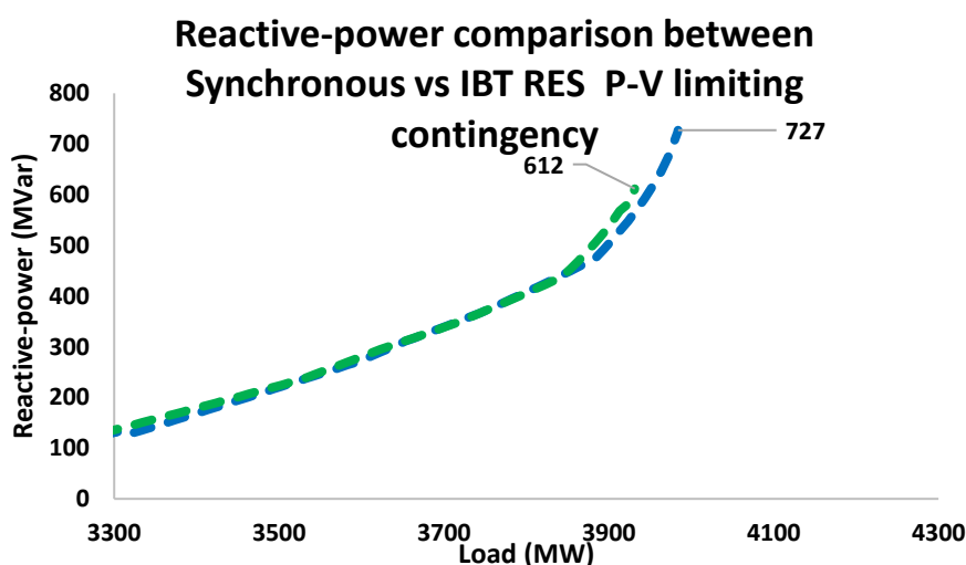
Figure 50 – Reactive-power comparison of the synchronous scenario (blue) and of the IBT RES scenario (green) for the limiting network contingency (dashed lines)
