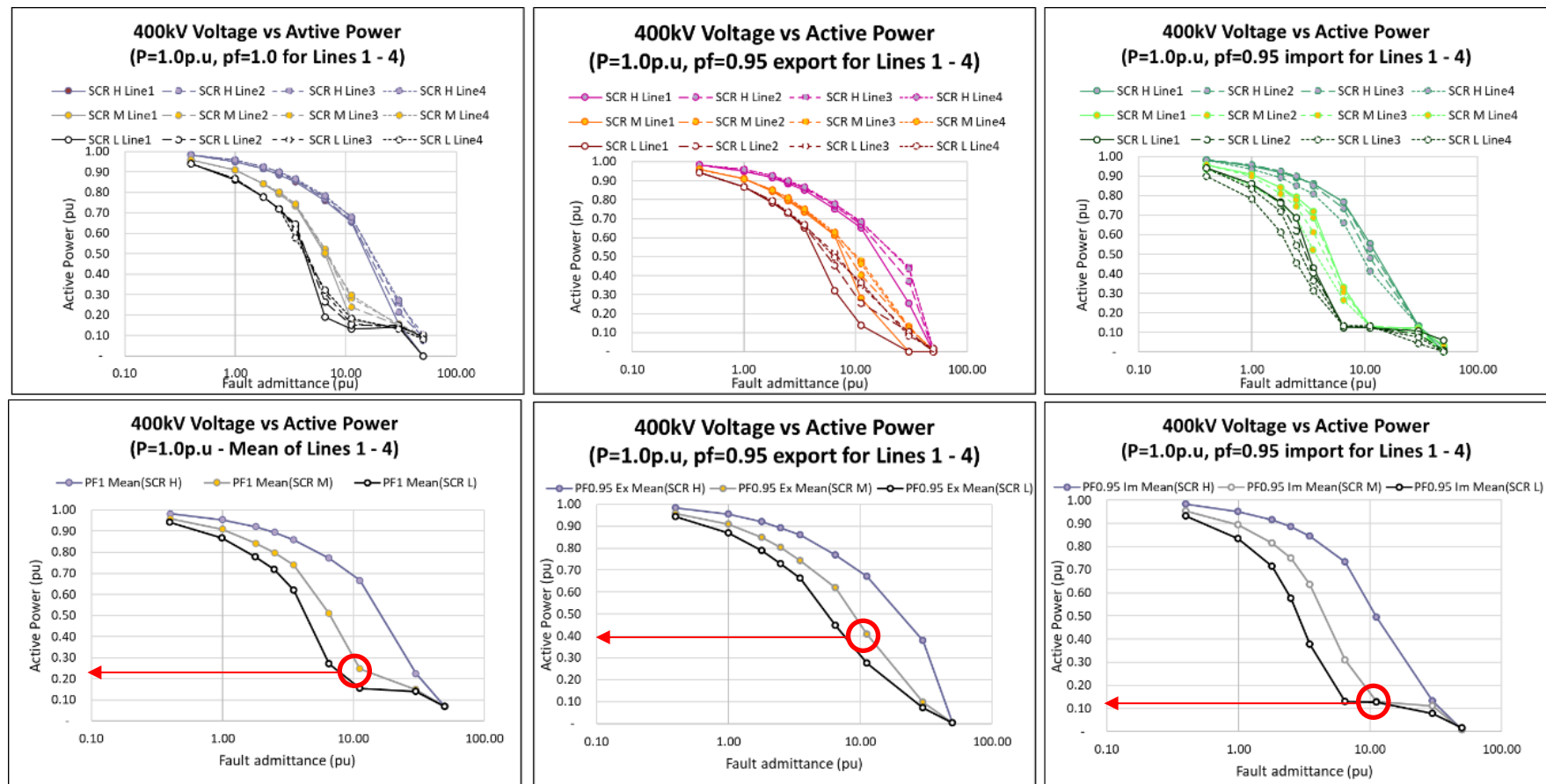
Figure 28 – Active-power export reduction for varied fault admittances for high, medium and low system strengths for various initial conditions of active-power and reactive-power.
