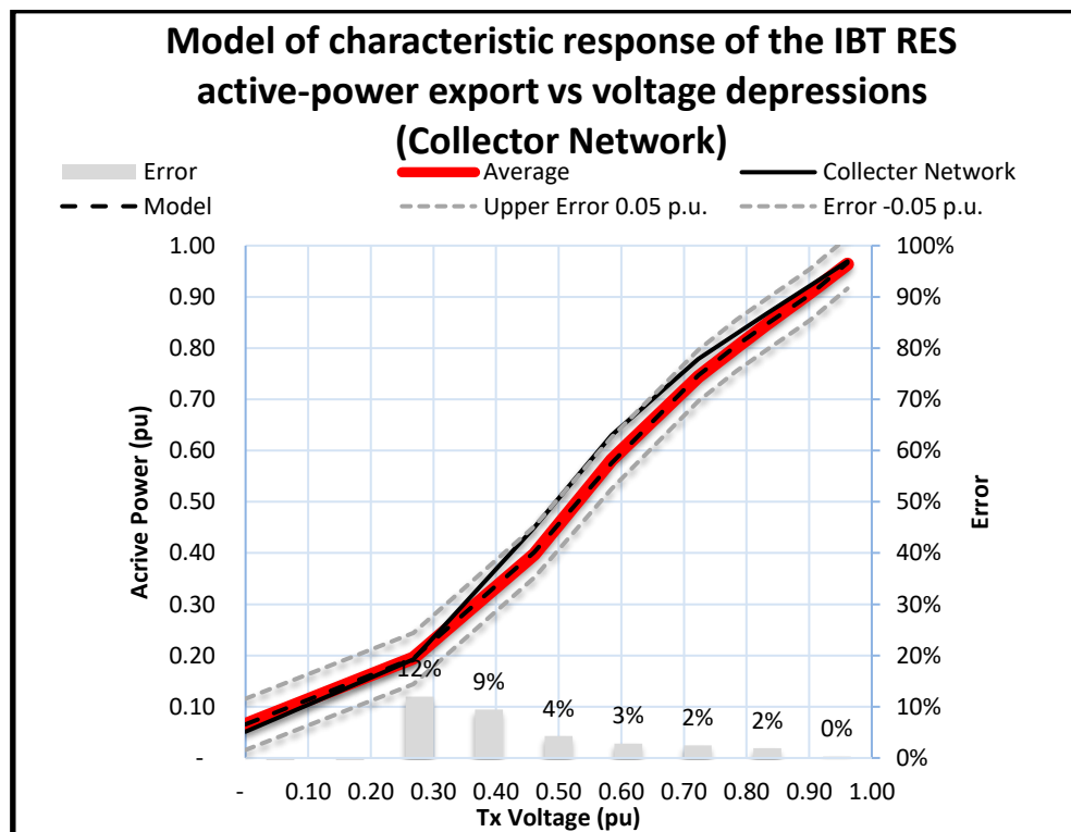
Figure 36 – Characteristic model versus collector network response
