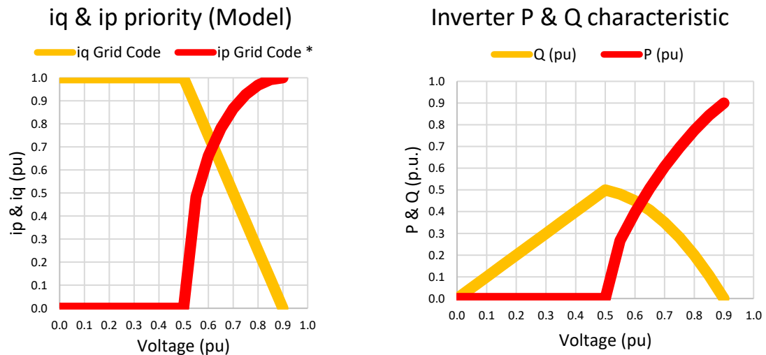
Figure 23 - IBT RES active current (ip) and reactive current (iq) priority (left) and active-power export (P) and reactive-power export (Q) as a function of the voltage at the IBT RES POC (assuming inverter initially exporting zero reactive-power and initially exporting maximum active-power)
