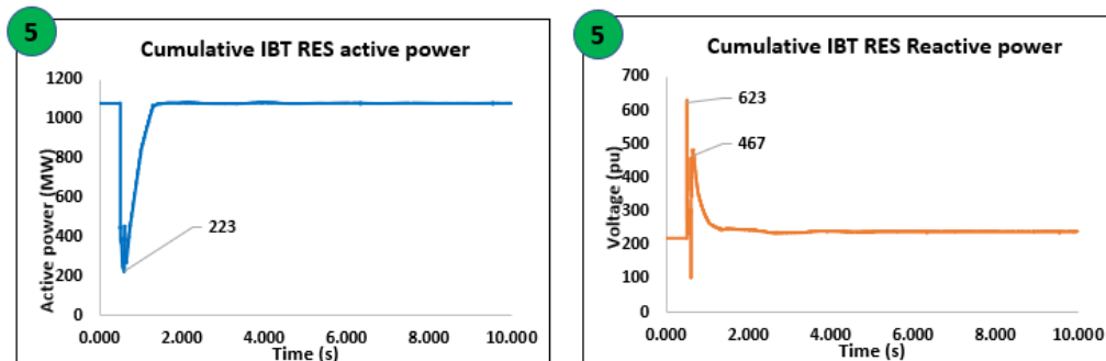
Figure 56 – IBT RES scenario cumulative active-power and reactive-power
