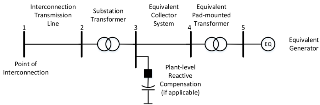
Figure 16 – Typical Single-Generator Equivalent Power Flow Representation [28]
