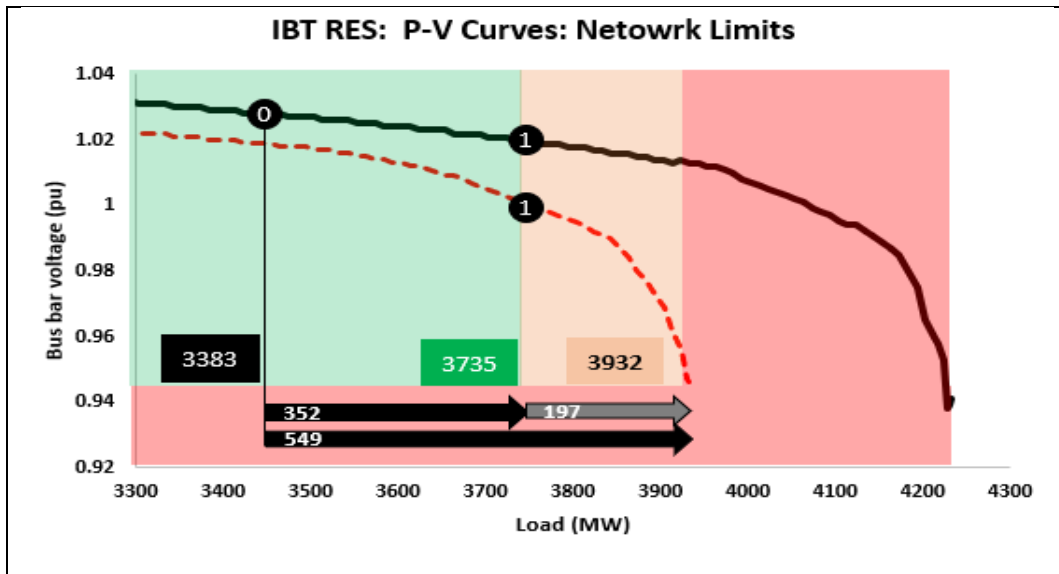
Figure 47 – IBT RES scenario: P-V steady-state analysis for Tx margin (still safe for limiting network contingency) and network limit (voltage collapse for worst network contingencies)
