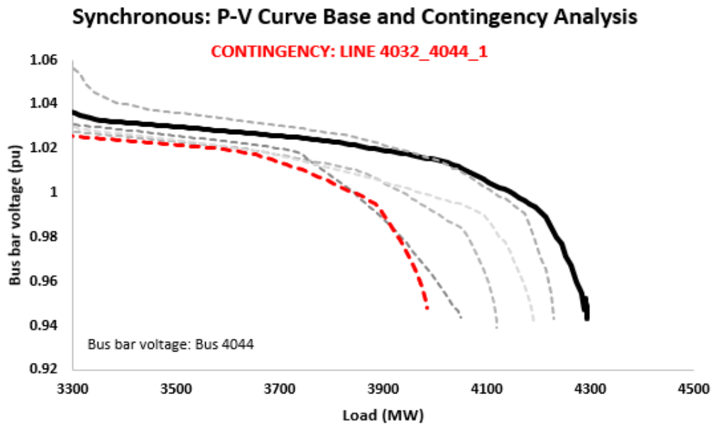
Figure 40 – Synchronous scenario: P-V steady-state analysis for base and contingencies
