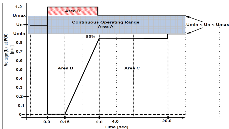
Figure 13 – RSA Renewable Grid Code Voltage Ride Through Capability requirement [37]
