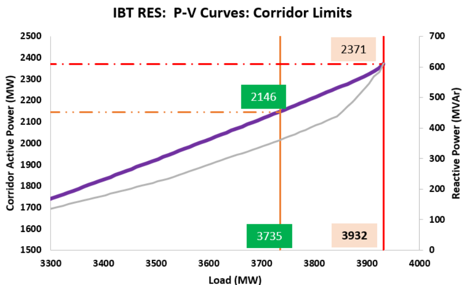
Figure 48 – IBT RES scenario: P-V steady-state analysis Tx-corridor margin and limit
