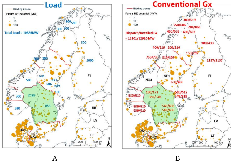
Figure 39 – Synchronous scenario: Load (MW) and generation (MW) location
