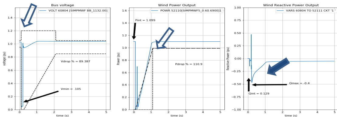
Figure 25 - IBT RES response for fault initial conditions
