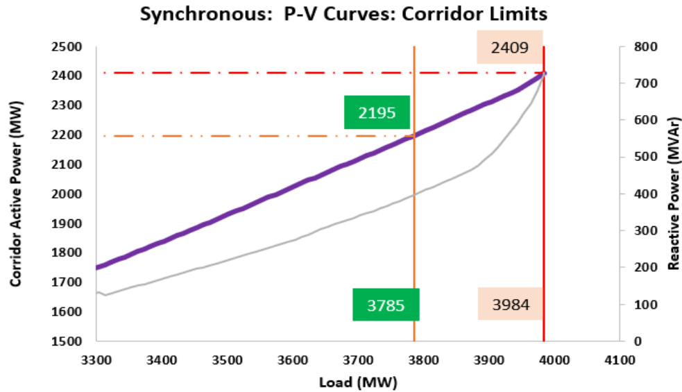
Figure 43 – Synchronous scenario: P-V steady-state analysis Tx-corridor margin and limit
