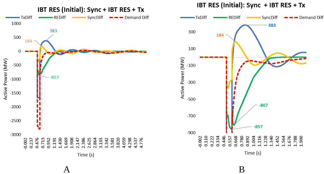
Figure 60 – IBT RES scenario: active-power response
