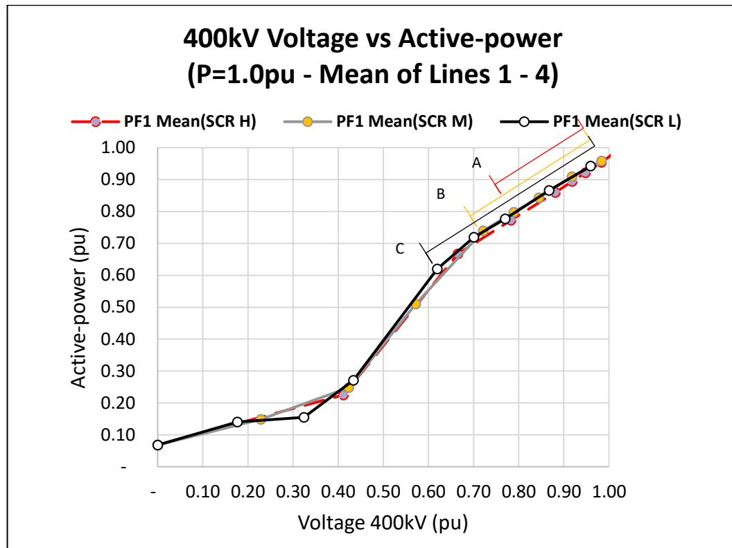
Figure 32 – Tx voltage vs active-power export reduction for the same pf with varying system strengths.
