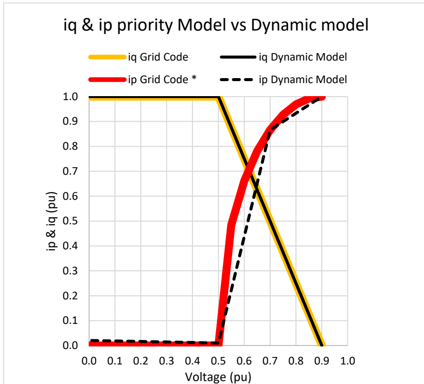
Figure 24 – iq and ip Grid Code requirement versus WECC dynamic model (assuming inverter initially exporting zero reactive current and exporting maximum active current)
