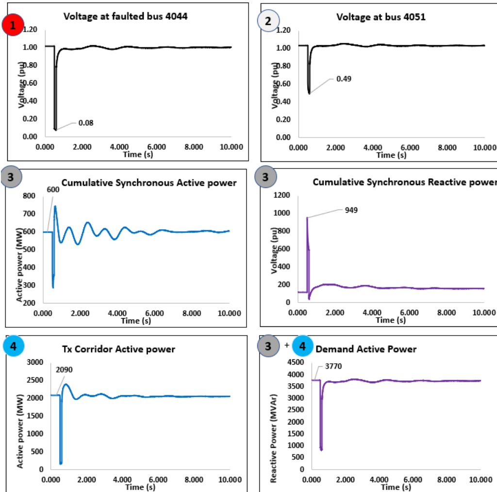
Figure 68 – IBT RES scenario: bus voltages, active-power and reactive-power
