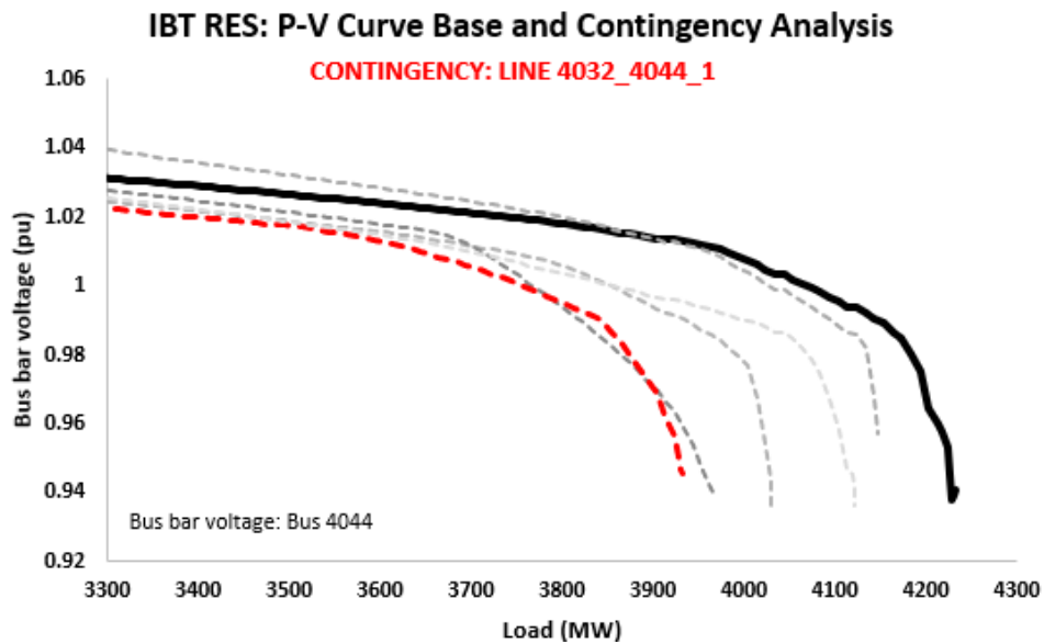
Figure 45 – IBT RES scenario: P-V steady-state analysis for base and contingencies
