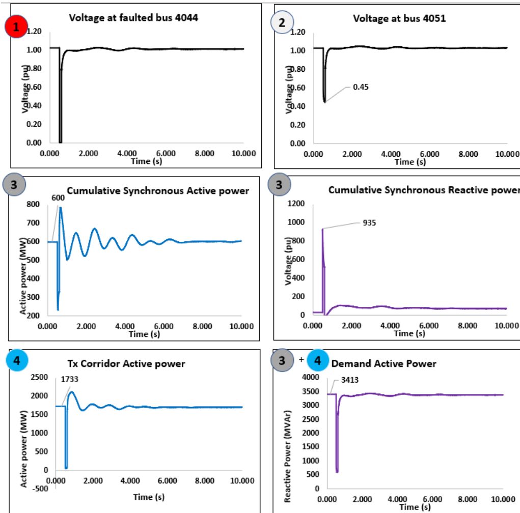
Figure 55 – IBT RES scenario
