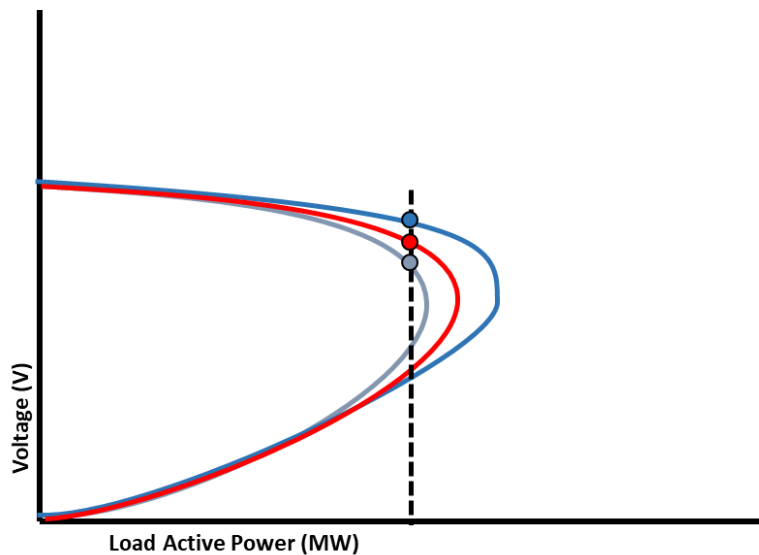
Figure 7 – Classical P-V curves including two contingencies
