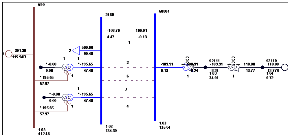
Figure 21 – PSSE Model
