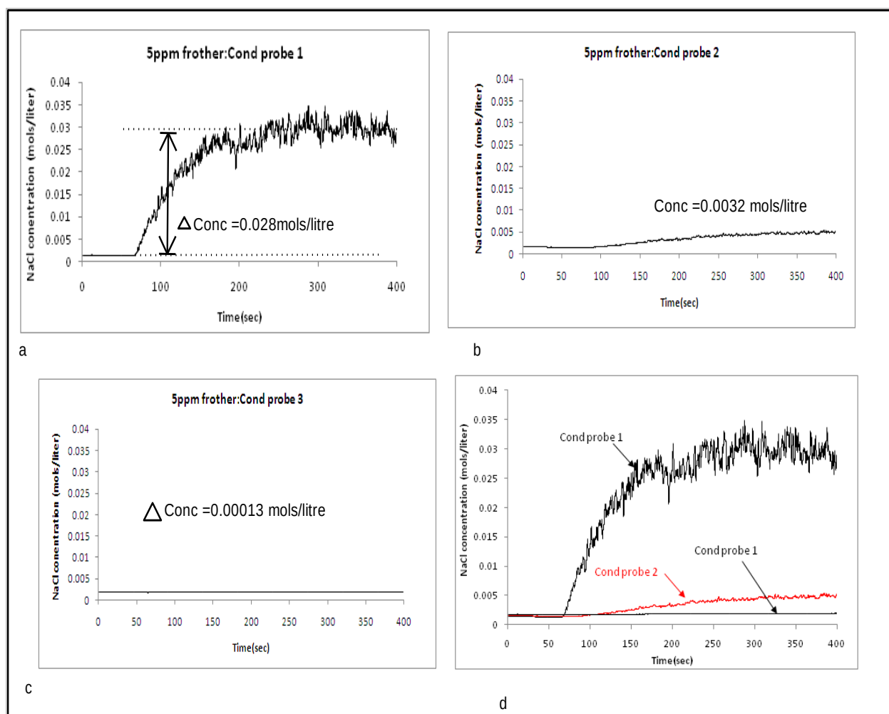
Figure B.2 Conductivity responses for the 50mm riser when 5ppm MIBC is added to the flotation cell
