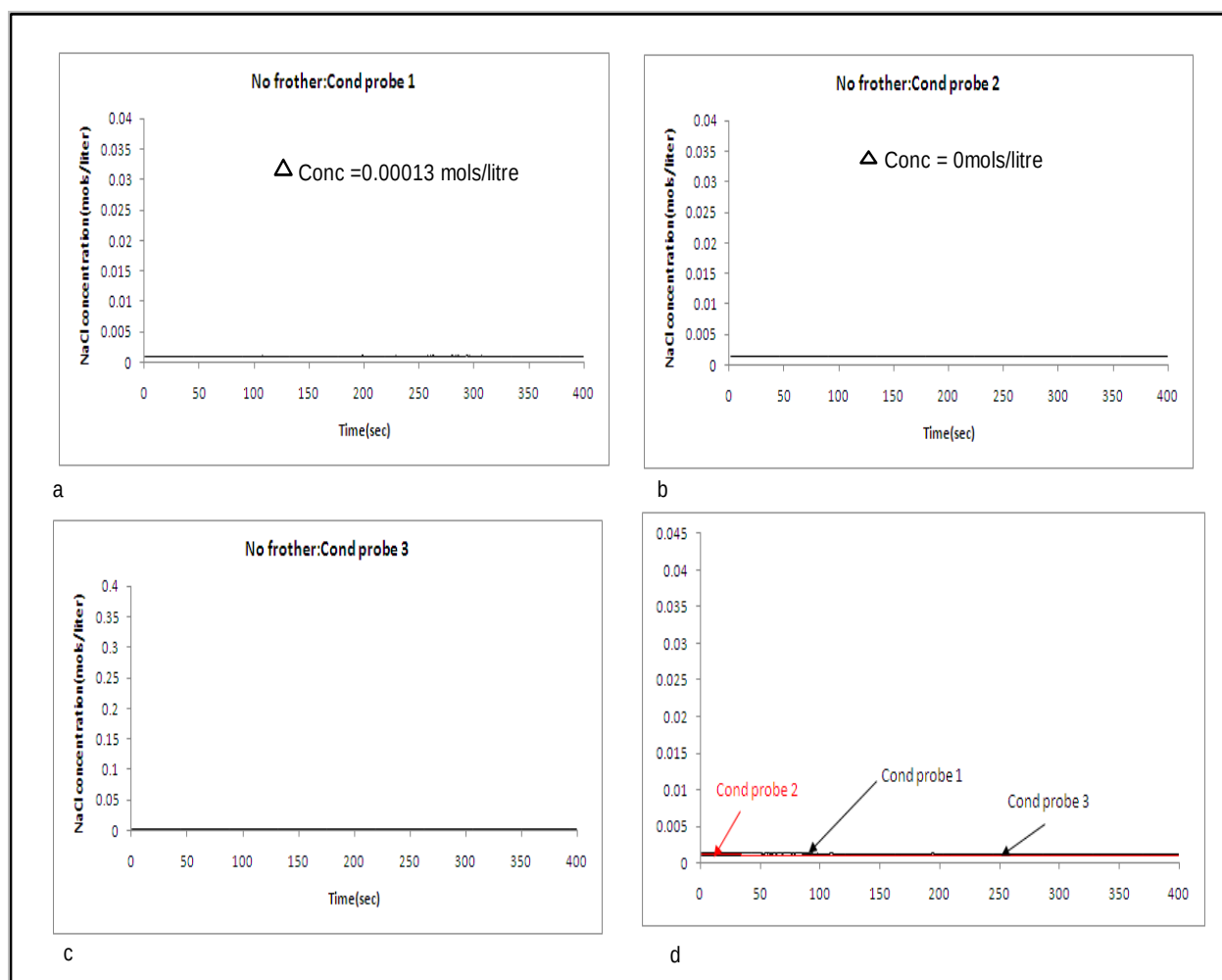
Figure B.5 Conductivity responses for the 20mm riser when No frother MIBC is added to the flotation cell
