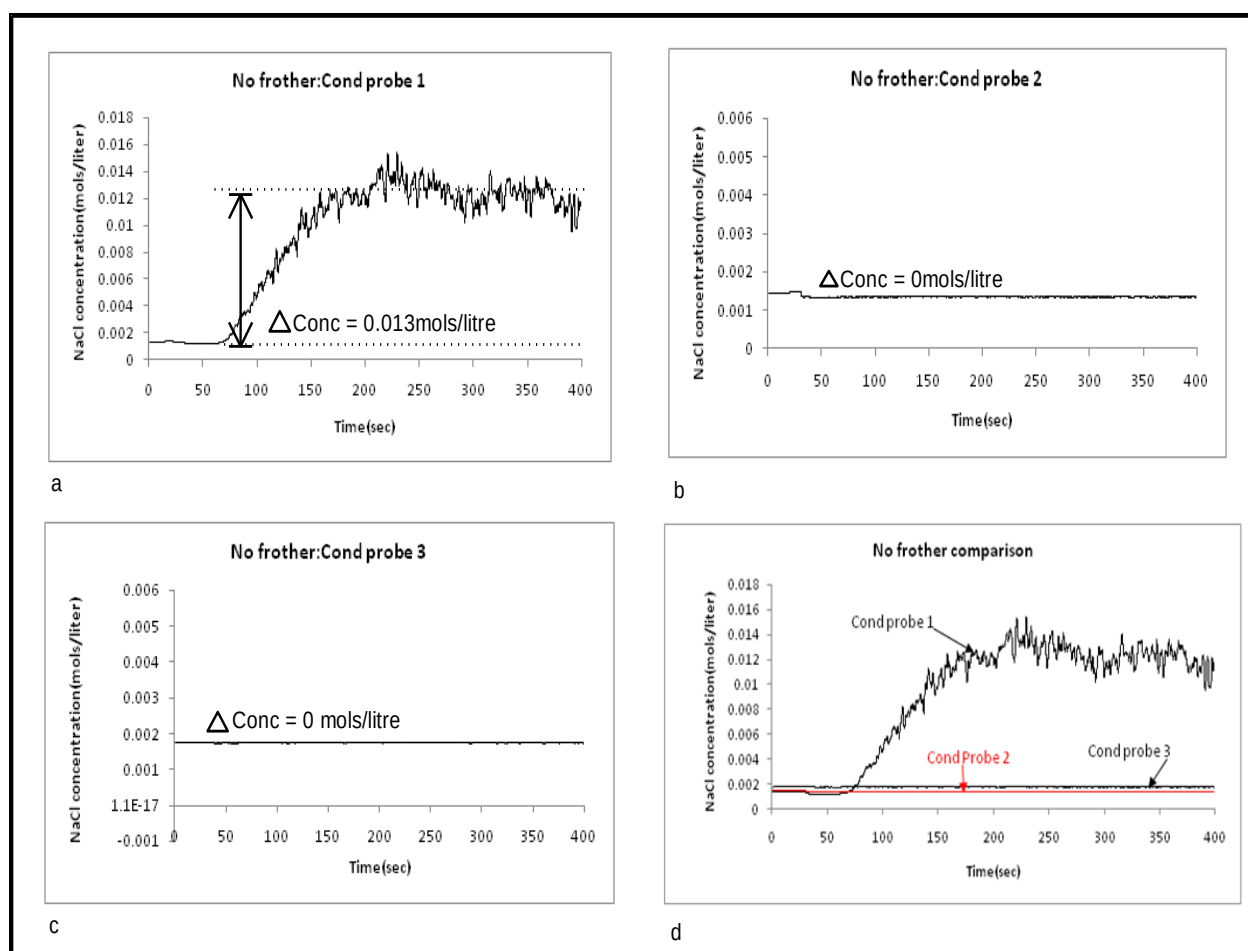
Figure B.1 Conductivity responses for the 50mm riser when no frother is added to the flotation cell
