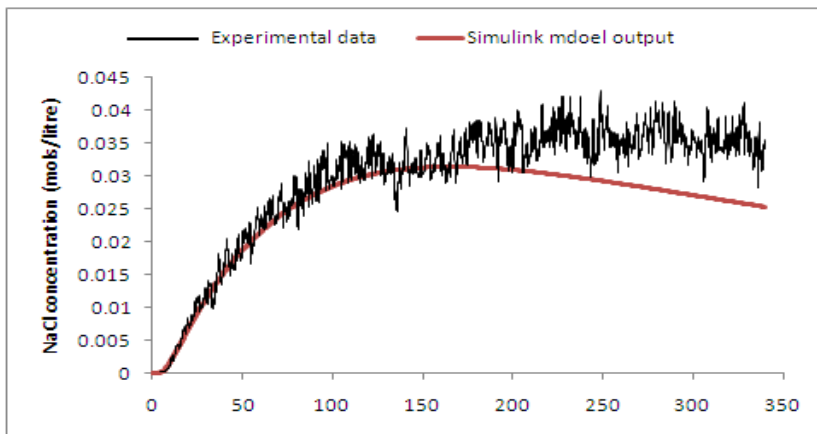
a) 5ppm MIBC 30mm riser
