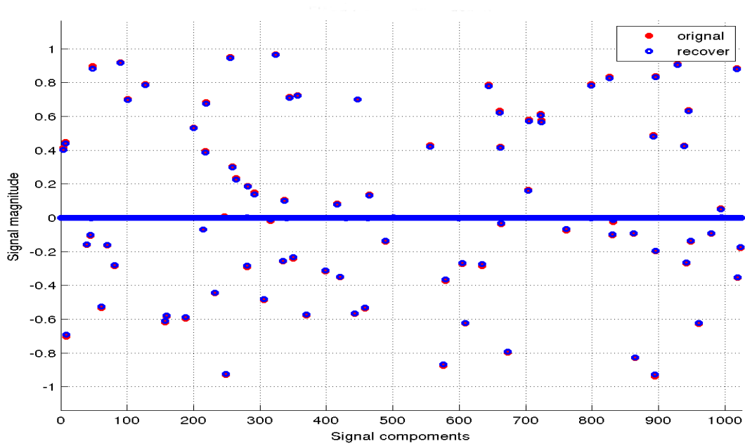
Figure 5.5: An example of signal reconstruction with fixed-point algorithm.
