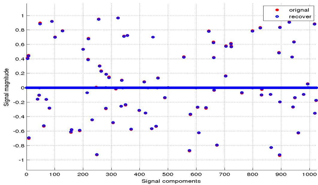
Figure 5.6: An example of signal reconstruction with interior point algorithm.
