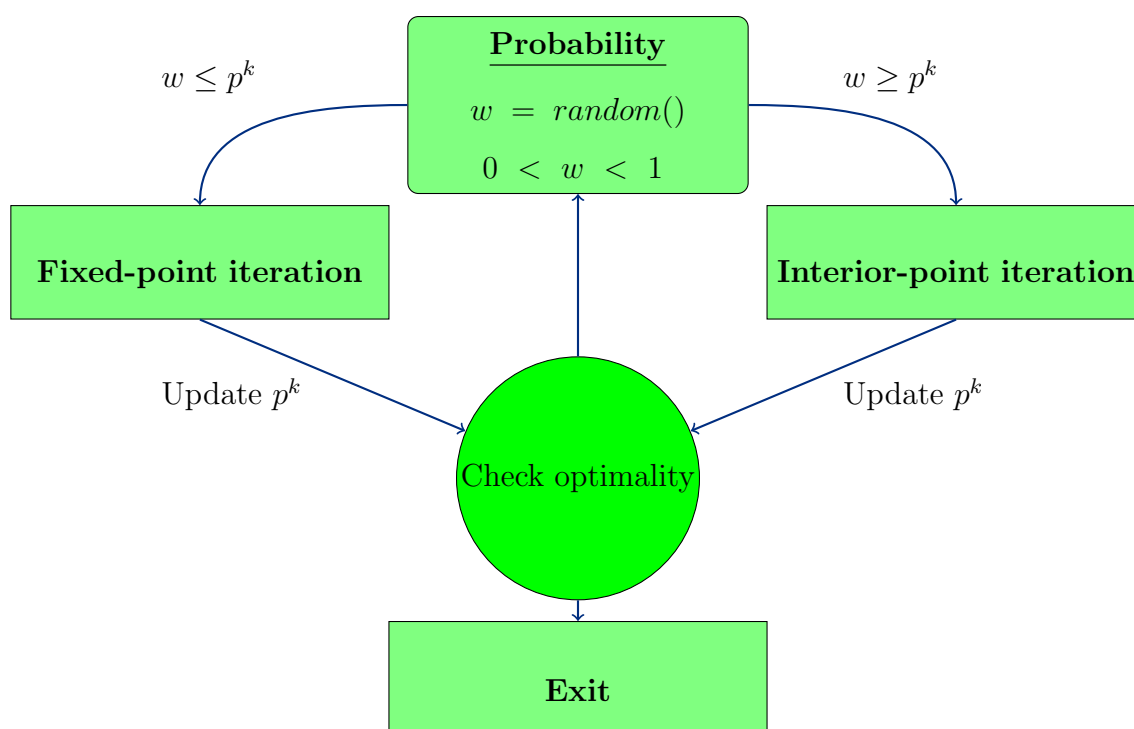
Figure 4.1: Schematic diagram of the probabilistic hybrid algorithm.
