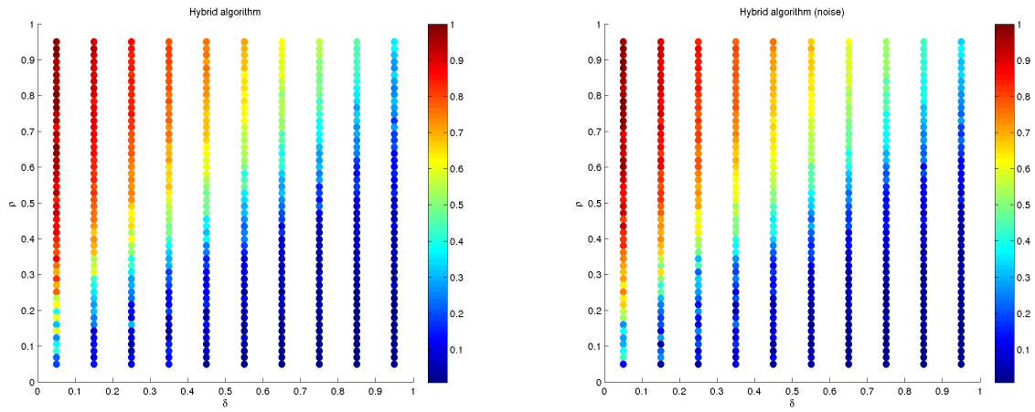
(a) Probabilistic hybrid algorithm noiseless measurements (b) Probabilistic hybrid algorithm noisy measurements
