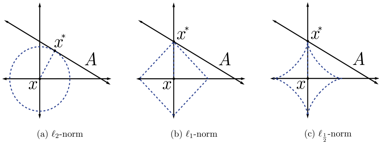
Figure 2.3: Best approximation of a point in \mathbb{R}^2 by a one-dimensional subspace using the \ell_p -norms for p = 2, 1 and the \ell_p quasi-norm with p = \frac{1}{2} .
