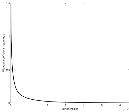
(c) Sorted magnitudes of Haar wavelets coefficients.
