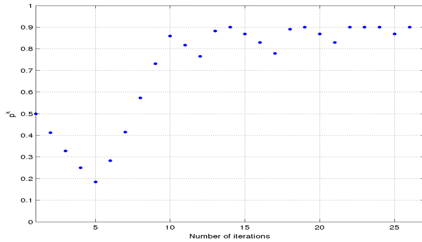
Figure 5.9: Probability profile of reconstruction for signal length n = 2^{10} .
