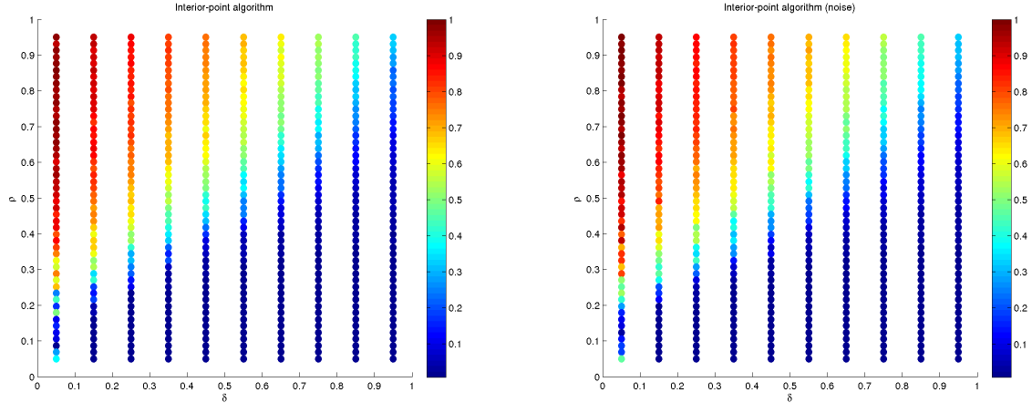
(a) Interior-point algorithm noiseless measurements (b) Interior-point algorithm noisy measurements
