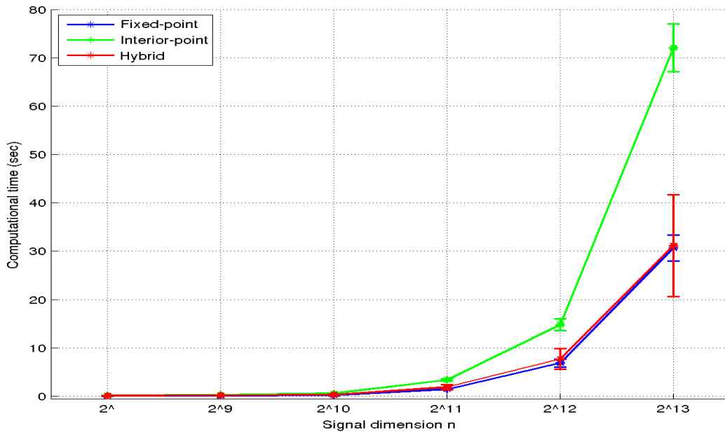
Figure 5.4: Speed comparison for different problem sizes
