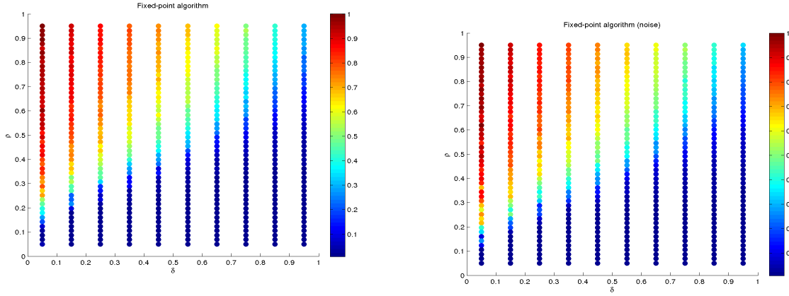
(a) Fixed-point algorithm noiseless measurements
