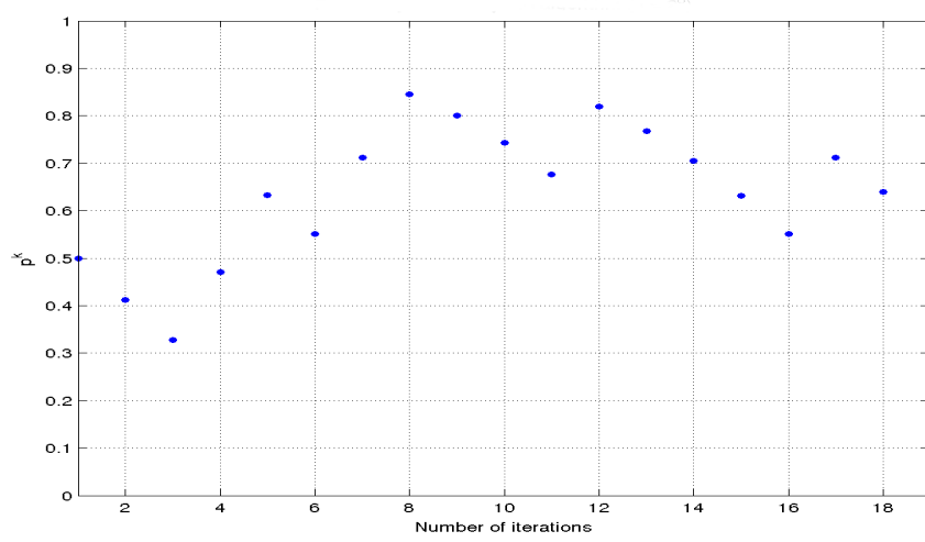
Figure 5.8: Probability profile of reconstruction for signal length n = 2^8 .
