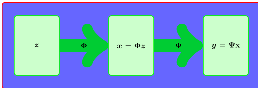
Figure 2.1: Compressive sensing measurement model.
