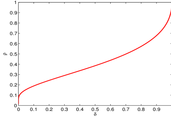
Figure 2.4: Phase transition diagram.
