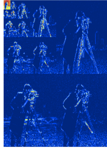
(b) Haar wavelets representation
