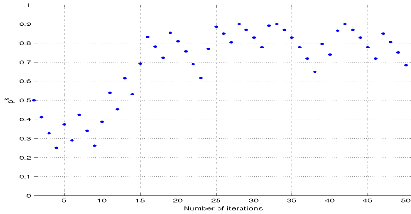
Figure 5.10: Probability profile of reconstruction for signal length n = 2^{13} .
