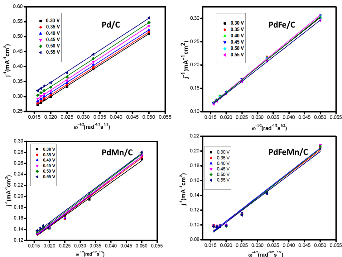
Figure 9.15: Koutecky-Levich Plots of ORR polarisation curves of electrocatalysts taken at varied potentials (0.3, 0.35, 0.40, 0.45, 0.50, 0.55 V vs RHE).
