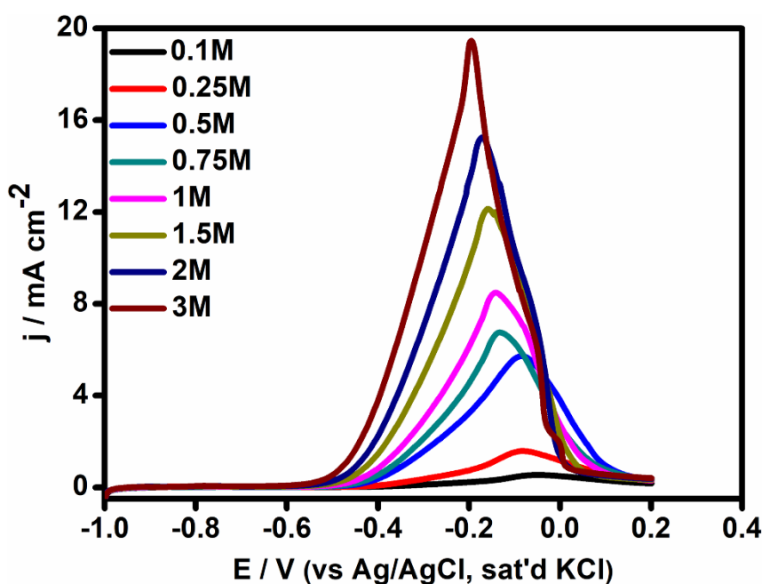
Figure 9.10: The LSV of the EGOR on the PdFeMn/C electrocatalysts in 0.5 M EG solution containing KOH solution of various concentrations. Scan rate: 1.0 mV / s.
