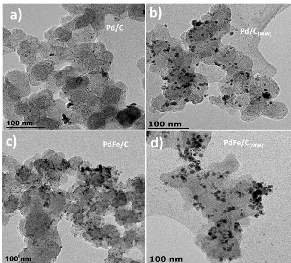
Figure 4.3: TEM images of Pd-based catalysts obtained from the conventional \text{NaBH}_4 method: a) Pd/C and c) PdFe/C; and microwave-assisted method: b) Pd/C and d) PdFe/C.
