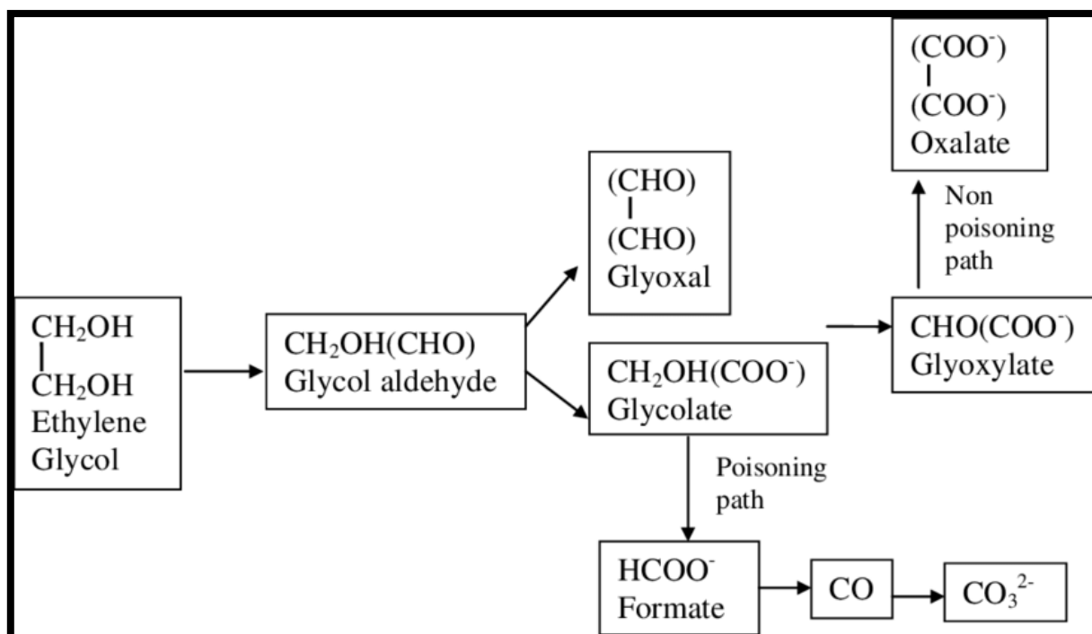
Scheme 9.1 Schematic diagram for the illustration of reaction pathways for EG electro-oxidation in an alkaline medium [35]
