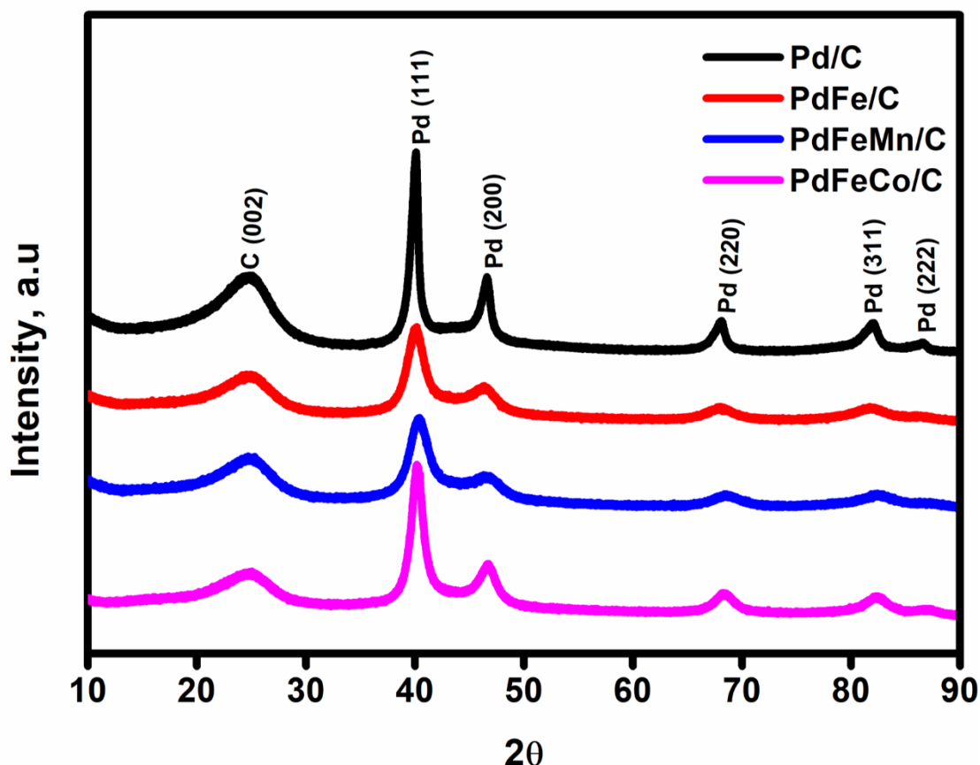
Figure 8.1: XRD patterns of electrocatalysts.
