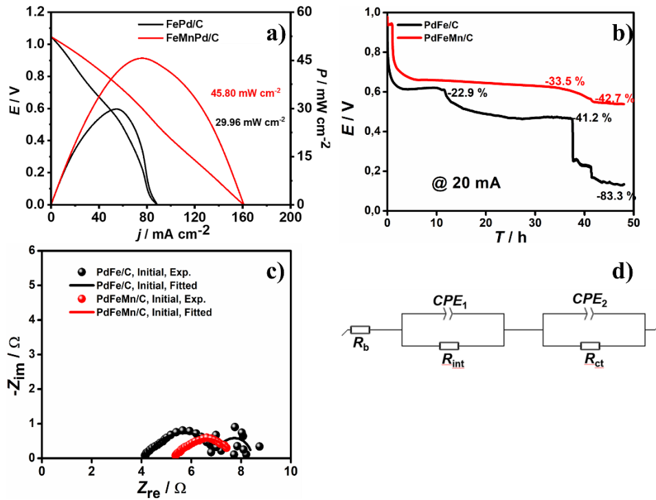
Figure 8.18: (a) Voltage (I-V) and power density curves for PdFe/C and PdFeMn/C, (b) galvanostatic discharge curves, (c) Nyquist plots, and (d) Voigt EEC for PdFe/C and PdFeMn/C supplied with 4 M KOH/EG solution.
