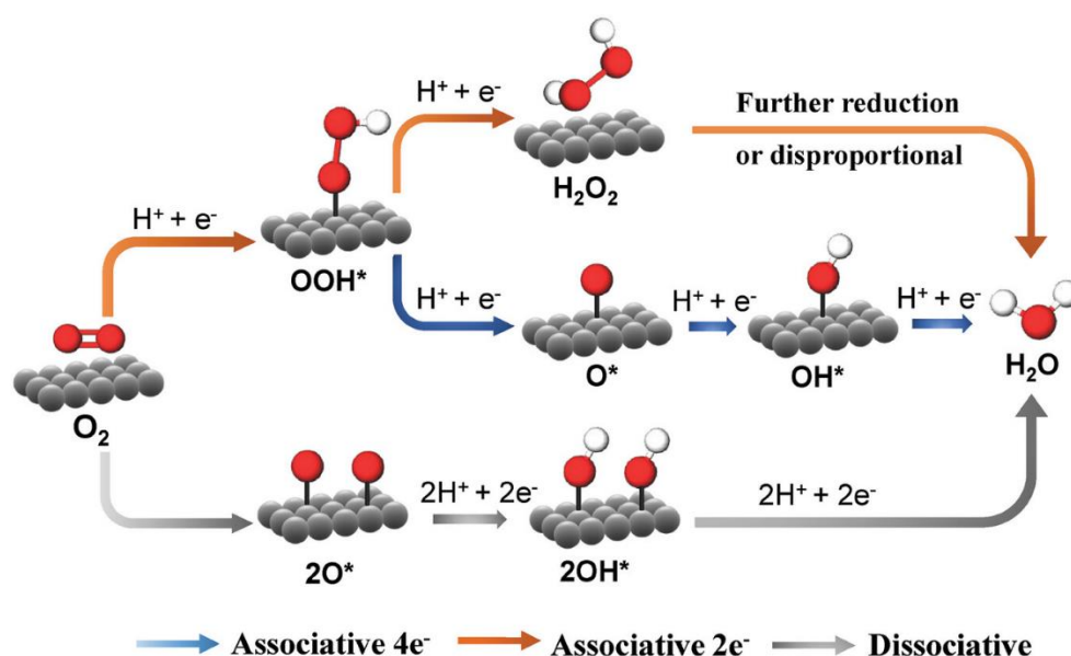
Scheme 2.2: Schematic diagram of the two and four ORR pathways in neutral environment [108].
