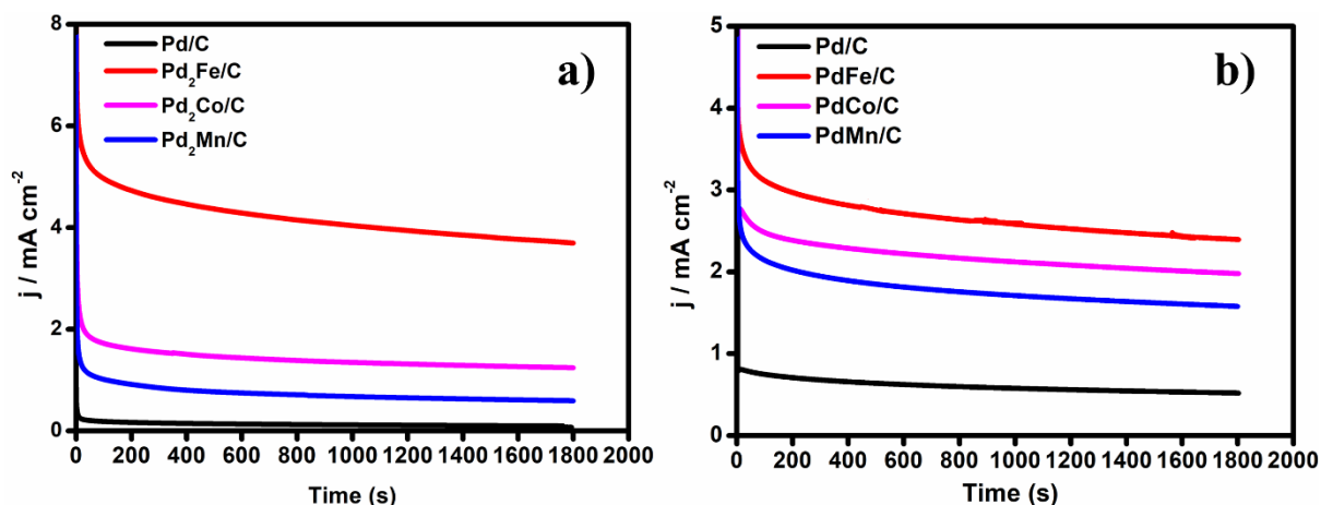
Figure 6.6: The CA curves of electrocatalysts (at varied atomic ratios of a) Pd 2 M/C and b) PdM/C) in 0.5 M KOH/ EG solution under the influence of N 2 gas at 0.2 V.
