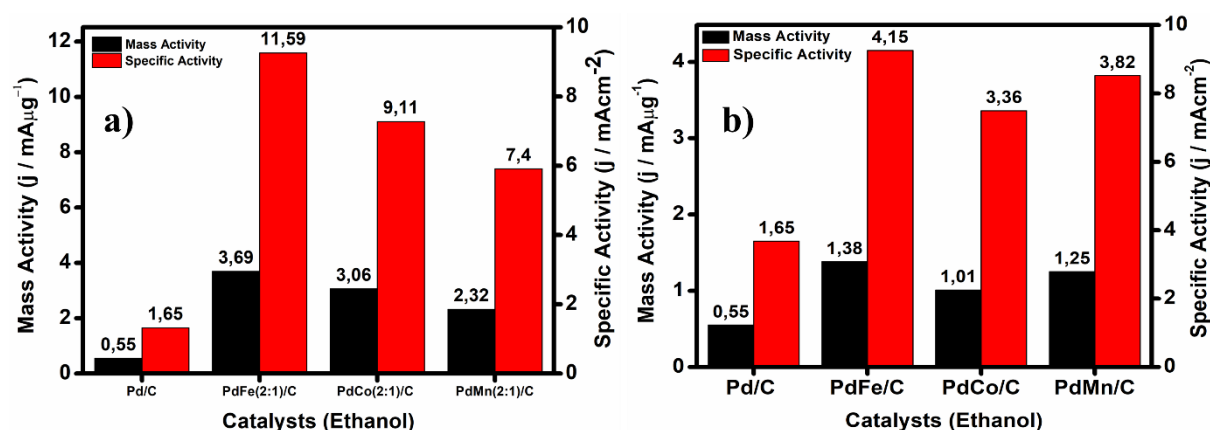
Figure 5.5: Comparison of mass and specific activities of Pd, PdFe/C, PdMn/C, and PdCo/C (Pd 2 M/C and PdM/C) in KOH + EtOH both in (0.5 M), N 2 gas at a scan rate = 50 mV / s.
