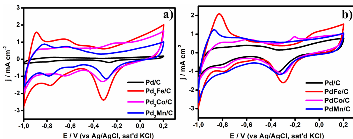
Figure 5.3: Cyclic voltammetry of Pd, PdFe/C, PdMn/C, and PdCo/C (atomic ratio of Pd 2 M/C and PdM/C in (0.5 M) KOH solution, N 2 gas - sweep rate = 50 mV / s.
