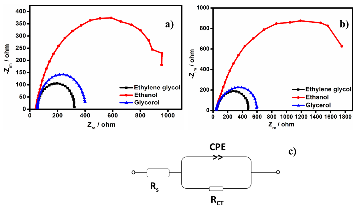
Figure 8.16: a) Nyquist plot of a) PdFeMn/C and b) PdFeCo/C electrocatalysts using the same parameters as CV and c) insert is the EEC (equivalent external circuit) used to fit the spectra.
