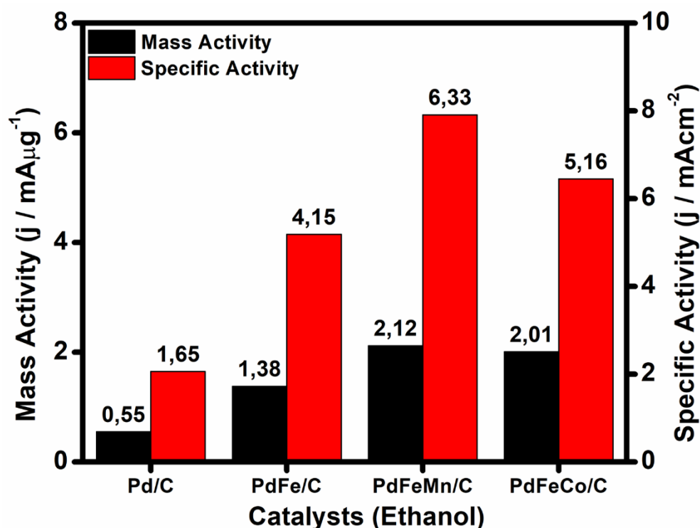
Figure 8.10: Comparison of various activities to study the electrocatalysts in 0.5M KOH/ EtOH solution, bubbled with N 2 gas at a sweep rate = 50 mV / s.
