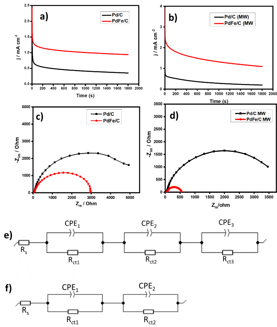
Figure 4.9: Chronoamperometric measurements of the Pd-based nano-electrocatalysts from conventional \text{NaBH}_4 method: a) Pd/C and PdFe/C, and microwave-assisted synthesis b) Pd/C (MW) and PdFe/C (MW) in 0.5 M KOH/0.5 M glycerol solution under \text{N}_2 atmosphere at -0.2 V and their corresponding Nyquist plots curves of the Pd-based nano-electrocatalysts obtained from the c) \text{NaBH}_4 method and d) microwave-assisted method, respectively. All data were obtained at a fixed potential of -0.2 V in glycerol electrooxidation. The electrical equivalent circuit (EEC) was used to fit e) monometallic while f) bimetallic.
