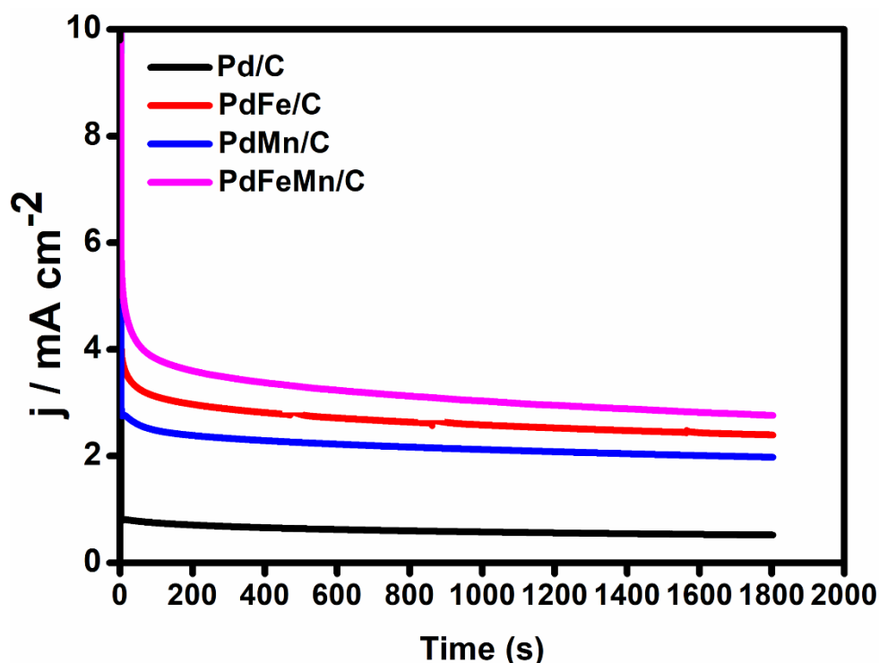
Figure 9.11: Chronoamperometric curves of Pd/C, PdFe/C, PdMn/C and PdFeMn/C in 0.5 M KOH / EG solutions at -0.2 V.
