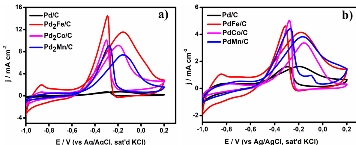
Figure 5.4: CV of Pd, PdFe/C, PdMn/C, and PdCo/C (molar ratio: Pd 2 M/C and PdM/C) in (0.5 M KOH solution + 0.5 M) EtOH, N 2 atmosphere using sweep rate of 50 mV / s.
