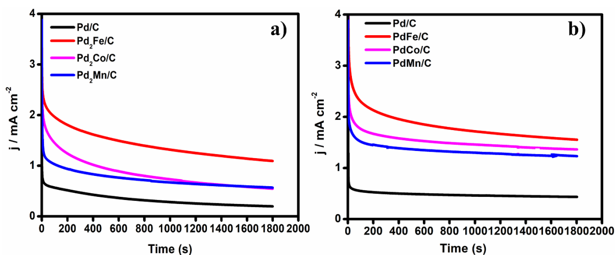
Figure 7.6: The CA curves (a) Pd 2 M/C and (b) PdM/C in KOH/ Gly (0.5 M) solution under N 2 atmosphere at 0.2 V.
