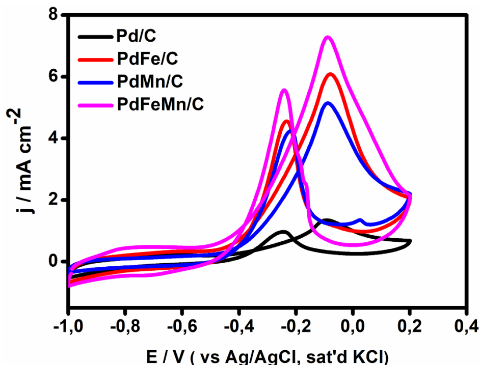
Figure 9.5: CV for EGOR on the electrocatalysts in 0.5 M KOH / EG, scan rate: 50 mV / s.
