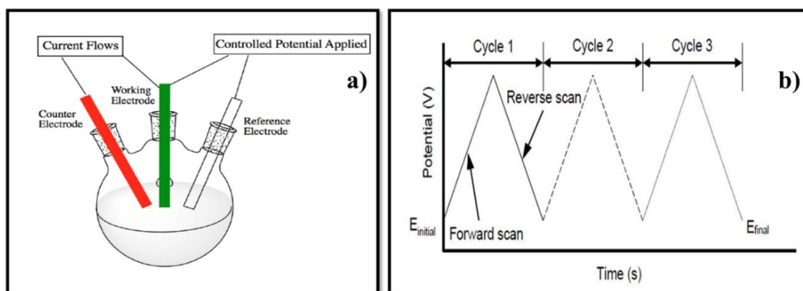
Figure 2.7: a) Typical three-electrode system [91] and b) The excitation signal of CV via a triangular potential waveform with switching potentials at (0.8, -0.2 V) vs SCE [92]
