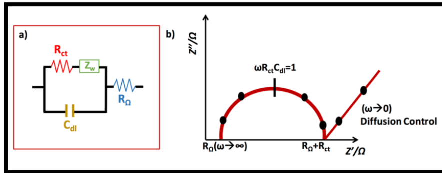
Figure 2.12: a). The Randles equivalent circuit and b). Nyquist plot obtained from the Randles circuit [101]
