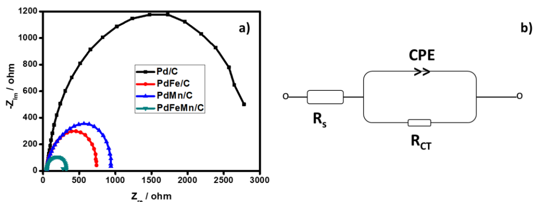
Figure 9.12: (a) Nyquist curves of electrocatalysts at -0.2 V, b) the EEC used in fitting the spectra.
