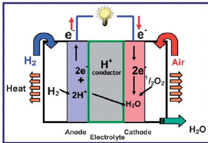
Figure 2.5: Operating principles of Polymer exchange membrane Fuel Cells (PEMFCs) [20]
