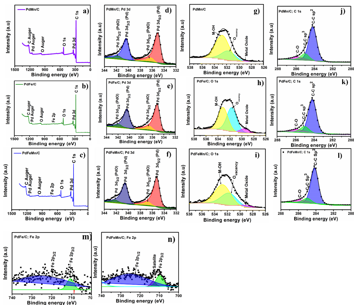
Figure 9.2: XPS spectra of a-c) with the wide survey spectra, deconvoluted elemental scans d-f) Pd 3d, g-i) O 1s, j-l) C 1s and m,n) Fe 2p of PdFeC, PdMn/C and PdFeMn/C electrocatalysts.
