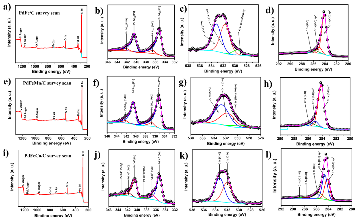
Figure 8.2 XPS spectra of (a, e, i) with the wide survey spectra, deconvoluted elemental scans b, f, j) Pd 3d, c, g, k) O 1s and d, h, l) C 1s) of PdFeC, PdFeMn/C and PdFeCo/C electrocatalysts.
