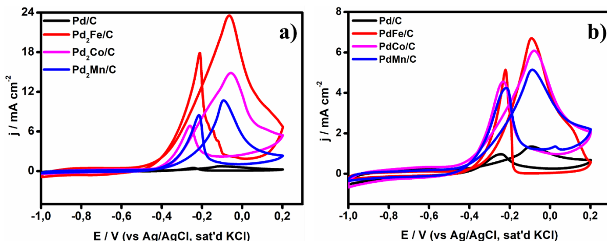
Figure 6.4: The CV curves of electrocatalyst at different atomic ratio of a) Pd 2 M/C and b) PdM/C) immersed in 0.5 M KOH/EG solution under N 2 gas at a scan rate = 50 mV / s.
