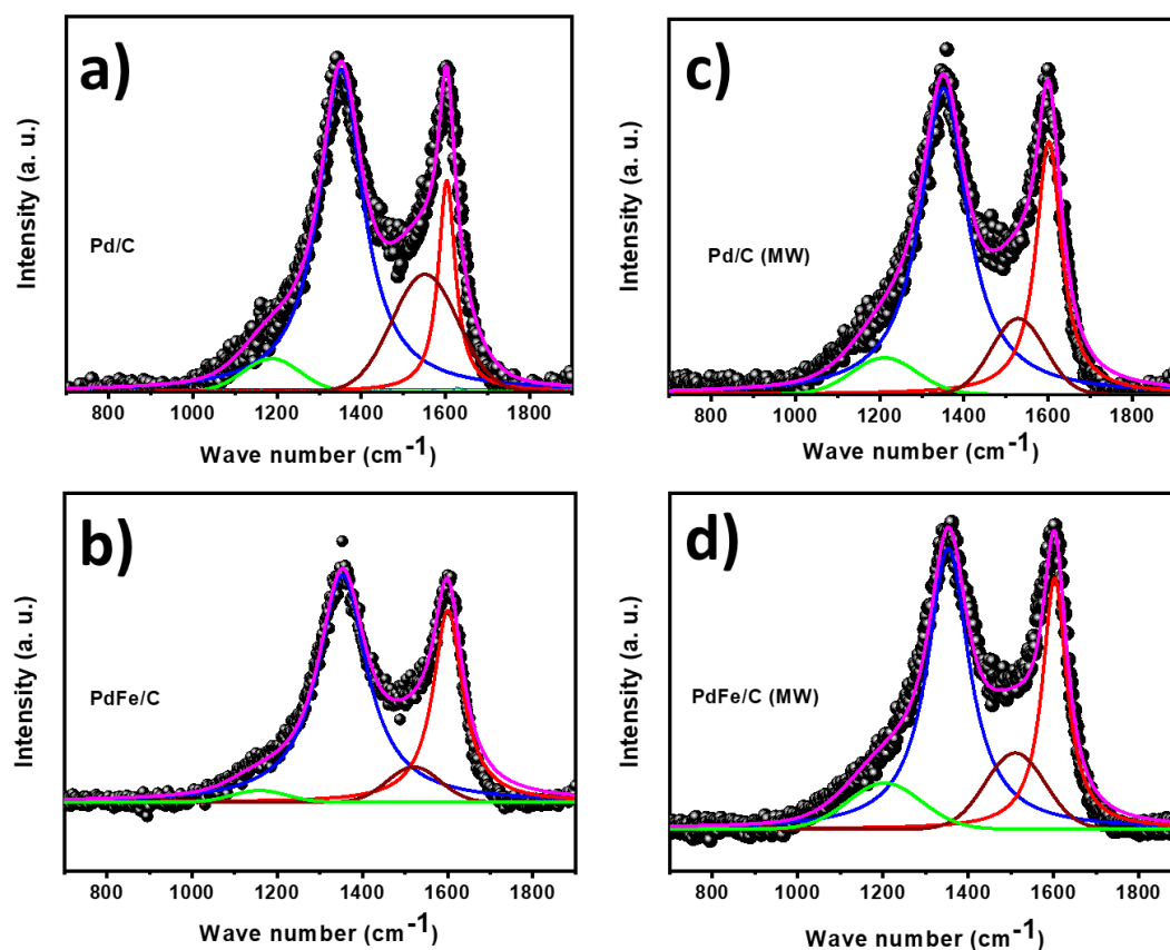
Figure 4.6: Raman spectra of NaBH 4 a) Pd/C, and b) PdFe/C and MW c) Pd/C, and d) PdFe/C.
