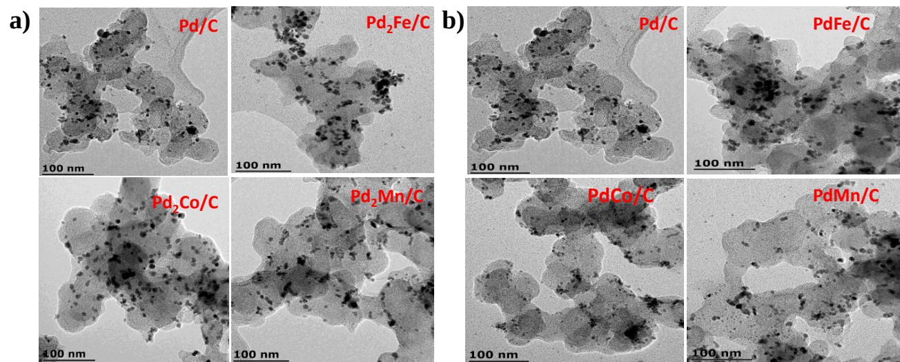
Figure 7.2: TEM micrographs of a) Pd 2 M/C and b) PdM/C ratios of electrocatalyst.
