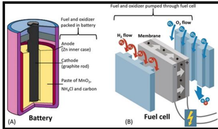
Figure 2.3: A schematic diagram displaying the A, Batteries and B Fuel cells. The picture shows how the fuel cells are supplied with fuel. [105]
