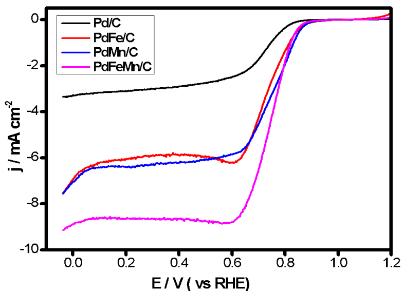
Figure 9.14: The ORR polarisation curves compare the electrocatalysts measured at 1600 rpm.
