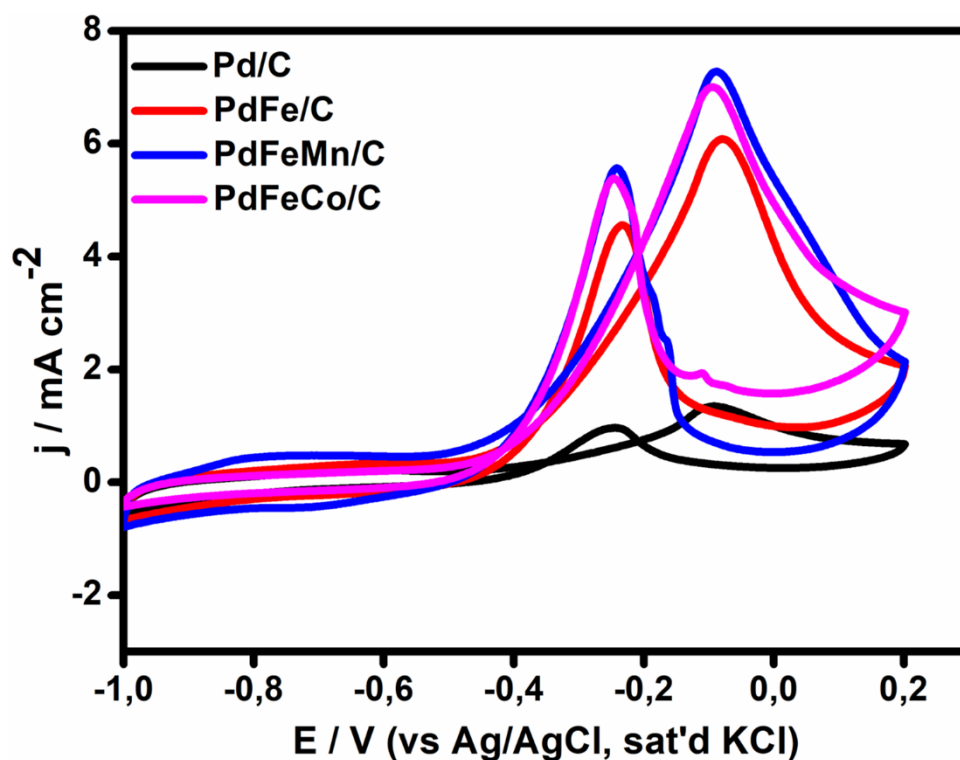
Figure 8.6: The CV of Pd/C, PdFe/C, PdFeMn/C, and PdFeCo/C for EGOR was reached at 50 mV / s in a KOH/Gly solution containing 0.5 M.
