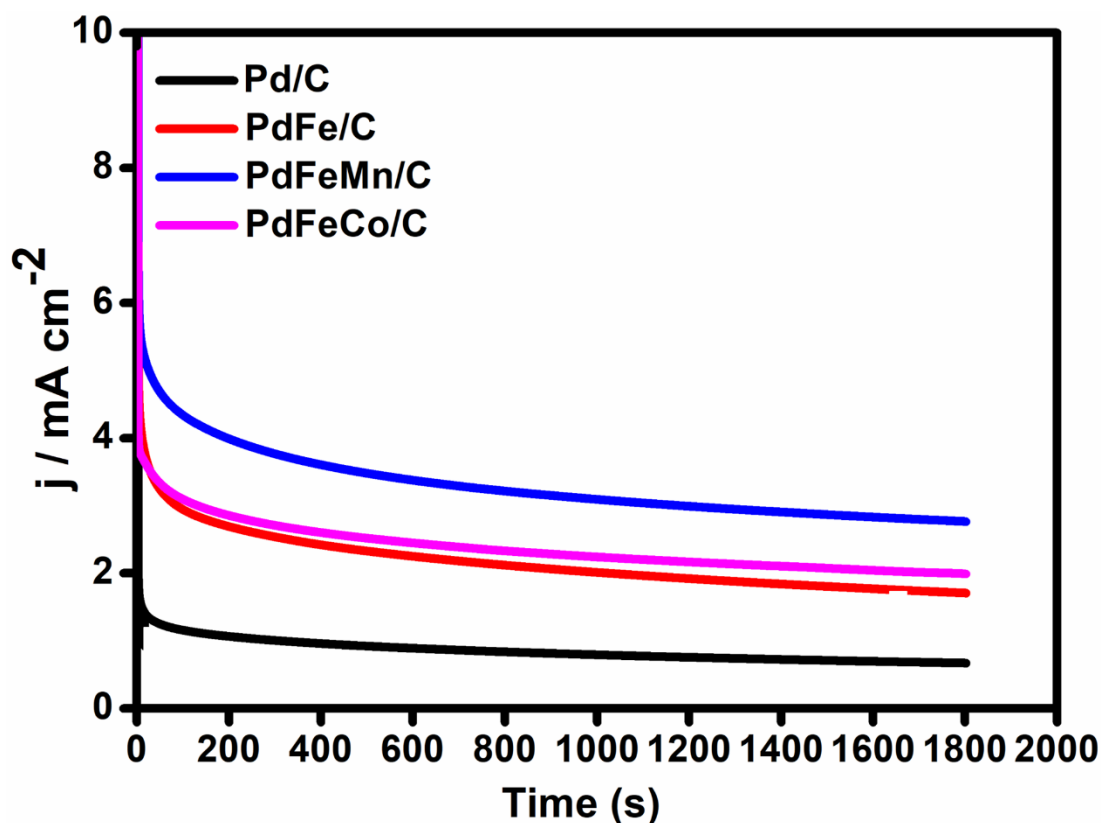
Figure 8.11: Current-times curve of examined electrocatalysts with a -0.2 V, containing 0.5 M KOH / 0.5 M ethanol.
