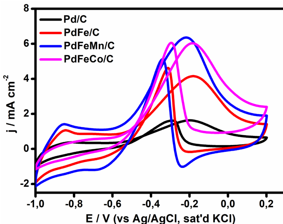
Figure 8.9: Cyclic voltammetry of electrocatalysts for EOR, reached = 50 mV / s, containing the solution of 0.5 M KOH / EtOH.
