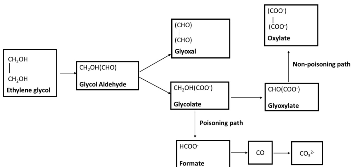
Scheme 2.1: Schematic diagram representing the ethylene glycol pathways indicating the poisoning and non-poisoning paths [72]
