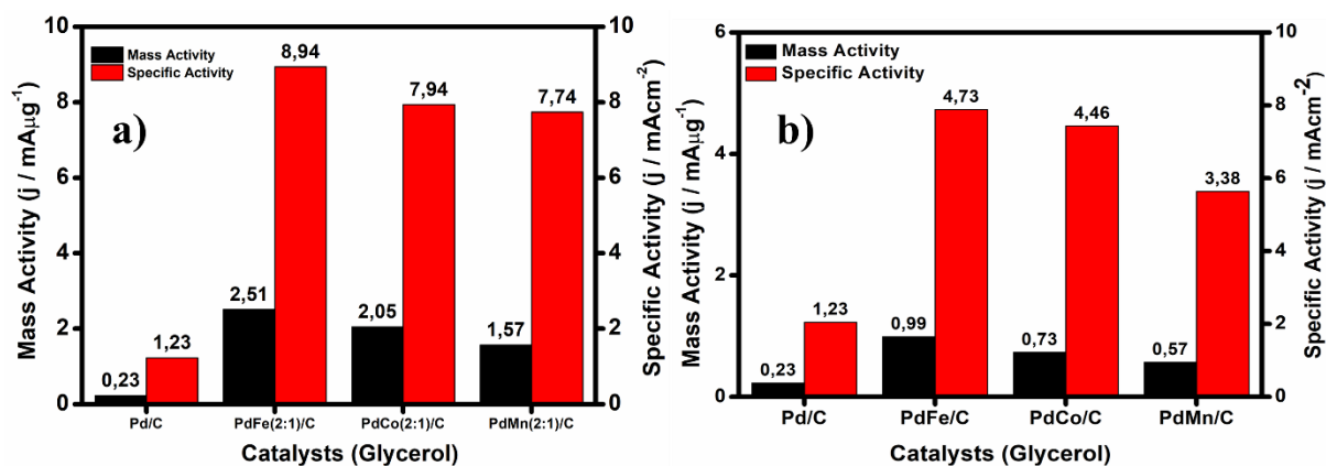
Figure 7.5: Comparison of mass and specific activities of (a) Pd 2 M/C and (b) PdM/C in 0.5 M KOH solution / Gly, N 2 gas at a sweep rate of 50 mV / s.
