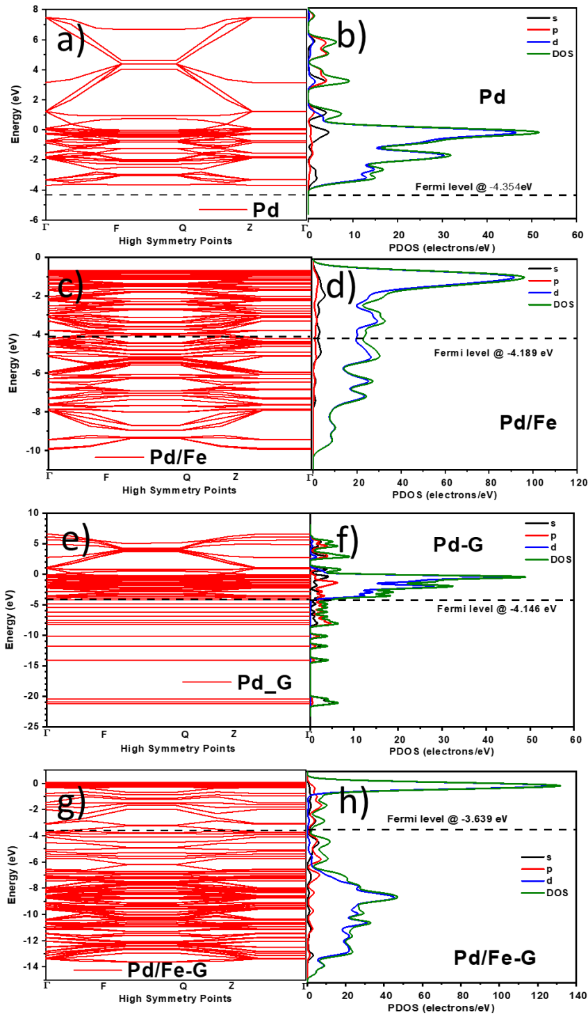
Figure 4.2: a,c,e,g) Band structure and b,d,f,h) partial density of states (PDOS) of the a,b,e,f) Pd and c,d,g,h) PdFe. The dotted lines represent the Fermi energy level, the PDOS shows that the electrons in the conduction band are mainly from the 3d orbital of the 3d orbital of the Pd and Fe.
