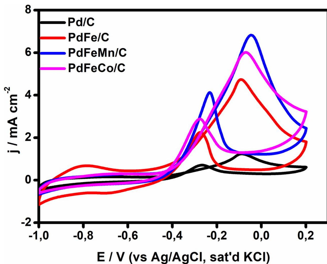
Figure 8.12: Cyclic voltammetry of electrocatalysts for GOR with a scan rate of 50 mV / s, 0.5 M KOH / 0.5 M Gly.
