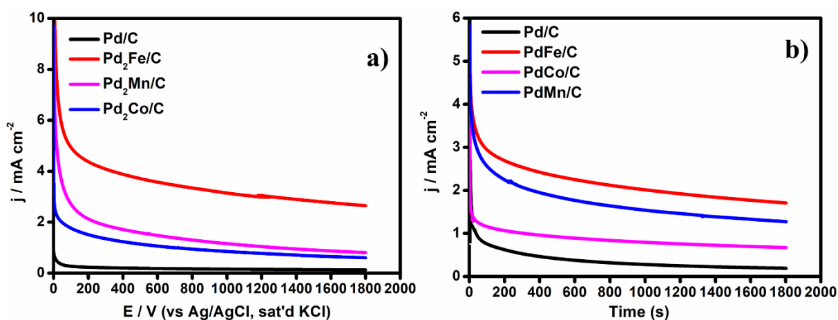
Figure 5.6: Chronoamperometry curves for of Pd, PdFe/C, PdMn/C, and PdCo/C (a) Pd 2 M/C and b) PdM/C) in (0.5 M - KOH solution, ethanol) bubbled with N 2 atmosphere at -0.2 V.
