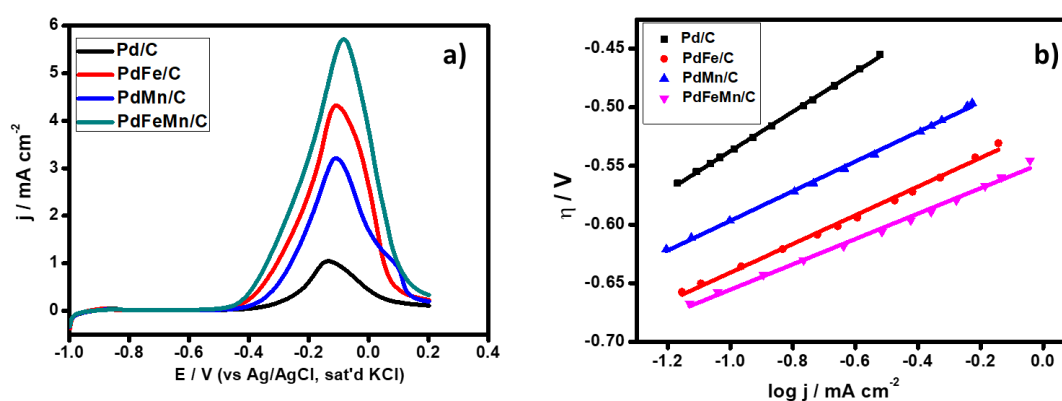
Figure 9.7: a) The LSV and (b) Tafel plots towards EGOR on the Pd/C, PdFe/C, PdMn/C and PdFeMn/C, EG, Scan rate of 1.0 mV / s.
