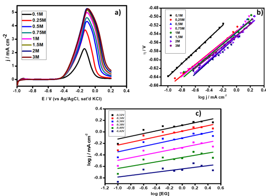
Figure 9.9: (a) LSV, (b) Tafel plot and (c) The log-log plot of current density vs EG concentration obtained for PdFeMn/C in 0.5 M KOH solution containing different EG concentration at scan rate: 1.0 \text{ mV / s} .
