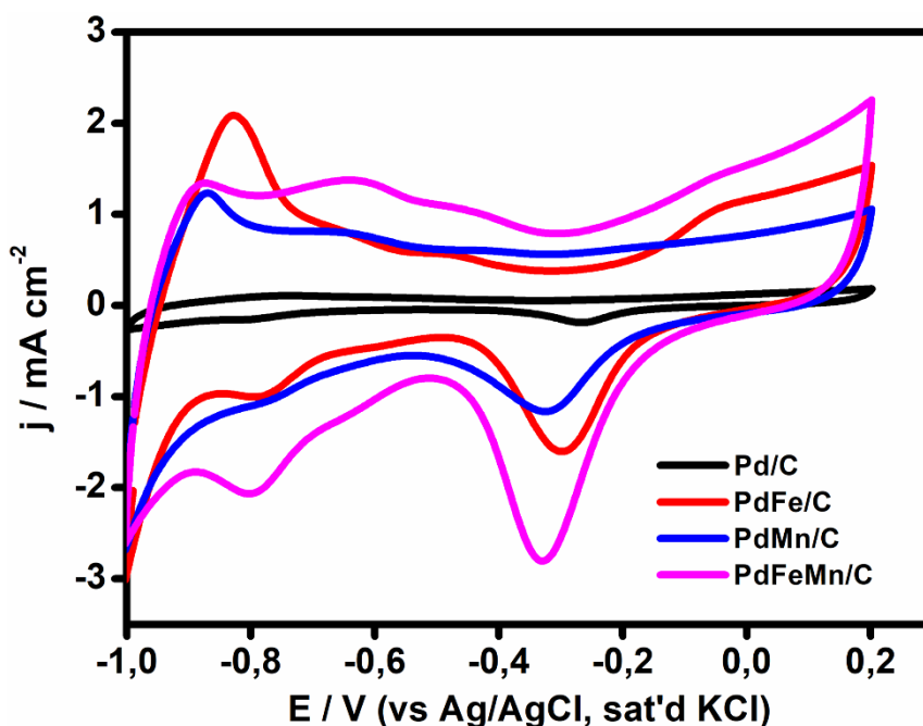
Figure 9.4: CV curves of catalysts in KOH (0.5 M), with 50 mV / s scan rate.
