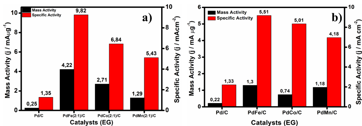
Figure 6.5: Comparison of mass and specific activities of Pd, PdFe/C, PdMn/C and PdCo/C (atomic ratio of a) Pd 2 M/C and b) PdM/C) in 0.5 M KOH solution + 0.5 M EG N 2 atmosphere at a sweep rate of 50 mV / s.
