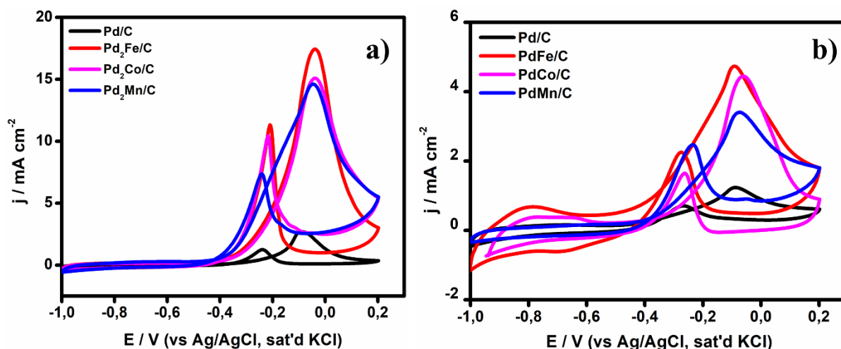
Figure 7.4: CV curves of Pd/C, PdFe/C, PdMn/C and PdCo/C (a) Pd 2 M/C and b) PdM/C) in 0.5 M KOH/ 0.5 M Gly mixture under N 2 gas at a scan rate = 50 mV / s.
