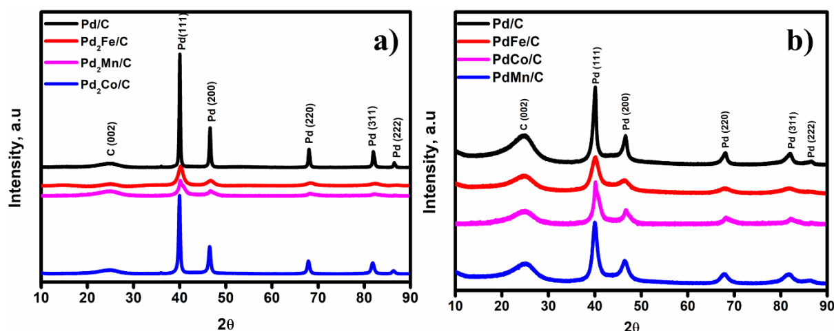
Figure 5.1: XRDs patterns of bimetallic electrocatalysts (at varied Pd 2 M/C and PdM/C).
