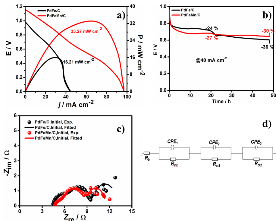
Figure 8.17: (a) Voltage (i-v) and power density curves, (b) galvanostatic discharge curve, (c) Nyquist plots and (d) Voigt EEC model for PdFe/C and PdFeMn/C fed with 4.0 M KOH/4.0 M Ethanol solution.
