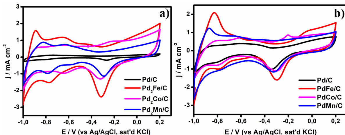
Figure 7.3. Cyclic voltammetry of electrocatalysts in 0.5 M KOH solution under N 2 gas at a scan rate of 50 mV / s.
