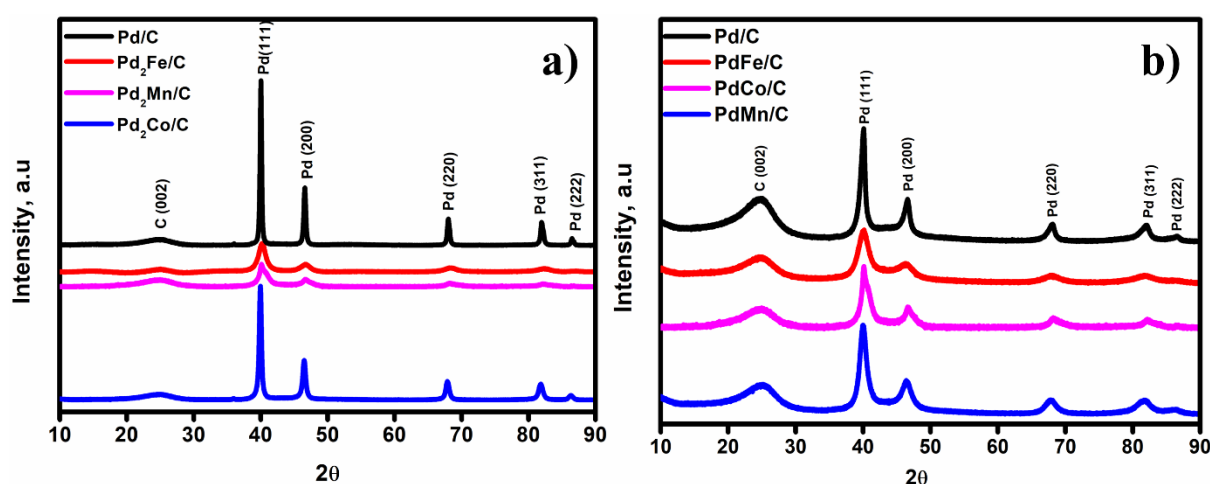
Figure 7.1. XRD diffractograms of (a) Pd 2 M/C and (b) PdM/C electrocatalysts.
