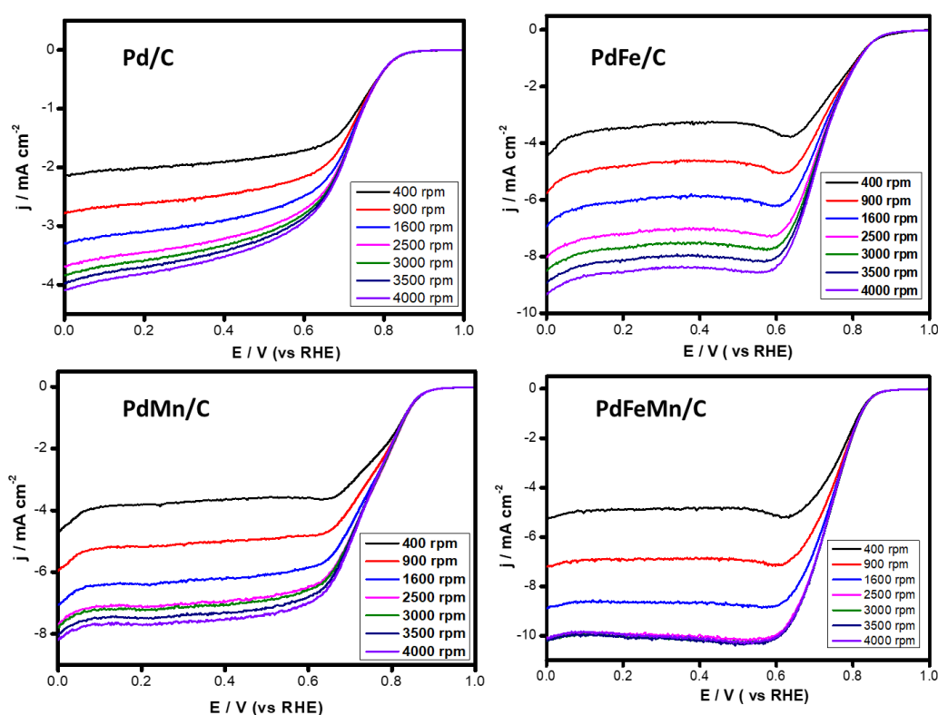
Figure 9.13: ORR polarisation curves of Pd/C, PdFe/C, PdMn/C and PdFeMn/C electrocatalysts in 0.1 M KOH electrolyte purged with O 2 at the scan rate 10 mV / s with rotating speeds from 400 to 4000 rpm.
