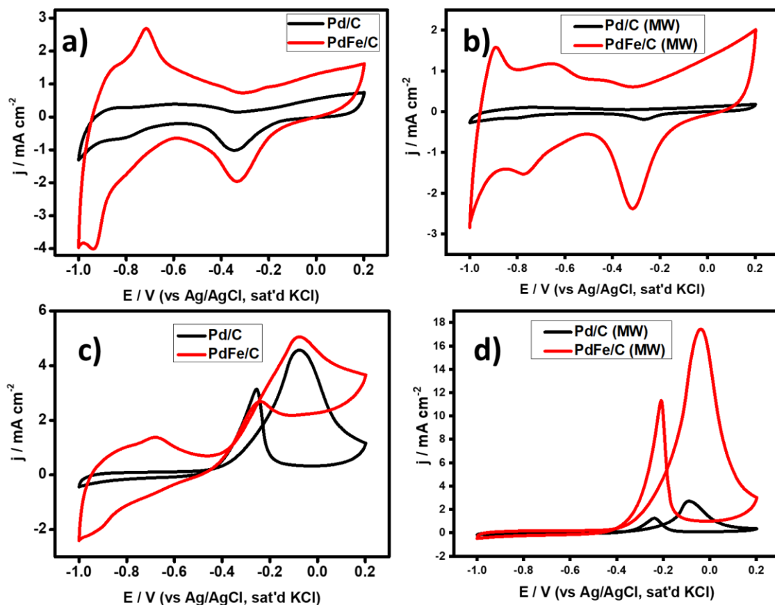
Figure 4.8: Cyclic voltammograms of Pd-based nano-electrocatalysts from conventional NaBH 4 method: a) Pd/C and PdFe/C, and microwave-assisted synthesis b)
