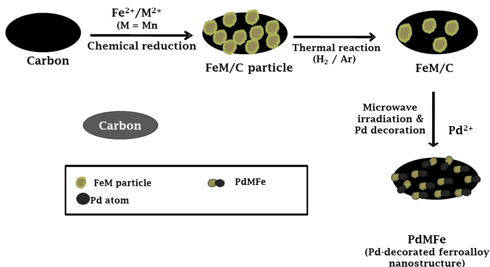
Scheme 3.2: Schematic diagram representing the preparation of trimetallic electrocatalysts.
