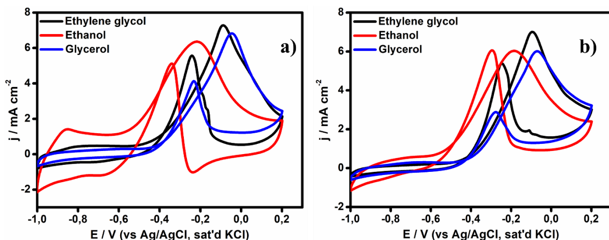
Figure 8.15: Comparative cyclic voltammetry of a) PdFeMn/C and b) PdFeCo/C nano-catalysts in the solution containing 0.5 M KOH / alcohols (EG, EtOH, GOR) @ 50 mV / s.
