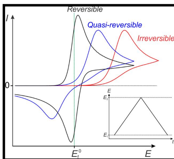
Figure 2.9 Compares CV wave-shapes of three types of reactions that occurred inside electrochemical cells [94].
