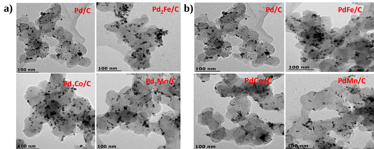
Figure 5.2: TEM micrographs representing a) Pd 2 M/C) and b) PdM/C electrocatalysts.
