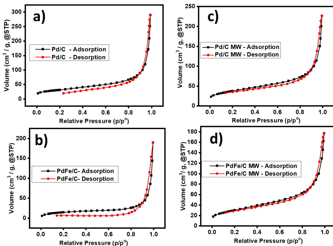
Figure 4.5: N 2 adsorption and desorption isotherms of Pd-based catalysts obtained from the conventional NaBH 4 method: a) Pd/C and b) PdFe/C; and microwave-assisted method: c) Pd/C and d) PdFe/C.
