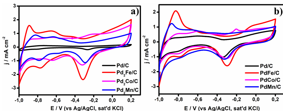
Figure 6.3: CV profiles of catalysts (presented at varied atomic ratio of Pd 2 M/C and PdM/C) in KOH solution (0.5 M), bubbles with N 2 atmosphere at a scan rate = 50 mV / s.
