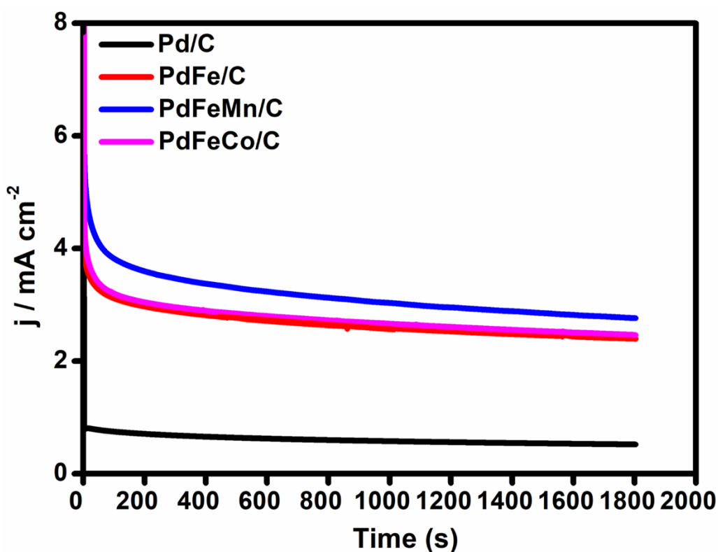
Figure 8.8 Current-times curve of Pd/C, PdFe/C, PdFeMn/C and PdFeCo/C electrocatalysts, potential of -0.2 V in (0.5 M) KOH/EG solution.
