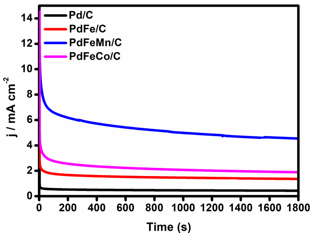
Figure 8.14: Current-times curve of Pd/C, PdFe/C, PdFeCo/C with PdFeMn/C electrocatalysts at -0.2 V in 0.5 M KOH/ 0.5 M Gly solution.
