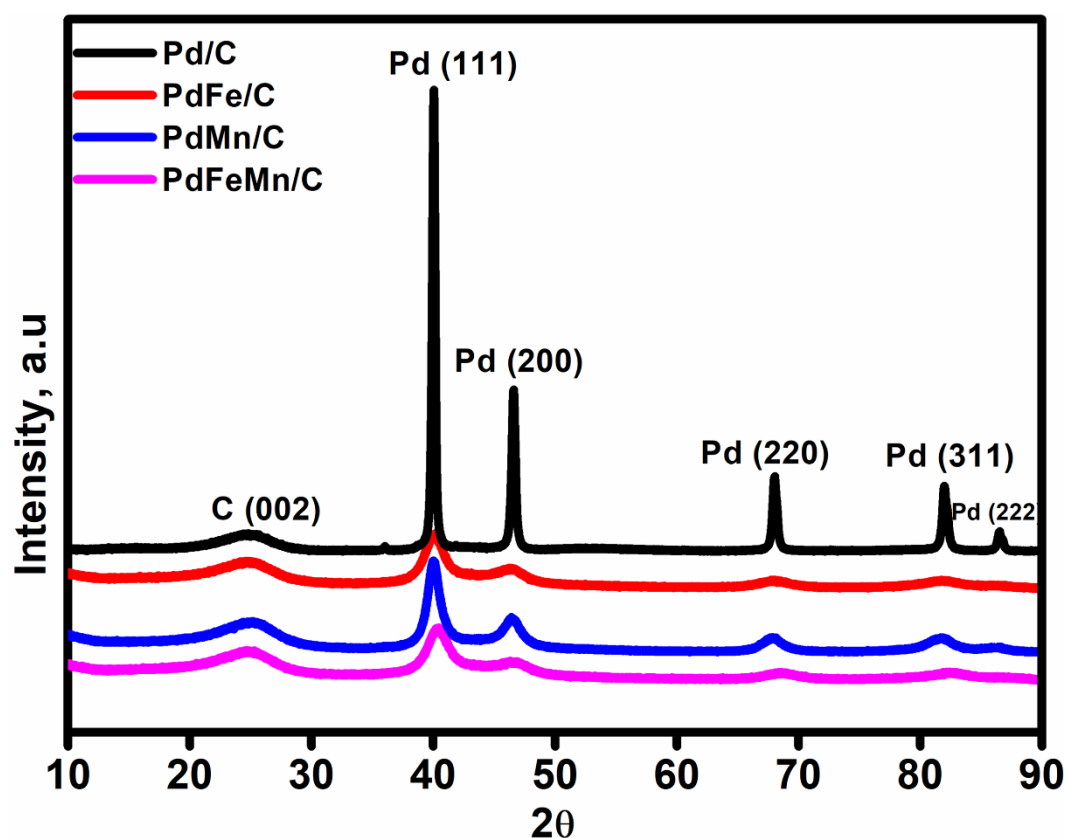
Figure. 9.1: XRD diffractogram of (a) Pd/C, PdFe/C, PdMn/C and PdFeMn/C electrocatalysts.
