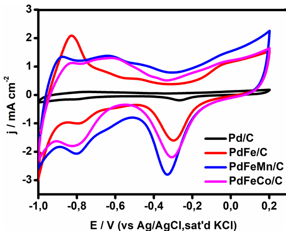
Figure 8.5: Cyclic voltammograms of electrocatalysts containing a solution of (0.5 M) KOH at a sweep rate = 50 mV / s.
