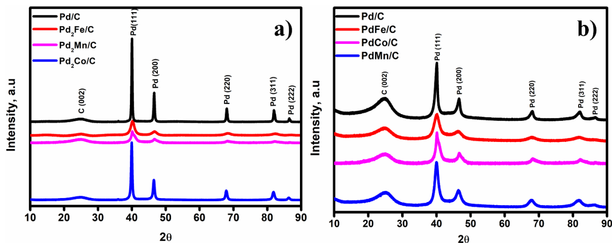
Figure 6.1: XRD diffractograms of electrocatalysts.
