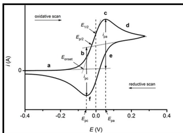
Figure 2.8: A typical CV curve representing an electrochemical of reversible one and electron redox process [93].
