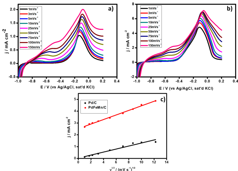
Figure 9.8: LSV of EGOR at the a) Pd/C and b) PdFeMn/C electrocatalysts at varied scan rates, c) Tafel plots of current density vs square root of the scan rate for both electrocatalysts, scan rate 1.0 mV / s.
