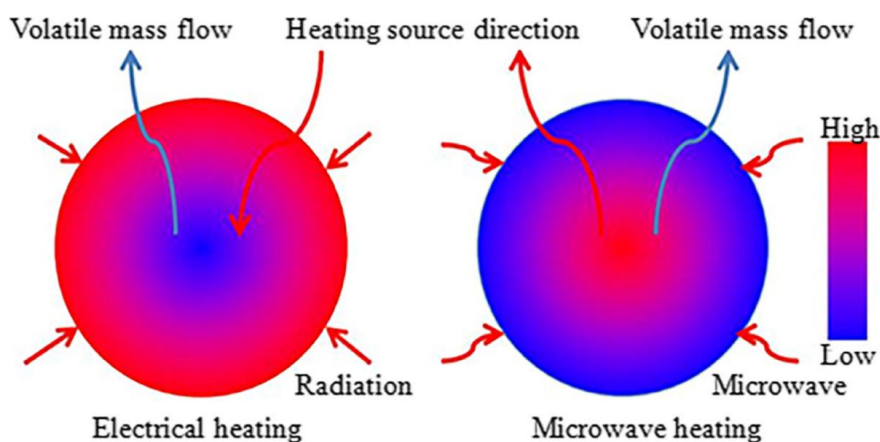
Figure 2.6: A schematic diagram representing microwave vs conventional heating [110]
