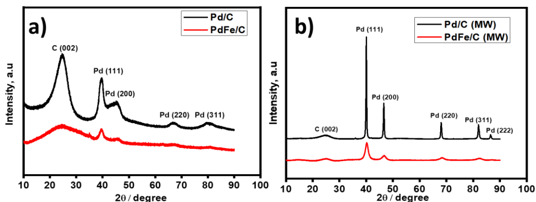
Figure 4.4: Comparison of the XRD patterns of the various Pd-based nanoelectrocatalysts supported on carbon synthesised using a) the NaBH 4 and b) the microwave-assisted methods.
