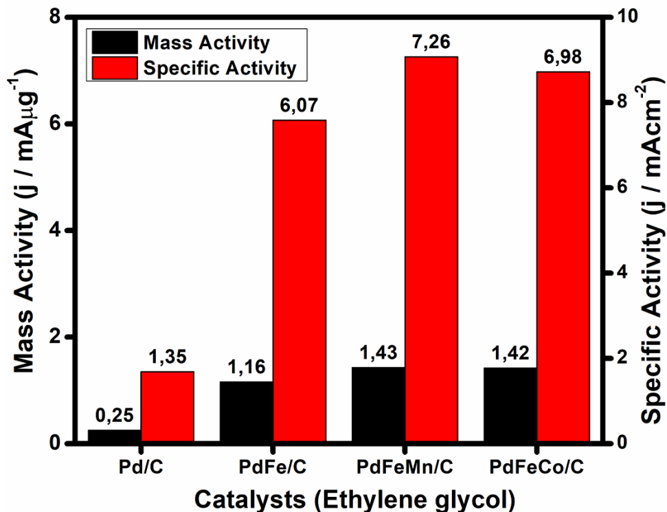
Figure 8.7: Comparison between mass & specific activities of Pd, PdFe/C, PdFeMn/C and PdFeCo/C in KOH/EG containing 0.5 M solution under N 2 gas, 50 mV / s.
