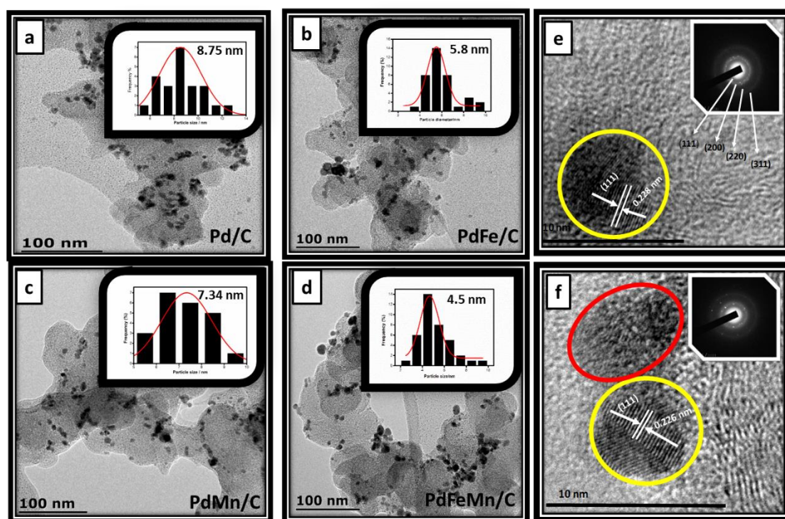
Figure 9.3: Comparative TEM images with particle size distribution histogram insert of (a) Pd/C, (b) PdFe/C, (c) PdMn/C, (d) PdFeMn/C; HRTEM with Insert in (e) and (f) show the SAED pattern of PdFe/C and PdFeMn/C.
