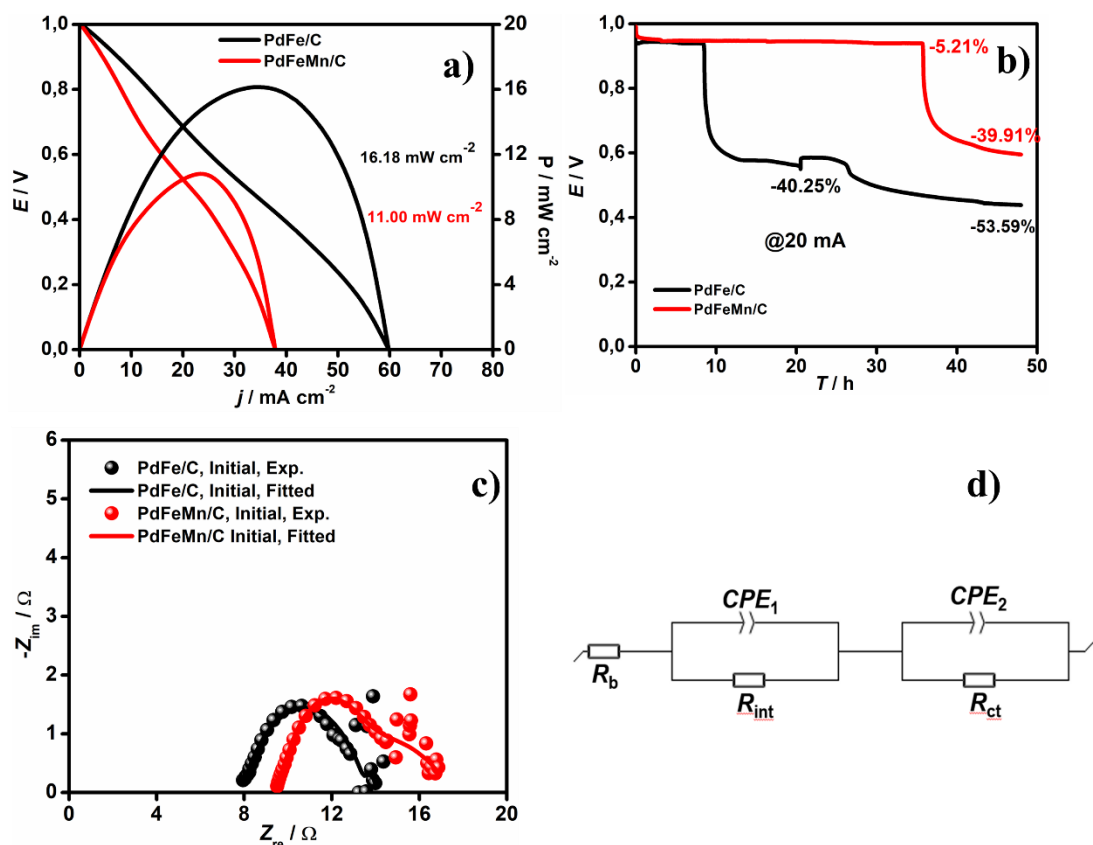
Figure 8.19: (a) Voltage (I-V) and power density curves, (b) galvanostatic discharge curve, (c) Nyquist curves and (d) Voigt EEC for PdFe/C and PdFeMn/C fed with 4 M KOH/ Gly solution.
