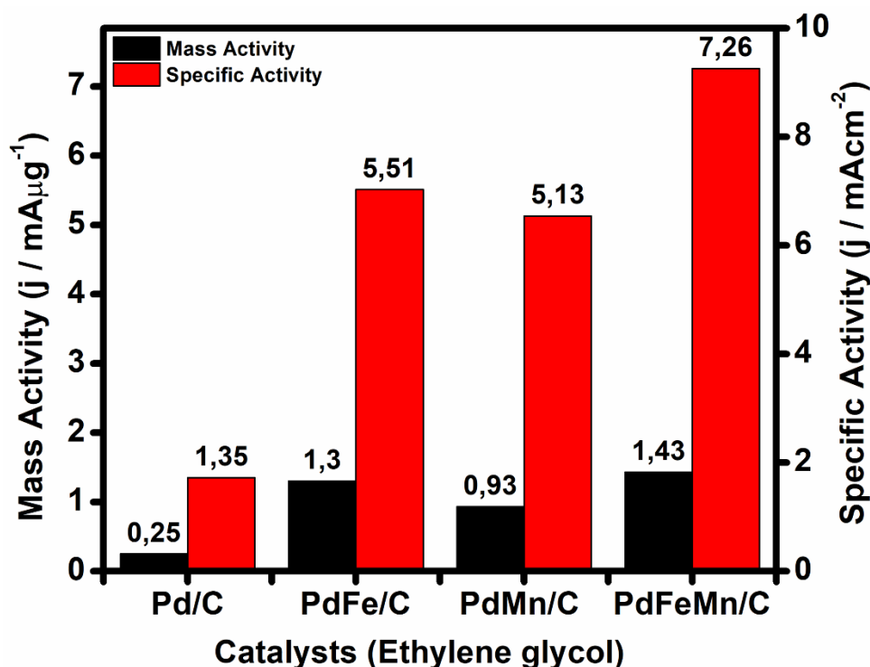
Figure 9.6: EGOR mass and specific activities of Pd, PdFeC, PdMn/C, and PdFeMn/C catalysts.
