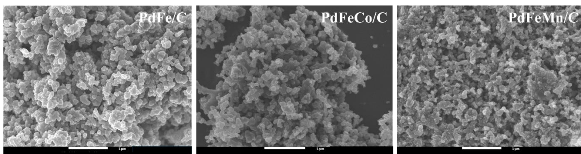
Figure 8.3: SEM images of PdFe/C, PdFeMn/C and PdFeCo/C electrocatalysts.
