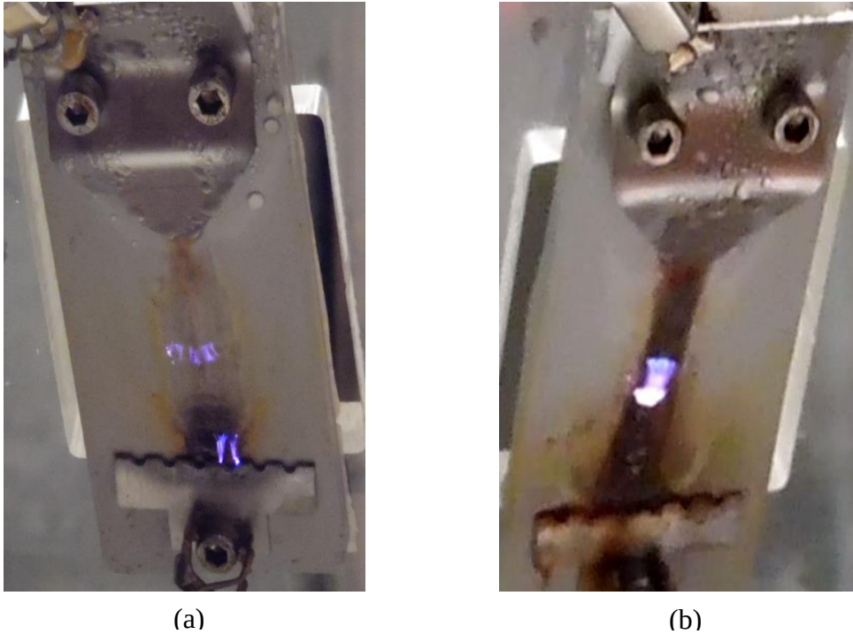
Figure 4.12: Samples of (a) 3.5 kV AC and (b) 3.5 kV DC after 5 hours.
