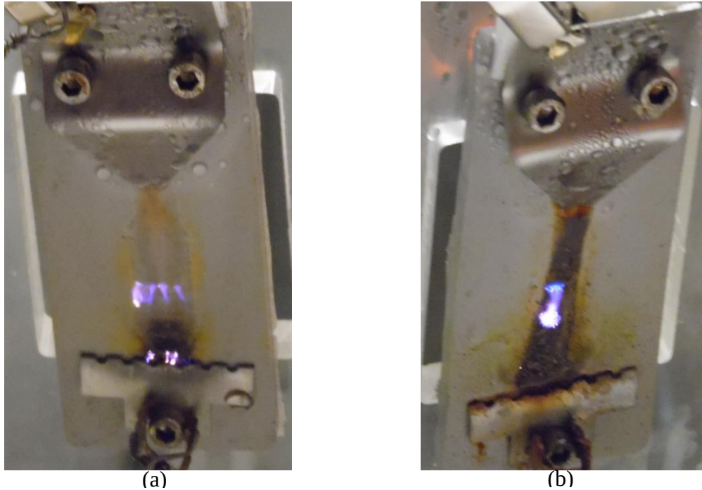
Figure 4.11: Samples of (a) 3.5 kV AC and (b) 3.5 kV DC after 4 hours.
