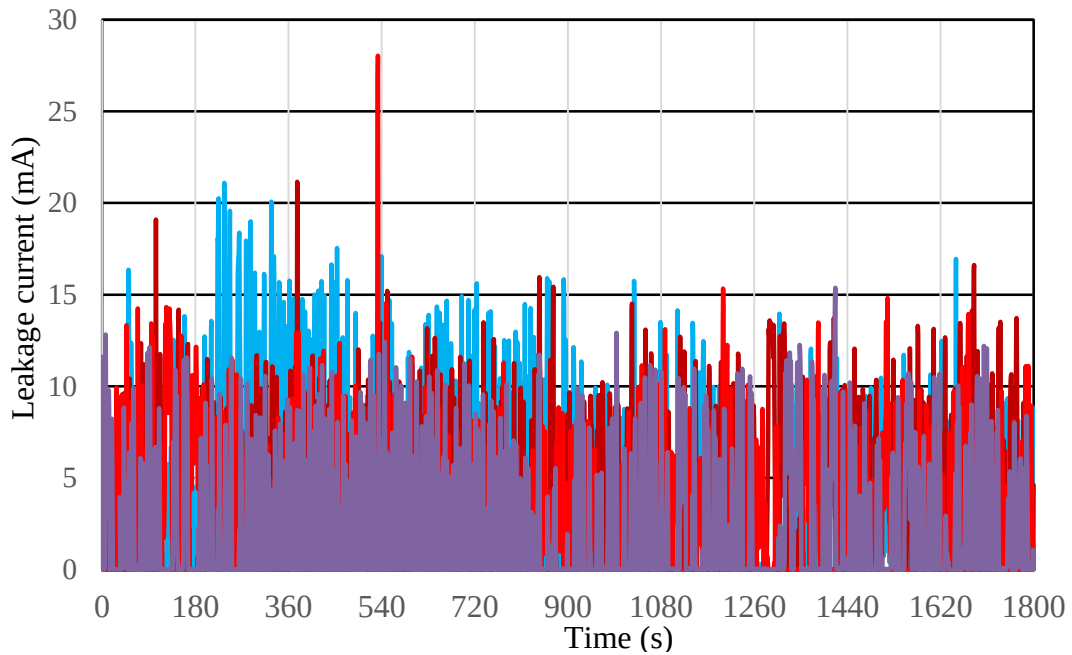
Figure A.1: Absolute Peak leakage currents of 3.5 kV AC samples.
