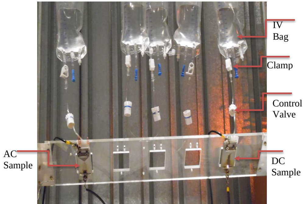
Figure 4.1: Concurrent AC and DC testing of the inclined plane test setup.
