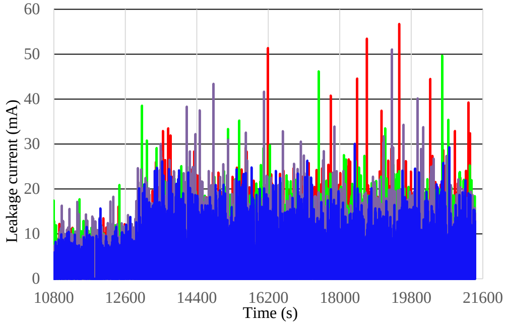
Figure A.2: Absolute Peak leakage currents of 4.5 kV AC samples.
