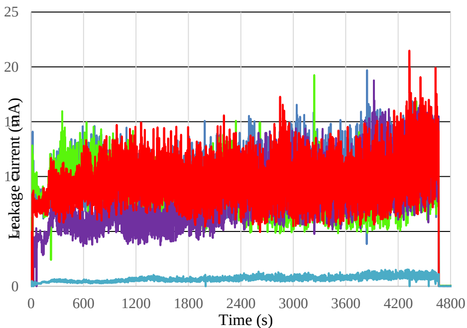
Figure A.3: Absolute peak leakage currents of 4.5 kV DC.samples.
