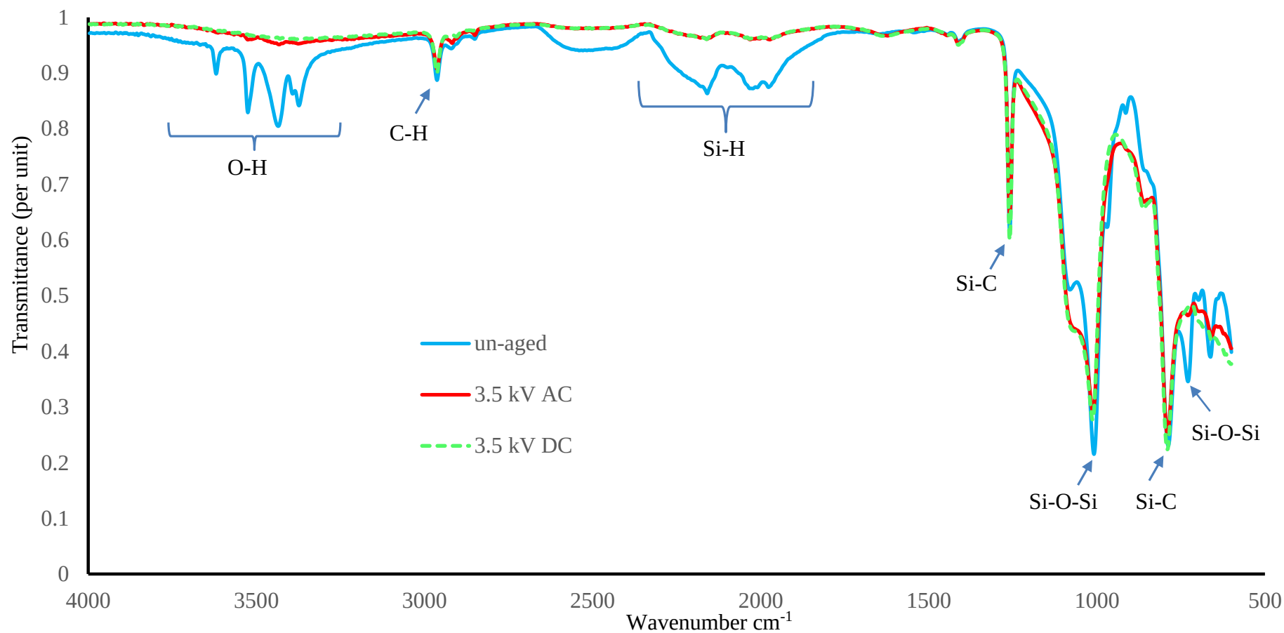
Figure 4.23: Infrared spectra of 3.5 kV AC and DC aged SiR samples with un-aged as the reference.
