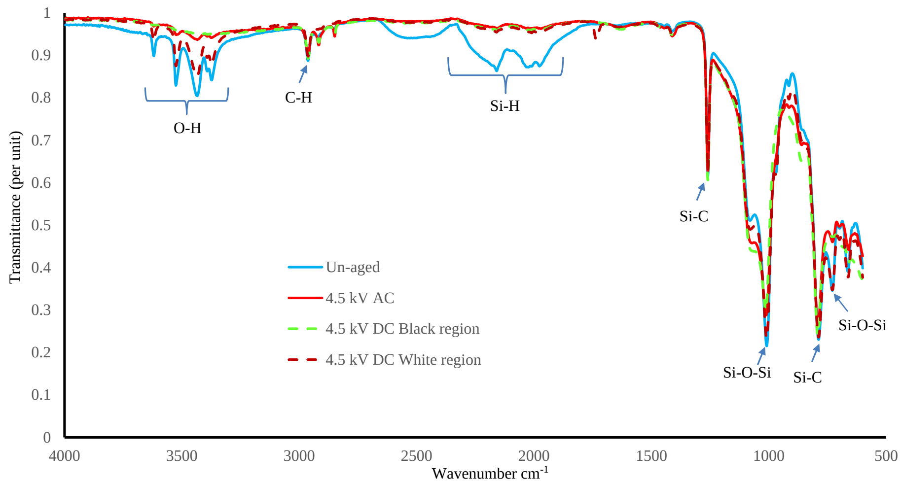
Figure 4.24: Infrared spectra of 4.5 kV AC and DC aged SiR samples with un-aged as the reference.
