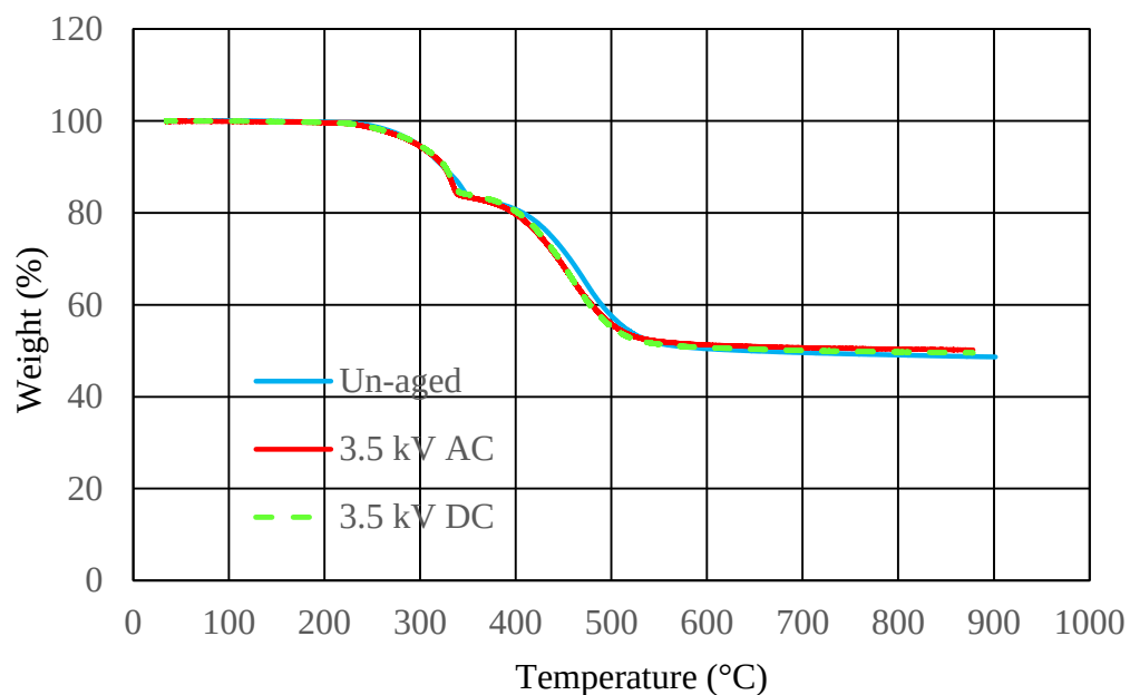
Figure 4. 19: TGA curves of 3.5 kV AC & DC aged and un-aged SiR samples.
