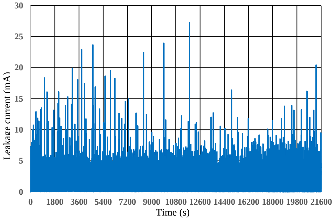
Figure 4.5: Absolute peak leakage current of 4.5 kV AC for one sample.
