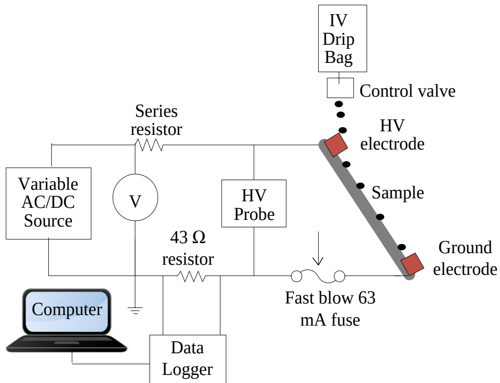
Figure 3.2: Implemented setup of the inclined plane test.
