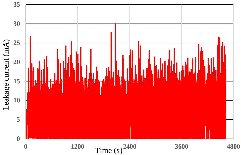
Figure 4.6: Absolute peak leakage current of 4.5 kV DC for one sample.
