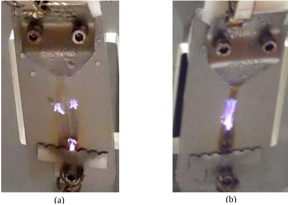
Figure 4.16: Samples of (a) 4.5 kV AC and (b) 4.5 kV DC after 1 hour.
