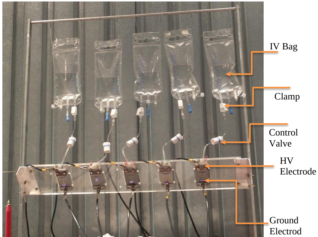
Figure 3.3: Adopted inclined plane test circuit using intravenous drip systems.
