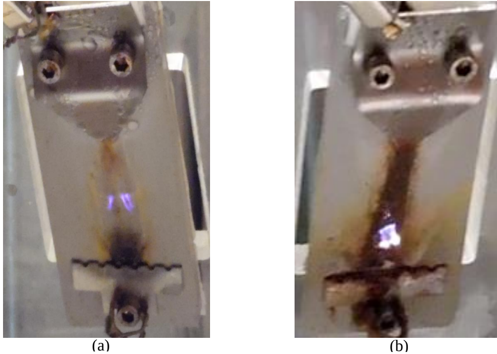
Figure 4.13: Samples of (a) 3.5 k VAC and (b) 3.5 kV DC after 6 hours.
