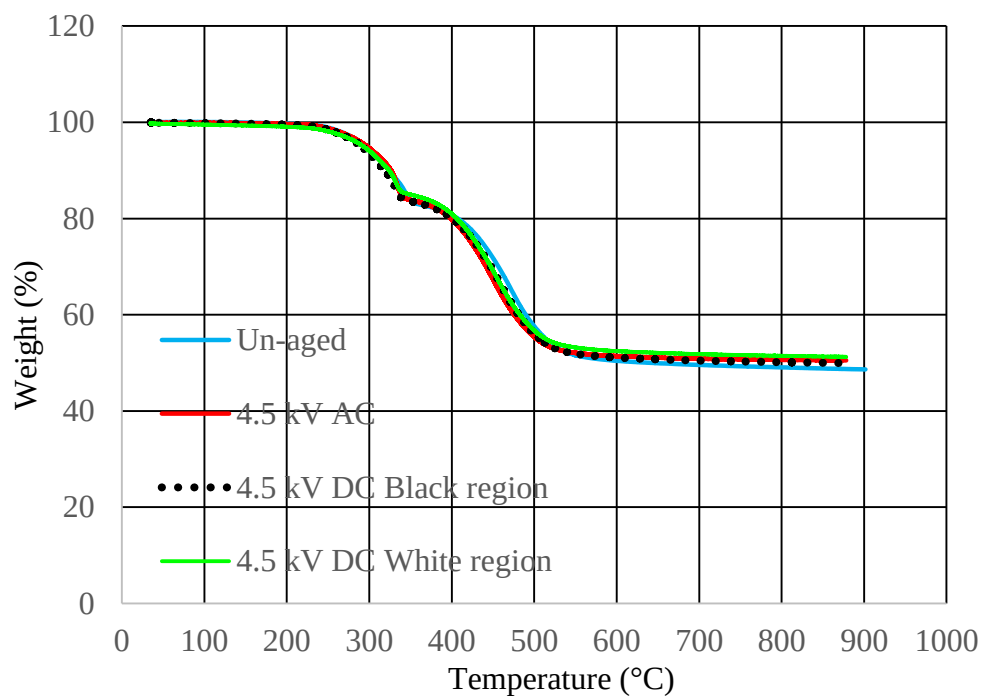
Figure 4. 20: TGA curves of 4.5 kV AC & DC aged and un-aged SiR samples.
