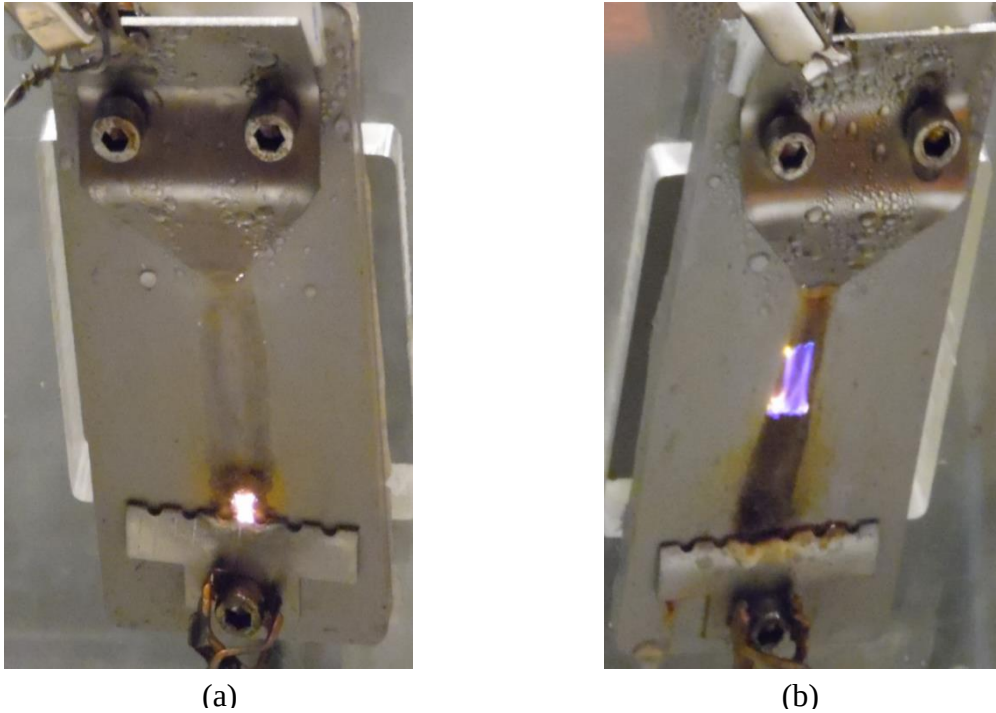
Figure 4.9: Samples of (a) 3.5 kV AC and (b) 3.5 kV DC after 2 hours.
