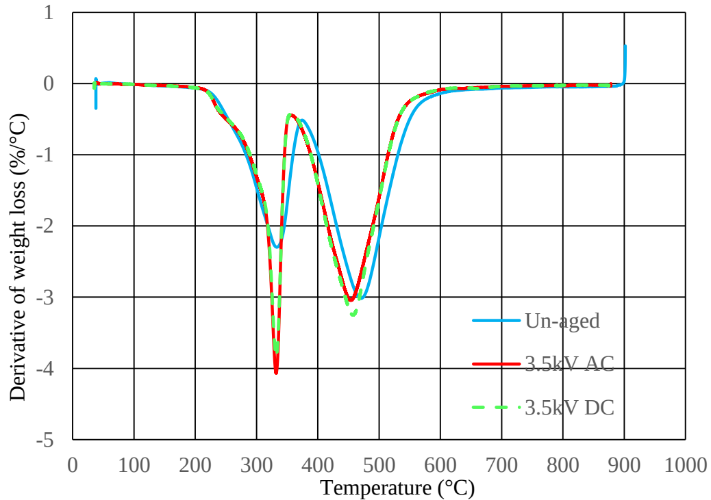
Figure 4. 21: DTG curves of 3.5 kV AC & DC aged and un-aged SiR samples.
