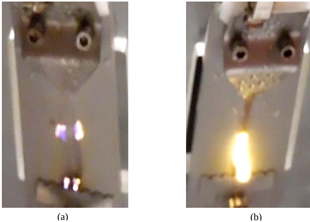
Figure 4.15: Samples of (a) 4.5 kV AC and (b) 4.5 kV DC after 30 minutes.
