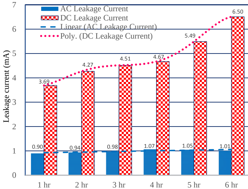
Figure 4.4: Hourly Average leakage currents of 3.5 kV AC and DC samples.
