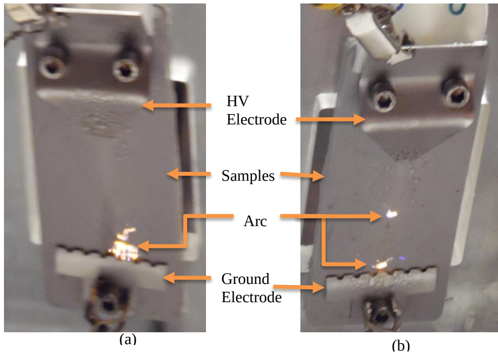
Figure 4.7: Samples of (a) 3.5 kV AC and (b) 3.5 kV DC after 5 minutes.
