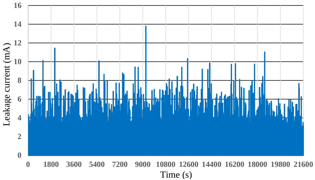
Figure 4.2: Absolute peak leakage current of 3.5 kV AC for one sample.
