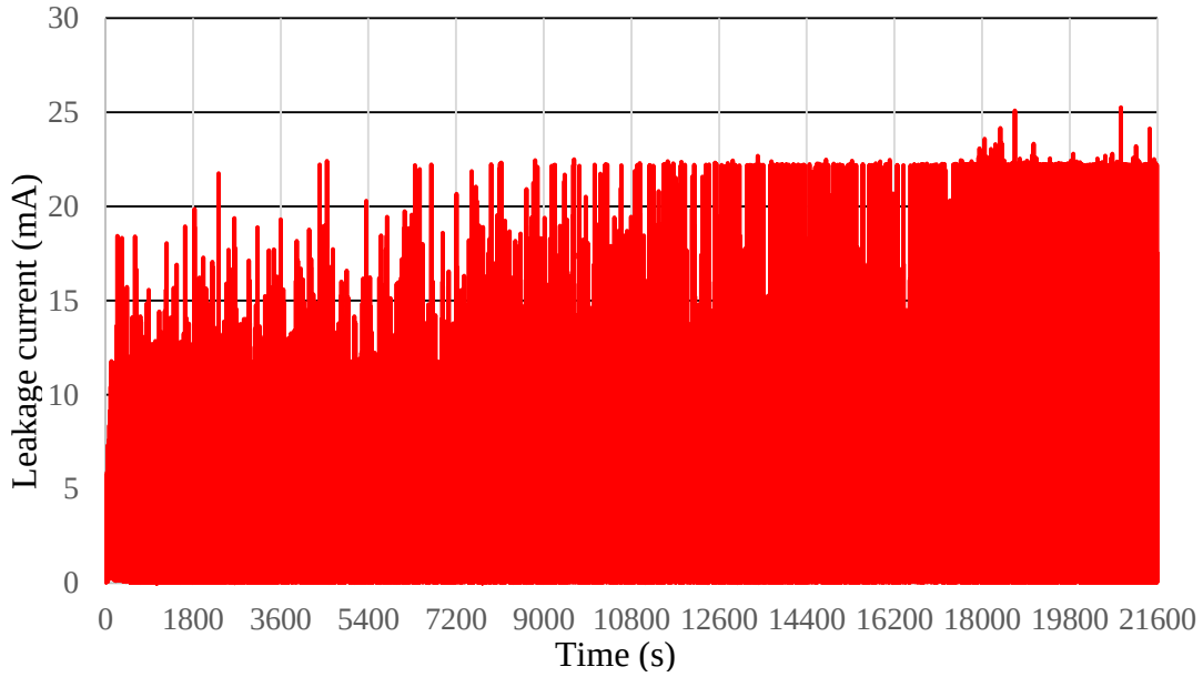
Figure 4.3: Absolute peak leakage current of 3.5 kV DC for one sample.
