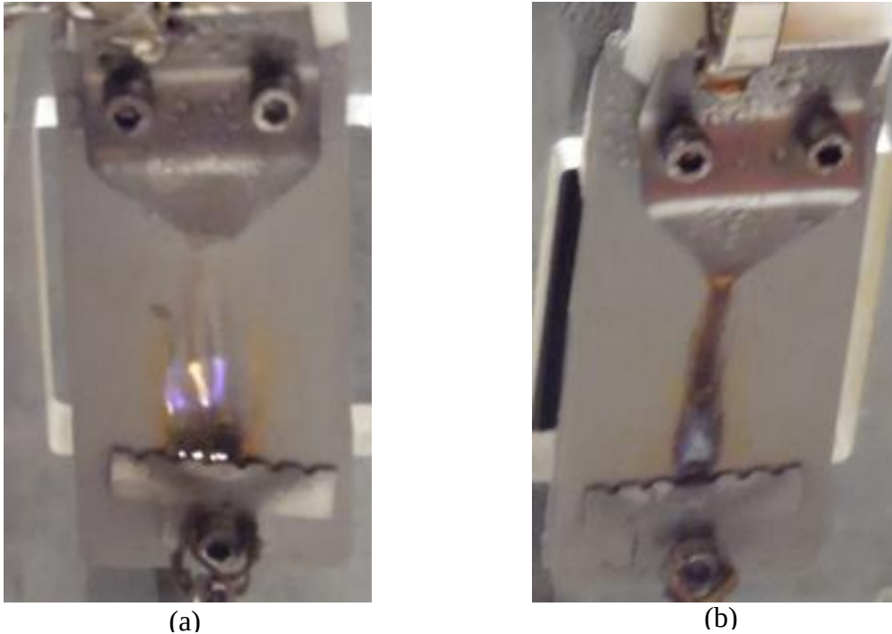
Figure 4.17: Samples of (a) 4.5 kV AC and (b) 4.5 kV DC after 1 ½ hour.
