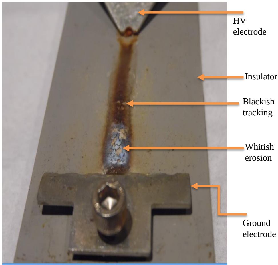
Figure 4.18: 4.5 kV DC sample after 1 ½ hour.
