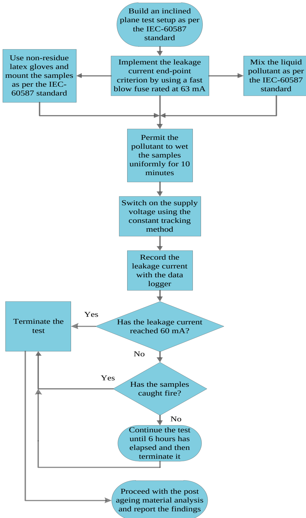
Figure 3.1: Flowchart of the test procedure.
