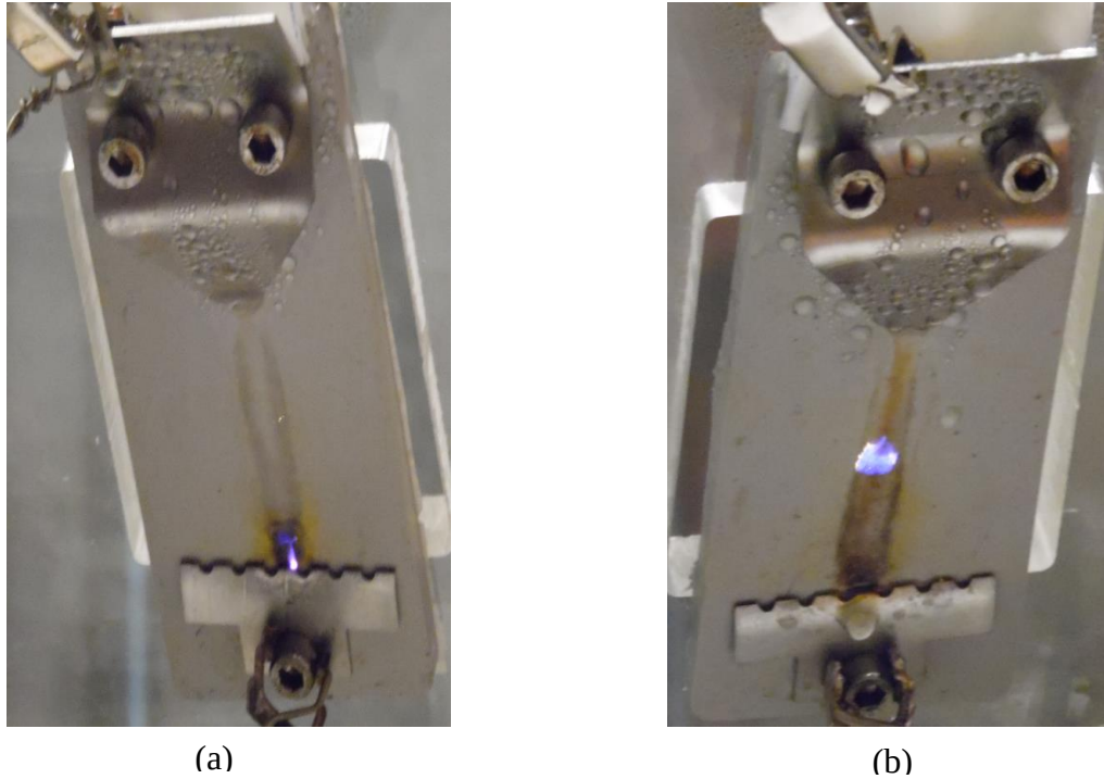
Figure 4.8: Samples of (a) 3.5 kV AC and (b) 3.5 kV DC after 1 hour.
