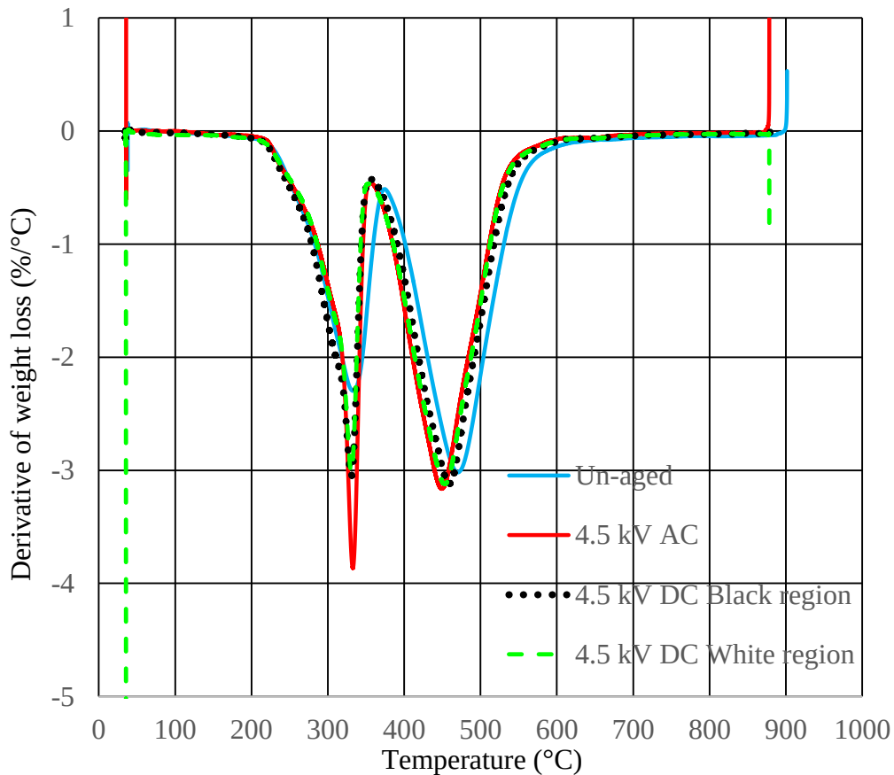
Figure 4.22: DTG curves of 4.5 kV AC & DC aged and un-aged SiR samples.
