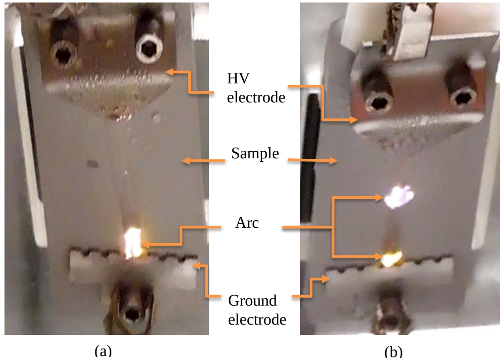
Figure 4.14: Samples of (a) 4.5 kV AC and (b) 4.5 kV DC after 10 minutes.
