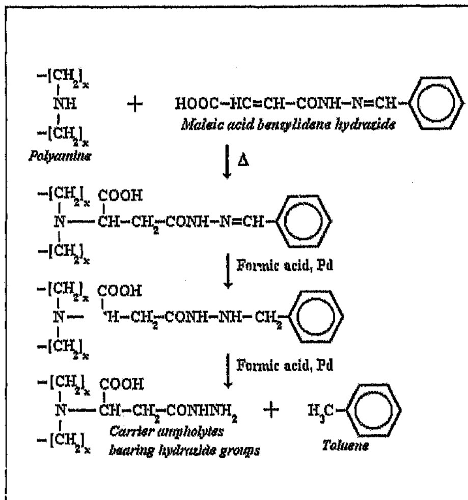
Figure 62 Attempted synthesis of carrier ampholytes bearing hydrazide groups by reacting polyamines such as PEHA with MABH. (The hydrazide group is protected in the form of its benzyl hydrazone.)
