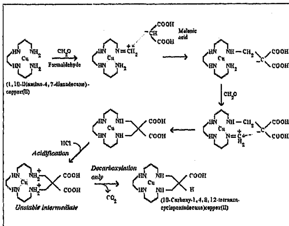
Figure 53 Result of attempted synthesis of 14-amino-2-carboxy-4,8,11-triazatetradec-1-ene.
