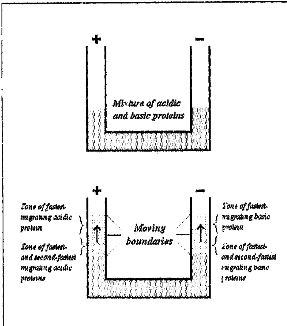
Figure 1 Moving boundary electrophoresis in a U tube.
