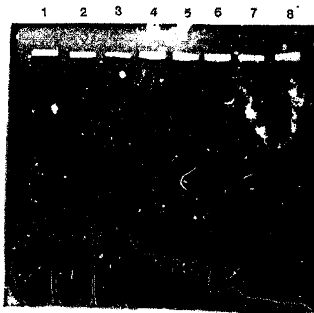
Figure 18 Zone electrophoresis of polyAMPS spacers in a 1% agarose gel, TBE buffer pH 8.7. The filter paper electrode strips were soaked in 10 ml of 16x TBE (62.5 mM Tris, 52 mM boric acid and 0.6 mM Na 2 -EDTA) buffer, pH 8.7. Each well contained 20 \mu l of a 30 mM solution of polyAMPS spacers in TBE buffer containing bromophenol blue and xylene cyanol as markers. The samples were run at 300-400 V at room temperature until the bromophenol blue band was 1 cm from the anode strip. The polyAMPS spacers were stained in a 0.05% solution of methylene blue. The bromophenol blue and xylene cyanol bands diffused out of the gel during staining. Lane 1: polyAMPS-7.5, lane 2: polyAMPS-10, lane 3: polyAMPS-15, lane 4: polyAMPS-30, lane 5: polyAMPS-50, lane 6: polyAMPS-100, lane 7: polyAMPS-200, lane 8: polyAMPS-300.
