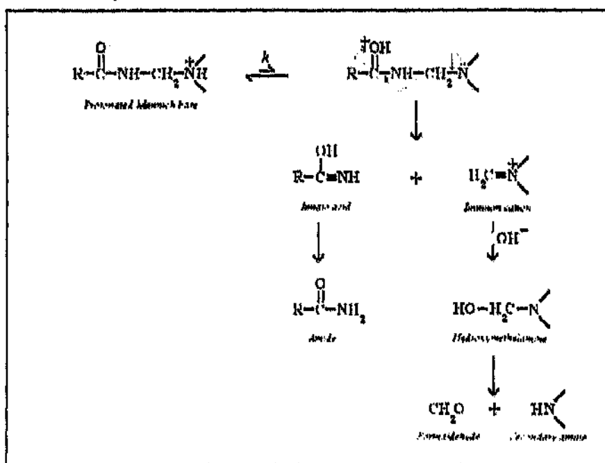
Figure 38 Mechanism of acidic hydrolysis of aminomethylated amides.
