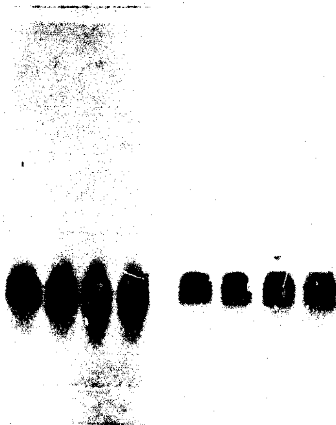
Figure 29 TEP of the 3B7T ampholytic dye fraction in a 5%T, 4%C polyacrylamide gel, using polyAMPS-50 (left) or polyAMPS-30 (right) spacers. The gel buffer was composed of a 10 mM solution of polyAMPS spacer polymers adjusted to pH 9.5 with ethanolamine ( pK=9.5 ). The anolyte and catholyte (terminating electrolyte) were both composed of 400 ml of 100 mM EACA titrated to pH 9.5 with ethanolamine. Solutions (20 \mu l) of the 3B7T fraction were applied to shallow wells on the gel surface. The gels were run at 200 V at room temperature. The ampholytic dyes were fixed by placing the gel in a saturated solution of picric acid containing 10% acetic acid and 2% glycerol, followed by washing in saturated picric acid containing 2% glycerol.
