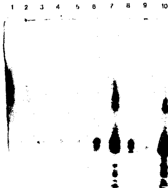
Figure 2B. IEF of ampholytic dyes in a pH 6-10.5 gradient. The gel was composed of 10BT, 4% polyacrylamide, and contained 2% Pharmalyte pH 6-10.5, 10% sorbitol, 8 M urea and 30% DMF. The ampholytic dye solutions were loaded directly on the gel surface. Since the various ampholytic dye fractions varied in concentration, the volumes loaded (20-50 \mu l) were accordingly adjusted in an effort to obtain an equal band intensity of the various fractions. However, the 3B7T and 10T fractions are slightly overloaded. The anode and cathode consisted of thin filter paper strips soaked in 1 M HClO 4 or NaOH, respectively, upon which were laid the platinum electrodes. Focusing was performed at 10°C at an initial voltage of 200 V, with the voltage gradually increased to a final value of 1200 V. Focusing was continued at 1200 V for a further 4 hr. The focused ampholytic dyes were fixed by placing the gel in a saturated solution of picric acid containing 10% acetic acid and 2% glycerol, followed by washing in saturated picric acid containing 2% glycerol. The Pharmalytes were also fixed by the picric acid, and appear as orange bands. Lane 1: 10B, Lane 2: 3B6T, Lane 3: 3B7T, Lane 4: 4B6T, Lane 5: 5B6T, Lane 6: 4B5G, Lane 7: 4B7T, Lane 8: 3B6T, Lane 9: 1B6T, Lane 10: 10T. The anode is at the bottom.
