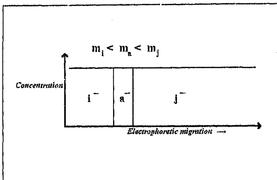
Figure 4 The starting conditions: a zone of intermediate ion a^- has been introduced between the leading and terminating ions, j^- and i^- , respectively.
