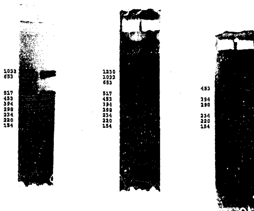
Figure 34 TEP of DNA on a 5%T, 4% polyacrylamide gel, using the polyAMPS-50 (left), 30 (centre) and 15 (right) fractions as spacers. The gel buffer was composed of a 10 mM solution of polyAMPS spacer polymers adjusted to pH 9.5 with ethanolamine ( pK_a 9.5). Both the anolyte and the catholyte (terminating electrolyte) were composed of 400 ml each of 100 mM EACA titrated to pH 9.5 with ethanolamine. The extremities of the gel were connected to the electrode buffer by filter paper strips soaked in electrode buffer. Boehringer Mannheim molecular weight marker VI was used as sample DNA. Nine, ten and six DNA bands are resolved by TEP using the polyAMPS-50, 30 and 15 spacers, respectively, compared to 12 by PAGE (Figure 43). Samples (5 \mu l) of a 40 \mu g/ml solution of DNA (200 ng DNA per well) in 15 mM of EACA ethanolamine buffer, pH 9.5 were loaded in shallow wells on the polyacrylamide gel surface. The sample buffer contained bromophenol blue as a migration marker. The gels were run at room temperature at constant voltage (0.5 W), with an initial voltage of 200 V, and a final voltage of 450 V. Electrophoresis was stopped when the bromophenol blue was 1 cm away from the filter paper electrode strip. The DNA bands were detected with the silver staining method of Sambinetti et al. (1994).
