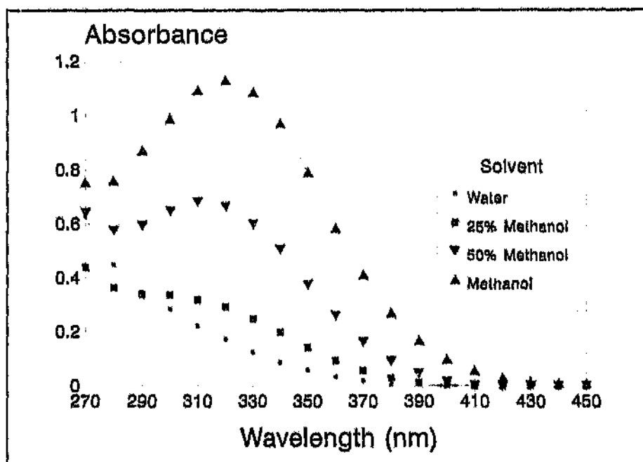
Figure 58 Shift in the UV absorbance spectrum of maleic acid monohydrazide on going from a water to a methanol environment.
