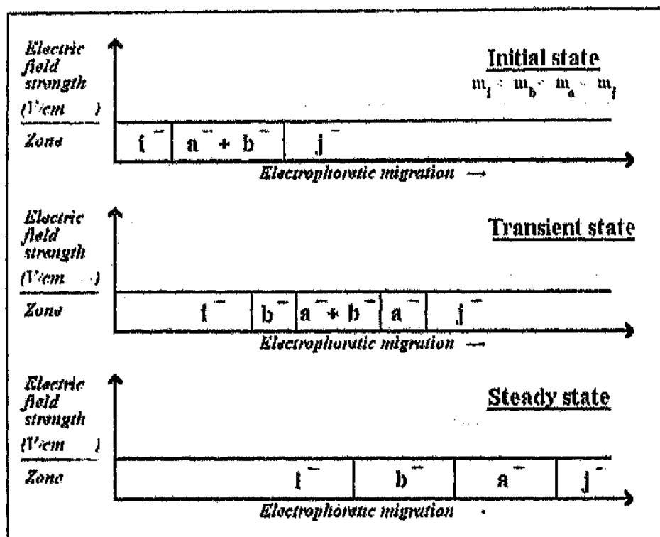
Figure 8 Isotachopheresis of two sample ions a^- and b^- , where a^- has a higher ionic mobility than b^- . As the leading ion j^- migrates in the applied electric field, a stepwise electric field gradient develops across the boundaries of adjacent zones so that all the zones migrate at an equal velocity. The (a^- + b^-) mixed zone gradually becomes separated into two distinct zones. However, while it exists, the (a^- + b^-) mixed zone behaves as a unique zone, of a net ionic mobility equalling the average of the ionic mobilities of the constituent a^- and b^- ions.
