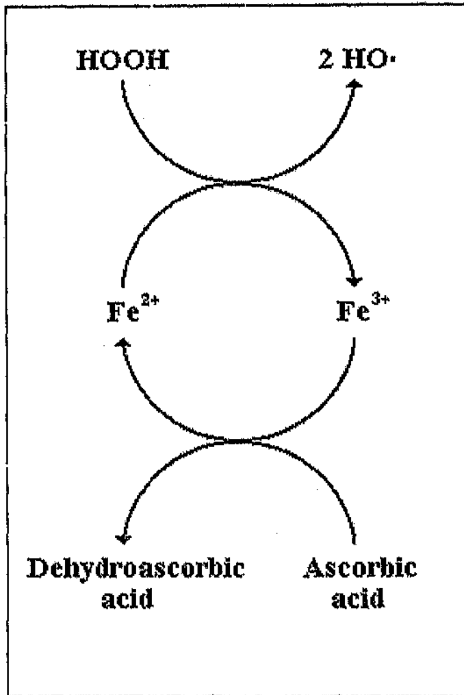
Figure 12 Mechanism of free radical production by Fenton's reagent.
