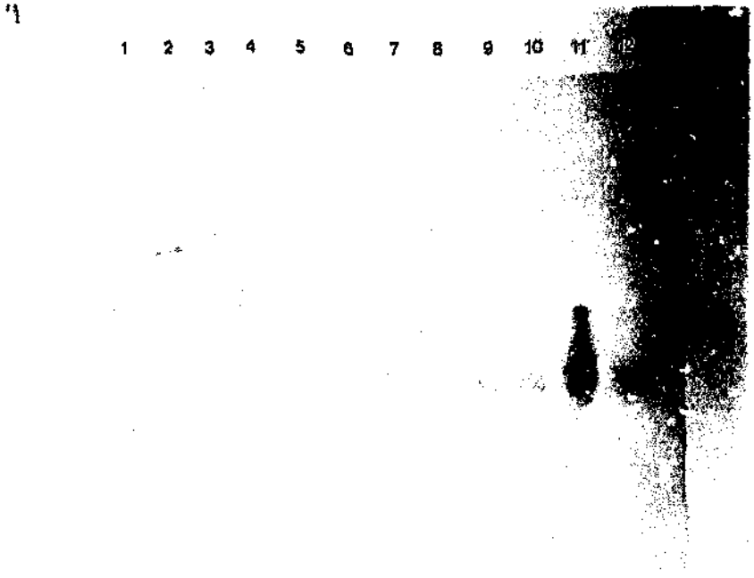
Figure 27 Estimation of the pI range of the ampholytic dye fractions by PAGE in a 4.5%T, 4%C polyacrylamide gel, with 15 mM HCl-ethanolamine, pH 9.5, as the gel buffer. Thin filter paper strips soaked in a 1.5 M solution of the same buffer were applied to the extremities of the gel, upon which the platinum electrodes were placed. 15 \mu l of the ampholytic dye fractions were loaded in narrow wells in the centre of the gel. Lanes 1 and 12: bromophenol blue and xylene cyanol FF dissolved in gel buffer. Lane 2: 10B, lane 3: 8B2T, lane 4: 7B3T, lane 5: 6B4T, lane 6: 5B5T, lane 7: 4B6T, lane 8: 3B7T, lane 9: 2B8T, lane 10: 1B9T, lane 11: 10T. Electrophoresis was conducted at 100 V at 5°C until the bromophenol blue had migrated 5 cm. The ampholytic dyes were fixed by placing the gel in a saturated solution of picric acid containing 10% acetic acid and 2% glycerol, followed by washing in saturated picric acid containing 2% glycerol. The bromophenol blue cannot be seen because it is in its acidic form (yellow). The 10B to 3B7T fractions (lanes 1 to 8) contain a significant proportion of ampholytic dye isomers with pI values greater than 9.5.
