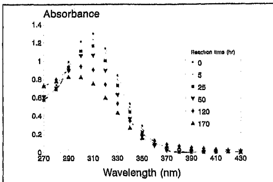
Figure 63 Reaction of MABH with PENA in methanol at room temperature by following the decrease in A_{310} .
