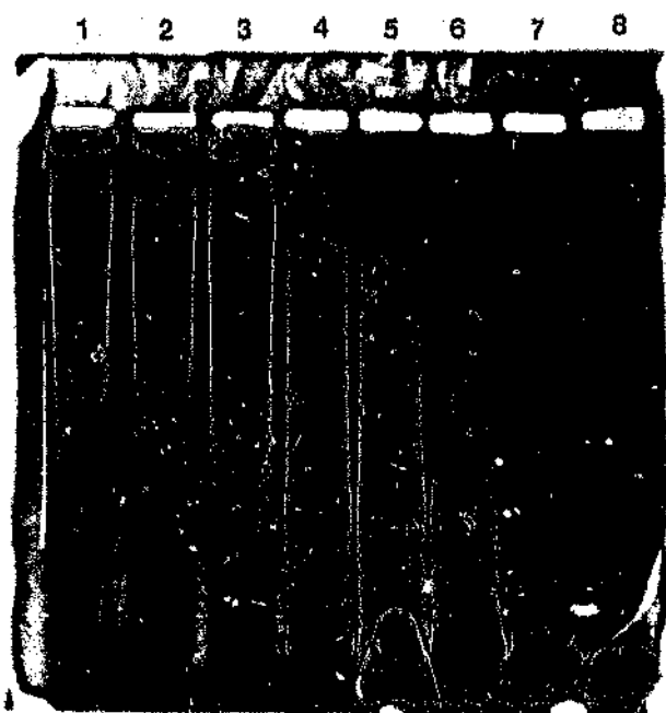
Figure 20 Zone electrophoresis of polyAMPS spacers in a 3.5%T, 4%C polyacrylamide gel, TBE buffer pH 8.7. The procedure of electrophoresis and staining of the polyAMPS polymers is as for Figure 18. Lane 1: polyAMPS-7.5, lane 2: polyAMPS-10, lane 3: polyAMPS-15, lane 4: polyAMPS-30, lane 5: polyAMPS-50, lane 6: polyAMPS-100, lane 7: polyAMPS-200, lane 8: polyAMPS-300.
