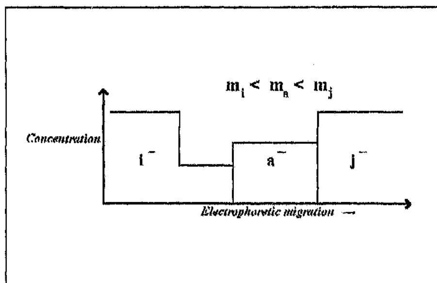
Figure 5 Steady state: the concentrations of a^- and the terminating ion i^- have been regulated according to the concentration of the leading ion j^- .
