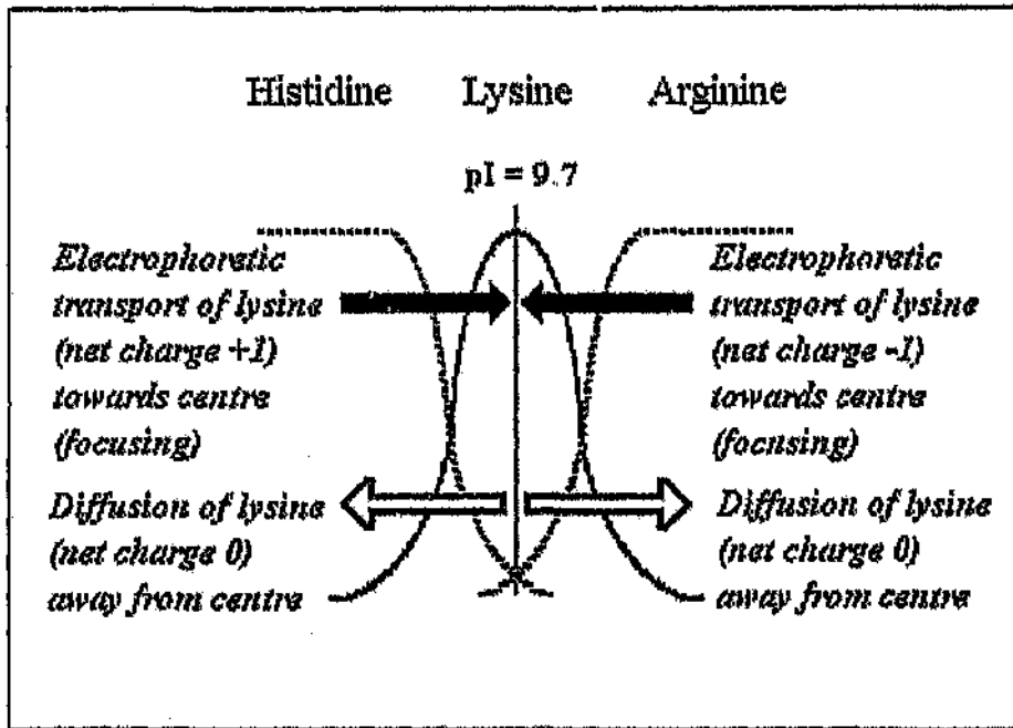
Figure 54 Illustration of a focused zone of lysine, represented as a symmetrical Gaussian peak about its pI . The electrophoretic inward migration of lysine is balanced by the outward movement due to diffusion.
