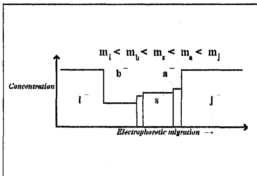
Figure 11 The effect of the addition of a spacer ion s of intermediate ionic mobility to a and b .
