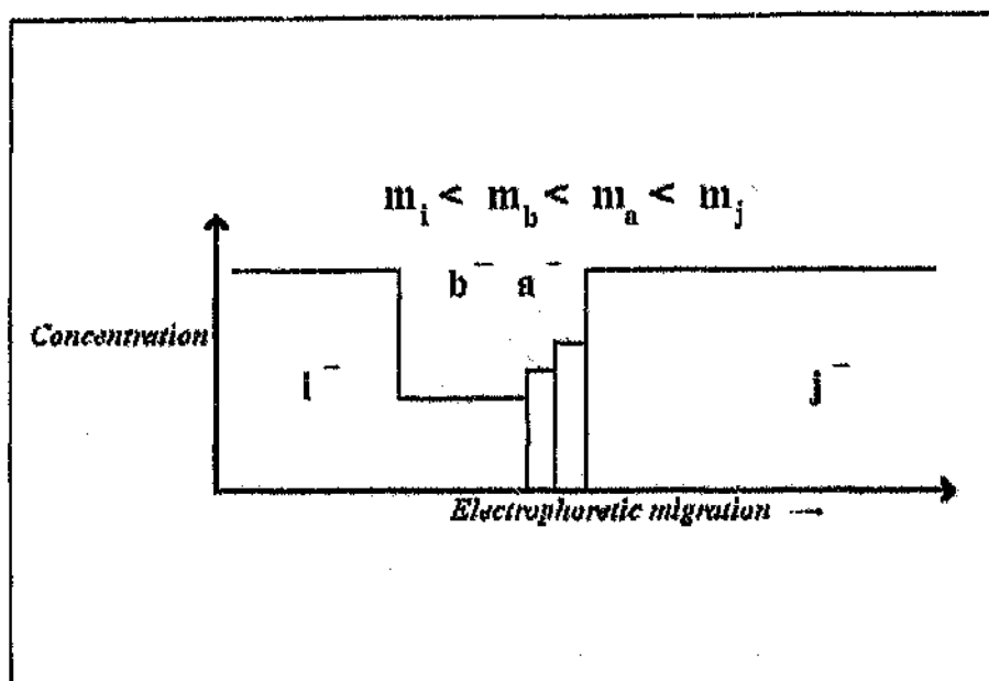
Figure 10 Steady state conditions for a sample containing two ions, a and b . Although their zones have been completely separated, they cannot be visually distinguished.
