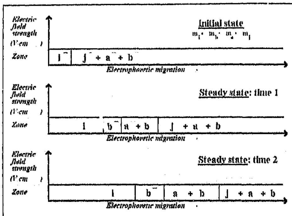
Figure 9 A modification of isotachopheresis in which the leading ion j^- is contaminated with two sample ions a^- and b^- , where a^- has a higher ionic mobility than b^- . Hence the leading electrolyte is composed of the mixed zone ( j^- + a^- + b^- ), of a net ionic mobility equalling the average of the ionic mobilities of the constituent ions. As the leading ion j^- migrates in the applied electric field, it leaves behind the slower moving a^- and b^- ions, resulting in the formation of a permanent mixed zone ( a + b ), where the net ionic mobility of the zone equals the average of the ionic mobilities of the constituent a^- and b^- ions. In a similar fashion the a^- ion leaves behind the slower moving b^- ion, resulting in the formation of a pure zone of b^- ions. These zones grow in a telescopic fashion during the course of electrophoresis hence this modification of isotachopheresis has been named telescope electrophoresis by Schafer-Nielsen and Svendsen (1980, 1981). Although the electric field strength gradient is shallower in telescope electrophoresis than in isotachopheresis, it has the advantage that the steady state is immediately attained, i.e. the formation of discrete zones.
