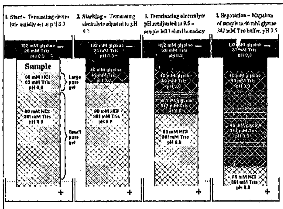
Figure 17 The mechanism of operation of the Ornstein-Davis discontinuous buffer system.
