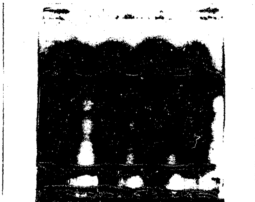
Figure 49 Focusing of myoglobin from horse heart on a pH 7.3-7.5 IPG, prepared using \alpha -( N -morpholinomethyl)acrylic acid as the buffer and the pK 9.3 Immobiline ® as the titrant, in concentrations calculated using the DoctorpH program. The same procedure for prefocusing and loading of the IPG gels was used as for Figure 48. Focusing was performed at 5°C overnight at an initial field strength of 1000 V. The next day the electric field strength was gradually raised over the course of seven hours to a final value of 4900 V. Focusing was continued at 4900 V for a further 56 hr. The gel was stained with Coomassie Blue G-250 according to Reisner (1984). The major band is the myoglobin. The anode is at the bottom.
