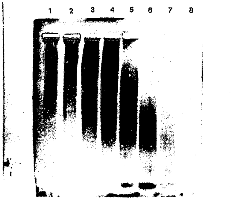
Figure 23 Zone electrophoresis of polyAMPS samples in a 15%T, 2.5%C polyacrylamide gel, TBE buffer pH 8.7. The procedure of electrophoresis and staining of the polyAMPS polymers is as for Figure 18. Lane 1: polyAMPS-10, lane 2: polyAMPS-15, lane 3: polyAMPS-30, lane 4: polyAMPS-50, lane 5: polyAMPS-100, lane 6: polyAMPS-200, lane 7: polyAMPS-300, lane 8: polyAMPS-500.
