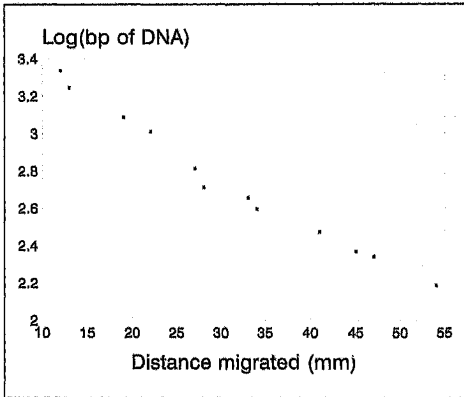
Figure 33 Plot of the logarithm of the size (in bp) of each DNA molecule versus its migration distance, for the PAGE experiment of Figure 33.
