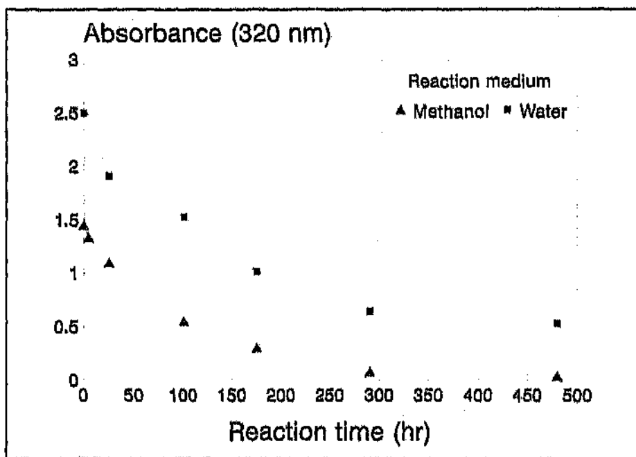
Figure 61 Comparison of the rates of reaction of maleic acid monohydrazide with TEPA at room temperature in methanol and water.
