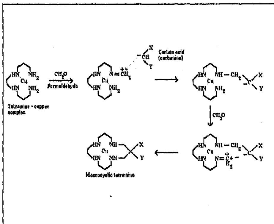
Figure 51 Reaction of carbon acids and formaldehyde with a tetramine-copper complex. The X and Y groups of the carbon acid are carbonyl groups such as carboxylic acids and their esters, ketones and nitriles.
