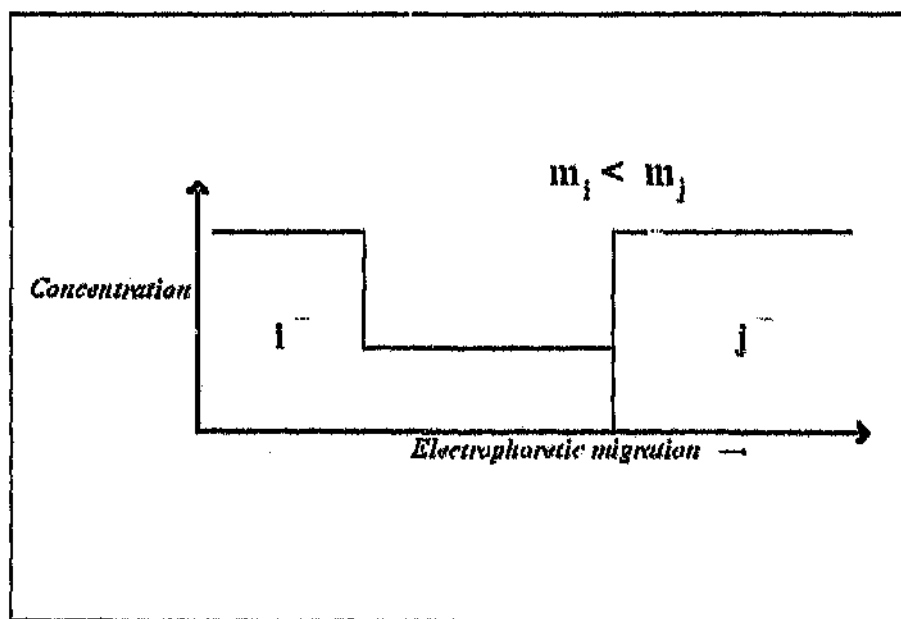
Figure 3 Attainment of the steady state. The concentration of l^- has been regulated according to the concentration of j^- .
