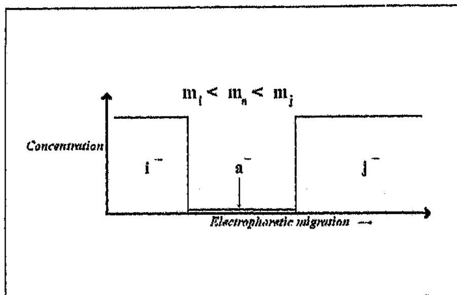
Figure 6 The starting conditions: a dilute zone of sample ion a^- has been introduced between the leading and terminating ions, j^- and i^- , respectively.
