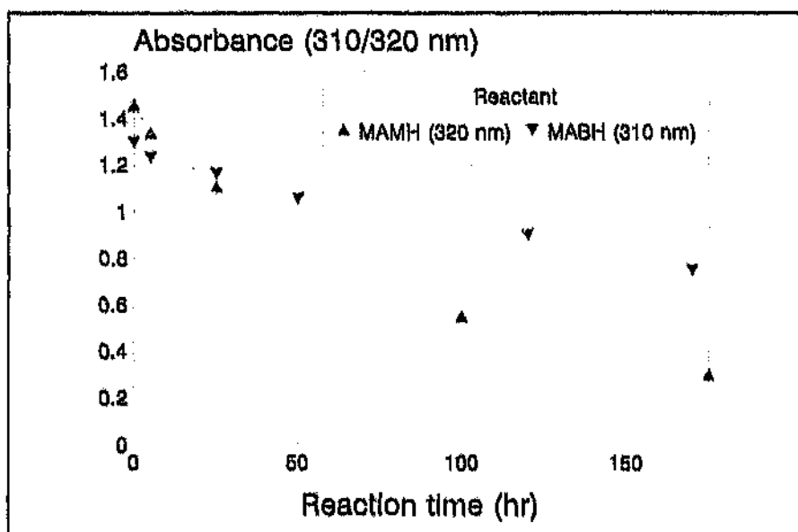
Figure 64 Comparison of the rates of reaction of MAMH and MABH with a polyamine at room temperature in methanol.
