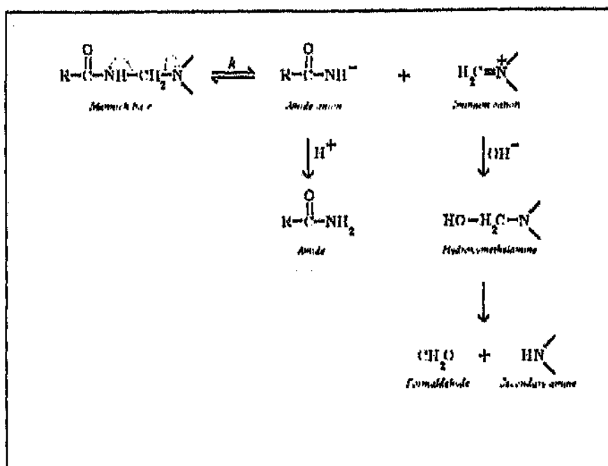
Figure 37 Mechanism of basic hydrolysis of aminomethylated amides.
