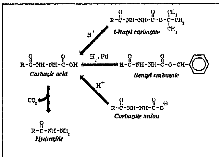
Figure 57 Different methods of protecting of one of the nitrogen atoms of hydrazine so as to get acylation of only one nitrogen by maleic anhydride.
