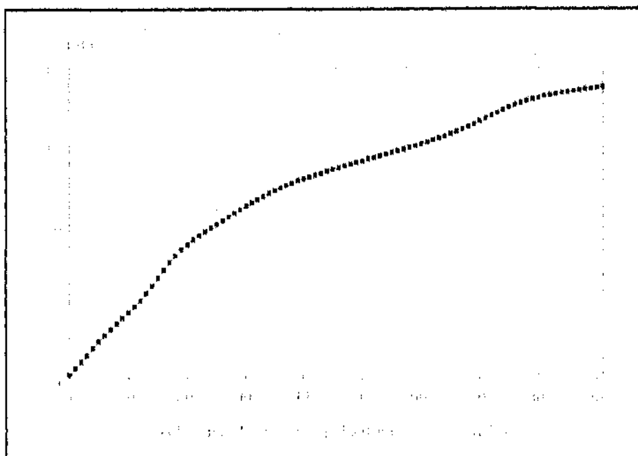
Figure 45 Titration curve of crude \alpha -( N,N -dimethylaminomethyl)acrylic acid. The \alpha -( N,N -dimethylaminomethyl)acrylic acid was synthesized by dissolving 0.25 mole of malonic acid in 26% (w/v) dimethylamine solution (dimethylamine content: 0.25 mole), followed by the slow addition of 0.5 mole formaldehyde (commercial 37% solution), with cooling in ice-water. The reaction was conducted at room temperature. A 0.5 ml sample of reaction mixture was diluted in 35 ml of distilled water, and titrated with 0.1 N NaOH at 20°C. The titration curve shows the product to be impure. The major contaminant is probably bis( N,N -dimethylaminomethyl)acetic acid, as obtained by Pelletier and Franz (1952).
