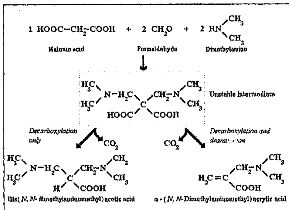
Figure 39 Reaction between malonic acid, formaldehyde and dimethylamine in aqueous solution (Pelletier and Franz, 1952).
