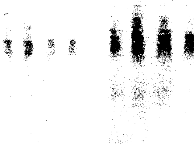
Figure 31 TEP, in the presence of urea, of the 3B7T ampholytic dye fraction in a 5%T, 4%C polyacrylamide gel, using polyAMPS-15 (left) and polyAMPS-10 (right) spacers. The gel buffer was composed of a 10 mM solution of polyAMPS spacer polymers containing 9.5 M urea, adjusted to pH 9.5 with ethanolamine ( pK=9.5 ). The anolyte and catholyte (terminating electrolyte) were both composed of 400 ml of 100 mM EACA titrated to pH 9.5 with ethanolamine. Solutions (20 \mu l) of the 3B7T fraction were applied to shallow wells on the gel surface. The gels were run at 200 V at room temperature. The ampholytic dyes were fixed by placing the gel in a saturated solution of picric acid containing 10% acetic acid and 2% glycerol, followed by washing in saturated picric acid containing 2% glycerol.
