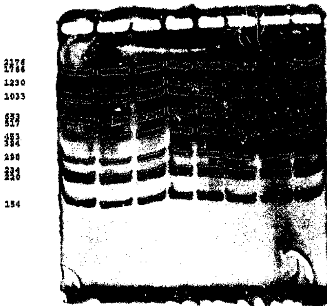
Figure 32 Zone electrophoresis of DNA on a horizontal 5%T, 4%C polyacrylamide gel in TBE buffer (62.5 mM Tris, 52 mM boric acid and 0.6 mM Na-EDTA, pH 8.7). The filter paper electrode strips were soaked in a 18X solution of the same buffer. Boehringer Mannheim molecular weight marker VI was used as sample DNA. The mixture contains 15 fragments with the following number of base pairs (1 base pair = 660 daltons): 2176, 1766, 1230, 1033, 653, 517, 453, 394, (2x 298), (2x 234), 220, (2x 154), but only 12 bands are resolved. Samples (5 \mu l) of a 40 \mu g/ml solution of DNA ( \approx 200 ng DNA per well) in 15 mM of EACA-ethanolamine buffer, pH 9.5 were loaded in shallow wells on the polyacrylamide gel surface. The sample buffer contained bromophenol blue as a migration marker. The gels were run at 200 V at room temperature until the bromophenol blue was 1 cm away from the filter paper electrode strip. The DNA bands were detected with the silver staining method of Sanguinetti et al. (1994).
