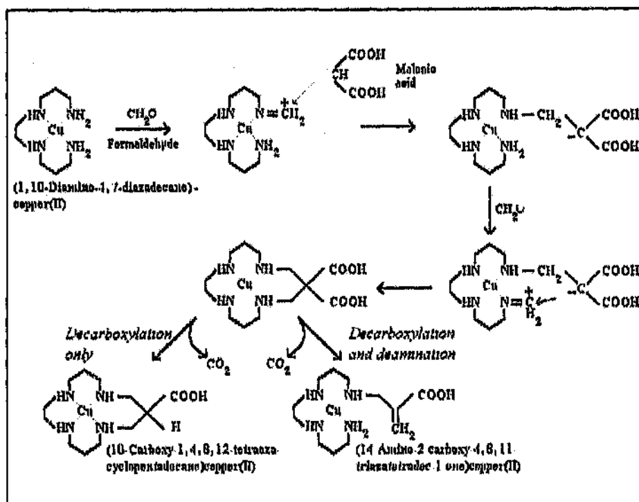
Figure 52 Proposed pathway for the synthesis of 14-amino-2-carboxy-4,8,11-triazatetradec-1-ene.
