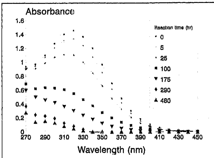
Figure 59 Reaction of maleic acid monohydrazide with TEPA at room temperature in methanol followed by measuring the decrease in A_{320} .
