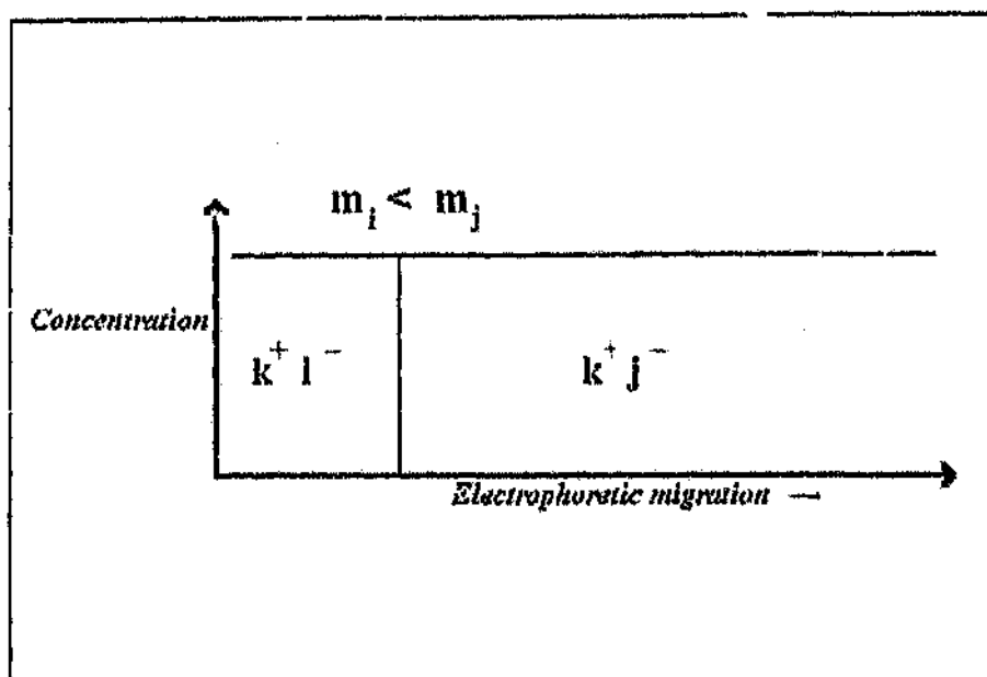
Figure 2 The initial condition in the separating column, with the concentrations of the adjacent salt solutions, k^+ l^- and k^+ j^- , arbitrarily set equal.
