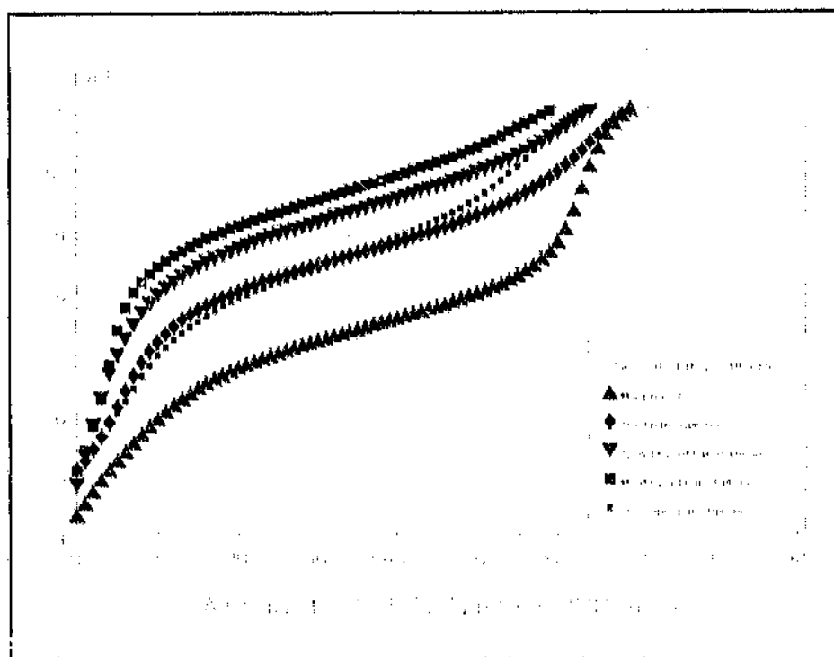
Figure 44 Titration curves of various \alpha -aminomethylated acrylic acids. The \alpha -aminomethylated acrylic acids were synthesized by dissolving 0.25 mole of malonic acid and 0.25 mole of secondary amine in 50 ml of distilled water, followed by the slow addition of 0.5 mole formaldehyde (commercial 37% solution), with cooling in ice-water. The reaction was conducted at room temperature. A 0.5 ml sample of reaction mixture was diluted in 35 ml of distilled water, and titrated with 0.1 N NaOH at 20°C. The titration curves show the presence of only one buffering group in each reaction mixture, differing in pK from the original secondary amine, i.e. the products are essentially pure.
