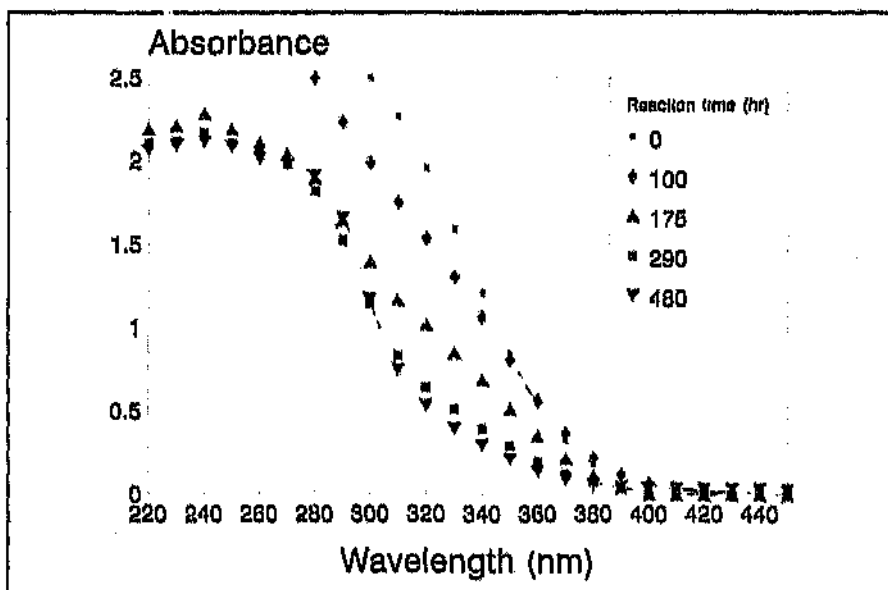
Figure 60 Reaction of maleic acid monohydrazide with TEPA at room temperature in water followed by measuring the decrease in A_{320} .
