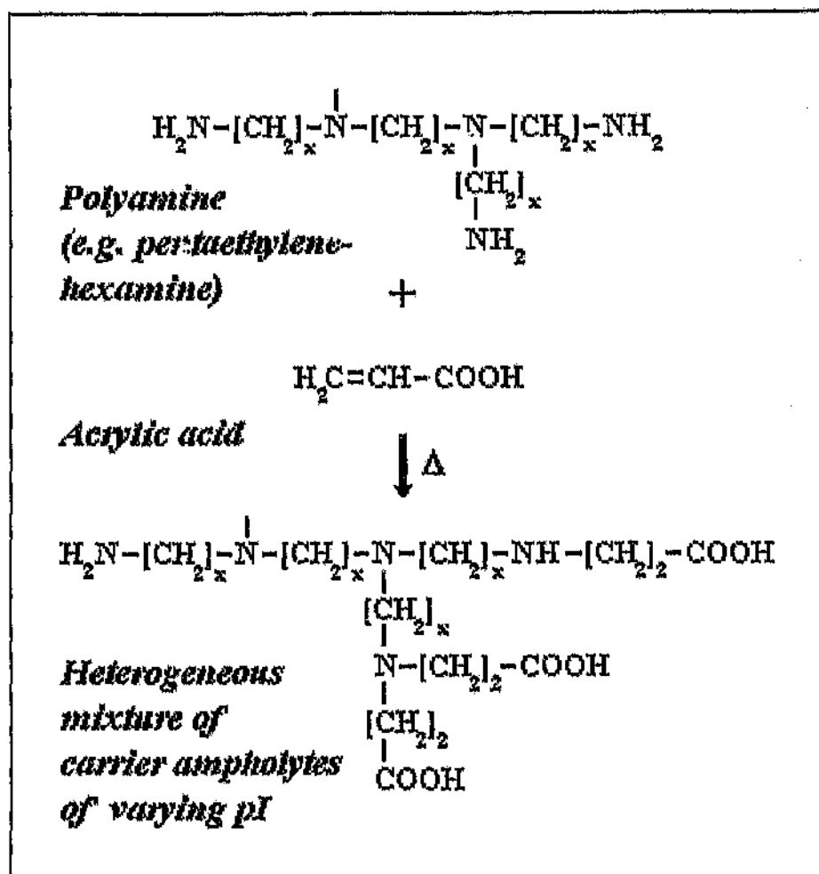
Figure 55 Synthesis of carrier ampholytes by reaction of a polyamine with acrylic acid to produce a highly heterogeneous mixture of polyamino-polycarboxylic acid buffers of varying pI.
