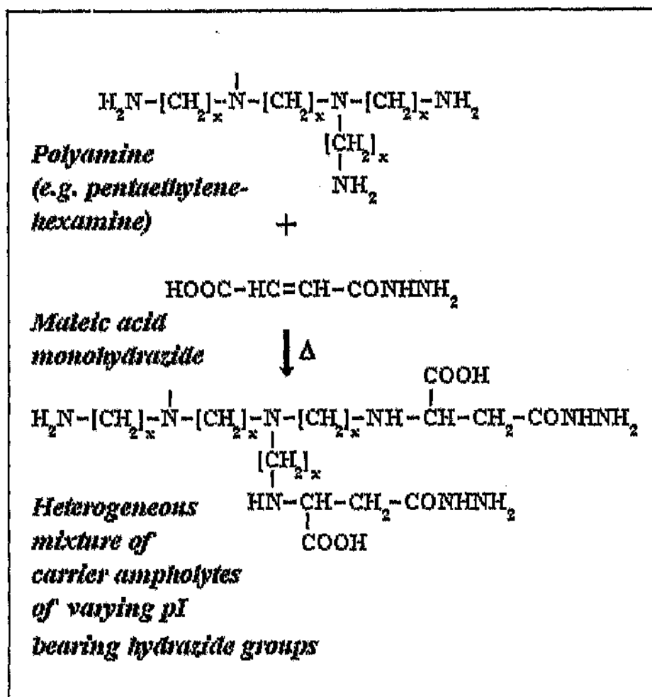
Figure 56 Attempted synthesis of carrier ampholytes bearing hydrazide groups by reacting polyamines such as PEHA with maleic acid monohydrazide.
