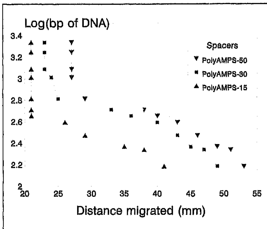
Figure 35 Plot of the logarithm of the size (in bp) of each DNA molecule versus its migration distance, for the TEP experiment of Figure 35.
