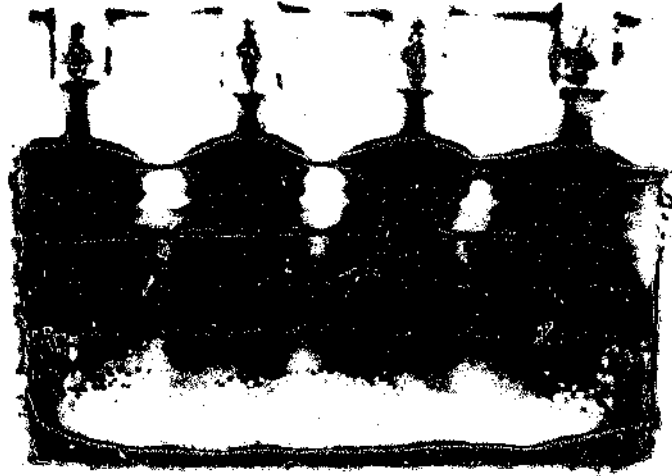
Figure 46 Focusing of myoglobin (pI 7.4) from horse heart on a pH 6.9-7.9 IPG, prepared using \alpha -(N-morpholinomethyl)-acrylic acid as the buffer and the pK 9.3 Immobiline ® as the titrant, in concentrations calculated using the DoctorpH program. Filter paper electrode strips (distilled water) were applied and prefocusing of the gel performed at a maximum power of 15 W until the salt fronts had migrated into the electrode strips. Fresh electrode strips were then applied (anode - 10 mM glutamic acid, cathode - 10 mM histidine). The myoglobin sample was loaded on shallow wells (2 mm deep) on the gel surface as 100 \mu l samples of approximately 10 mg/ml solutions in 20% glycerol. Focusing was performed at 5°C for 2 hr at an initial field strength of 2000 V, which was gradually raised to a final value of 5000 V. The gel was stained with Coomassie Blue G-250 according to Reisner (1984). The major band is the myoglobin. The anode is at the bottom.
