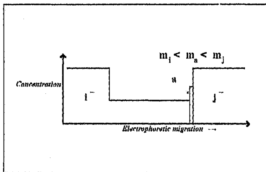
Figure 7 Sample stacking effect: the concentration of the sample ion, a , has been regulated according to the concentration of the leading ion i^- .
