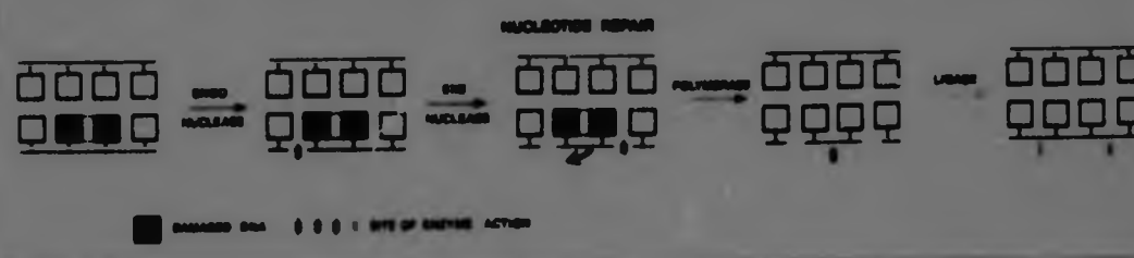
Figure 1.6 Nucleotide excision repair (after Bartram, 1980)
