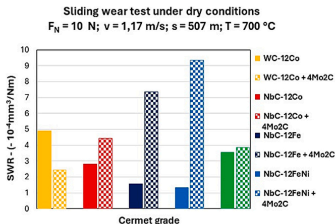
Fig. 10. Sample Wear Rates for the cermet grades at 700 °C.
