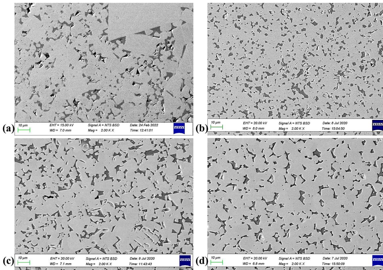
Fig. 2. BSE images showing the effect of \text{Mo}_2\text{C} additions in the Ni and Fe binder cermets; (a) NbC-Ni, (b) NbC-Ni- \text{Mo}_2\text{C} , (c) NbC-Fe and (d) NbC-Fe- \text{Mo}_2\text{C} .
