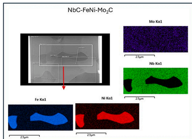
Fig. 4. X-ray maps showing the dispersion of \text{Mo}_2\text{C} in the NbC and FeNi phases.
