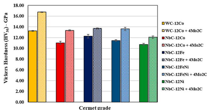
Fig. 8. Vickers hardness (HV 30 ) for the different cermet grades.
