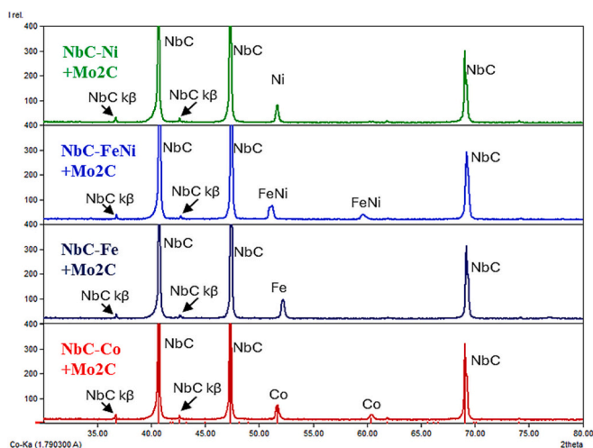
Fig. 5. XRD patterns of NbC cermets sintered at 1390 °C with Mo 2 C additives showing a two-phase structure.
