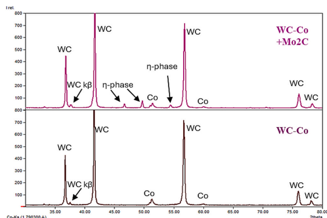
Fig. 6. XRD patterns of the WC-12Co grades.
