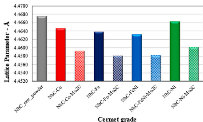
Fig. 7. Effect of Mo 2 C additions on the NbC lattice parameters.
