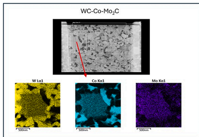
Fig. 3. X-ray maps of the eta-phase observed in the WC-Co- \text{Mo}_2\text{C} grade.
