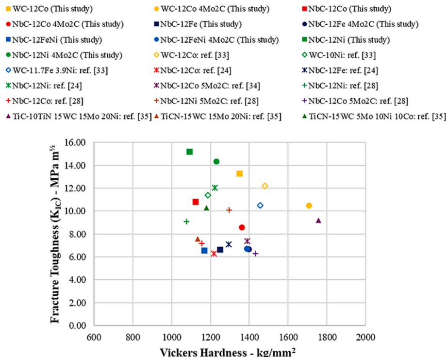
Fig. 9. Hardness and fracture toughness properties compared to literature data [24,28,33–35].
