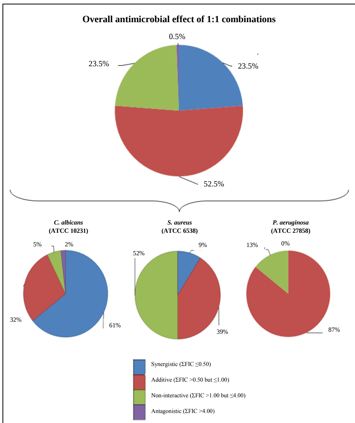
Figure 4.3 The antimicrobial interactions determined for the essential oil combinations against C. albicans , S. aureus and P. aeruginosa .
