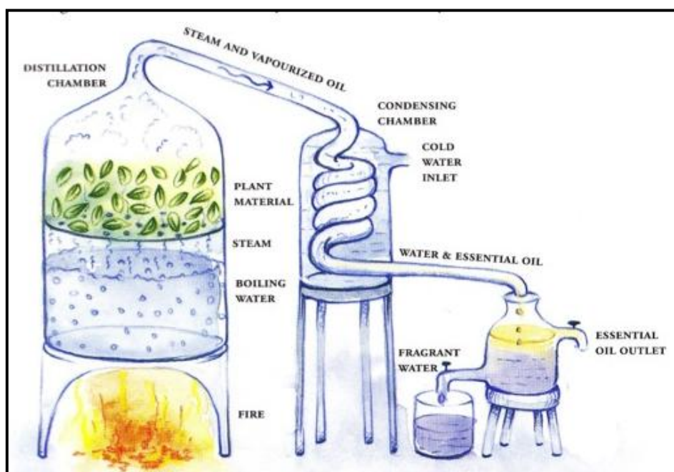
Figure 1.1 Schematic indication of the process of steam distillation ( www.attunearoma.com ).
