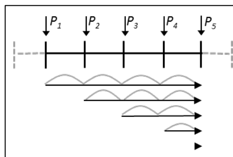
Fig. 16.1 FV scenario: 5 payments covering 4 periods
