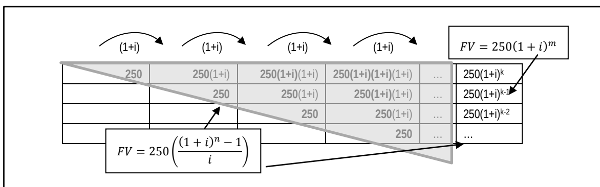
Fig. 15.6 Links between processes and objects at multiple levels in an annuities spreadsheet
