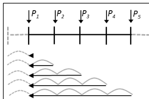
Fig. 16.2 PV scenario: 5 payments covering 4 periods
