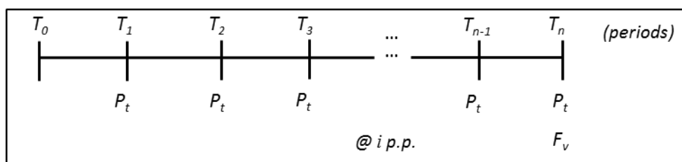
Fig. 12.2a Timeline for future value of an ordinary annuity (reproduced from Young (1993))
