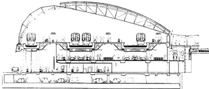
Figure 3.56: Waterloo Channel Tunnel Terminal - the top floor of a multi-storey building (Abbott, n.d.).
