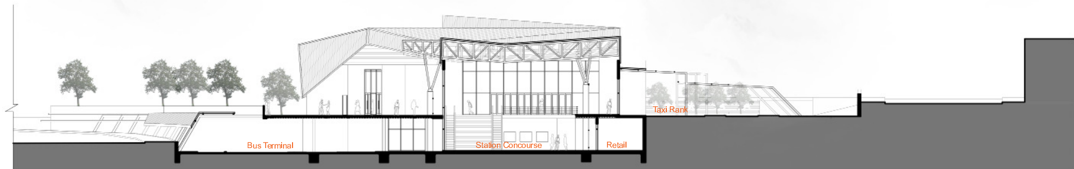
Section A-A not to scale
