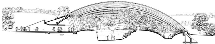
Figure 3.50: Great Glasshouse - Hollow portal constructed from circular-hollow-sections. (Foster & Partners, 2014).
