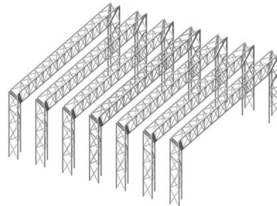
Figure 3.48: IBM Sports Hall- Built-up lattice , also IBM Sports Hall, Waterloo Channel Tunnel Terminal, and Leipzig Trade Fair Building (Boake & Hui, 2014).
