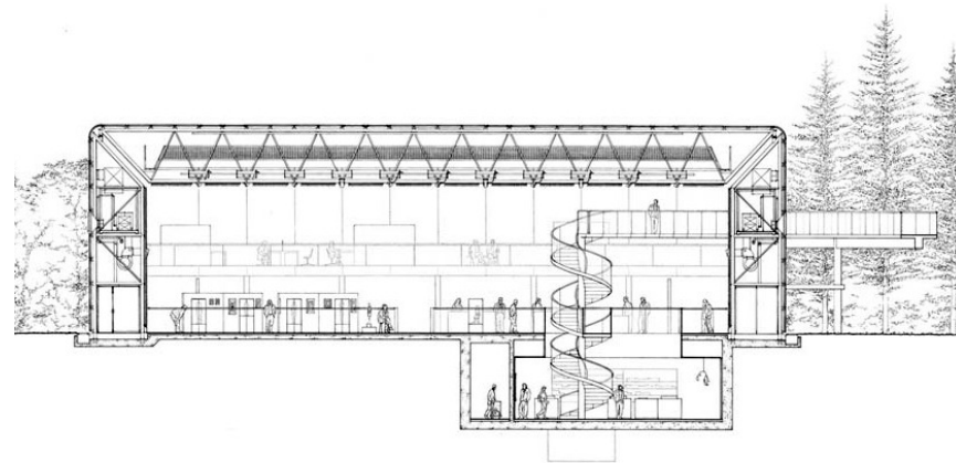
Figure 3.57: Sainsbury Centre - horizontal spanning member, also IBM Sports Hall (Foster & Partners, 2014)
