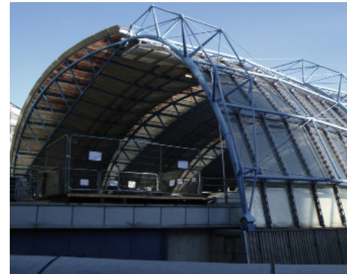
Figure 3.53: Waterloo Channel Tunnel Terminal - the portal frame is outside the building envelope, aslo IBM Sports Hall (Alex, n.d.).
