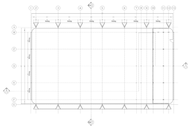
Figure 3.59: IBM Sports Hall- all the portal frames within the structural bay are normally of a similar size and span , resulting in rectangular plan forms. Also Sainsbury Centre, IBM-Sports Hall, and Leipzig Trade Fair Building (Nasrollahi, 2008).
