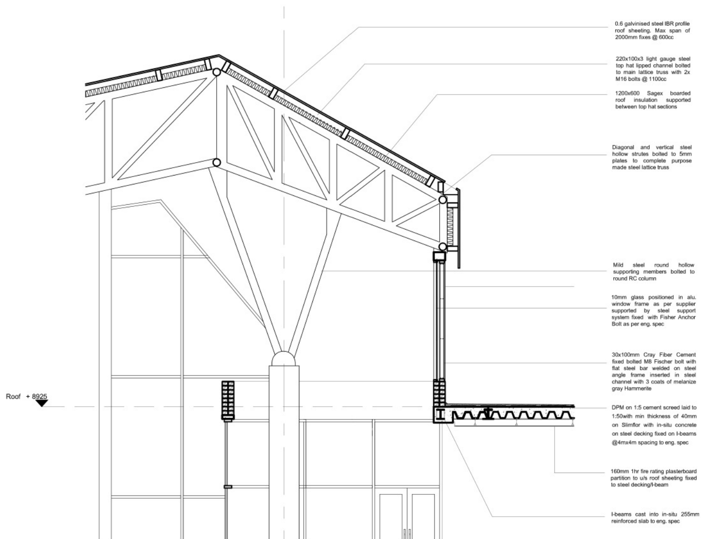
Detailed Section not to scale
