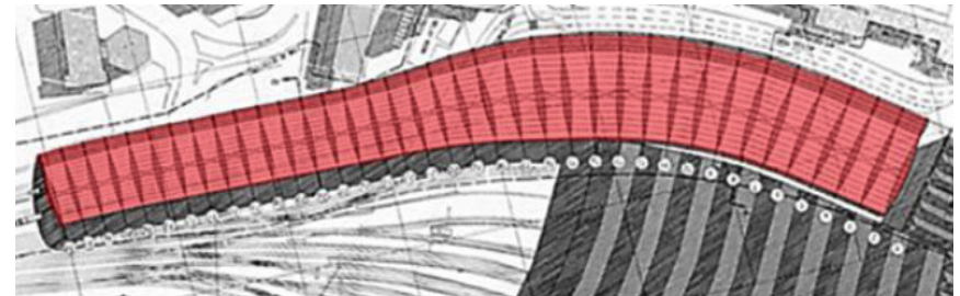
Figure 3.61: Waterloo Channel Tunnel Terminal - the asymmetrical 3 pin portal frame with variable sizes and spans (Steel: my, 2014)
