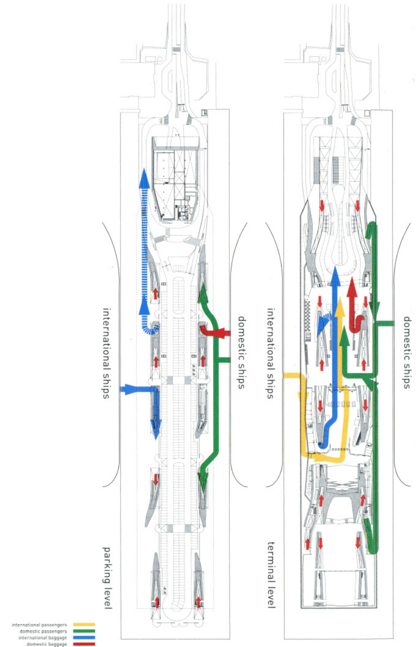
Figure 3.9: Terminal passenger and baggage circulation (Ferre, Sakamoto, Kubo, 2002: 264)
