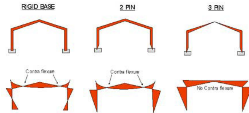
Figure 3.43: Three types of portal frame (Fitzgerald et. al, 2004).
