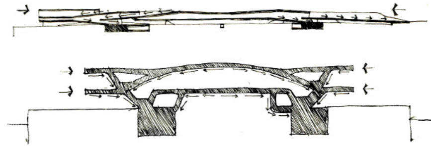
Figure 3.11: Transmission of lateral loads through surface (Ferre, Sakamoto, Kubo, 2002: 11)
