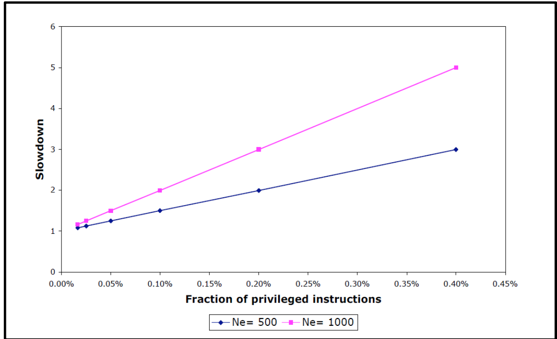
FIGURE 2.4: Execution Slowdown, taken from [27]
