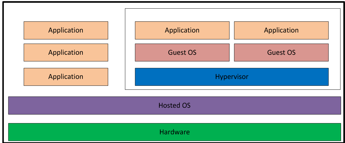
FIGURE 2.6: Full Virtualisation, Hosted [28]
