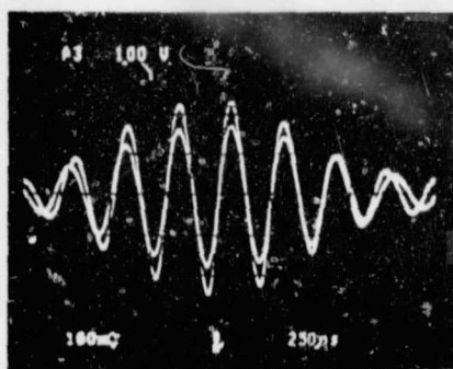
Fig. 3.2(c) Two echoes being overlapped (after Grigg et al., 1986)
