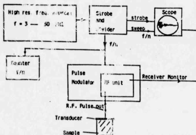
Fig. 3.1 The essential components of the pulse echo overlap system
