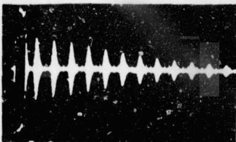
Fig. 3.2(a) A series of diminishing echoes after Schreiber et al., 1973)
