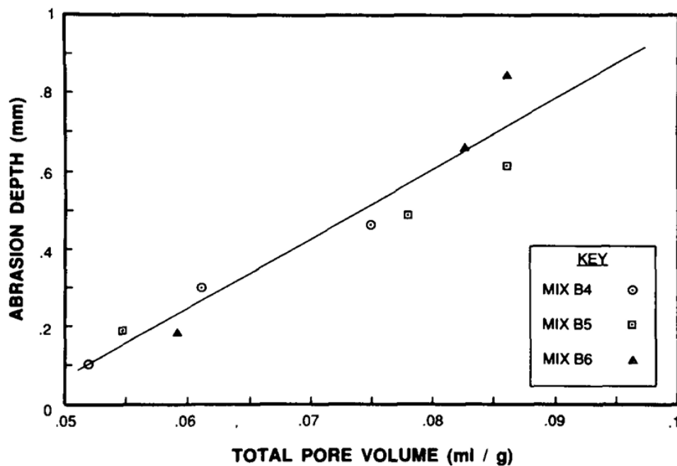
Figure 2.15: Influence of pore volume on the abrasion resistance performance of concrete, where the mix labels B4, B5 and B6 refer to the w/c ratios of 0.44, 0.54 and 0.65, respectively (Sadegzadeh, et al., 1987).
