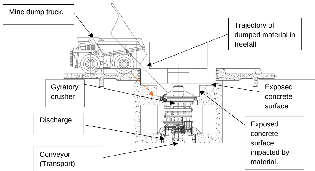
Figure 1.2: Typical bin elevation drawing showing RoM tip bin structure (Hayes, 2022).
