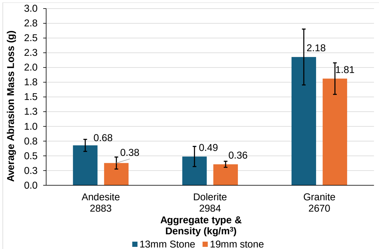
Figure 4.7: Abrasion mass loss comparison for various aggregate types and size at 28 days.
