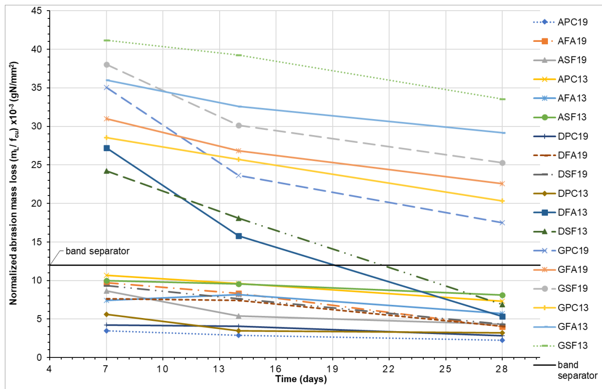
Figure 4.4: Normalized time dependent development of abrasion resistance.
