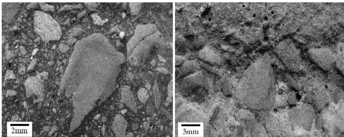
Figure 2.14: Abraded concrete surfaces with varying w/c ratios. 0.28 (left) and 0.36 (right) (Liu, et al., 2005).
