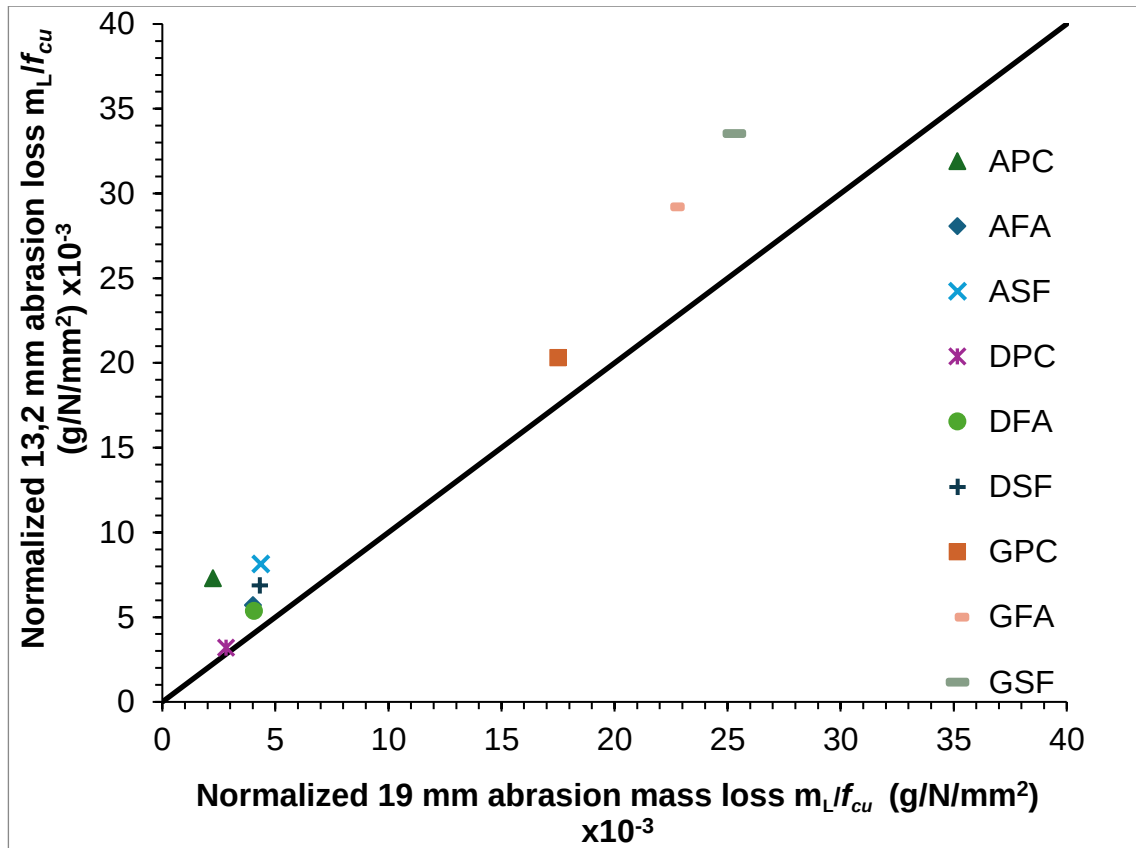
Figure 4.10: Effect of aggregate size on abrasion mass loss at 28 days for different aggregate types, normalized with strength.
