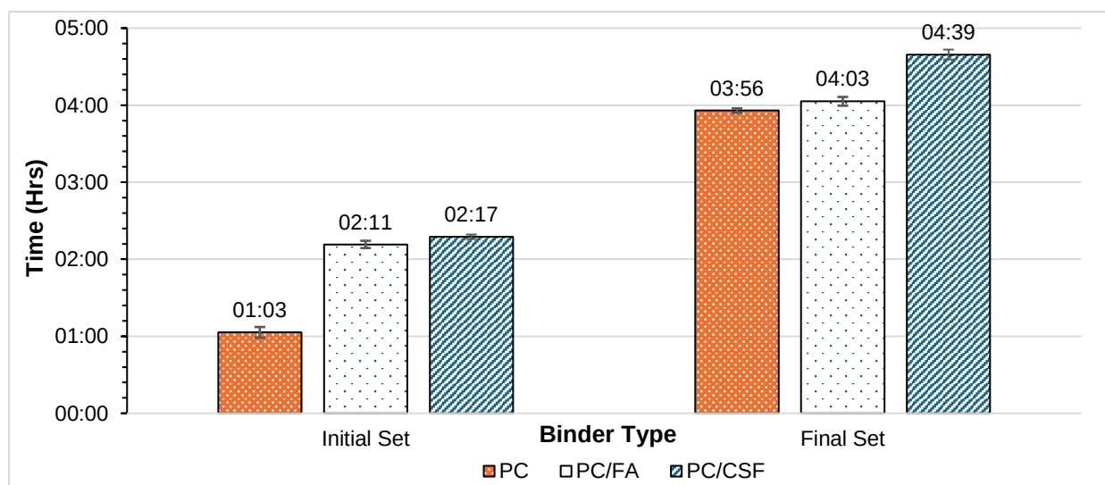
Figure 3.5: Average setting times for the various binder types.
