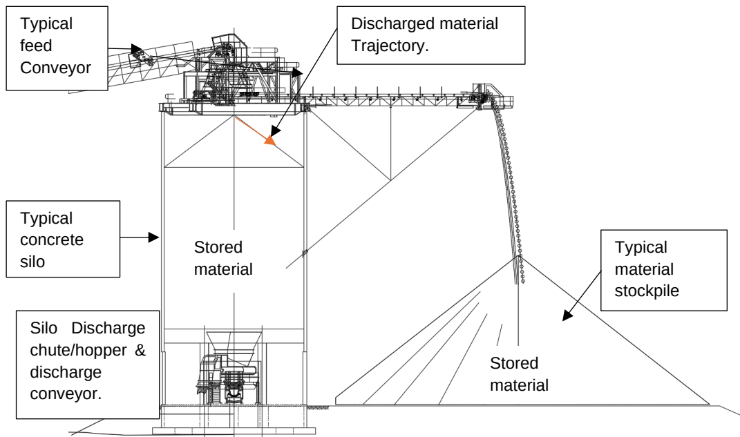
Figure 1.3: Diagram depicting typical ore material stores in minerals processing plants (Hayes, 2022).
