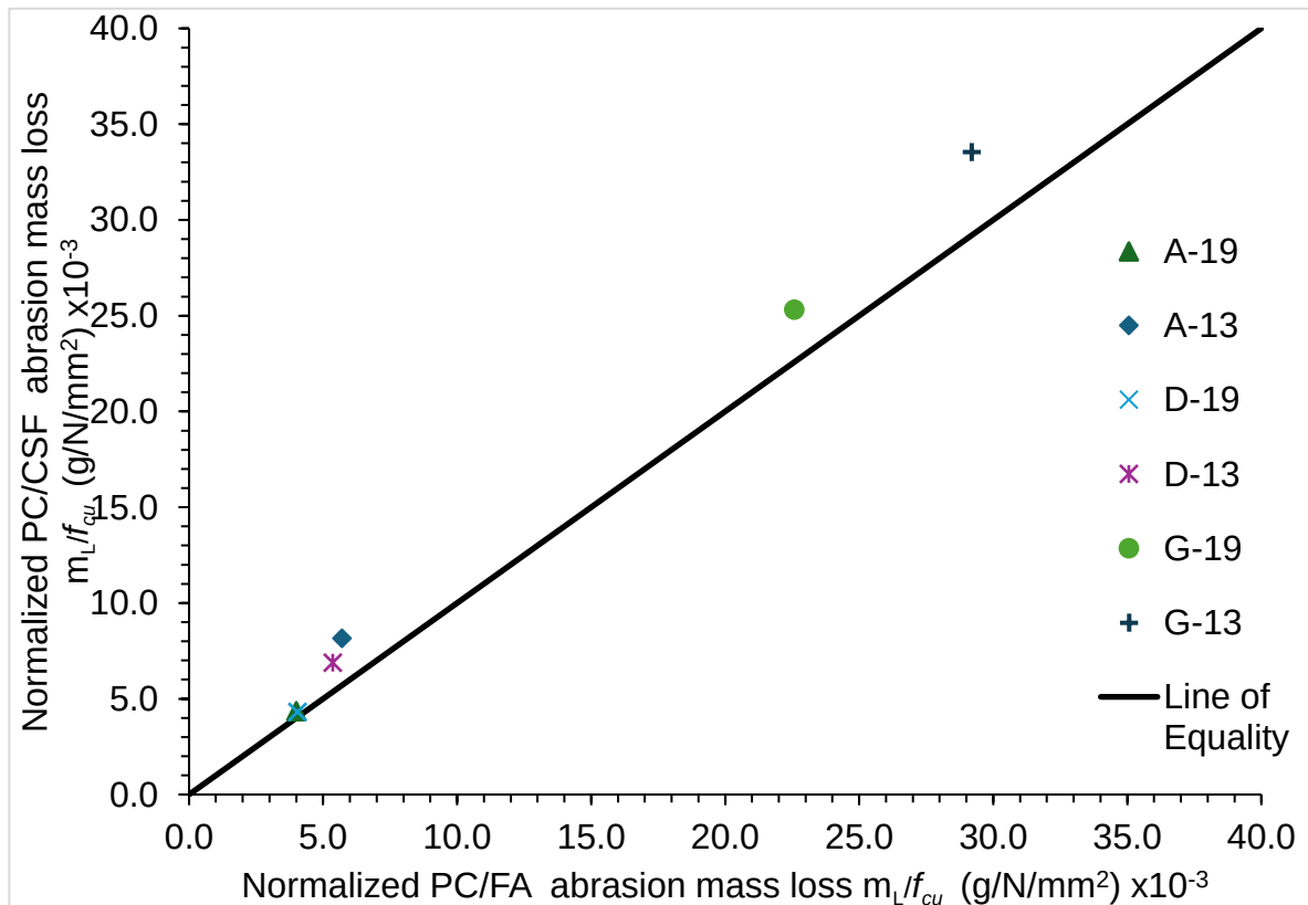
4.12 iii: Normalized PC/FA and PC/CSF abrasion mass loss comparison Figure 4.12: i, ii and iii Effect of binder type on abrasion mass loss at 28 days for different aggregate types and sizes, normalized with strength.
