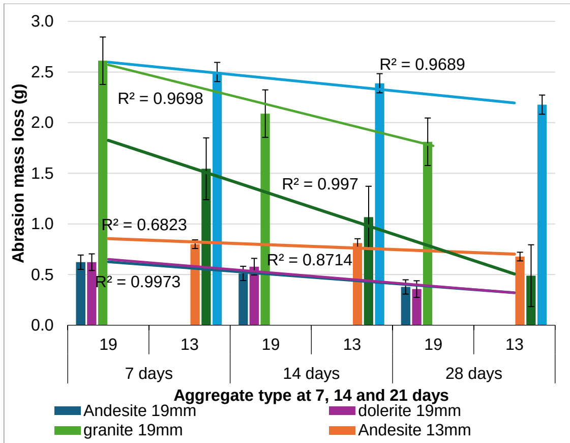
Figure B 8: Time development of abrasion mass loss with respect to aggregate type at 7, 14, and 28 days.
