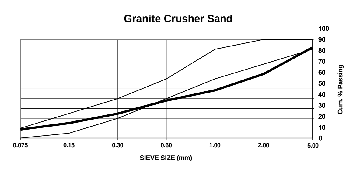
Figure D 10: Granite sand envelope range as per Specification: SANS 1083:2002
