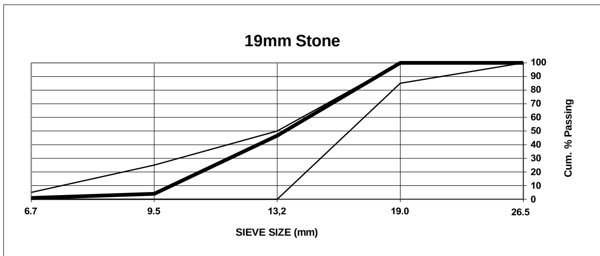
Figure D 7:19 mm norite envelope range as per Specification: SANS 1083:2002
