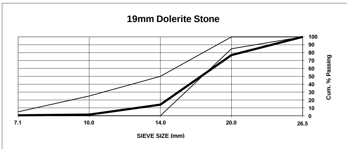
Figure D 2: 19 mm dolerite envelope range as per Specification: SANS 1083:2002
