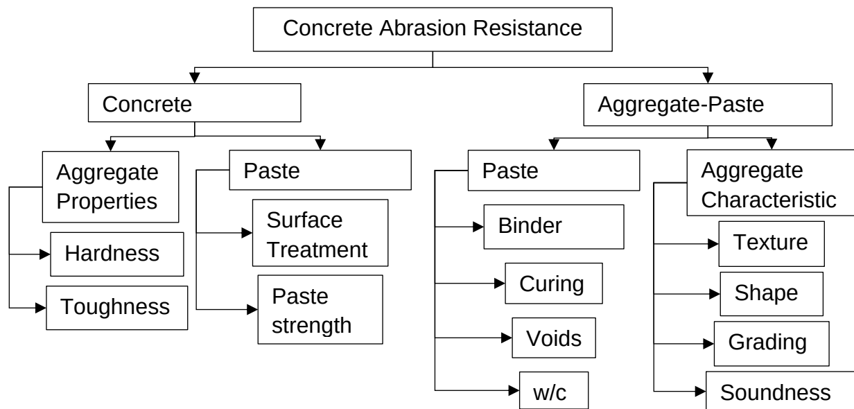
Figure 2.11: Factors affecting abrasion resistance of concrete (Papenfus, 2003).
