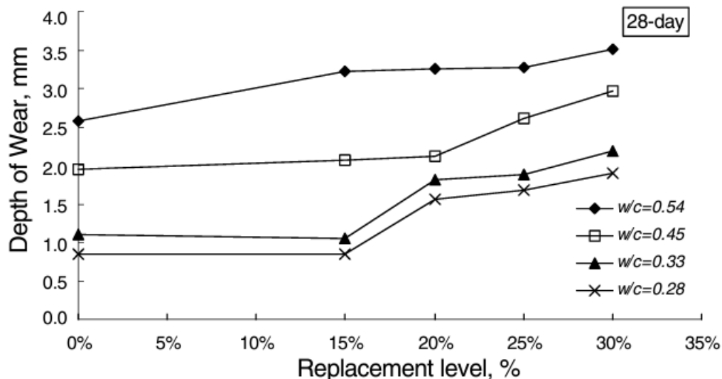
Figure 2.13: Effect of fly ash on the abrasion resistance of concrete at the age of 28 days (Yen, et al., 2007).
