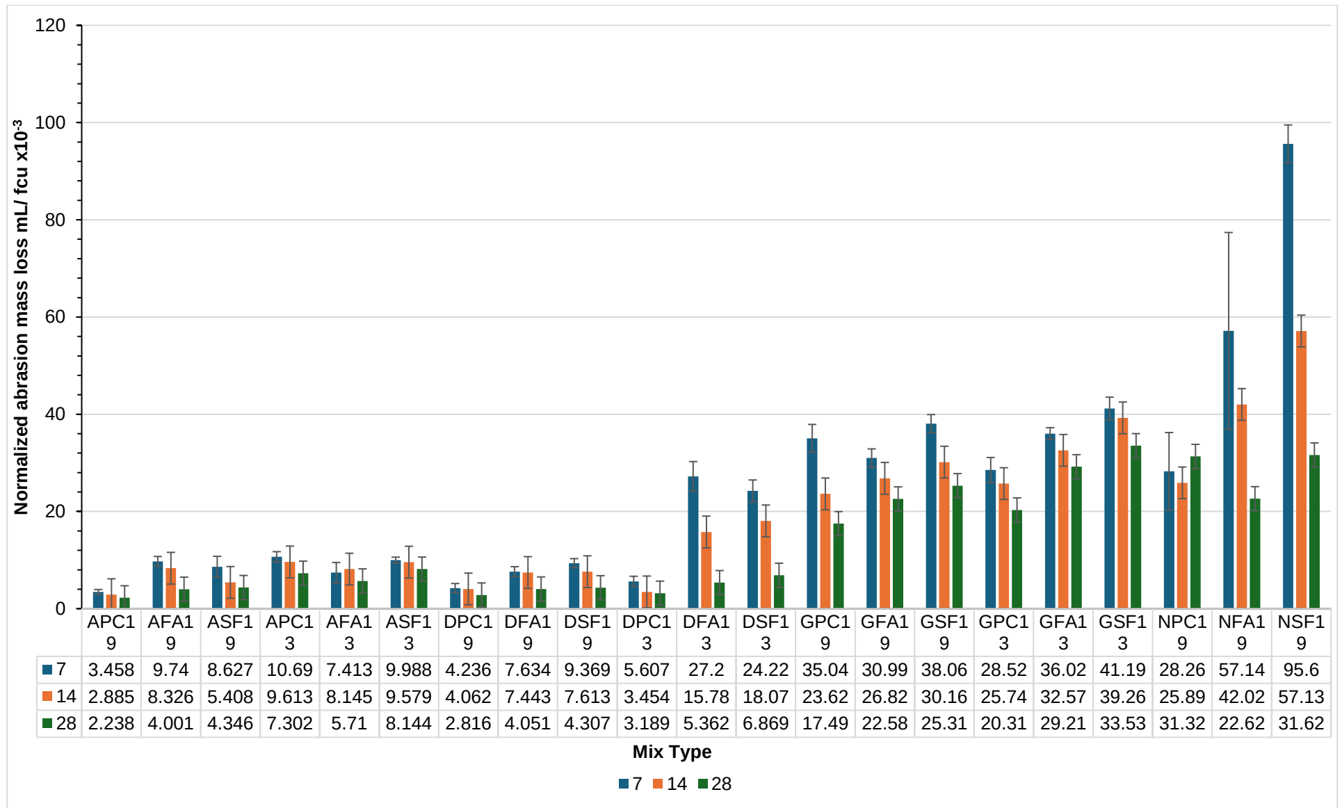
Figure B 2: Normalized graph of abrasion mass loss observed at 7,14, and 28 days for the various 21 mixes.
