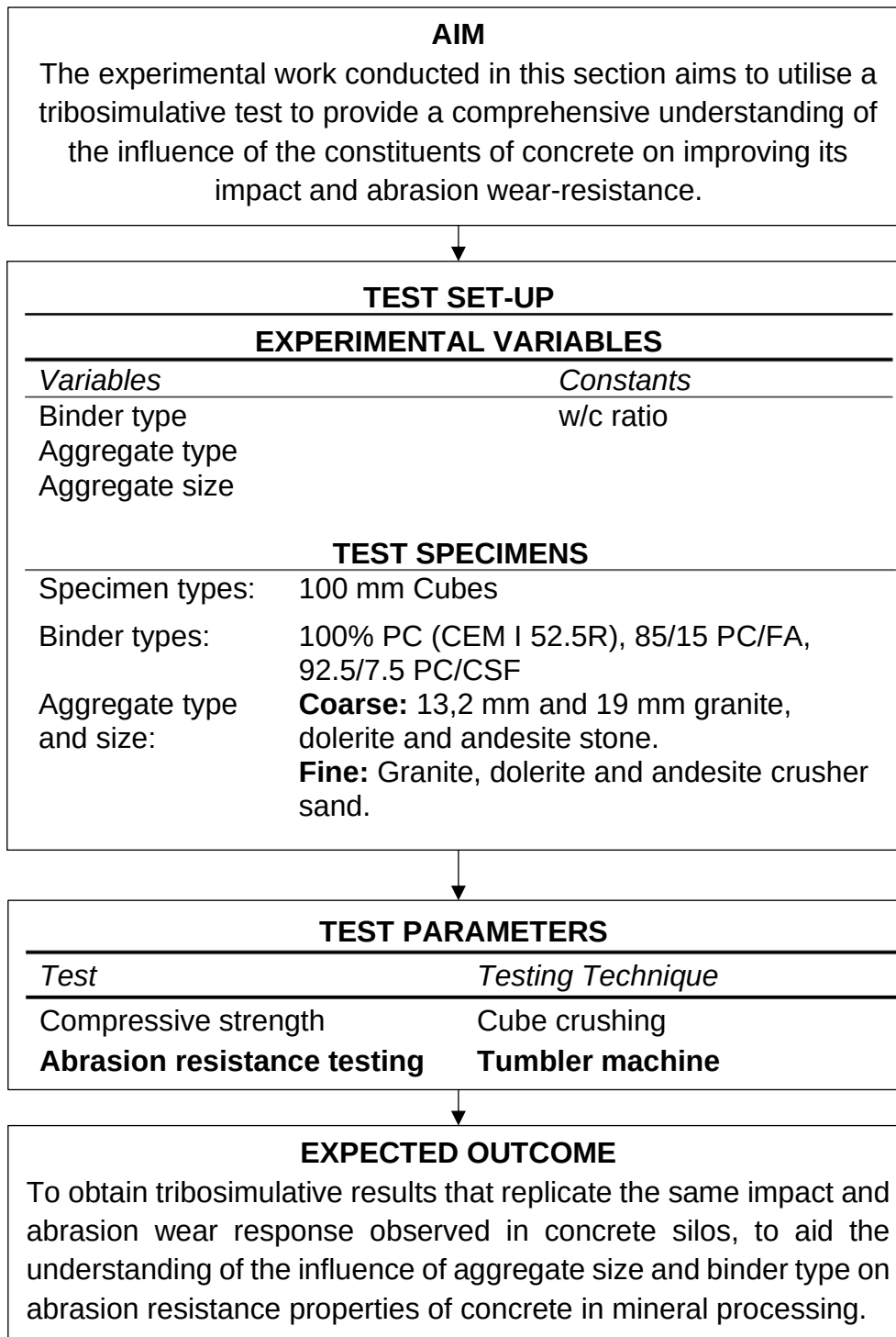
Figure 3.1: Experimental Methodology flow chart.
