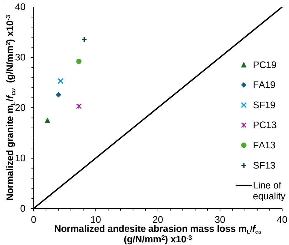
4.9 ii: Normalized andesite and granite abrasion mass loss comparison at 28 days
