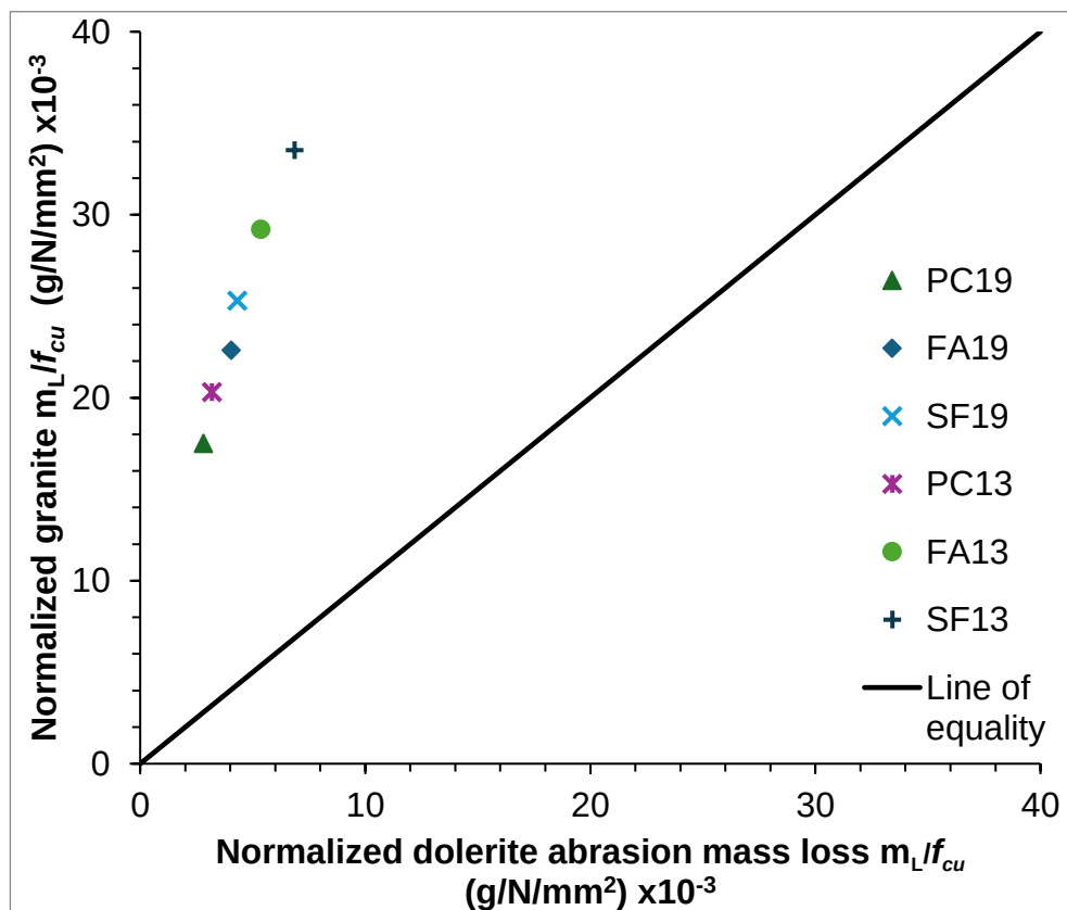
4.9 i: Normalized dolerite and granite abrasion mass loss comparison at 28 days
