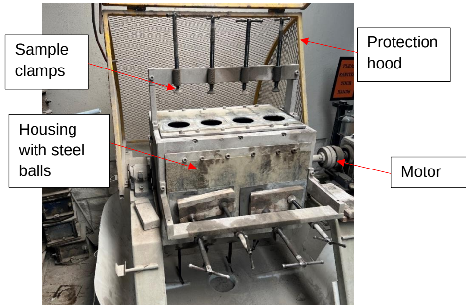
Figure 3.6 Tumbling abrasion test machine.
