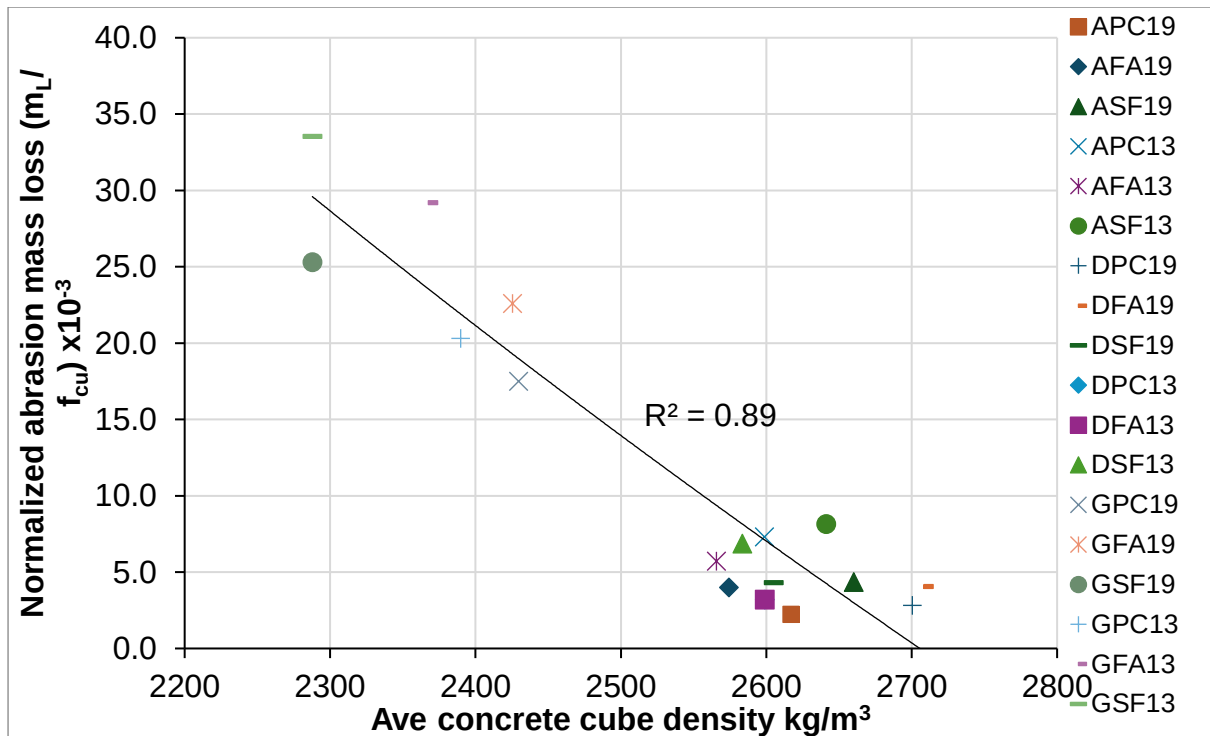
Figure B 6: Relationship between abrasion mass loss observed and 28-day average concrete cube density \text{kg/m}^3 .
