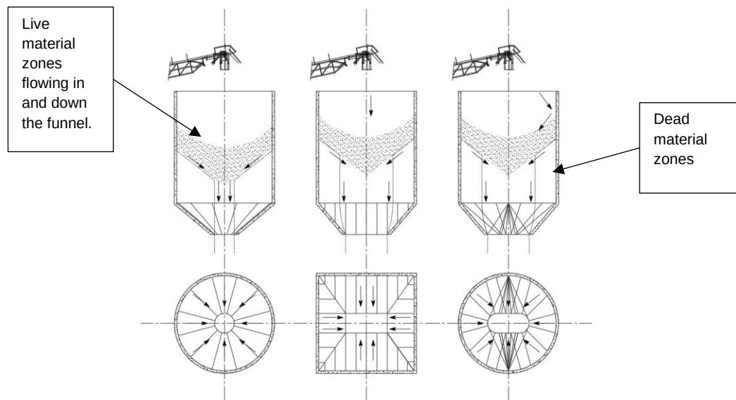
Figure 2.7: Diagram showing silo funnel flow with different discharge and hopper arrangements, recreated based on (Lobato, et al., 2016).
