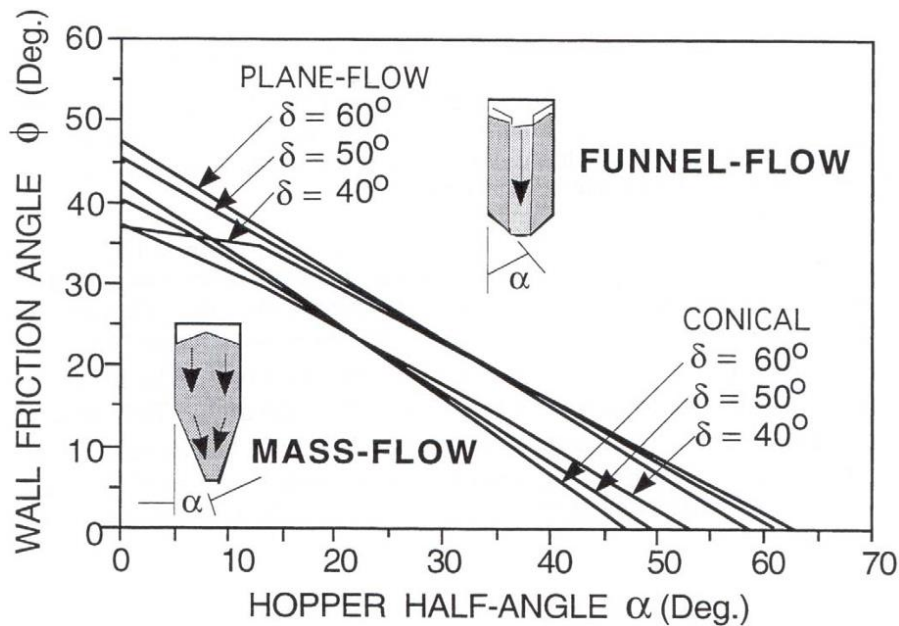
Figure 2.9: Limits for Mass-flow for Conical and Plane-Flow Channels (Roberts, 2009).
