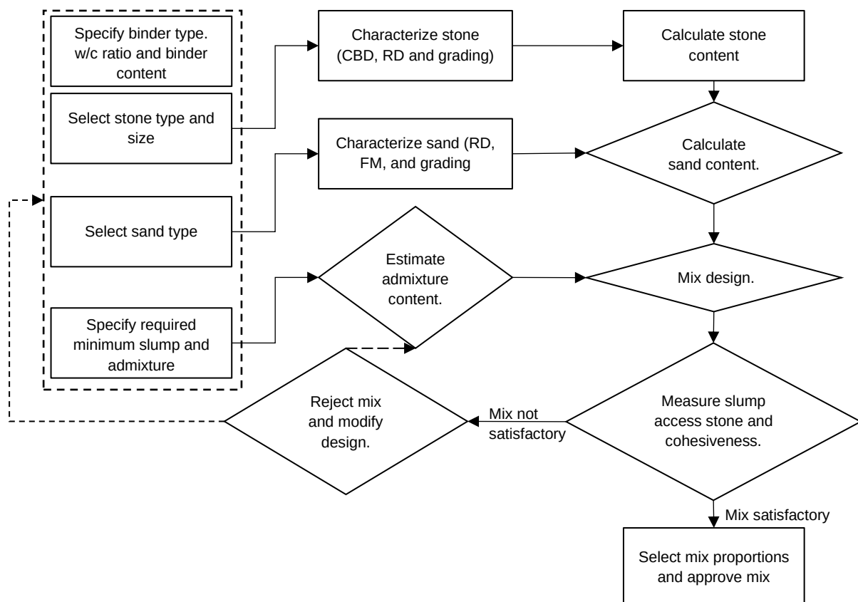
Figure 3.3: Concrete mix design flow adaptation (Addis and Goodman, 2009).
