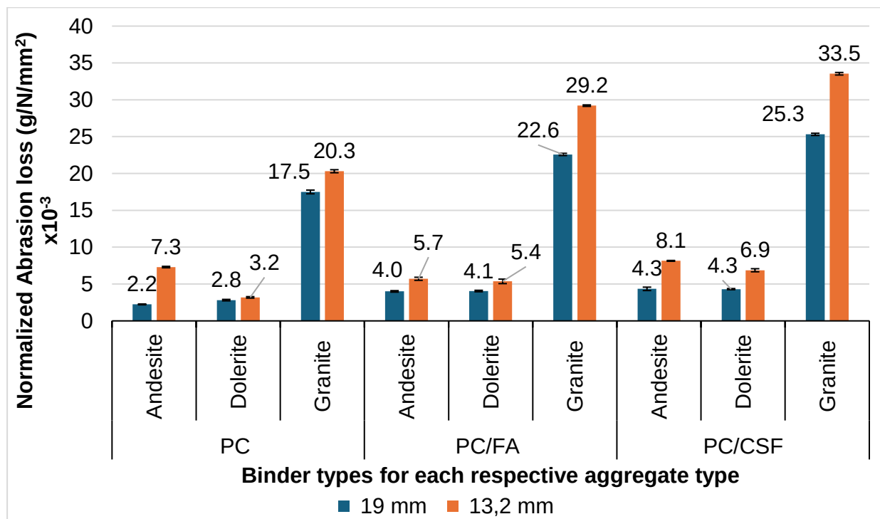
Figure 4.11: Effect of binder type on the average abrasion mass loss measured at 28 days, Normalized with compressive strength.
