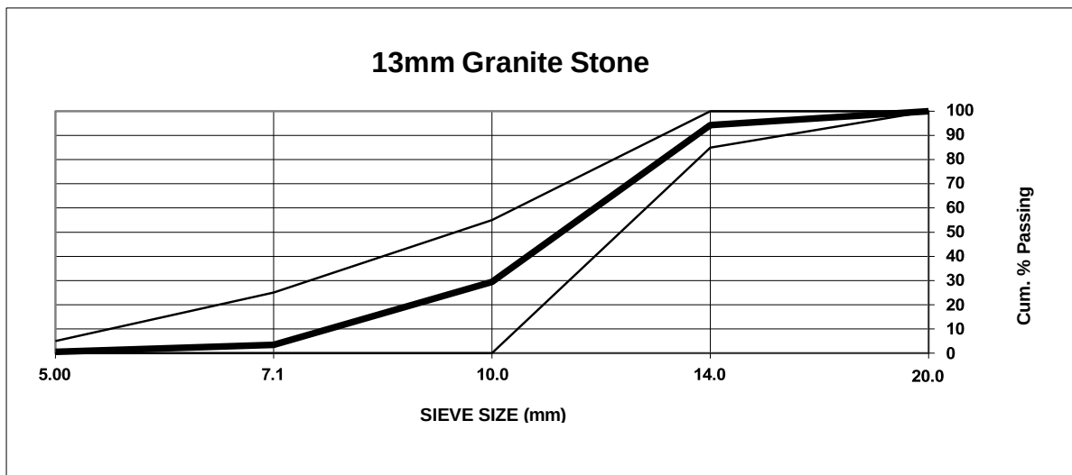
Figure D 6:13,2 mm granite envelope range as per Specification: SANS 1083:2002
