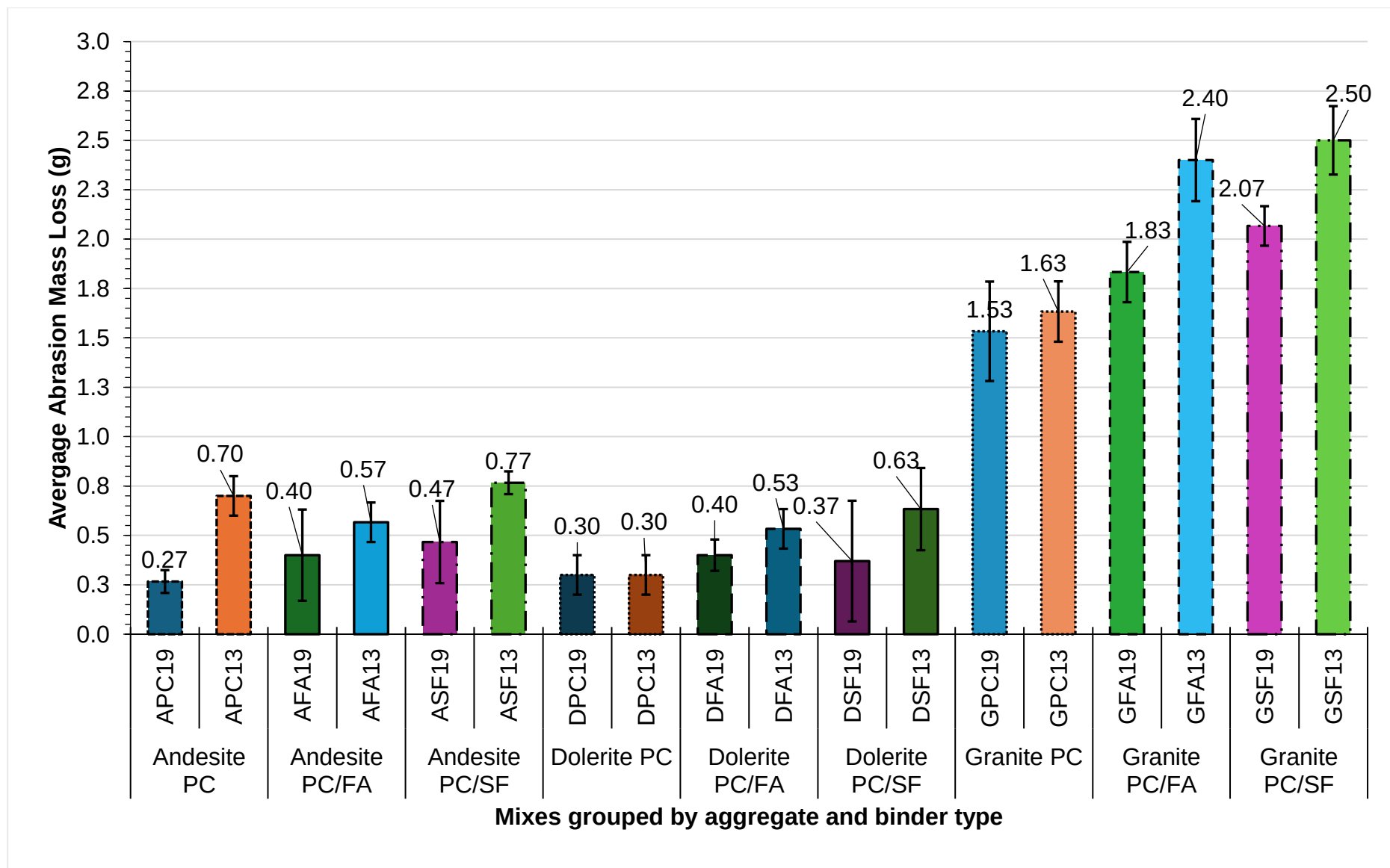
Figure B 5: 28-day comparison of the abrasion mass loss values for the various mixes grouped by aggregate and binder type.
