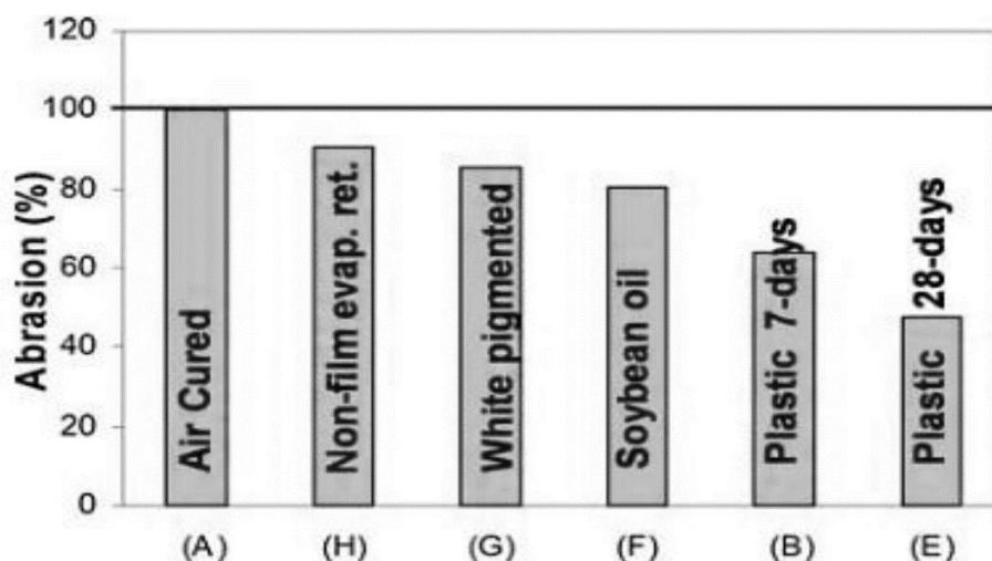
Figure 2.16: Effects of curing regime on concrete abrasion at 28 days (A to E indicates the curing regime) (Kevern, et al., 2009).
