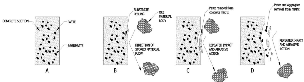
Figure 2.4: Adaptation of the sequence of abrading concrete surfaces. A: initial stage, B: concrete surface under abrasive action, C: loss of coarse aggregate and mortar from the concrete surface, and D: further loss of coarse aggregate and mortar from the concrete surface (Scott and Safiuddin, 2015).
