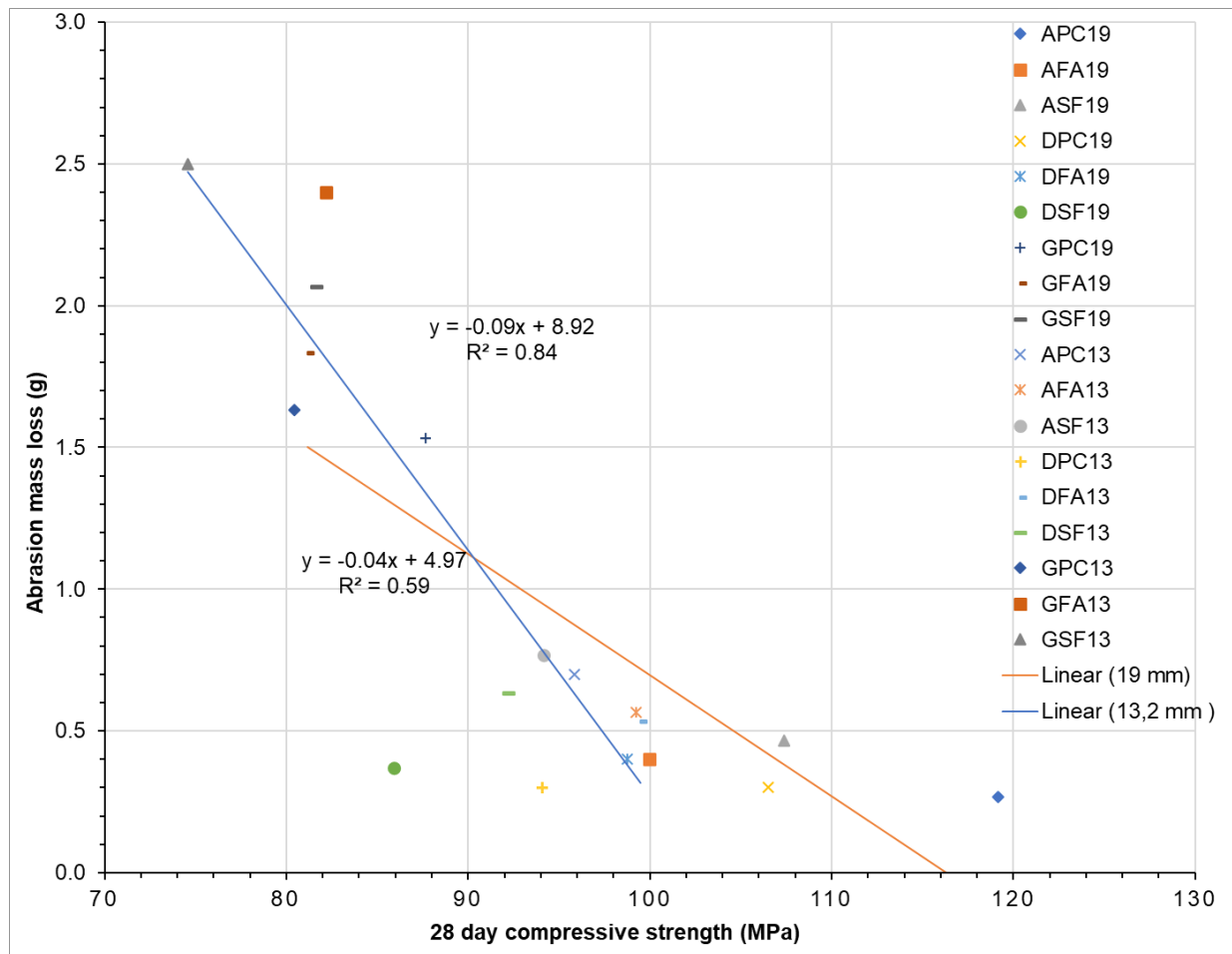
Figure 4.3: Comparison between compressive strength and abrasion resistance of concrete for both 13,2 and 19 mm aggregate mixes at 28 days.
