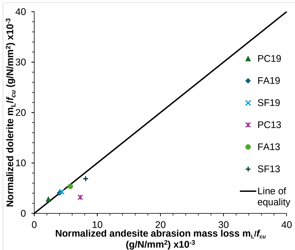
4.9 iii: Normalized andesite and dolerite abrasion mass loss comparison at 28 days Figure 4.9: Effect of aggregate type on abrasion mass loss at 28 days, normalized with compressive strength.
