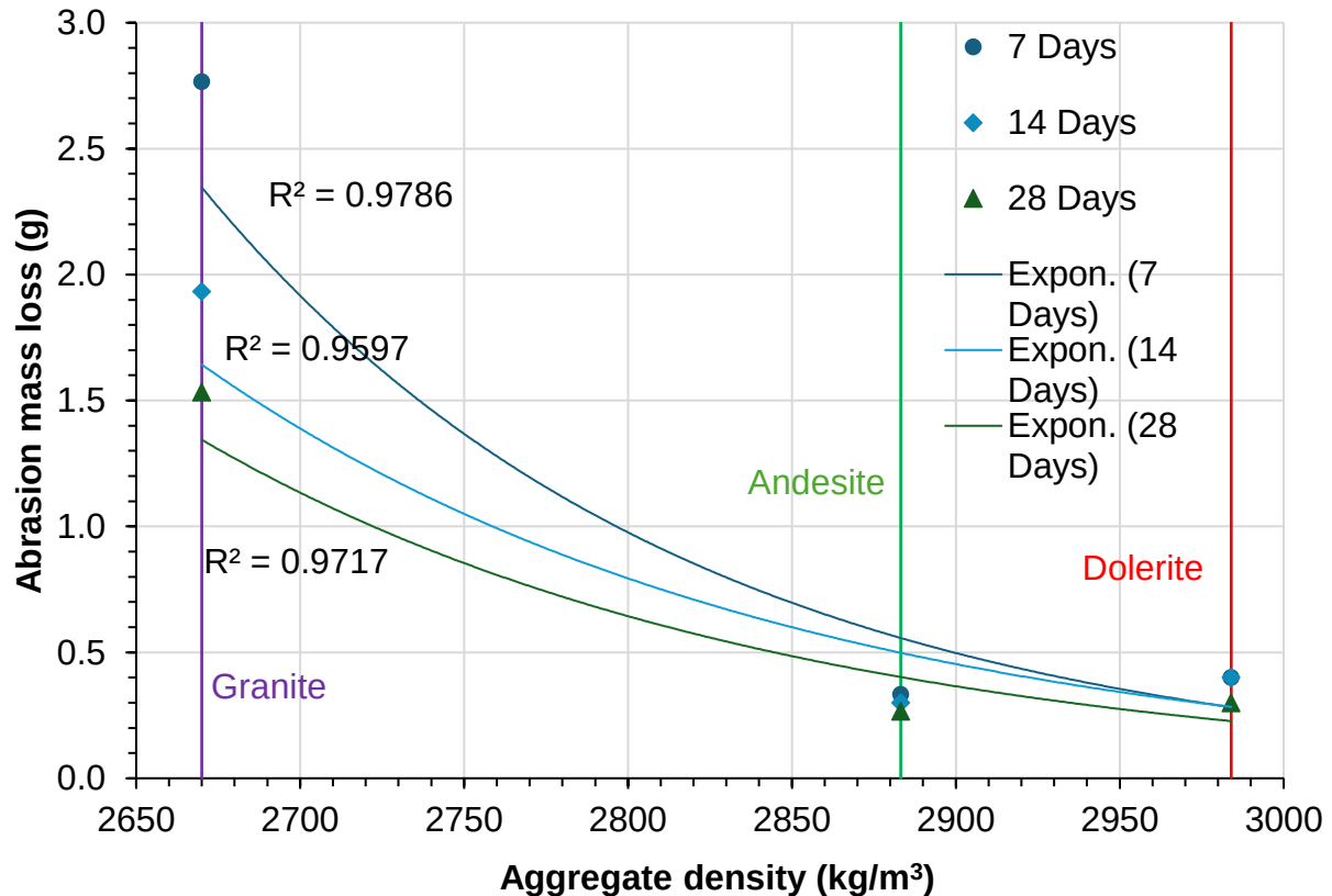
Figure 4.8: The abrasion mass loss measured at 7,14, and 28 days in relation to the aggregate densities of each respective aggregate type used to produce mixes with a 0.4 w/c ratio.
