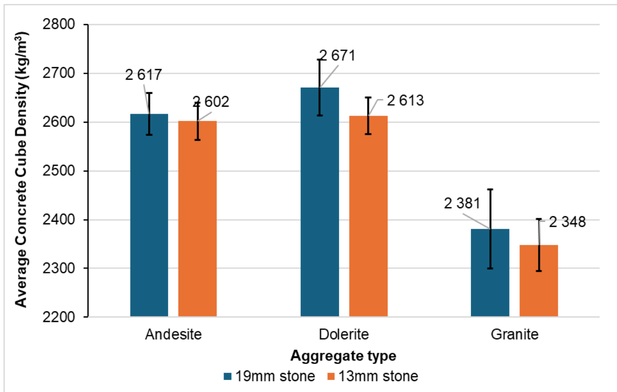
Figure 4.6: Comparison between aggregate type and average cube density at 28 days.
