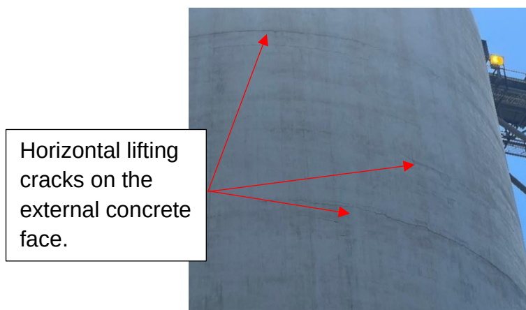
Figure 3.8: Picture of silo showing horizontal cracks on the external wall.
