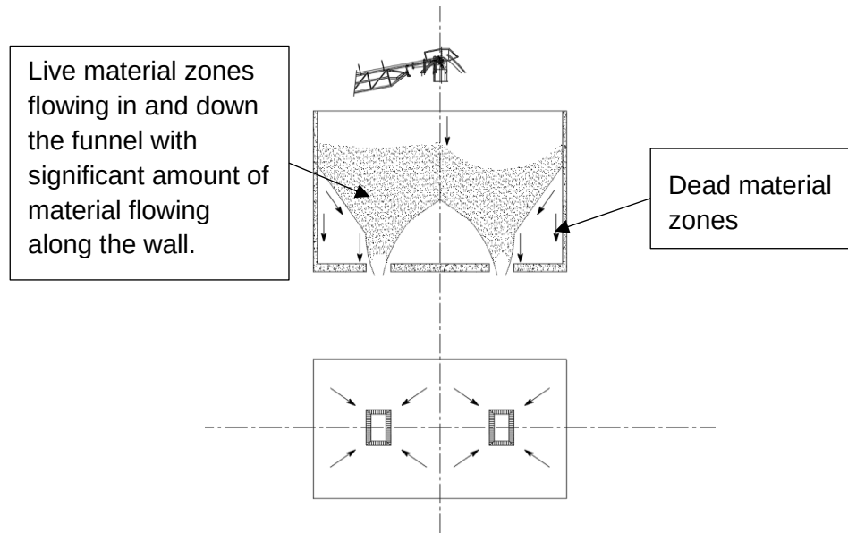
Figure 2.8: Diagram showing bin expanded flow, recreated based on (Schulze, 2021).
