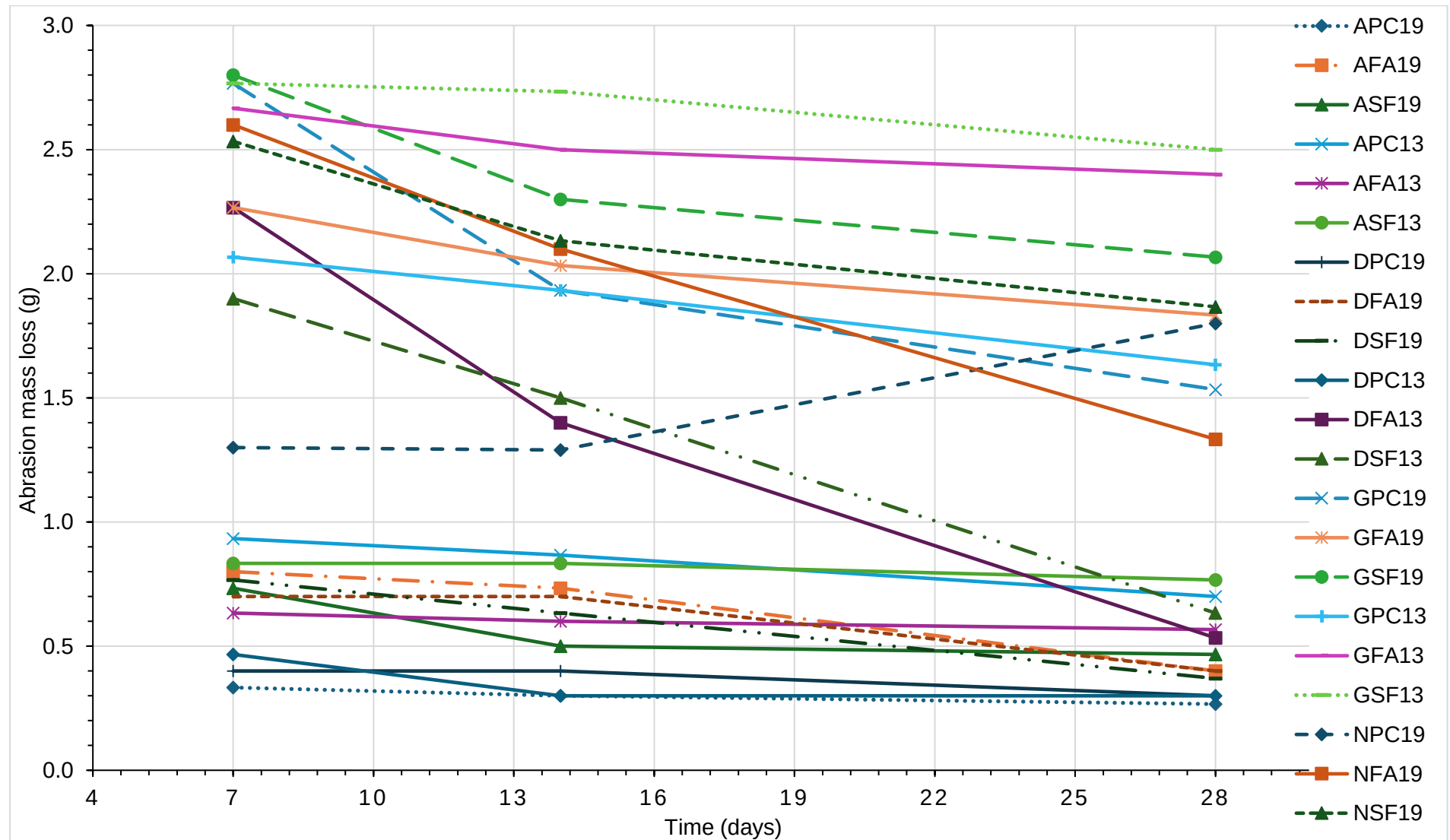
Figure B 1: 28-day time development of abrasion mass loss for the various mixes
