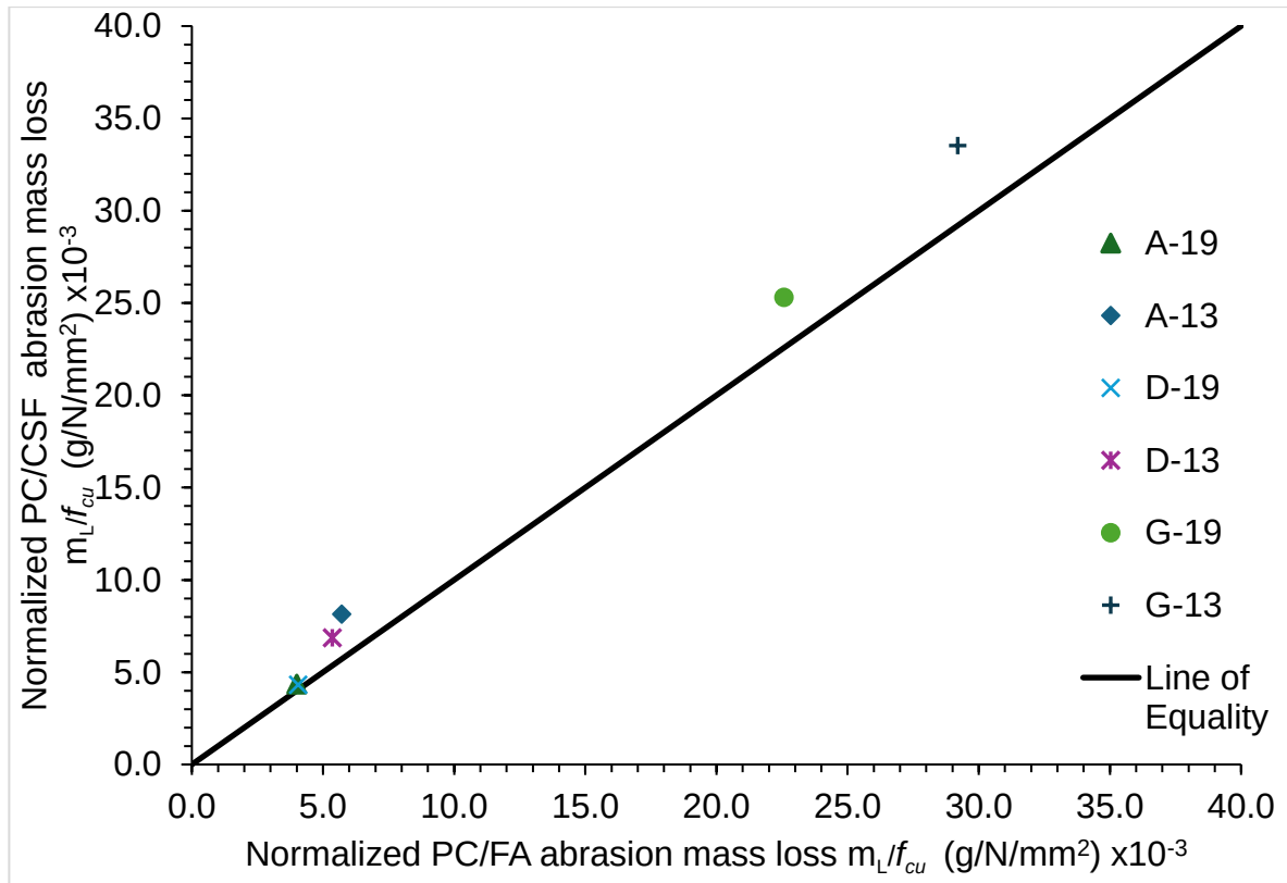
4.12 ii: Normalized PC and PC/CSF comparison
