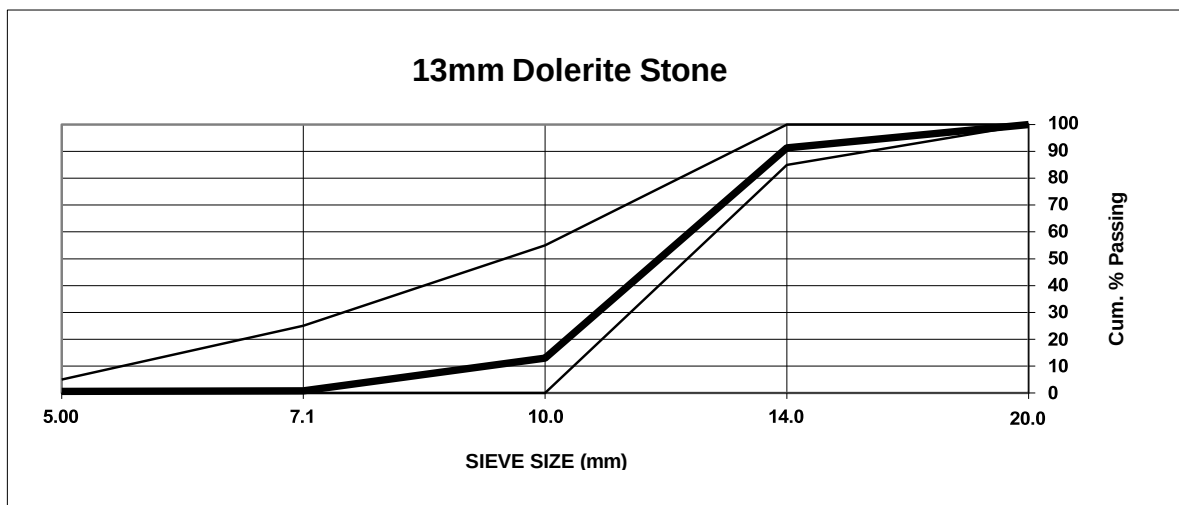
Figure D 5: 13,2 mm dolerite envelope range as per Specification: SANS 1083:2002
