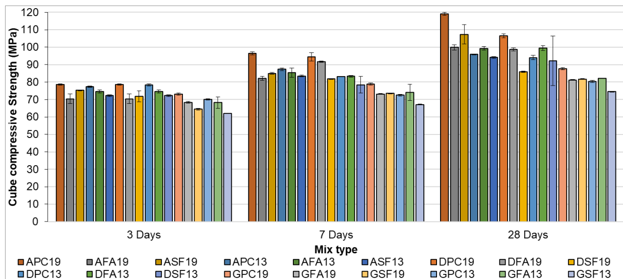
Figure 4.1: Average 3-, 7- and 28-day compressive strengths for all 18 concrete mixes.
