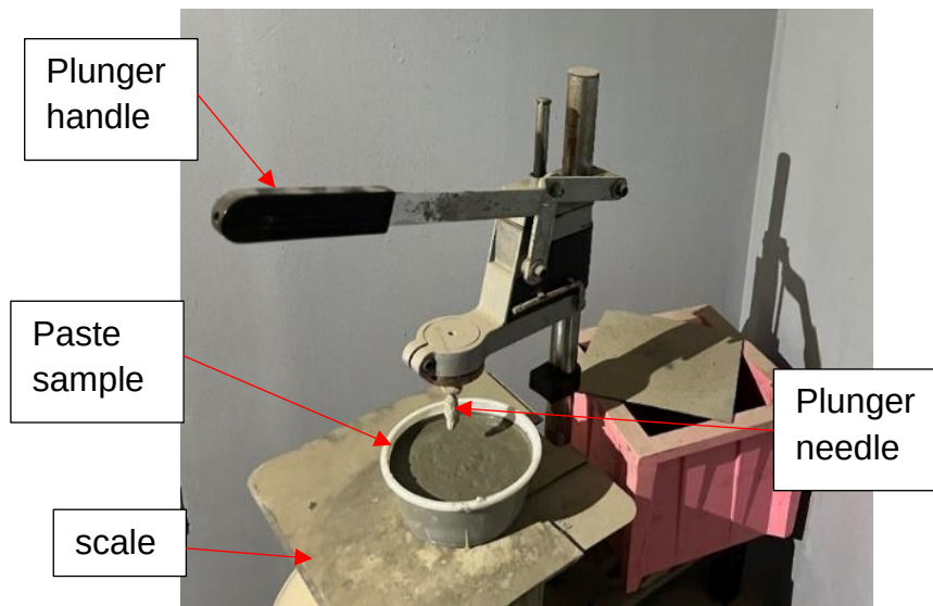
Figure 3.4: Vicat Setting time test apparatus.
