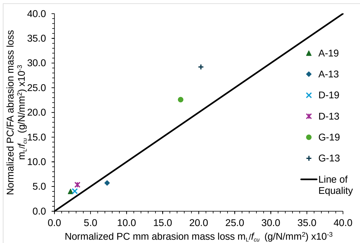
4.12 i: Normalized PC and PC/FA Comparison
