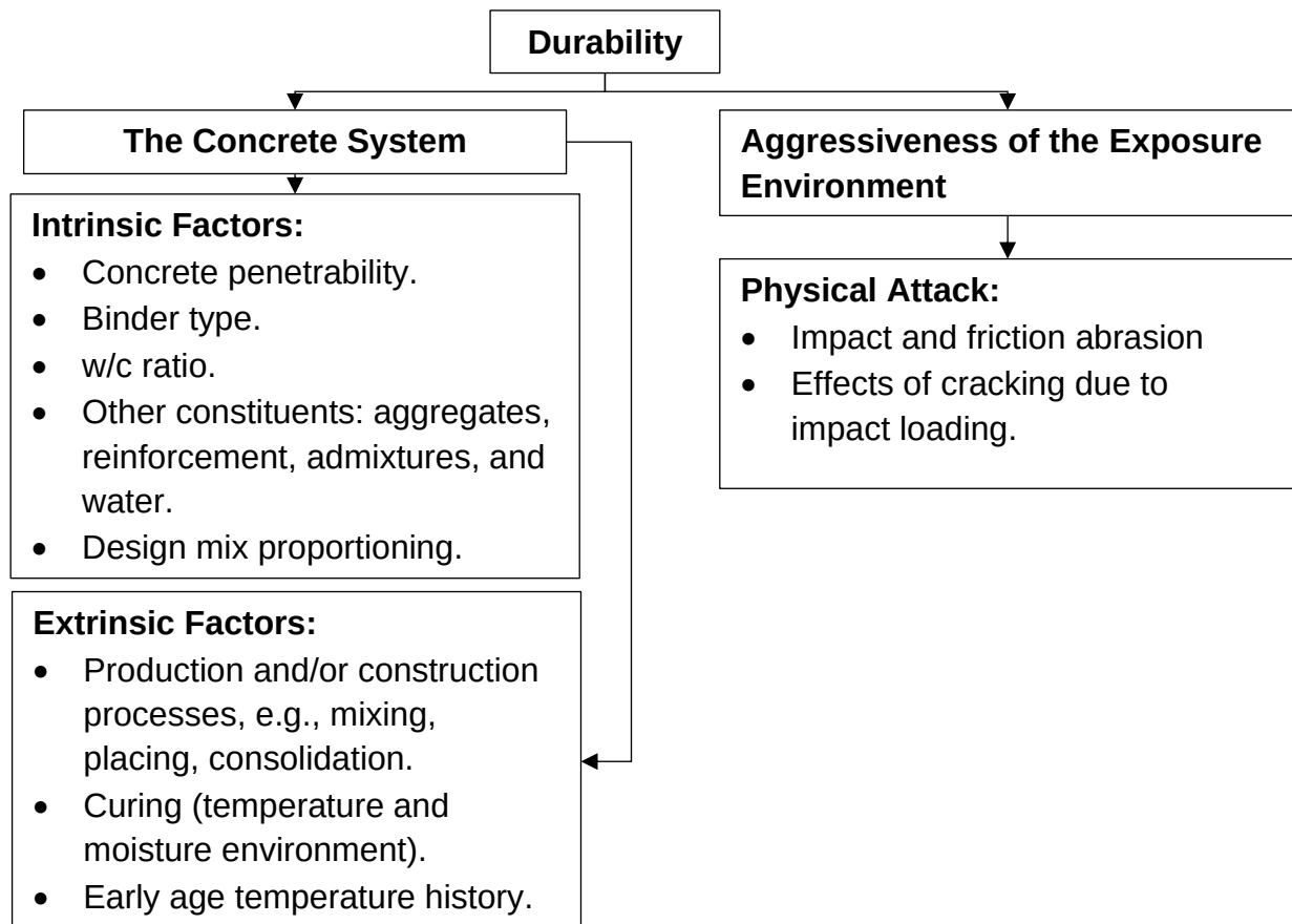
Figure 2.1: An adaptation of the concrete intrinsic, extrinsic, and environmental factors influencing the durability by (Beushausen, et al., 2021a).
