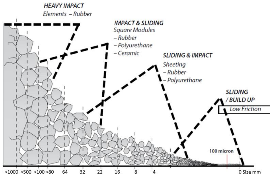
Figure 2.3: Diagram showing tribological contact types experienced by equipment liners for different material gradation (Metso, 2011).
