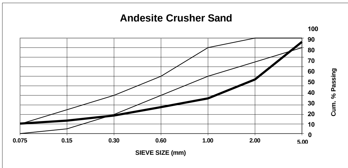
Figure D 8: Andesite sand envelope range as per Specification: SANS 1083:2002
