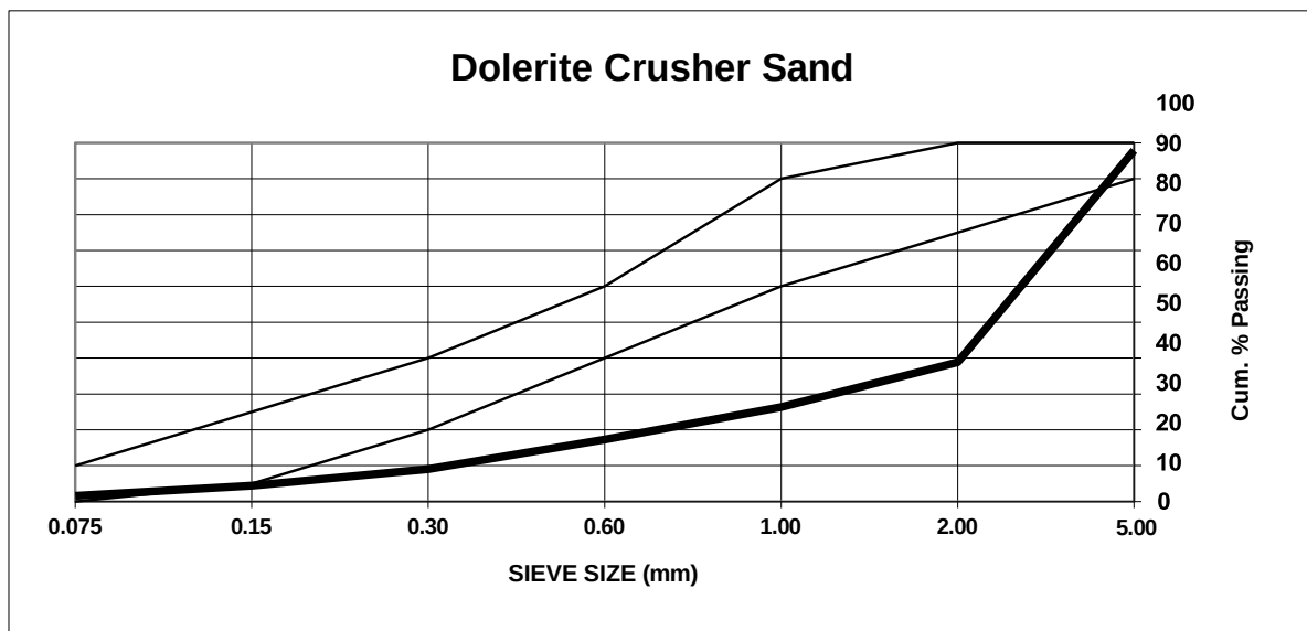
Figure D 9: Dolerite sand envelope range as per Specification: SANS 1083:2002
