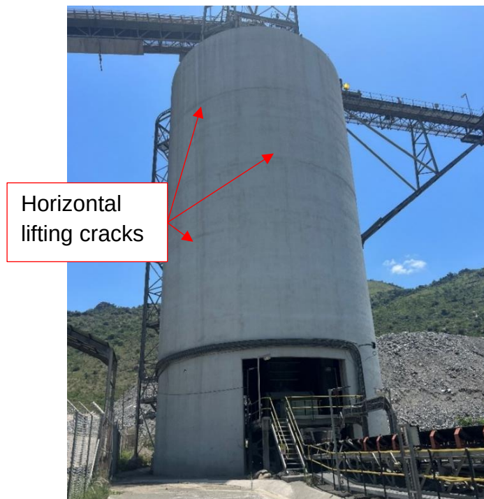
Figure 3.7: Picture showing the eastern external face TRP UG2 RoM silo.
