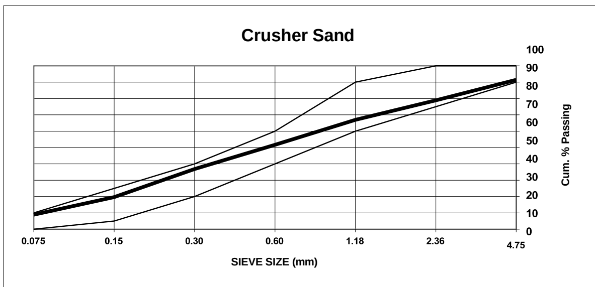
Figure D 11: Norite sand envelope range as per Specification: SANS 1083:2002
