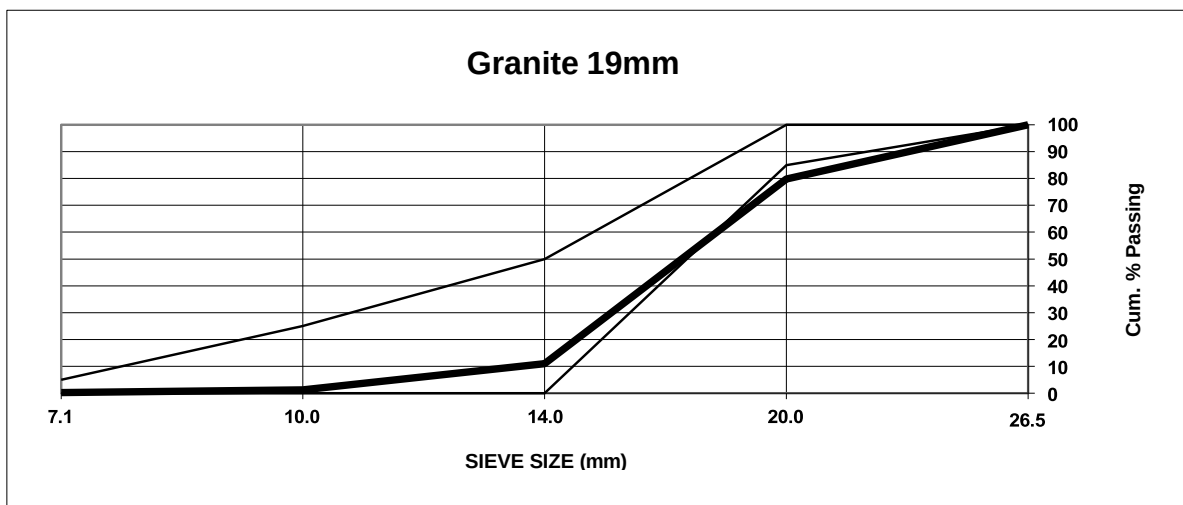
Figure D 3: 19 mm granite envelope range as per Specification: SANS 1083:2002
