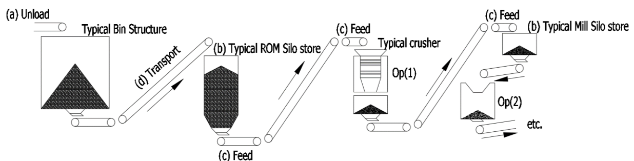
Figure 1.1: Diagram showing a process flow for dry materials handling: (a) Unloading and unloading, (b) Storage, (c) Feed, (d) Transport (Metso, 2011).
