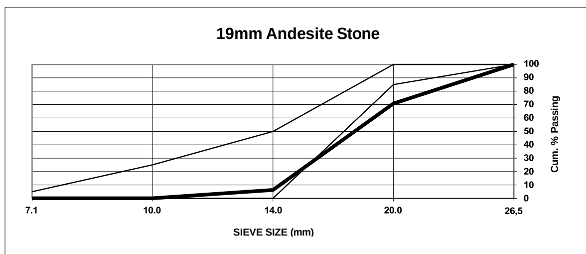
Figure D 1: 19 mm andesite envelope range as per Specification: SANS 1083:2002
