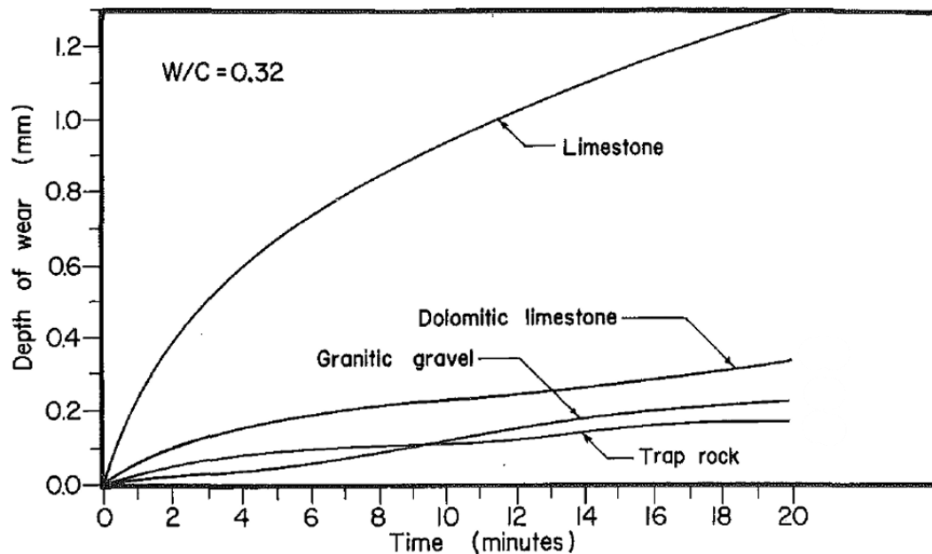
Figure 2.12: Abrasion wear of concrete with various aggregate types adapted from (Laplante, et al., 1991).
