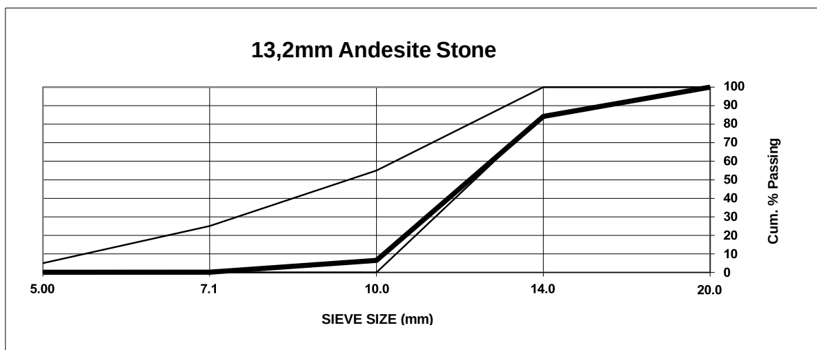
Figure D 4: 13,2 mm andesite envelope range as per Specification: SANS 1083:2002
