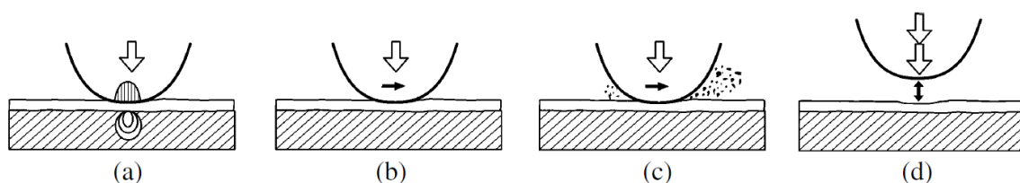
Figure 2.2: Various contact conditions in tribological applications (a) contact stresses at normal load; (b) sliding; (c) abrasion; (d) impact (Holmberg and Matthews, 2006).
