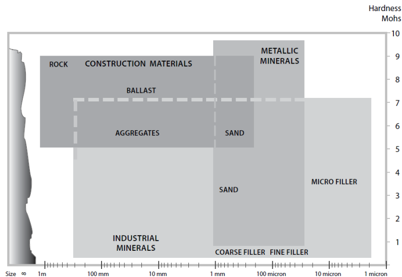
Figure 2.5: Diagram showing the relationship between size and hardness of different materials (Metso, 2011).
