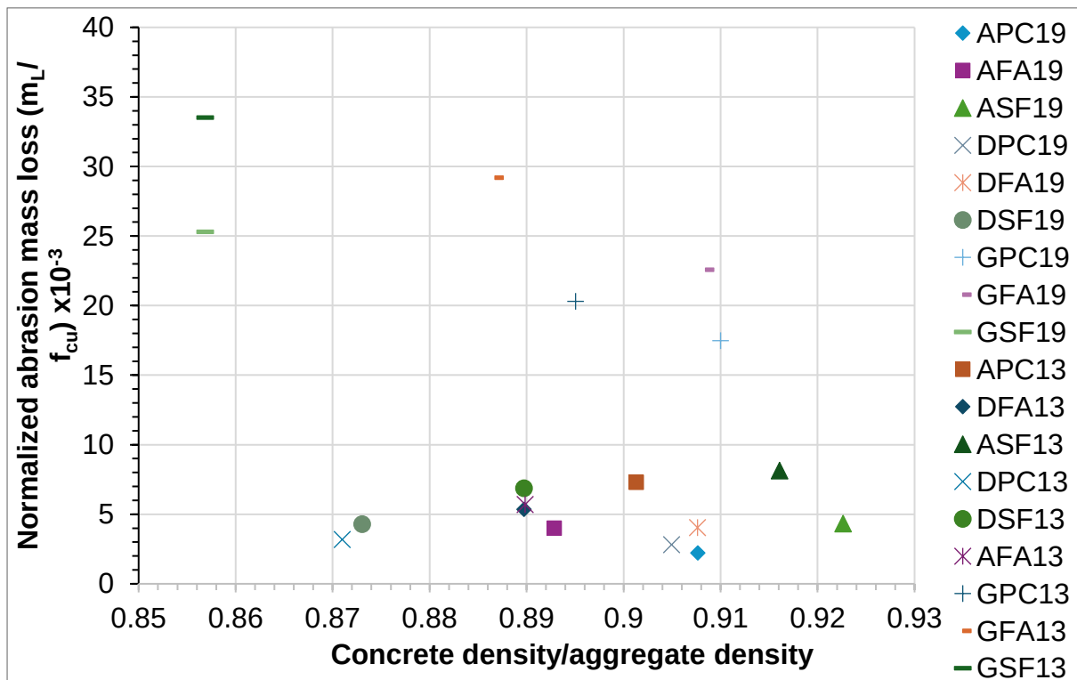
Figure B 7: Graph showing relationship between abrasion mass loss and concrete density, normalized with both compressive strength and concrete density respectively.
