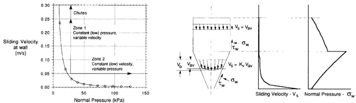
Figure 2.10 : Velocity versus pressure characteristics (left), and bin wear parameters and profiles (right) (Roberts and Wiche, 1993).
