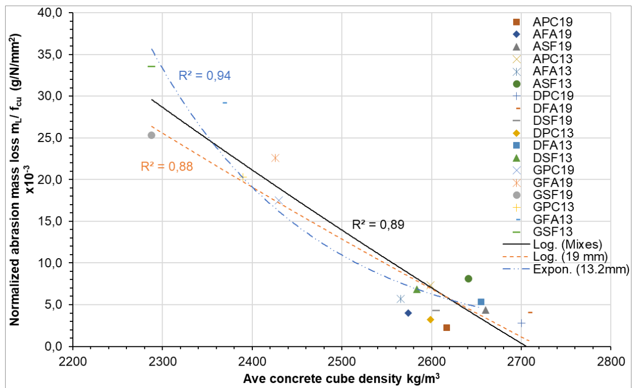
Figure 4.5: Normalized comparison of average concrete density and abrasion mass loss.
