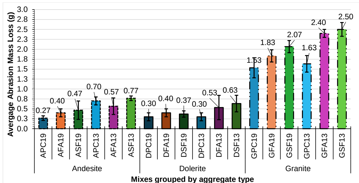
Figure 4.2: 28-day comparison of the abrasion mass loss values for the various mixes.
