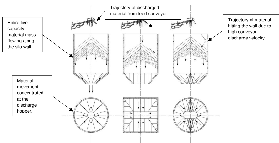
Figure 2.6: Diagram showing silo mass flow with different discharge and hopper arrangements, recreated based on (Roberts, 2009).
