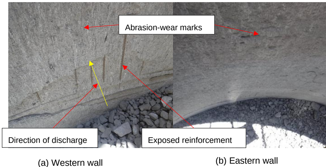
Figure 3.9:RoM silo internal wall (a) Western wall - wall adjacent to the discharge, (b) Eastern wall - on the side behind the discharge chute.
