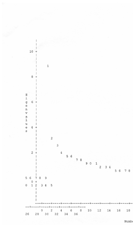
Diagram 4.2: Scree Plot showing Eigenvalues as represented by Five Factors
