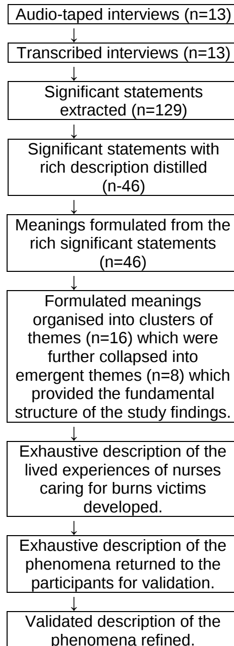
Figure 3.1 Schematic Summary of the Data Analysis
