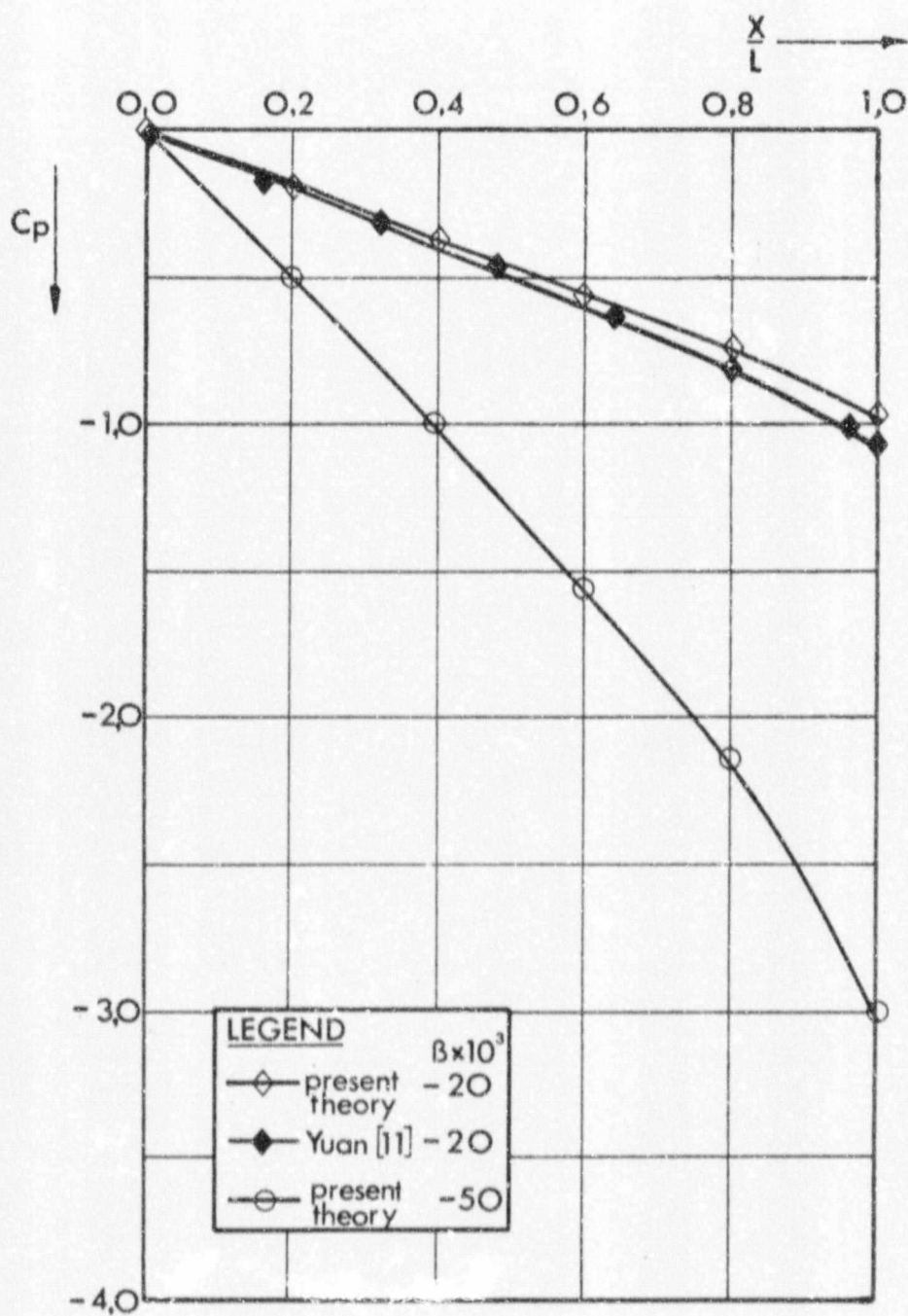
Fig 6.28 - Comparison between two theories of pressure drop with blowing
