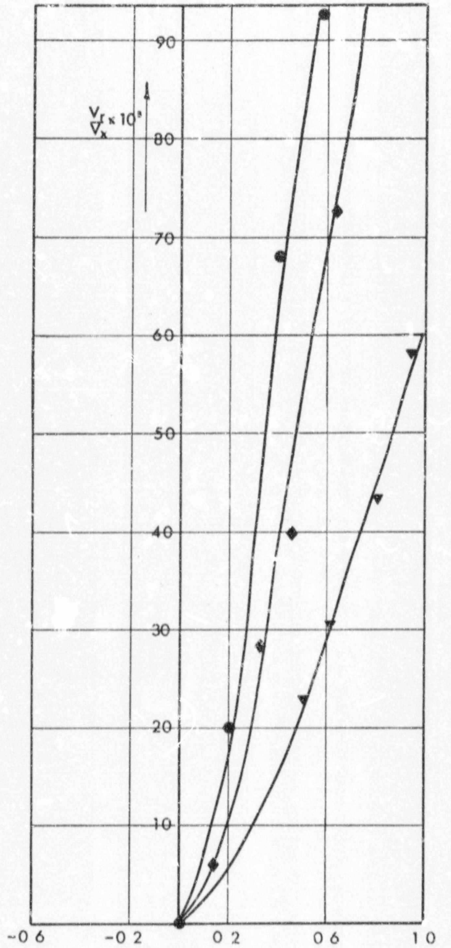
Fig 6.24 - Experimental variations of radial velocity across the pipe \frac{r}{R} \longrightarrow
