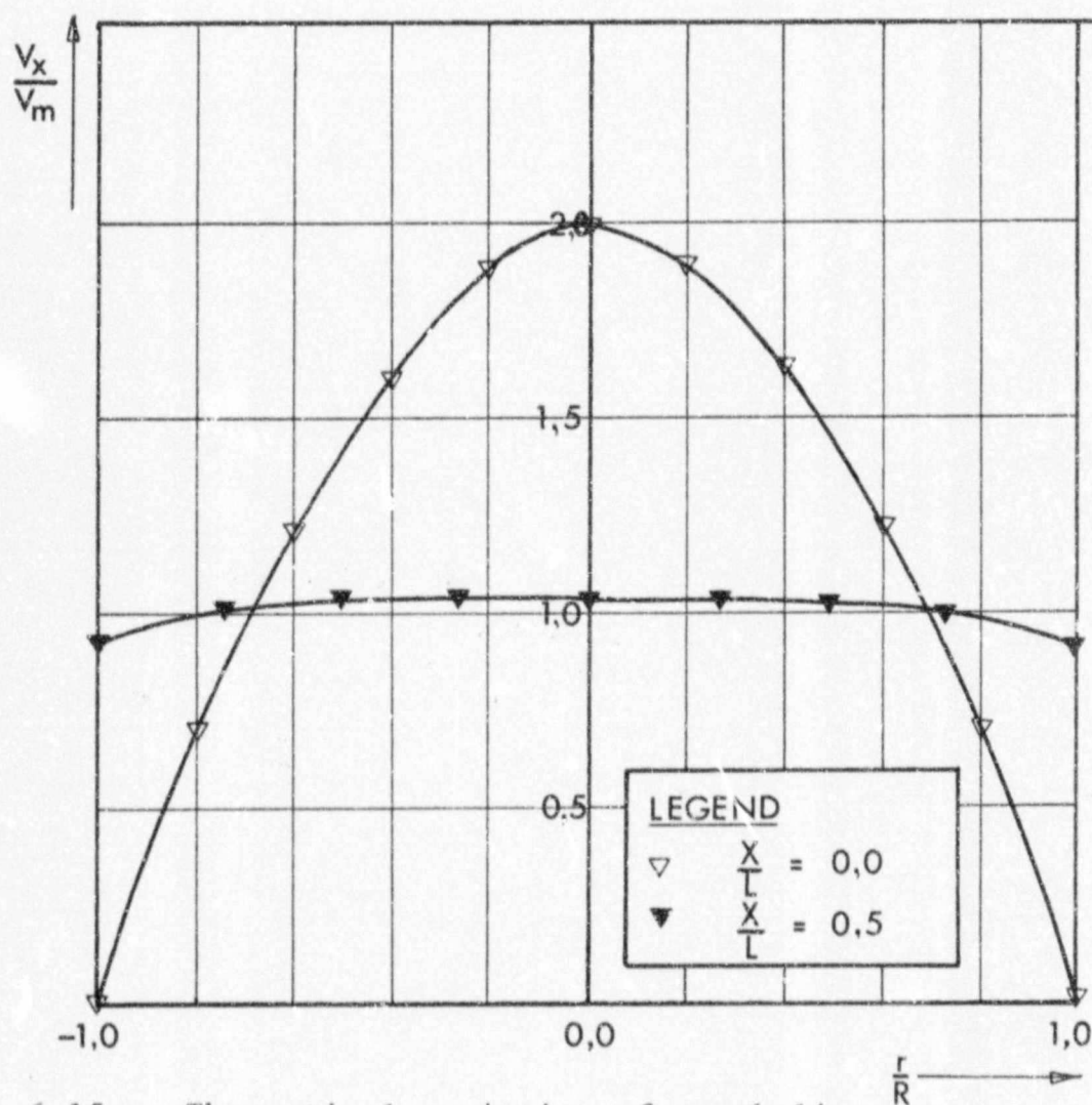
Fig 6.15 - Theoretical variation of parabolic velocity profile with suction
