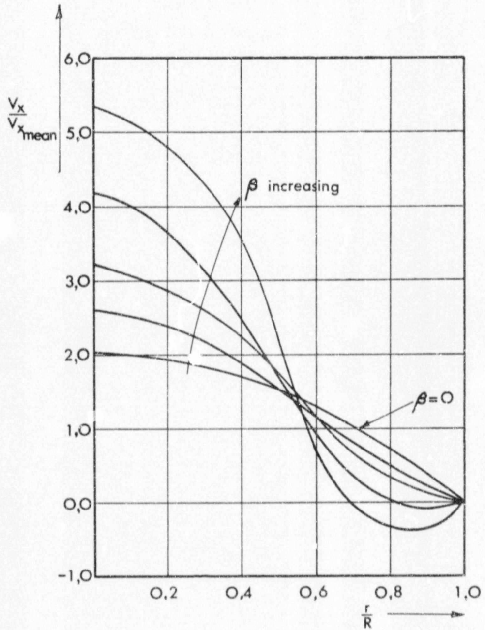
Fig 6.30 - Typical velocity profiles obtained from similarity solutions
