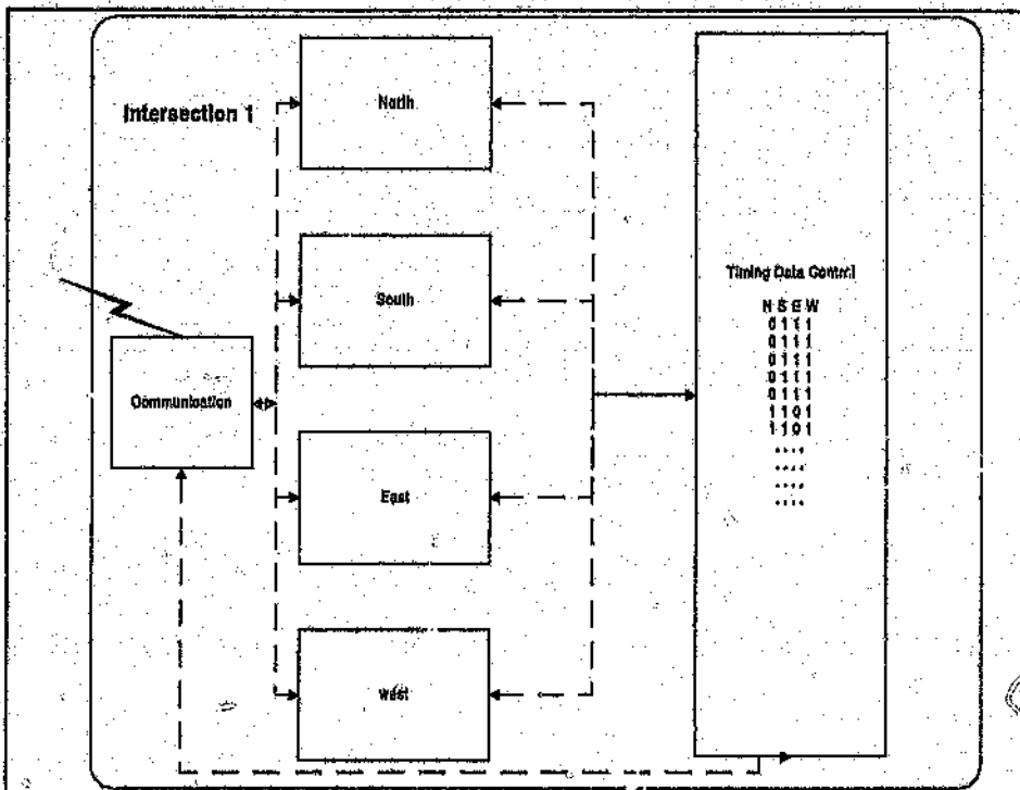
Figure 4: The conceptual overview of a single agents blackboard. This diagram shows the structural breakdown of a blackboard. All flow information is shown. Information flows from the min-blackboards North, South , East and West to the timing data control structure and then back again.
