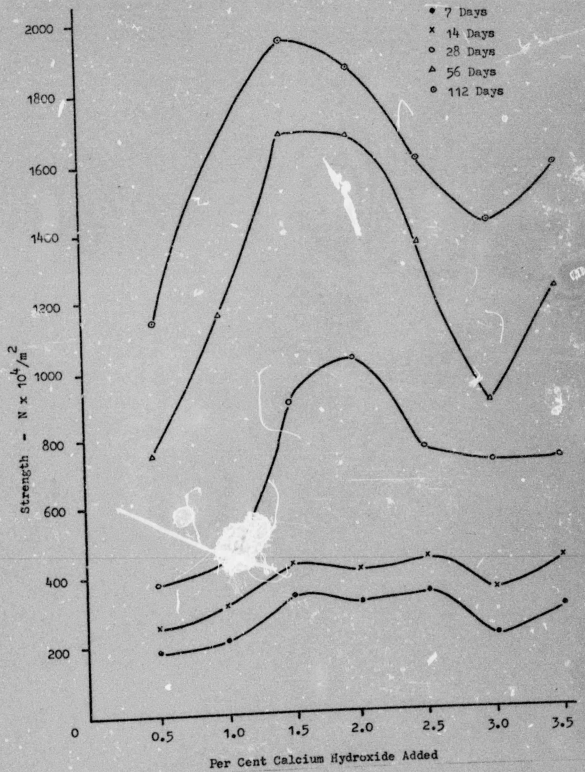
Figure 4. Effect of the Amount of Calcium Hydroxide Activator on the Strength Developed By Standard Blast Furnace Slagment
