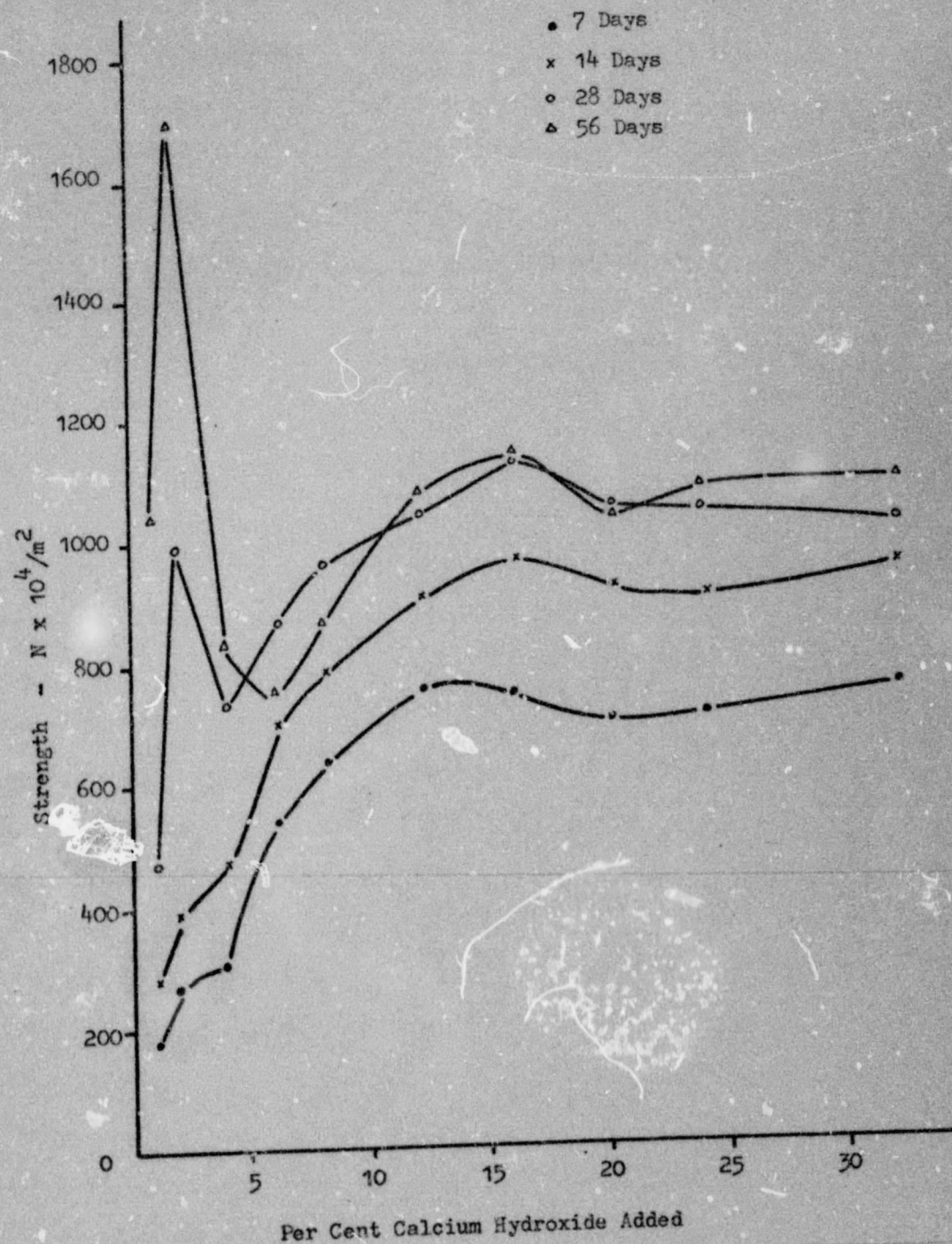
Figure 3. Effect of the Amount of Calcium Hydroxide Activator on the Strength Developed By Standard Blast Furnace Slagment
