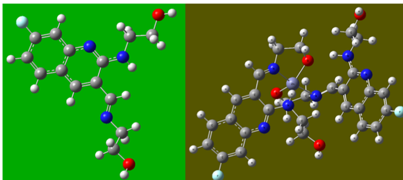
Figure 1. Optimized structure of the ligand and complex 1.
