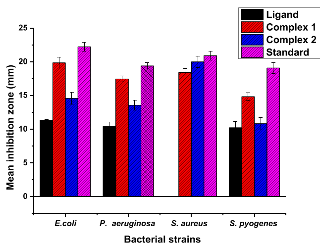
Figure 7. Mean inhibition zone of the antibacterial activity of the ligand and the complexes ( n = 3 ). Error bars indicate standard deviation.
