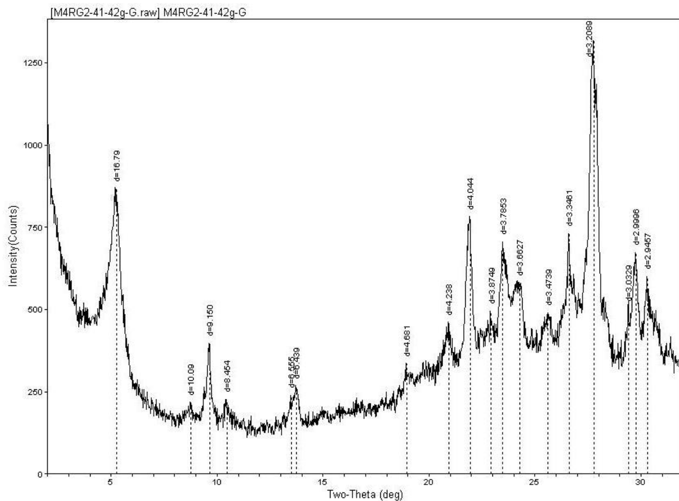
Figure 1.12. Glycolated XRD spectra for sample M4 RG2 from 262 m showing major peaks labelled in Figure 7. Spectra shows 42g of measured rock powder.
