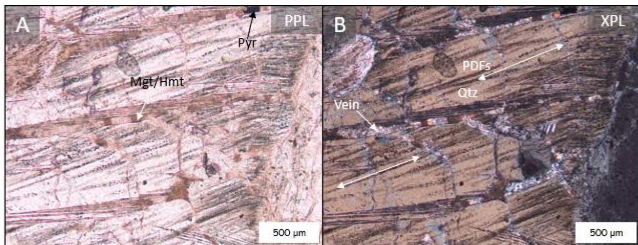
Figure 4.2. Optical microscope images (A - PPL; B - XPL) of sample M4 GG8 (152 m) showing closely spaced decorated PDFs showing fluid inclusion trails cut by a polymineralic vein. PPL = plane polarised light; XPL = crossed polarised light; Pyr = pyrite; Mgt/Hmt = magnetite/haematite; Qtz = quartz; PDFs = planar deformation features.
