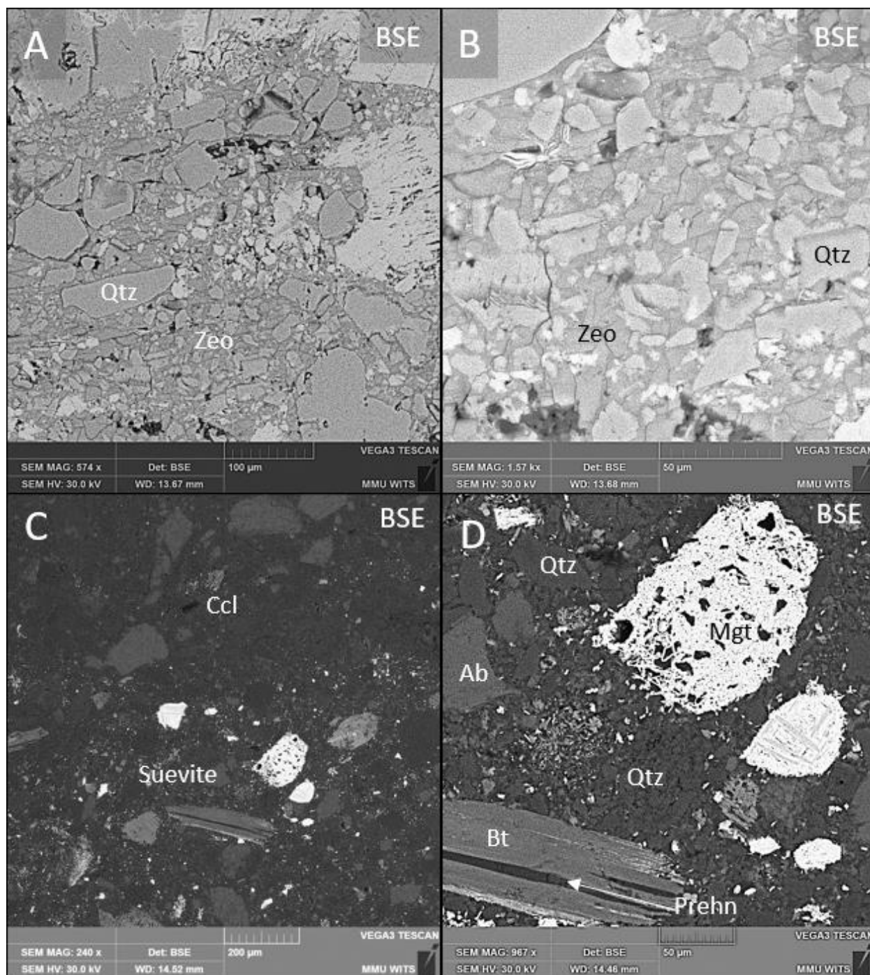
Figure 4.11. BSE scans showing post-impact hydrothermal alteration in impactite rocks. A) Sample M4 GG15 (324 m) showing zeolite cement in suevite matrix. B) Close-up of A showing the matrix-supported nature of the suevite. C) Sample M4 IM9 (299 m) showing a lithological contact between suevite and cataclasite. D) Close-up of the suevite matrix in C, showing alteration in biotite and magnetite. BSE = backscattered electron; Zeo = zeolite; Qtz = quartz; Ccl = cataclasite; Ab = albite; Bt = biotite; Mgt = magnetite; Prehn = prehnite.
