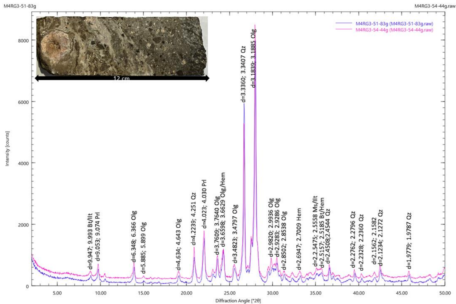
Figure 1.8. Aired-dried XRD spectra for sample M4 RG3 from 301 m showing major peaks of Prl = pyrophyllite; Olg = oligoclase; Ilt = illite; Bt = biotite; Qz = quartz; Hem = haematite. Pink spectra shows 44g of measured rock powder and blue spectra shows 83g of measured rock powder.
