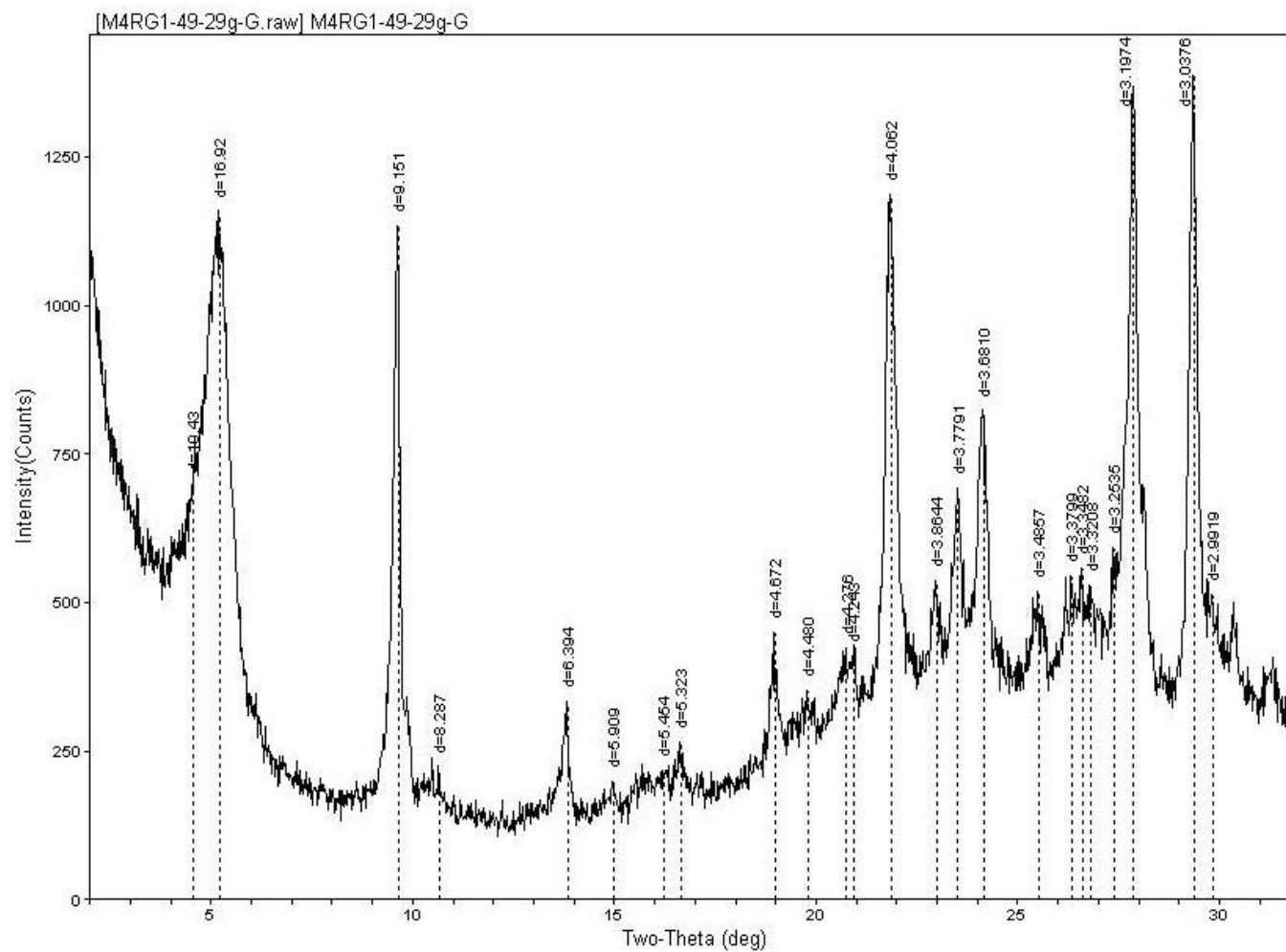
Figure 1.11. Glycolated XRD spectra for sample M4 RG1 from 146 m showing major peaks labelled in Figure 6. Spectra shows 29g of measured rock powder.
