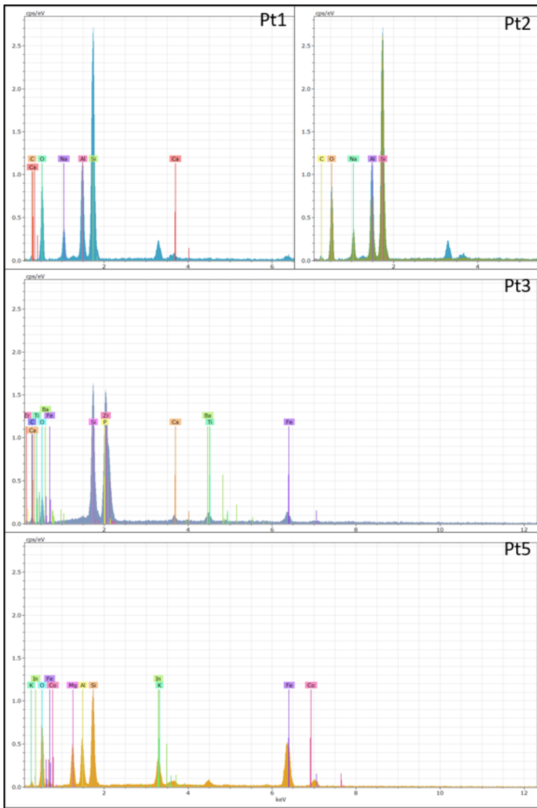
Figure 1.1. EDS spectra showing point 1 and 2 representing plagioclase, Pt3 representing zircon and Pt5 representing biotite.
