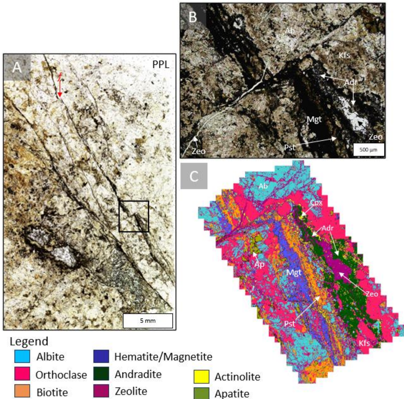
Figure 4.10. Photomicrograph of granitic gneiss sample M4 R12 (264 m). (A) Overview in plane polarised light (B) Closeup of box in A in plane polarised light, showing ~1 mm wide, steeply oriented shear fault defined by thin magnetite-dominated fractures and vugs characterised by neoblastic andradite and zeolite. The magnetite-pseudotachylite fractures are cut by a shallowly dipping shear fault with normal displacement, and by zeolite veins. (C) TIMA phase map of B. For elemental distribution maps of this texture in Appendix 1.2A-B. PPL = plane polarised light; Ab = albite; Kfs = alkali feldspar; Adr = andradite; Mgt = magnetite; Zeo = zeolite; Ap = apatite; Cpx = clinopyroxene; Pst = pseudotachylite.
