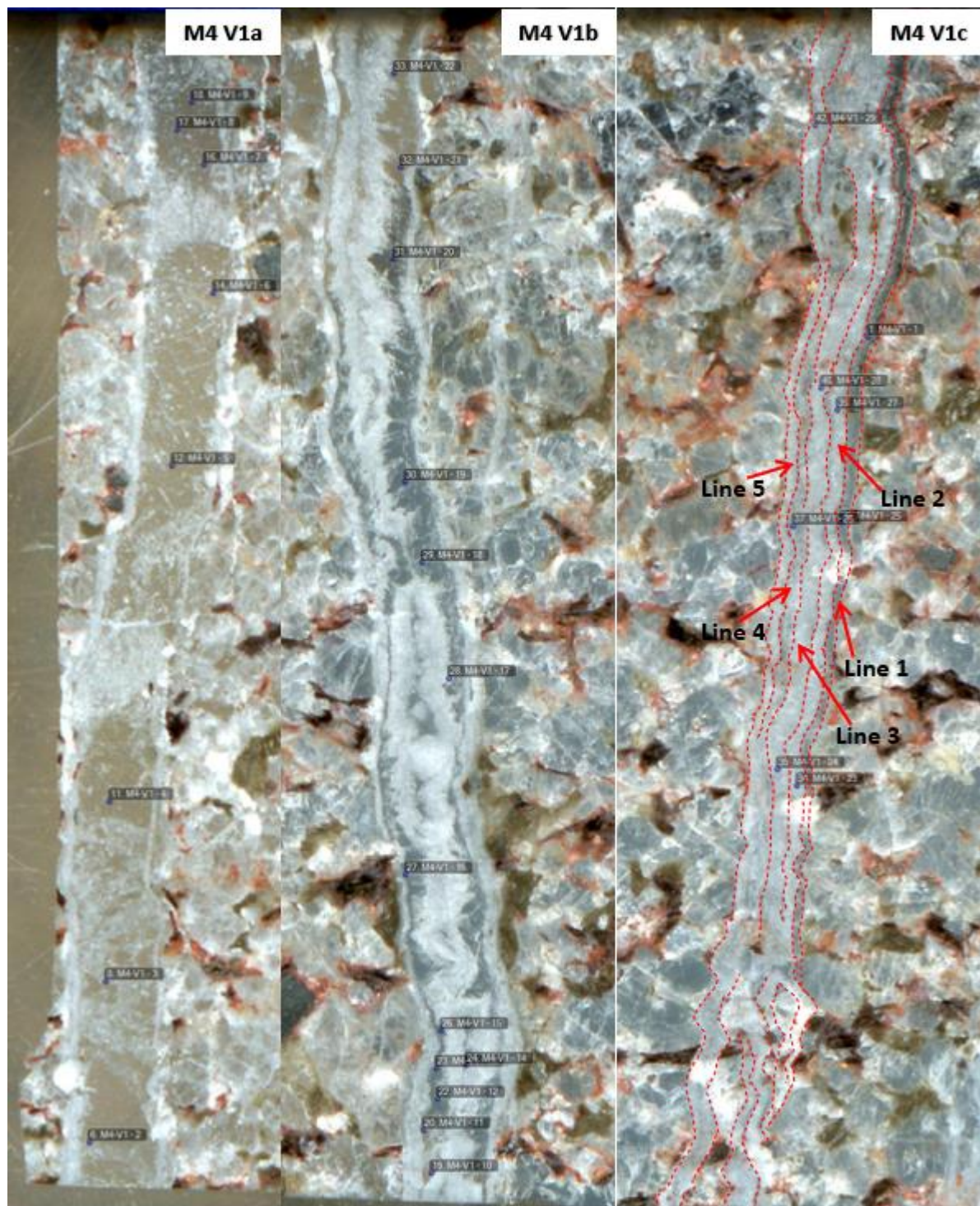
Figure 4.28. Laser spot locations in sample M4 V1a-b and within the five layers of calcite in M4 V1c.
