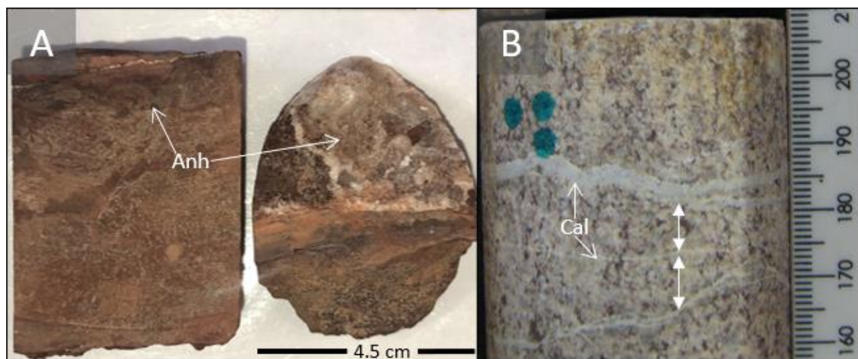
Figure 4.15. Macroscopic evidence of monomineralic veins in the M4 drillcore. A) Metadolerite sample M4 ML (195.30 m) showing white anhydrite vein. B) Granodioritic gneiss from Box 2 (110.08 – 119.39 m) showing irregular to anastomosing subhorizontal calcite veins. Anh = anhydrite; Cal = calcite.
