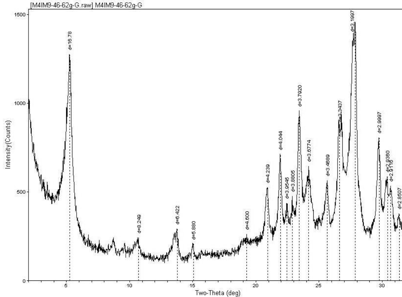
Figure 1.16. Glycolated XRD spectra for sample M4 IM9 from 299 m showing major peaks labelled in Figure 8. Spectra shows 62g of measured rock powder
