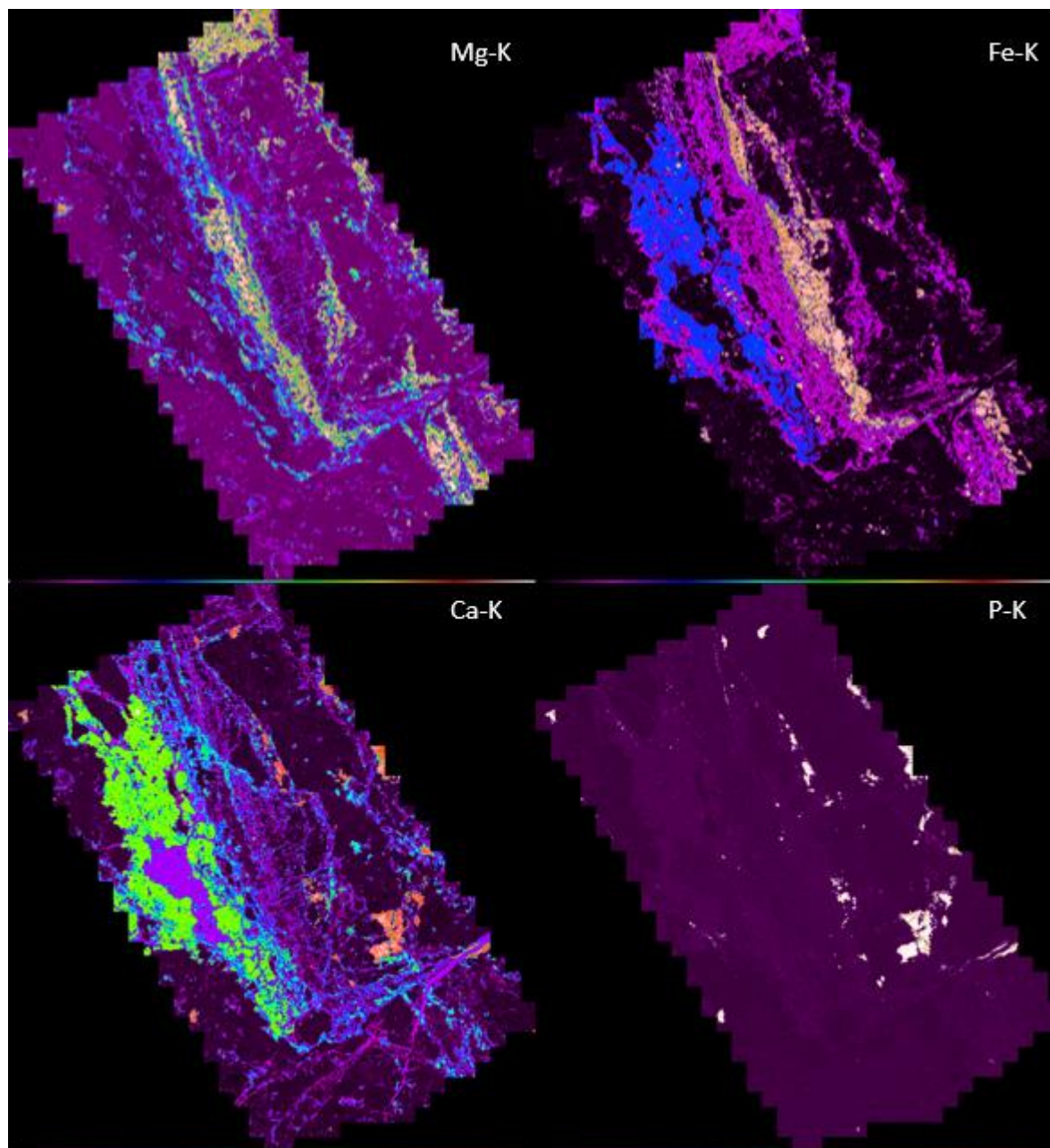
Figure 1.5. Elemental maps showing the distribution of Mg, Fe, Ca and P. Each map is displaying relative intensity scale dark/black (element-deficient; left) and bright/white (element-rich). The fracture is depleted in P and show Mg, Ca and Fe distribution from rim to core.
