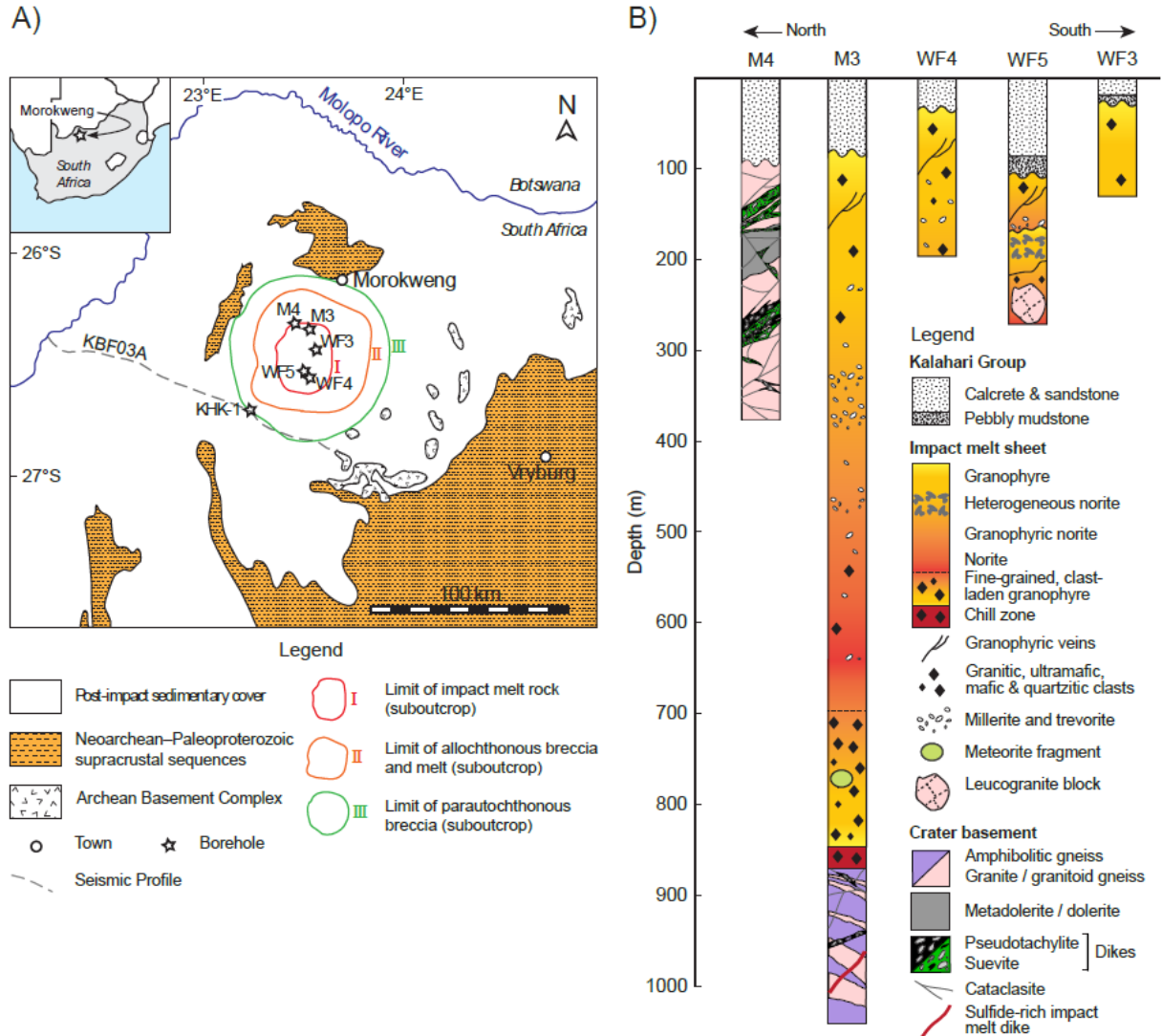
Figure 2.1. A) Simplified geological map of the Morokweng Impact Structure displaying concentric rings identified by Andreoli et al. (2007) from geophysical data. Also shown are locations of boreholes, and B) stratigraphic columns of boreholes M4, M3, WF5, WF4 and WF3. The locations of the KBF03A seismic profile and KHK-1 drillcore discussed, respectively, in Westgate et al. (2021) and Reimold et al. (2002) are also shown. Inset shows the locality of the MIS in South Africa. (From Gibson et al. 2024a).
