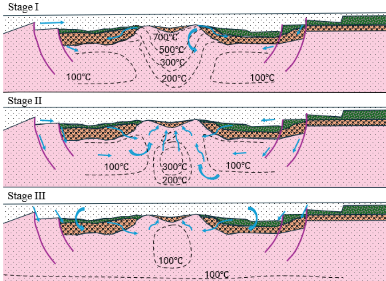
Figure 1.3. Illustration of regressive hydrothermal circulation of fluids within a complex crater showing three successive stages. Stage I (initial/early stage) displays variability in temperature from top downward, with hydrothermal activity occurring in the periphery of central uplift. Stage II (main stage) displays lateral variations in temperature with circulation of fluids within both the central uplift and its periphery. Stage III (final stage) is characterised by temperatures < 100 °C and fluid circulation occurs only near the surface. Pink colour = Brecciated crystalline basement; Brown-black = lithic breccias; Green colour = impact melt rock responsible for local circulation systems in the annular depression; white color = crater basin deposits; the dotted lines = isotherms; blue arrows = direction of circulation. (Modified from Naumov, 2005).
