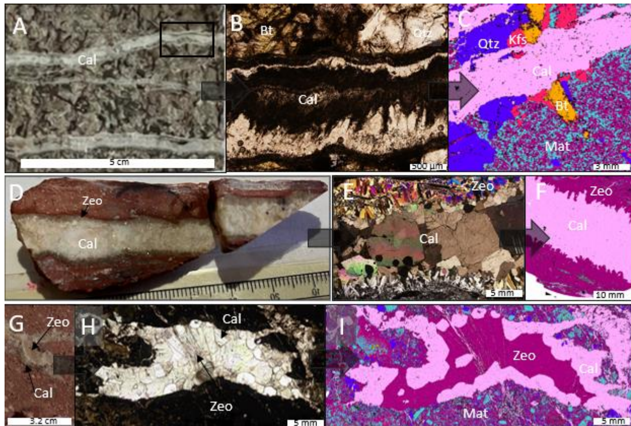
Figure 4.24. Photographs of hand specimens, plane and crossed polarised light, and phase maps of three calcite veins in the upper part of the M4 drillcore. A) Sample M4 V1 (114 m) shows white composite calcite veins with spacing < 5 cm cutting through a granodioritic gneiss. The vein, in plane polarised light (B), shows elongated calcite veins pointing towards fine-grained calcite. The phase map (C) identifies the entire vein as filled with calcite. D) Sample M4 V3 (142.95 m) shows vitreous grey zeolite enclosing a white calcite vein; the calcite grains are up to 15 mm wide. G) Coarse-grained calcite-zeolite vein cutting suevite from 143.02 m. Calcite grains occur along vein walls and around clasts, with zeolite forming the core of the vein.
