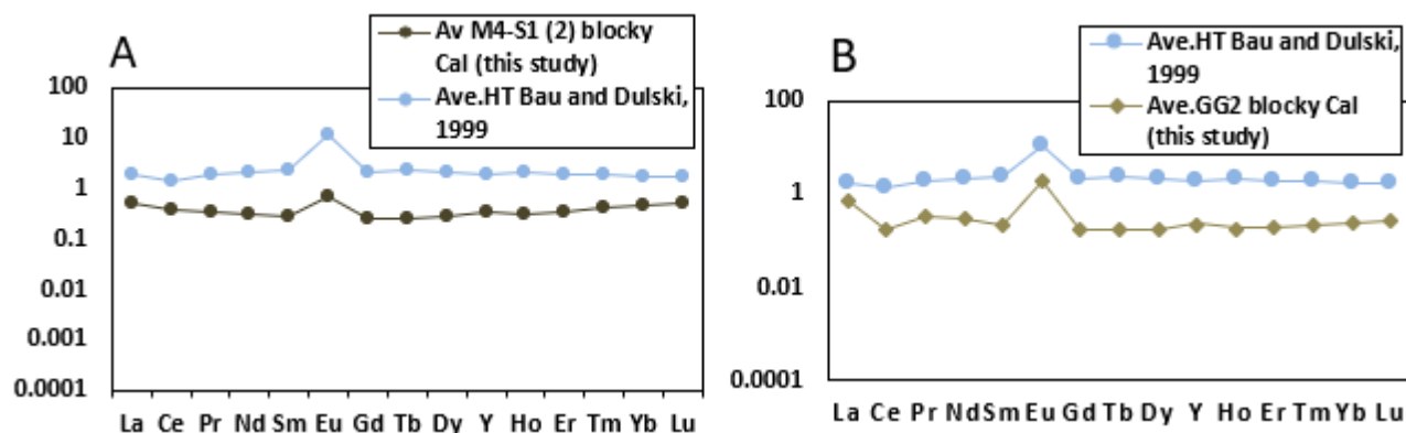
Figure 5.2. MUQ-normalised (mud sediments from Queensland) REE patterns of calcite veins in samples M4 S1(2) shown in A and M4 GG2 shown in B, matched with hydrothermal fluids (Bau and Dulski, 1999).
