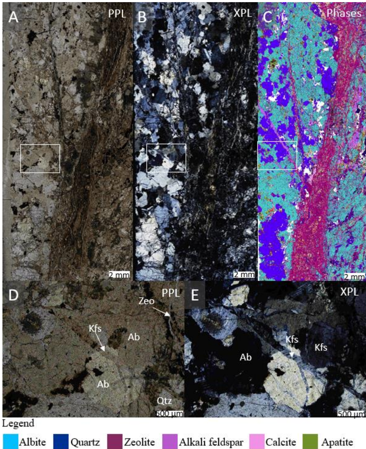
Figure 4.3. Microphotographs and phase map of sample M4 INJ2 (158.06 m) showing a subvertical pseudotachylite vein and alkali feldspar veins cutting through albite and quartz (box). A) Plane-polarized light image showing alkali feldspar cutting through albite and quartz and terminating at the pseudotachylite dyke boundary. Zeolite veins cut through both the pseudotachylite and granodioritic gneiss wallrock. B) cross-polarised light of A. C) TIMA phase map of A, B. D) Close-up PPL image of white box in A-C,
