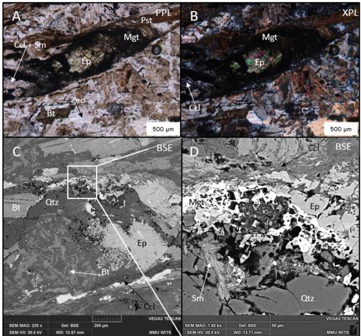
Figure 4.7. Primary epidote grains from sample M4 R8 (348.4 m). A) PPL image of Brecciated and fractured epidote string along the cataclasite displaying magnetite and smectite along the rims. B) XPL
