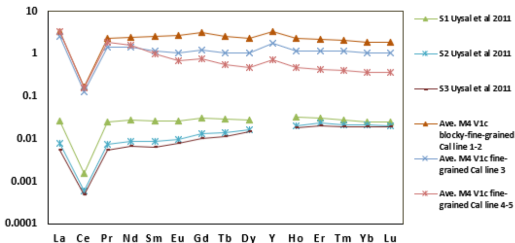
Figure 5.4. MUQ-normalised (mud sediments from Queensland) REE patterns of calcite veins in samples M4 V1C from calcite line 1 to line 5, matched with calcite veins from Uysal et al. (2011). S1-3 represents stage 1 of formation to stage 3.
