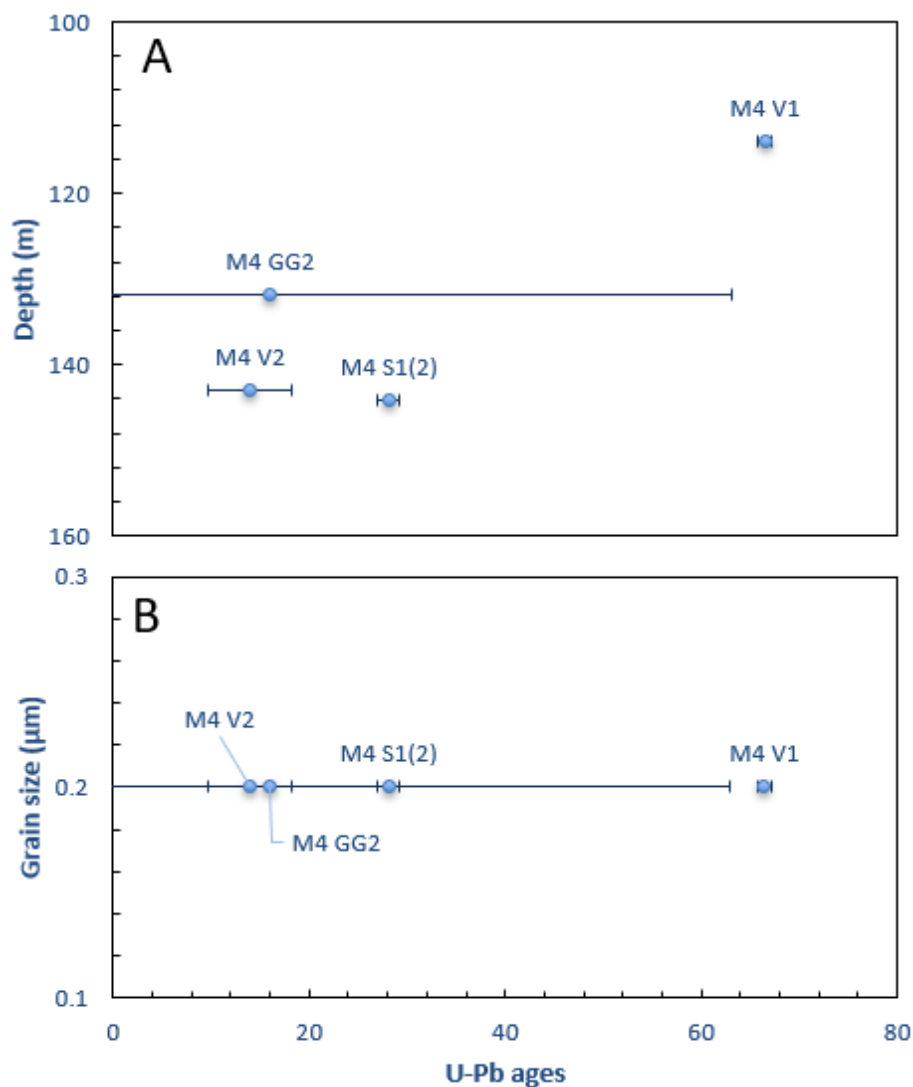
Figure 4.33. Relationship between U-Pb ages versus A) depth and B) calcite grain spot size analysis for the calcite veins from sample M4 V1, M4 GG2, M4 V2, and M4 S1(2). The plots include error estimates for each age.
