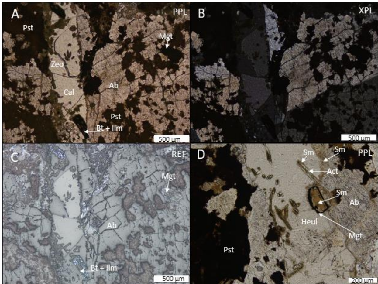
Figure 4.18. Photomicrographs of sample M4 R22 (139 m) showing relatively high-T assemblage of zeolite, clinopyroxene, smectite, calcite and Fe-(hydr)oxide in a vein matrix. A) Plane-polarized image showing the oxides are magnetite and ilmenite. The zeolite vein contains inclusions of calcite, actinolite, smectite, and biotite showing alteration to ilmenite. B) Crossed-polarized image of A. C) Reflected light of A-B. D) A close-up plane-polarized light image of inclusions within the zeolite veins. PPL = plane polarised light; XPL = crossed polarised light; REF = reflected light; Zeo = zeolite; Cal = calcite; Bt = biotite; Ilm = ilmenite; Ab = albite; Mgt = magnetite; Pst = pseudotachylite; Heul = heulandite; Sm = smectite; Act = actinolite.
