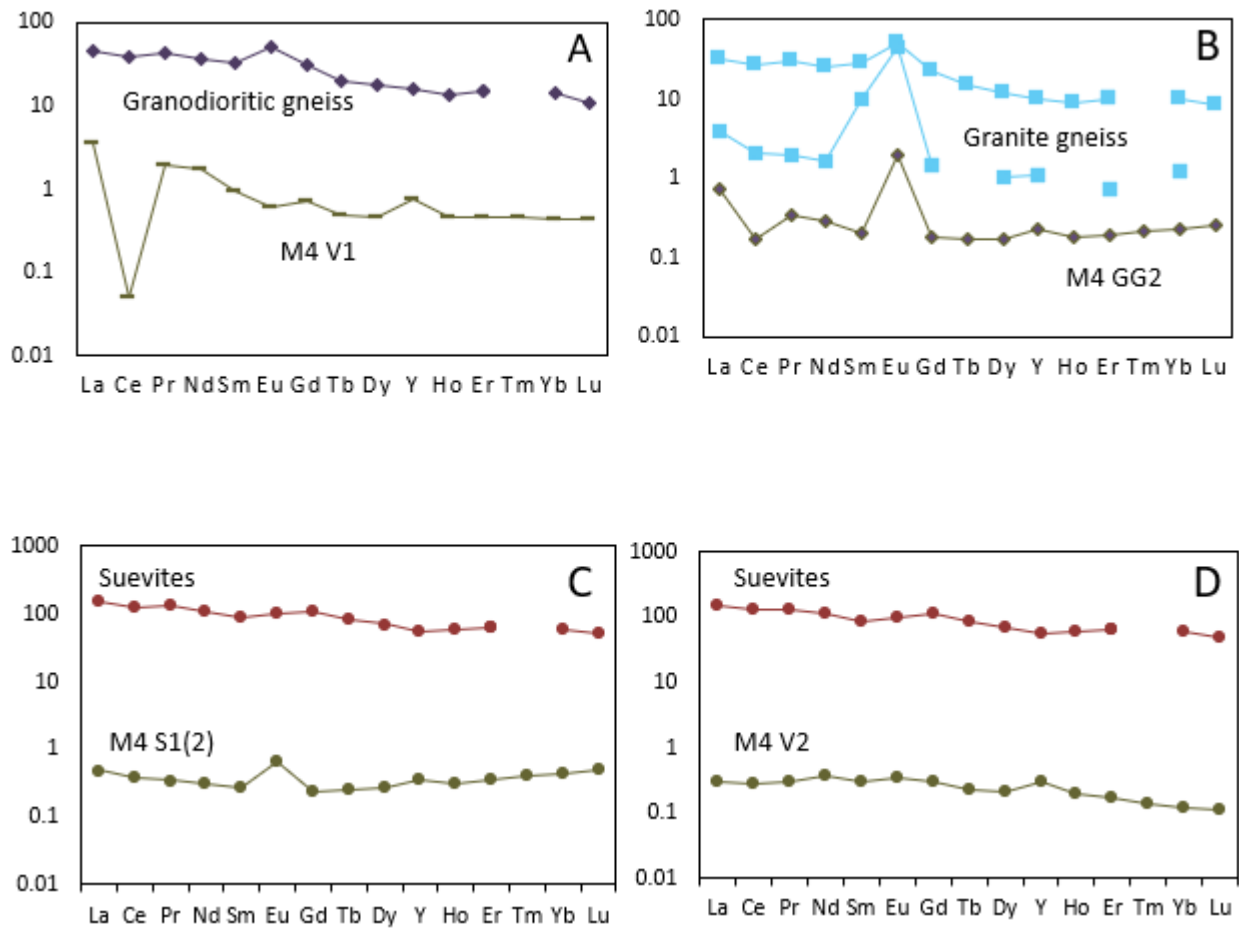
Figure 4.30. MUQ-normalized REE + Y patterns of calcite veins and host rocks (Wela, 2017; granodioritic gneiss, leucocratic granitic gneiss, and suevite).
