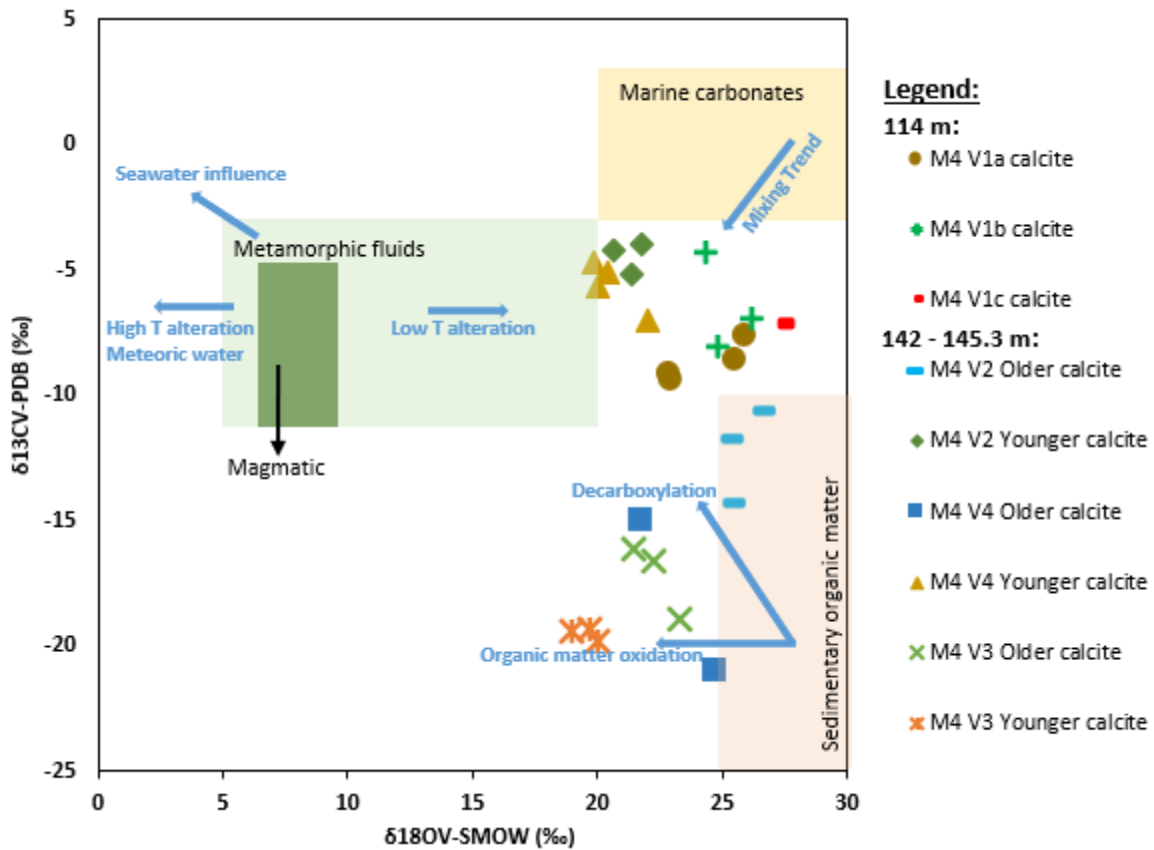
Figure 4.26. \delta^{18}\text{O}_{\text{V-SMOW}} - \delta^{13}\text{C}_{\text{V-PDB}} diagram showing compositions of vein calcites from the M4 drillcore. The oxygen and carbon isotope reservoirs and diagenetic trends are adapted from literature sources (Liu et al., 2007; Duuring et al., 2008; Broom-Fendley et al., 2016; Guo et al., 2018; Tan et al., 2015; Quandt et al., 2019).
