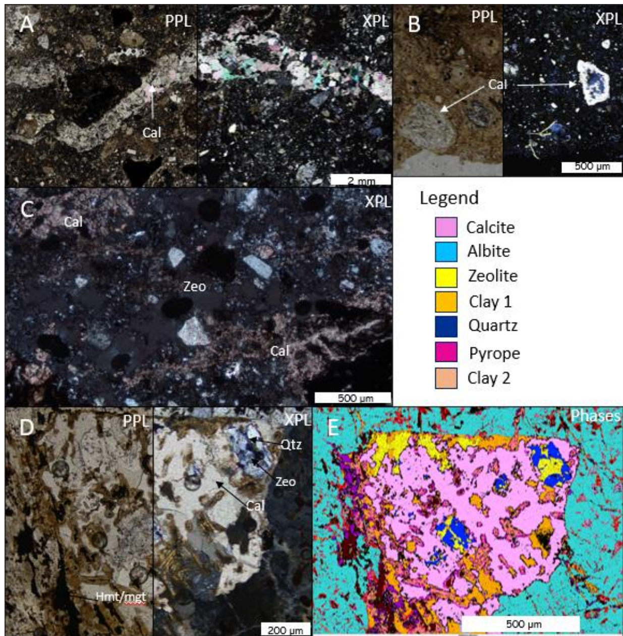
Figure 4.25. Photomicrograph showing morphology and textures of calcite across the M4 drillcore. A) Blocky calcite vein in PPL and XPL of sample M4 S1 (2) (144.09 m). B) Sample M4 S12 (148 m) showing fine-grained calcite around zeolite vugs. C) Sample M4 S3 (160 m) in XPL showing fine-grained calcite cement. D) Combined PPL and XPL image showing a polymineralic, calcite-dominated vug in granitoid gneiss. Apart from calcite, the vug contains quartz, zeolite, haematite/magnetite, and neoblasts of actinolite in sample M4 R22 (139 m). E) Phase map of D. Colors in phase maps labelled in the legend provided. XPL = crossed polarized light; PPL = plane polarized light.
