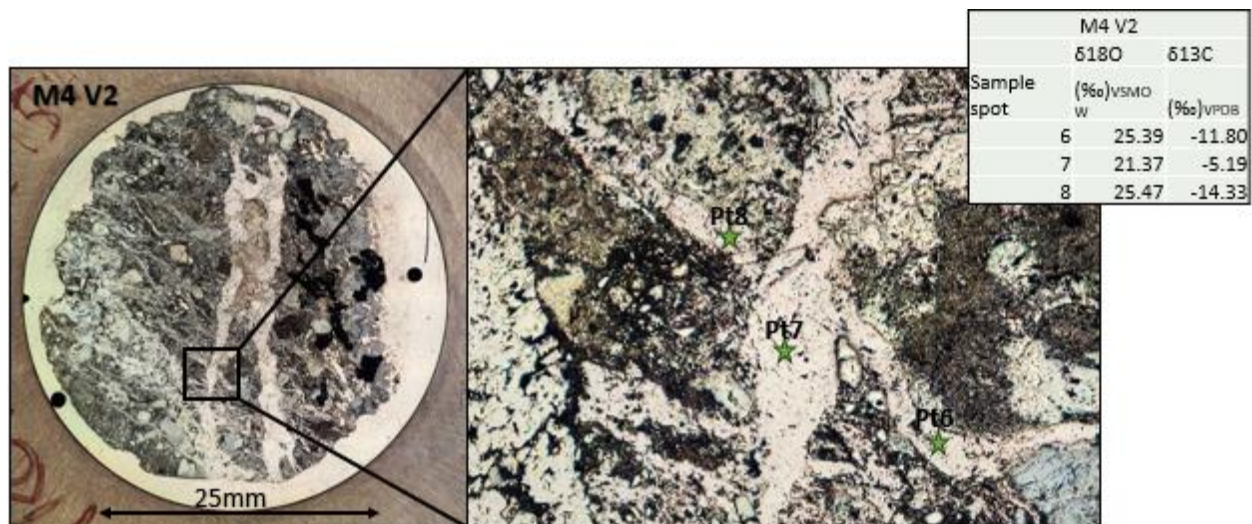
Figure 4.27. Crosscutting relationships between two calcite veins in sample M4 V2, show variation in \delta^{13}\text{C} and \delta^{18}\text{O} values from three points. Two points are from the older vein and one from the younger vein.
