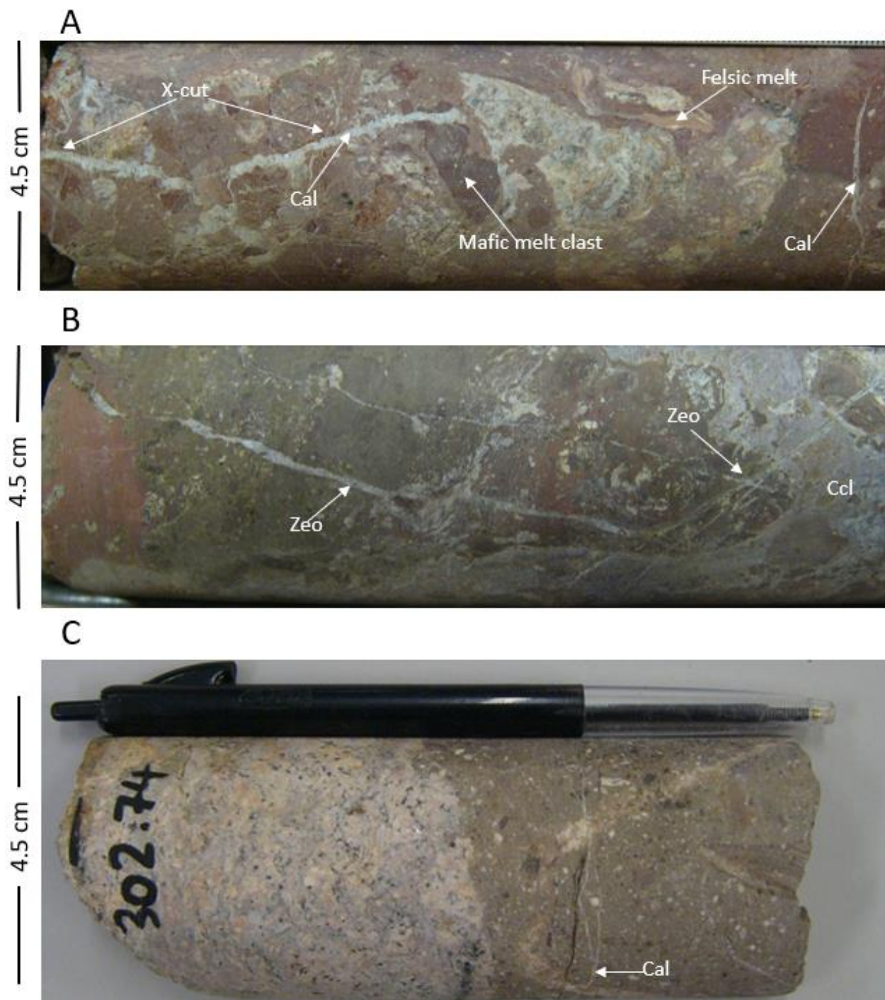
Figure 4.14. Macroscopic evidence of post-impact vein in the M4 drillcore. A) Suevite within the upper fault zone at a depth of 146.05 m. The calcite vein exhibits both vertical and sub-horizontal orientations and crosscuts mafic melt clasts and lithic fragments. B) Metadolerite containing cataclasite and pseudotachylite cut by zeolite veins within the lower fault zone at depth of 292 m. C) Contact between granitic gneiss and grey suevite, showing zeolite and calcite veins in the suevite matrix at a depth of 302.74 m. The drillcore width is 4.5 cm. Zeo = zeolite; Cal = calcite; x-cut = crosscut; Ccl = cataclasites.
