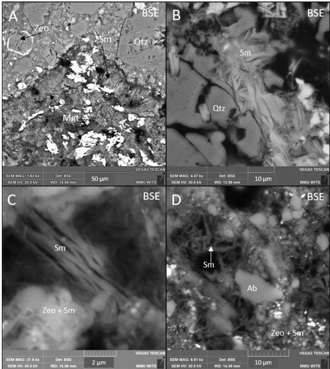
Figure 4.12. BSE microphotographs showing smectite minerals within the M4 drillcore. A) Sample M4 SB3 (353 m) showing smectite, zeolite and magnetite in brecciated suevite. B) Sample M4 R8 (348.4 m) showing smectite in brecciated quartz in cataclasite. C) Sample M4 RG2 (262 m) shows flaky smectite morphology within suevite matrix. D) Sample M4 RG3 (301 m) shows fibrous smectite within a pseudotachylite matrix. The matrix is a mix of zeolites and smectites (Wela, 2017). BSE = backscattered electron; Zeo = zeolite; Sm = smectite; Qtz = quartz; Bt = biotite; Mgt = magnetite; Ab = albite.
