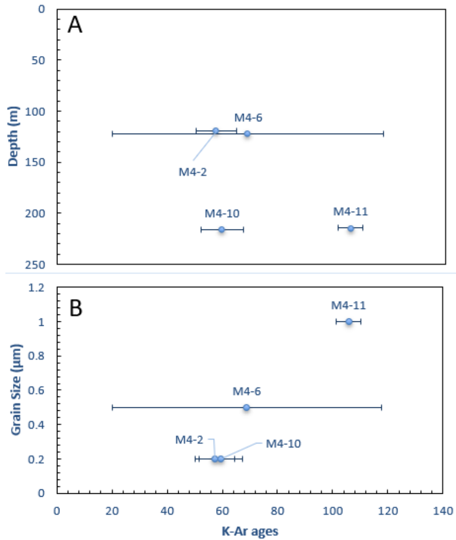
Figure 4.34. Plots showing the relationship between smectite-illite clay K-Ar ages grain size and depth for samples in the M4 drillcore. The plots include error estimates for K-Ar ages.
