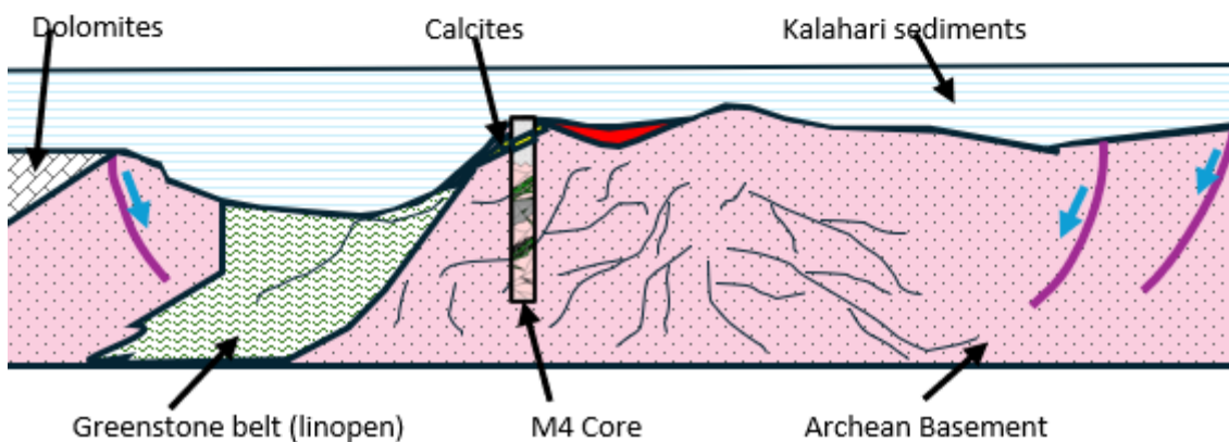
Figure 5.5. Schematic proposed exhumation-related events around the Morokweng impact structure region.
