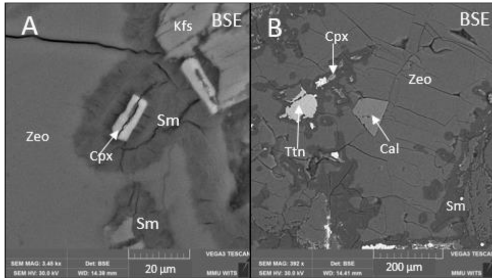
Figure 4.21. A) Close up BSE scans showing zeolite vein/vug in M4 GG10 (166 m) with clinopyroxene and smectite on the rims and alkali feldspar alteration. B) Close up BSE scan of zeolite vug showing titanite, calcite, clinopyroxene and smectite. BSE = backscattered electron; Zeo = zeolite; Cpx = clinopyroxene; Sm = smectite; Kfs = alkali feldspar; Ttn = titanite; Cal = calcite.
