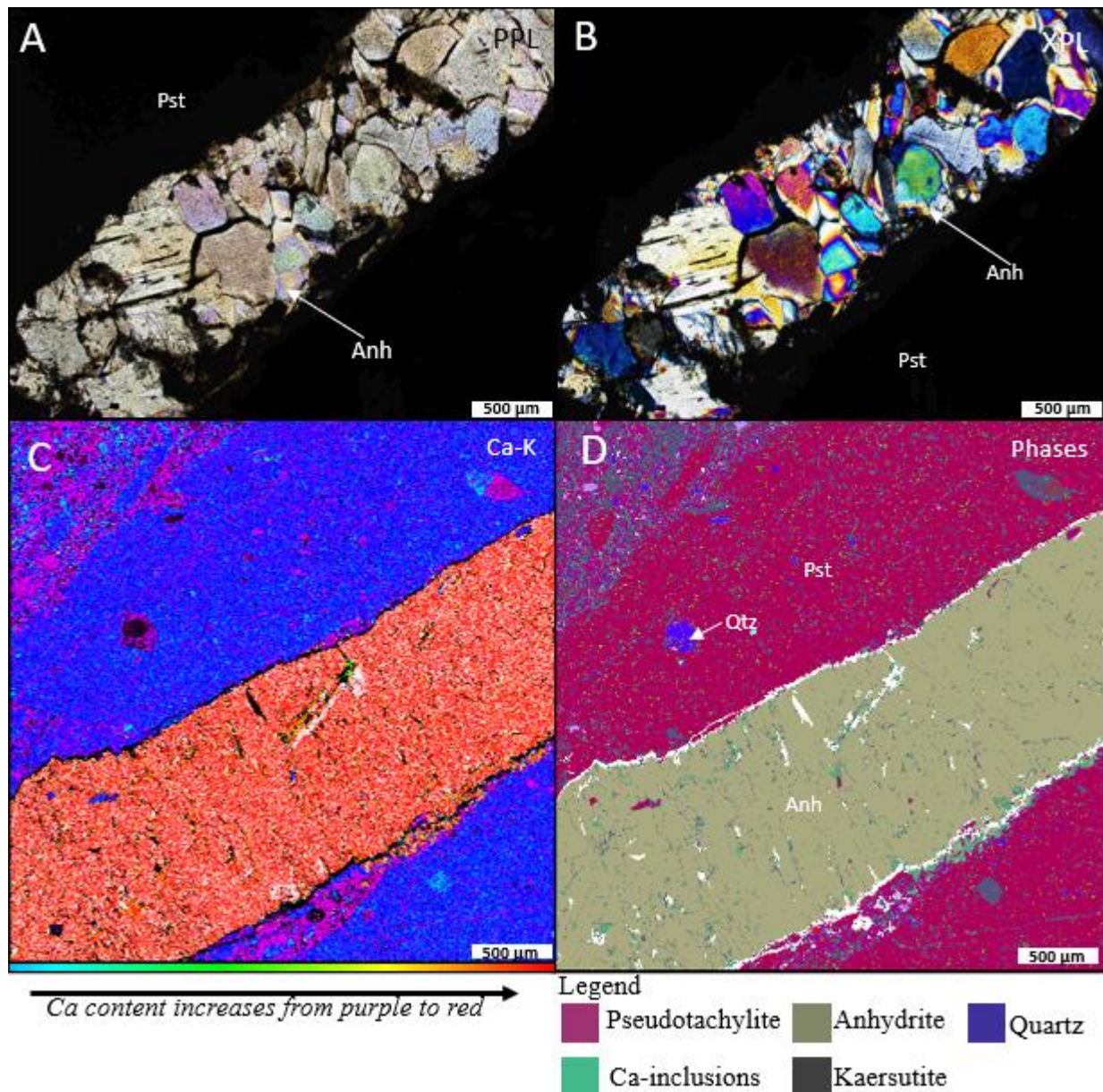
Figure 4.17. Photomicrographs of sample M4 ML (195.30 m) showing anhydrite vein cutting across pseudotachylite. A) Plane polarised light image showing subidioblastic granoblastic grains. B) Cross-polarised light of A. C) Calcium elemental map showing Ca enrichment localized within anhydrite vein. D)
