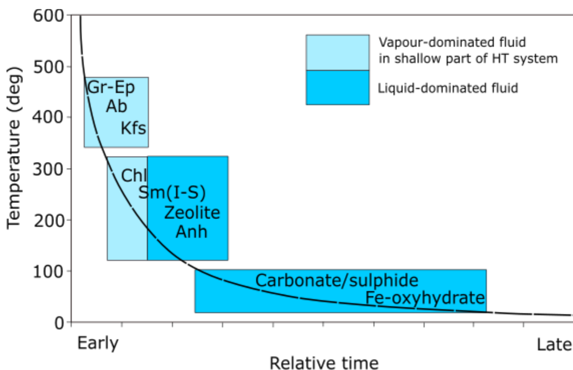
Figure 1.4. Proposed sequence of the cooling of post-impact mineral growth. Gr: garnet; Ep: epidote; Ab: albite; Kfs = alkali feldspar; Chl = chlorite; Sm = smectite; I-S = mixed-layer illite-smectite; Anh = anhydrite. (Adapted from Kirsmae and Osinski, 2013).
