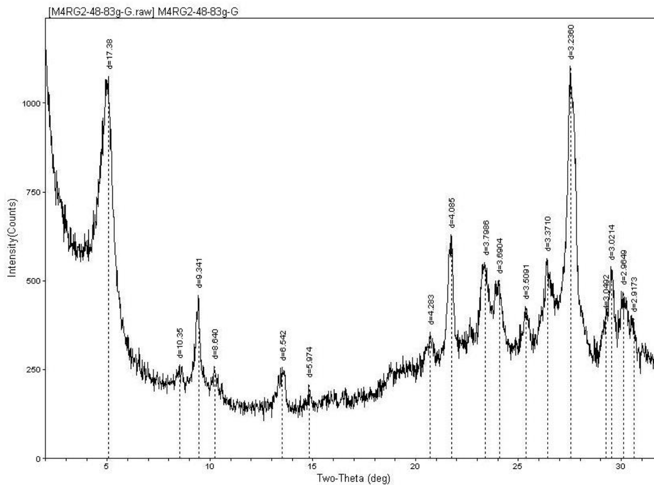
Figure 1.13. Glycolated XRD spectra for sample M4 RG2 from 262 m showing major peaks labelled in Figure 7. Spectra shows 83g of measured rock powder.
