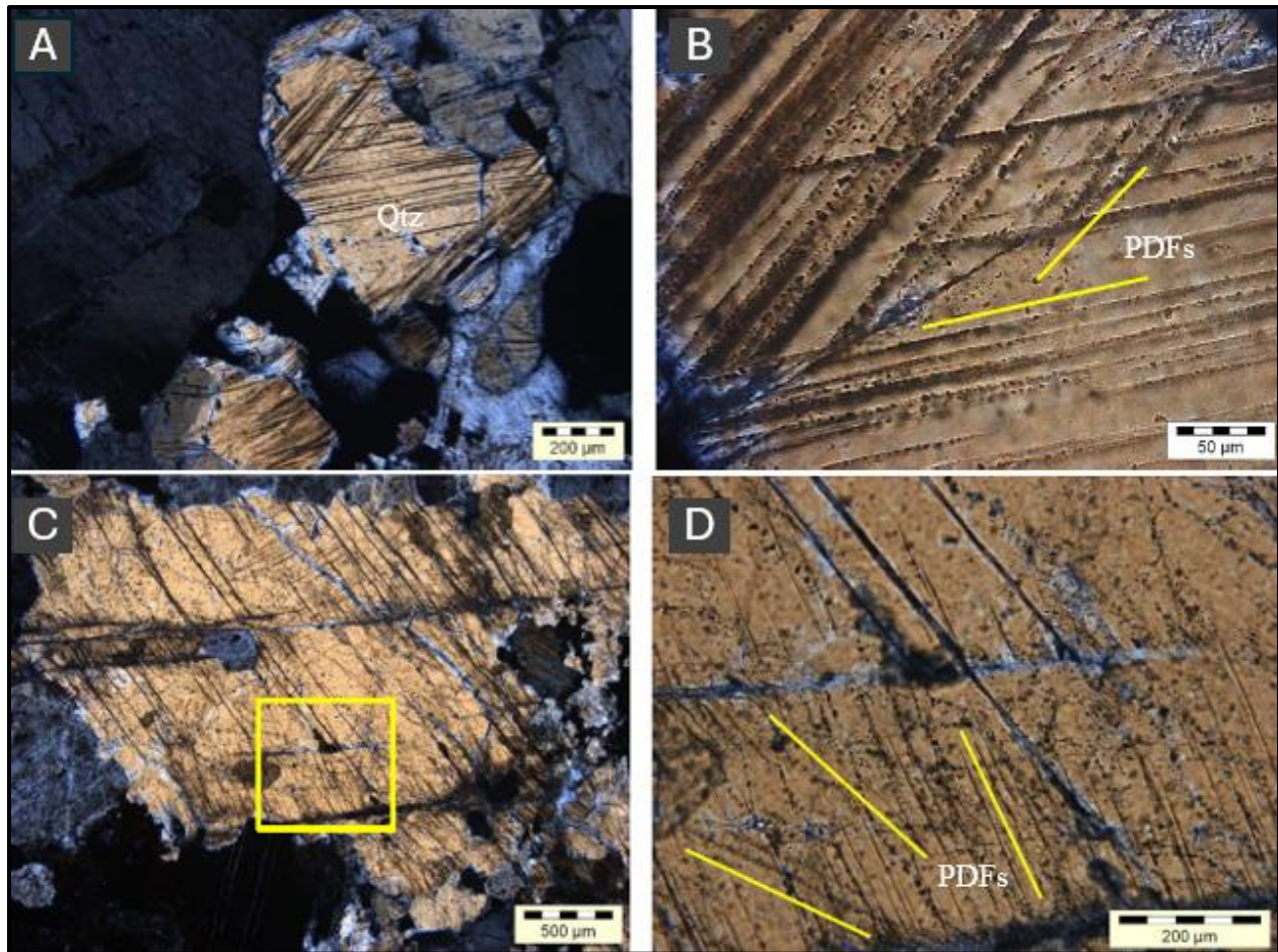
Figure 2.3. Microphotographs of quartz grains showing multiple sets of decorated PDFs (images from Wela, 2017). A) Cross polarised light image showing two sets of decorated PDFs from Sample M4 GG 4 (109.20 m). B) Enlargement of A, showing fluid inclusion trails. C) Cross polarised light image showing microfractures and PDFs in shocked quartz grain from sample M4 FZ-2 (219.30 m). D) Enlargement of C, showing three sets of decorated PDFs and microfractures containing zeolite fill. PDFs = planar deformation features.
