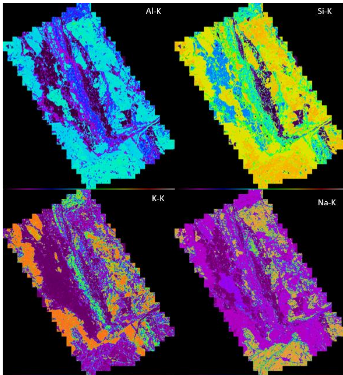
Figure 1.4. Elemental maps showing the distribution of Al, Si, K and Na. Each map is displaying relative intensity scale dark/black (element-deficient; left) and bright/white (element-rich). The fracture is more enriched in Si and K in the core and depleted around the rims. Na more depleted than Al.
