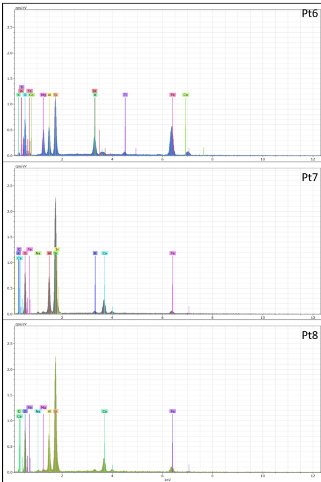
Figure 1.2. EDS spectra showing point 6 representing biotite, Pt7 and Pt8 representing Prehnite.
