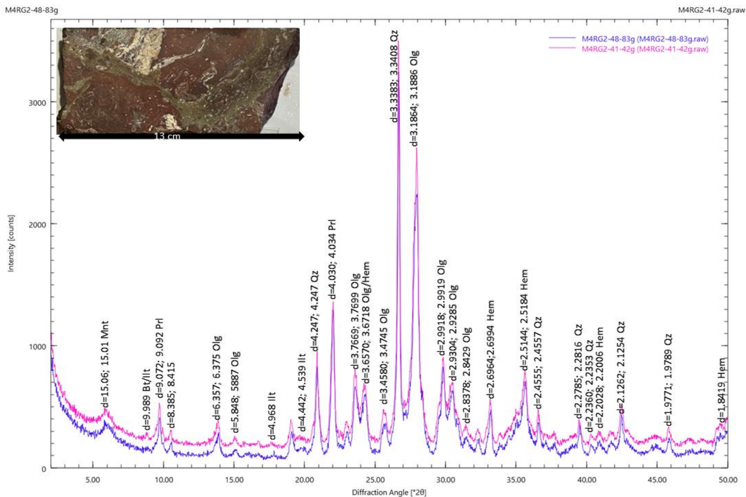
Figure 1.7. Aired-dried XRD spectra for sample M4 RG2 from 262 m showing major peaks of Mnt = Montmorillonite; Prl = pyrophyllite; Olg = oligoclase; Ilt = illite; Bt = biotite; Qz = quartz; Hem = haematite. Pink spectra shows 42g of measured rock powder and blue spectra shows 83g of measured rock powder.
