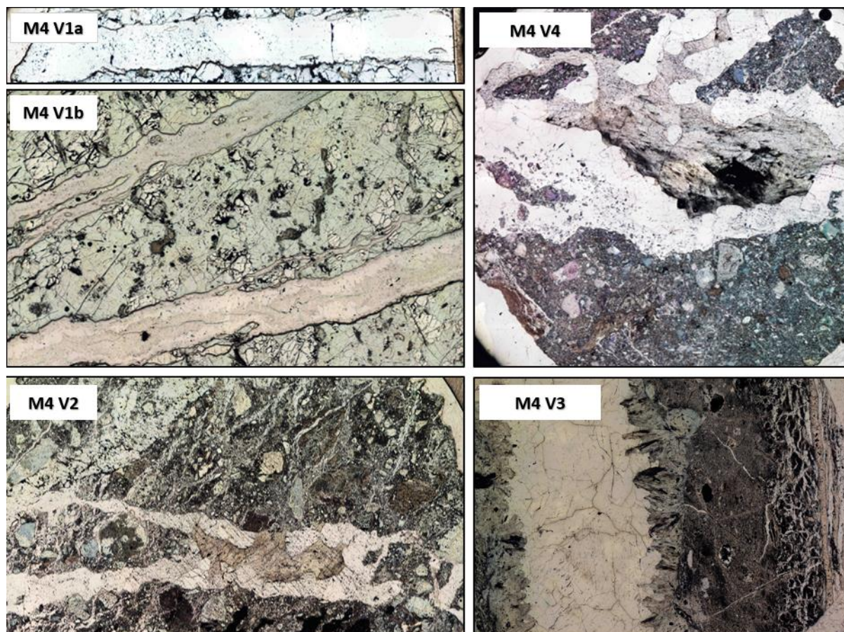
Figure 2.1: Cross-section of 25 mm thick mounts displaying the morphology of calcite veins analyzed for C-O isotope geochemistry. In M4 V1a and M4 V1b, two distinct tones are observed in the carbonates from rim to core: the lighter shade represents dolomite, while the darker shade represents calcite. In M4 V2, M4 V3, and M4 V4, the veins are a few millimeters thick, traversing a fine matrix of suevite rock. Blocky calcite veins are associated with zeolite in M4 V2 and M4 V4, and with plagioclase in M4 V3.
