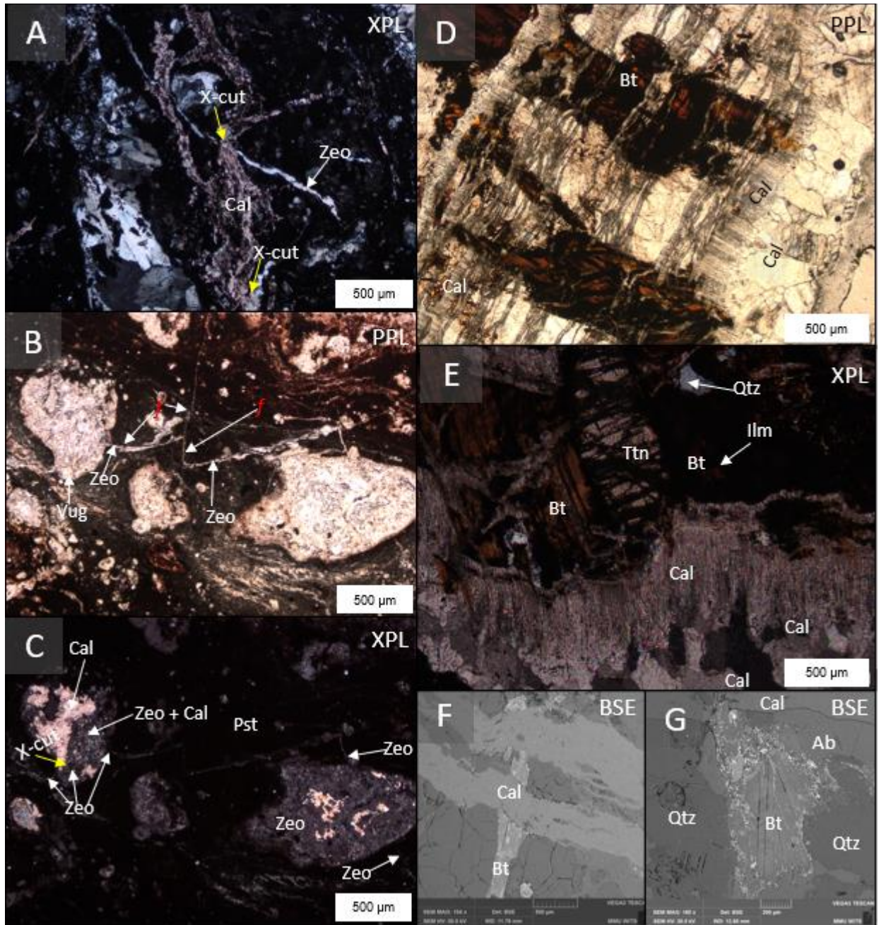
Figure 4.16. Photomicrographs showing crosscutting relationships of calcite veins with other minerals. A) calcite veins crosscutting zeolite veins from M4 V3 (142.95 m). Cross polarised light. B) Calcite-smectite-zeolite vugs in M4 RG1 (146 m), crosscutting zeolite veins, in plane polarised light. C) Cross polarised light image of B. D) Stretched to syntaxial elongate blocky calcite vein in sample M4 GG1.1 (129 m), crosscutting altered biotite, in plane polarised light. E) Sample M4 GG1.1 shows Stretched to syntaxial elongate blocky calcite cutting through biotite, titanite, and quartz. F) BSE scan of sample M4 V1 (114 m) showing calcite vein cutting through partially altered biotite. G) Sample M4 V1 shows a sharp contact between calcite veins and granodioritic gneiss containing partially altered biotite. No obvious enhanced alteration occurs along the vein edge. PPL = plane polarised light; XPL = crossed polarised light; BSE = backscattered electron; Zeo = zeolite; Cal = calcite; Bt = biotite; Ttn = titanite; Ilm = ilmenite; Qtz = quartz; f = fault; Pst = pseudotachylite.
