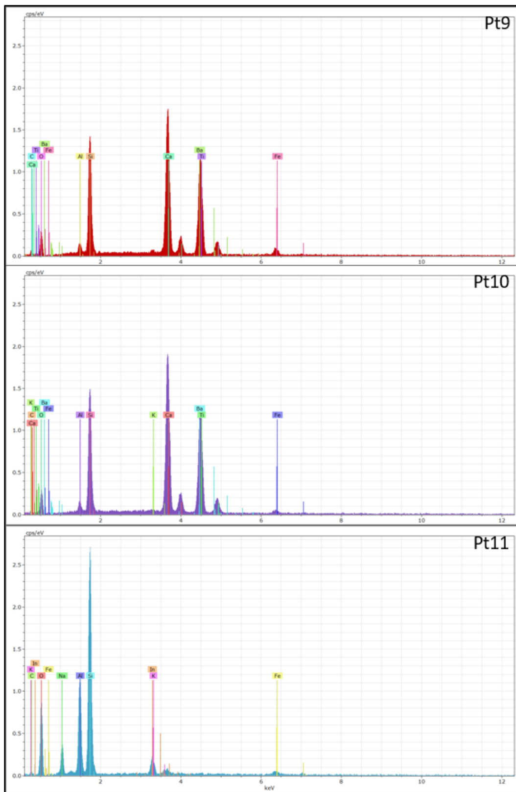
Figure 1.3. EDS spectra showing point 9 and 10 representing titanite and Pt11 representing alkali feldspar.
