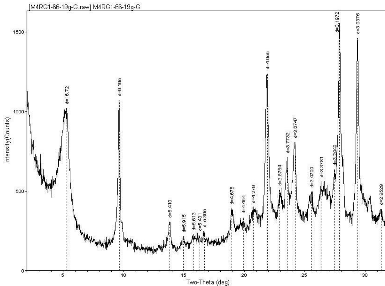
Figure 1.10. Glycolated XRD spectra for sample M4 RG1 from 146 m showing major peaks labelled in Figure 6. Spectra shows 19g of measured rock powder.
