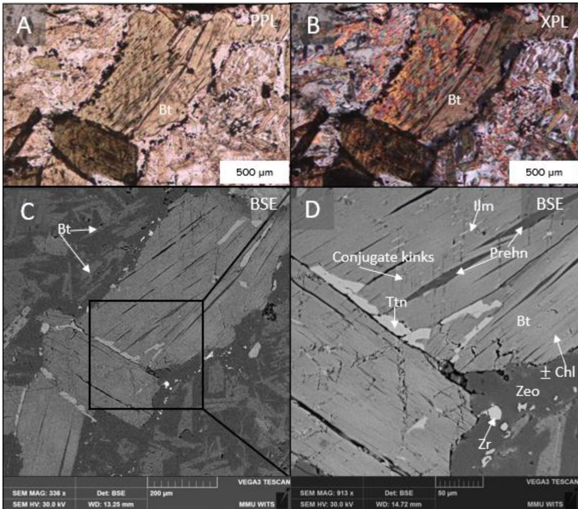
Figure 4.6. Kinked biotite replaced by secondary minerals in sample M4 R8 (348.4 m). A-B) Strongly pleochroic biotite rimmed by zeolite and Ti-oxides (white rim with black neoblasts in (A)) in monzonitic gneiss; PPL- XPL. C-D) BSE images of A-B showing titanite, prehnite and ilmenite replacing the biotite, which locally shows conjugate kink bands. The zeolite rim contains neoblastic titanite and a single zircon grain. The black box in C extrapolates to image D. Light grey laths in C are igneous biotite inclusions in plagioclase (Gibson et al., 2022). PPL = plane polarised light; XPL = crossed polarised light; BSE = backscattered electron; Bt = biotite; Ttn = titanite; Prehn = prehnite; Ilm = ilmenite; Zeo = zeolite; Chl = chlorite; Zr = zircon.
