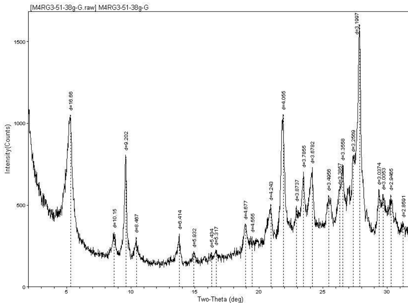
Figure 1.14. Glycolated XRD spectra for sample M4 RG3 from 301 m showing major peaks labelled in Figure 8. Spectra shows 38g of measured rock powder.
