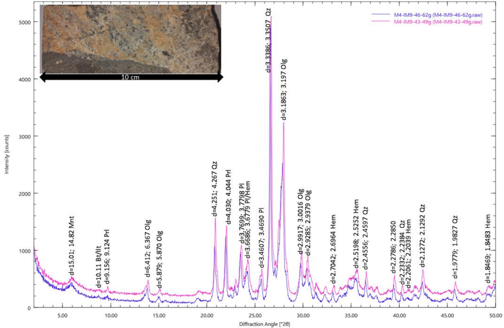
Figure 1.9. Aired-dried XRD spectra for sample M4 IM9 from 299 m showing major peaks of Mnt = Montmorillonite; Prl = pyrophyllite; Olg = oligoclase; Ilt = illite; Bt = biotite; Qz = quartz; Pl = plagioclase; Hem = haematite. Pink spectra shows 49g of measured rock powder and blue spectra shows 62g of measured rock powder.
