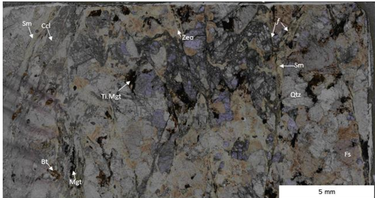
Figure 4.9. Microphotograph showing shear fault / cataclasite network in granitic gneiss (299.76 m; partial crossed-polars). The cataclasites extend within the quartz and feldspar grains. The sample is dominated by feldspar and quartz and contains interstitial biotite and titanomagnetite. The quartz grains are highly fractured and form an approximately in situ breccia (centre), whereas feldspar is typically altered to microcrystalline clay aggregates, both in situ and in cataclasite (left). Fe-oxides are typically smeared along the faults. Bt = biotite; Zeo = zeolite; Ccl = cataclasite; Sm = smectite; Ti. Mgt = titanomagnetite; Qtz = quartz; Fs = feldspar; f = fault.
