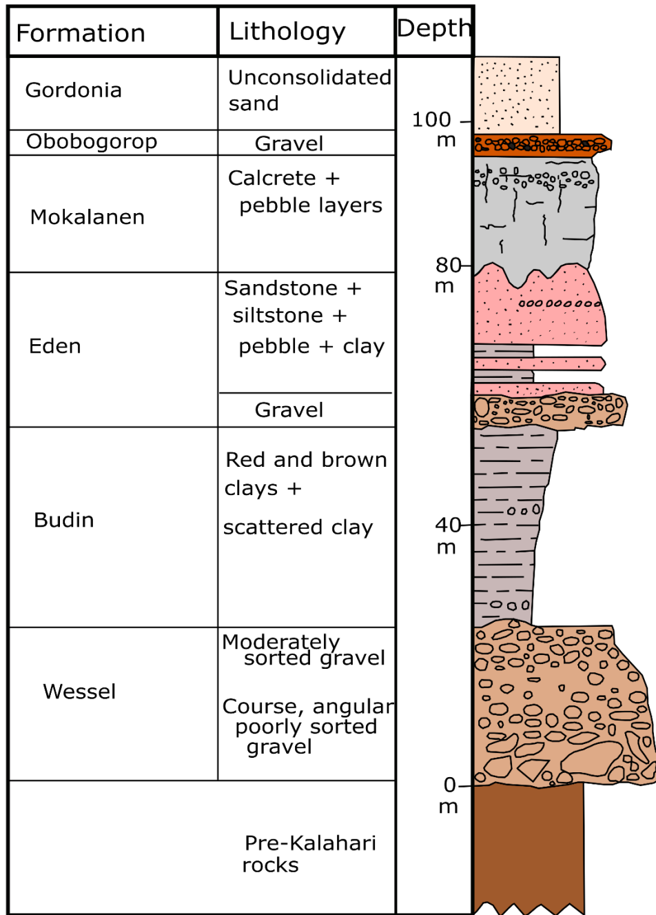
Figure 2.2. A generalized Kalahari Group stratigraphy (Adapted from Patridge et al., 2006)
