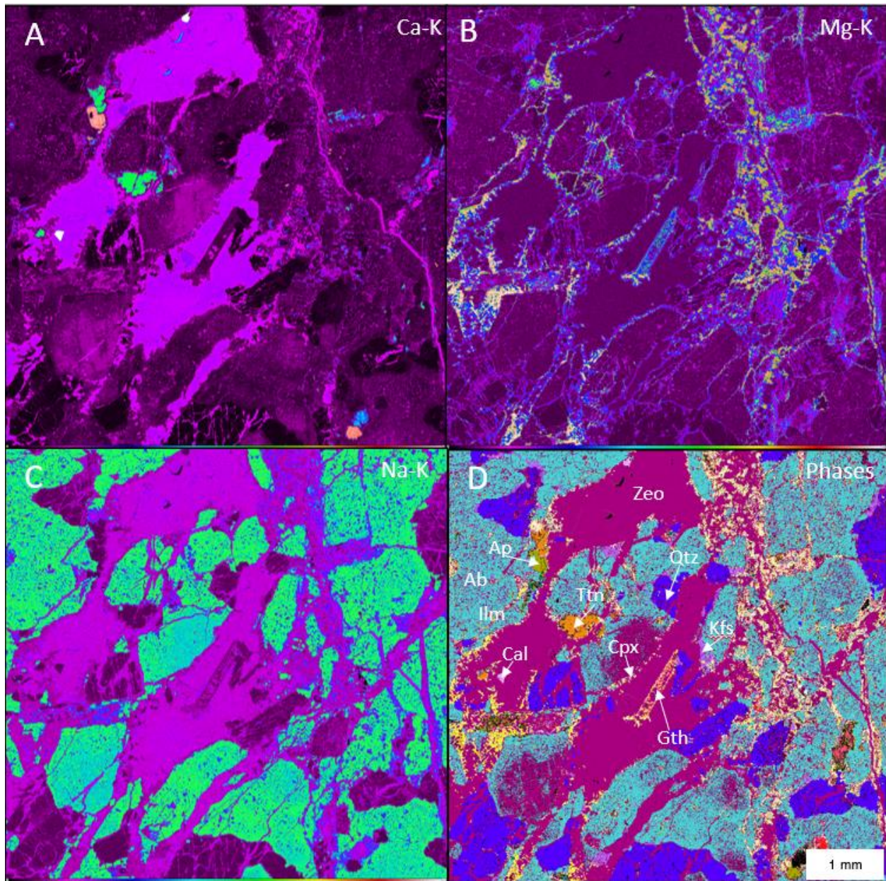
Figure 4.22. TIMA elemental maps and phase map of sample M4 GG10 (116 m) showing a steeply-inclined irregular zeolite vein network linked to a vertical fracture (left) that shows smectite + goethite > zeolite. A) Ca distribution abundant in apatite, titanite, and clinopyroxene crystals on the zeolite margins. B) Mg distribution abundant along the fractures and zeolite vugs. C) Na distribution depleted in the zeolite vugs and enriched in the matrix. D) Phase map showing albite and quartz cut by fractures and vugs filled with heulandite. For further details, see Figures 4.19 and 4.20. Elemental scale increases from dark purple (0%; left) to white (100%; right). Zeo = zeolite; Ab = albite, Qtz = quartz, Kfs = alkali feldspar; Ttn = titanite; Cal = calcite; Gth = goethite; Ap = apatite; Cpx = clinopyroxene; Ilm = ilmenite.
