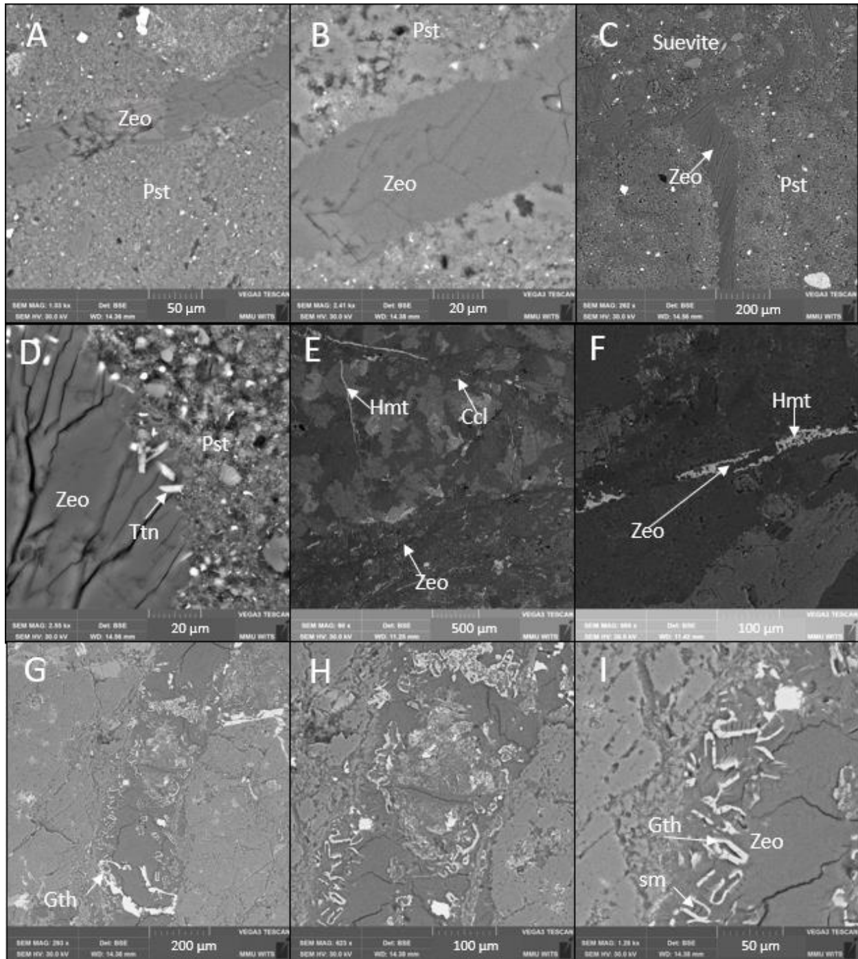
Figure 4.19. BSE images showing morphology and textures of zeolite veins across the M4 drillcore. A) Monomineralic zeolite vein in pseudotachylite from sample M4 IM9 (299 m). B) Close-up of A. C) Zeolite vein from M4 RG2 (262 m) through pseudotachylite matrix and merging in the suevite. D) Close-up of C showing titanite neoblasts along vein edge. E) Sample M4 Sill1 (261 m) showing zeolite veins with haematite rims. F) Close-up of E. G) Sample M4 GG10 (166 m) showing smectite and haematite/goethite pseudomorphs (possibly after clinopyroxene, see Figure 4.21) in zeolite veins. H-I) Close-up of G. BSE = backscattered electron; Zeo = zeolite; Pst = pseudotachylite; Ttn = titanite; Hmt = haematite; Ccl = cataclasites; Gth = goethite.
