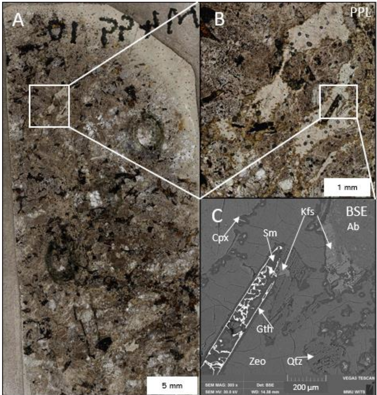
Figure 4.20. Microphotographs, and BSE image of sample M4 GG10 (166 m) showing highly irregular zeolite veins/vugs enclosing neoblastic clinopyroxene that is rimmed by smectite and skeletal haematite/goethite also rimmed by smectite. A) Overview in plane-polarized light image showing monzonite sample. B) Close up image showing white cloudy heulandite with light brown inclusions at the margins. C) BSE image showing K-feldspar metasomatic replacement of primary plagioclase in the wallrock and corroded quartz grains with zeolite replacing PDF lamellae (See also Fig. 4.2). PPL = plane polarised light; BSE = backscattered electron; Zeo = zeolite; Ab = albite; Kfs = alkali feldspar; Qtz = quartz; Cpx = clinopyroxene; Sm = smectite; Gth = goethite.
