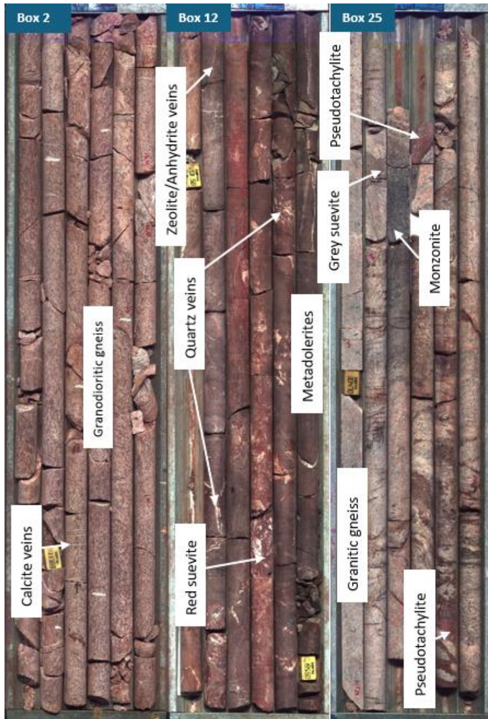
Figure 2.4 Drillcore trays from 110 – 119 m (Box 2; upper part), 194.46 – 202.6 m (Box 12; middle part) and 297.08 – 305.35 m (Box 25; deeper part), showing host rocks and vein types within the M4 drillcore. The veins show different abundances and orientations: Subhorizontal veins occur in the upper part, inclined to vertical orientations occur in the middle part, and the deeper part shows little to no veins. Box 12 shows thick pre-impact quartz veins. Drillcore width is 4.5 cm.
