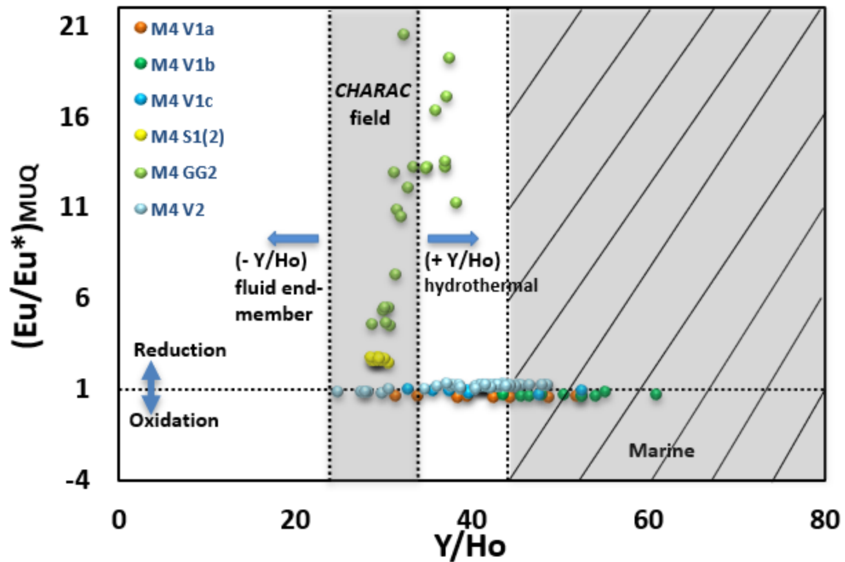
Figure 5.1. Y/Ho versus MUQ-normalised Eu anomalies (Eu/Eu^*) of calcite veins in the M4 drillcore. Hydrothermal and marine Y/Ho ratios refer to Bau and Dulski (1996) and Bau et al. (1996), respectively.
