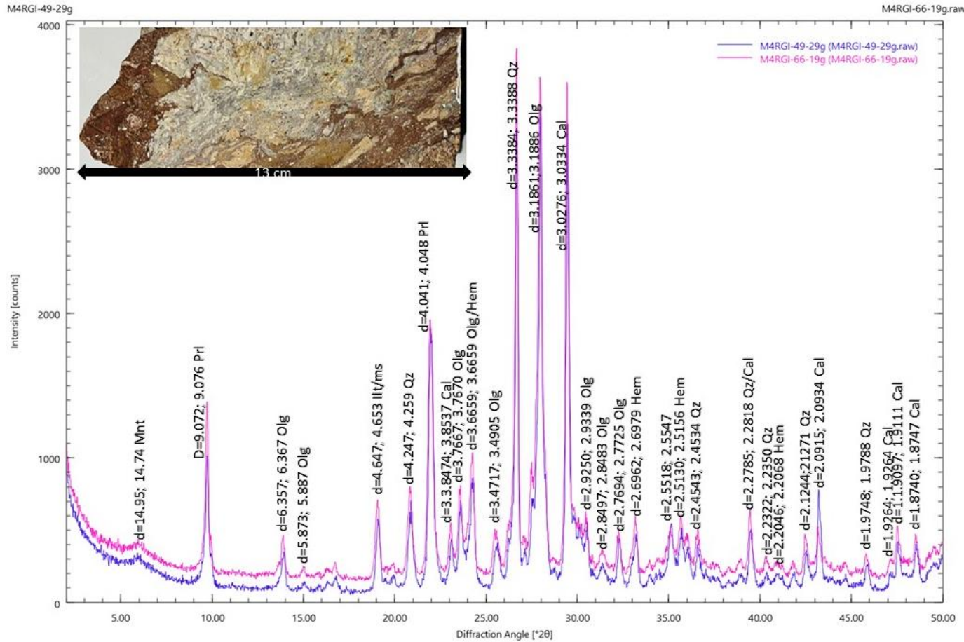
Figure 1.6. Aired-dried XRD spectra for sample M4 RG1 from 146 m showing major peaks of Mnt = Montmorillonite; Phl = pyrophyllite; Olg = oligoclase; Ill = illite; Ms = muscovite; Qz = quartz; Cal = calcite; Hem = haematite. Pink spectra shows 19g of measured rock powder and blue spectra shows 29g of measured rock powder.
