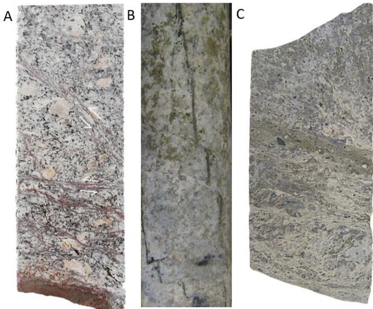
Figure 4.8. Hand specimens showing shear faults within target rocks of the M4 drillcore. A) Shear fault network showing reverse slip and monoclinic-sigmoidal internal fabric of cataclasites (131.0 m; Gibson et al., 2024a) in a granitoid gneiss. B) Shear fault network defined by white zeolite and clay cutting and displacing a vertical magnetite \pm haematite fracture in a granitic gneiss (272.73 m). C) Cataclasites and zeolite-smectite-filled fractures in granodioritic gneiss (347,4 – 354,38 m), hosting a thin suevitic dyke containing mineral and dark melt clasts. Drillcore width is 4.5 cm.
