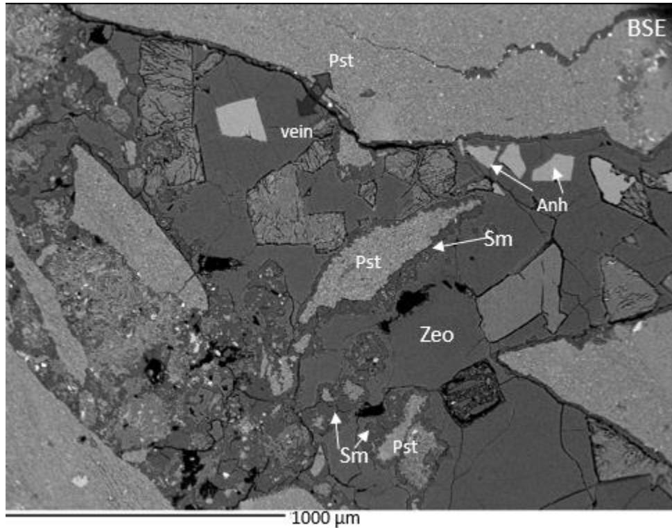
Figure 4.23. BSE image showing a polyminerale vein sample M4 ML (195.30 m). The zeolite vein cuts through the pseudotachylite and contains inclusions of anhydrite, clay and pseudotachylite clasts. BSE = backscattered electron; Zeo = zeolite; Pst = pseudotachylite; Ttn = titanite; Hmt = haematite; Ccl = cataclasites; Gth = goethite.
