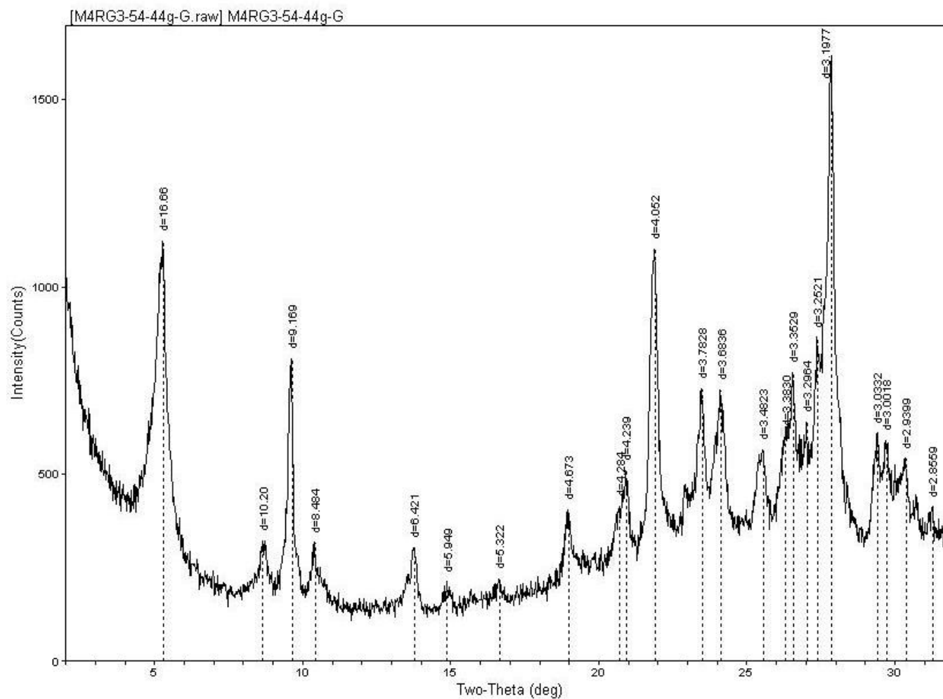
Figure 1.15. Glycolated XRD spectra for sample M4 RG3 from 301 m showing major peaks labelled in Figure 8. Spectra shows 44g of measured rock powder
