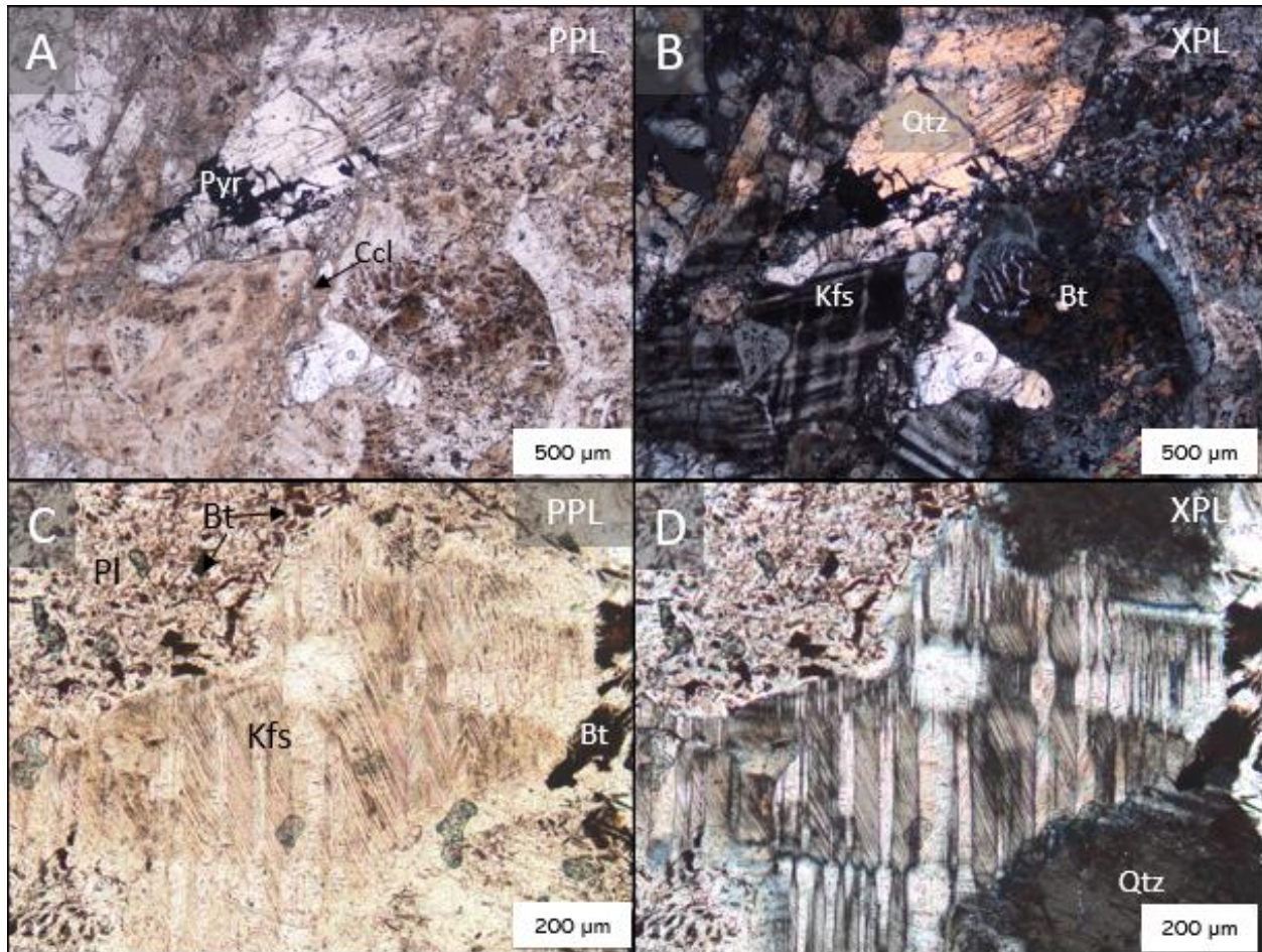
Figure 4.4. Photomicrographs of altered feldspar. A, B) Sample M4 GG15 (324 m) showing microcline with tartan twins and fine-grained alteration; above the grain is quartz grain showing PFs, PDFs, and jigsaw brecciation filled with opaques, and cataclasites in PPL and XPL. C, D) Sample M4 GG8 (152 m) showing microcline with distinct chevron pattern and plagioclase with inclusions of biotite in PPL and XPL. The microcline shows oblique planar features that show differing degrees of alteration. PPL = plane polarised light; XPL = crossed polarised light; Pyr = pyrite; Ccl = cataclasites; Kfs = alkali feldspar; Qtz = quartz; Bt = biotite; Pl = plagioclase.
