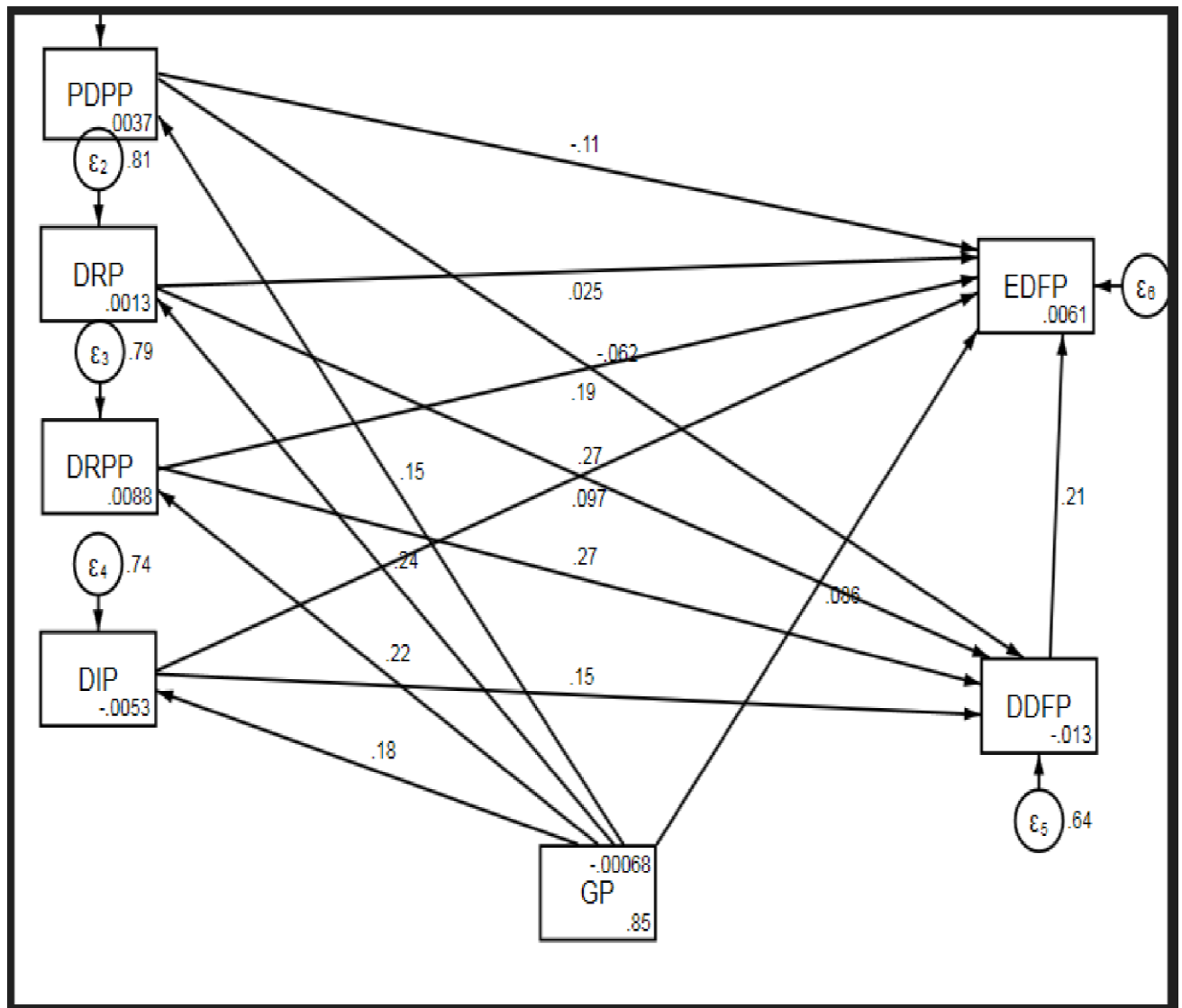
Figure 4.20: Structural Equation Pathway
