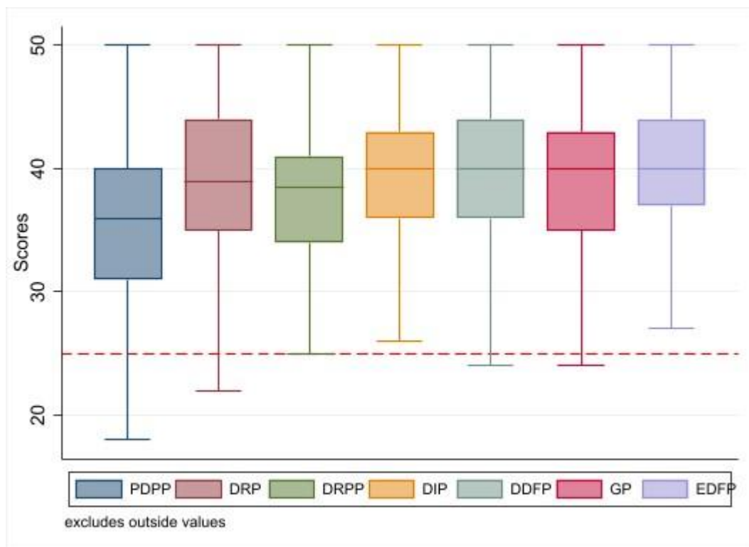
Figure 4.19: Box and whisker
