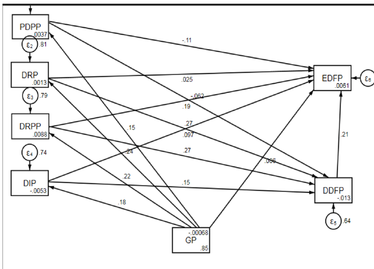
Figure 6.21: Tested Structural Equation Model
