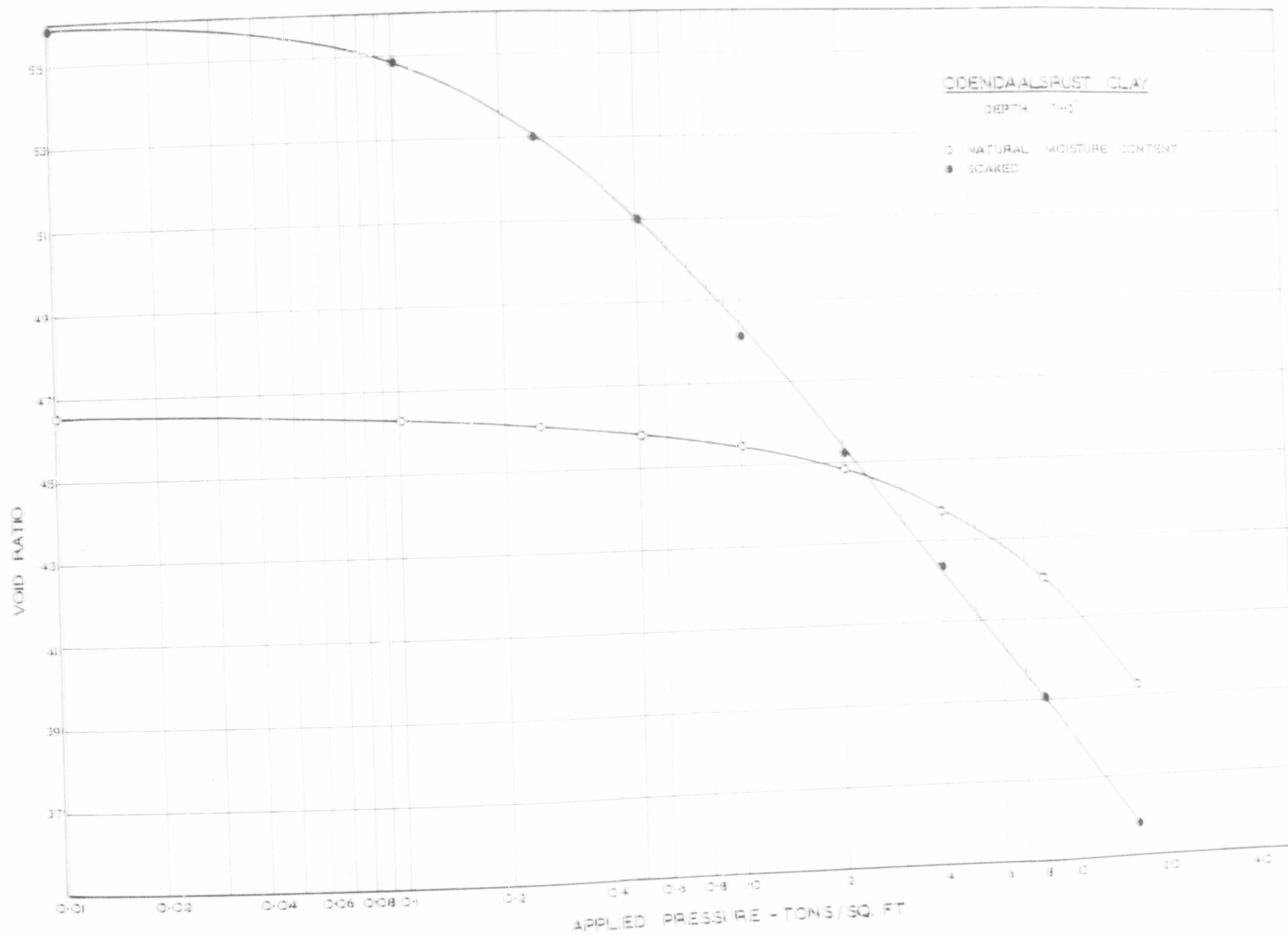
TYPICAL DOUBLE OEDOMETER CURVES FOR ODENDAALSRUST EXPANSIVE CLAY
