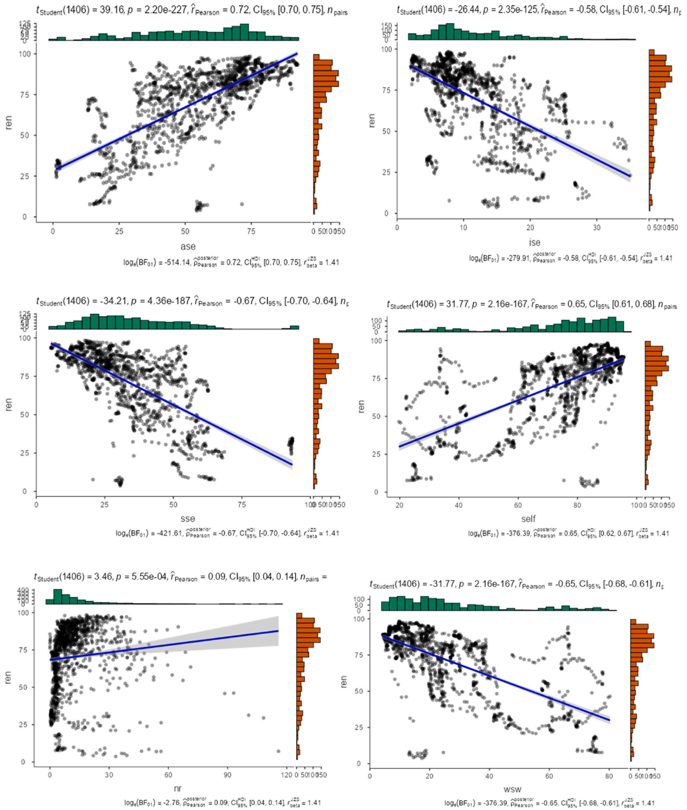
Fig. 2. A–F: Scatter plot for variables.
