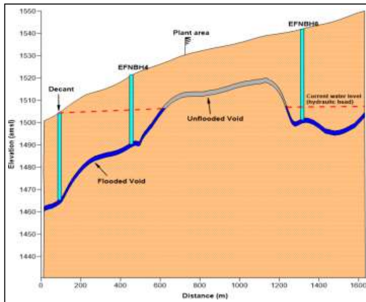
Figure 3-18: Hydrogeological profile along the line AB in Figure 3-17 (Digby Wells, 2015).
