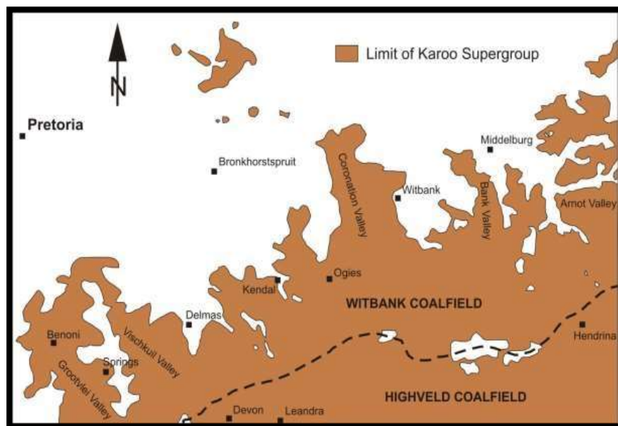
Figure 3-2. Limit of the Karoo Supergroup Rocks in the Witbank Coalfield (Hancox & Götz, 2014).
