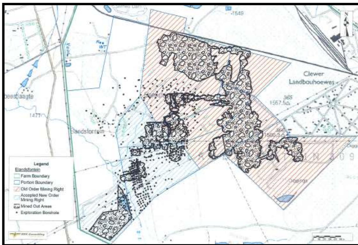
Figure 3-6: Elandsfontein Colliery old workings (Anker, 2008).
