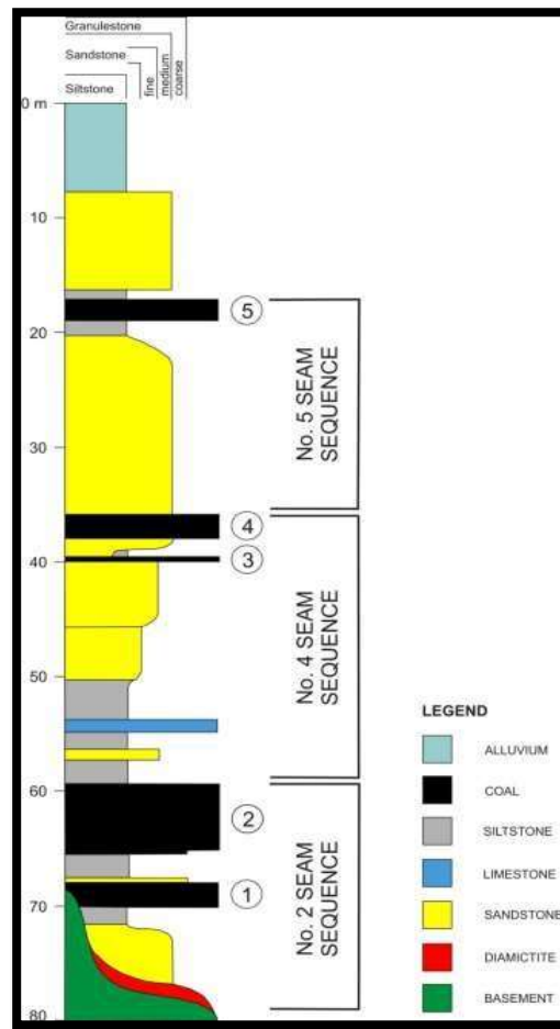
Figure 3-3. General stratigraphic column for the Vryheid Formation in the Witbank Coalfield (Hancox & Götz, 2014).
