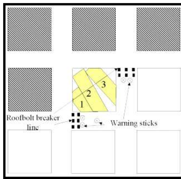
Figure 3-12: Extraction of pillars using the angled cuts method (Coaltech 2020, 2003).
