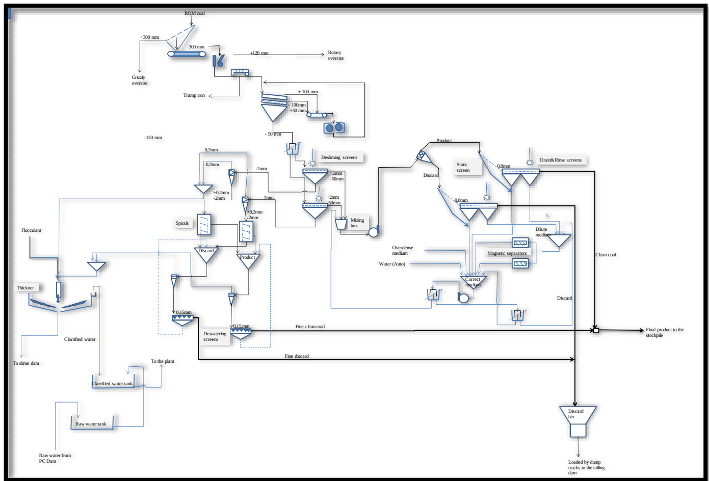
Figure 3-15: Elandsfontein Plant layout (Anker, 2008).
