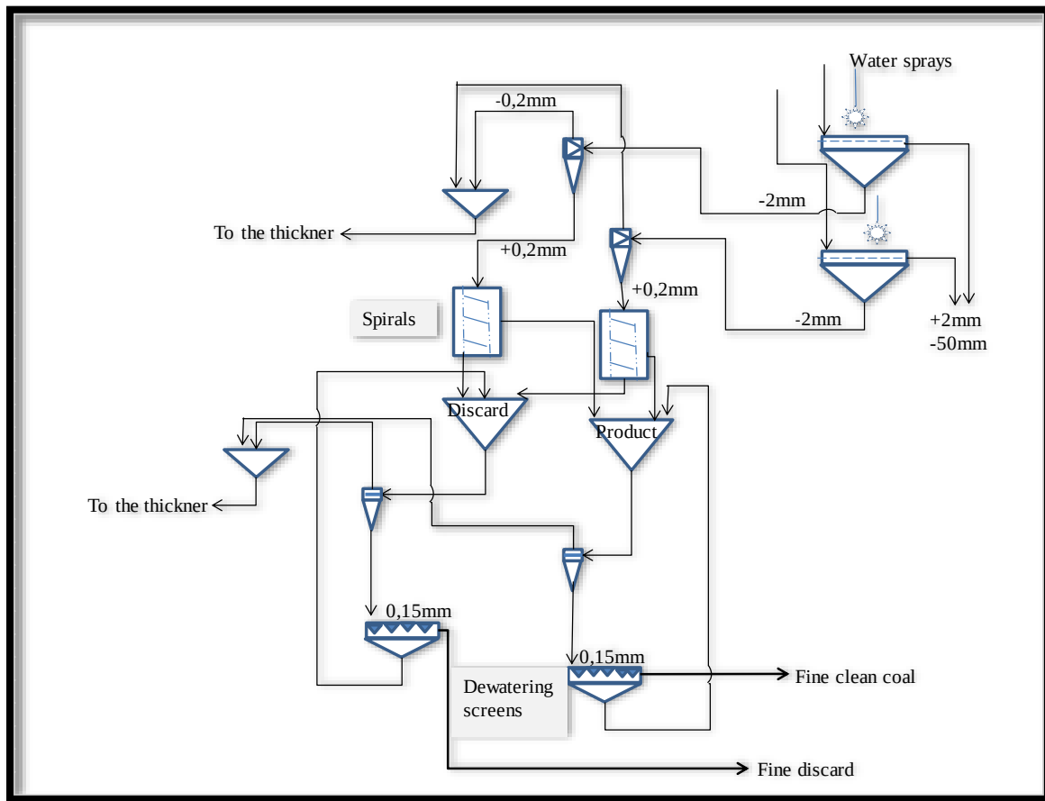
Figure 3-14: Fines treatment unit (Namane Resources, 2013).
