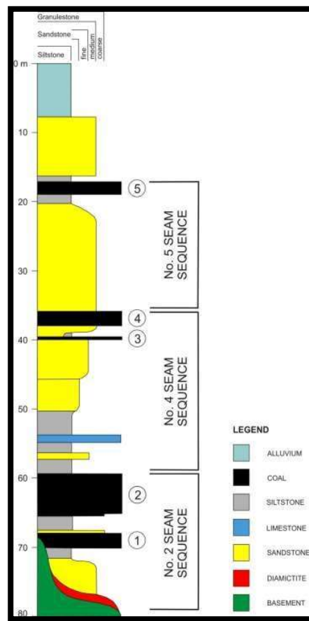
Figure 1-2: General stratigraphic column for the Vryheid Formation in the Witbank Coalfield (Hancox & Götz, 2014).
