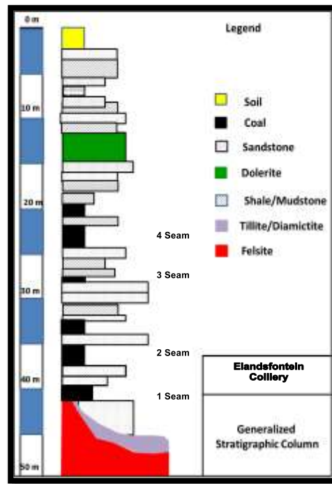
Figure 3-4: General stratigraphy at Elandsfontein Colliery (Geo Soil & Water, 2020)
