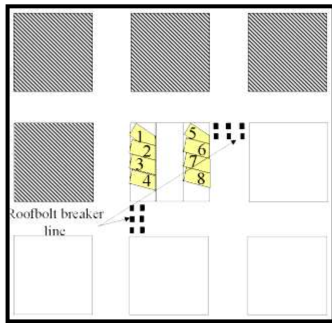
Figure 3-11: Extraction of pillars using split and fender method (Coaltech 2020, 2003).
