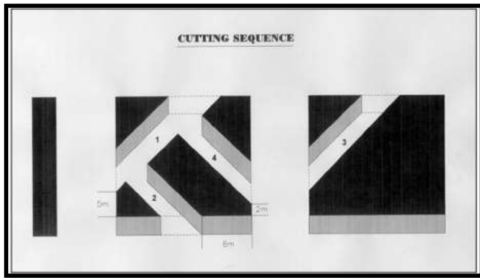
Figure 3-10: NEVID method cutting sequence method (World Intellectual Property Organisation, 2015).
