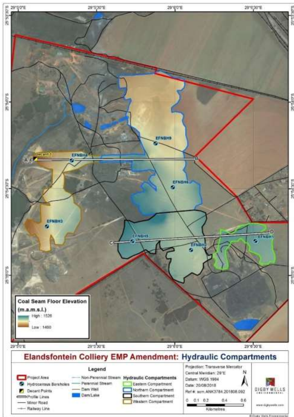
Figure 3-17: Hydraulic compartment in the mine void (Digby Wells, 2015)
