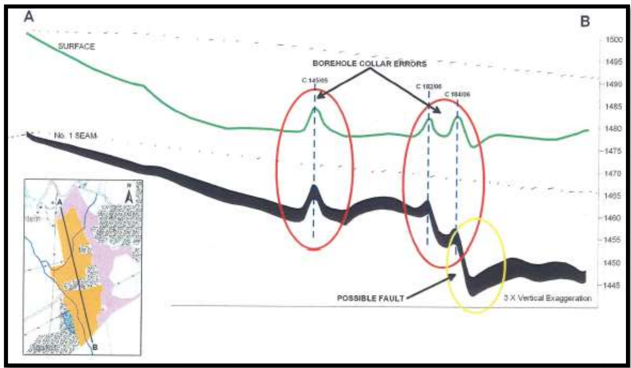
Figure 3-5: Cross-section through the No1 seam at Elandsfontein Colliery (Anker, 2008).
