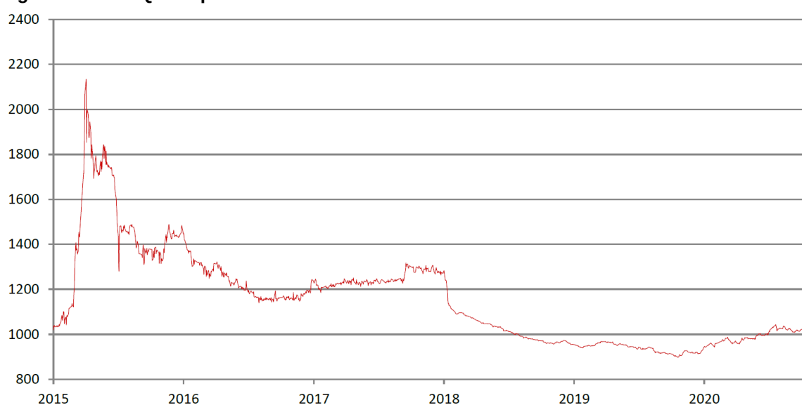
Figure 4.2: NEEQ Composite Index
