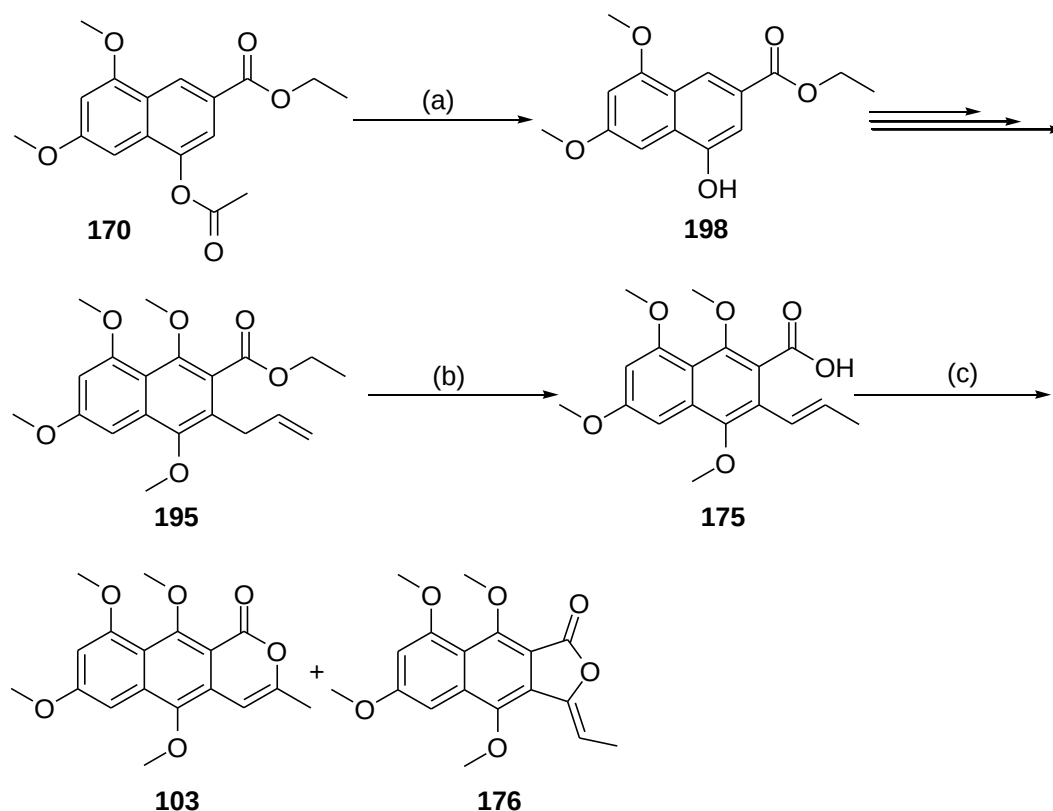
Scheme 6.1: Reagents and conditions: (a) (i) diethyl succinate, t -BuOH, t -BuOK, reflux, 2 hrs (ii) NaOAc-Ac 2 O, 130 °C, 12 hrs (iii) 1% NaOH in EtOH, rt, 6 hrs (iv) HCl (aq) (b) KOH, MeOH/H 2 O, reflux, 72 hrs (c) cat. PdCl 2 , CuCl 2 ·2H 2 O, DMF/H 2 O, O 2 (g), rt, 24 hrs.
