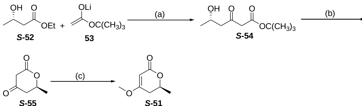
Scheme 1.9: Reagents and conditions: (a) -78^{\circ}\text{C} , THF (b) TFA, \text{CH}_2\text{Cl}_2 (c) \text{K}_2\text{CO}_3 , \text{Me}_2\text{SO}_4 , \text{Me}_2\text{CO} , reflux.
