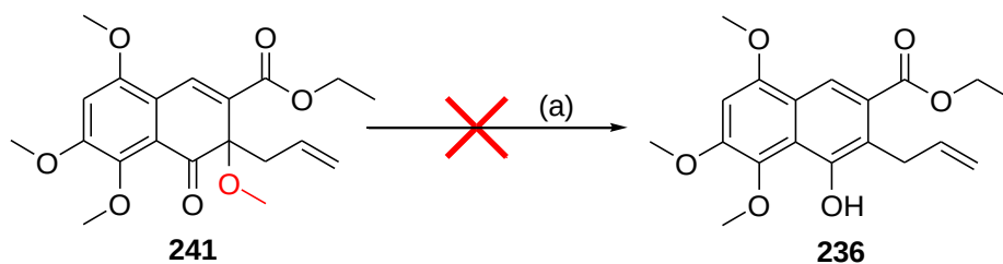
Scheme 2.64: The failed re-aromatization under mild basic conditions.
