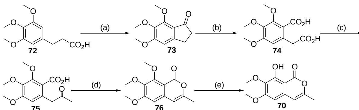
Scheme 1.13: Reagents and conditions: (a) PPA, 90 °C, 2 hrs (b) (i) (\text{EtO}_2\text{C})_2 , NaOMe, PhMe (ii) 30% \text{H}_2\text{O}_2 , KOH, MeOH (c) \text{Ac}_2\text{O} , pyridine, dry \text{Et}_2\text{O} , overnight, rt (d) \text{Ac}_2\text{O} , 2 hrs, reflux (e) \text{BBr}_3 , dry \text{CH}_2\text{Cl}_2 , -78 °C (20 min) then rt, 30 min.
