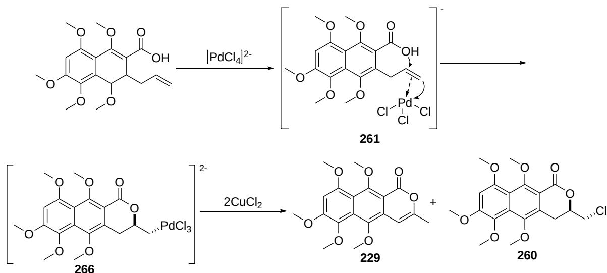
Scheme 2.82: The proposed intramolecular Wacker reaction pathway for the formation of lactones 229 and 260 .
