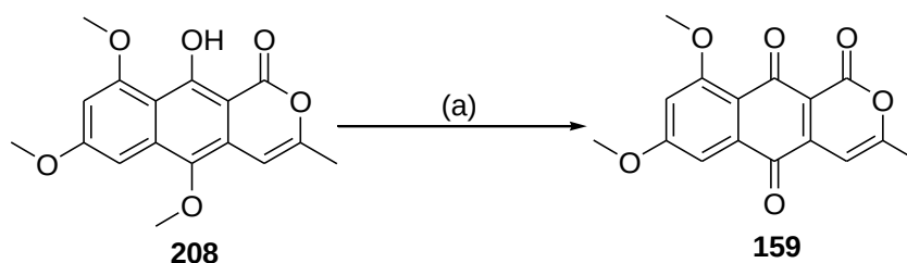
Scheme 2.39: Reagents and conditions: (a) PIFA, CH 3 CN/H 2 O, rt, 35 min, 81%.
