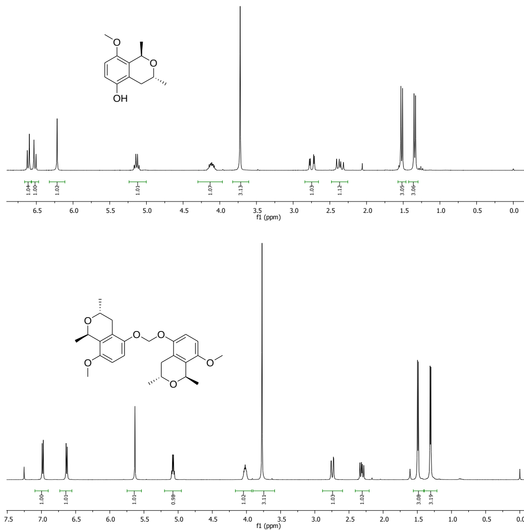
Figure 4.9: The ^1\text{H} NMR spectra of compounds trans-409 (top) and trans-410 (bottom).
