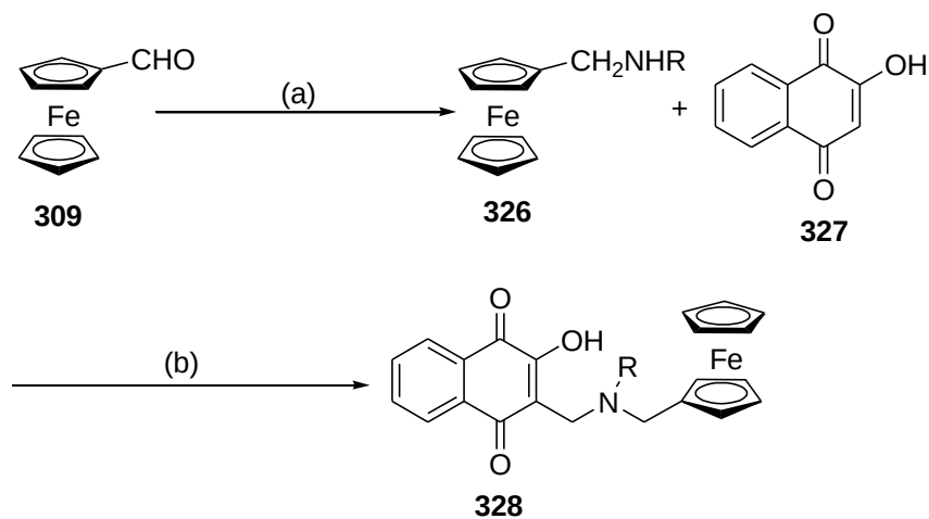
Scheme 3.8: Reagent and conditions: (a) (i) RNH 2 , t -BuMeO, reflux (ii) NaBH 4 , MeOH (b) HCHO, EtOH, reflux.
