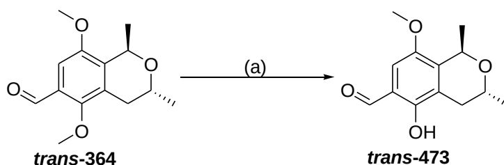
Scheme 6.11: Reagents and conditions: \text{BCl}_3 , \text{CH}_2\text{Cl}_2 , -78^\circ\text{C} \rightarrow \text{rt} .
