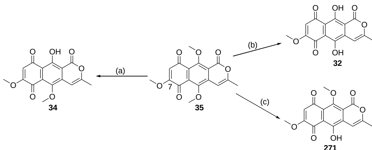
Scheme 2.90: Highlighting the 3 possible routes for demethylation of quinone intermediate 35 .
