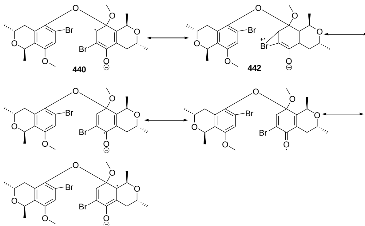
Scheme 4.62: Possible canonical forms of radical anion intermediate 440 .
