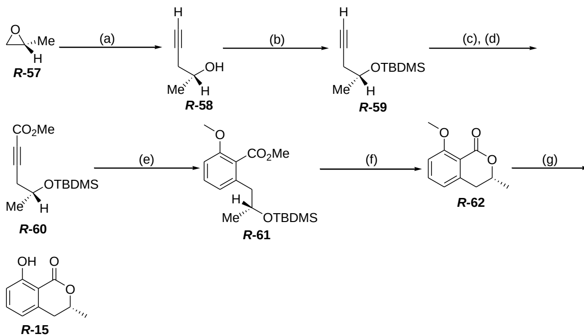
Scheme 1.11: Reagents and conditions: (a) \text{LiC}\equiv\text{CH}:\text{H}_2\text{N}(\text{CH}_2)_2\text{NH}_2 complex, DMSO, 0\text{ }^\circ\text{C} \rightarrow \text{rt} , 16 hrs (b) TBDMSCl, imidazole, DME, rt, 16 hrs (c) (i) n -BuLi, -78\text{ }^\circ\text{C} , 30 min (d) \text{ClCO}_2\text{Me} , -78\text{ }^\circ\text{C} \rightarrow \text{rt} , 2 hrs (e) 1-methoxy-1,3-cyclohexadiene, dichloromaleic anhydride, N -phenyl-13-naphthylamine, sealed tube, 185\text{ }^\circ\text{C} , 26 hrs (f) p -TsOH, \text{CH}_2\text{Cl}_2 , rt, 25 hrs (g) HBr, AcOH, reflux, 4 hrs.
