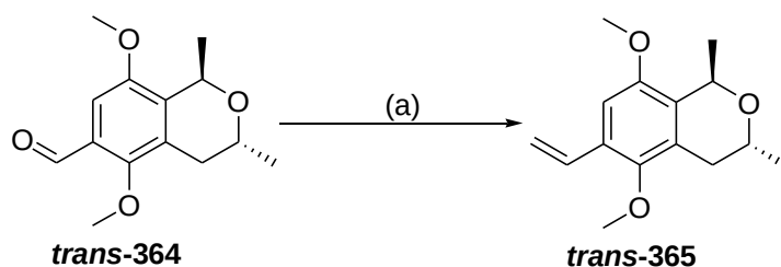
Scheme 4.11: Reagents and conditions: (a) MTPPBr, n -BuLi, THF, 0 °C → rt, 18 hrs, 82%.
