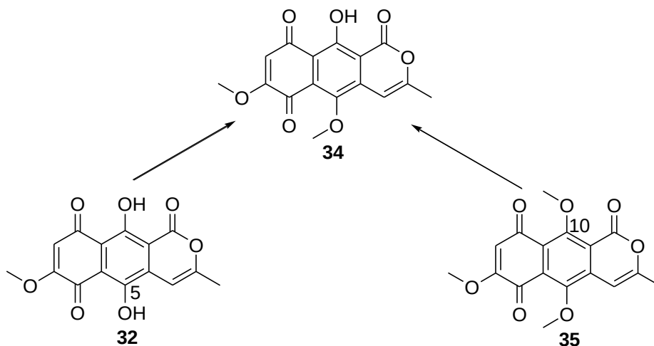
Scheme 1.4: Proposed biosynthesis of 5-methoxy-3,4-dehydroxanthomegnin 34 from anhydrofusarubin lactone 32 or its methylated analogue 35 .
