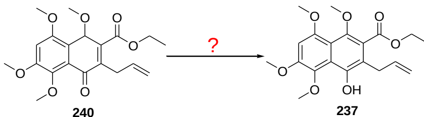
Scheme 2.60: Highlighting the desired base promoted re-aromatization step.
