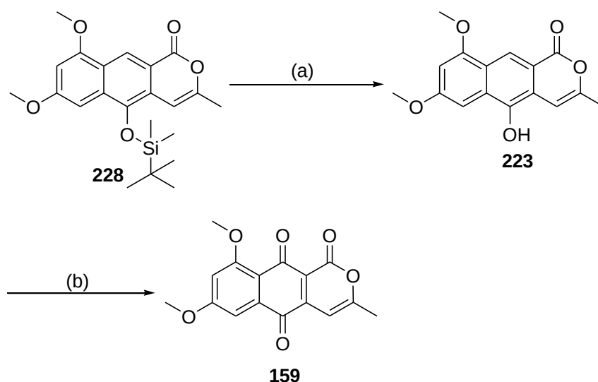
Scheme 2.51: Reagents and conditions: (a) TBAF, THF, 0 °C → rt, 24 hrs (b) CAN, CH 3 CN/H 2 O, 30 min, 10%.
