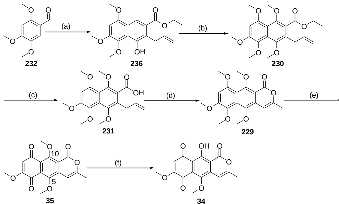
Scheme 6.5: Reagents and conditions: (a) (i) diethyl succinate, t -BuOH, t -BuOK, reflux, 2 hrs (ii) NaOAc-Ac 2 O, 130 °C, 12 hrs, 68% (iii) 1% NaOH in EtOH, rt, 6 hrs (iv) 32% aq. HCl, 79% (v) allyl bromide, K 2 CO 3 , Me 2 CO, reflux, 16 hrs, 89% (vi) 180 °C, 24 hrs, 71% (b) (i) PIFA, MeOH, rt, 15 min (ii) t -BuOK, EtOH, rt, 20 min, 60% (iii) K 2 CO 3 , Me 2 SO 4 , Me 2 CO, reflux, 18 hrs, 83% (c) (i) LiAlH 4 , Et 2 O, 0 °C → rt, 2 hrs, 80% (ii) PCC, silica, N 2 (g) (iii) NaH 2 PO 4 , NaClO 2 , H 2 O, t -BuOH, 2-methyl-2-butene, 66% (d) cat. PdCl 2 , CuCl 2 ·2H 2 O, DMF/H 2 O, O 2 (g), rt, 24 hrs, 72% (e) AgO, 55% aq. HNO 3 , 1,4-dioxane, 75% (f) BCl 3 , CH 2 Cl 2 , N 2 (g), -78 °C → rt, 20%.
