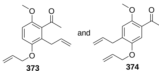
Figure 4.7: The molecular structures of allyl ethers 373 and 374 .
