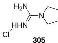
Figure 3.12: The molecular structure of pyrrolidine-1-carboxamidine hydrochloride intermediate 305 .
