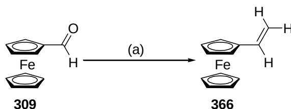
Scheme 4.12: Reagents and conditions: (a) MTPPBr, n -BuLi, THF, 0 °C → rt, 4 hrs, 85%.
