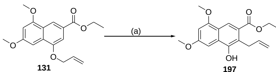
Scheme 2.24: Reagents and conditions: heat, 180 °C, N 2 (g), 24 hrs, 69%.
