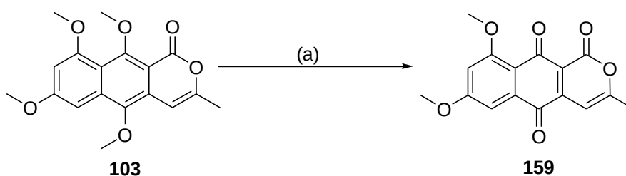
Scheme 2.34: Reagents and conditions: AgO, 55% aq. HNO 3 , 1,4-dioxane, rt, 56%.
