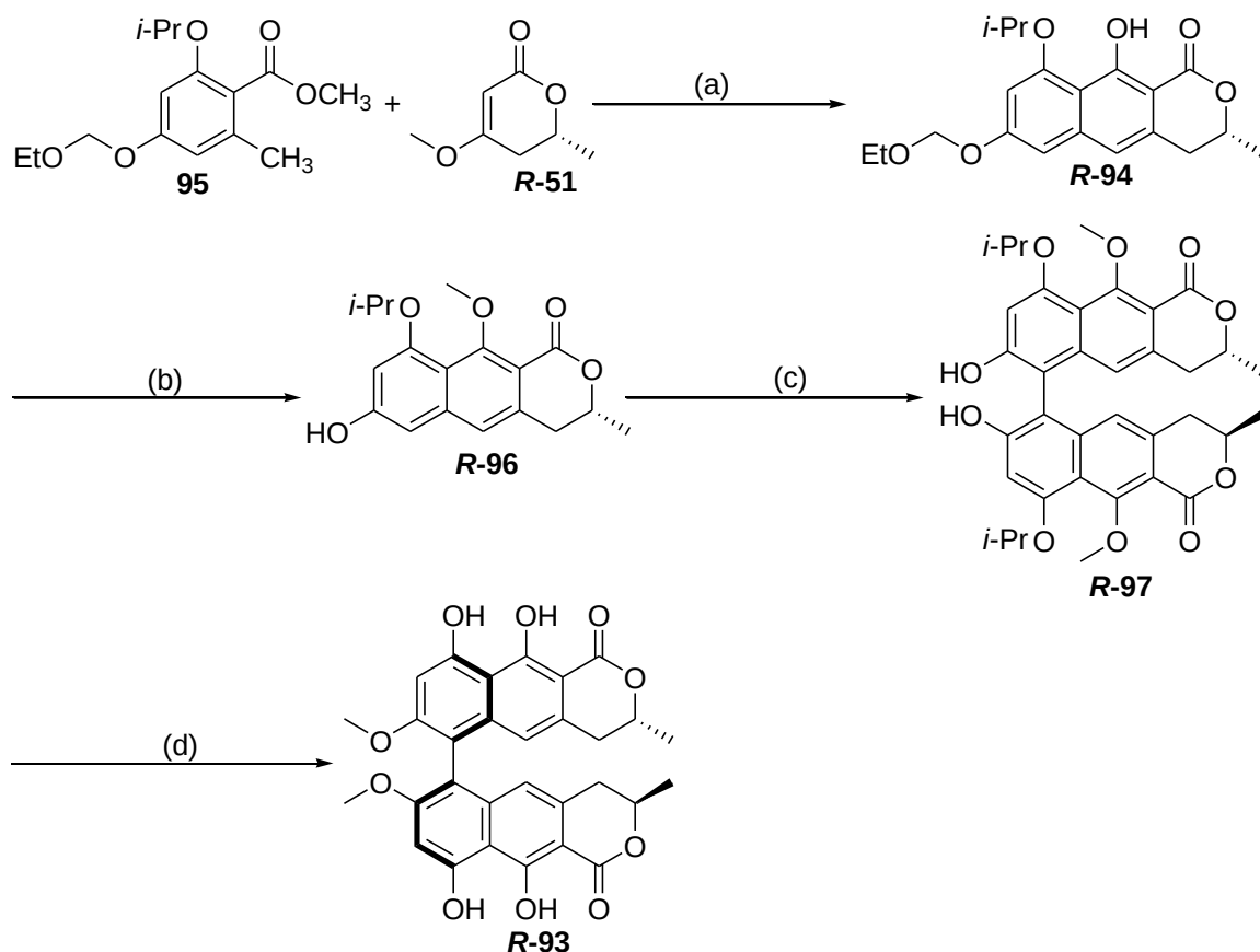
Scheme 1.17: Reagents and conditions: (a) (i) LDA, THF, -78 °C → 23 °C, overnight (ii) DDQ, benzene, 2 hrs (b) (i) K 2 CO 3 , Me 2 SO 4 , acetone, overnight (ii) 3 M aq. HCl, MeOH, 60 °C, 2 hrs (c) 20% mole VO(acac) 2 , CH 2 Cl 2 , 16 hrs (d) (i) Me 2 SO 4 , K 2 CO 3 , Me 2 CO, reflux (ii) BCl 3 , CH 2 Cl 2 , HPLC separation.
