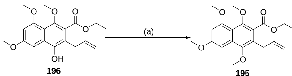
Scheme 2.26: Reagents and conditions: (a) \text{K}_2\text{CO}_3 , \text{Me}_2\text{SO}_4 , \text{Me}_2\text{CO} , reflux, 24 hrs, 89%.
