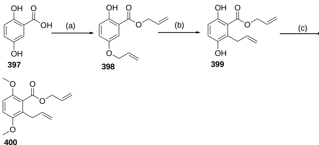
Scheme 4.27: Reagents and conditions: (a) K_2CO_3 , allyl bromide, Me_2CO , reflux, 18 hrs (b) 170\text{ }^\circ\text{C} , N_2 (g), 24 hrs (c) K_2CO_3 , Me_2SO_4 , Me_2CO , reflux, 18 hrs.
