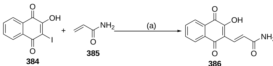
Scheme 4.21: Reagents and conditions: (a) cat. Pd(OAc) 2 , K 2 CO 3 , H 2 O, reflux.
