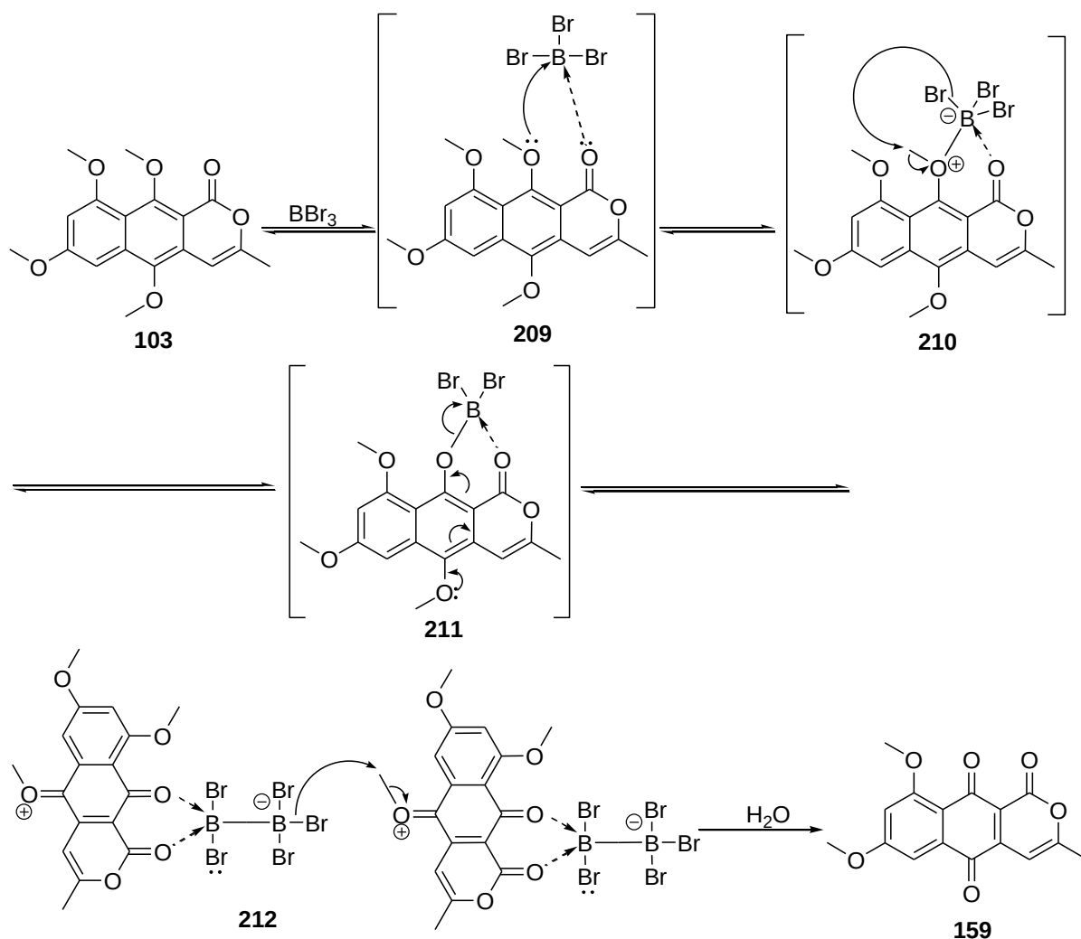
Scheme 2.38: Proposed mechanism for the oxidation of lactone 103 using \text{BBr}_3 .
