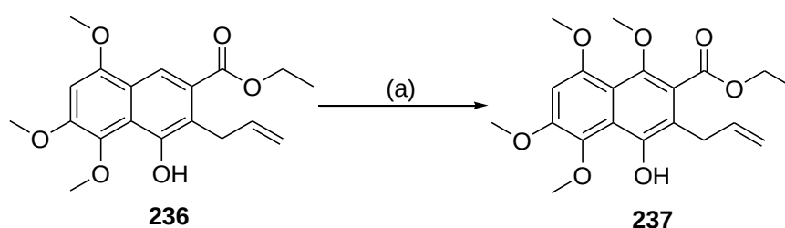
Scheme 2.57: Reagents and conditions: (a) (i) PIFA, MeOH, rt, 15 min, (ii) 21% NaOEt, EtOH, rt, 20 min, 52%.
