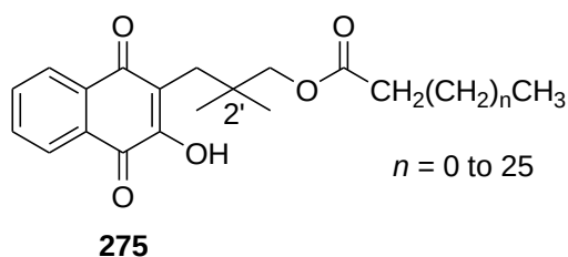
Figure 3.2: The general molecular structure of naphthoquinone aliphatic esters studied by Kongkathip and co-workers.
