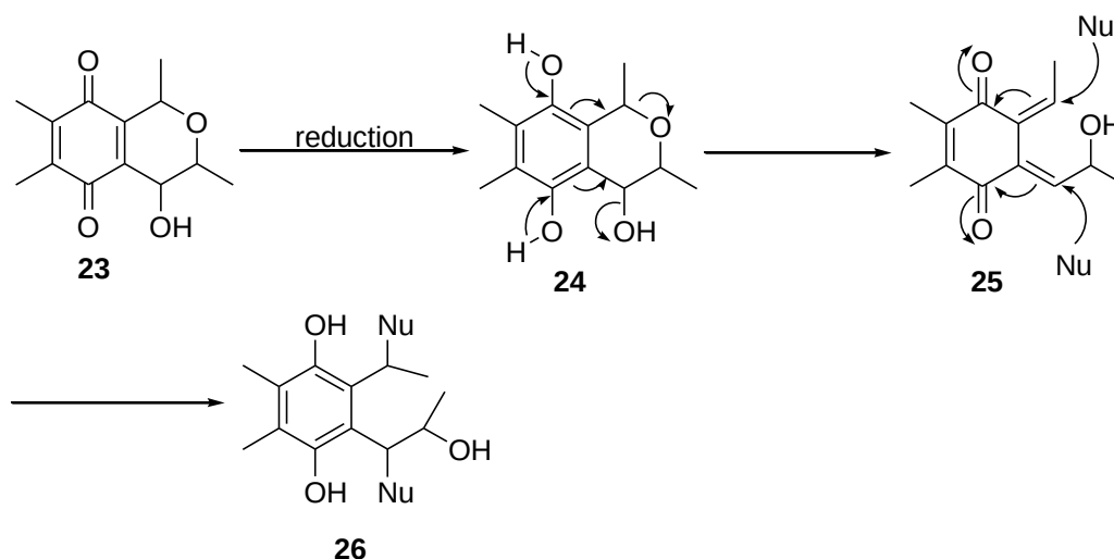
Scheme 1.1: Proposed bioreductive alkylation mechanism of quinone 23, where Nu represents biological molecules.
