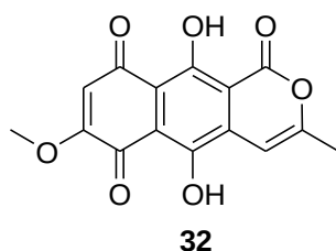
Figure 6.0: The molecular structure of anhydrofusarubin lactone 32 .
