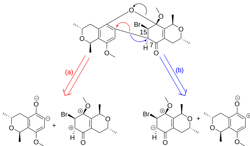
Scheme 4.55: Disconnection of the dimer JS-X10 resulting from purely ionic synthons.
