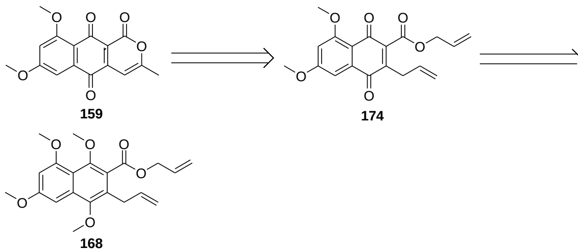
Scheme 2.10: Proposed new synthetic route encompassing naphthoquinone 174 .
