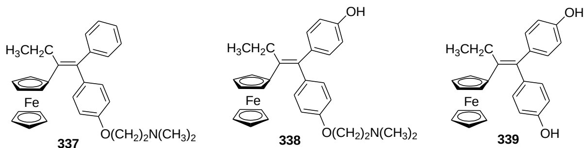
Figure 3.17: The molecular structures of ferrocifen 337 , hydroxyferrocifen 338 and ferrocenyl diphenol 339 .
