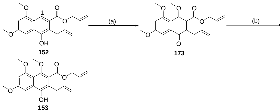
Scheme 2.6: Reagents and conditions: (a) PIFA, MeOH, rt, 15 min (b) t -BuOK, EtOH, rt, 20 min, 58% (over two steps).
