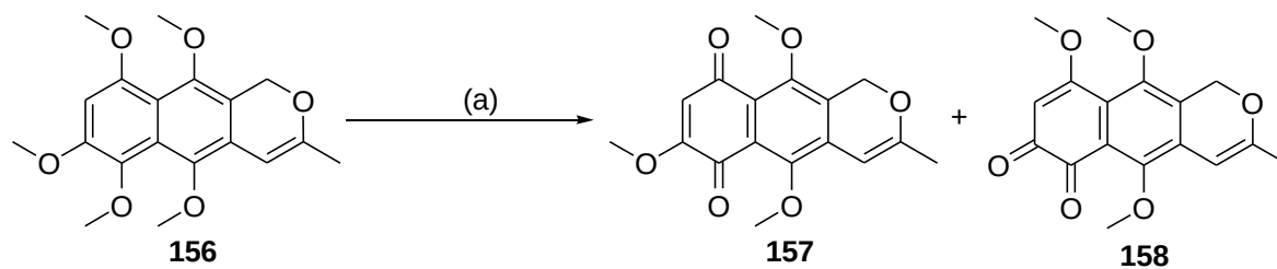
Scheme 2.89: Reagents and conditions: AgO, 55% aq. HNO 3 , 1,4-dioxane, rt.
