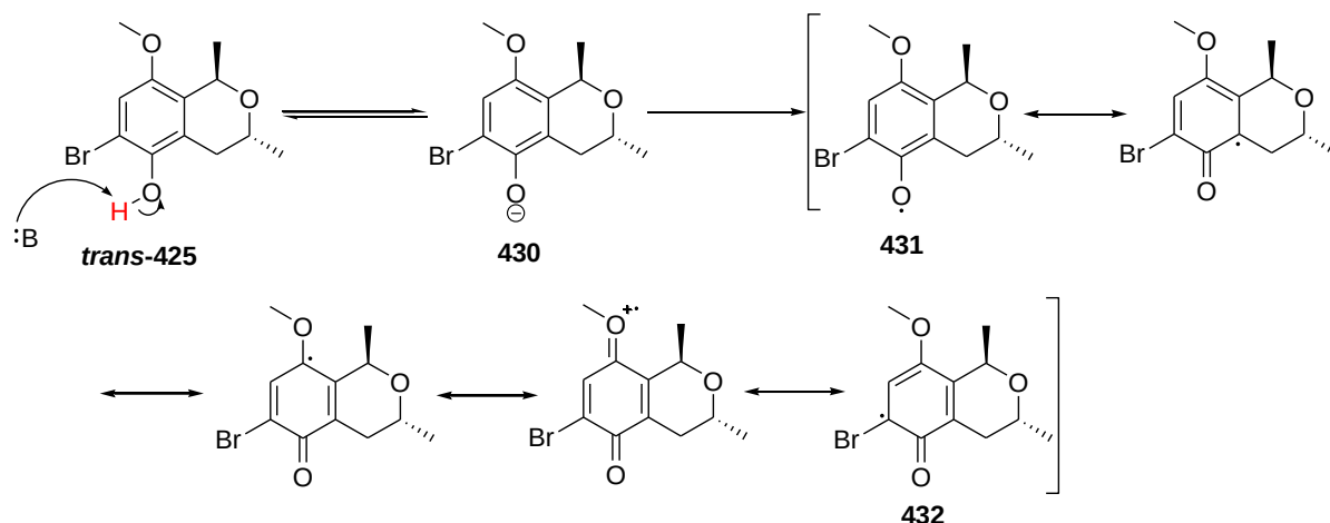
Scheme 4.57: The formation of radical intermediate from anion 430 under basic conditions.
