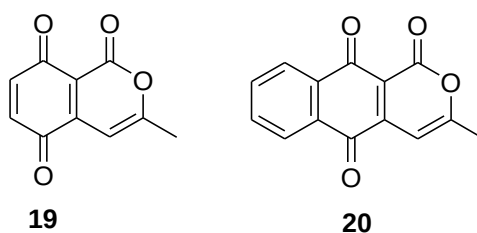
Figure 1.7: The methyl substituted pyranoquinones, 3-methyl-1 H -isochromene-1,5,8-trione 19 and 3-methyl-1 H -benzo[ g ]isochromene-1,5,10-trione 20 .
