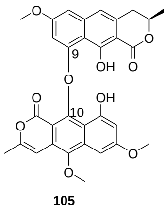
Figure 1.19: The molecular structure of planifolin 105 .
