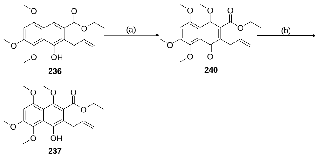
Scheme 2.59: Reagents and conditions: (a) PIFA, MeOH, rt, 15 min (b) 21% NaOEt, EtOH, rt, 20 min.
