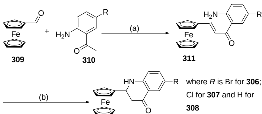
Scheme 3.5: Reagents and conditions: (a) NaOH (b) K-10, MW or AcOH/H 3 PO 4 , rt.
