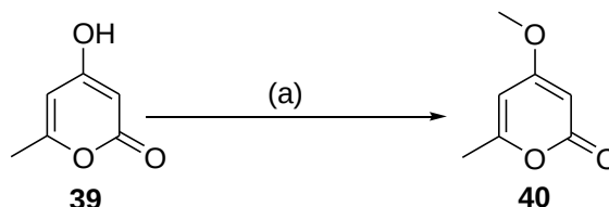
Scheme 1.9: Reagents and conditions: (a) Me 2 SO 4 , K 2 CO 3 , Me 2 CO, reflux.
