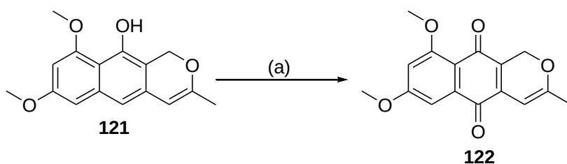
Scheme 1.32: Reagents and conditions; (a) CAN, H 2 O/CH 3 CN, rt, 30 min.
