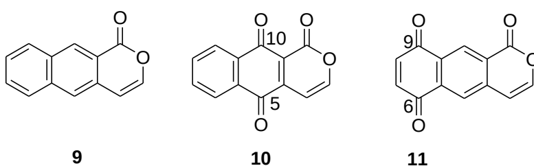
Figure 1.3: The basic molecular structures of isocoumarin 9 and pyranonaphthoquinones 10 and 11 .
