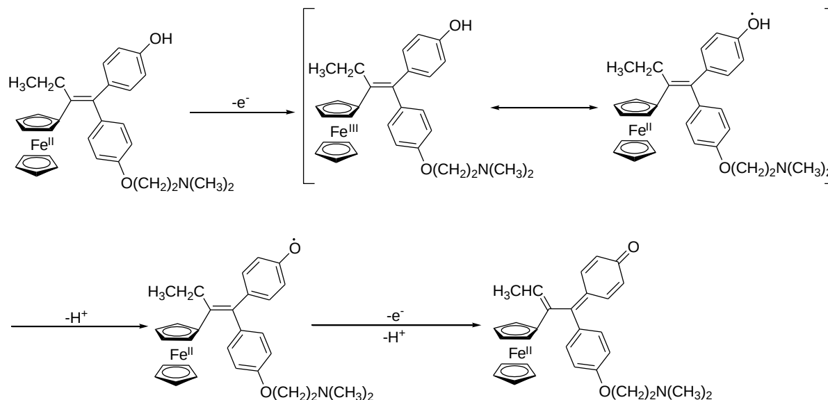
Scheme 3.12: The proposed mechanism of activation of hydroxyferrocifen.
