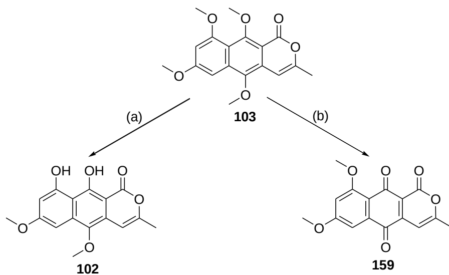
Scheme 1.36: Reagents and conditions; (a) BBr 3 , CH 2 Cl 2 , -78 °C (b) AgO, 55% aq. HNO 3 , 1,4-dioxane.
