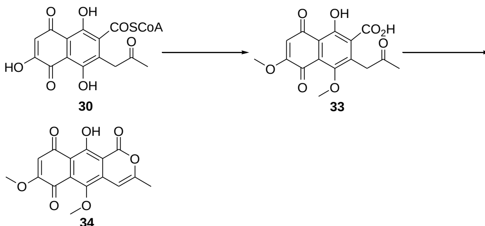
Scheme 1.3: Proposed biosynthesis of 5-methoxy-3,4-dehydroxanthomegnin from naphthoquinone 30 .
