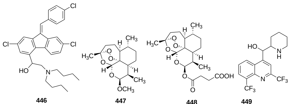
Figure 5.1: The molecular structures of lumefantrine 446 , artemether 447 , artesunate 448 and mefloquine 449 .
