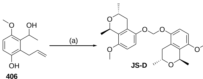
Scheme 6.10: Reagents and conditions: (a) t -BuOK, NMP, 110 °C, 30 min.
