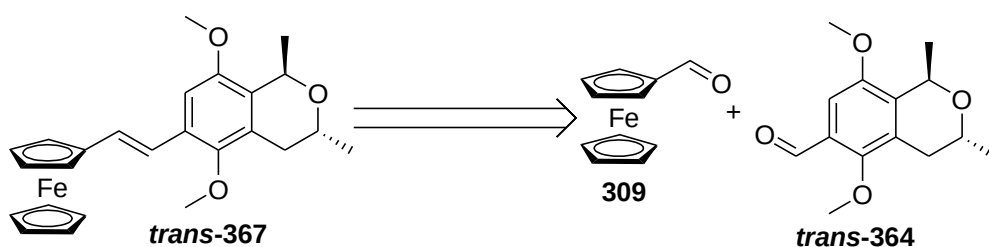
Scheme 4.2: Retrosynthetic analysis for the synthesis of ferrocenyl 3,4-dihydroisochromene trans-367 .
