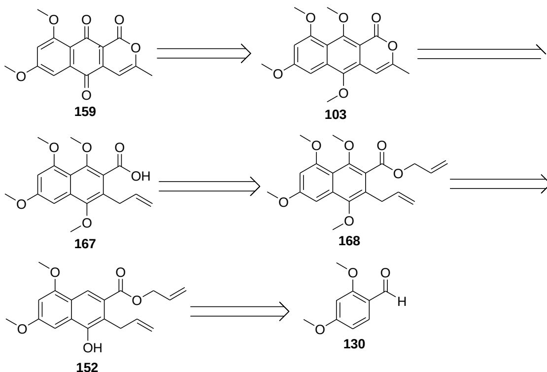
Scheme 2.2: Retrosynthetic analysis towards the synthesis of dehydroherbarin lactone 159 .
