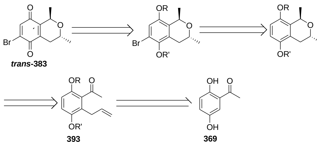
Scheme 4.25: Retrosynthetic analysis towards the synthesis of 6-bromo-3,4-dihydropyranobenzoquinone trans - 383 .
