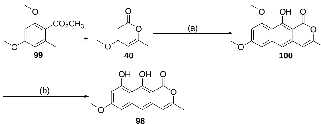
Scheme 1.18: Reagents and conditions: (a) 2.0 equiv. LDA, THF, -78 °C → rt then aq. HCl (b) BBr 3 , CH 2 Cl 2 , rt.
