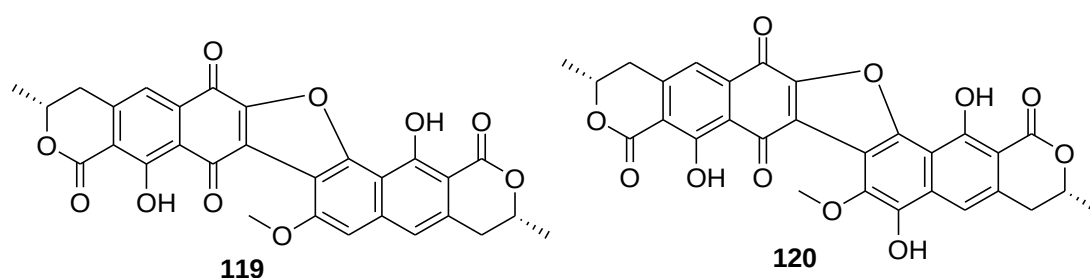
Figure 1.24: The molecular structures for rubrosulphin 119 and viopurpurin 120 .
