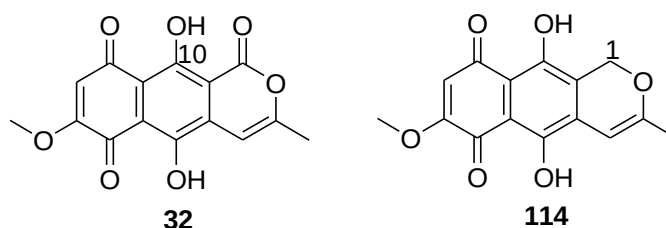
Figure 1.20: The molecular structure of anhydrofusarubin lactone 32 and anhydrofusarubin 114 .
