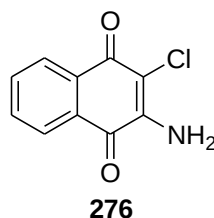
Figure 3.3: The molecular structure of 2-amino-3-chloro-1,4-naphthoquinone 276 .
