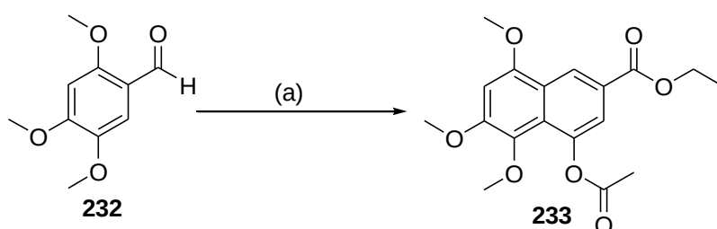
Scheme 2.53: Reagents and conditions: (a) (i) diethyl succinate, t -BuOK/ t -BuOH, reflux, N 2 (g), 4 hrs (ii) 32% aq. HCl (iii) NaOAc/Ac 2 O, 130 °C, N 2 (g), overnight, 68%.
