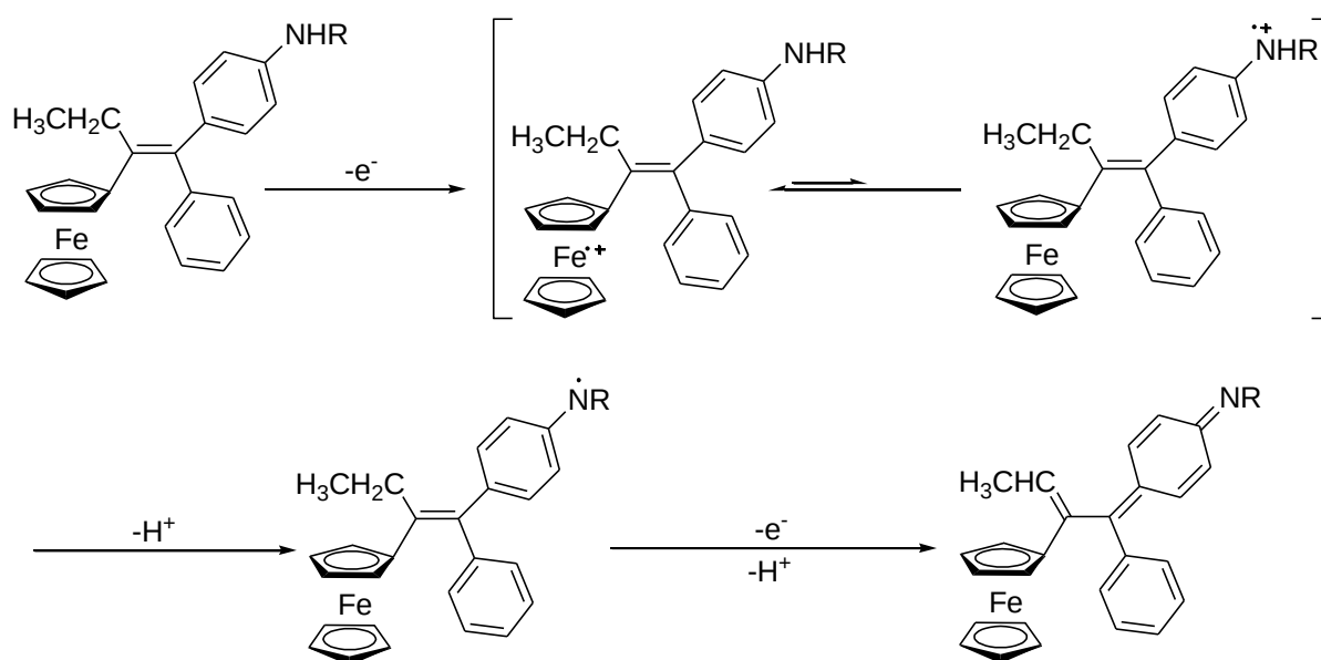
Scheme 3.13: Proposed mechanism of activation of ferrocenyl compounds 349 and 350 ; where R is \text{H} for compound 349 and acetyl group for compound 350 .
