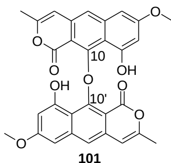
Figure 1.17: The molecular structure of eriocauline 101 .
