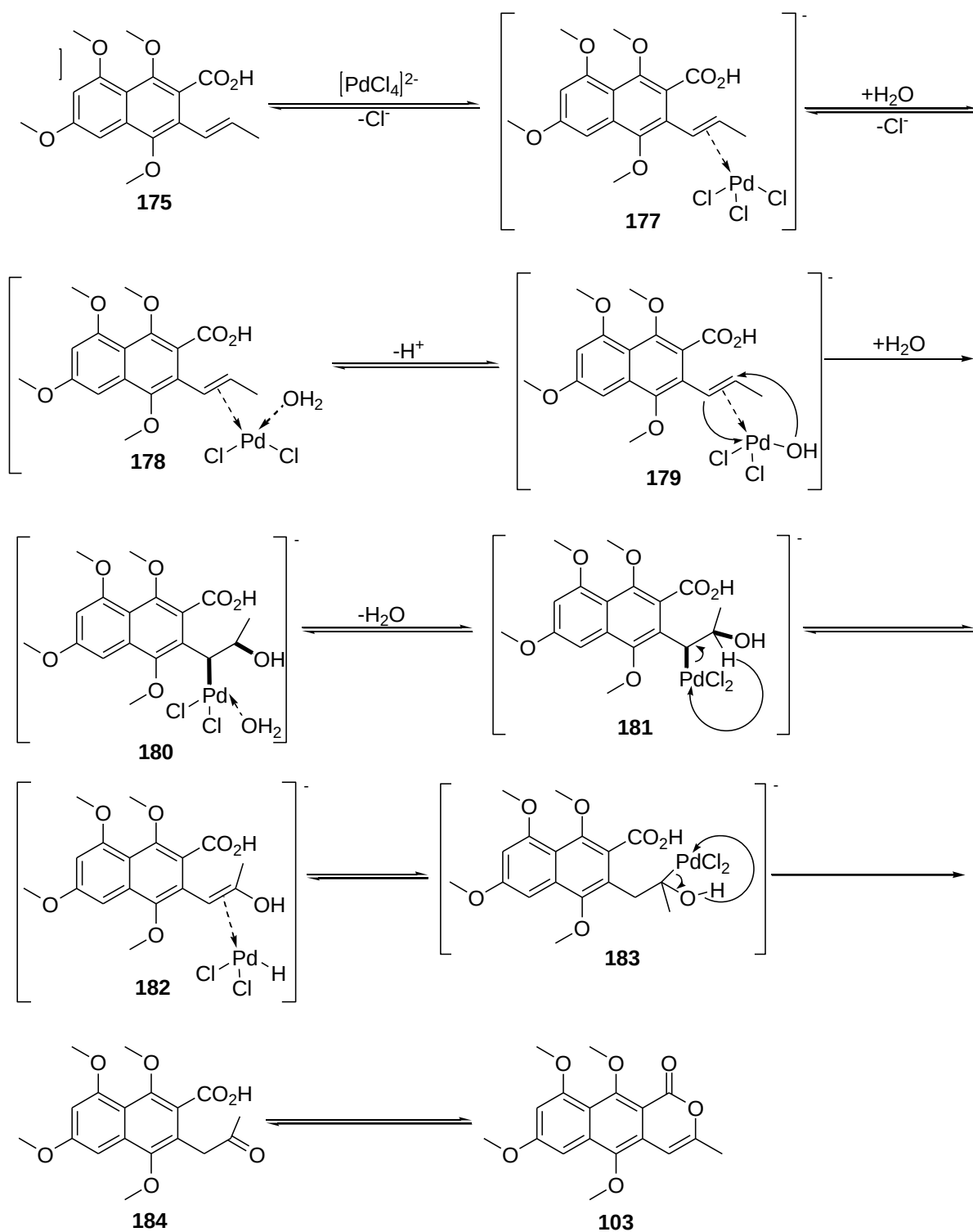
Scheme 2.15: Wacker inner-sphere mechanism for the formation of the 6-membered ring lactone 103 .
