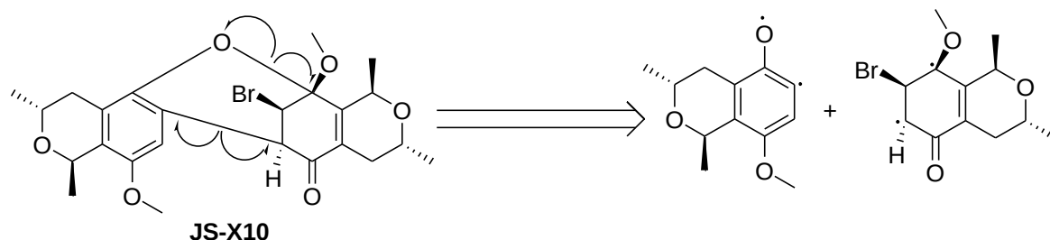
Scheme 4.65: Disconnection of the dimer JS-X10 resulting from purely radical synthons.
