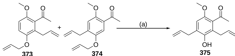
Scheme 4.6: Reagents and conditions: (a) 170 °C, \text{N}_2 (g), 24 hrs, 71%.
