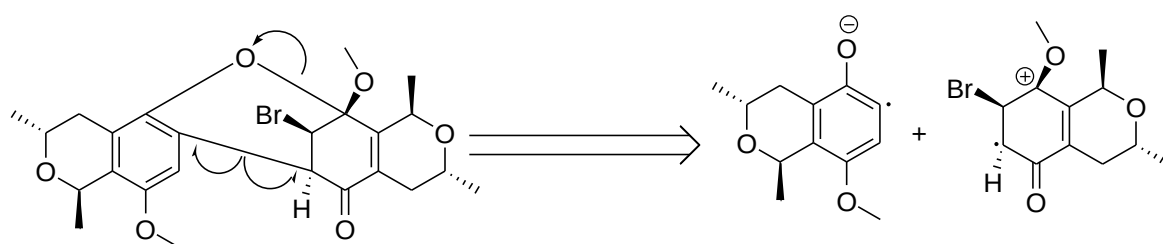
Scheme 4.56: Disconnection of the dimer resulting from radical-ionic synthons.
