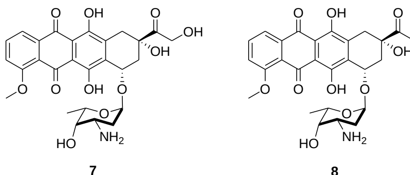
Figure 1.2: The molecular structures of anthraquinones, doxorubicin 7 and daunorubicin 8 .
