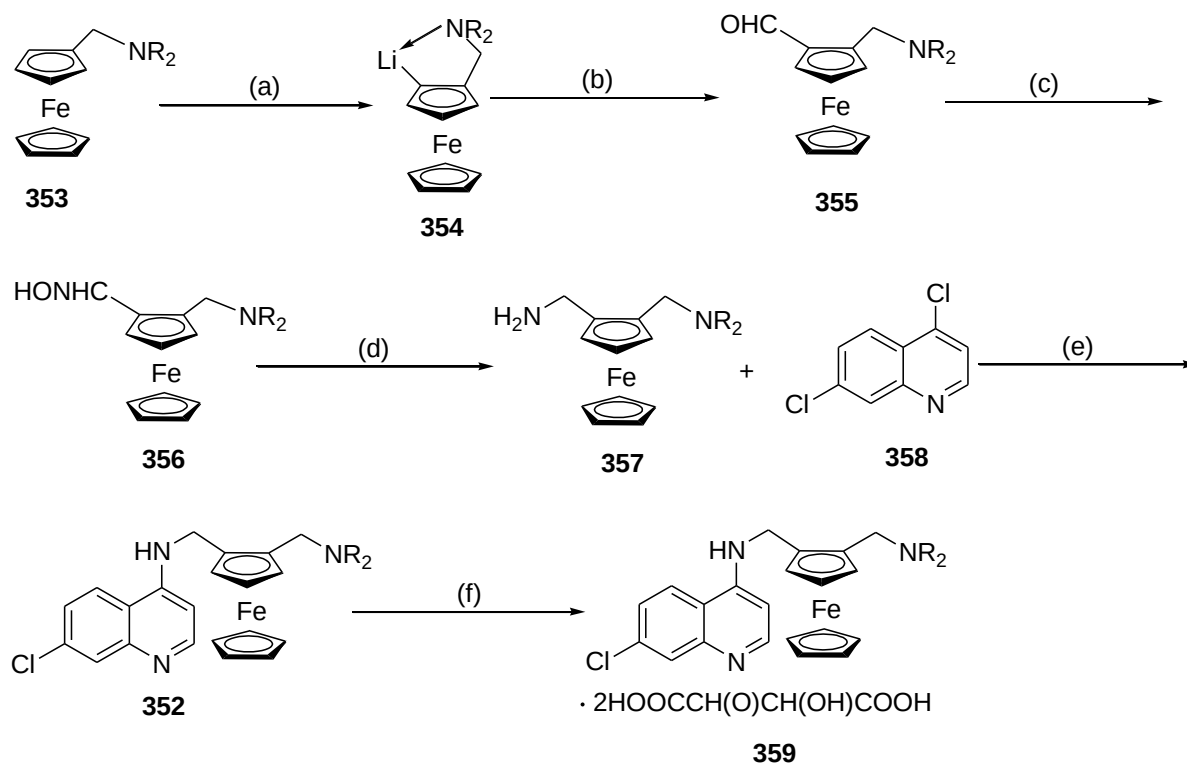
Scheme 3.14: Reagents and conditions: (a) n -BuLi, Et 2 O (b) DMF, Et 2 O (c) NH 2 OH.HCl, NaOH, EtOH/H 2 O (d) LiAlH 4 /THF (e) K 2 CO 3 , NMP (f) (CH(OH)CO 2 H) 2 , HCl/Me 2 CO (where R 2 stands for N,N -dimethyl group).
