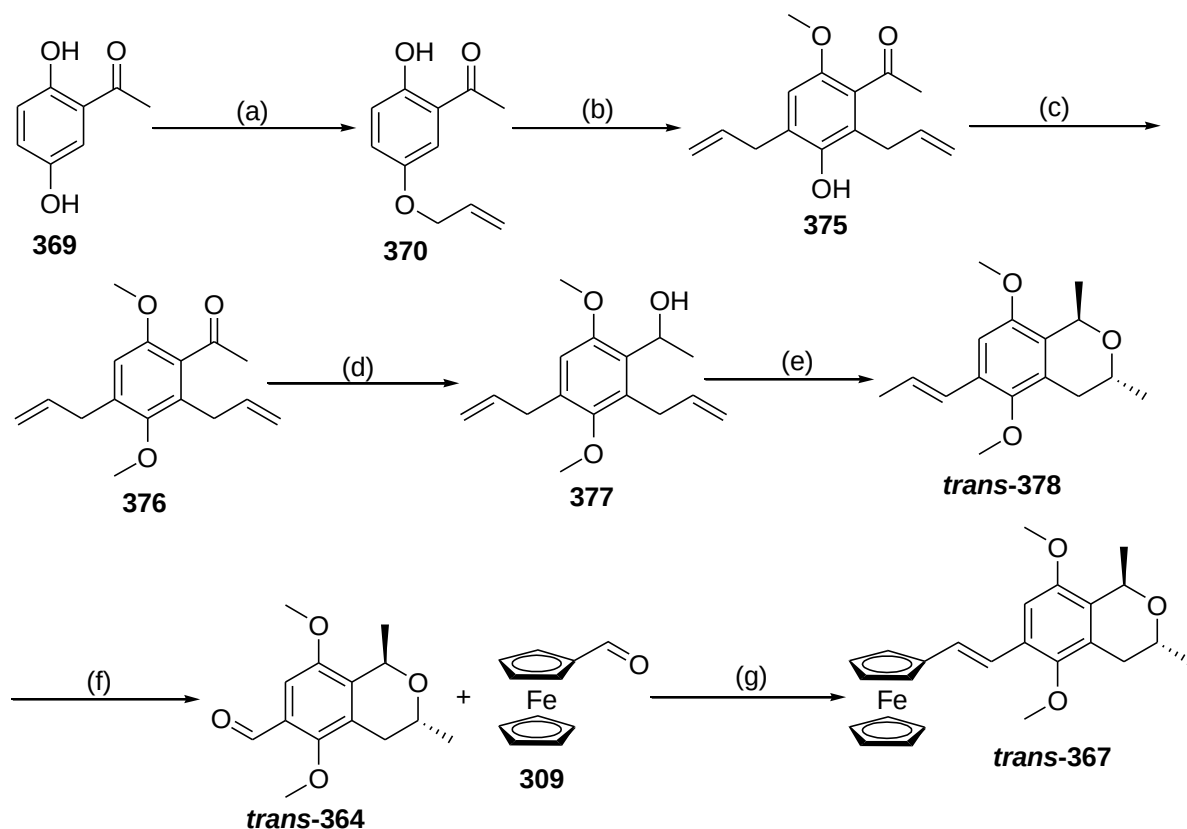
Scheme 6.7: Reagents and conditions: (a) allyl bromide, K_2CO_3 , Me_2CO , reflux, 18 hrs, 62% (b) Me_2SO_4 , K_2CO_3 , Me_2CO , reflux, 72 hrs, 82% (c) (i) 170 °C, N_2 (g), 24 hrs (ii) allyl bromide, K_2CO_3 , Me_2CO , reflux, N_2 (g), 18 hrs, 74% (iii) 170 °C, N_2 (g), 24 hrs, 71% (iv) Me_2SO_4 , K_2CO_3 , Me_2CO , reflux, 18 hrs, 87% (d) LiAlH_4 , THF, N_2 (g), 0 °C \rightarrow rt, 12 hrs, 71% (e) t -BuOK, NMP, 110 °C, 30 min, 63% (f) O_3 (g), CH_2Cl_2 , -78 °C then N_2 (g), (CH_3)_2S , 68% or; cat. OsO_4 , NaIO_4 , H_2O , 1,4-dioxane, rt, 12.5 hrs, 84% (g) TiCl_4 , Zn, THF, 14 hrs, 82%.
