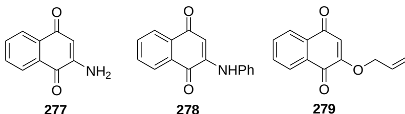
Figure 3.4: The molecular structures of 2-amino-1,4-naphthoquinone 277 , 2-(phenylamino)-1,4-naphthoquinone 278 and 2-(allyloxy)-1,4-naphthoquinone 279 .
