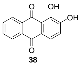
Figure 1.9: The molecular structure of alizarin 38 .
