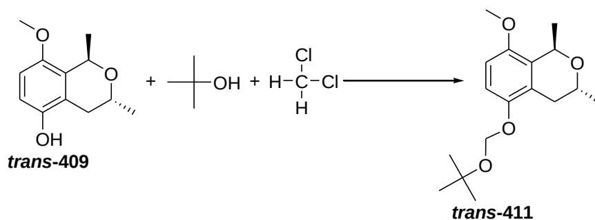
Scheme 4.42: The possible reaction equation for the formation of trans-411 .
