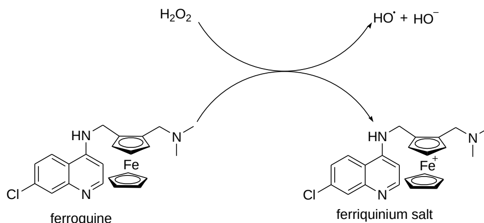
Scheme 3.15: The schematic representation of the oxidation of ferroquine into ferriquinium ion.
