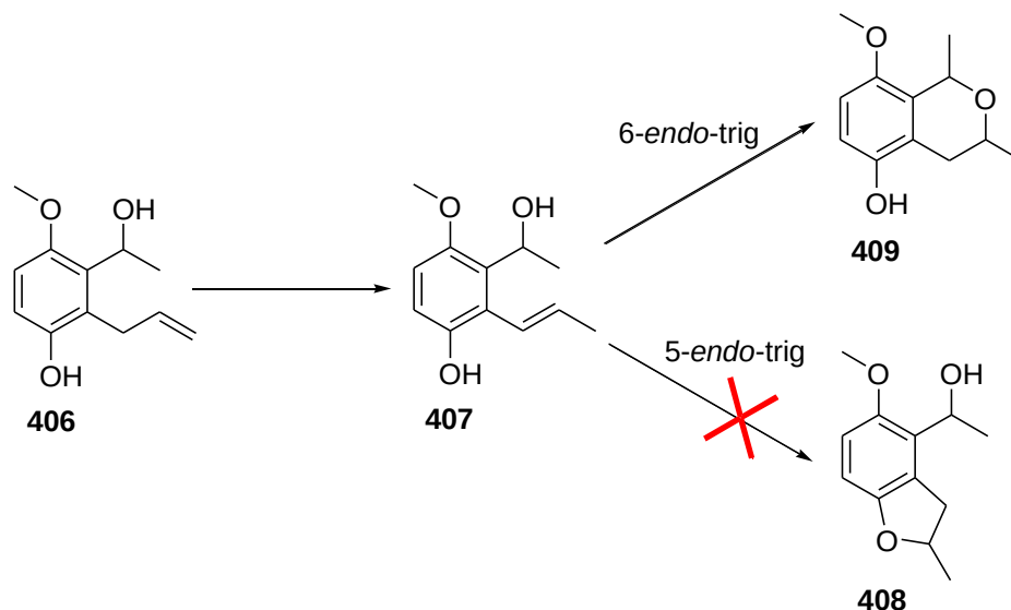
Scheme 4.31: Two possible potassium tert -butoxide mediated cyclization pathways for phenol 406 .
