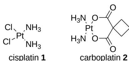
Figure 1.0: The molecular structures of cisplatin, cis -diamminedichloroplatinum (II), 1 and carboplatin, cis -diammine-1,1-cyclobutanedicarboxylatoplatinum (II), 2 .
