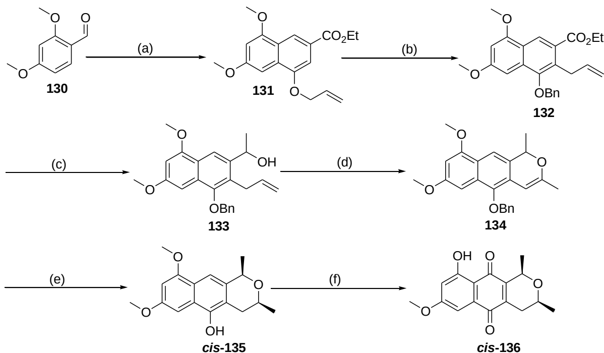
Scheme 1.26: Reagents and conditions; (a) (i) diethyl succinate, t -BuOH, t -BuOK, reflux, 4 hrs (ii) NaOAc-Ac 2 O, 130 °C, 4 hrs (iii) guanidine, EtOH-CH 2 Cl 2 , rt, 1 hr (iv) allyl bromide, K 2 CO 3 , Me 2 CO, reflux, 16 hrs (b) (i) DMF, 170 °C, 12 hrs (ii) BnCl, KI, K 2 CO 3 , Me 2 CO, reflux, 18 hrs (c) (i) LiAlH 4 , THF, 0 °C → rt, 18 hrs (ii) PCC-Al 2 O 3 , CH 2 Cl 2 , rt, 8 hrs (iii) MeMgI, Et 2 O-THF, 0 °C → rt, 8 hrs (d) (i) 10% PdCl 2 -CuCl 2 ·H 2 O-DMF, rt, O 2 (g), 3 hrs (e) 10% Pd/C, H 2 (g), CH 2 Cl 2 /dioxane, rt, 48 hrs (f) (i) 0.5 eq. salcomine, DMF, O 2 (g), rt, 18 hrs (ii) BCl 3 , CH 2 Cl 2 , -78 °C.
