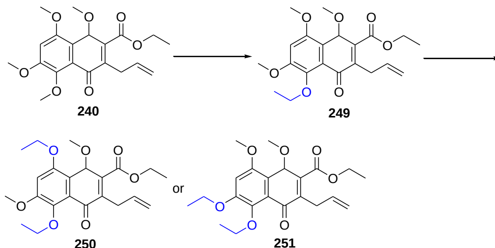
Scheme 2.69: Reagents and conditions: (a) 21% NaOEt, EtOH, rt, 35 min.
