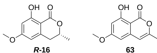
Figure 1.14: The molecular structures of 6-methoxymellein R-16 and 8-hydroxy-6-methoxy-3-methylisocoumarin 63 .
