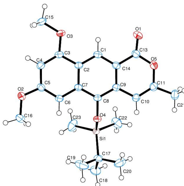
Figure 2.10: The ORTEP diagram of lactone 228 . Thermal ellipsoids are shown at the 50% probability level.
