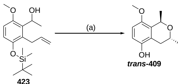
Scheme 4.47: Reagents and conditions: (a) t -BuOK, NMP, 110 °C, 30 min, 70%.
