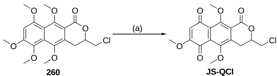
Scheme 2.83: Reagents and conditions: AgO, 55% aq. HNO 3 , 1,4-dioxane, rt, 70%.
