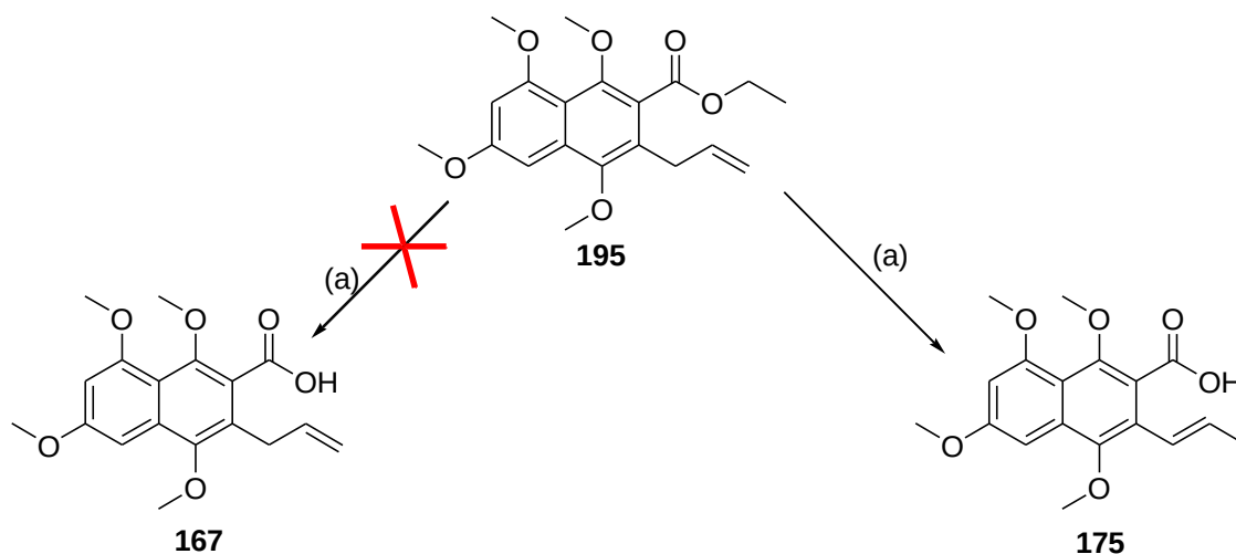
Scheme 2.27: Reagents and conditions: (a) (i) NaOH/KOH, MeOH/H 2 O, reflux, 84 hrs (ii) 32% aq. HCl, 55%.
