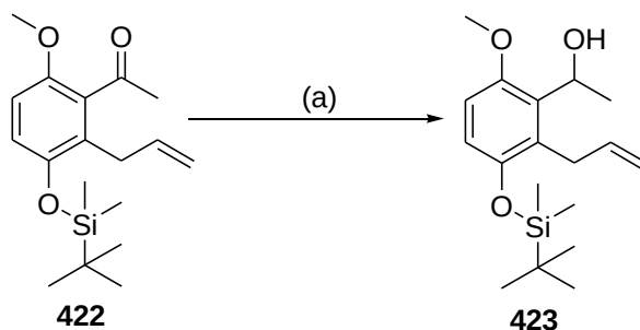
Scheme 4.46: Reagents and conditions: (a) LiAlH_4 , THF, 0\text{ }^{\circ}C \rightarrow rt , N_2 (g), 4 hrs, 89%.
