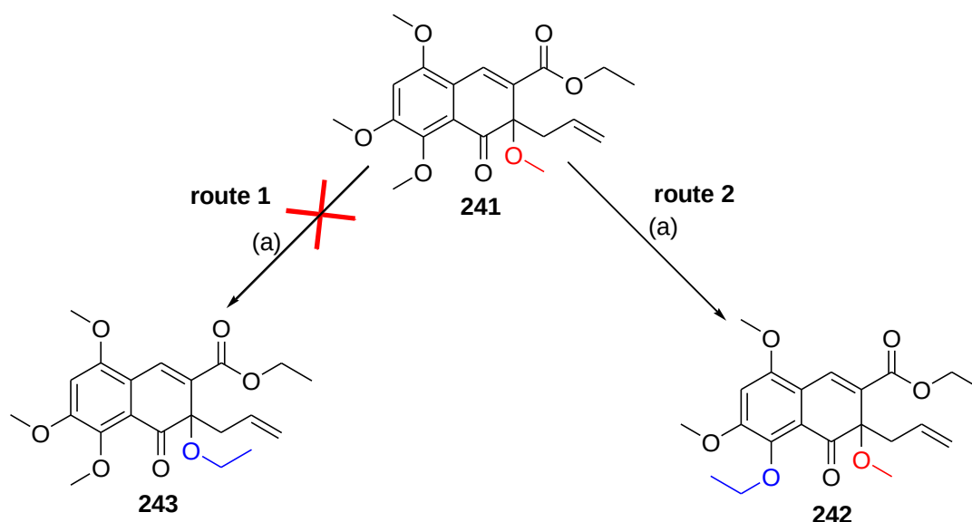
Scheme 2.65: Reagents and conditions: (a) 21% NaOEt, EtOH, 30 min, rt, 10%.
