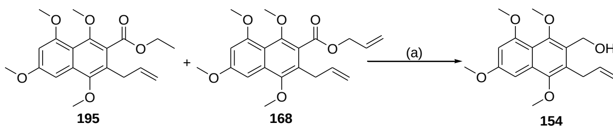
Scheme 2.28: Reagents and conditions: LiAlH 4 , THF, 0 °C → rt, N 2 (g), 4 hrs (% yield not determined).
