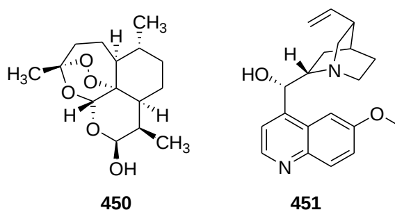
Figure 5.3: The molecular structures of dihydroartemisinin 450 and quinine 451 .
