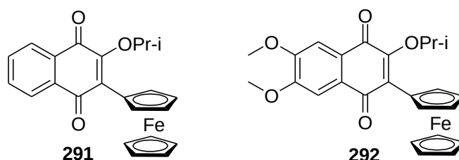
Figure 3.10: The molecular structures of ferrocene coupled naphthoquinones 291 and 292 reported by Yucel and co-workers.
