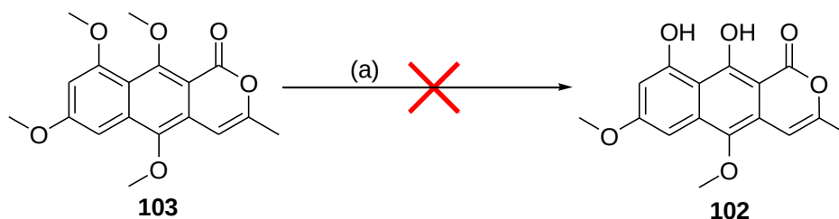
Scheme 2.36: Reagents and conditions: (a) \text{BCl}_3 , \text{CH}_2\text{Cl}_2 , \text{N}_2 (g), -78^\circ\text{C} \rightarrow \text{rt} ; or \text{BBr}_3 , \text{CH}_2\text{Cl}_2 , \text{N}_2 (g), -78^\circ\text{C} \rightarrow \text{rt} .
