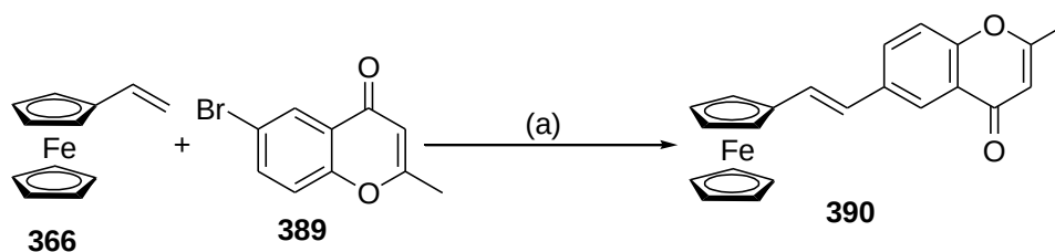
Scheme 4.23: Reagents and conditions: (a) cat. Pd(OAc) 2 , K 2 CO 3 , BU 4 NBr, DMF, 95 °C, 18 hrs.
