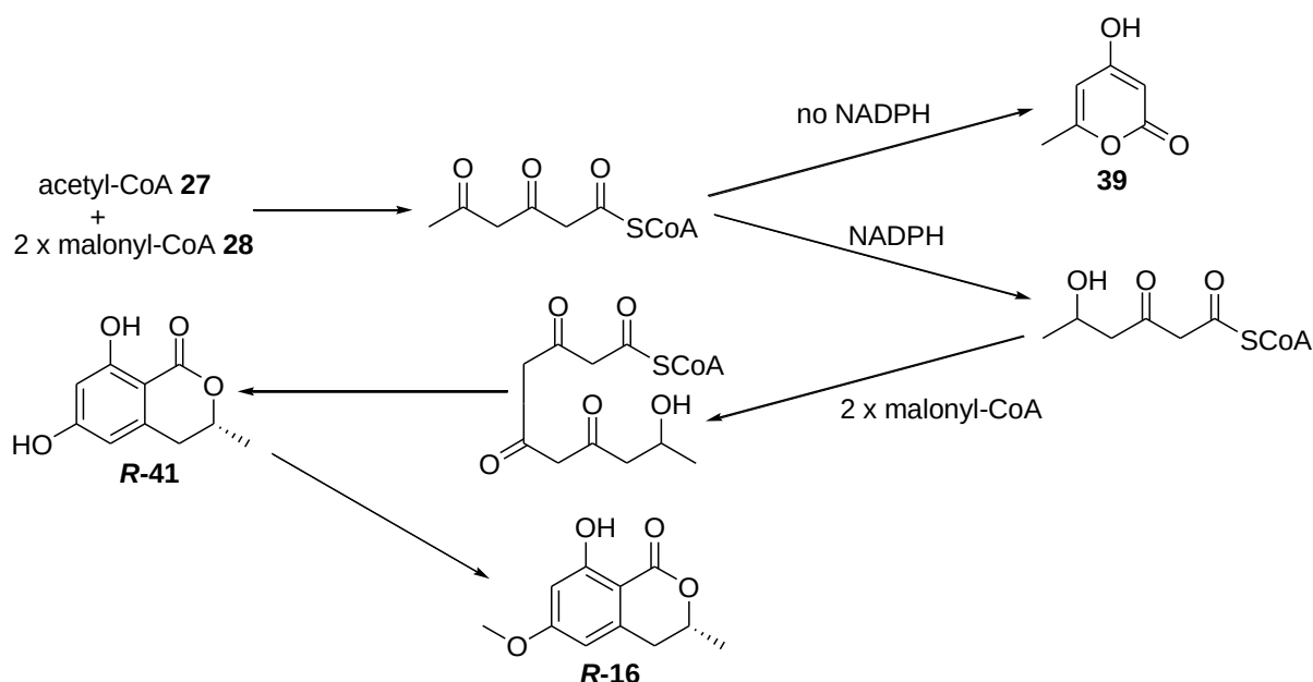
Scheme 1.5: Biosynthetic pathway for the synthesis of triacetic acid lactone 39 .
