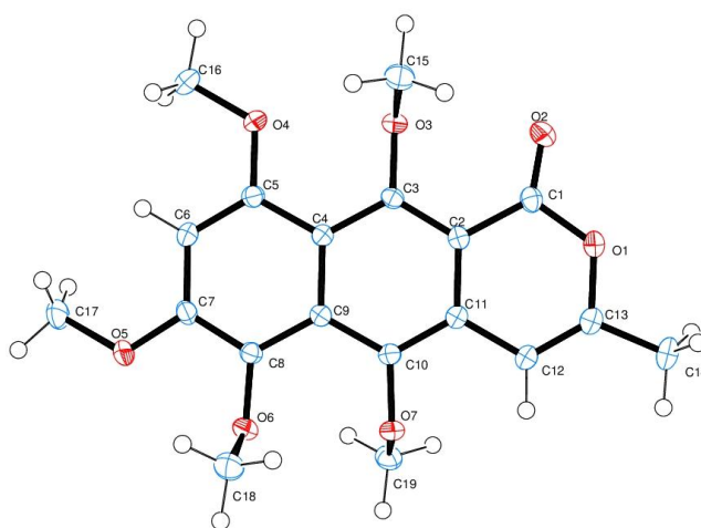
Figure 2.16: The ORTEP diagram for lactone 229 . Thermal ellipsoids are shown at the 50% probability level.
