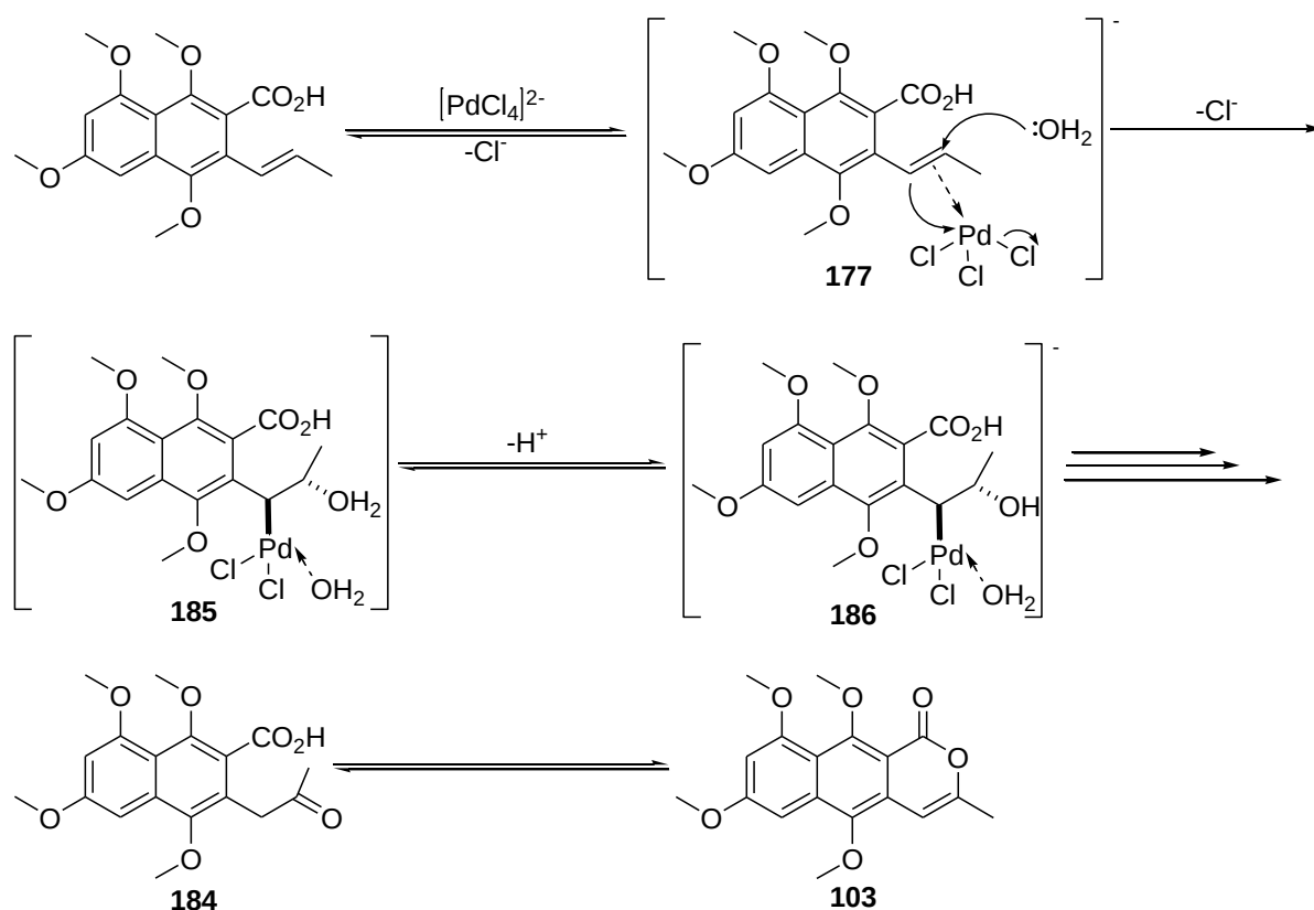
Scheme 2.16: Wacker outer-sphere mechanism for the formation of lactone 103 .
