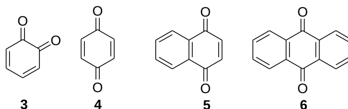
Figure 1.1: The molecular structures of o -benzoquinone 3 , p -benzoquinone 4 , p -naphthoquinone 5 and p -anthraquinone 6 .
