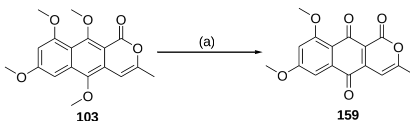
Scheme 2.37: Reagents and conditions: (a) BBr 3 , CH 2 Cl 2 , N 2 (g), -78 °C → rt, 25%.
