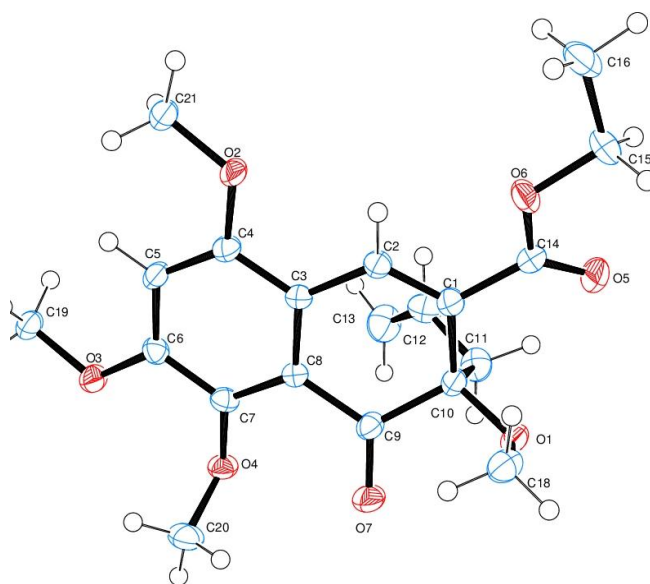
Figure 2.13: The ORTEP diagram of 241 . Thermal ellipsoids are shown at the 50% probability level.
