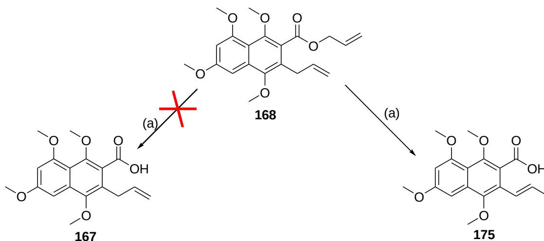
Scheme 2.13: Reagents and conditions: (a) cat. Pd(OAc)_2 , PPh_3 , morpholine, rt, N_2 (g), 12 hrs, 56%.
