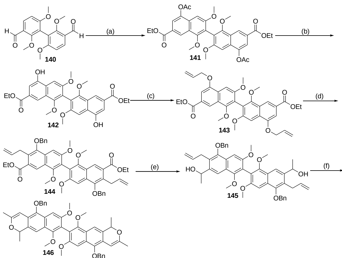
Scheme 1.29: Reagents and conditions; (a) diethyl succinate, t -BuOK, t -BuOH, N 2 (g), reflux, 4 hrs (b) guanidine·HCl, t -BuOK, EtOH-CH 2 Cl 2 , rt, 1.5 hrs (c) allyl bromide, K 2 CO 3 , Me 2 CO, reflux, 18 hrs (d) (i) DMF, microwave (200 W), 170 °C, 250 psi, 25 min (ii) BnCl, KI, K 2 CO 3 , Me 2 CO, reflux, 18 hrs (e) (i) LiAlH 4 , THF, 0 °C, 18 hrs (ii) PCC-Al 2 O 3 , CH 2 Cl 2 , rt, 8 hrs (iii) MeMgI-Et 2 O-THF, rt, 18 hrs (f) 10% PdCl 2 , CuCl 2 ·H 2 O-DMF, rt, O 2 (g), 18 hrs.
