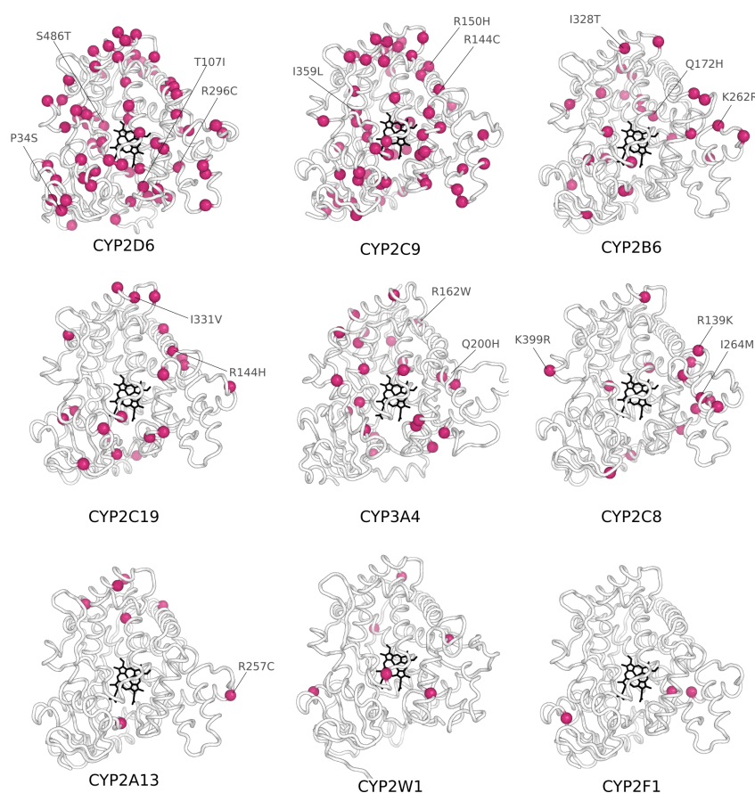
Figure 3.2: Mapping of single amino acid variants on CYP P450 proteins. The localisation of the catalytic site is indicated by the haem atoms (black). We have also labelled the positions of some clinically relevant amino acids (magenta) in selected protein structures.
