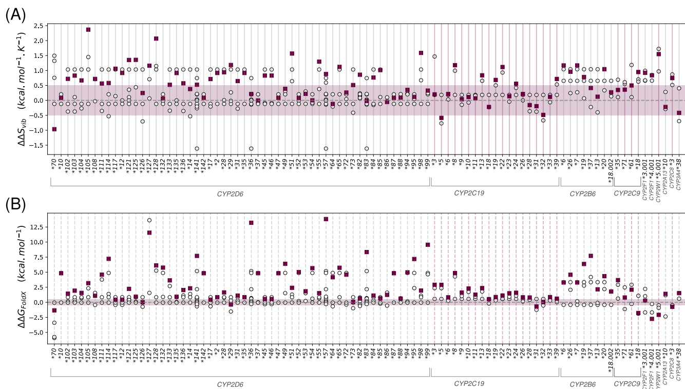
Figure S1. Comparison of ENCoM-computed ( \Delta\Delta S_{vib} ) and FoldX-computed ( \Delta\Delta G ) star allele and missense variant energy scores. (A) ENCoM \Delta\Delta S_{vib} scores. (B) FoldX \Delta\Delta G scores. Each haplotype is represented by a maroon square and their defining missense variants are represented by circles. Figure points that fall within the highlighted region are expected to have neutral effects on protein stability (Frappier & Najmanovich 2014). \Delta\Delta G predicts most of the variants and haplotypes as destabilising to the protein-encoded protein structures. Both \Delta\Delta G and \Delta\Delta S_{vib} seem to exhibit a destabilising bias for both haplotype and variants. However, \Delta\Delta S_{vib} predicted more haplotypes and variants to have neutral effects on protein stability than \Delta\Delta G (see also Figure 3.3A).
