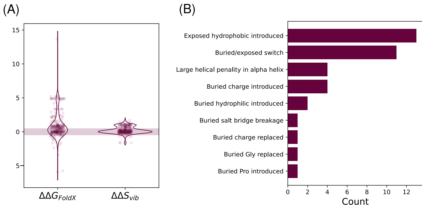
Figure 3.3: Distribution of Fold-X ( \Delta\Delta G ) and ENCoM-computed ( \Delta\Delta S_{\text{vib}} ) missense variant scores and SWAAT red-flag protein structural feature count. (A) FoldX and ENCoM-computed scores distribution. The highlighted region represents energies where the missense variants are expected to have neutral effects on protein stability (Frappier & Najmanovich 2014). (B) SWAAT red-flag. Many SWAAT structural consequences are linked to potentially functional altering disruptions in protein electrostatic forces (Gonzalez et al. 2022, Vascon et al. 2020, Gong et al. 2017, Ittisoponpisan et al. 2019).
