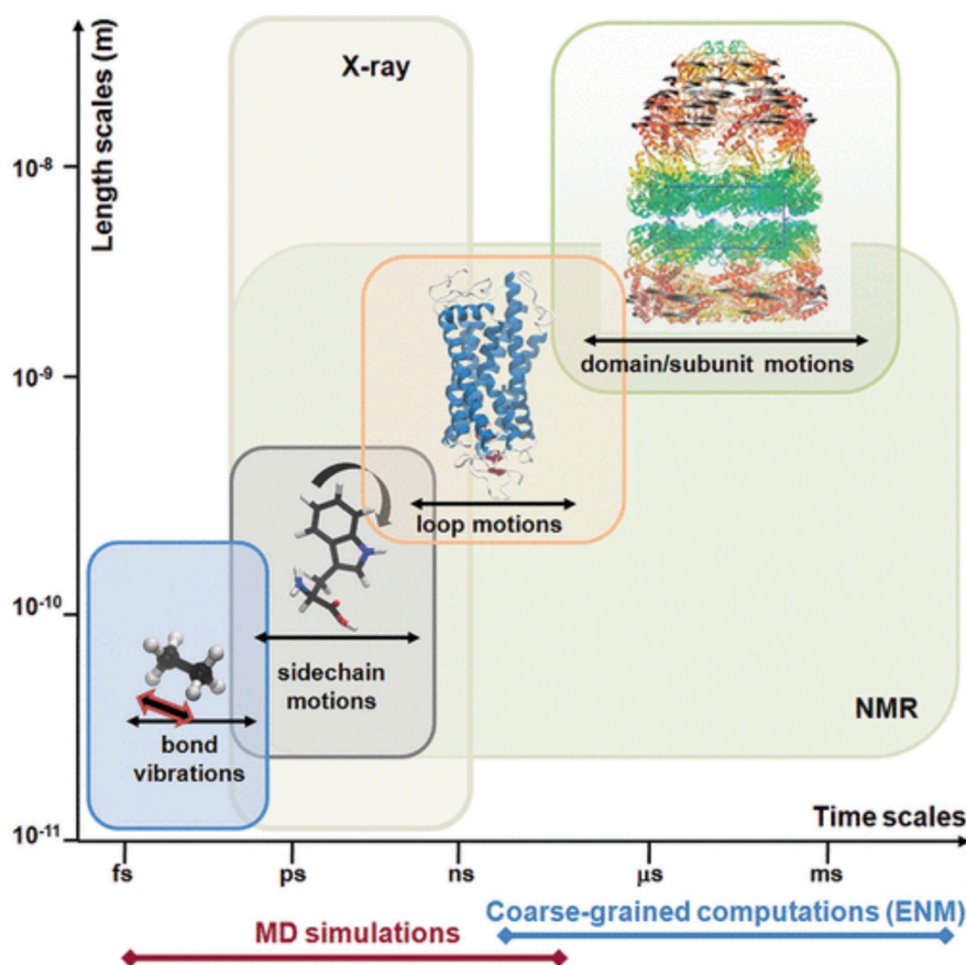
Figure 2.5: Broad range of equilibrium motions accessible under native state conditions , adapted from Bahar et al. (2010). Cooperative motions occur at the low frequency end of the mode spectrum, where fluctuations are lower. These modes engage large substructures (domain/subunit motions).
