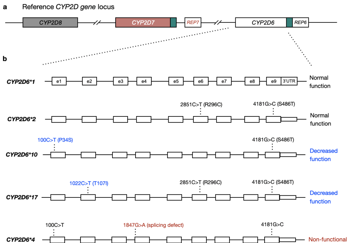
Figure 2.1: Examples of CYP2D6 star alleles. This figure highlights the concept of using a star allele nomenclature to refer to various haplotypes. Consensus star allele functions according to the Clinical Pharmacogenetics Implementation Consortium are provided on the right.
