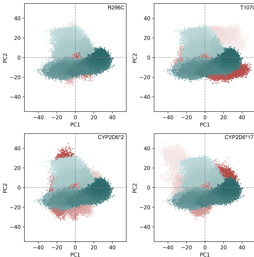
Figure 3.7: Principal Component Analysis from Molecular Dynamics simulations. The coordinates of C atoms of mutant (red) CYP2D6 protein systems ( CYP2D6*2 , CYP2D6*17 , R296C and T107I) overlapped with CYP2D6 wildtype (blue) protein coordinate, on the first and second principal components, for 600ns trajectories. The structure encoded by T107I sampled a larger subspace along the two principal components compared to the other mutant protein structures.
