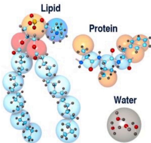
Figure 2.4: Illustration of coarse-graining adapted from Kmieciak et al. (2016). The ball-and-stick model represents all-atom representation and the larger sphere encompassing the ball-and-stick models represents coarse-graining – it condenses the molecule by grouping atoms for relatively simpler and quicker simulation of biological molecules.
