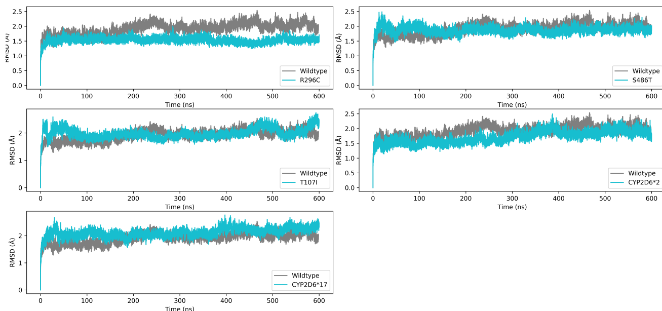
Figure 3.5: Analysis of backbone protein structural deviations by selected CYP2D6 variants and haplotypes. RMSD of the CYP2D6 mutant protein systems is shown in blue while that for the wild-type is shown in grey. The protein structure encoded by R296C exhibited the most deviations from the wildtype protein structure; however, it converged early in the simulation time ( 50ns). No clear convergence was observed for T107I. RMSD for the two haplotypes, CYP2D *2 (R296C and S486T) and *17 (*2-backbone + T107I), was inconclusive regarding the characterisation of protein structural deviations.
