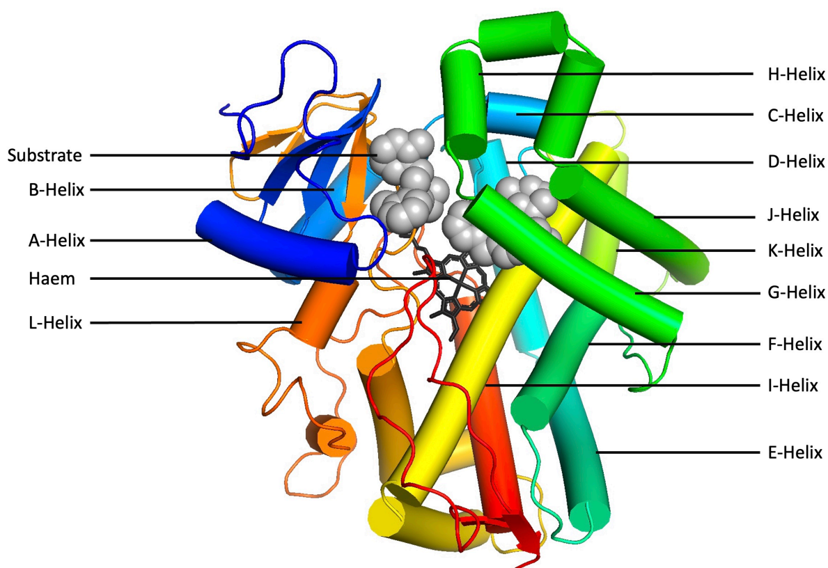
Figure 2.2: Structure of a CYP protein adapted from Wang et al. (2015). This figure visualises the major helices and the CYP protein family together with two bound substrates and the haem cofactor which enables the enzymatic oxidation of substrates via an electron transport chain.
