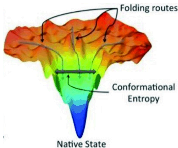
Figure 2.3: Illustration of a protein folding energy landscape adapted from Sinner et al. (2014). The top (red) of the folding funnel represents isoenergetic unfolded proteins with high conformational entropy (represented by the width of the folding funnel) and high total energy. The protein has to move down the funnel to reach an energetically minimum state (blue) with the least conformational entropy while avoiding intermediate states (green) that may present an energy barrier and undesirably folded proteins.
