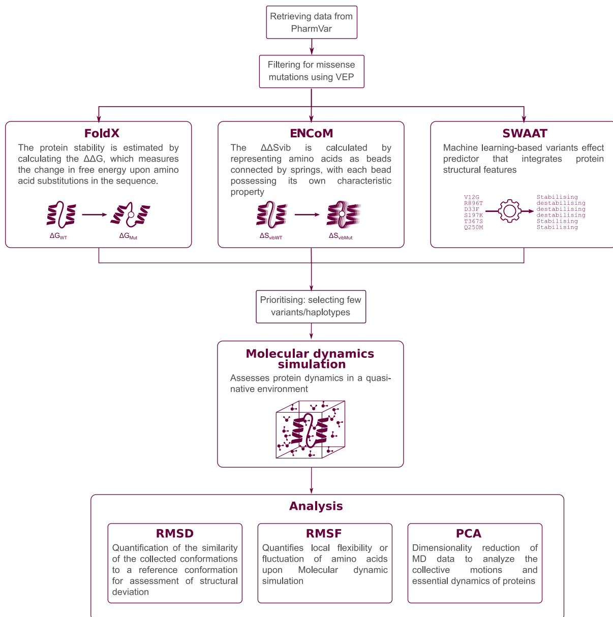
Figure 3.1: An overview of the employed methodologies and their interrelationships.
