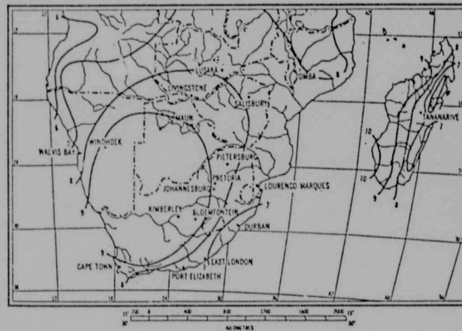
Fig.50: Mean annual sunshine (hours/day)
