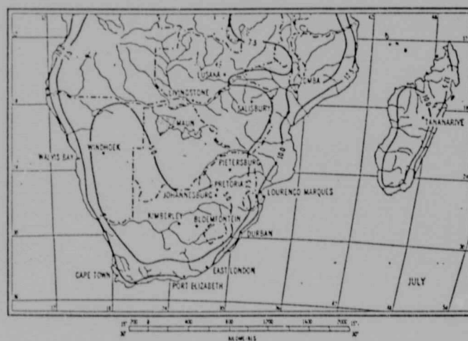
Fig.47: Atmospheric moisture (gm/kgm) for Jan. and July.
