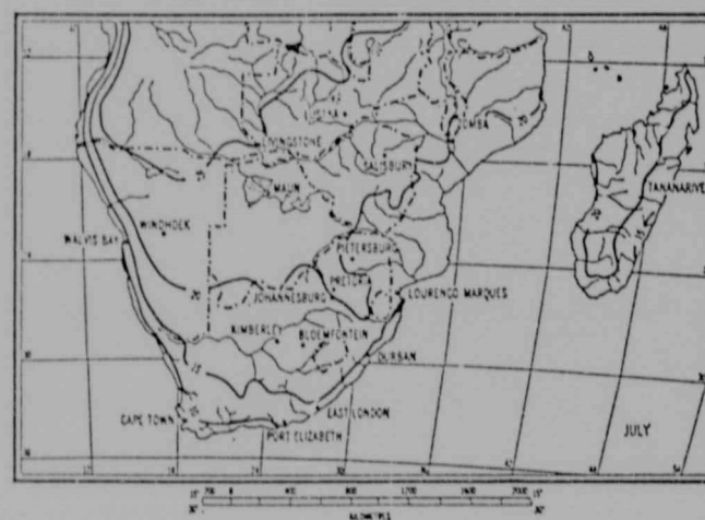
Fig.54: Mean daily maximum temp. in °C
