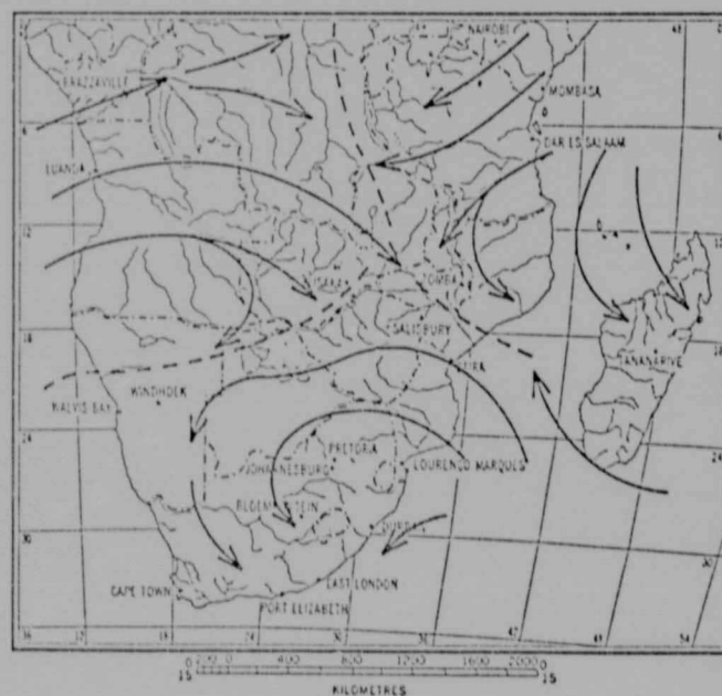
Fig.48: Converging air-streams in summer
