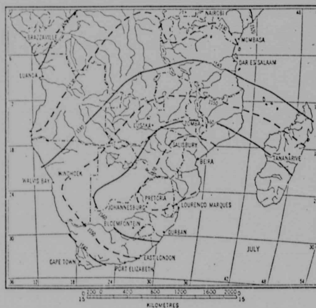
Fig.46: Contours (in meters) of the surface for Jan. and Jul.
