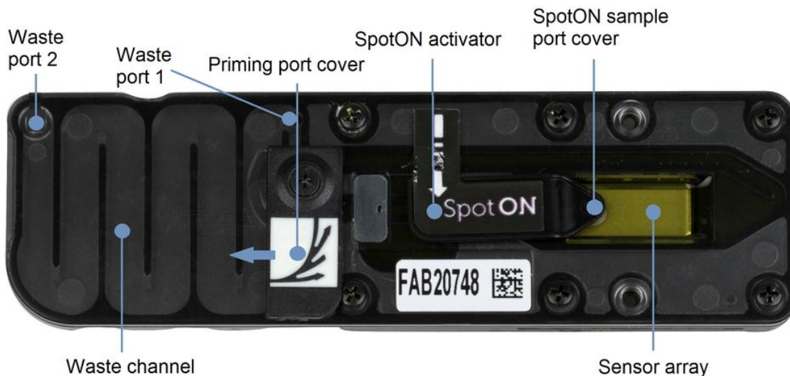
Figure A1: Oxford Nanopore Flow Cell
