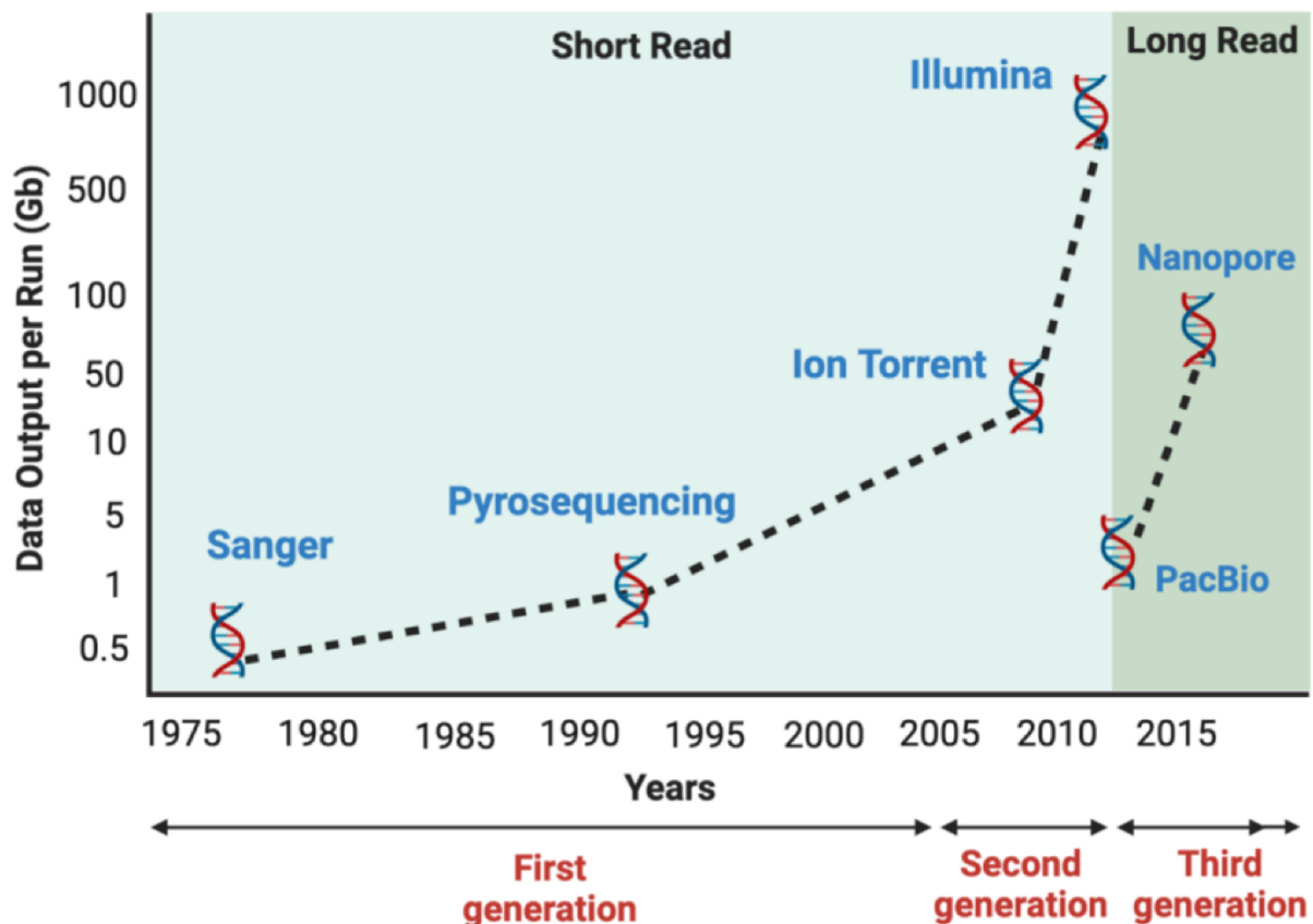
Figure 2.1: Evolution of sequencing technologies categorized into three generations (Satam et al. , 2024).
