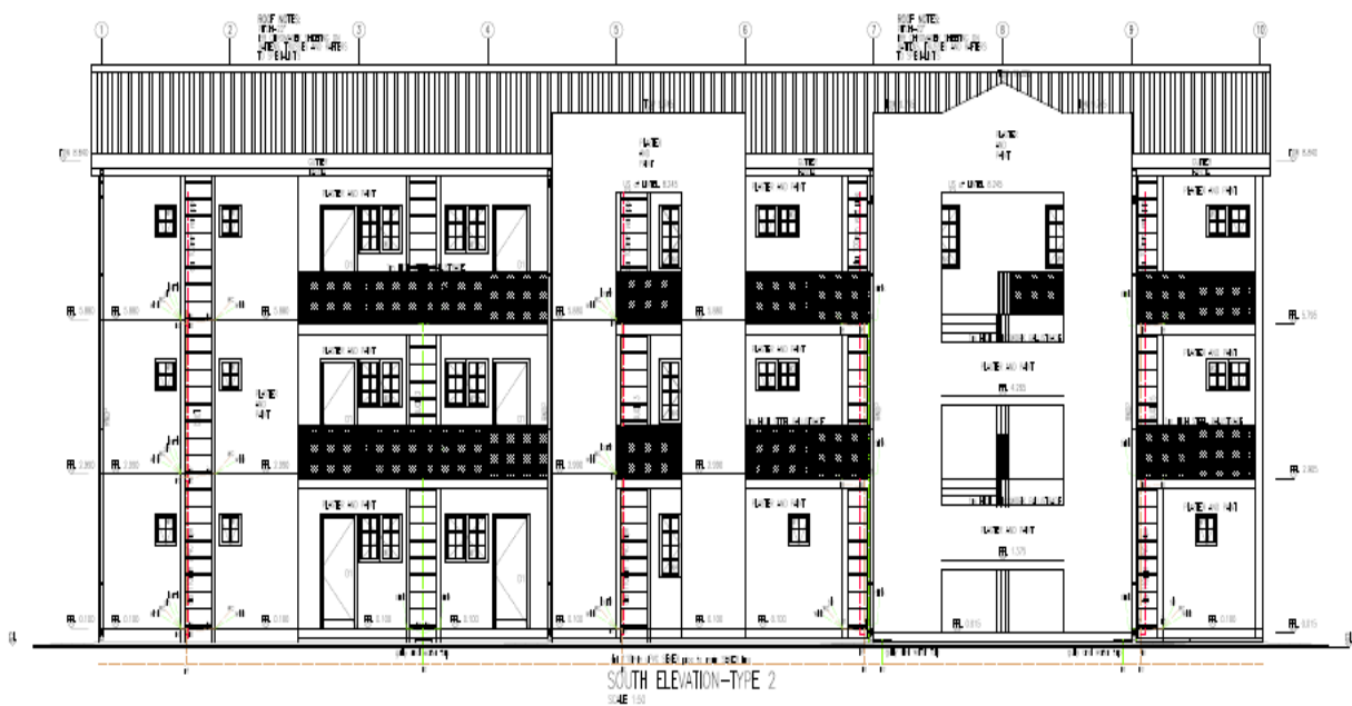
Figure 13: South Elevation
