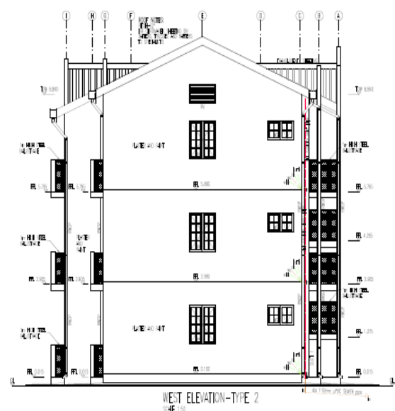
Figure 16: West Elevation
