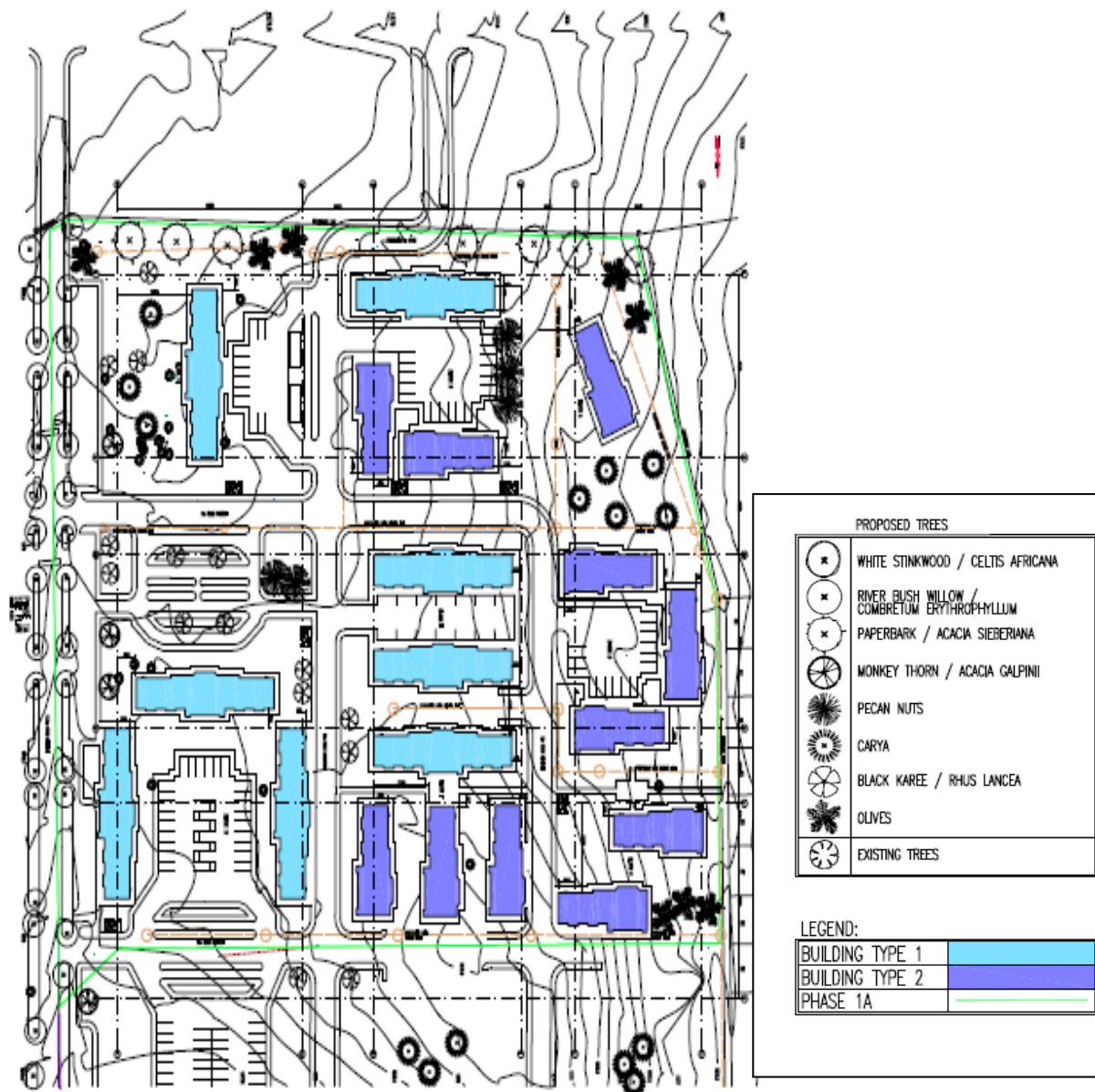
Figure 10: Phase 1 – site development plan
