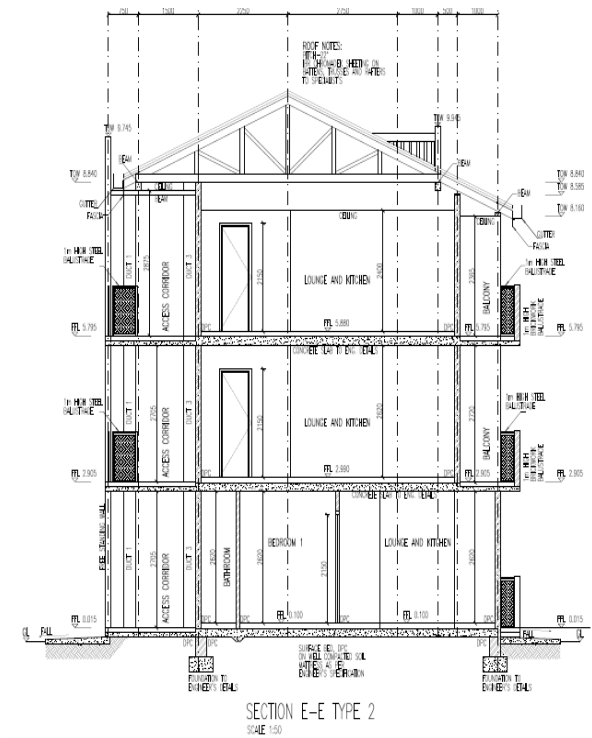
Figure 12: Architects, Section E – E
