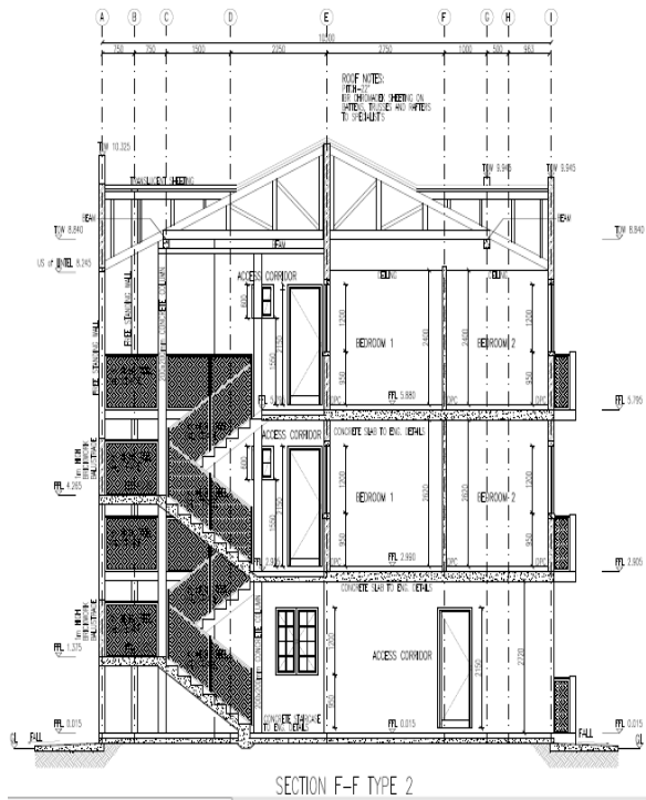
Figure 11: Architects, Section F – F
