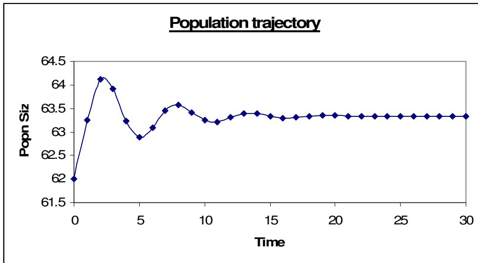
Figure 2.3: A typical trajectory predicted by Equation (2.3.7)
