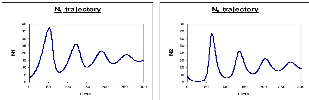
Figure 2.4 Cyclic Decays to equilibrium for a host-parasite assemblage
