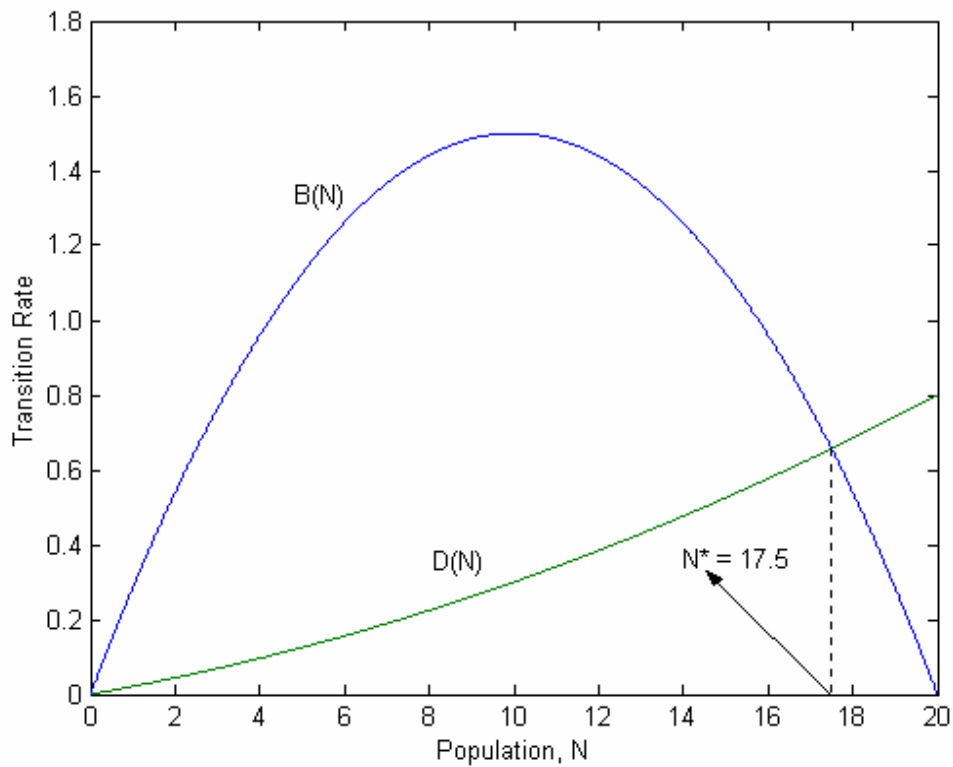
Figure 2.1 Birth and Death transition rates for Equation (2.2.6)
