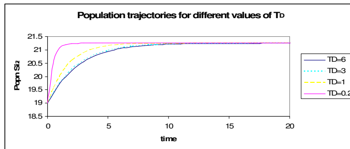
Figure 2.2: Predicted population numbers for a range of time delays
