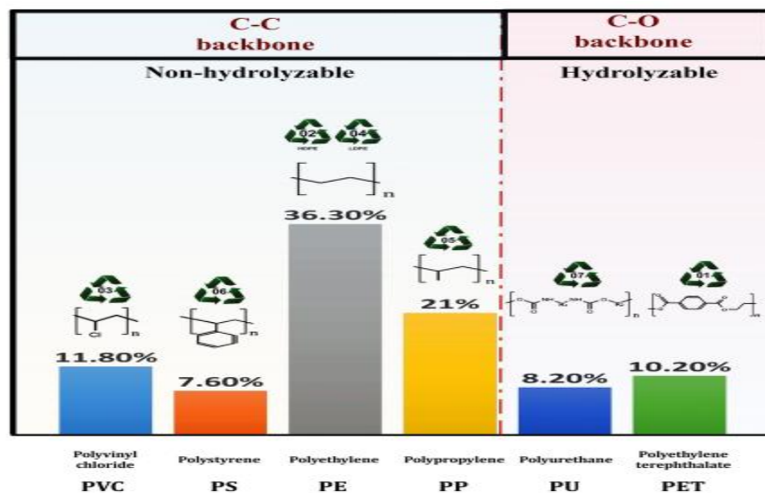
Fig 2.1: The most prevalent plastics, and their classification according to chemical backbone structure (Ali et al. 2021)
