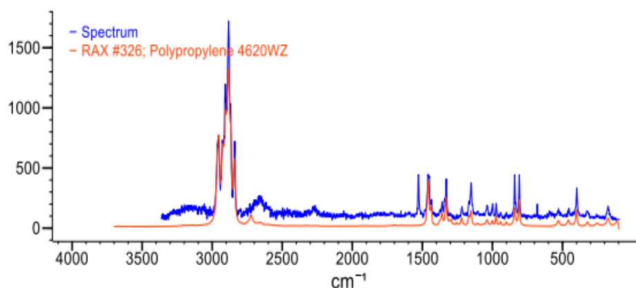
Fig 4.10: Raman spectrum of polypropylene
