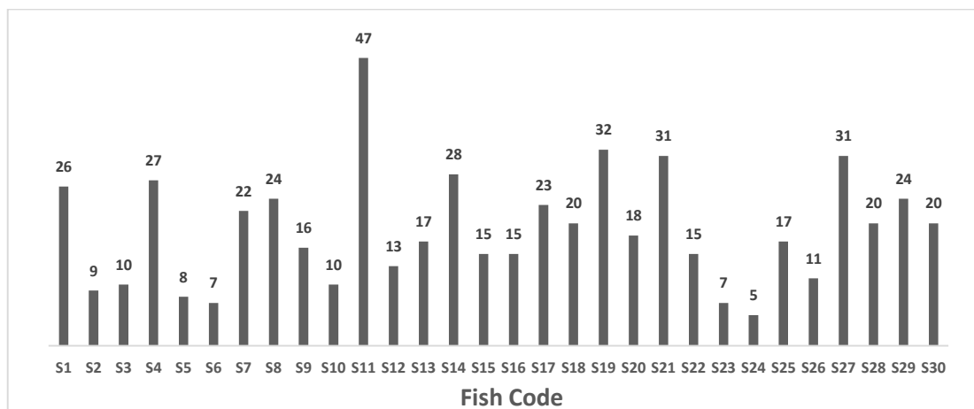
Fig 4.1: MP intensity in Nile Tilapia fish sampled from the River Nile
