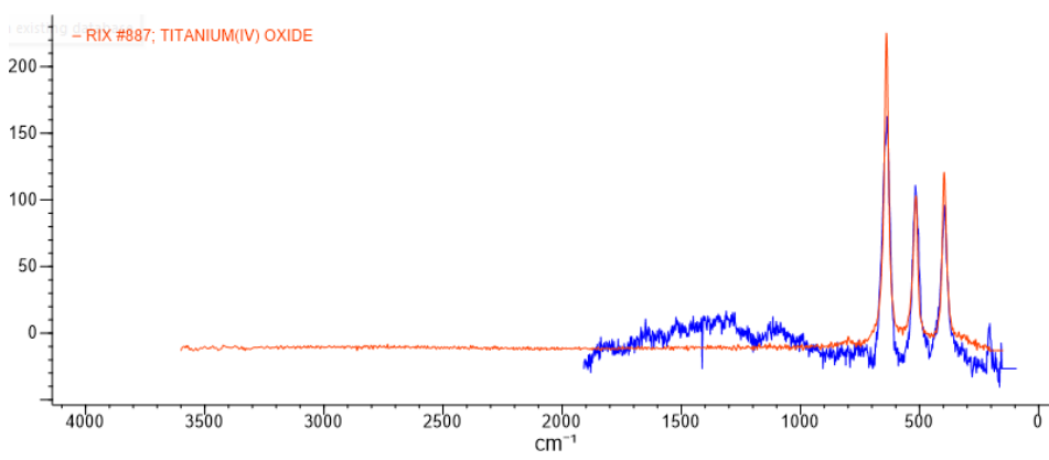
Fig 4.13: Raman spectrum of titanium dioxide
