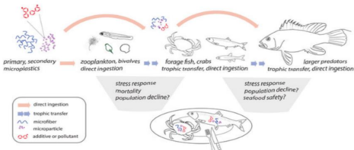
Fig 2.4: MPs in the food chain (Baechler, et al. 2019)
