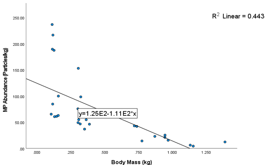
Fig 4.15: Correlation between MP and body mass of fish
