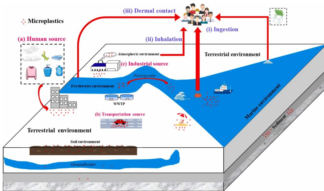
Fig 2.3: Microplastic source (Wang et al. 2021)
