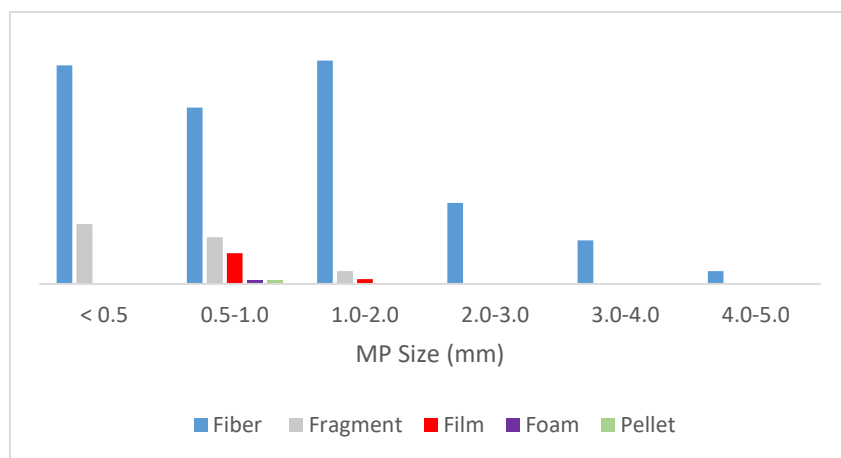
Fig 4.5: Distribution of MP shapes per size class
