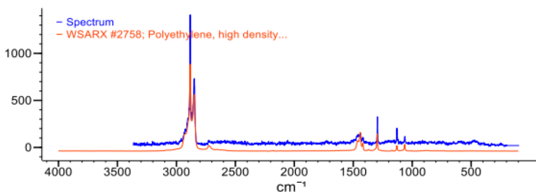
Fig 4.9: Raman spectrum of high-density polyethylene
