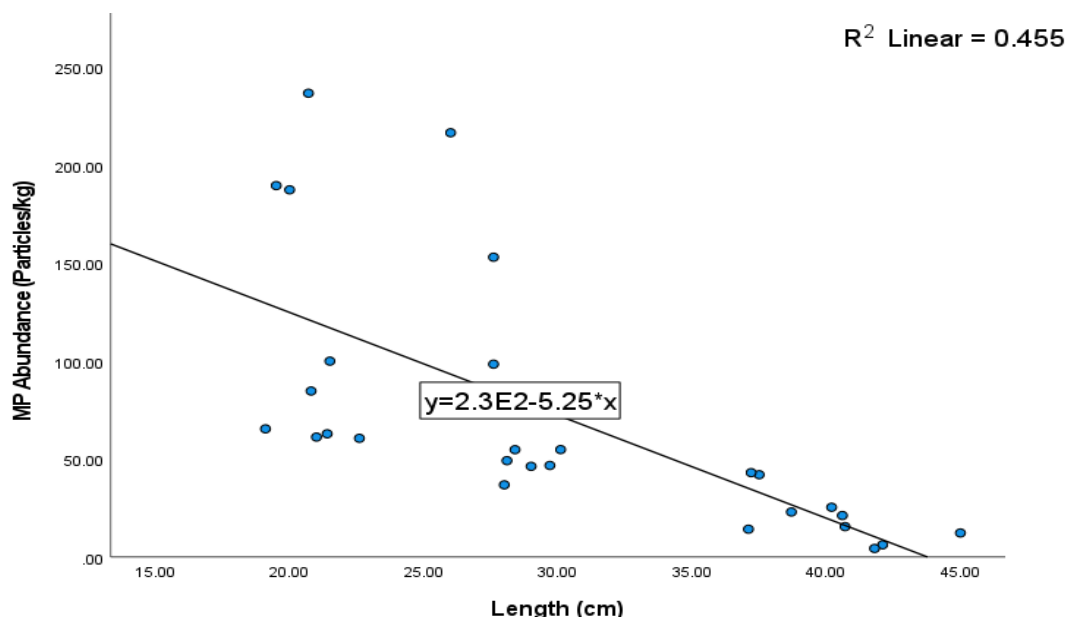
Fig 4.16: Correlation between MP and total length of fish
