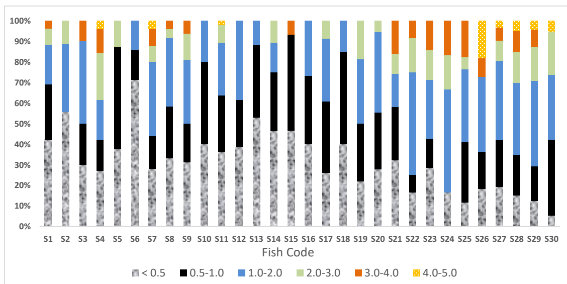
Fig 4.2: Distribution of MP sizes per individual fish
