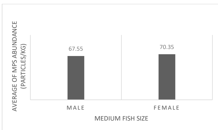
Fig 4.17: Average of MP abundance in medium size fish of both male and female
