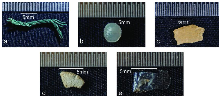
Fig 2.2: Shapes of MPs: (a) fiber, (b) pellet, (c) fragment, (d) foam and (e) film (Alvarez-Zeferino et al. 2020)
