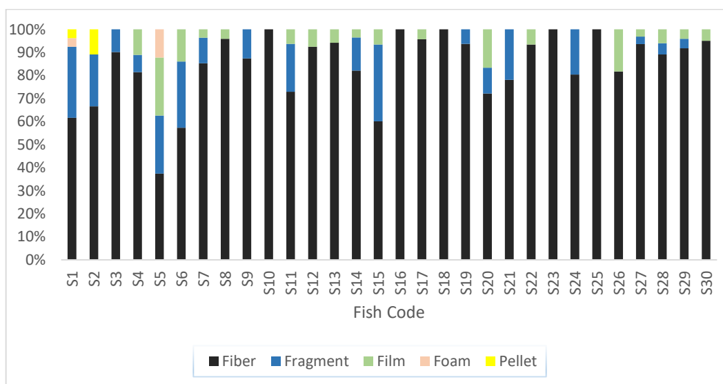
Fig 4.4: Distribution of MP shapes per individual fish.
