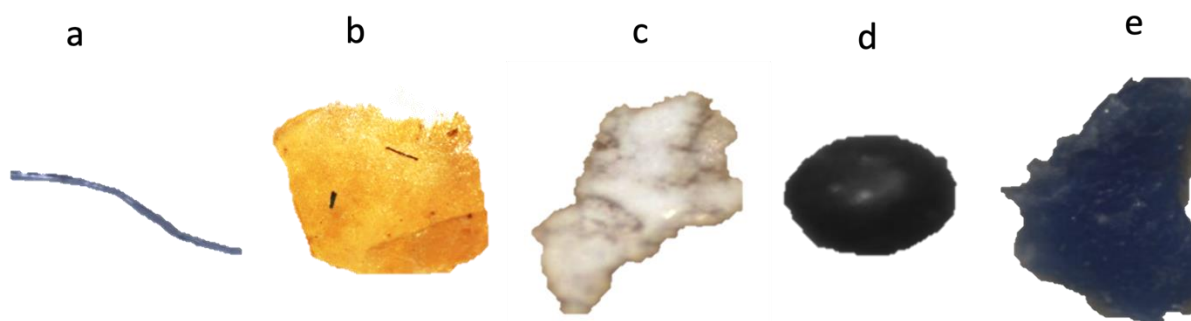
Fig 4.3: MP images captured under the optical microscope (a) fiber, (b) film, (c) foam, (d) pellet, (e) fragment.
