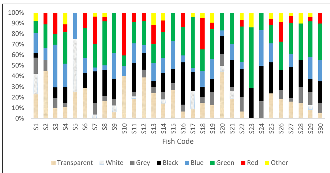
Fig 4.6: Distribution of MP colours per individual fish
