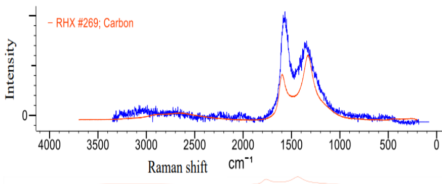
Fig 4.11: Raman spectrum of carbon
