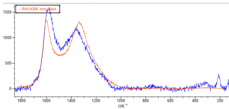
Fig 4.12: Raman spectrum of ivory black
