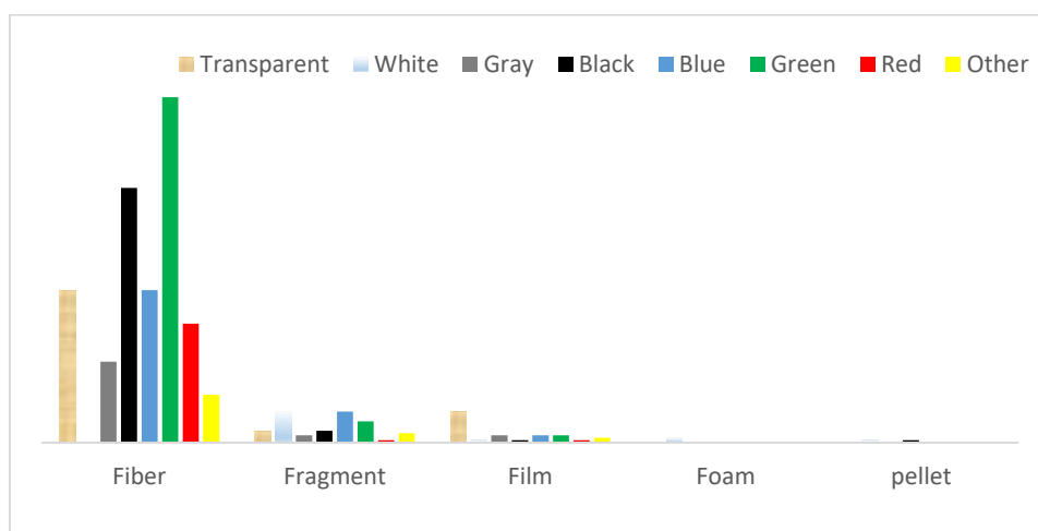
Fig 4.7: Distribution of MP colours per shape
