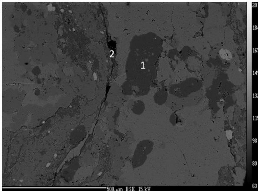
Fig 4.1.9 Microprobe image of the stylolite on Beestekraal sample SAM 12.
