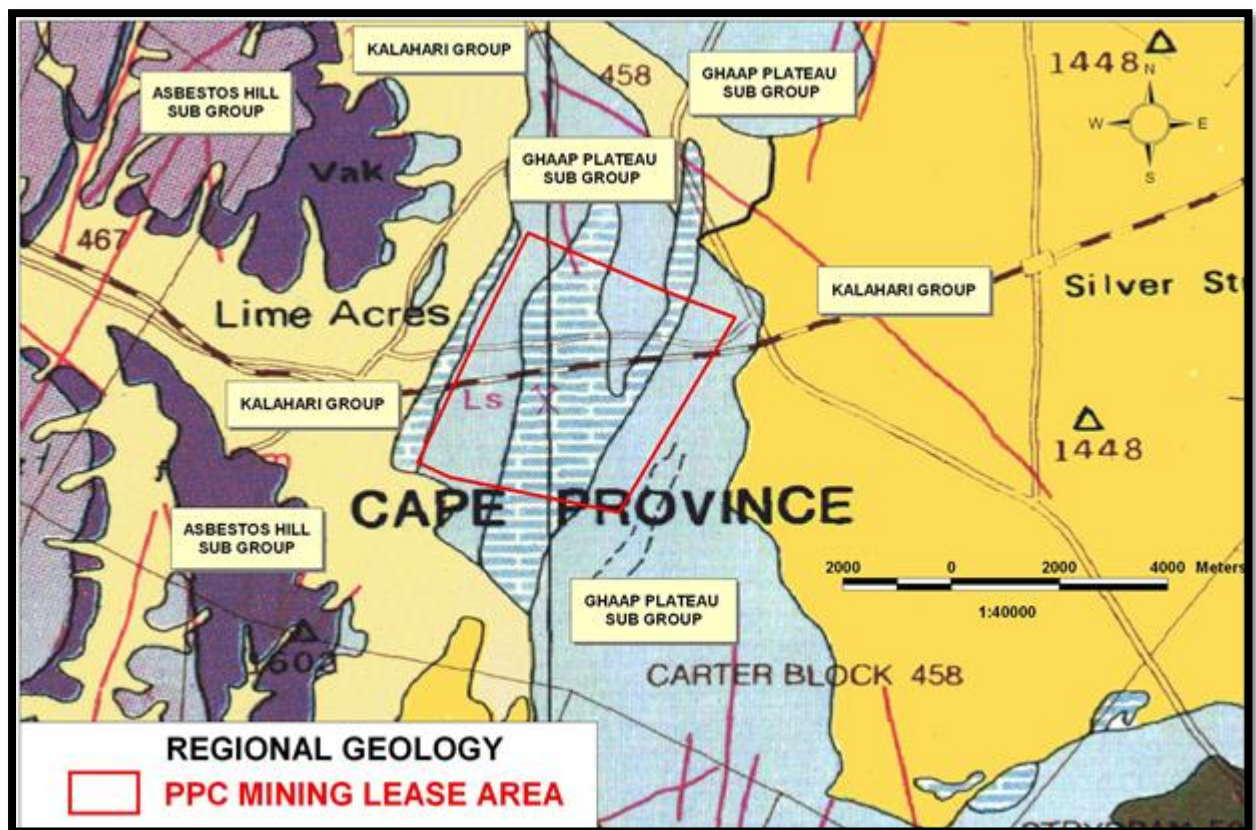
Figure 1.6 Geology of the Lime Acres mine (Modified after Eriksson et al. , 2006).
