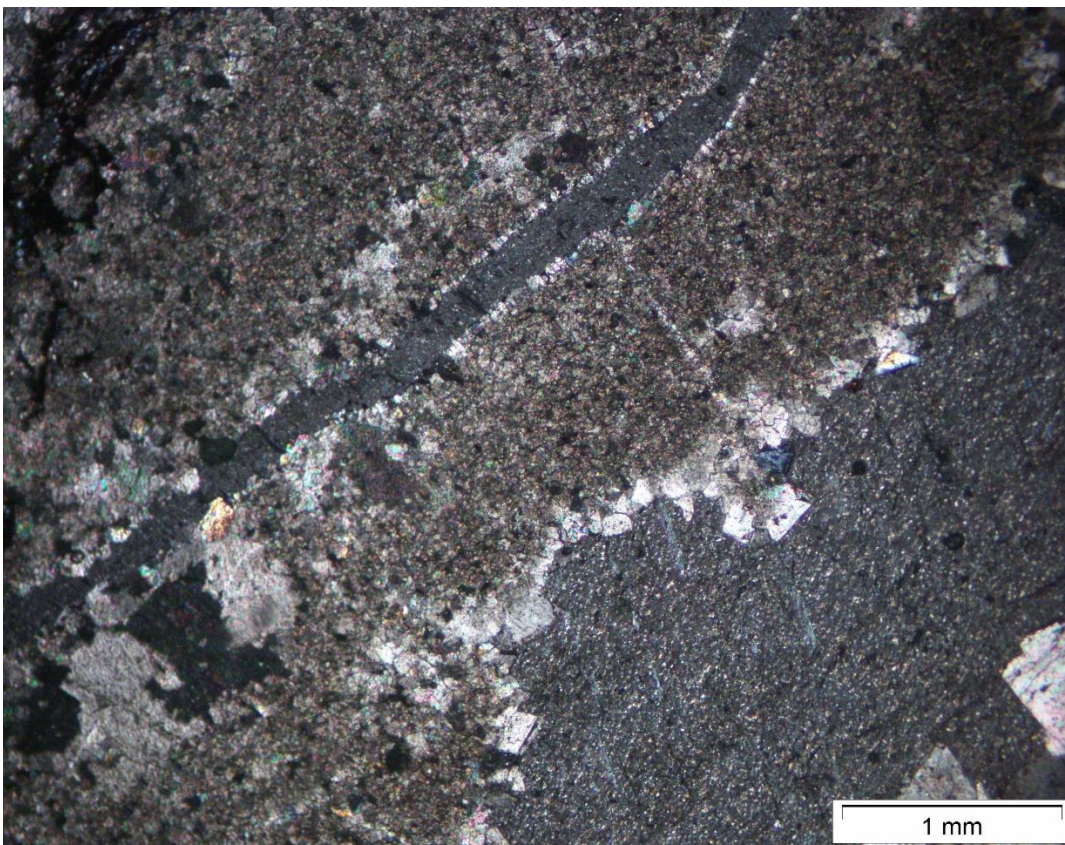
Figure 4.1.6 bedding plane showing the quartz crystals on the contacts.
