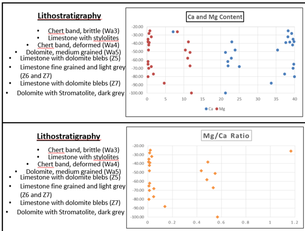
Figure 4.2.11 Whole rock XRF data showing Calcite (blue) Magnesium (red) representation at the Lime Acres limestone quarry and Mg/Ca (yellow) ratios with corresponding depths.
