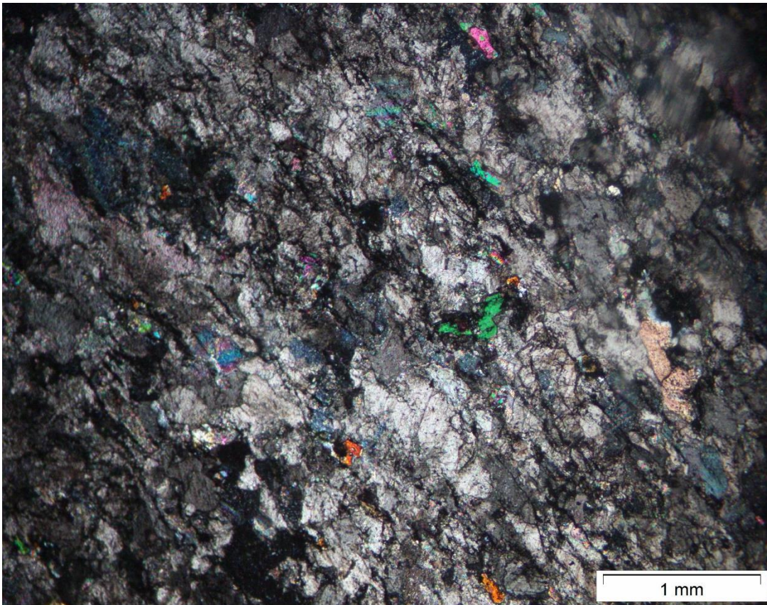
Figure 4.1.7 Deformed crystals of dolomite with some quartz inclusions.
