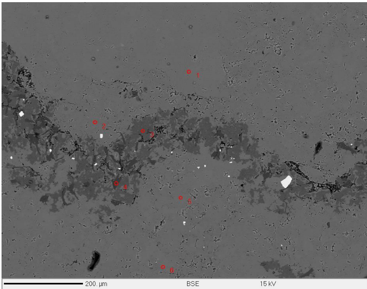
Fig 4.2.12 Point analysis analysed on the stylolite of Lime Acres sample TMN 24.
