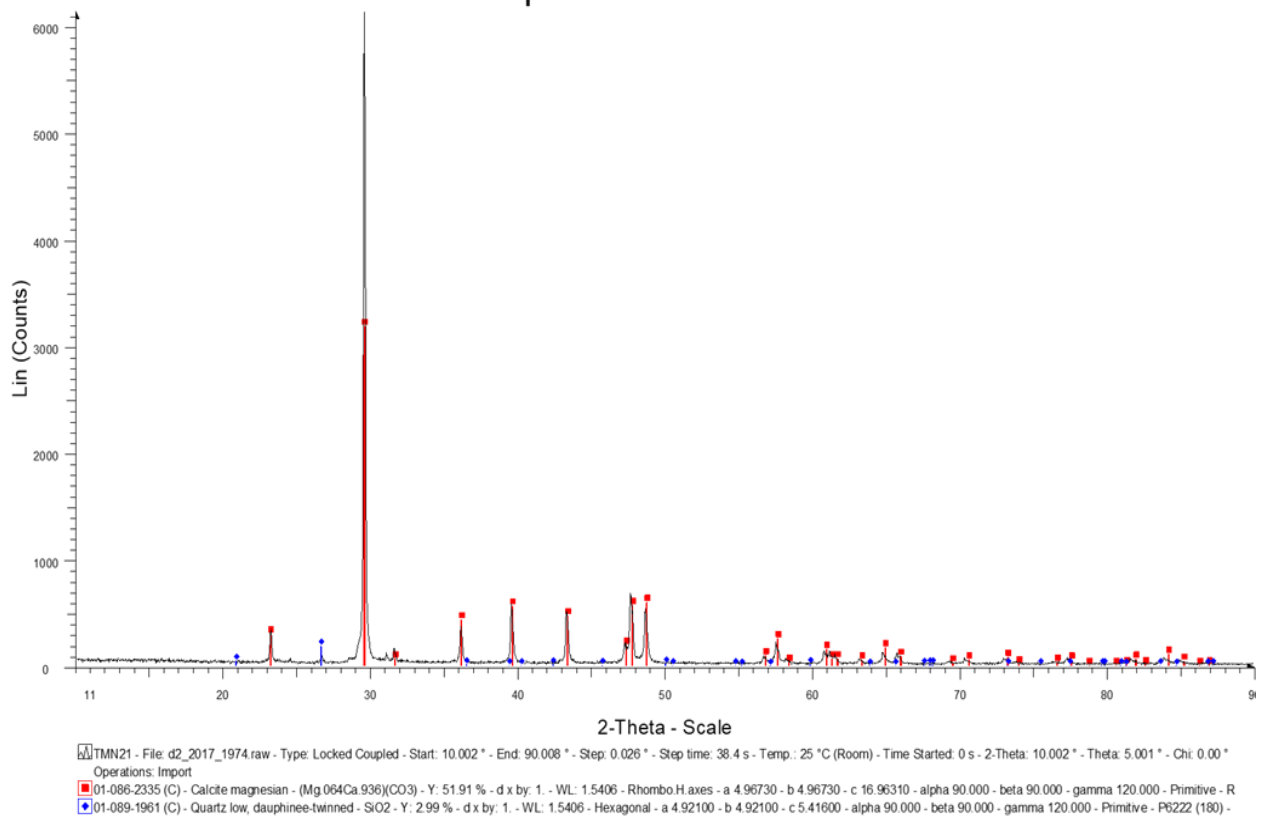
Figure 4.2.18 Whole rock XRD data showing magnesium calcite (red) and quartz (blue) of TMN 21 collected in Lime Acres.
