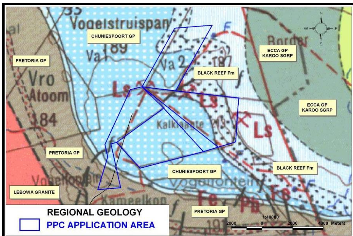
Figure 1.5 Geology at the Beestekraal Mine. (Modified after Eriksson et al. , 2006).
