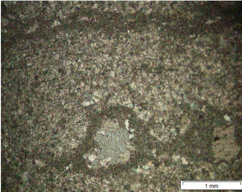
Figure 4.2.9 Irregular shaped silicate crystals are surrounded by fine grained crystals.
