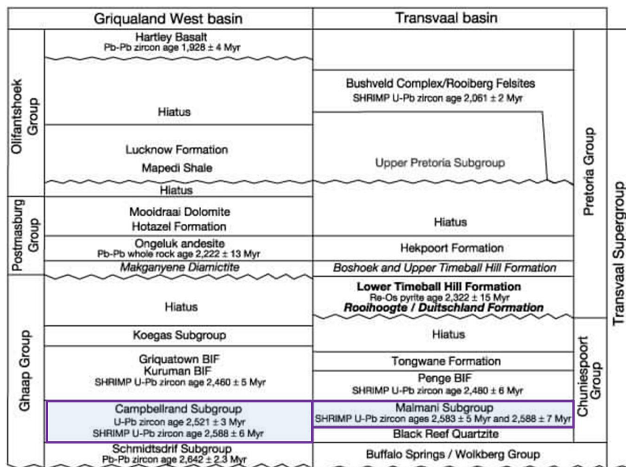
Figure 2.2 Correlation chart for the Transvaal Supergroup in the Griqualand West and Transvaal structural basins, South Africa (Bekker et al. , 2004).
