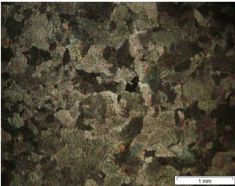
Figure 4.2.5 coarse to medium grained dolomite with fenestrae and re-entrance angles.
