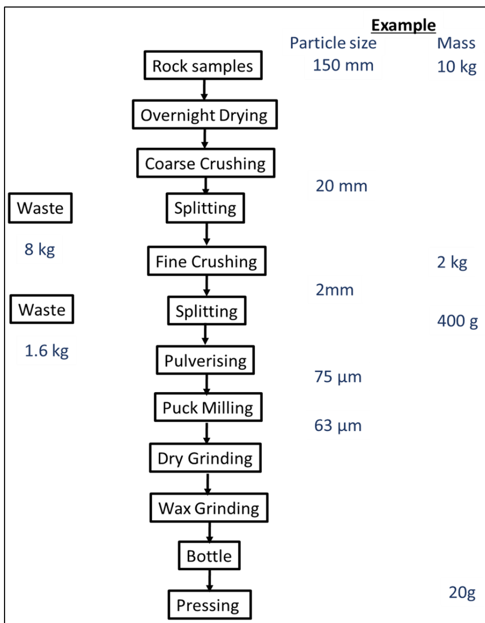
Figure 2.7 Steps in preparation of a sample for XRF analysis. The particle size and mass are given as examples (Modified from Willis et al. , 2014).
