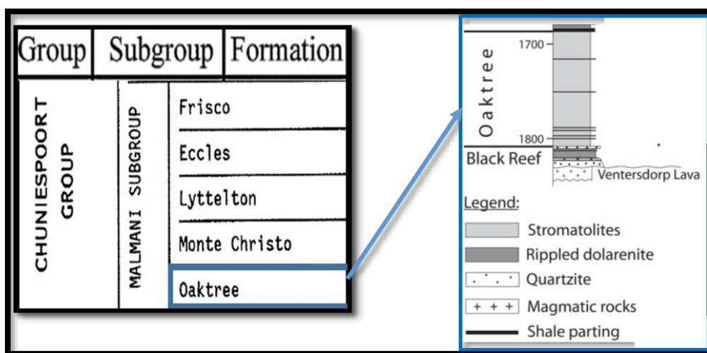
Figure 2.5 Simplified stratigraphic columns for a portion of the Malmani Subgroup with emphasis to the Oaktree Formation. ( Modified from Truswell, 1990 and Eroglu et al. , 2015).
