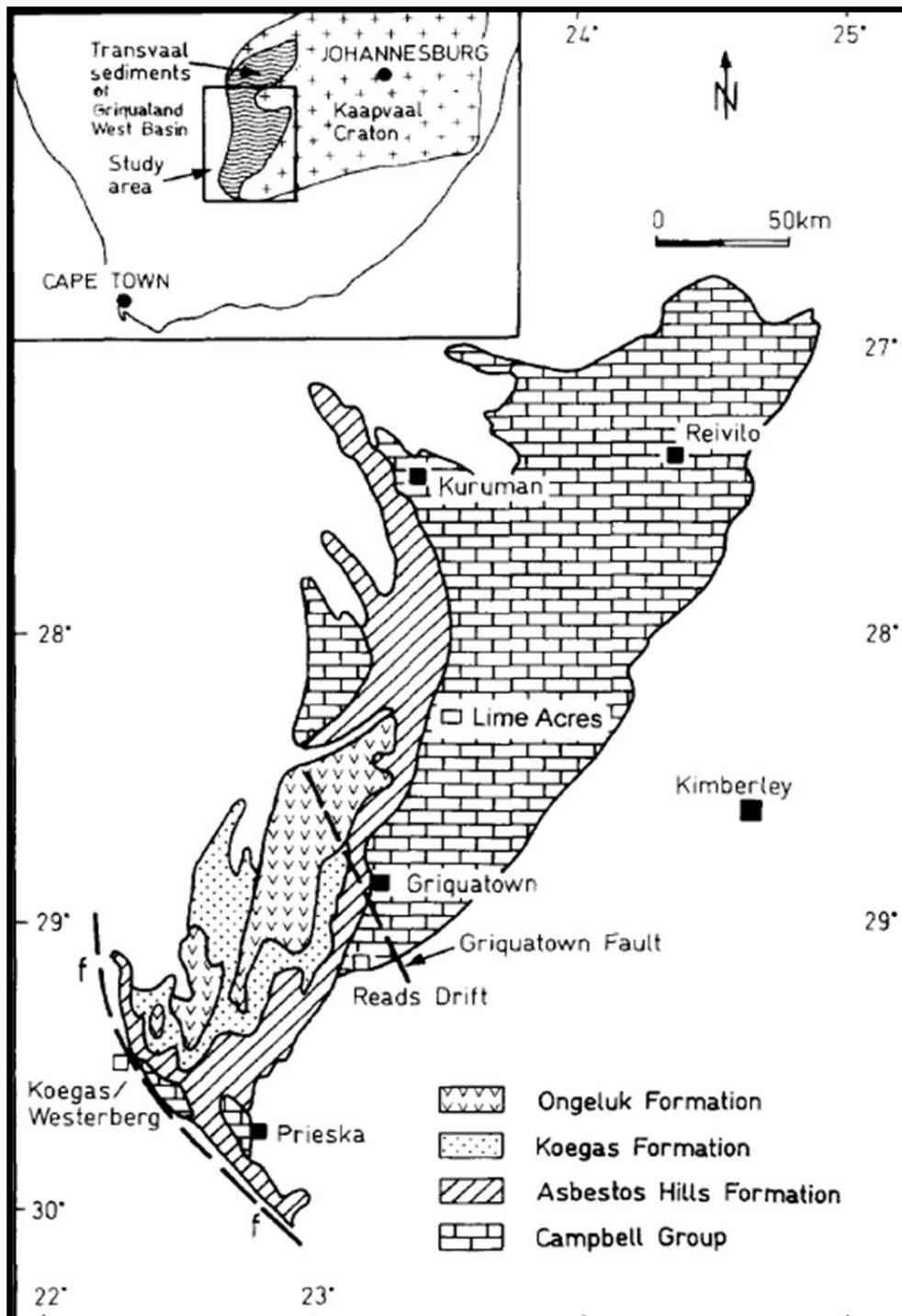
Figure 2.3 Map showing the location of Lime Acres (Note: the Griquatown Fault which cuts across the Campbellrand Subgroup), Northern Cape Province, and South Africa in the Campbellrand Subgroup (Altermann et al. , 1995).
