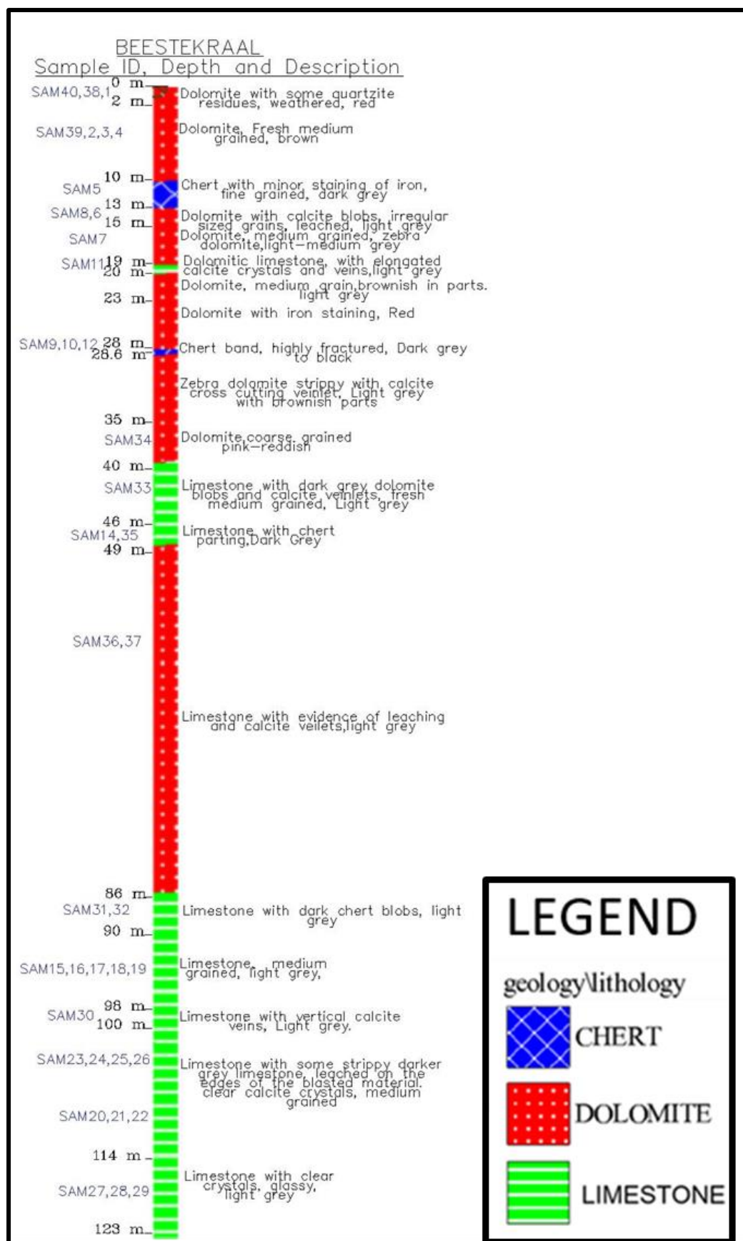
Figure 4.1.1: Lithostratigraphical log of Beestekraal's exposed face.
