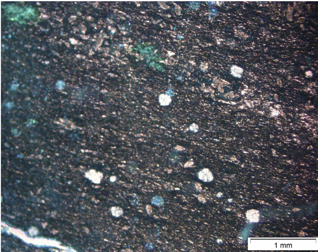
Figure 4.1.5 Fenestrae filled with chert nodules in high magnesium calcites.
