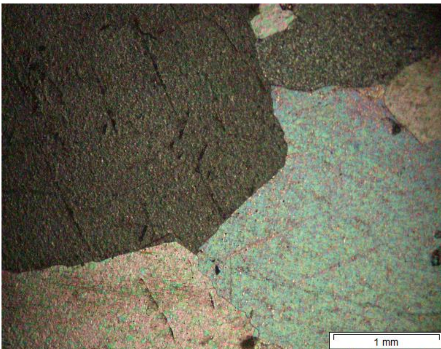
Figure 4.2.7 Coarse grained crystals with re-entrance angles.
