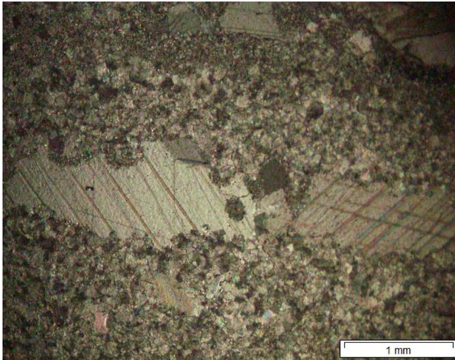
Figure 4.2.8 fenestrae in varying grain sizes filled with well-defined twinning structures.
