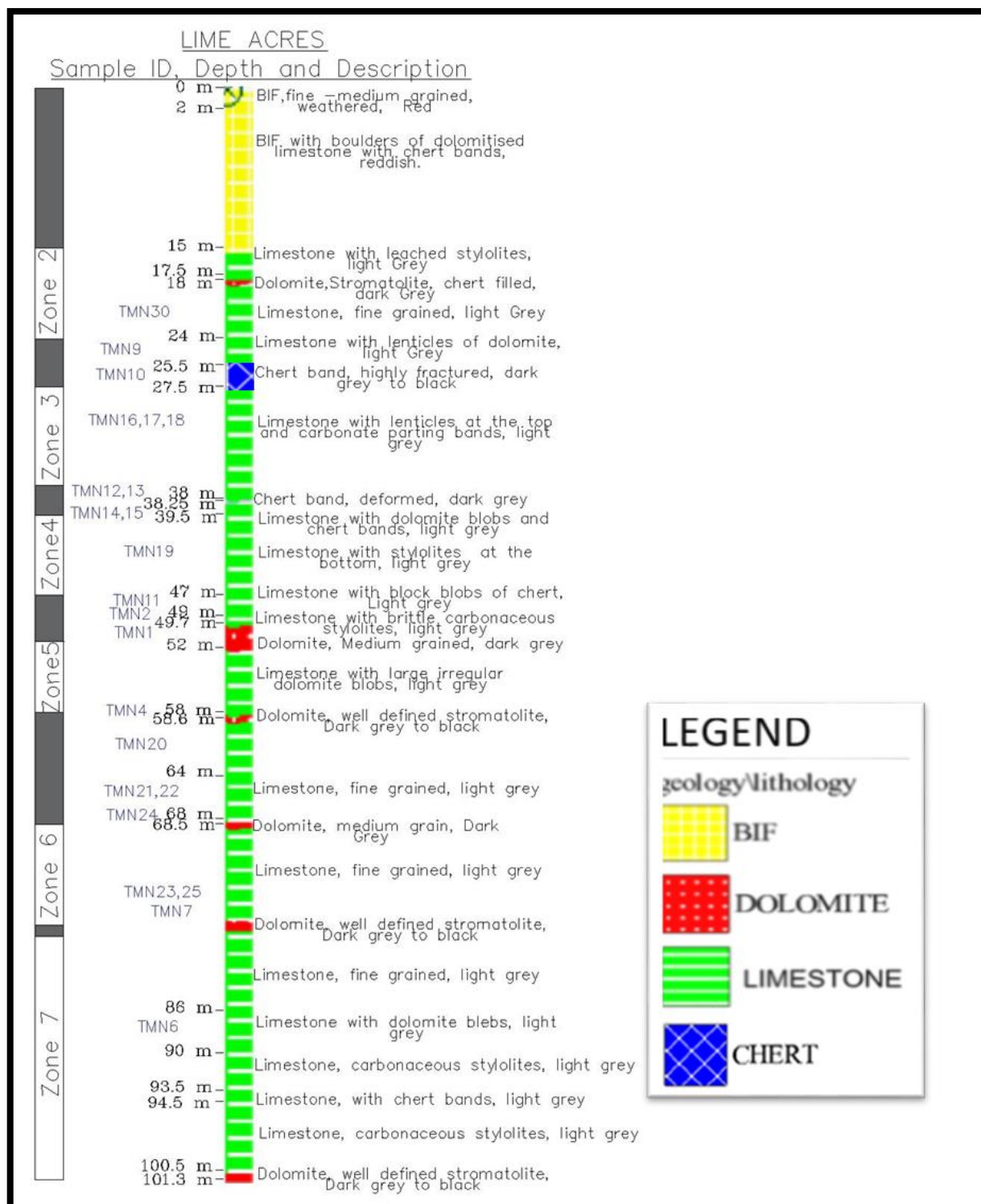
Figure 4.2.1 Cross sectional indication of the lithostratigraphic mapping at Lime Acres' mining face.
