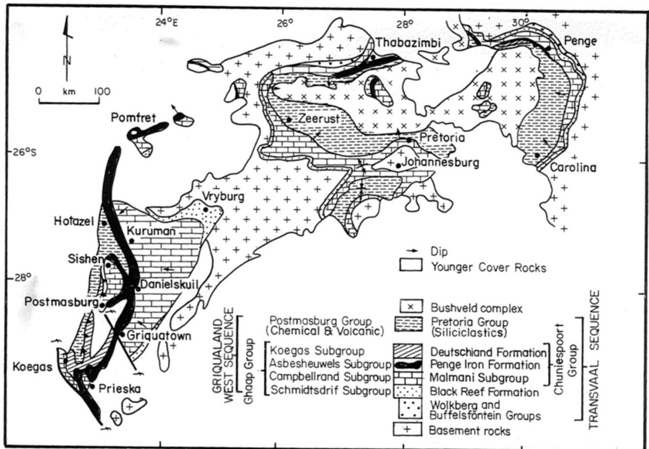
Figure 1.3 Geology of the Transvaal and Griqualand west sequences (Truswell, 1990).
