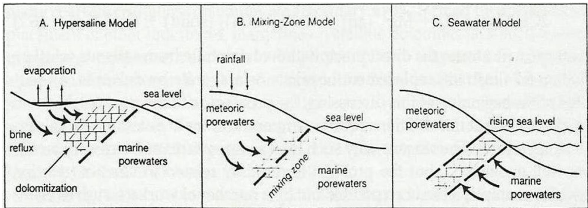
Figure 1.1 Dolomite models (Boggs, 2006).
