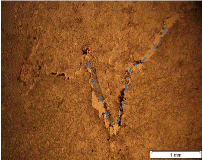
Figure 4.2.4: wavy stylolite on the fine grained dolomite with some quartz crystals.
