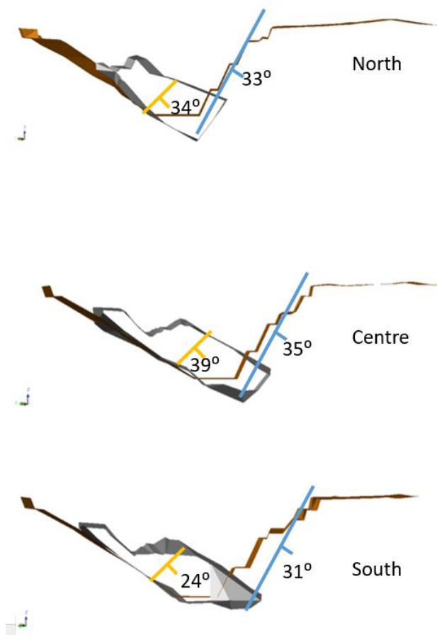
Figure 4.1.2: West-East cross sectional view of the Beestekraal quarry with indications of dip and strike.
