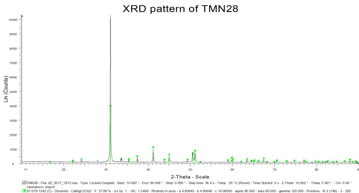
Figure 4.2.14 Whole rock XRD data showing dolomite (green) of TMN 28 collected at Lime Acres.
