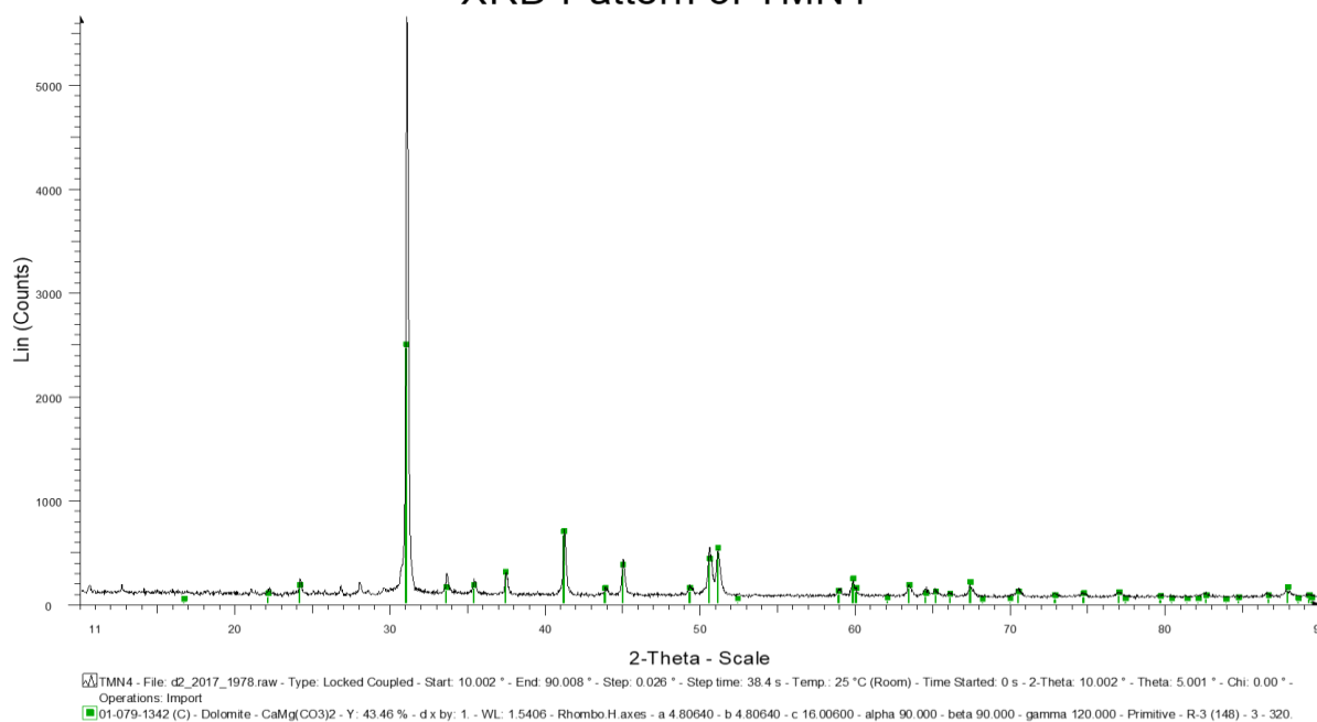
Figure 4.1.17 Whole rock XRD data showing dolomite (green) of TMN 4 collected at Lime Acres.
