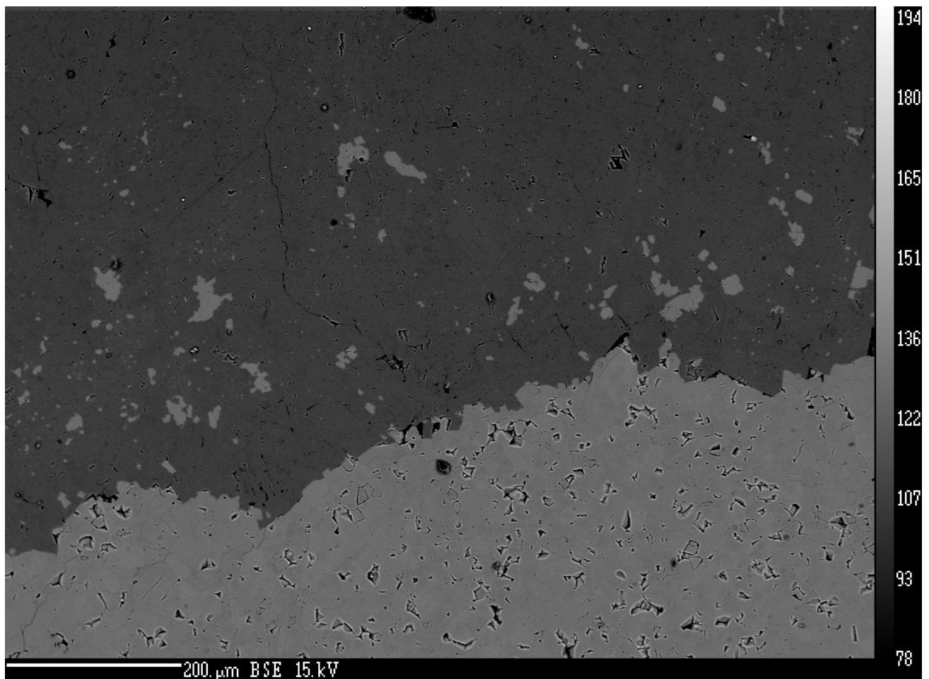
Fig 4.2.13 Microprobe image of Lime Acres sample TMN 6.
