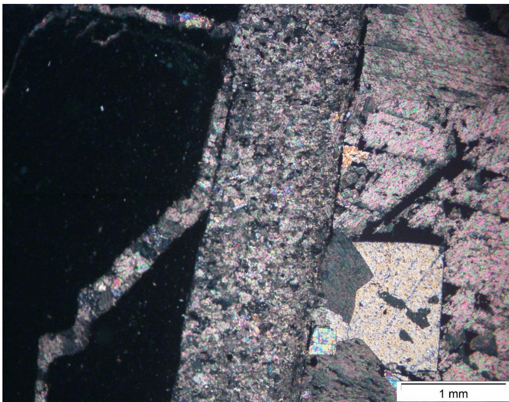
Figure 4.1.4 Calcite veinlets which cuts between the coarse grained crystals with twinning and quartz in cementation.
