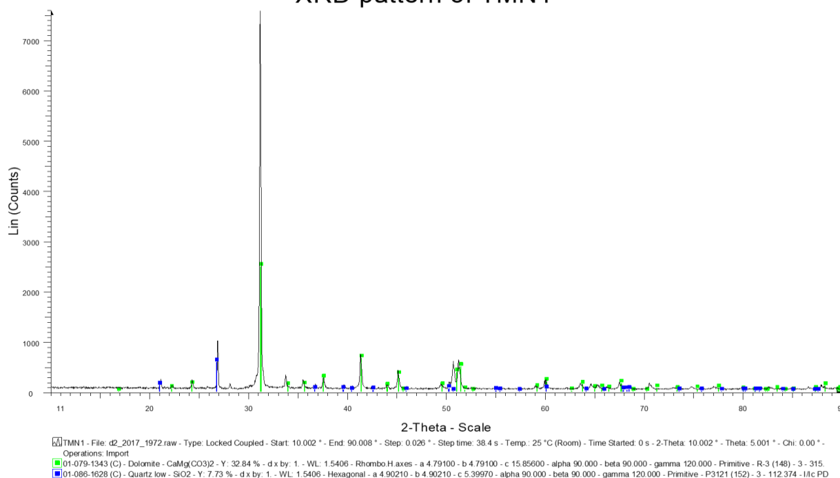
Figure 4.2.16 Whole rock XRD data showing dolomite (green) and quartz (blue) of TMN 1 collected at Lime Acres.
