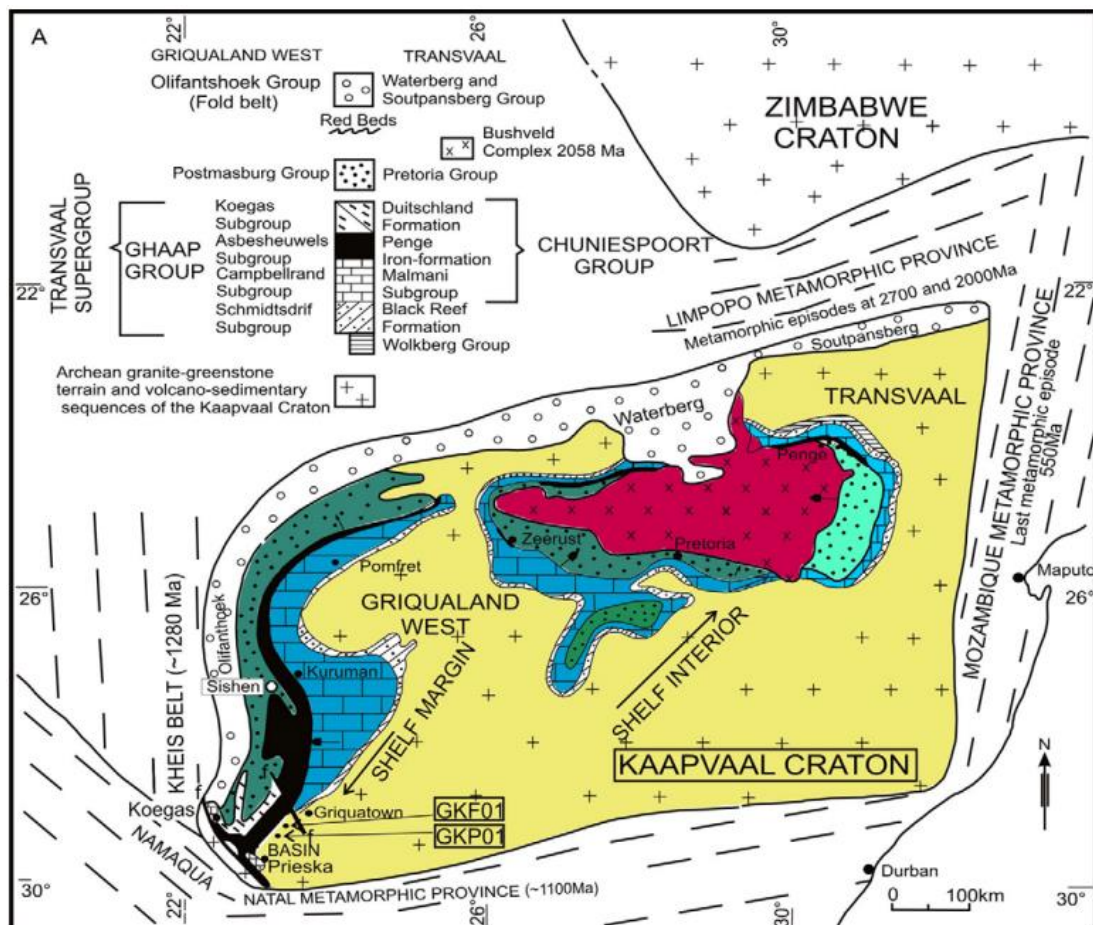
Figure 1.4 Map of the Transvaal Supergroup stratigraphic units, showing the distribution of the Campbellrand–Malmani carbonate platform (Knoll and Beukes, 2009).
