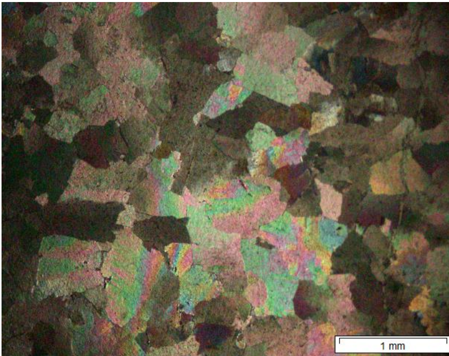
Figure 4.2.6 dolomite sample with re-entrance angles and no twinning.
