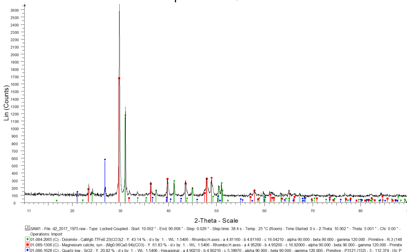
Figure 4.1.10 Whole rock XRD data for SAM1 showing dolomite (green) magnesium calcite (red) and quartz (blue) of SAM 1 collected in Beestekraal.
