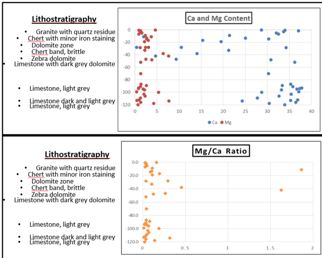
Figure 4.1.8 Calcite Magnesium representation at Beestekraal and Mg/Ca ratios with corresponding depths and brief field descriptions of the samples.
