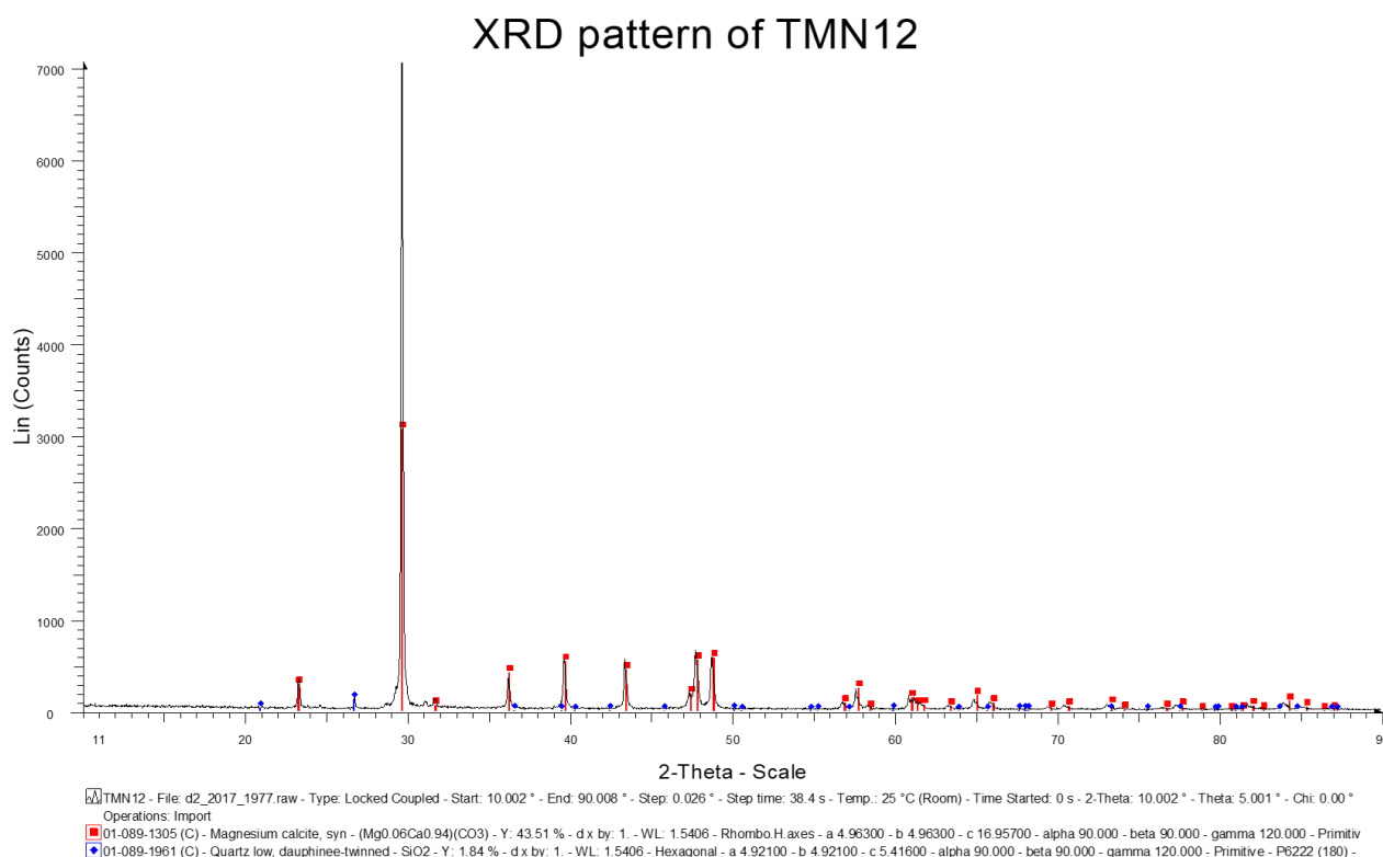
Figure 4.2.15 Whole rock XRD data showing magnesium calcite (red) and quartz (blue) of TMN 12 collected at Lime Acres.
