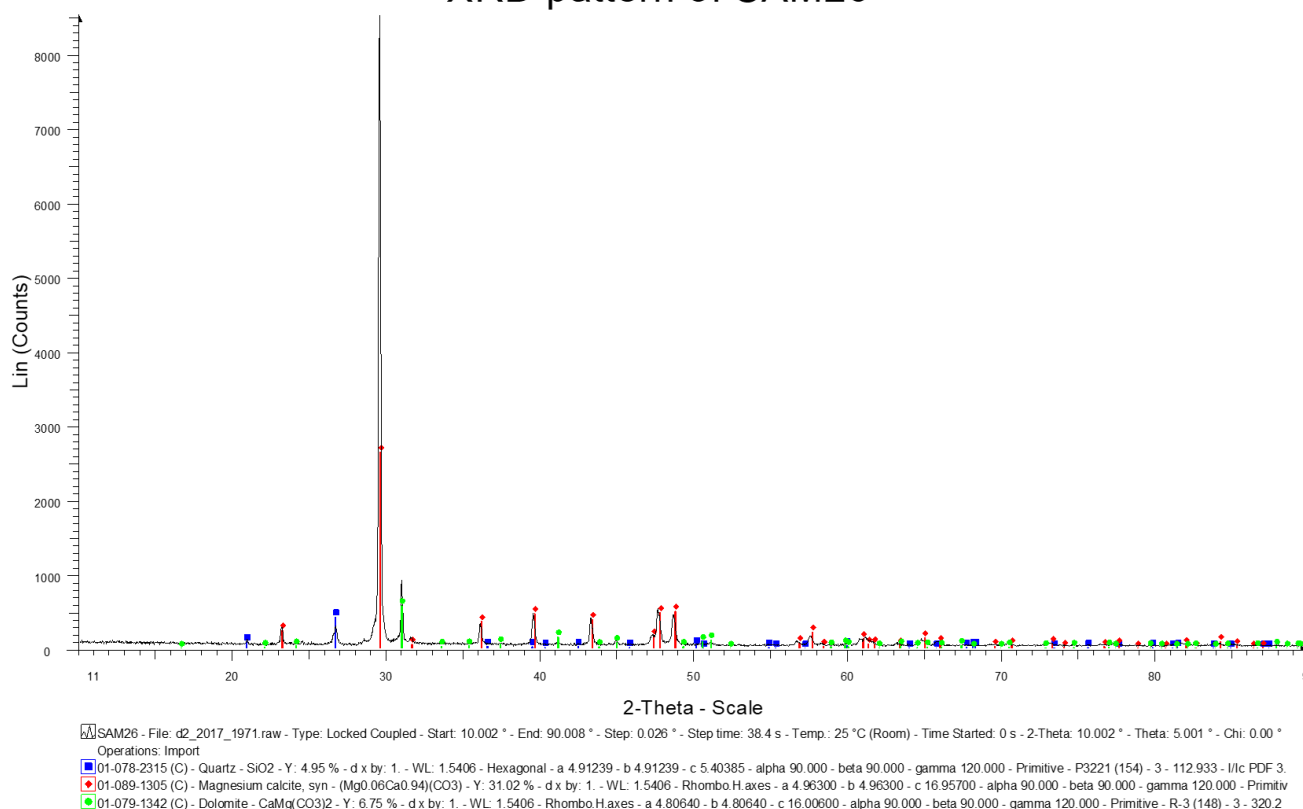
Figure 4.1.12 Whole rock XRD data showing dolomite (green) magnesium calcite (red) and quartz (blue) of SAM 26 collected at Beestekraal.
