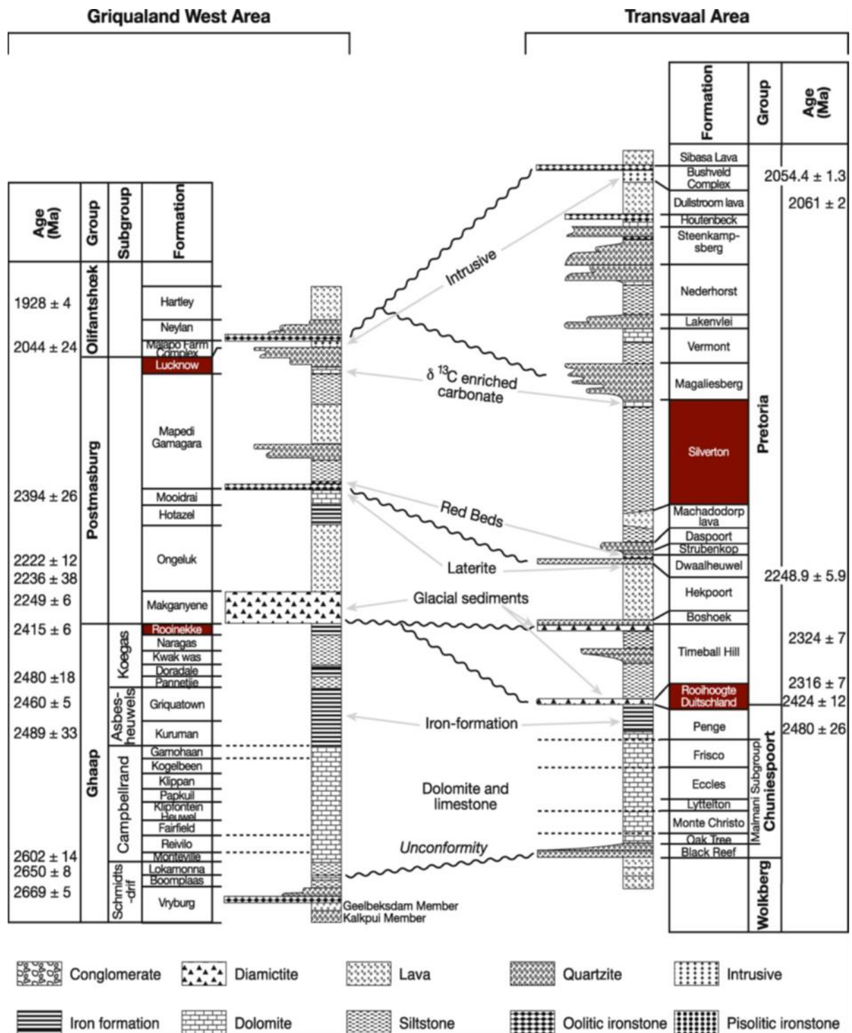
Figure 1.2: Generalized stratigraphy and correlation of the Transvaal Supergroup in the Griqualand West and Transvaal (Frauenstein et al., 2009).
