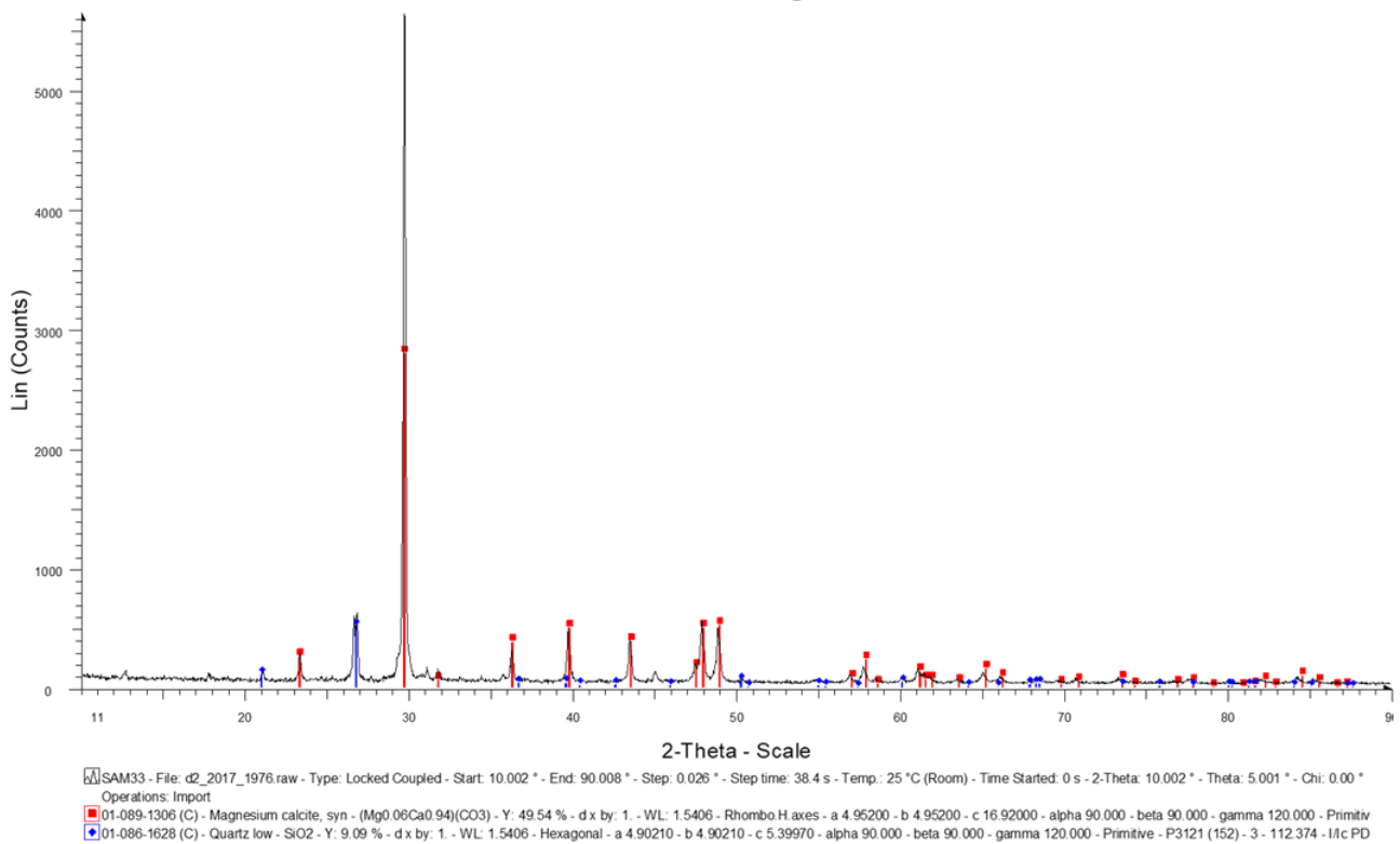
Figure 4.1.11 Whole rock XRD data showing magnesium calcite (red) and quartz (blue) of SAM 33 collected at Beestekraal.
