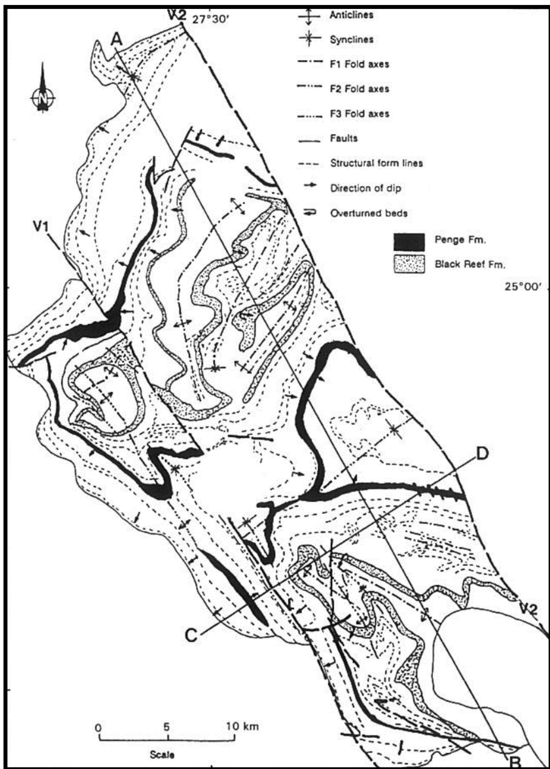
Figure 2.6 Simplified geological structure of the Crocodile River Fragment (Hartzer, 2000).
