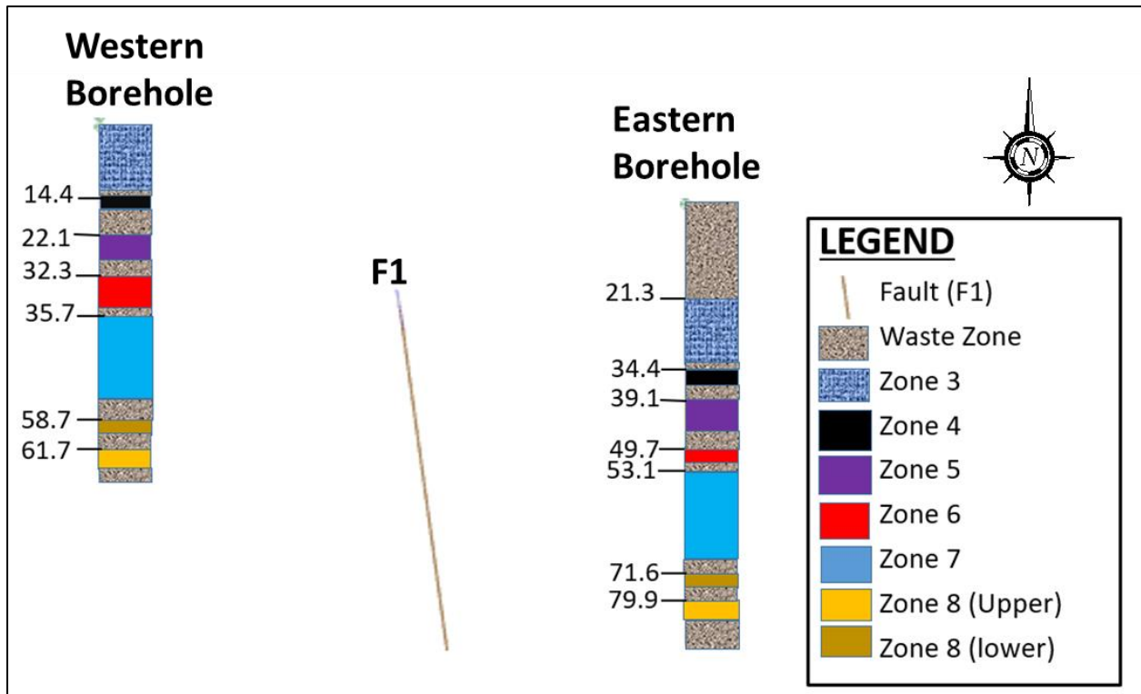
Figure 4.2.3 West-East cross sectional view Fault 1 with depth indications of how each limestone zone is shifted.
