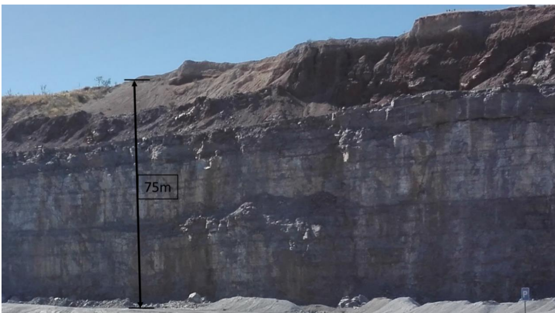
Figure 3.2: Cross sectional indication of Lime Acres' Mining face.
