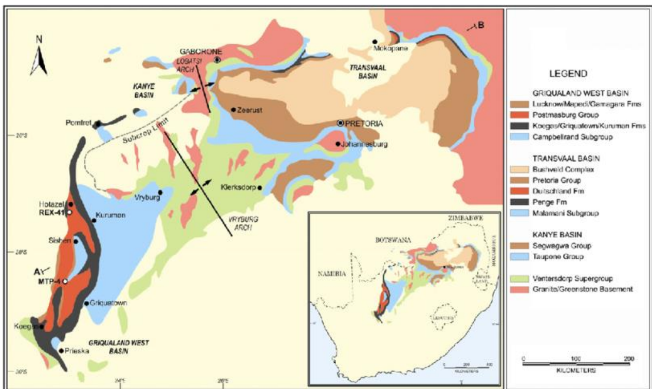
Figure 2.1 The regional geological map of exposures of the Transvaal Supergroup with indications on the Campbellrand Subgroup and Malmani Subgroup (Moore et al. , 2012).
