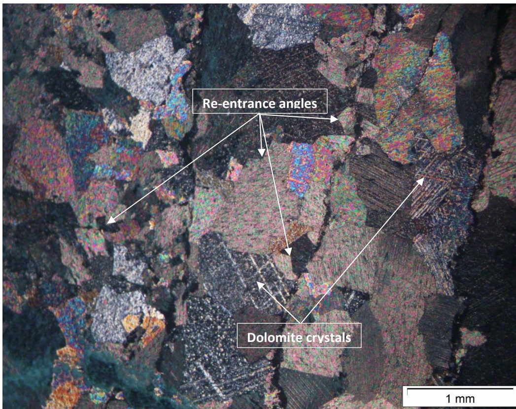
Figure 4.1.3. An indication of the crystal structure with re-entrance angles and twinning patterns.
