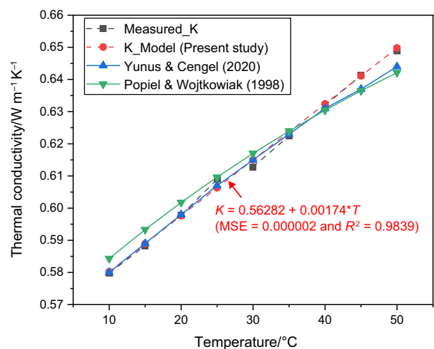
Fig. 6 Validation of thermal conductivity model
