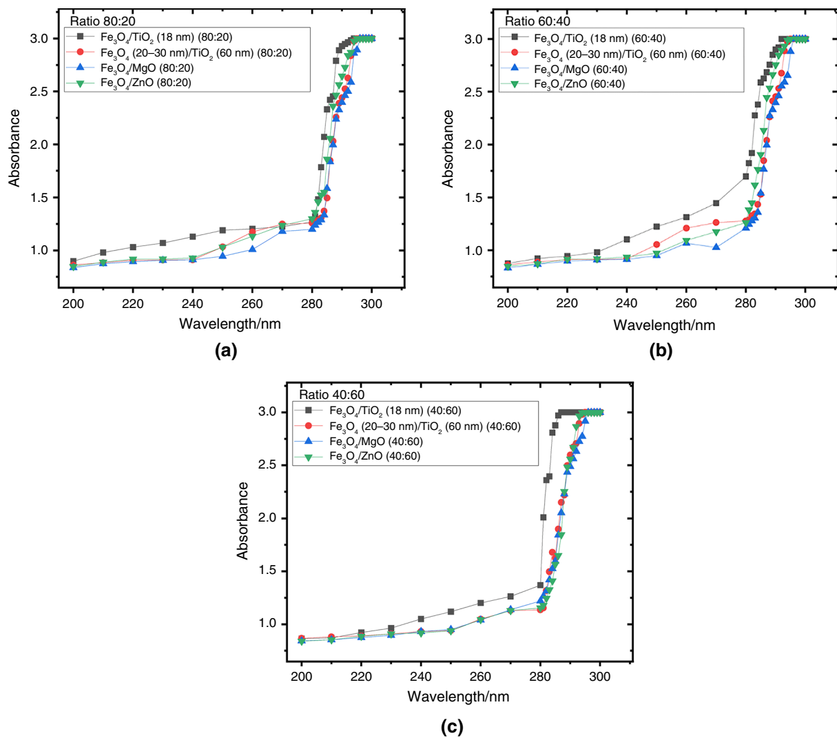
Fig. 3 UV–Vis spectrum of magnetic hybrid nanofluid dispersed in DIW with ratio a 80:20, b 60:40, and c 40:60
