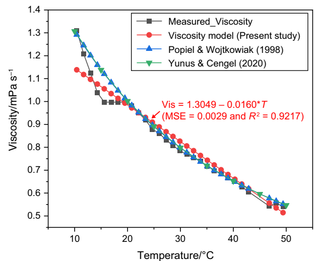
Fig. 14 Validation of viscosity model with experimental results and previous studies
