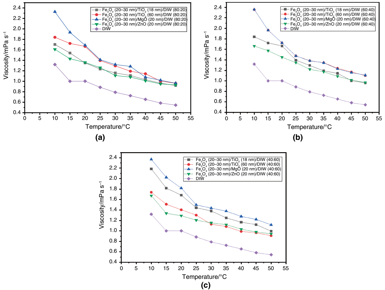
Fig. 13 Viscosities of MHFs/DIW with a 80:20, b 60:40, and c 40:60 at different temperatures
