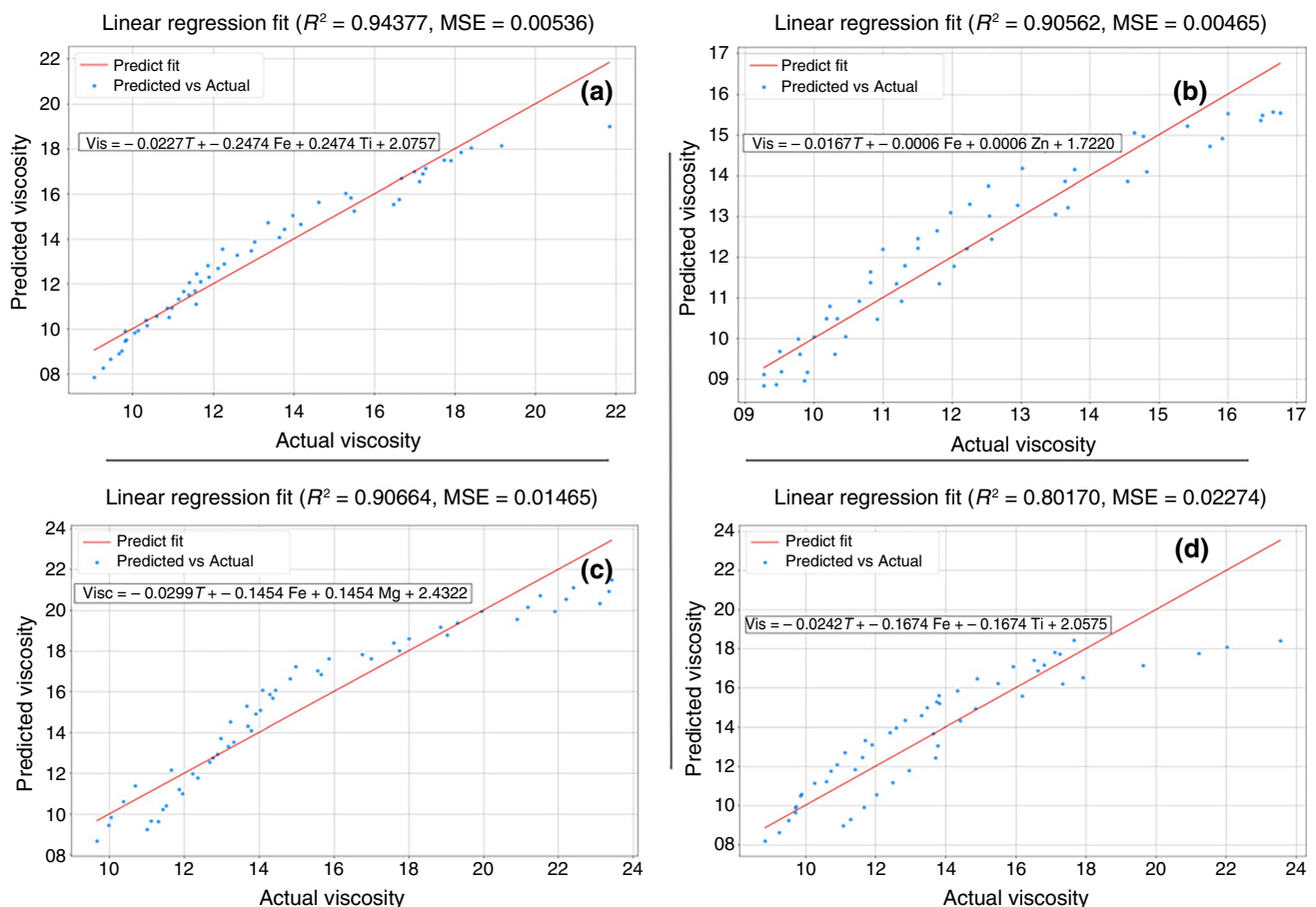
Fig. 15 Linear regression model predictions for viscosity ( K ) of a \text{Fe}_3\text{O}_4\text{-TiO}_2 (18 nm), b \text{Fe}_3\text{O}_4\text{-ZnO} , c \text{Fe}_3\text{O}_4\text{-MgO} , and d \text{Fe}_3\text{O}_4\text{-TiO}_2 (60 nm) DIW hybrid ferrofluids
