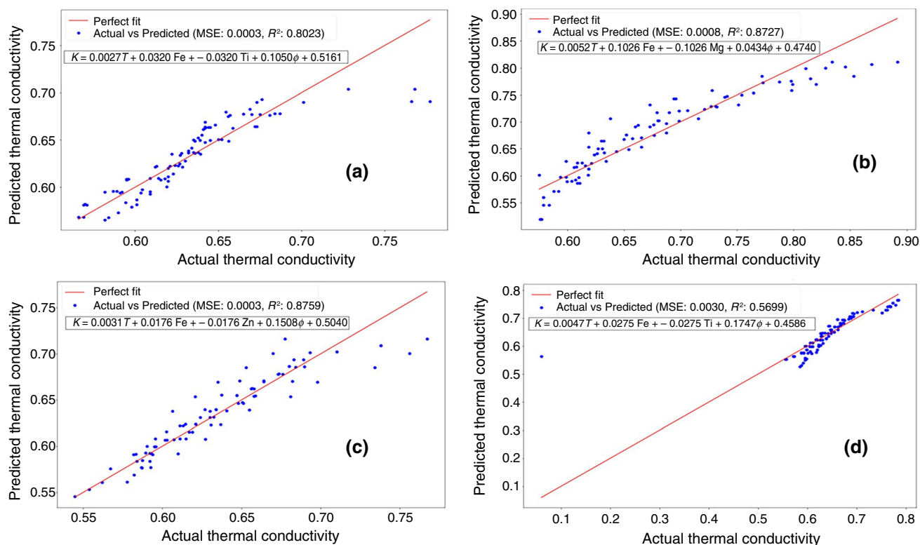
Fig. 7 Linear regression model predictions for thermal conductivity ( K ) of a \text{Fe}_3\text{O}_4\text{-TiO}_2 (18 nm), b \text{Fe}_3\text{O}_4\text{-MgO} , c \text{Fe}_3\text{O}_4\text{-ZnO} , and (d) \text{Fe}_3\text{O}_4\text{-TiO}_2 (60 nm) DIW hybrid ferrofluids
