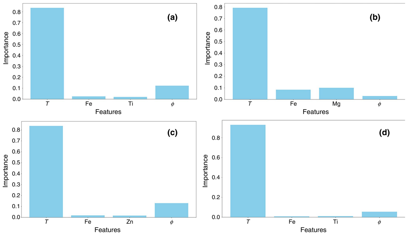
Fig. 8 Feature importance analysis for predicting thermal conductivity of a Fe 3 O 4 -TiO 2 (18 nm), b Fe 3 O 4 -MgO, c Fe 3 O 4 -ZnO and (d) Fe 3 O 4 -TiO 2 (60 nm) DIW hybrid ferrofluids
