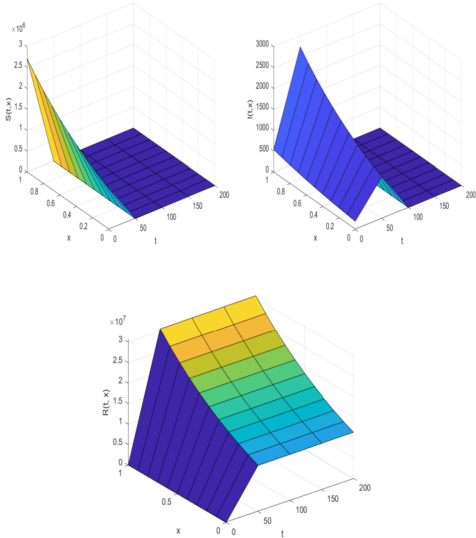
FIGURE 1. The surface plots for S(t, x) , I(t, x) and R(t, x) for 0 \leq t \leq 200 and 0 \leq x \leq 1 . We used S_0 = 10^6 - 200 - 50 , I_0 = 200 , R_0 = 50 , \lambda = 1.0 , d_1 = 0.2 , d_2 = 0.3 , \beta = 1.5 , \gamma = 0.5 .
