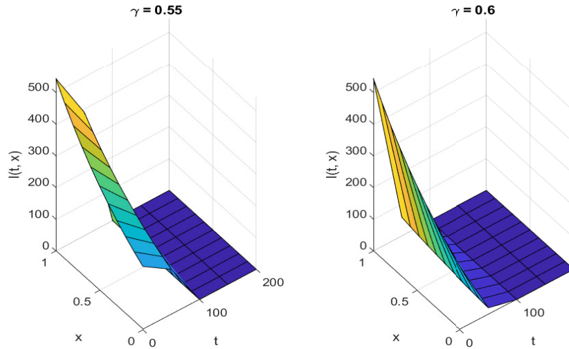
FIGURE 4. The effect of changing the recovery rate \gamma on the epidemic peak for 0 \leq t \leq 200 and 0 \leq x \leq 1 . We used S_0 = 10^6 - 200 - 50 , I_0 = 200 , R_0 = 50 , \lambda = 1.0 , d_1 = 0.2 , d_2 = 0.3 , \beta = 1.5 .
