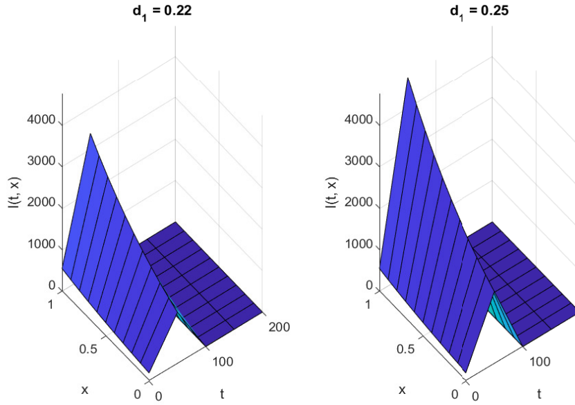
FIGURE 2. The effect of changing the diffusion coefficient d_1 of the infected population on the epidemic peak for 0 \leq t \leq 200 and 0 \leq x \leq 1 . We used S_0 = 10^6 - 200 - 50 , I_0 = 200 , R_0 = 50 , \lambda = 1.0 , d_2 = 0.3 , \beta = 1.5 , \gamma = 0.5 .
