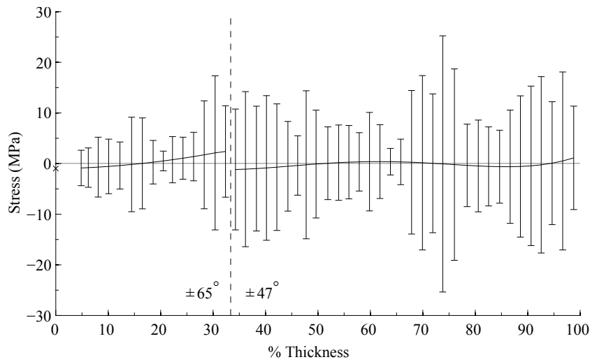
Fig. 18 Shear stress of \pm 65^\circ/\pm 47^\circ layered pipe
