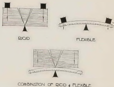
EFFECT OF FLEXIBILITY OF FOUNDATIONS FIG. 4
