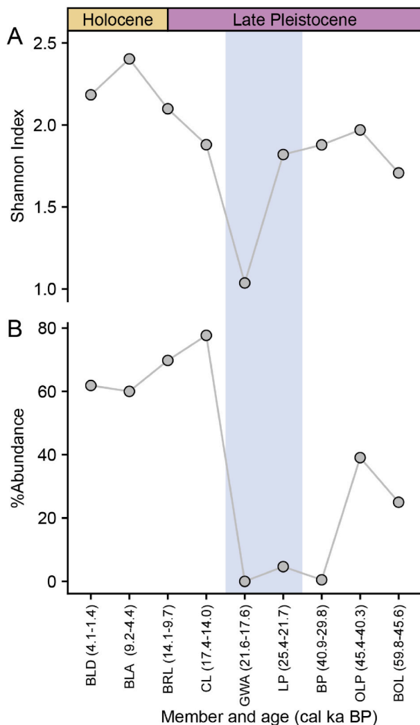
Fig. 10. A: Taxonomic diversity (Shannon index) of the charcoal assemblages through the Boomplaas Cave sequence. B: The percent abundance of trees and tall shrubs recovered from Boomplaas Cave. Data from Scholtz (1986). Vertical bar denotes the LGM members.
