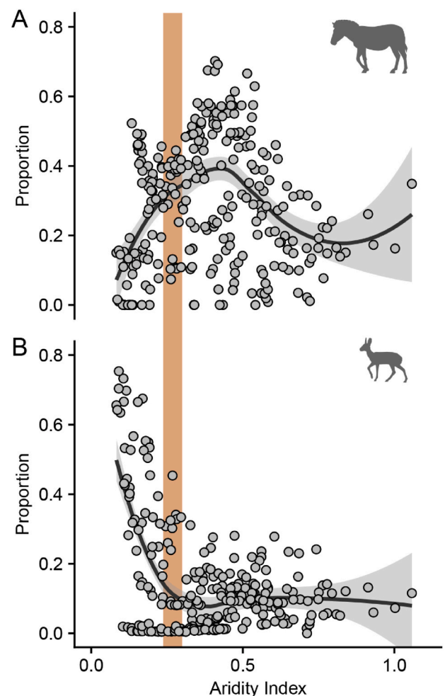
Fig. 4. A: The proportion of equids and alcelaphins across southern Africa as a function of aridity (Aridity index = MAP/MAE; MAP = mean annual precipitation; MAE = mean annual evapotranspiration; larger values indicate greater moisture). B: The relative abundance of Raphicerus spp., Oreotragus oreotragus , Pelea capreolus , and Redunca fulvorufula as a function of aridity. Solid lines are LOESS curves (span = 0.75) with 95% confidence interval in grey. Vertical bar denotes range of aridity index values within a 2.5 km radius of Boomplaas Cave today (from Trabucco and Zomer, 2009). Herbivore data are from Hempson et al. (2015) for the following ecoregions: Albany thickets, Drakensberg Escarpment savanna and thicket, Drakensberg grassland, fynbos shrubland, highveld grassland, Limpopo lowveld, Nama Karoo shrubland, Renosterveld shrubland, Succulent karoo xeric shrubland.
