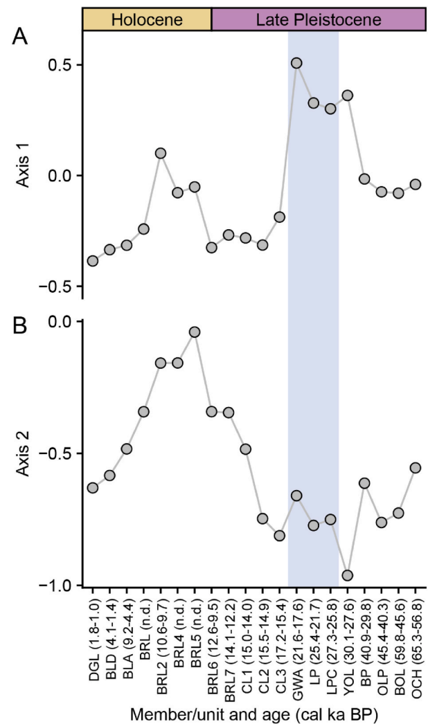
Fig. 9. A: Axis 1 scores derived from a canonical correspondence analysis (CCA) of the micromammal assemblages across the Boomplaas Cave sequence (from Faith et al., 2019). These values strongly correlate with rainfall seasonality in modern assemblages ( r = -0.88 ), with larger values indicating a greater proportion of winter rain. B: Axis 2 scores from the same analysis. These values strongly correlate with aridity in modern assemblages ( r = -0.86 ), with larger values indicating greater aridity. Vertical bar denotes the LGM members.
