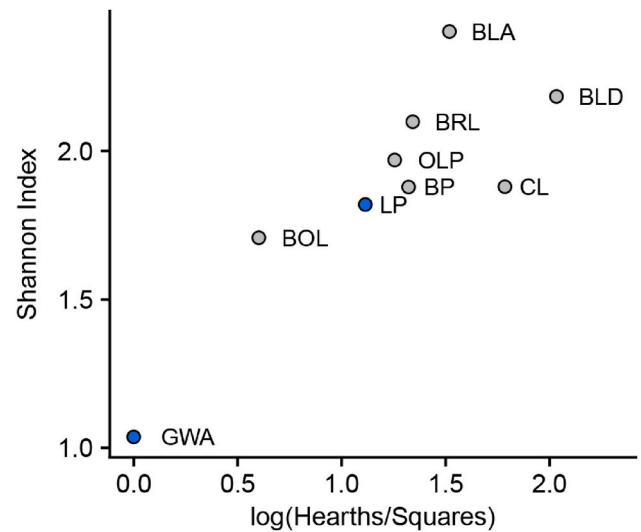
Fig. 11. The relationship between sampling strategy (log-transformed number of hearths or squares) and taxonomic diversity (Shannon index) for the Boomplaas charcoal assemblages. Scholtz (1986) provided counts of the number of specimens analyzed from each member and following his description of the sampling strategy, we assume that two charcoal specimens were analyzed from each hearth or square from members BLD to CL and that 10 specimens were analyzed from each hearth or square in the underlying levels. Scholtz (1986) notes that only one hearth was sampled in member GWA/HCA. Data from Scholtz (1986). Blue dots signify LGM members.
