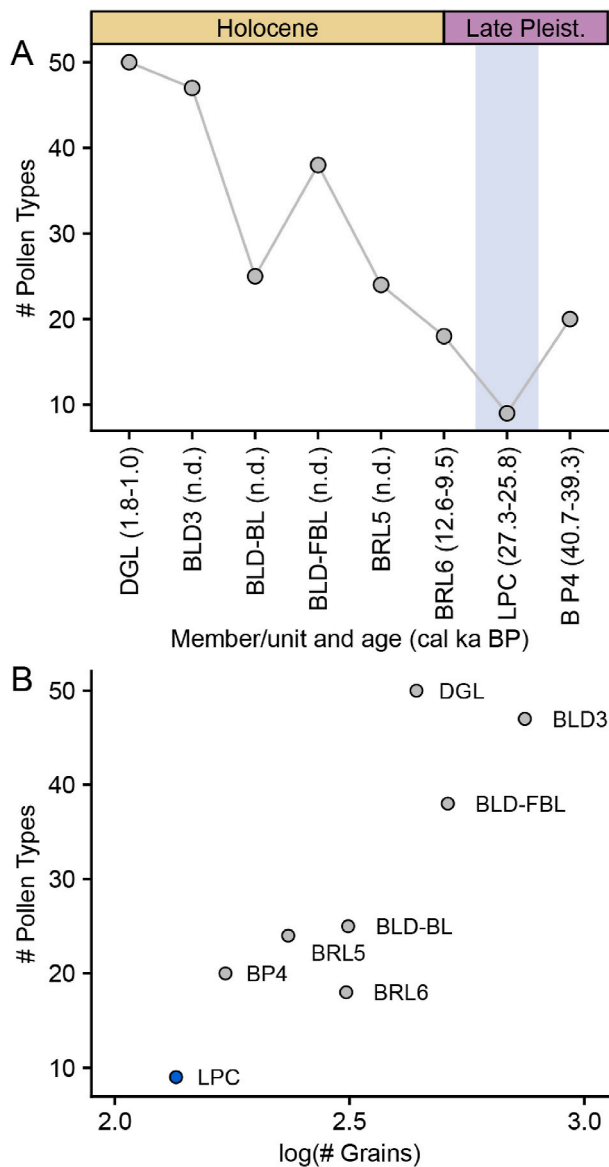
Fig. 12. A: The number of pollen types across the Boomplaas Cave sequence. Vertical bar denotes the LGM members. B: the relationship between sample size (# of grains counted) and the number of pollen types. The LGM member (LPC) is indicated in blue. Data from Deacon (1983b).
