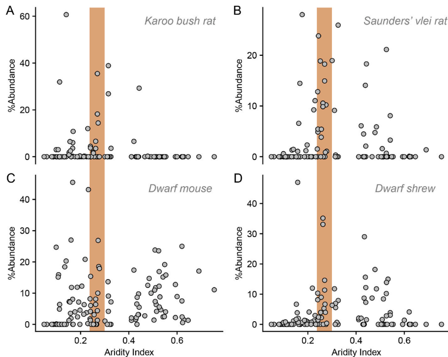
Fig. 7. The percent abundance of (A) Karoo bush-rat, (B) Saunders' vlei rat, (C) dwarf mouse, and (D) dwarf shrew as a function of aridity (Aridity Index [AI] = MAP/MAE; larger values indicate greater moisture availability) in present-day southern Africa (data from Faith et al., 2019). Vertical bars denote range of aridity index values in the vicinity of Boomplaas Cave today (as in Fig. 4).
