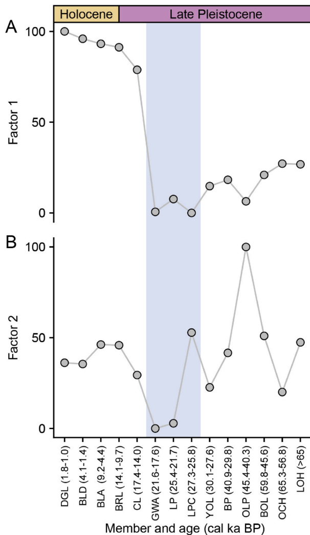
Fig. 8. A: Factor 1 summary statistics derived from a factor analysis of micromammals across the Boomplaas Cave sequence (following Deacon et al., 1984). These values were interpreted as tracking temperature changes through the sequence, with larger values indicating warmer conditions (see Thackeray, 1987). B: Factor 2 summary statistics from the same analysis. These values were interpreted as tracking moisture availability across the sequence, with larger values indicating more humid conditions. Vertical bar denotes the LGM members.
