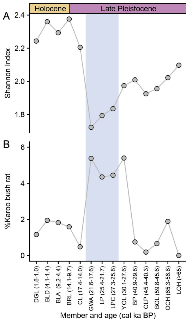
Fig. 6. A: Taxonomic diversity (Shannon index) of micromammals (bats excluded) through the Boomplaas Cave sequence. B: Changes in the abundance of Karoo bush-rat through the Boomplaas Cave sequence. Data from Avery (1982). Vertical bar denotes the LGM members.
