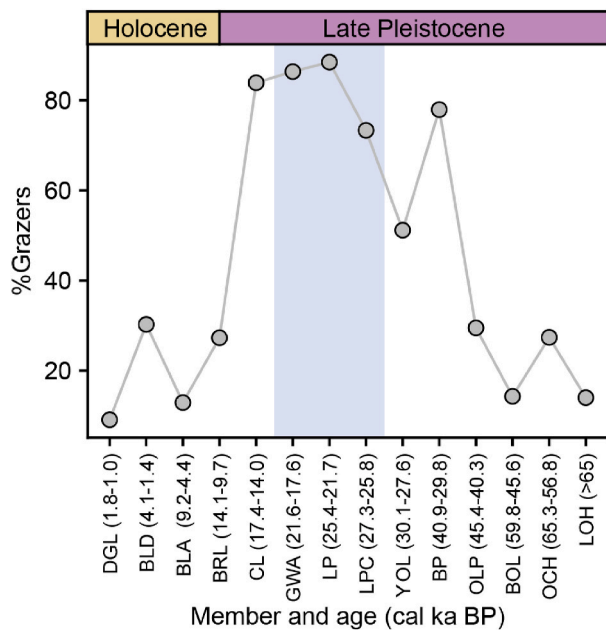
Fig. 3. Changes in the abundance (% of specimens) of ungulate grazers through the Boomplaas Cave sequence (data from Klein, 1983 for DGL; Faith, 2013a for BLD through LOH). Vertical bar denotes the LGM members.
