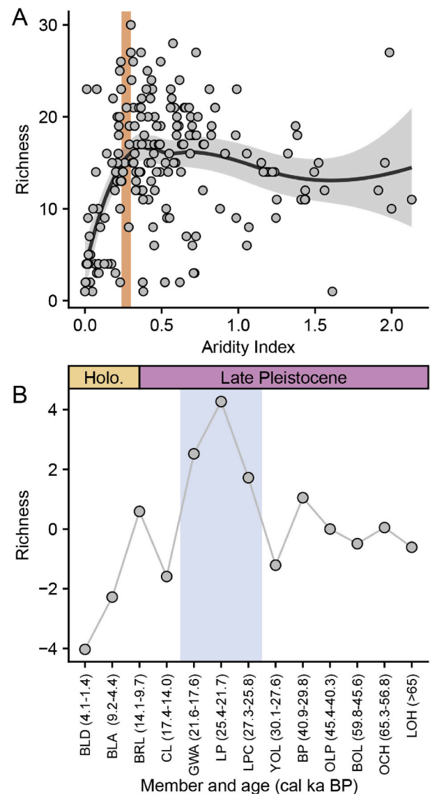
Fig. 5. A: Ungulate richness as a function of aridity across Africa (Aridity Index = MAP/MAE; larger values indicate greater moisture availability). Solid lines are LOESS curves (span = 0.75) with 95% confidence interval in grey. Vertical bar denotes range of aridity index values in the vicinity of Boomplaas Cave today (as in Fig. 4). Faunal data from Faith et al. (2018). B: Temporal trends in ungulate richness across the Boomplaas Cave sequence (from Faith, 2013a). Values represent residuals calculated from a linear regression of richness as a function of assemblage sample size. Vertical bar denotes the LGM members.
