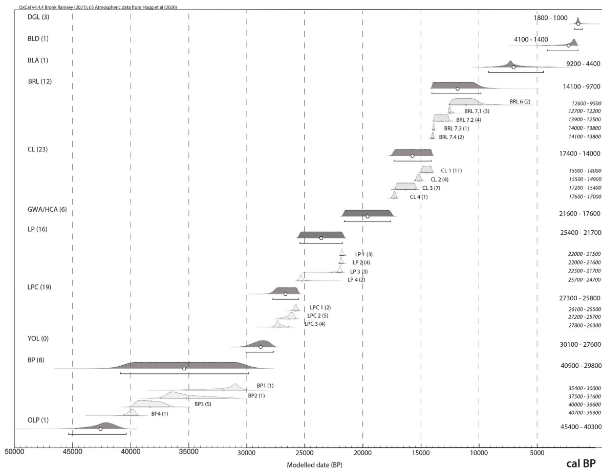
Fig. 2. The radiocarbon chronology of the Boomplaas Cave sequence. Ages for each member and for select units are modelled ^{14}\text{C} ages with 2\sigma ranges. The chronology is updated from Pargeter et al., (2018) in OxCal 4.4 (Bronk Ramsey 2009) using ShCal20 (Hogg et al., 2020). Values in parentheses indicate the number of dates. The ages of the underlying members (BOL, OCH, and LOH) are poorly constrained, though OCH is associated with U-series and amino acid racemization age estimates of ~60–65 ka (Miller et al., 1999; Vogel, 2001). Figure courtesy of Emma Loftus.
