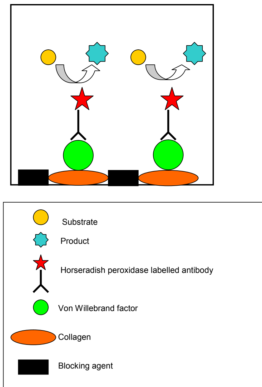
Figure 5. Schematic representation of the VWF binding ELISA assay. The microtitre plate well is coated with collagen. Any remaining sites on the microtitre plate are blocked with blocking agent. When the patient sample is added to the microtitre plate well, the patient's VWF binds the collagen covering the well surface. The wells are then washed, and horseradish peroxidase labelled anti-VWF antibody is added. Another wash step is performed, and substrate (ABTS TM ) is added which is enzymatically converted to product. The increase in absorbance is then measured spectrophotometrically at 405nm.
