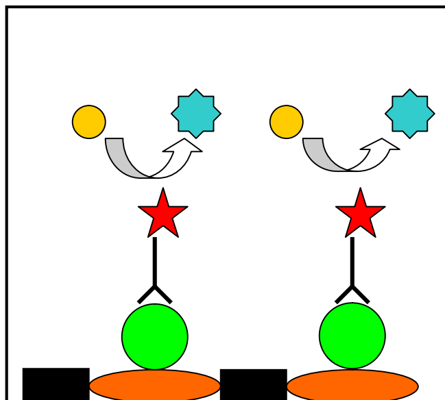
Figure 7. Schematic representation of microtitre plate well with deficient VWFCP activity. When a deficiency of VWFCP exists, such as in TTP, less VWF is cleaved by the VWFCP, leaving more VWF to bind to the collagen coating the microtitre plate well. This results in a dialysed: undialysed ratio of RCBA above the cut-off value.
