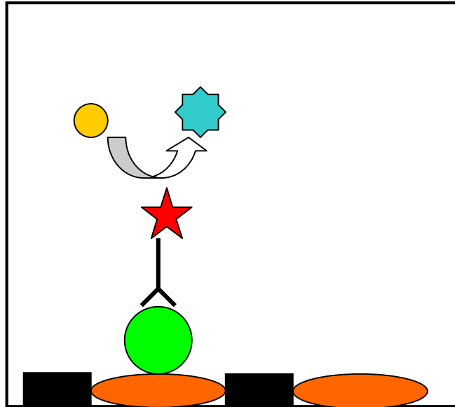
Figure 6. Schematic representation of microtitre plate well with normal VWFCP activity. Under normal circumstances, when there is no deficiency of VWFCP, the VWF is cleaved by the VWFCP which leaves less VWF remaining capable of binding to the collagen on the microtitre plate well. This results in a dialysed: undialysed ratio of RCBA below the cut-off value.
