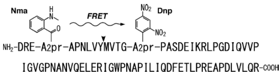
Figure 4. Schematic representation of structure of fluorescence resonance energy transfer (FRETs)-Von Willebrand factor (VWF)-73 substrate. Amino acid residues Q1599 and N1610 (which are within the 73 amino acid peptide corresponding to the region D1595-R1668 of VWF) are replaced by A2pr (Nma) and A2pr (Dnp) respectively. The arrow indicates the cleavage site of ADAMTS13. Diagram from: Kokame, K., Nobe, Y., Kokubo, Y., et al. 2005. FRETs-VWF73, a first fluorogenic substrate for ADAMTS13 assay. Br J Haematol , vol.129, pp. 94.
