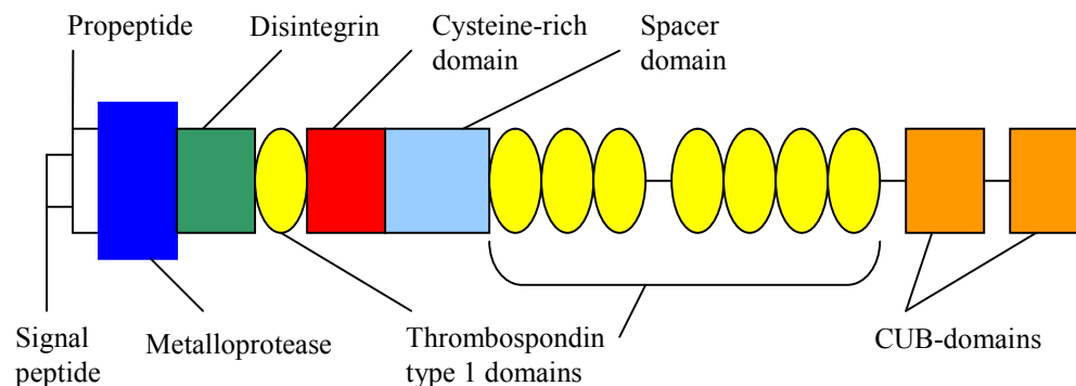
Figure 2. Schematic depiction of the ADAMTS13 protein. Adapted from: Lämmle, Kremer-Hovinga & Alberio, 2005. Thrombotic Thrombocytopenic Purpura. J Thromb Haemost , vol. 3, pp. 1665.
