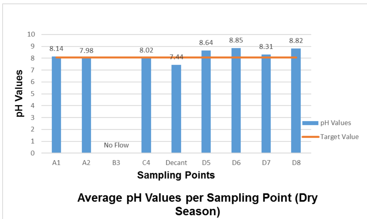
Figure 23: Average pH values per Sampling Point in the dry season
