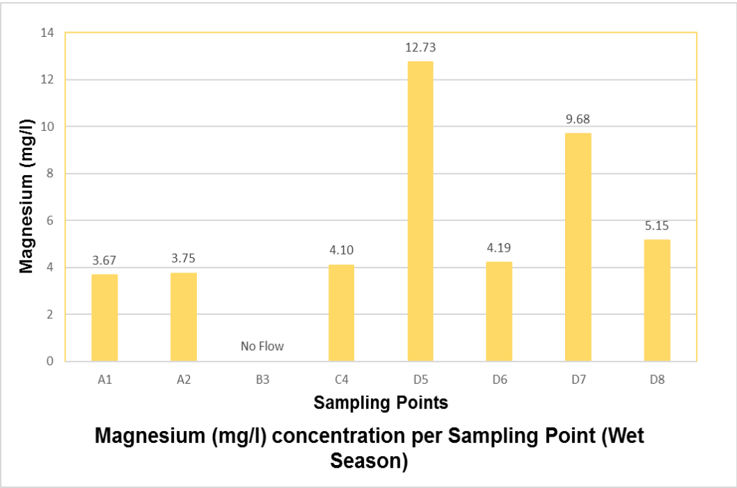
Figure 19: Magnesium concentration per sampling point in the wet season
