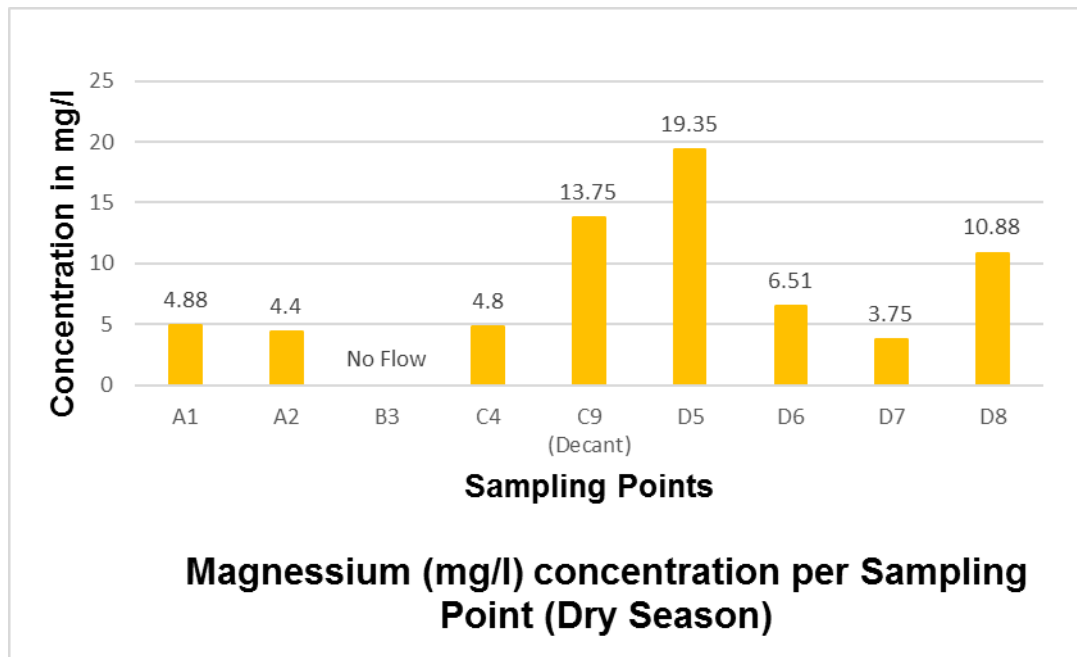
Figure 28: Magnesium concentration per sampling point during the dry season
