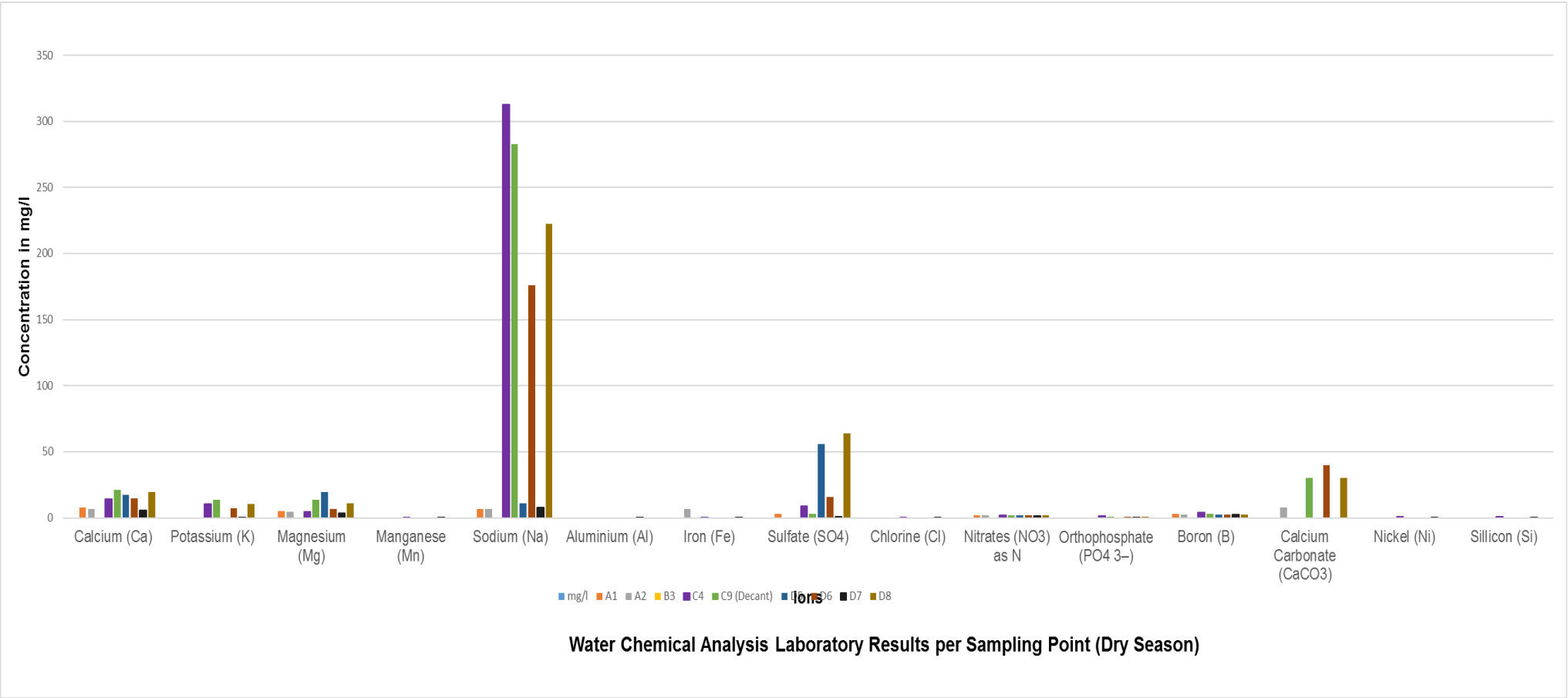
Figure 25: Water chemical analysis laboratory results for a dry season
