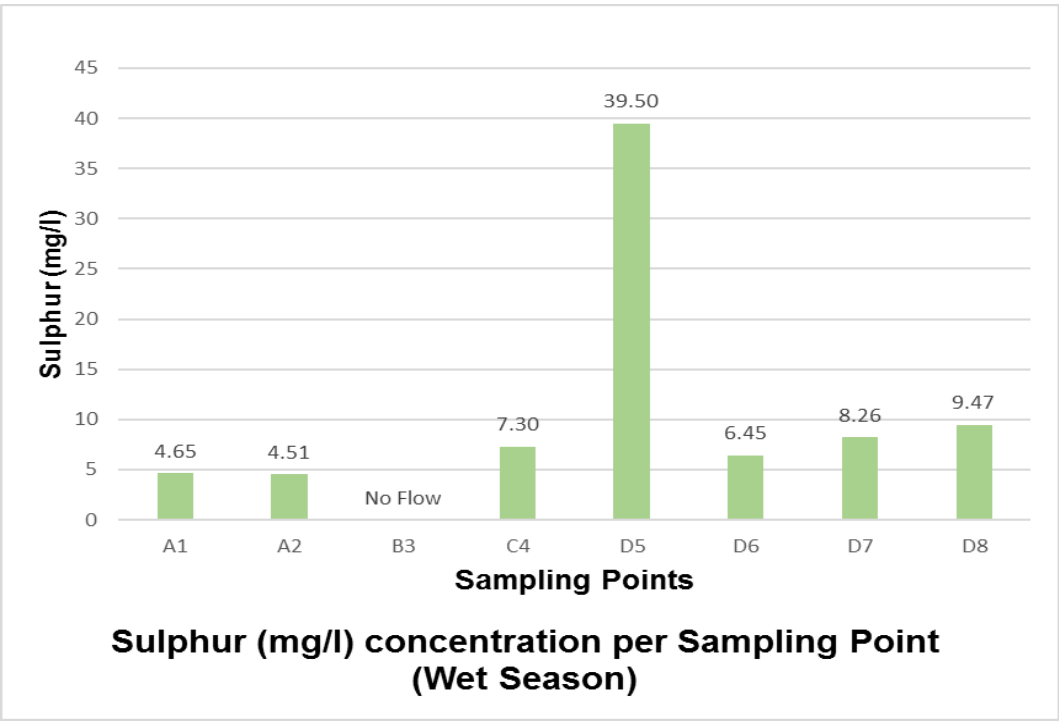
Figure 20: Sulphur concentration per sampling point in the wet season
