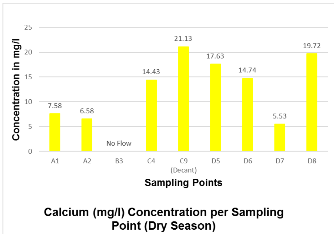
Figure 26: Calcium concentration per sampling point in the dry season
