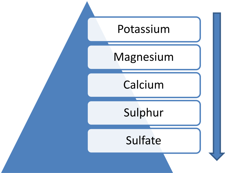
Figure 22: The ranking of water quality parameters that were above the target value, increasing downwards
