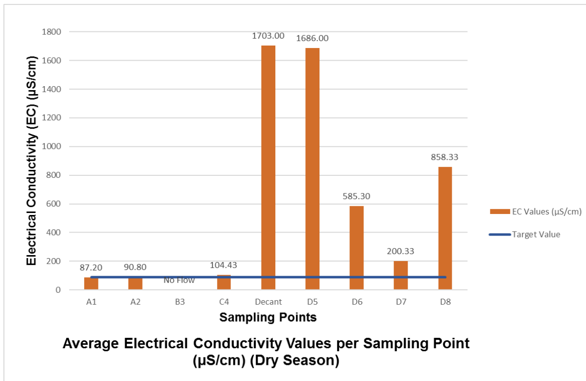
Figure 24: Average EC values per sampling points during the dry season
