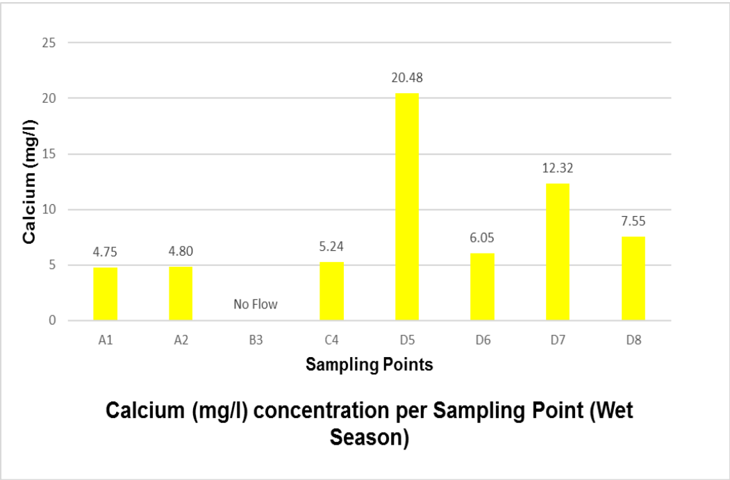
Figure 17: Calcium concentration per sampling point in the wet season
