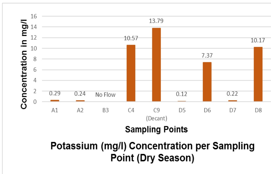
Figure 27: Potassium concentration per sampling point in the dry season
