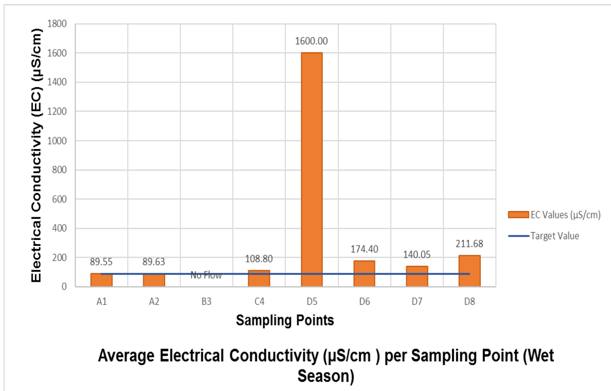
Figure 15: Average Electrical Conductivity per Sampling Point in the wet season
