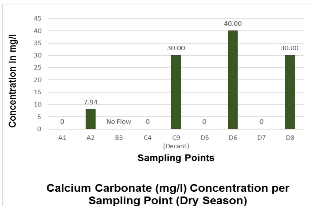
Figure 31: Calcium Carbonate concentration per sampling point in the dry season
