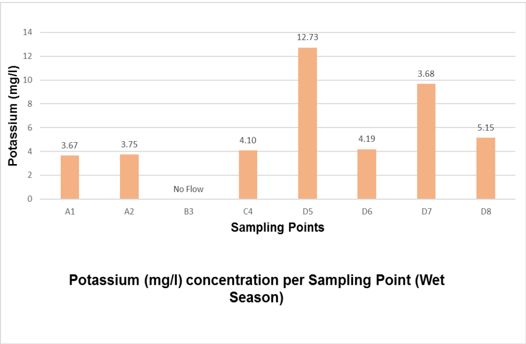
Figure 18: Potassium concentration per sampling point in the wet season
