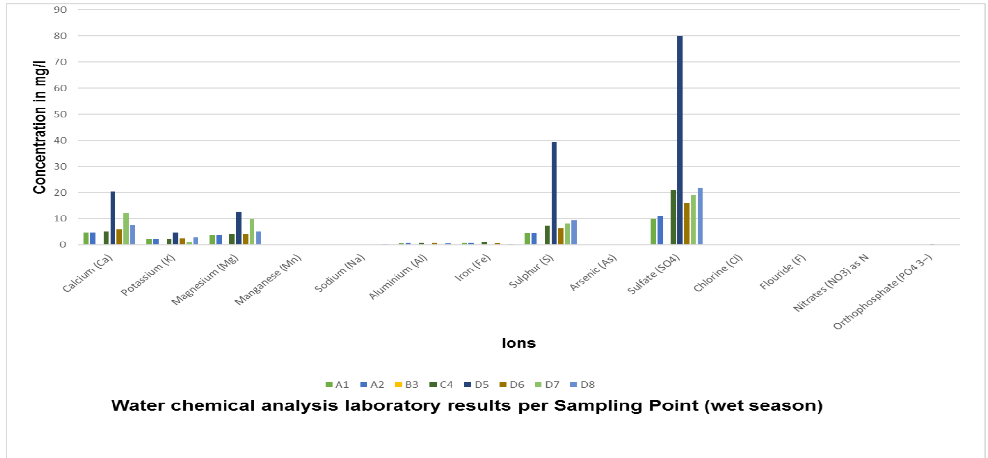
Figure 16: Laboratory results for chemical analysis per sampling point in the wet season
