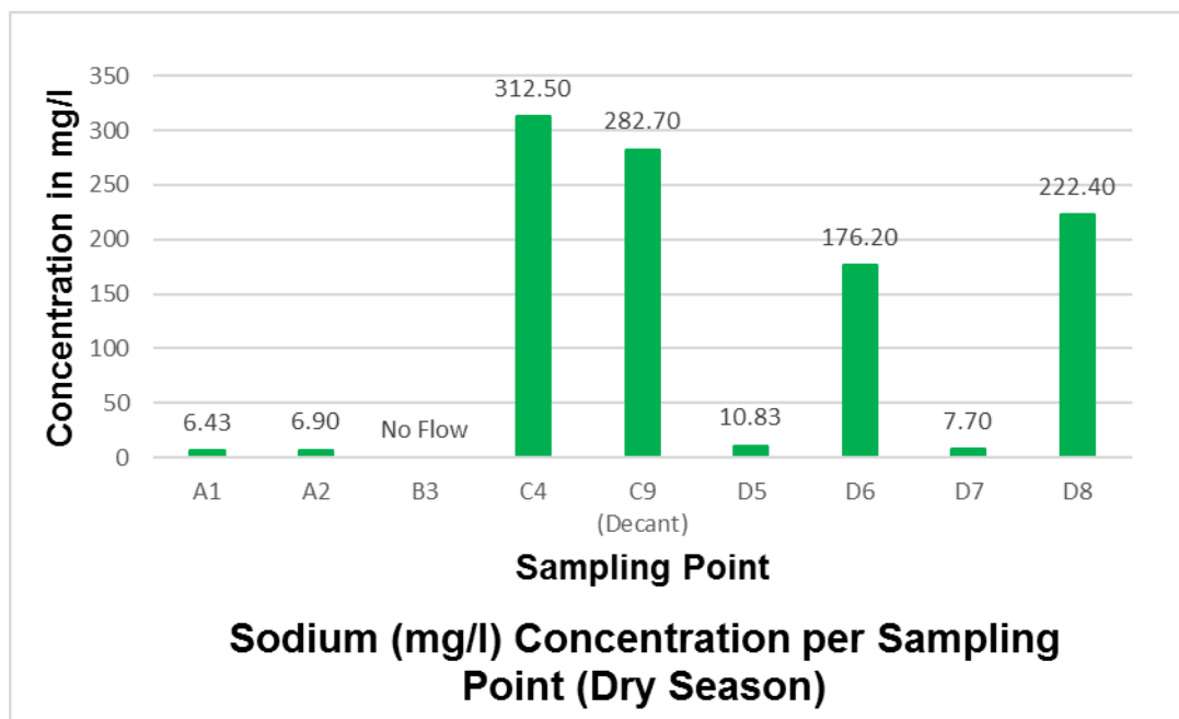
Figure 29: Sodium concentration per sampling point during the dry season
