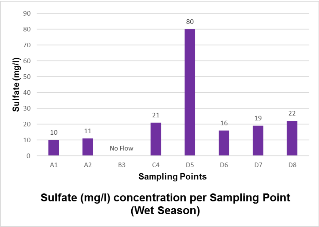
Figure 21: Sulfate concentration per sampling point in the wet season
