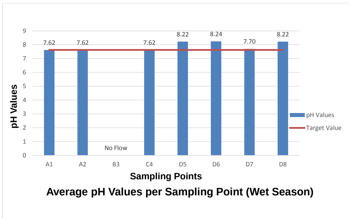
Figure 14: Average pH values per Sampling Point in the wet season
