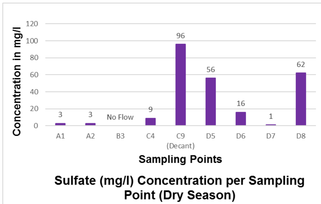
Figure 30: Sulfate concentration per sampling point in the dry season
