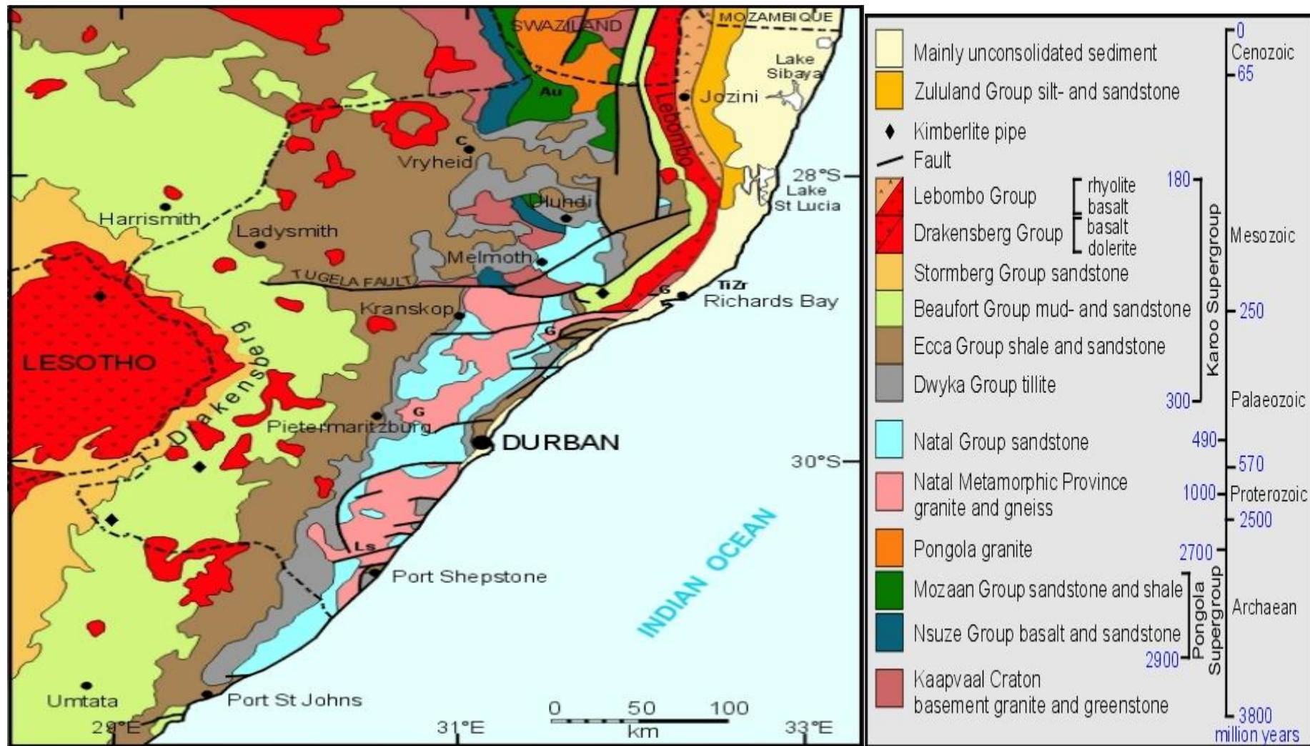
Figure 8: The Kwazulu-Natal Geology
