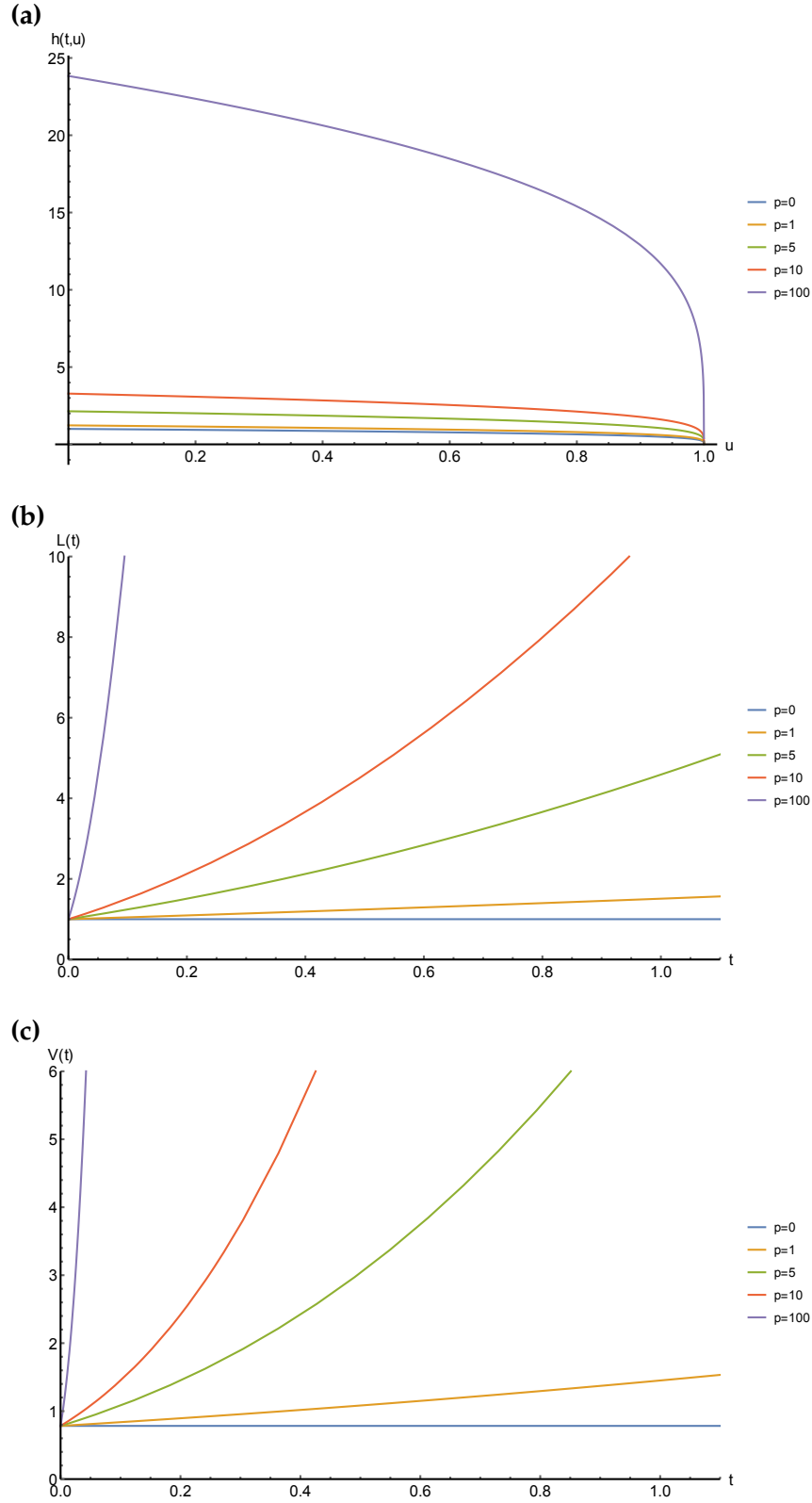
Figure 4.7: Graphs illustrating (a) the fracture half-width, (b) the fracture length and (c) the fracture volume, for \alpha = 2 , at a fixed value of t = 1 , where p = \frac{2K}{5l_0} varies, taking on the values p = 0, 1, 5, 10 and 100 .
