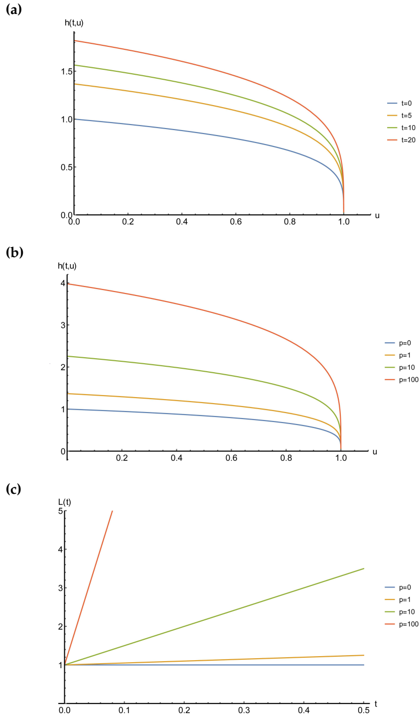
Figure 4.13: Graphs illustrating (a) the fracture half-width for different t for p = \frac{2K}{5l_0} = 1 , (b) the fracture half-width for different values of p = \frac{2K}{5l_0} at t = 1 and (c) the fracture length for varying p = \frac{2K}{5l_0} , where \alpha = 1 , corresponding to a constant speed of propagation of the fracture.
