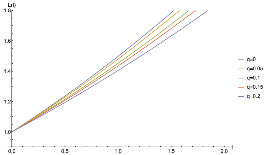
Figure 5.2: The fracture length, L(t) plotted against time t for p = 1 and q = 0, 0.05, 0.1, 0.15 and 0.2 .
