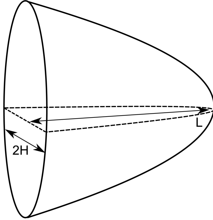
Figure 2.1: A simplified diagram of the PKN fracture model, adapted from [37].
