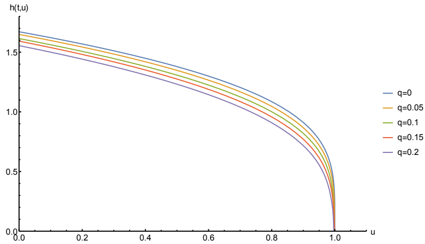
Figure 5.1: The fracture half-width, h(t, u) plotted against u at t = 3 for p = 1 and q = 0, 0.01, 0.05, 0.1, 0.15 and 0.2 .
