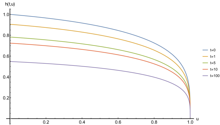
Figure 4.4: A graph showing the fracture half-width for \alpha = 0.5 , at a fixed value of p = \frac{2K}{5l_0} = 1 , where t varies, taking on the values t = 0, 1, 5, 10 and 100 .
