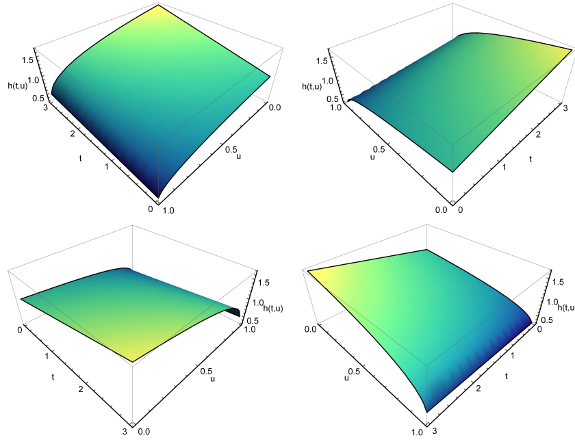
Figure 4.10: Graphs illustrating the fracture half-width varying across t and u for \alpha = 2 , at different view points. Here, the parameter \frac{2K}{5l_0} = 1 .
