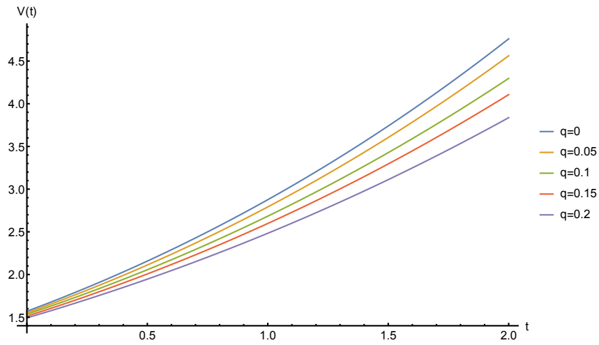
Figure 5.3: The fracture volume, V(t) plotted against time t for p = 1 and q = 0, 0.05, 0.1, 0.15 and 0.2 .
