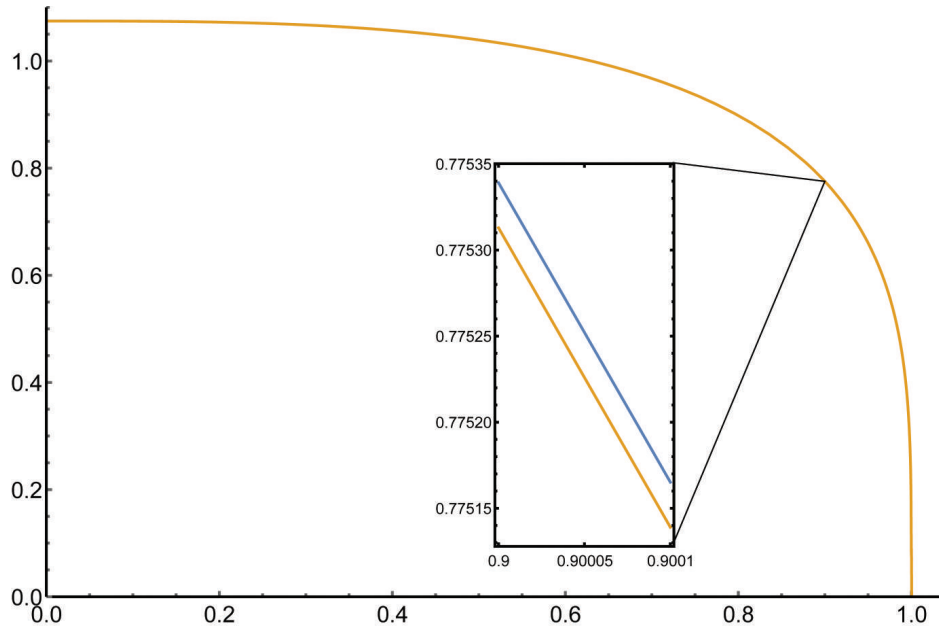
Figure 4.1: A graph illustrating the exact analytic solution for \alpha = \frac{2}{7} (orange) and numerical solution (blue) on the same set of axes. The box within the graph is a zoomed up portion of the graph from u = 0.9 to u = 0.9001 , to allow for closer inspection of the difference between the two graphs.
