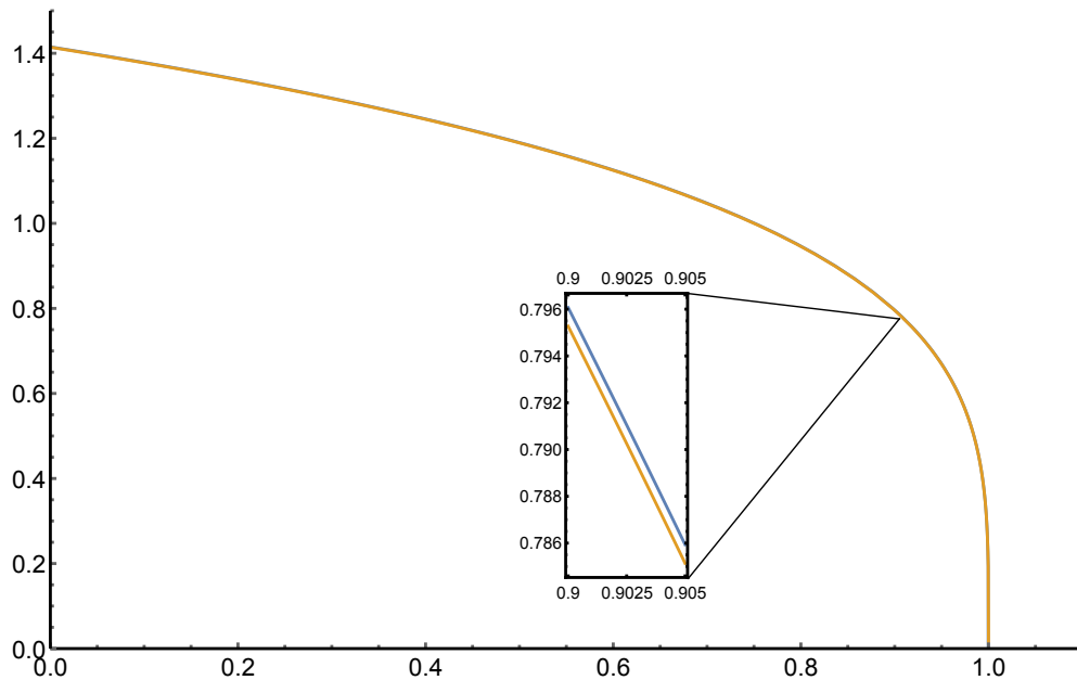
Figure 4.2: A graph illustrating the exact analytic solution for \alpha = 1 (orange) and numerical solution (blue) on the same set of axes. The box within the graph is a zoomed up portion of the graph from u = 0.9 to u = 0.905 .
