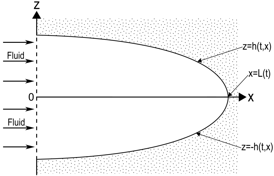
Figure 3.1: A simplified diagram of the two-dimensional fracture being modelled. The fracture is within a rock mass and it is of length L(t) with boundaries z = \pm h(t, x) . A viscous, incompressible fluid is injected at high pressures into the fracture at x = 0 , and the flow of this fluid within the fracture is turbulent. The fracture expands due to the high pressure fluid causing the rock to fail.
