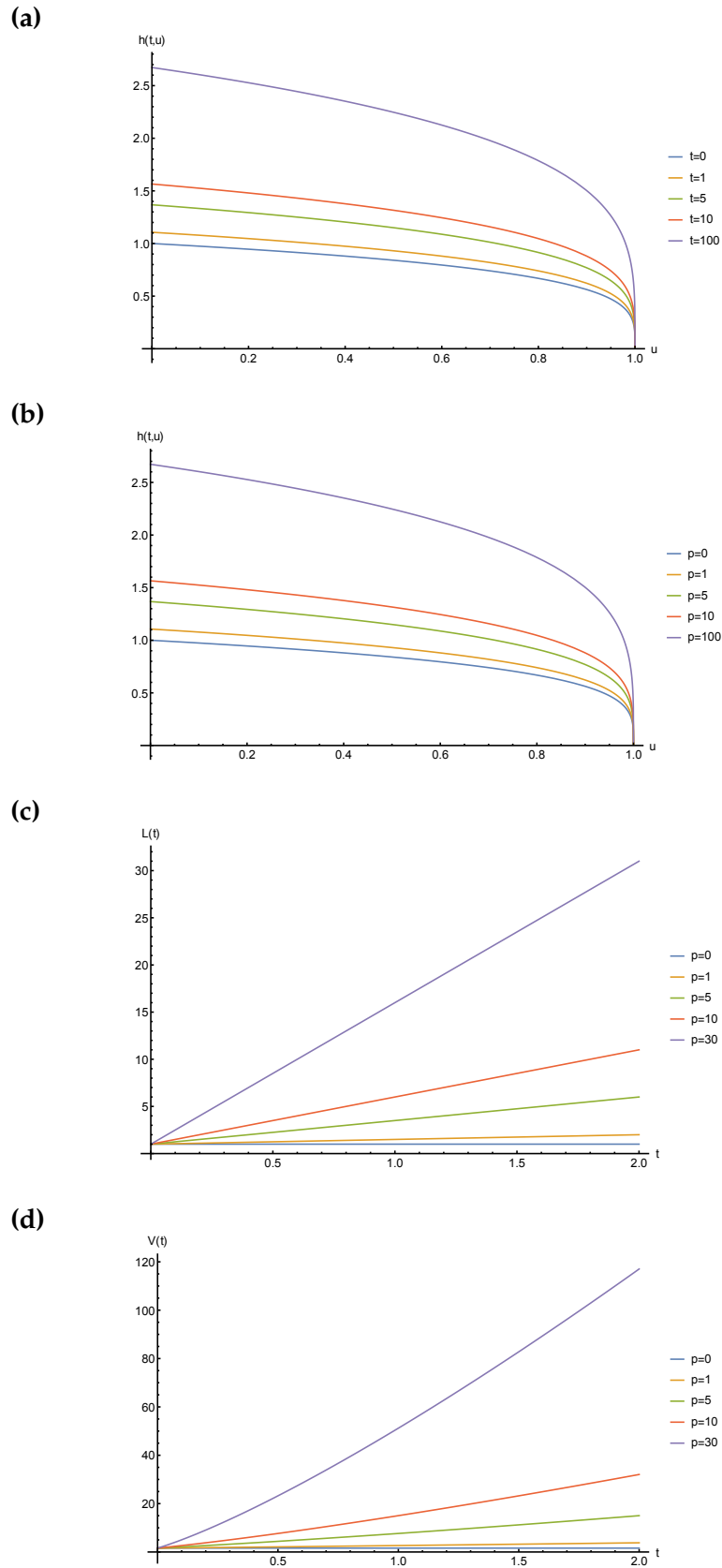
Figure 4.22: Graphs illustrating the non-classical symmetry solution for (a) the fracture profile for p = \frac{2K}{5l_0} = 1 , (b) the fracture profile for t = 1 , (c) the fracture length and (d) the fracture volume.
