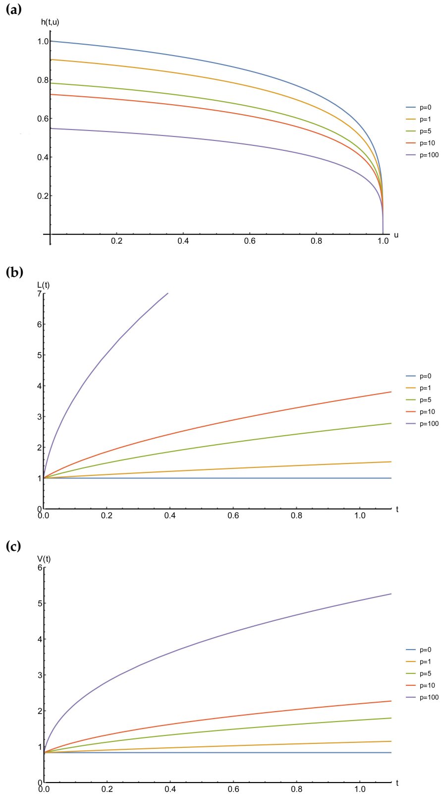
Figure 4.6: Graphs illustrating (a) the fracture half-width, (b) the fracture length and (c) the fracture volume, for \alpha = 0.5 , at a fixed value of t = 1 , where p = \frac{2K}{5l_0} varies, taking on the values p = 0, 1, 5, 10 , and 100 .
