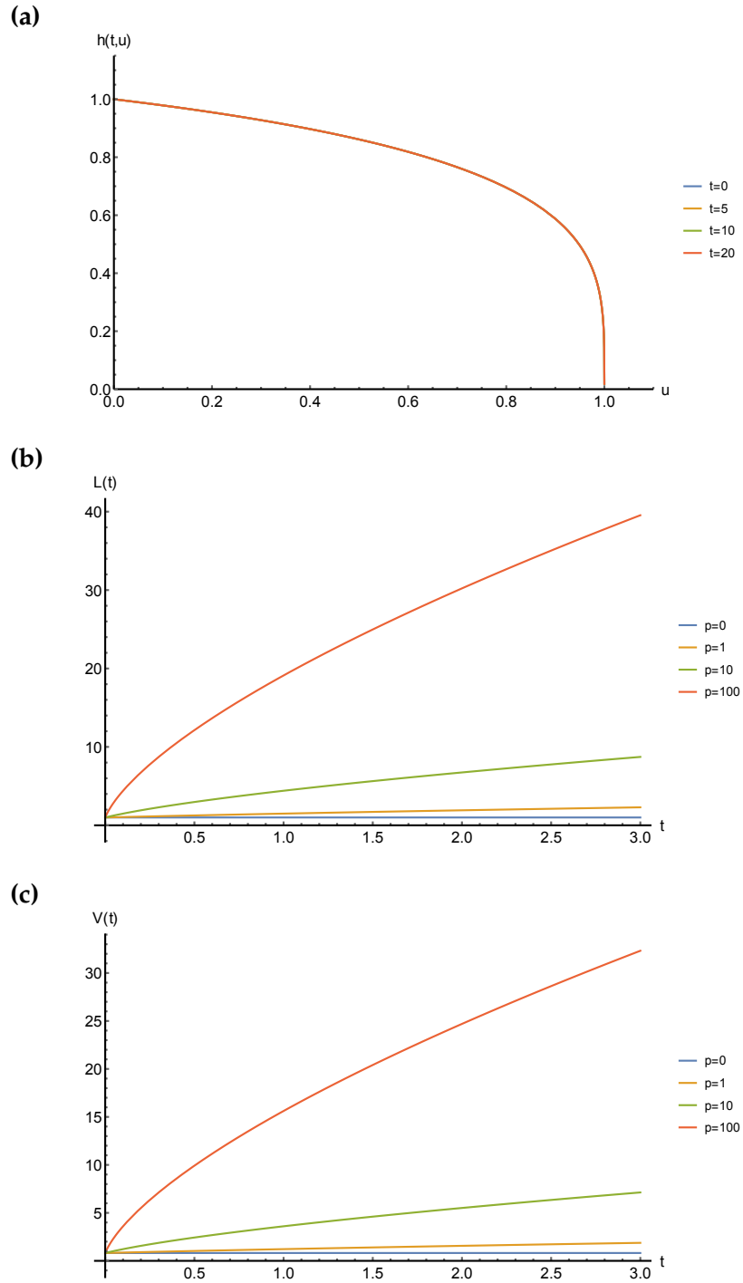
Figure 4.14: Graphs illustrating (a) the fracture half-width for different t at p = \frac{2K}{5l_0} = 1 , (b) the fracture length for different p = \frac{2K}{5l_0} and (c) the fracture volume for varying p = \frac{2K}{5l_0} , where \alpha = \frac{2}{3} , corresponding to a constant pressure at the fracture entry.
