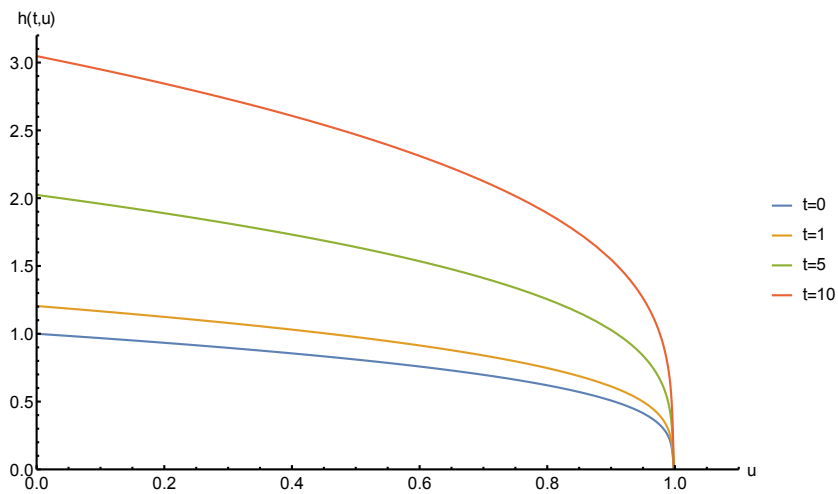
Figure 5.4: The fracture half-width h(t, u) plotted against u for p = 1 , q = 0.1 and t = 0, 1, 5 and 10 .
