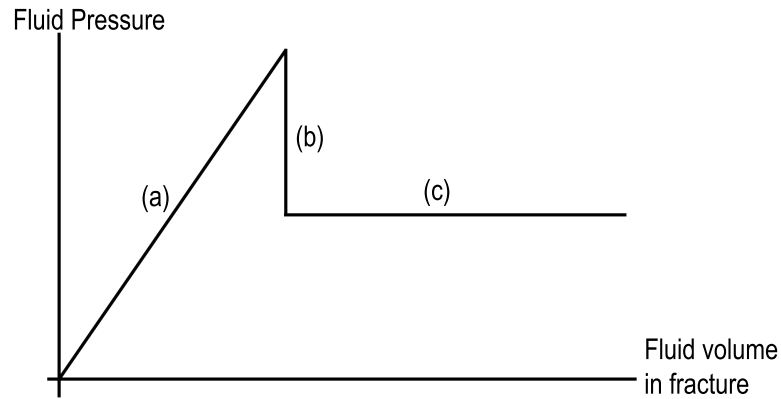
Figure 1.1: A graph showing the simplified behaviour of the relationship between fluid pressure and fluid volume in a fracture during hydraulic fracturing, adapted from [18]. (a) Initially, the fracture is filled with the fluid at great pressures. (b) Once the fracture is filled, if the fluid pressure is great enough to overcome the rock's tensile strength and the least principal stress component, (c) then the fracture will extend spontaneously, making the fluid pressure approximately constant after this point, while the volume of fluid in the cavity increases.
