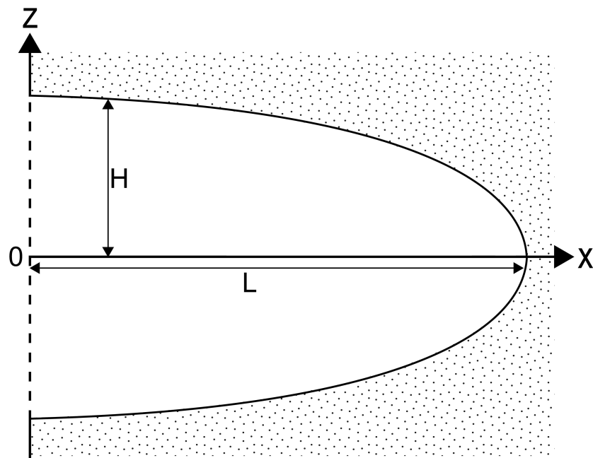
Figure 3.2: A simple diagram of the two-dimensional fracture at t = 0 illustrating the characteristic lengths L and H within the hydraulic fracture problem, whereby H \ll L .
