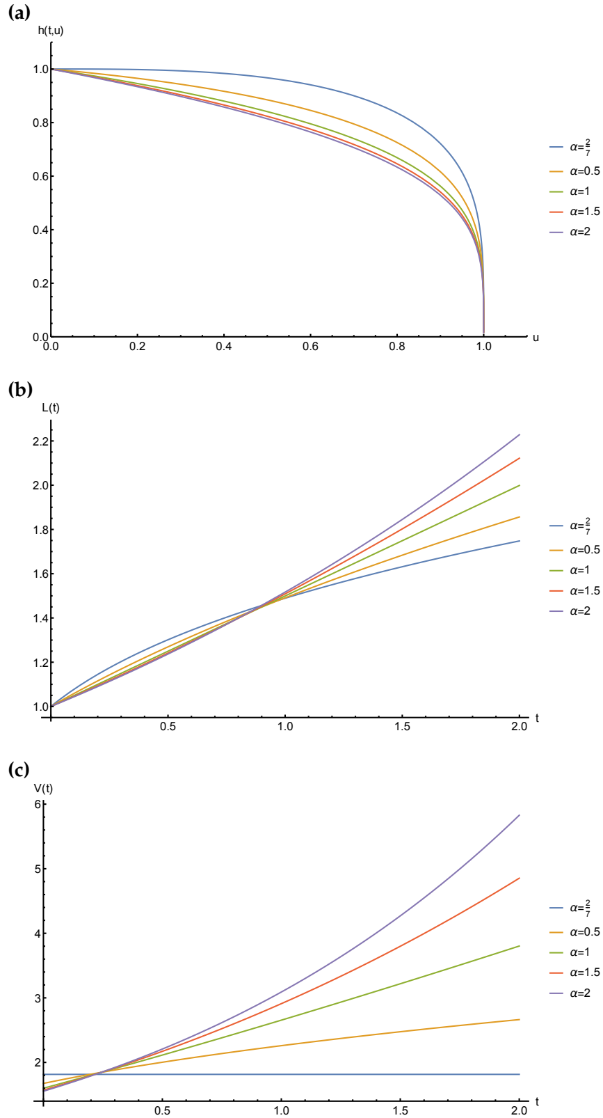
Figure 4.3: Graphs illustrating the effect of the parameter \alpha on (a) the initial fracture profile, (b) the fracture length and (c) the fracture volume. Here, the parameters \frac{2K}{5l_0} = 1 and \alpha takes on the values \frac{2}{7} , 0.5, 1, 1.5 and 2.
