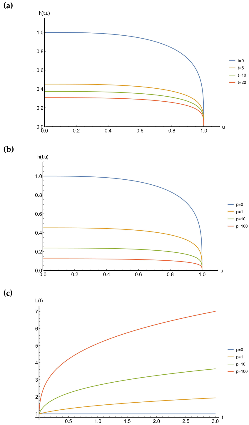
Figure 4.11: Graphs illustrating (a) the fracture half-width for different t at a fixed p = \frac{2K}{5l_0} = 1 , (b) the fracture half-width for varying p = \frac{2K}{5l_0} at t = 1 and (c) the fracture length for different p = \frac{2K}{5l_0} , where \alpha = \frac{2}{7} , corresponding to a constant fracture volume.
