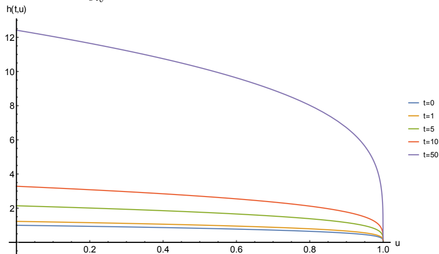
Figure 4.5: A graph showing the fracture half-width for \alpha = 2 , at a fixed value of p = \frac{2K}{5l_0} = 1 , where t varies, taking on the values t = 0, 1, 5, 10 and 50 .
