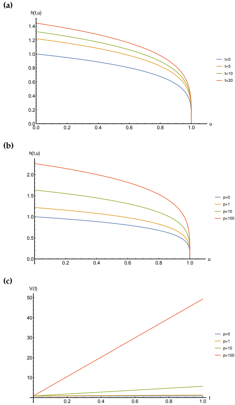
Figure 4.12: Graphs illustrating (a) the fracture half-width for different t at p = \frac{2K}{5l_0} = 1 , (b) the fracture half-width for different p = \frac{2K}{5l_0} at t = 1 and (c) the fracture volume for varying p = \frac{2K}{5l_0} , where \alpha = 0.857143 , corresponding to a constant rate of change of volume.
