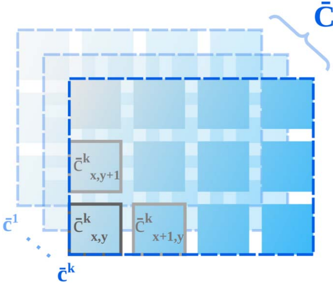
Figure 1. Visual representation of the coefficient matrix \tilde{C} . Each image layer \tilde{C}^k represents the coefficient weights for a basis term k , (\{\tilde{C}\}_k) organized by 2D sensor cell position. The mapping of light curve i to cell position i \rightarrow (x, y) is implicit in this notation, as described in the main text.
