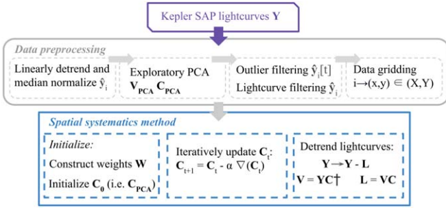
Figure 2. Data analysis framework for numerical evaluation of the spatial systematics algorithm. The data flow includes input data (purple box), preprocessing (gray box; Section 2.5.1), and application of the spatial systematics algorithm (blue box; Sections 2.4 and 2.5).
