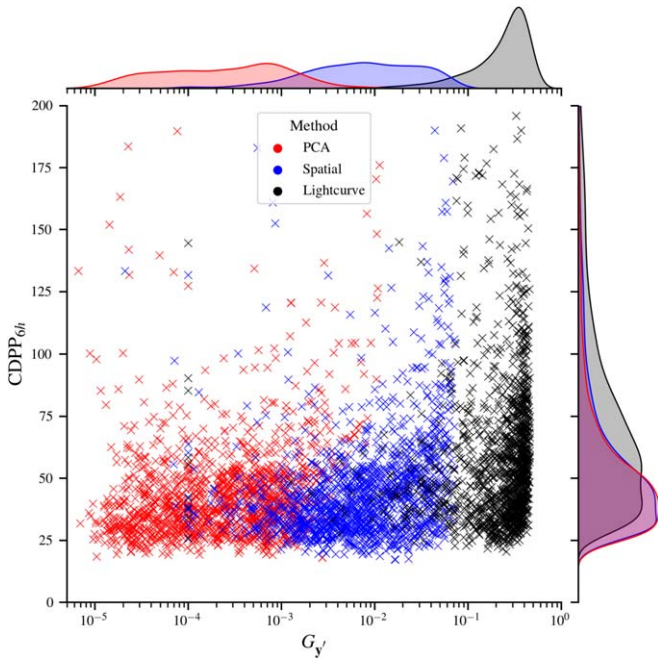
Figure 19. \text{CDPP}_{6h} vs. goodness metric G_{y'} per target light curve for a single run #0 of Experiment A. Three light-curve types are shown, including nondetrended preprocessed light curves (black), light curves detrended using PCA (red), and light curves detrended using the spatial systematics algorithm (blue). Empirical distribution functions for each light-curve type are plotted over G_{y'} (top) and \text{CDPP}_{6h} (right).
