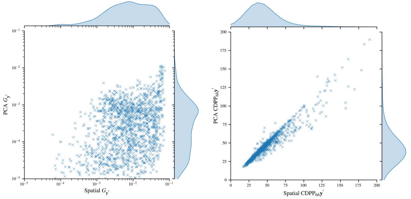
Figure 20. Metrics G_{y'} (left) and \text{CDPP}_{6h} (right) for the reference PCA method vs. the spatial systematics method. Both plots are per target light curve for a single run #0 of Experiment A. Empirical distribution functions for each light-curve metric are plotted over the spatial systematics method (horizontal axis) and the PCA method (vertical axis). Although correlated, there is significant scatter in the left plot due to the intrinsic nonlinear and pairwise nature of the metric G_{y'} . It is accordingly more sensitive to light curves with poorly modeled systematics or greater retained astrophysical variability.
