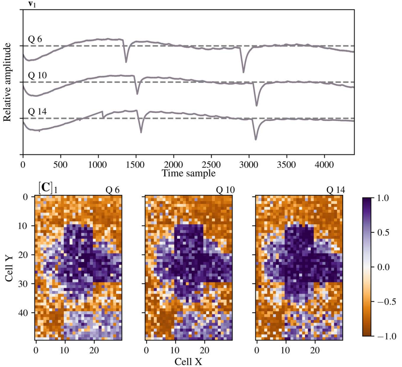
Figure 6. Leading PCA basis vector v_1 for quarters Q6, Q10, and Q14 (top) and an associated color map of the leading PCA coefficient c_{i-(x,y)}^1 at each spatial cell position (bottom). The spatial structure of the leading coefficient term is persistent between quarters.
