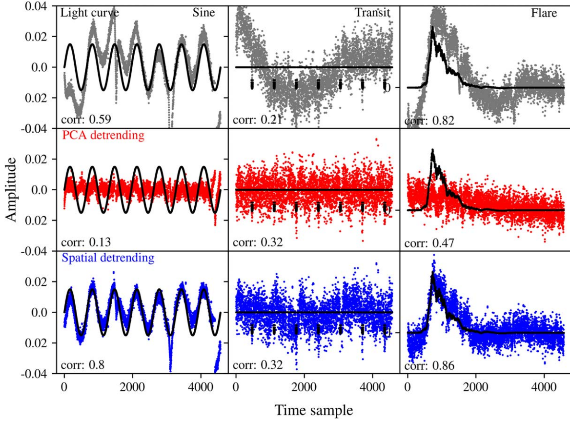
Figure 12. Three sample light curves across injected signal type a_{[m]} m \in \{s, t, f\} (sine, transit, and flare) from run #0, a representative run of Experiment A. The figure shows the preprocessed light curve before detrending y (upper row), the detrended light curve using PCA y'_{\text{PCA}} (middle row), and the detrended light curve using the spatial systematics algorithm y' (lower row). Simulated injected signals are overlaid in black. The x -axis is Kepler's long-cadence time sample index. This sample shows an instance where PCA detrending removed the injected astrophysical sine and flare signals, while spatial detrending preserved those signals.
