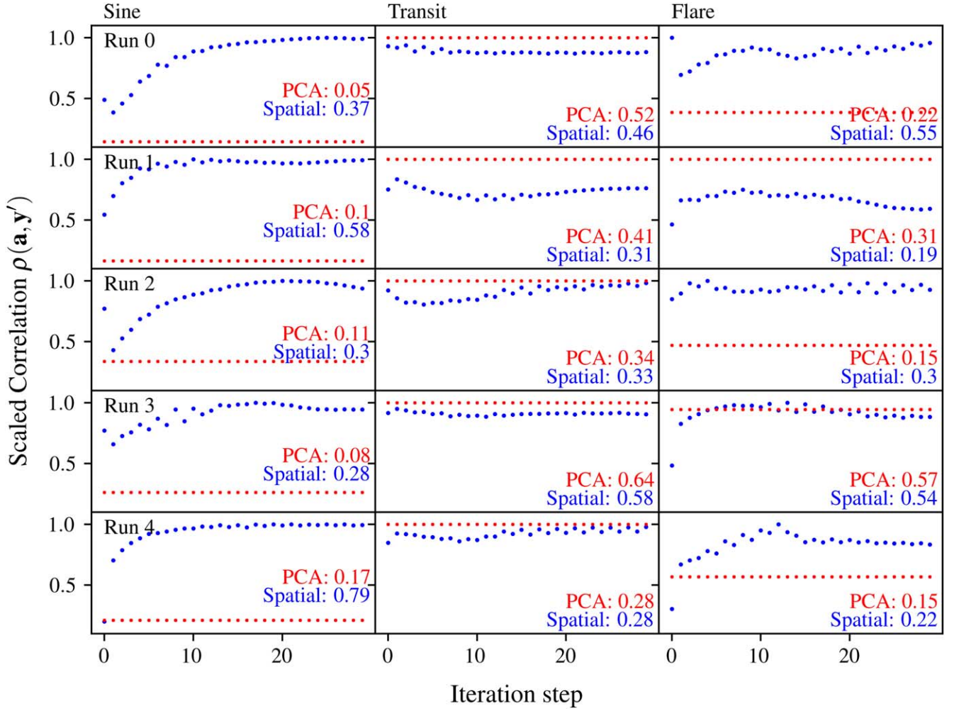
Figure 9. Scaled mean correlation of injected signals and associated detrended light curves \bar{\rho}(\mathbf{a}_{[m]}, \mathbf{y}'_{[m]}) for Experiment A for sine, flare, and transit signal types m \in \{s, t, f\} (across columns) for each of five separate simulation runs (across rows). This mean correlation, defined in the main text, is plotted for the spatial systematics algorithm (blue) and the PCA decomposition method (red). The mean correlation is scaled by the maximum value achieved by either method; this maximum is shown in the legend of each subplot. The PCA algorithm is noniterative and is depicted as a straight line accordingly. The x-axis label is the iteration number of the spatial systematics algorithm. The spatial systematics algorithm is generally convergent and typically has comparable or improved performance relative to PCA but this is not universal for all runs.
