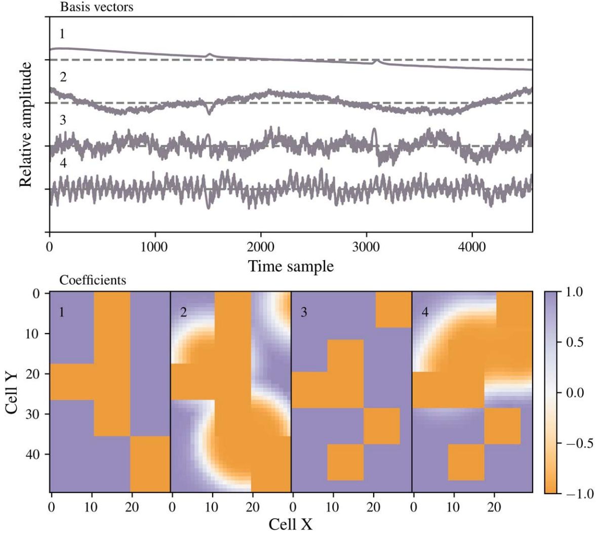
Figure 8. Basis vectors \mathbf{V} (upper) and coefficients \mathbf{C} (lower) used for the full simulation of light curves in experiment B using a rank K = 4 model. The basis vectors were selected at approximately equal spacing as index sets (1, 5, 11, 16) from the 16 Kepler CBV published for Q10 and channel 30 (Stumpe et al. 2012). The coefficient spatial dependence was simulated as a mixture of random smooth features and sharp discontinuities. Both components are arbitrarily chosen and the discontinuities are not constrained to match the Kepler module gridding.
