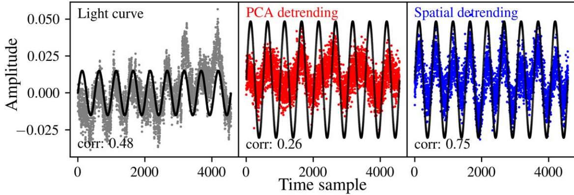
Figure 18. Simulated light curve y before detrending (left), the detrended light curve using PCA y'_{\text{PCA}} (middle), and the detrended light curve using the spatial systematics algorithm y' (right), all at the position of the maximum value of [C_{\text{PCA}}]_5 in Figure 17. Simulated injected signals are overlaid in black. The x -axis is Kepler's long-cadence time sample index. This shows an instance where PCA detrending overfits the injected astrophysical sine signal relative to the spatial systematics algorithm.
