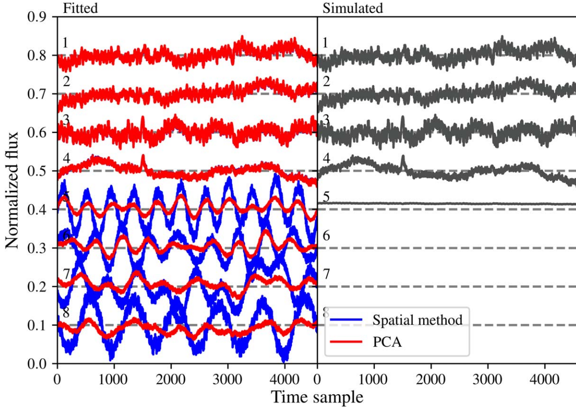
Figure 13. Estimated (left) and known simulated (right) basis vectors \mathbf{v}_k , k \in \{1, \dots, 8\} for Experiment B. The estimated basis vectors (left) are shown for the spatial systematics algorithm (blue) and the reference PCA method (red). The x -axis is in units of Kepler long-cadence time sample. The estimated spatial and PCA basis vectors (left) for the first four terms overlap one another in these plots.
