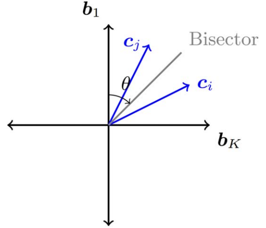
Figure 23. Bisector at angle \theta between coefficient vectors c_i and c_j in the 2D space spanned by basis vectors b_1 and b_K .
