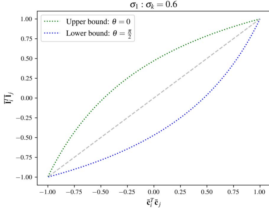
Figure 24. Deviation of the systematics correlation \bar{l}_i^T \bar{l}_j , upper bound (green) and lower bound (blue), from the coefficient correlation \bar{c}_i^T \bar{c}_j (gray) for \sigma_1 : \sigma_K = 0.6 .
