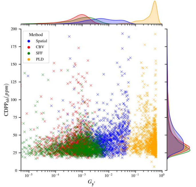
Figure 16. CDPP 6h (ppm) vs. goodness metric G_{y'} per target light curve shown for the spatial systematics method and comparison standard detrending methods CBV, SFF, and PLD. Empirical distribution functions for each light-curve type are plotted over G_{y'} (top) and CDPP 6h (right). The CDPP 6h metric is broadly comparable across methods while the G_{y'} metric is more strongly dependent on the detrending method.
