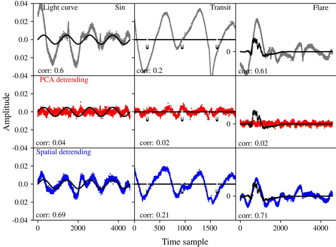
Figure 21. Noninjected light curves y_{a^c} for which the spatial systematics algorithm produces the highest incidental correlation \max_{y_{a^c}} \rho(a_{[m]}, y_{a^c}) , m \in \{s, t, f\} between the nondetrended light curve y_{a^c} and any injected astrophysical signal a_{[m]} used in the simulation run. The top row shows the nondetrended light curve and the astrophysical signal (injected into another light curve) with which the incidental correlation is highest. The detrended light curves y'_{a^c} are shown as obtained by the reference PCA method (middle row) and the spatial systematics algorithm (bottom row). Simulated injected signals are overlaid in black. In these worst cases, it can be seen that the high level of correlation of the spatial detrended light curve y' with an astrophysical signal a is incidental, as the original light curve y itself is incidentally correlated with a . This suggests that high values for the metric of corruption |\bar{\rho}(a, y'_{a^c})|/|\bar{\rho}(a, y_{a^c})| may result incidentally for the spatial systematics algorithm because it retains a higher level of astrophysical variability.
