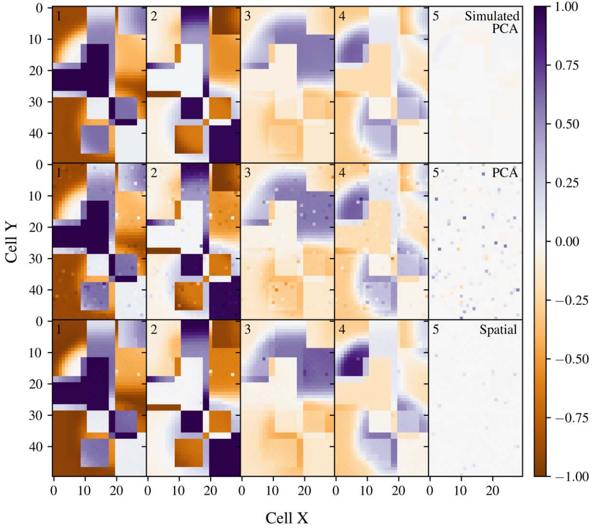
Figure 14. Coefficients c_i^k , k \in \{1, \dots, 5\} ( K = 8 ) for light curve i \rightarrow (x, y) \in (X, Y) for Experiment B. This figure shows the true simulated coefficients (top row), the coefficients obtained using the PCA method (middle row), and the coefficients obtained using the spatial systematics algorithm (bottom row). The coefficient index k is shown in the top left of each subfigure. The x - and y -axes are in units of gridded spatial cells. Coefficients fitted with PCA show speckling, indicative of the overfitting of injected astrophysical signals.
