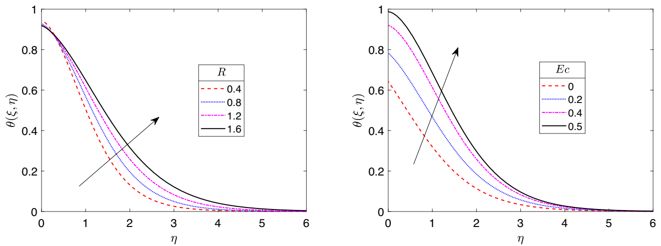
Fig. 11 Impact of R and Ec on temperature profiles
