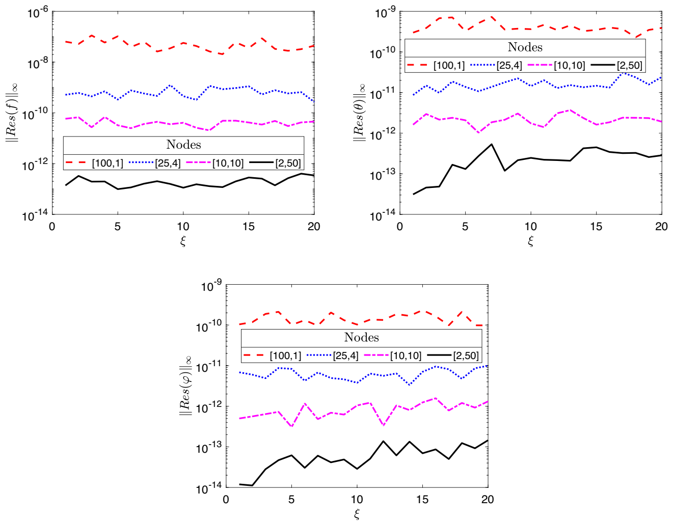
Fig. 5 Residual error graphs for different values of N and q
