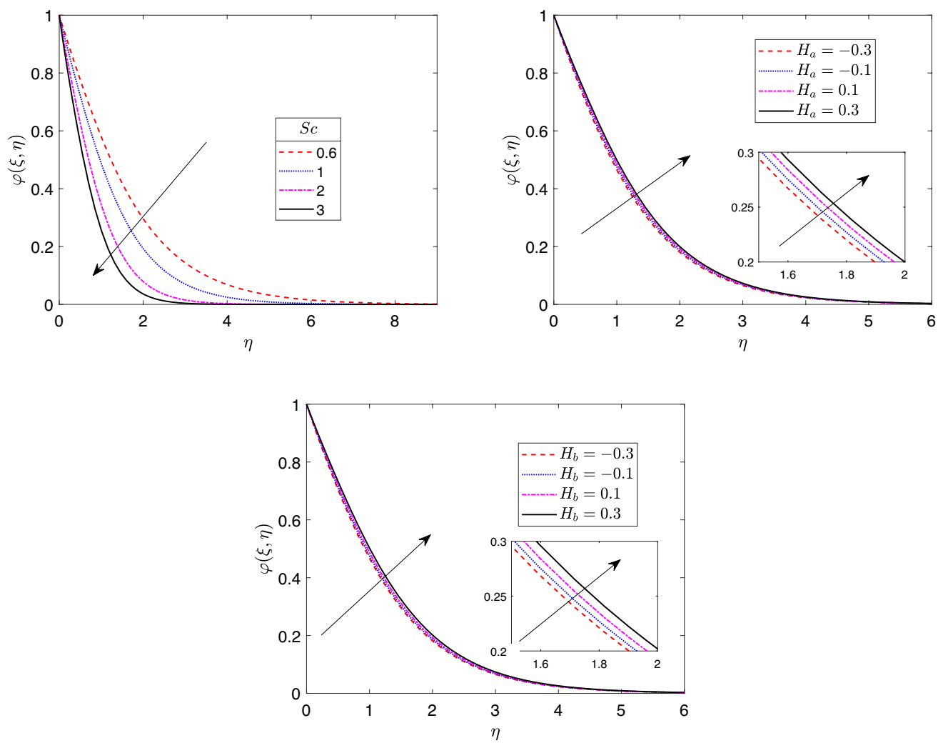
Fig. 14 Impact of Sc , H_a and H_b on concentration profiles
