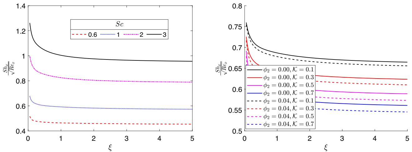
Fig. 23 Impact of Sc and K on mass transfer rate
