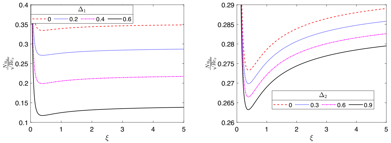
Fig. 20 Impact of \Delta_1 and \Delta_2 on heat transfer rate
