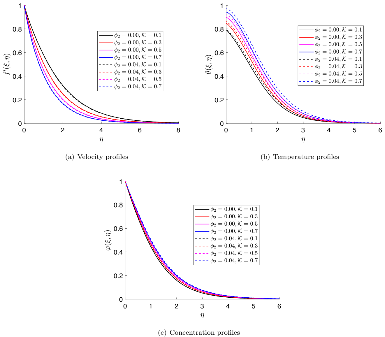
Fig. 6 Impact of \phi_2 and \mathcal{K} on the flow profiles
