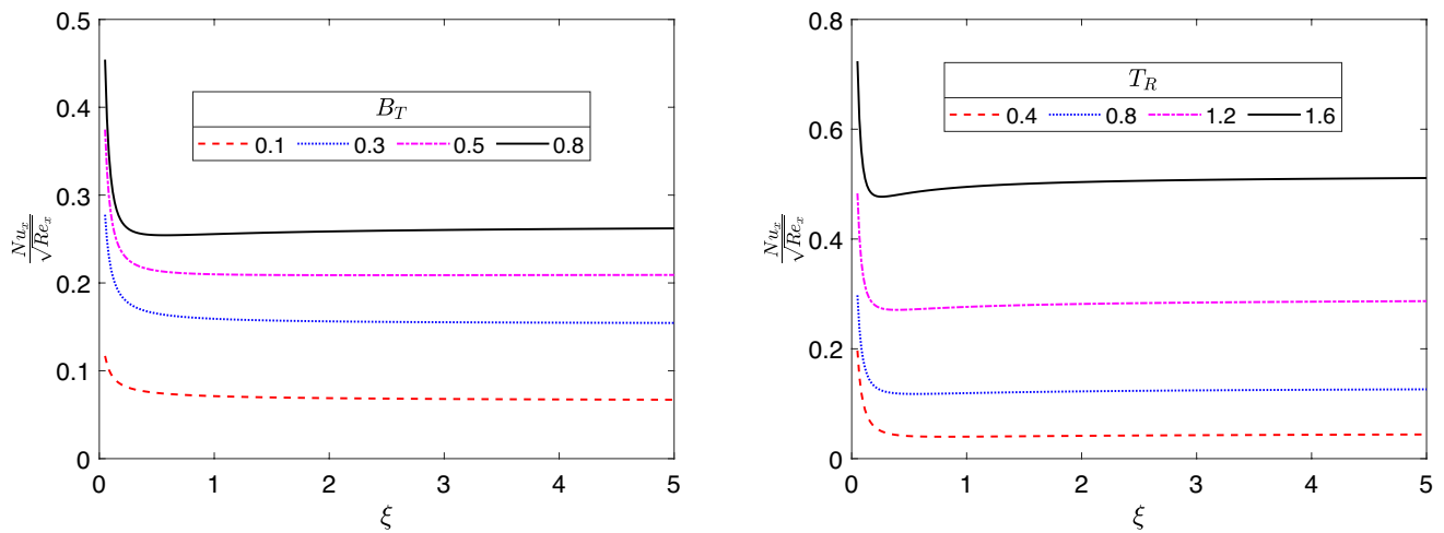
Fig. 22 Impact of B_T and T_R on heat transfer rate
