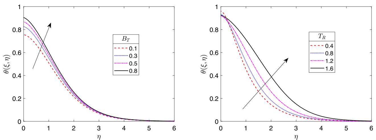
Fig. 13 Impact of B_T and T_R on temperature profiles
