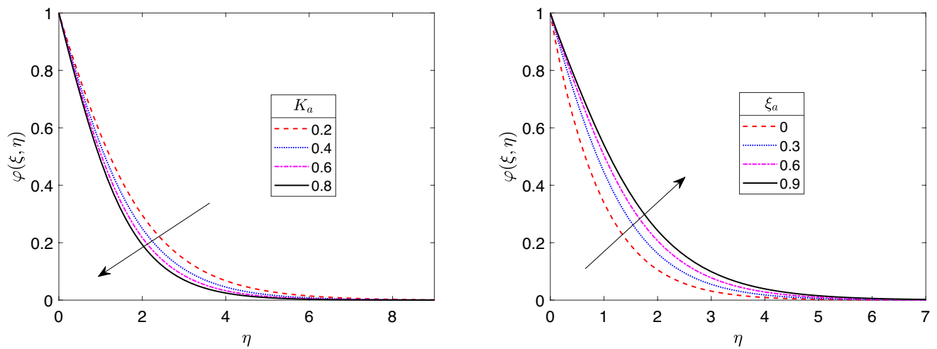
Fig. 15 Impact of K_a and \xi_a on concentration profiles
