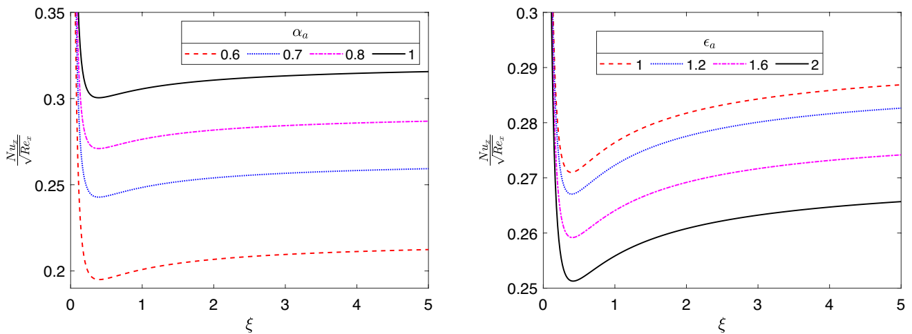
Fig. 19 Impact of \alpha_a and \epsilon_a on heat transfer rate
