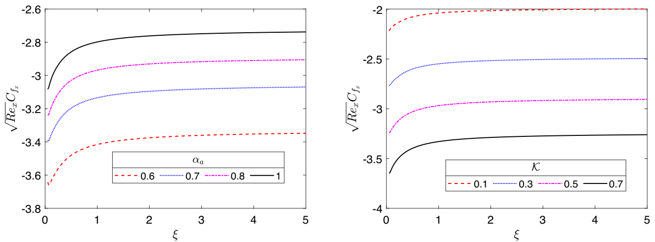
Fig. 18 Impact of \alpha_a and \mathcal{K} on skin friction coefficient profiles
