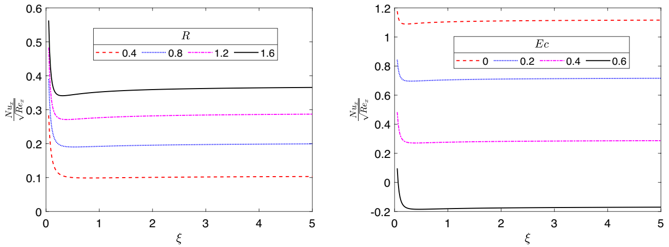
Fig. 21 Impact of R and Ec on heat transfer rate
