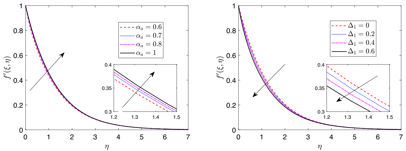
Fig. 8 Impact of \alpha_a and \Delta_1 on velocity profiles
