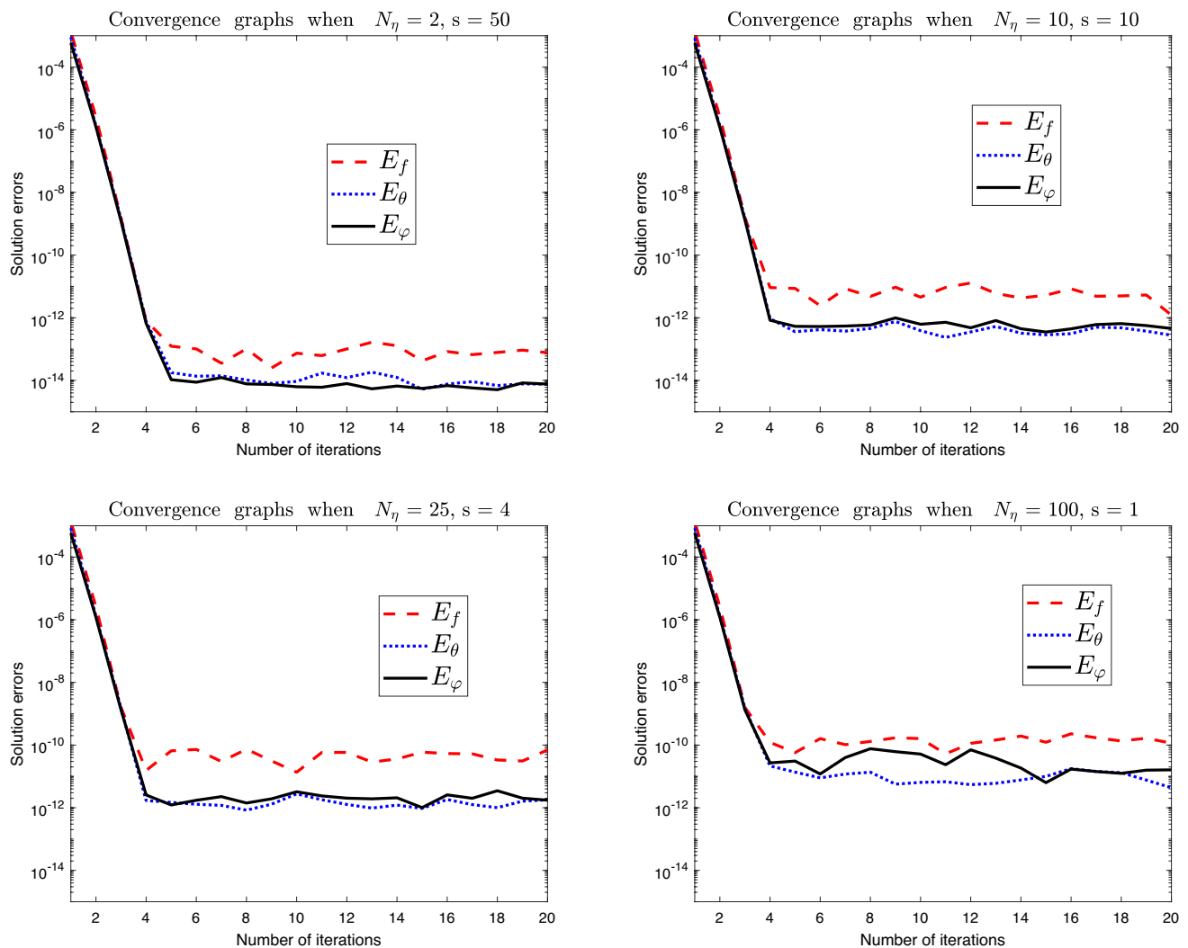
Fig. 4 Convergence graphs for different values of N_\eta and s
