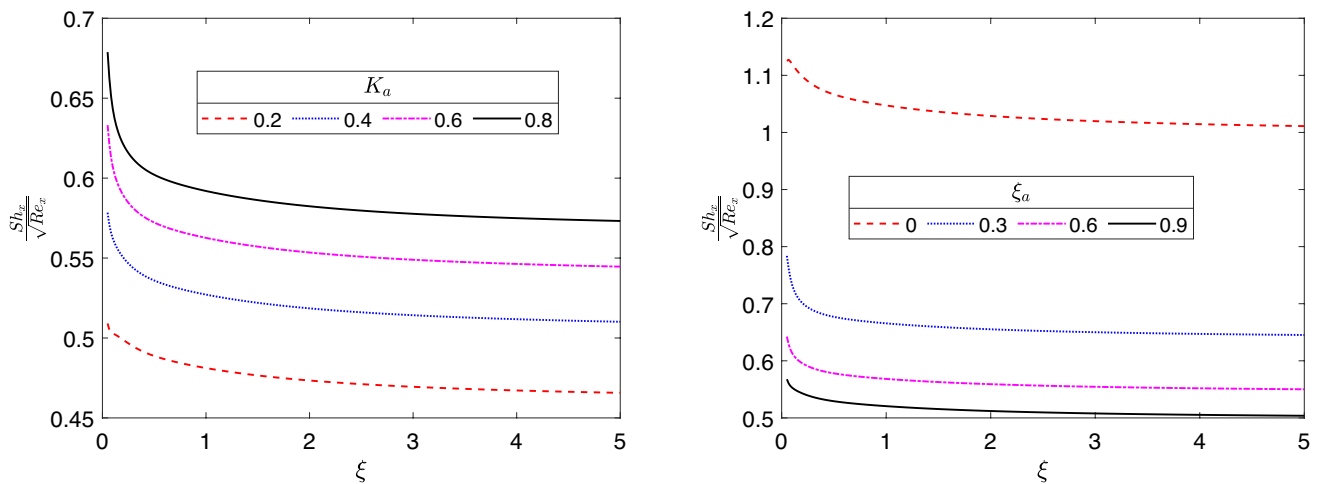
Fig. 24 Impact of K_a and \xi_a on mass transfer rate
