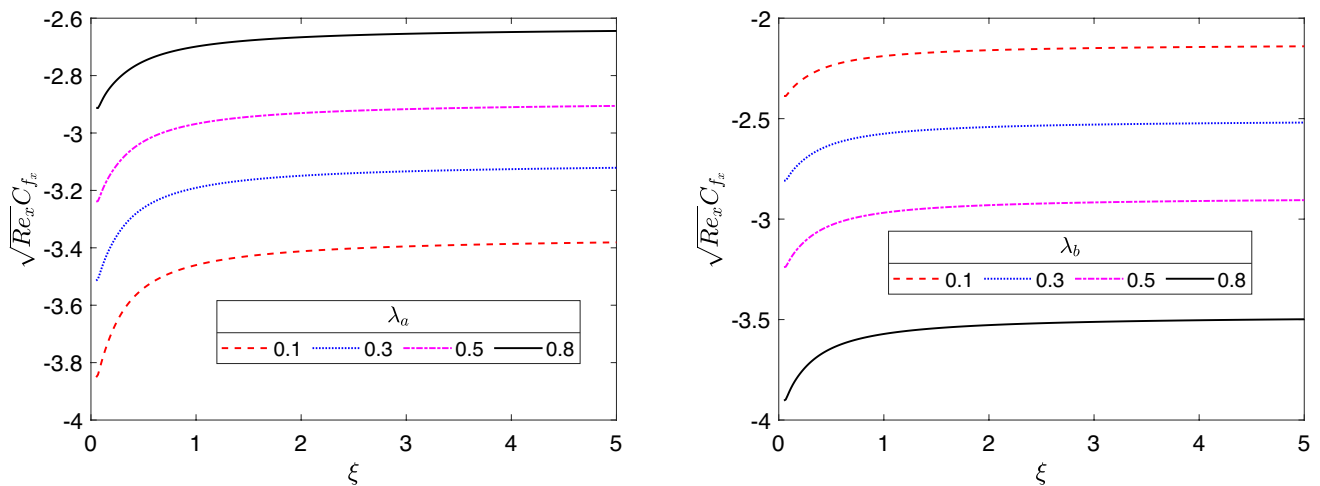
Fig. 17 Impact of \lambda_a and \lambda_b on skin friction coefficient profiles
