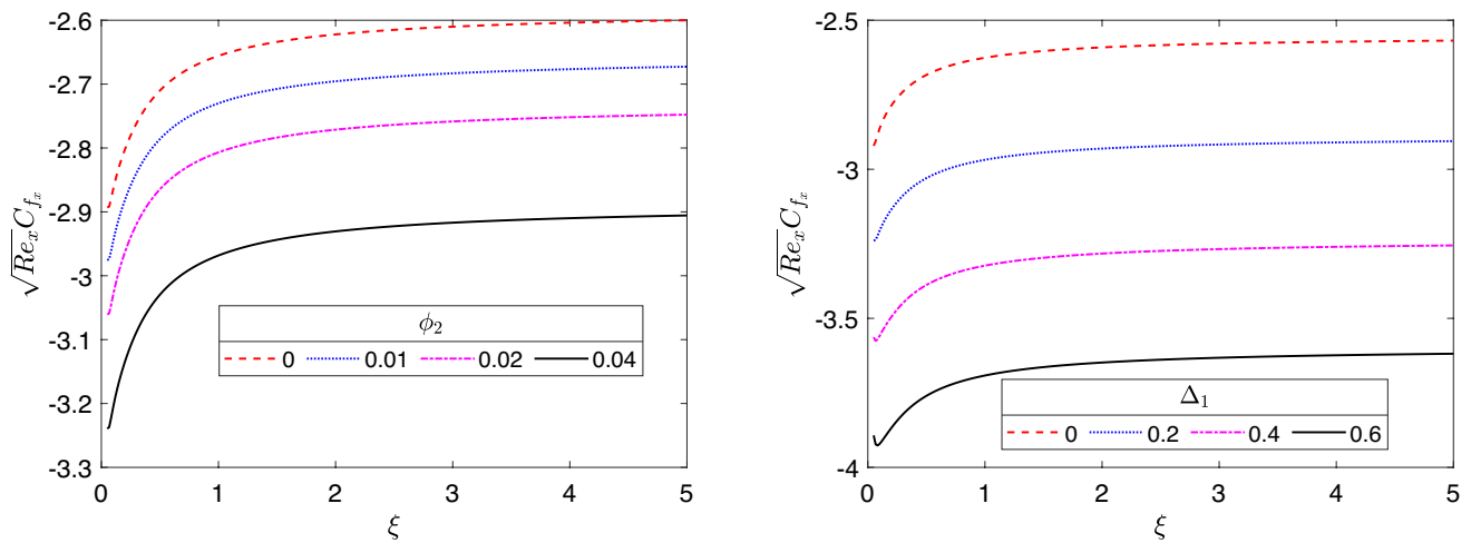
Fig. 16 Impact of \phi_2 , \mathcal{K} and \Delta_1 on skin friction coefficient
