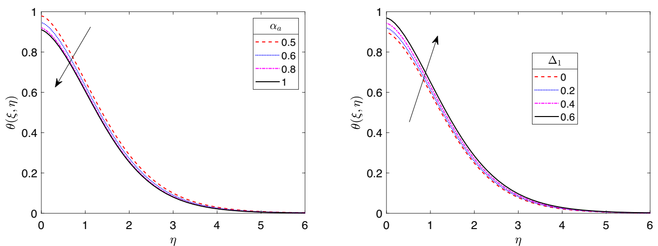
Fig. 10 Impact of \alpha_a and \Delta_1 on temperature profiles
