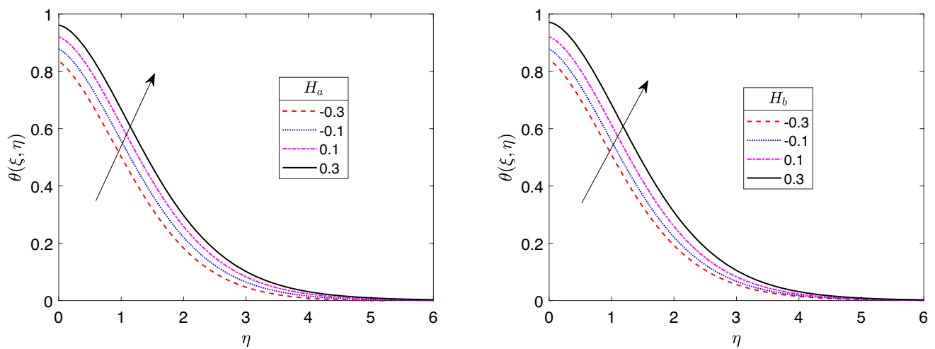
Fig. 12 Impact of H_a and H_b on temperature profiles
