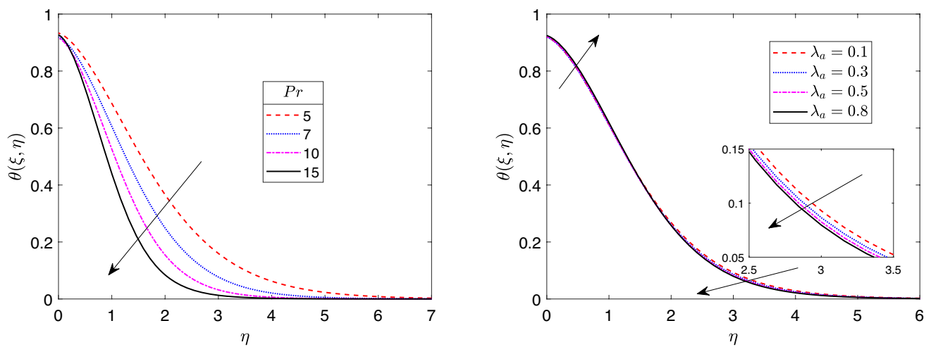
Fig. 9 Impact of Pr and \lambda_a on temperature profiles
