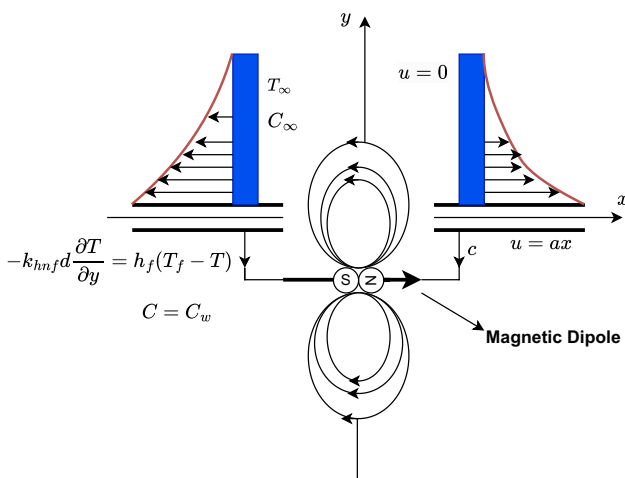
Fig. 1 Geometrical configuration of the flow
