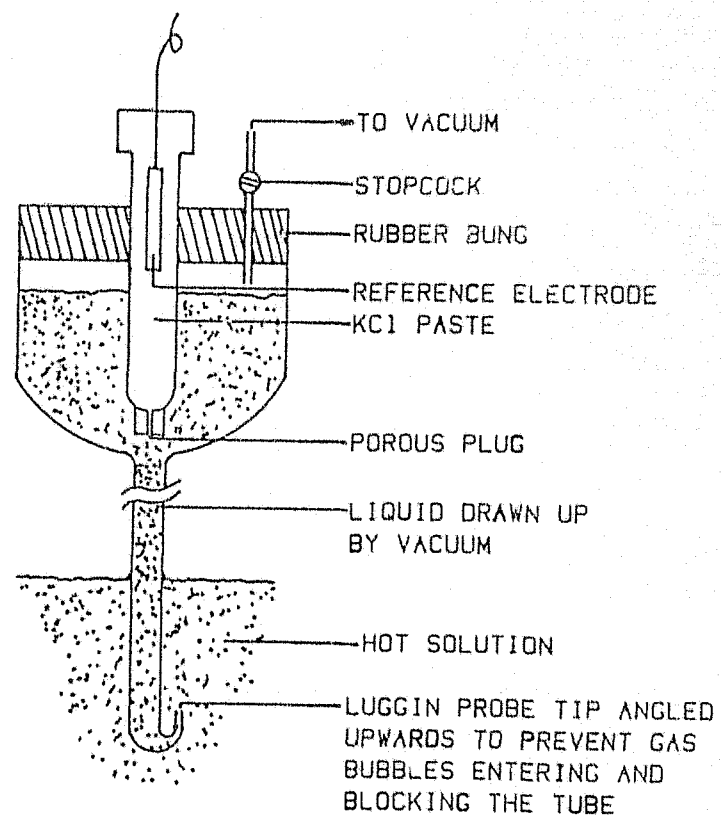
LUGGIN PROBE AND REFERENCE ELECTRODE
