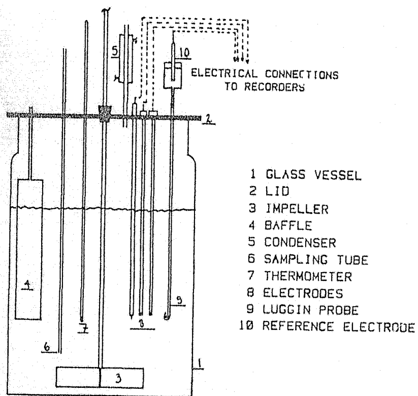
DIAGRAM OF THE LEACH REACTOR
