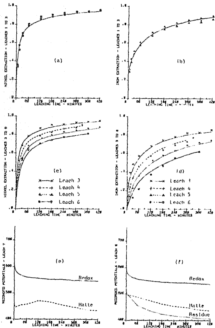
Fig. 3.1 Typical experimental results
