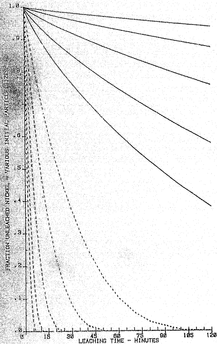
Fig. 5.2 Calculated fraction Ni in unleached particles
