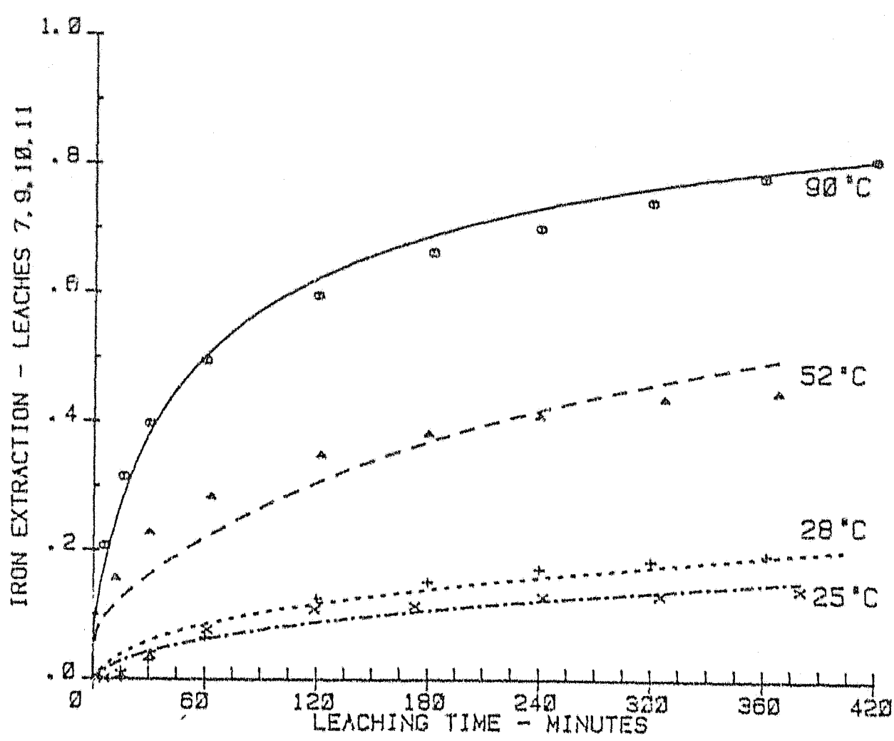
Fig. 3.4 Effect of temperature on leaching rates
