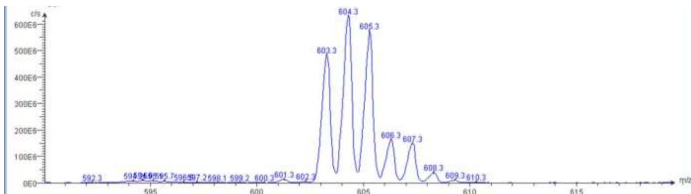
Mass Spectroscopy spectrum of [Pt(dmp)(L^3-O,S)]Cl .
