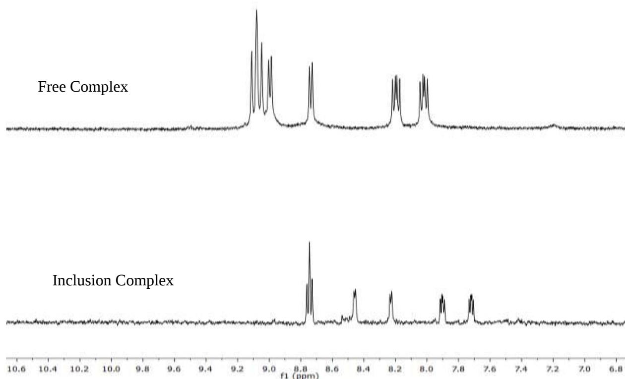
Figure 4.2: (a) The full spectrum ^1\text{H} NMR of the free complex (top) and inclusion complex (bottom). (b) Aromatic region of the free and inclusion complex.
