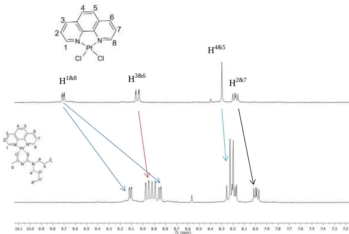
Figure 2.7: The aromatic region ^1\text{H} NMR of [\text{Pt}(\text{phen})(\text{L}^3\text{-O,S})]\text{Cl} and the precursor [\text{PtCl}_2(\text{phen})] showing the loss of symmetry upon coordination of \text{HL}^3 .
