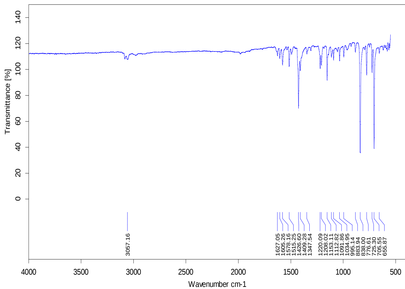
FTIR Spectroscopy spectrum of [PtCl 2 (1,10-phenanthroline)].
