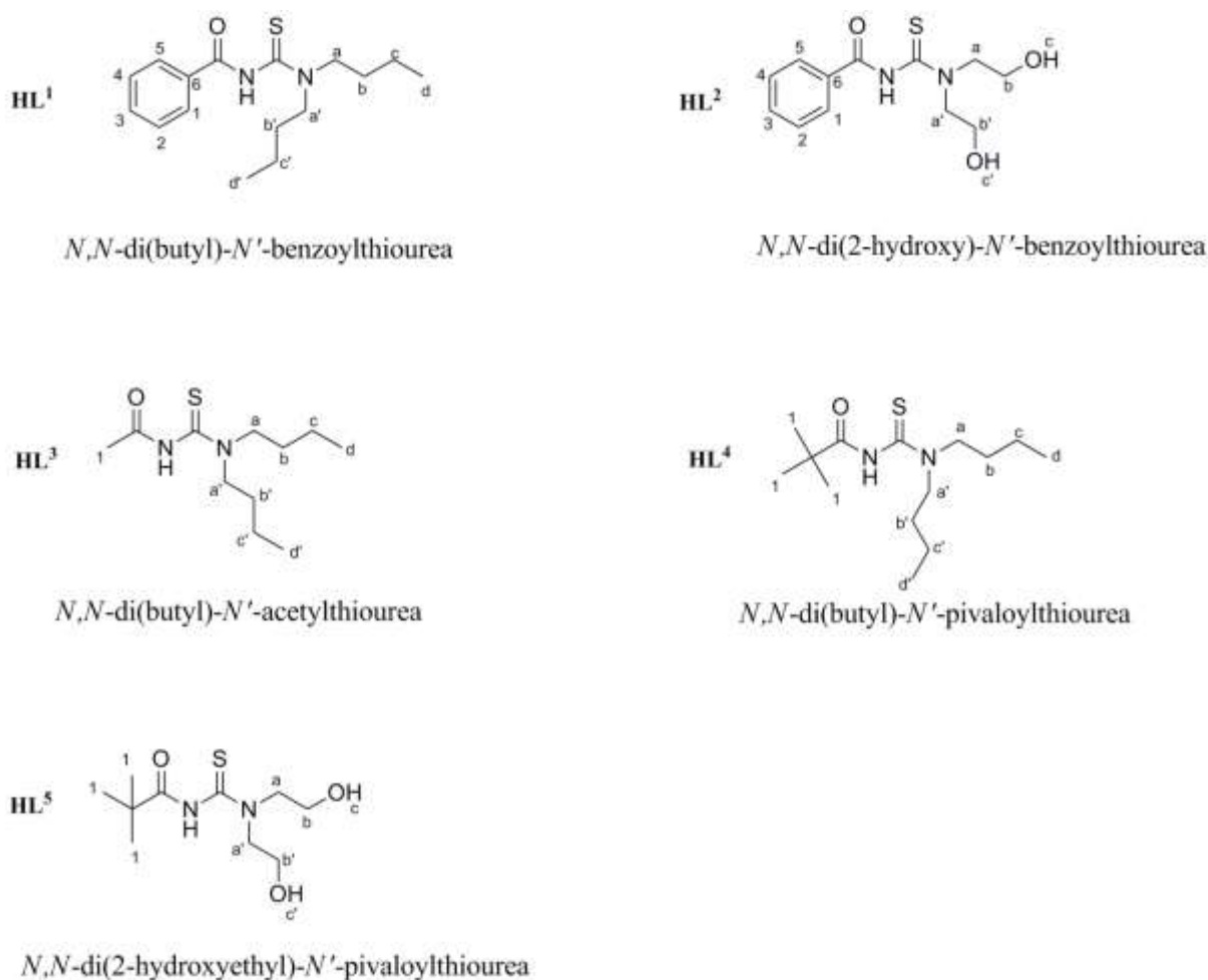
Figure 2.1: Ligands synthesised with their full and abbreviated names
