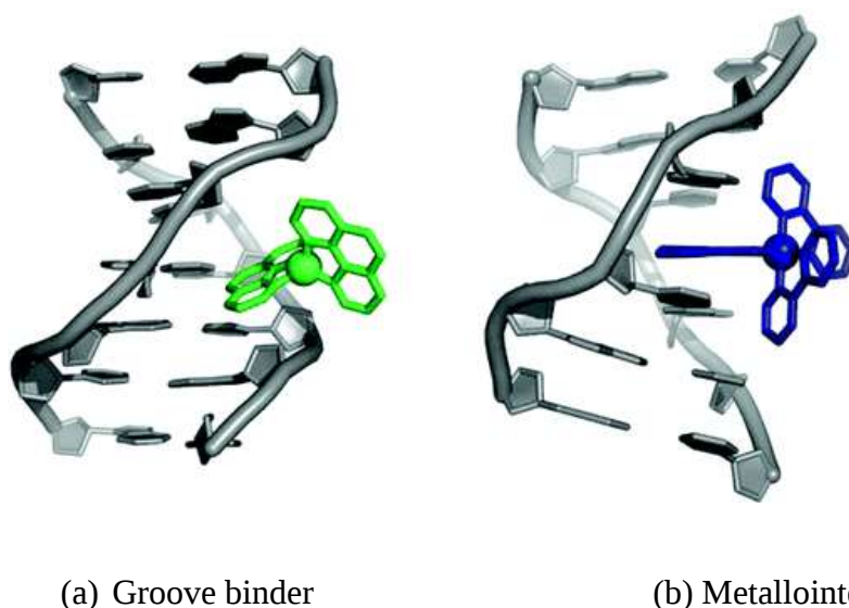
Figure1.2: The two binding modes of metal complexes with DNA: (a) groove binding and (b) intercalation 17
