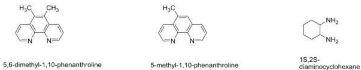
Figure 1.3: 1,10-phenanthroline derivatives and chiral diimine ligands tested for cancer against L1210 mouse leukaemia.
