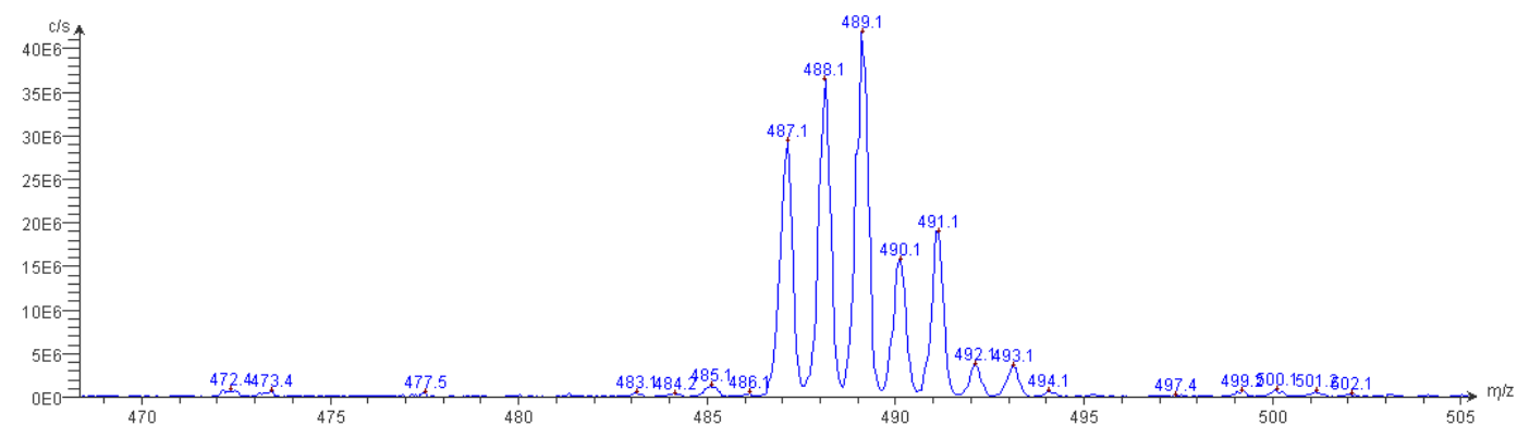
Mass Spectrometry spectrum of [\text{PtCl}_2(1,10\text{-phenanthroline})] .
