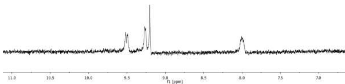
^1\text{H} NMR spectrum of [\text{PtCl}_2(\text{pyrazino}(2,3\text{-}f)(1,10\text{-phenanthroline}))] in \text{DMSO-}d_6 at 25\text{ }^\circ\text{C}
