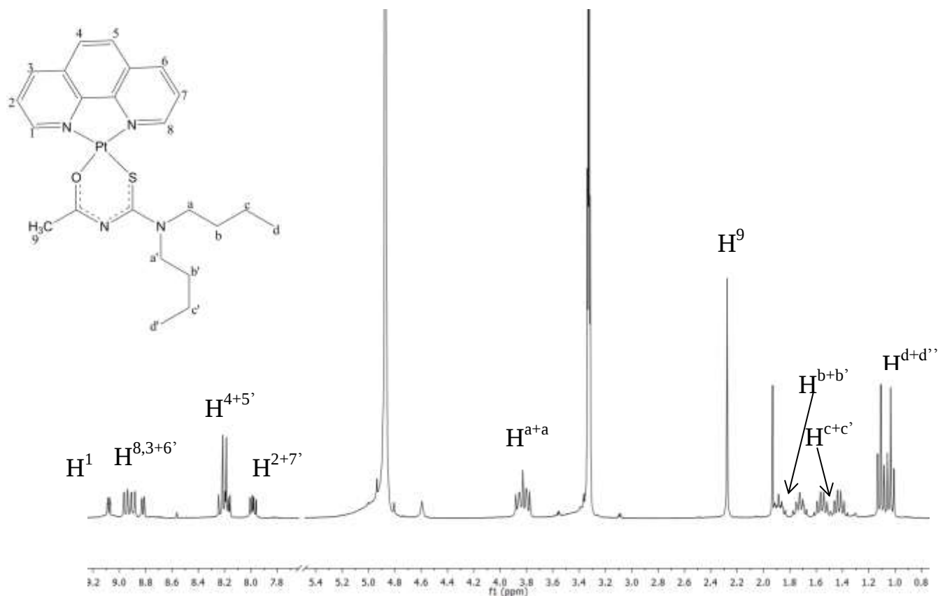
Figure 2.9: ^1\text{H} NMR spectrum full assignment of [\text{Pt}(\text{phen})(\text{L}^3\text{-O,S})]\text{Cl} in acetonitrile- \text{d}_3 at 25\text{ }^\circ\text{C} . (Note: the break on the horizontal scale between 5.4 and 7.7 ppm.)
