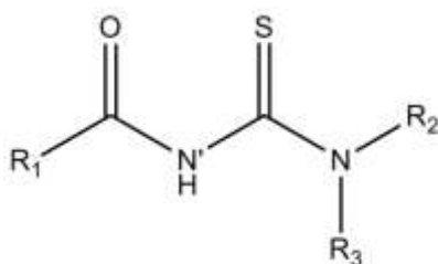
Figure 1.4: General chemical structure of 1-(acyl/aroyl)-3-substituted thioureas
