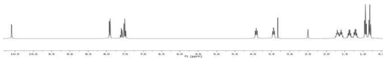
^1\text{H} NMR spectrum of \text{HL}^1 in \text{DMSO-d}_6 at 25\text{ }^\circ\text{C} .
