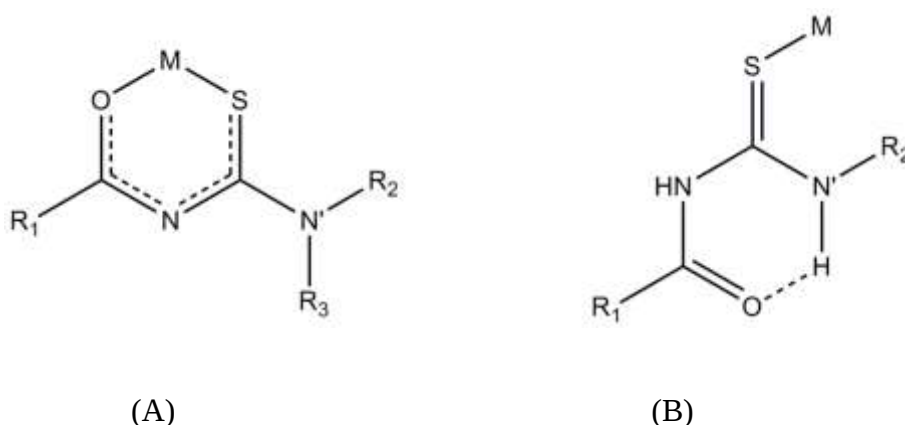
Figure 1.5: Most common coordination modes for monobasic O,S bidentate for dialkyl (A) and neutral monodentate through S atom (B) coordination mode for mono alkyl substituted thiourea.
