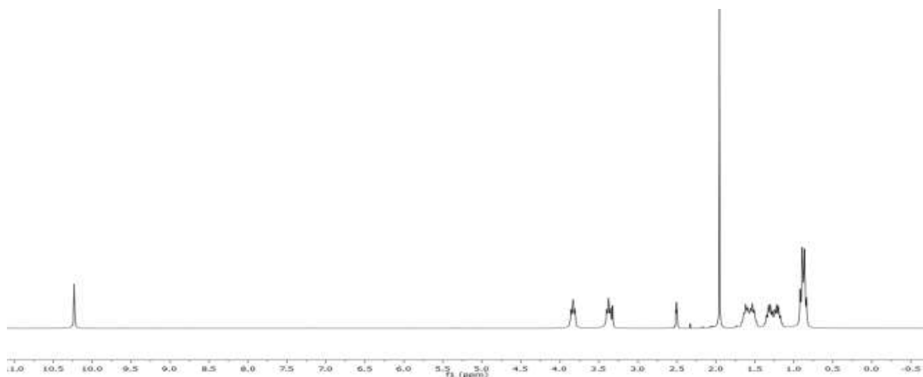
^1\text{H} NMR spectrum of \text{HL}^3 in \text{DMSO-d}_6 at 25\text{ }^\circ\text{C} .
