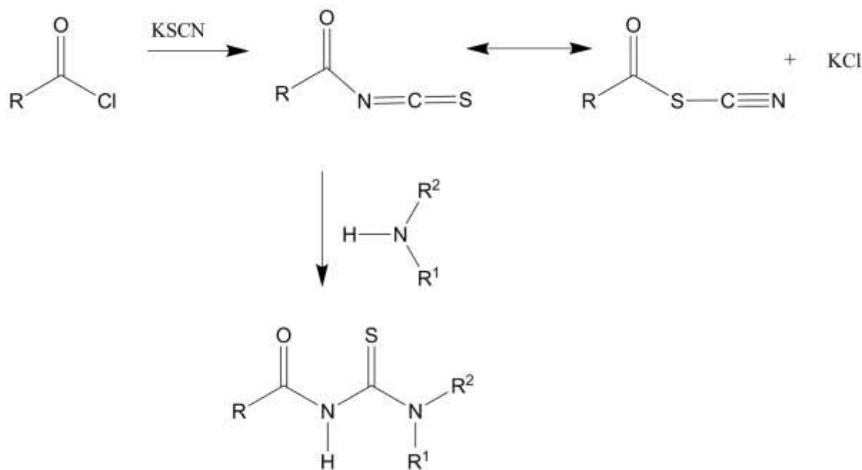
Scheme 2.2: Reaction scheme of the synthetic procedure used for the synthesis of N,N -di(alkyl)- N' -acylthioureas 3 .
