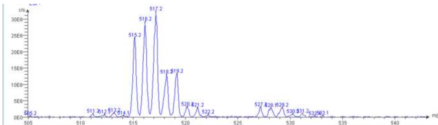
Mass Spectrometry spectrum of [\text{PtCl}_2(5,6\text{-dimethyl-1,10-phenanthroline})] .
