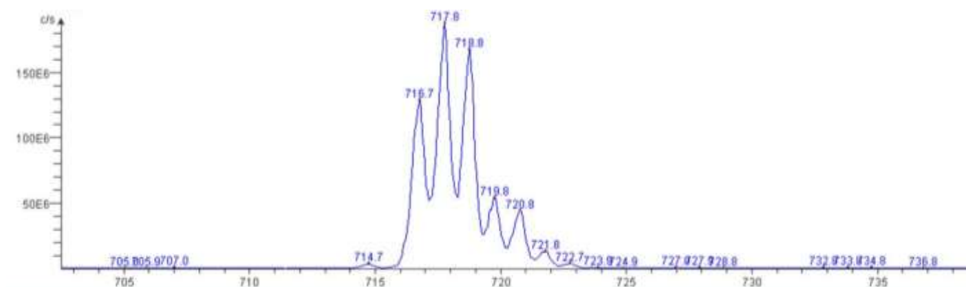
Mass Spectroscopy spectrum of [Pt(dpq)(L^1-O,S)]Cl .
