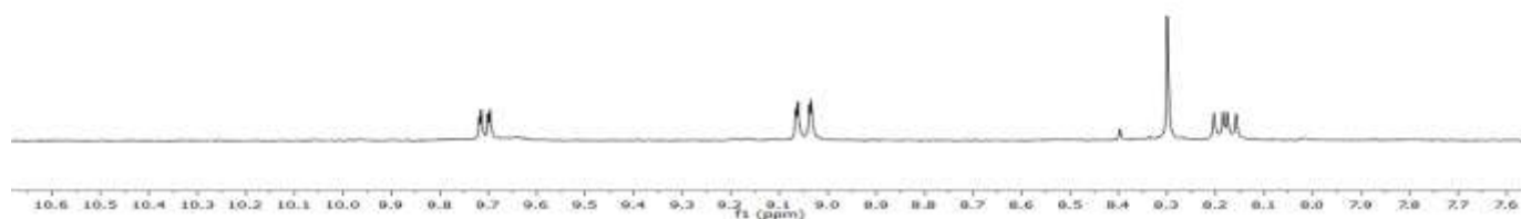
^1\text{H} NMR spectrum of [\text{PtCl}_2(1,10\text{-phenanthroline})] in \text{DMSO-d}_6 at 25\text{ }^\circ\text{C} .
