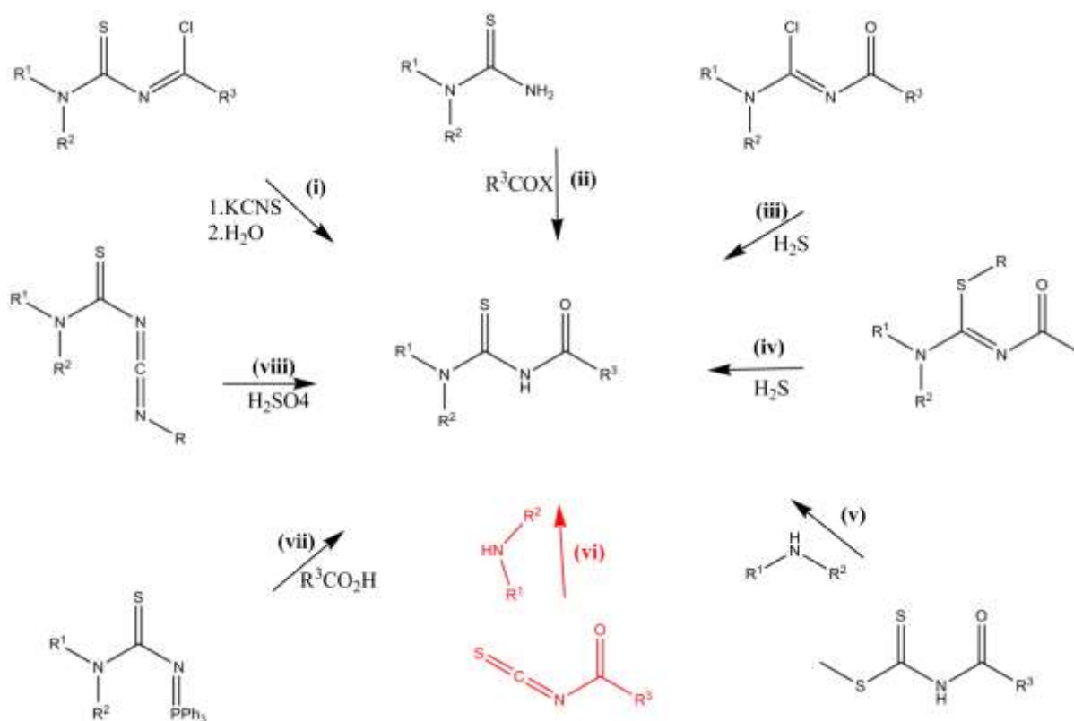
Scheme 2.1: The eight common synthetic routes for N,N -di (alkyl )- N' - cylthioureas: reaction (i) aninothiocarbonyl chloride with KCNS (ii) acylation of N,N -disubstitued thioureas (ii) N -acyl aminoimidoyl with H_2S (iv) N -acylisothiorea with H_2S (v) methyl- N -acylcarbomodithiated (vi) acyl isothiocyanates (vii) aminothiocabonyl with R^3CO_2H (viii) hydrolysis of N -aminothiocarbonylcarbodiimides with mineral acids. 2
