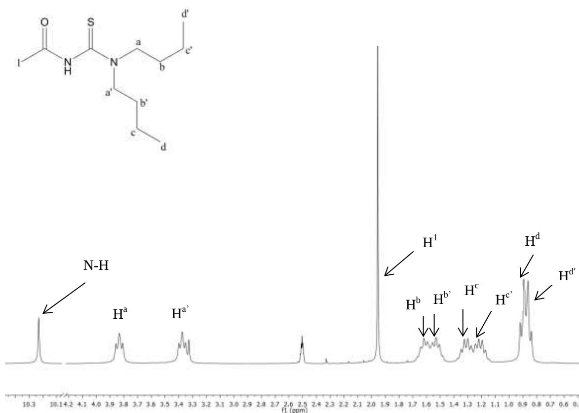
Figure 2.2: ^1H NMR of HL^3 in DMSO-d_6 at 25 °C. (Note: The break in horizontal scale between 10.1 and 4.2 ppm.)
