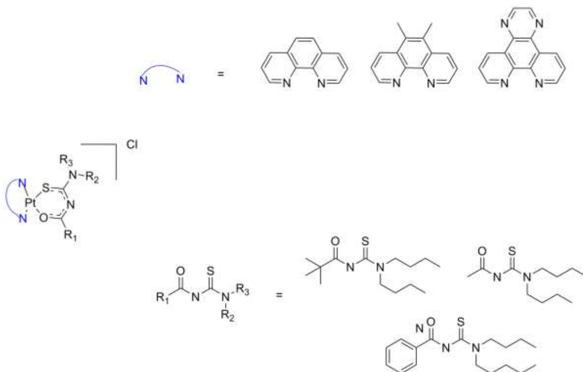
Figure 1.9: Structural variations of the series of [Pt(\text{diimine})(L^n\text{-O,S})]Cl complexes to be synthesised.
