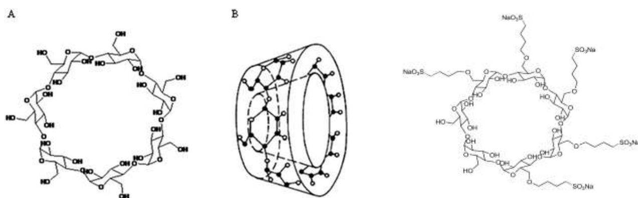
Figure 1.6: The chemical structure (A) and the toroidal shape (B) of the \alpha -cyclodextrin molecule, (C) captisol structure. 39
