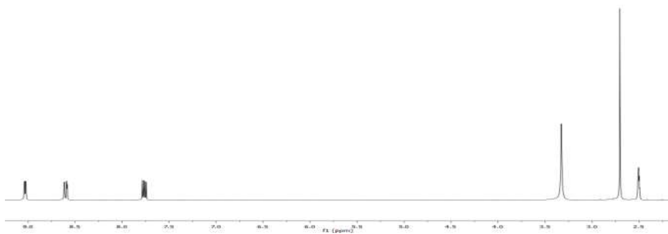
^1\text{H} NMR spectrum of [\text{PtCl}_2(5,6\text{-dimethyl-1,10-phenanthroline})] in \text{DMSO-d}_6 at 25\text{ }^\circ\text{C} .
