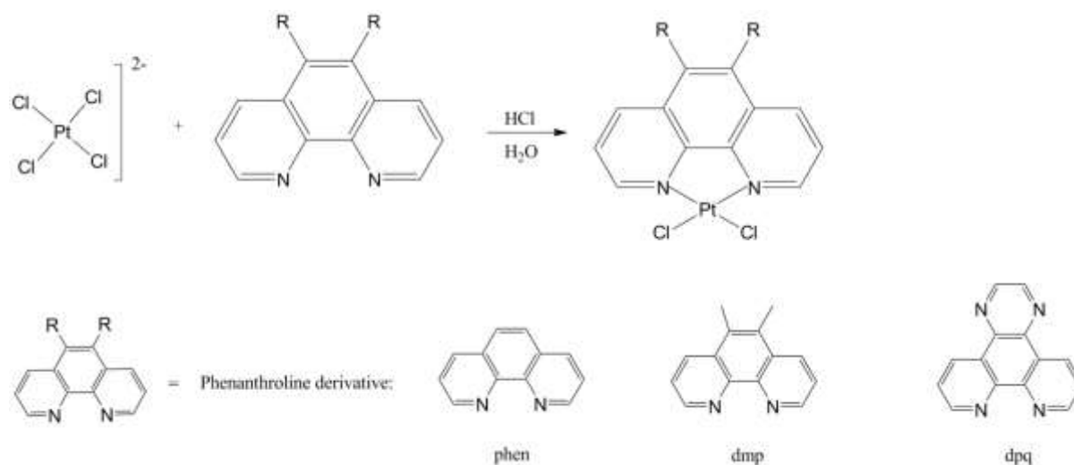
Scheme 2.3: Reaction scheme for the synthesis of [\text{PtCl}_2(\text{diimine})] . 6
