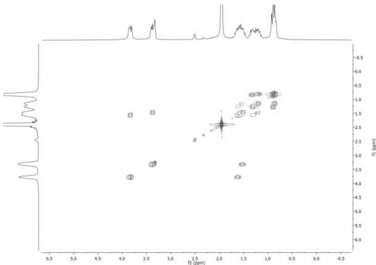
Figure 2.3: The COSY enlarged in the aliphatic region for HL 3 in DMSO- d 6 at 25 °C.
