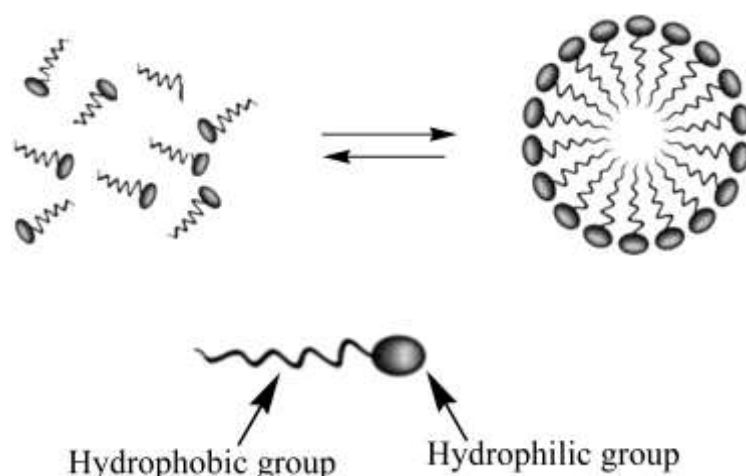
Figure 1.7: Illustration of the hydrophobic and hydrophilic groups and the micelle formation. 43
