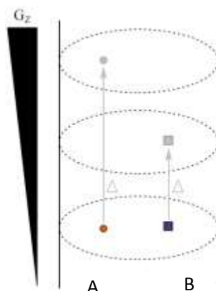
Scheme 4.1: Representation of the translation of molecule A and B.
