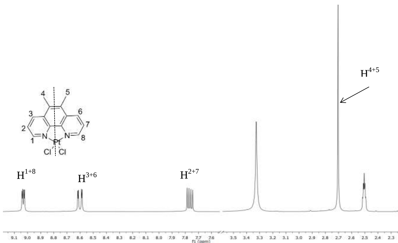
Figure 2.5: ^1\text{H} NMR of [\text{PtCl}_2(\text{dmp})] in DMSO at 25 °C (Note: the break in the horizontal scale between 3.5 and 7.5ppm)
