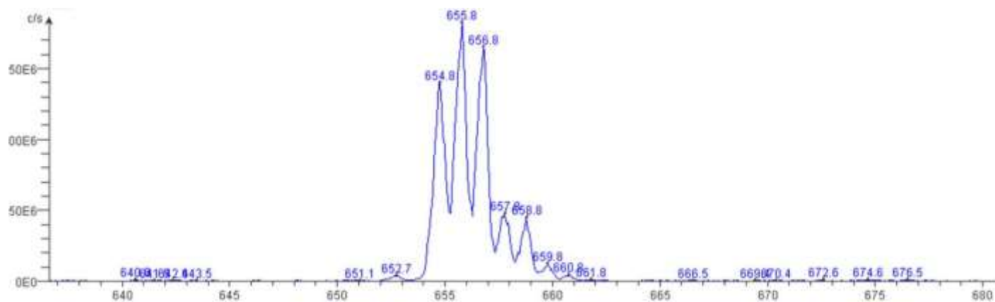
Mass Spectroscopy spectrum of [Pt(dpq)(L^3-O,S)]Cl .
