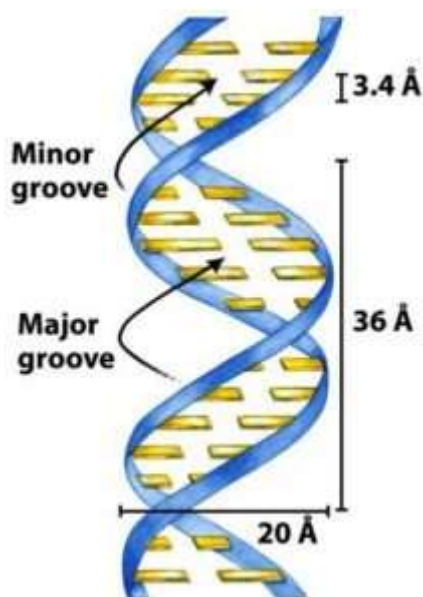
Figure 1.1: Position of the Minor and Major groove in the DNA double helix. 15
