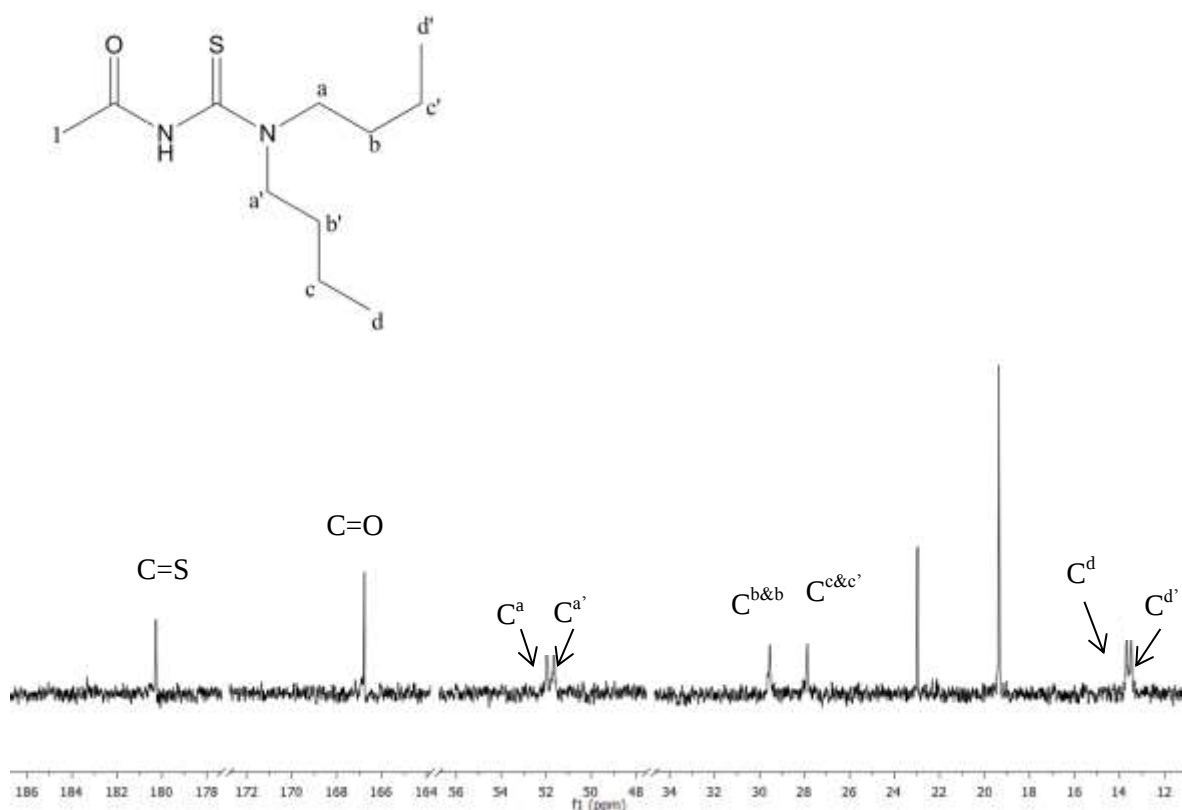
Figure 2.4: 13 C NMR spectrum of HL 3 in DMSO- d 6 at 25 °C. (Note: Two breaks in the horizontal scale between 34-48 ppm, 56-164 ppm and 172-178 ppm).
