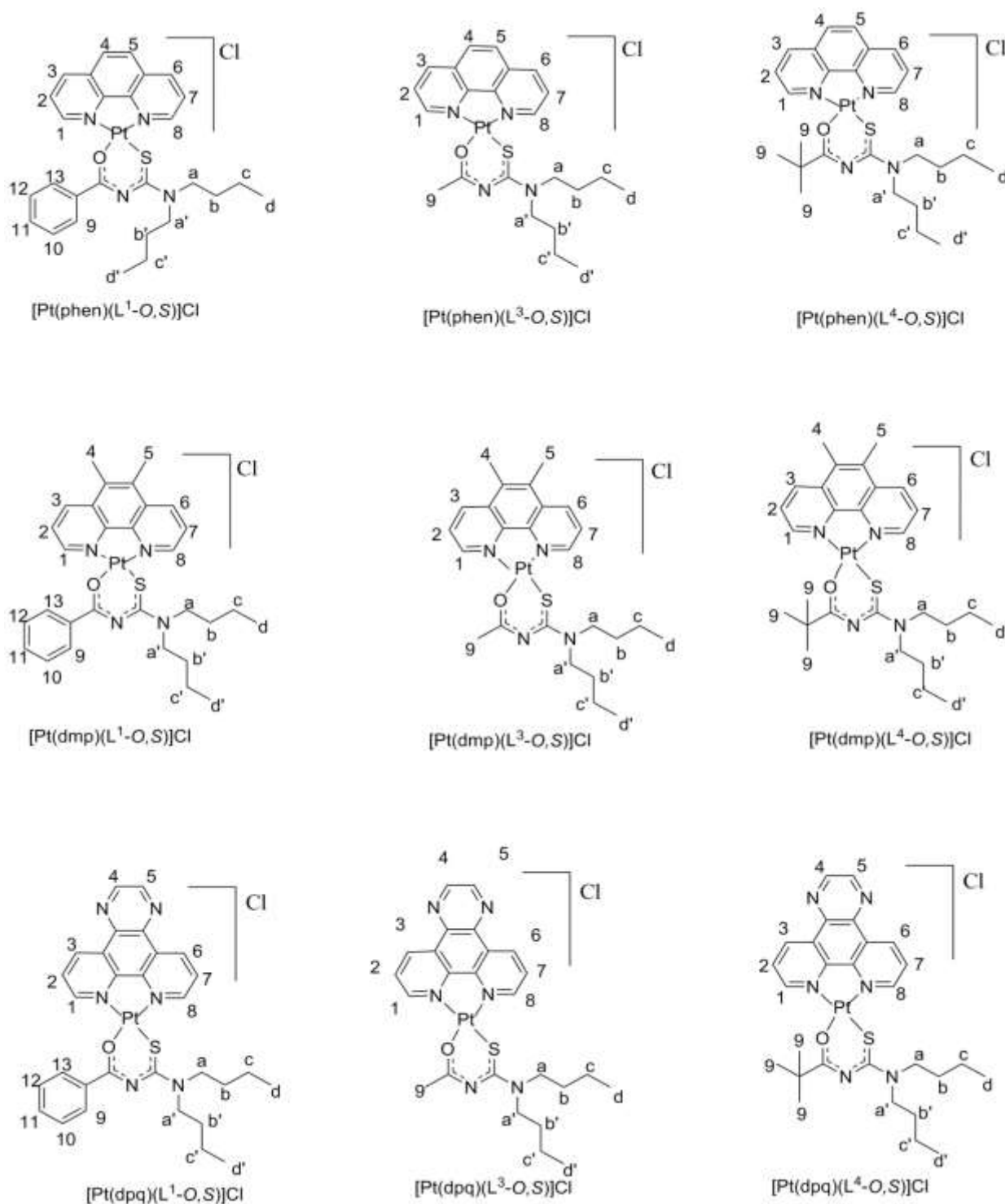
Figure 2.6: [\text{Pt}(\text{diimine})(L^n\text{-O,S})]\text{Cl} Complexes synthesised with abbreviation of the names.
