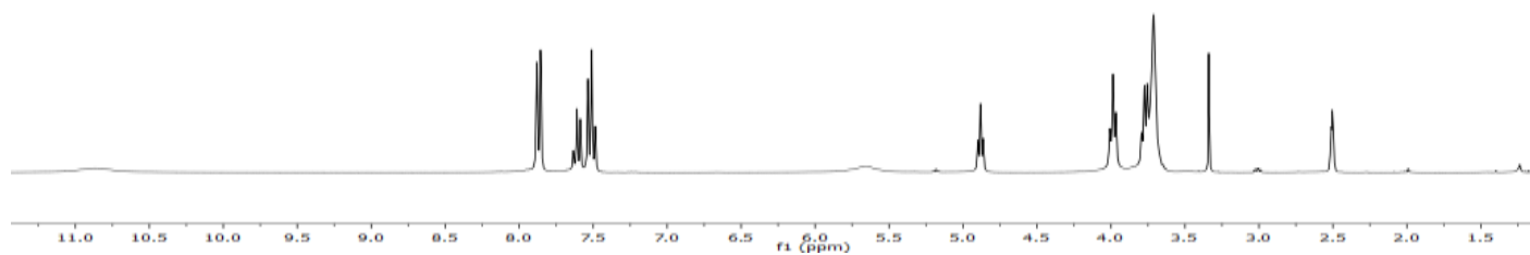
^1\text{H} NMR spectrum of \text{HL}^2 in \text{DMSO-d}_6 at 25\text{ }^\circ\text{C} .
