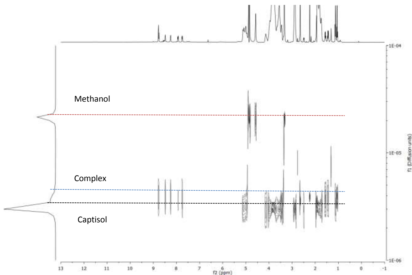
Figure 4.4: DOSY plot of a mixture of [Pt(dmp)(L^3-O,S)]^+ , methanol and water showing the diffusion coefficients.
