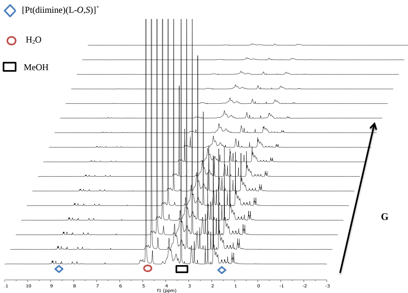
Figure 4.3: Attenuation of the ^1\text{H} NMR of the mixture of inclusion complex, methanol, water during a typical DOSY experiment with the increasing gradient strength ( G ).
