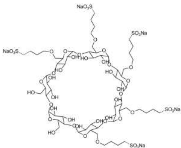
Figure 4.1: Representation of the structure of captisol.
