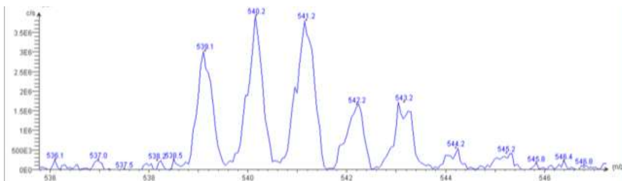
Mass Spectroscopy spectrum of [PtCl_2(pyrazino(2,3-f)(1,10-phenanthroline))] .
