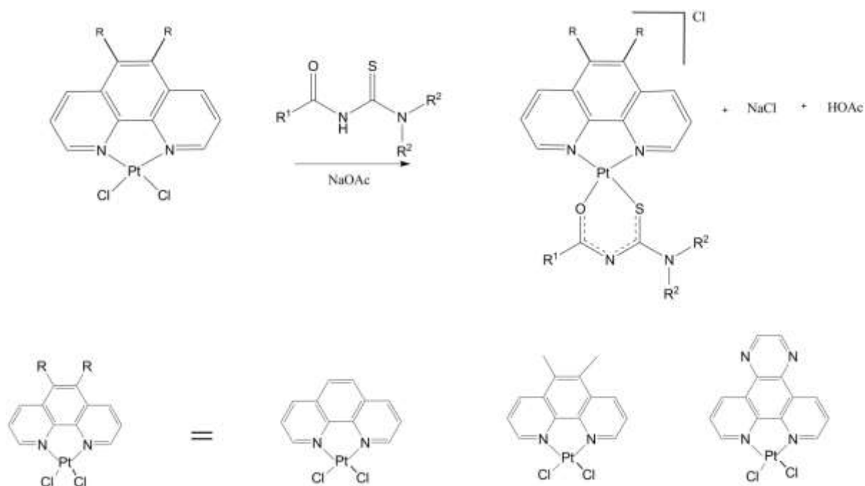
Scheme 2.4: Reaction scheme of the synthetic procedure of [Pt(diimine)(L-O,S)]^+ complexes 7
