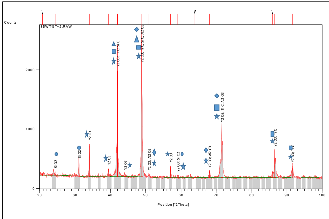
Figure 5.1 c) 85 wt.% TiC (+SiO 2 ) (5:8:7) + 20 vol.% SiCw powder (■TiC, ♦ Al 2 O 3 , ▲SiC, ●SiO 2 , ★Y 2 O 3 )
