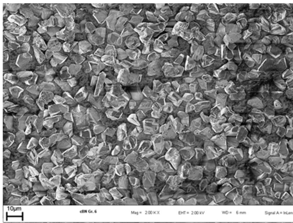
Figure 3.4 A SEM image of cBN crush grade 6
