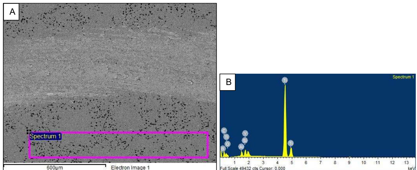
Figure 7.26 A: Spectrum 1 Area alongside the wear track scanned by EDS for composition B: Results of EDS qualitative analysis on Spectrum 1.
