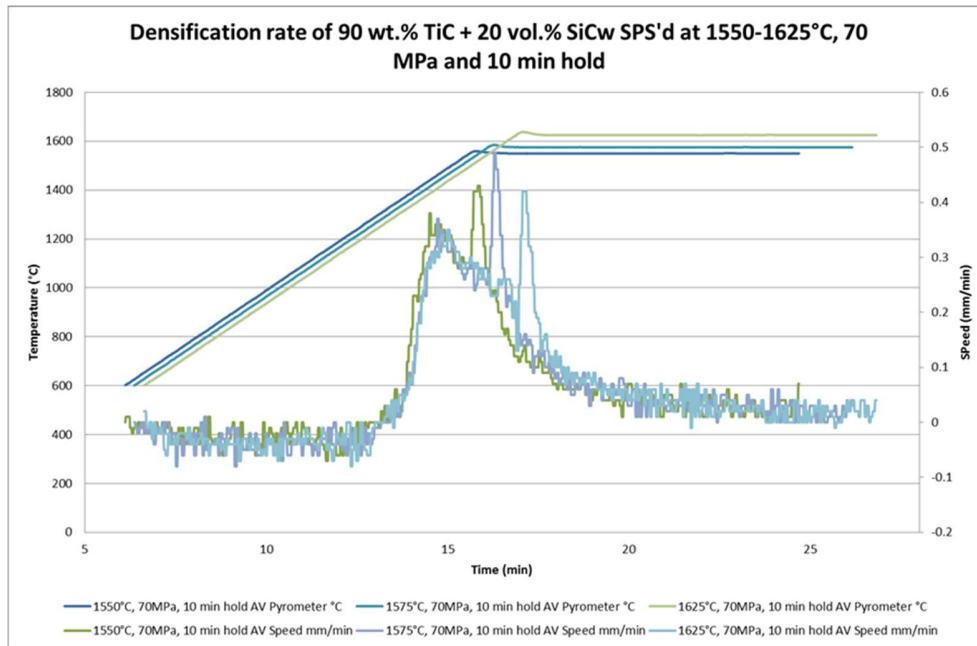
Figure 1 b) Densification rate
