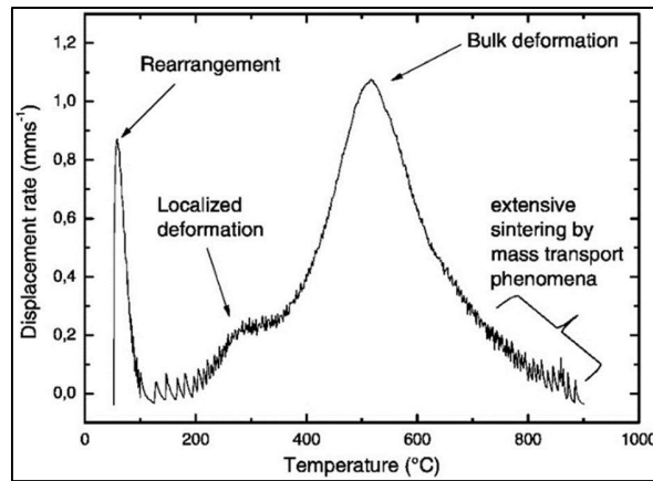
Figure 2.2 Displacement rate Vs temperature for powder processed with the initial pressure and densification mechanisms (Diouf & Molinari, 2012).
