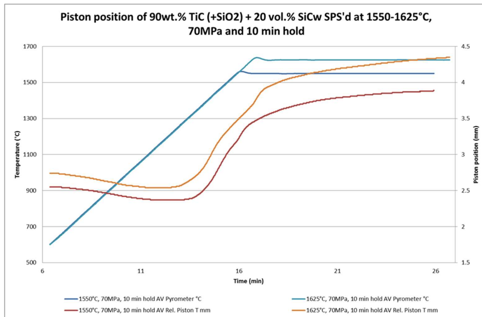
Figure 1 a) Piston position
