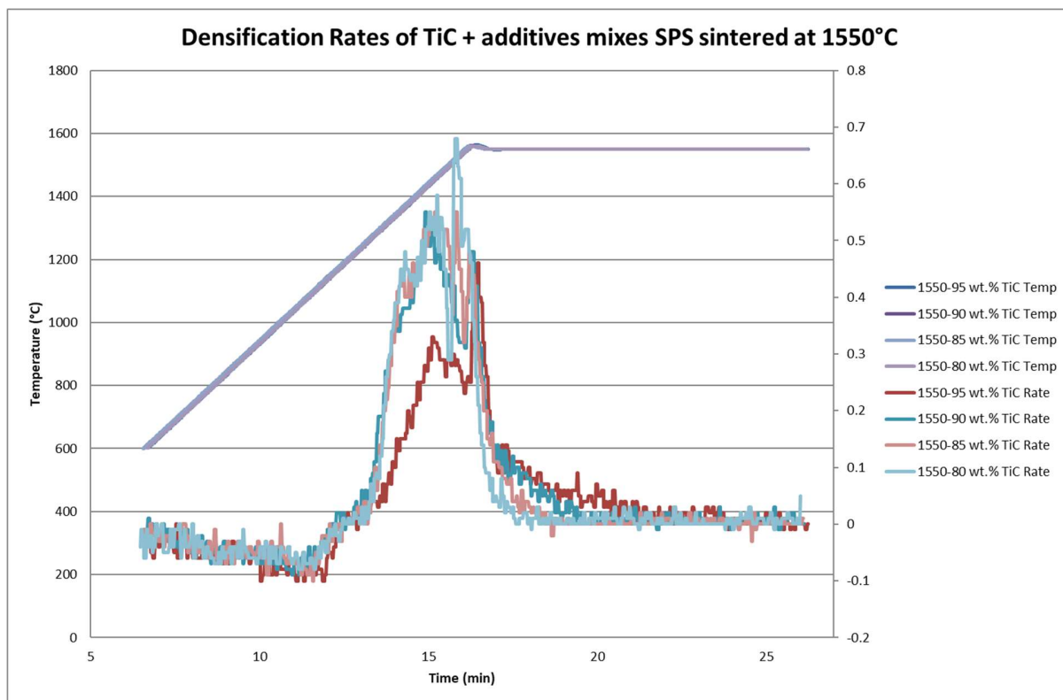
Figure 2 b) Densification rate
