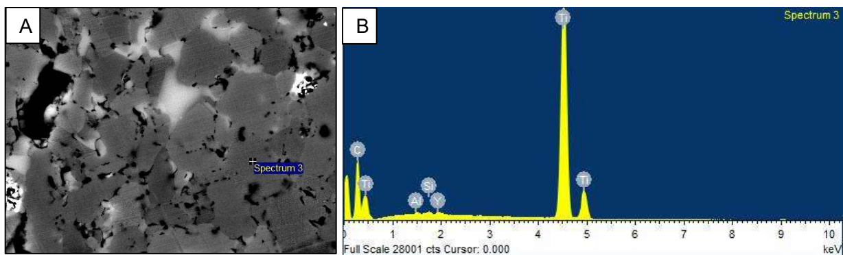
Figure 4.14 A: Image of the area of sintered 90TiC-2.5Al 2 O 3 -4Y 2 O 3 -3.5SiO 2 SPS'd at 1625°C, 70MPa and 10 min hold scanned by EDS for composition B: Results of EDS qualitative analysis on the area highlighted in Fig. 4.14 A.
