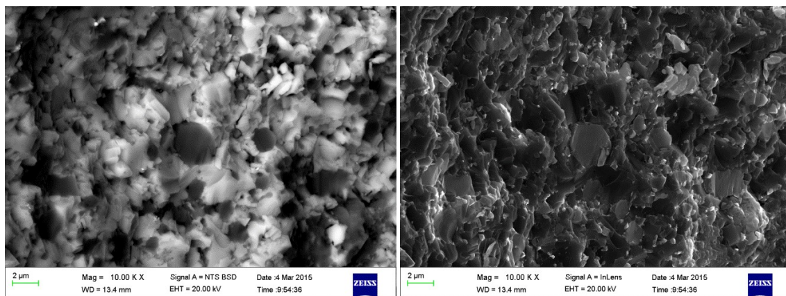
Figure 6.23 A - Fracture surface analysed under high magnification (10.0 K X) using Backscatter Detector and B- same surfaced analysed under high magnification using Secondary Electron Detector
