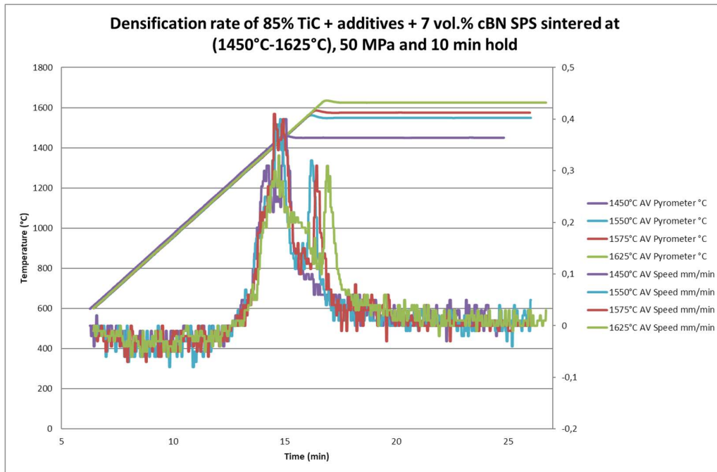
Figure 1 b) Densification rate
