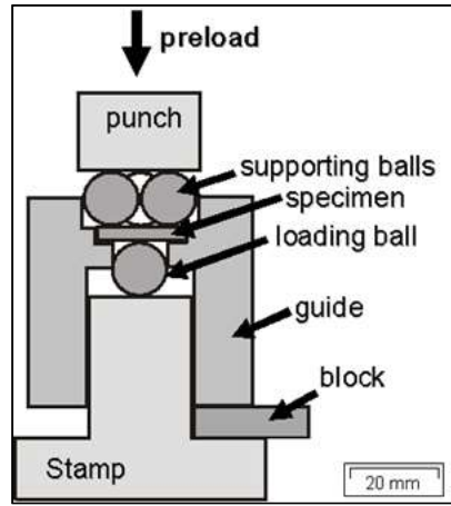
Figure 3.8 Sketch of the B3B experimental setup (Harrer et al., 2012)
