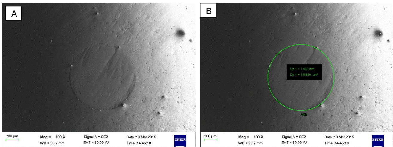
Figure 7.10 A: Wear scar on the surface of the worn AISI 52100 steel ball bearing. B: Diameter and area of the wear scar on the worn AISI 52100 steel ball bearing. (Diameter: 1.032mm and Area: 0.837mm 2 )
