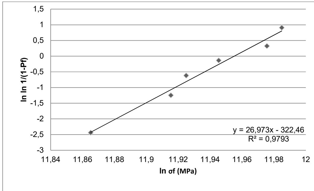
Figure 6.24 Graph of the regression line used to determine the Weibull modulus for 77.8TiC-6.9Al 2 O 3 -1.7Y 2 O 3 -14(20 vol.%) SiCw
