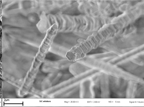
Figure 3.3 SEM images of SiC whiskers (higher magnification)
