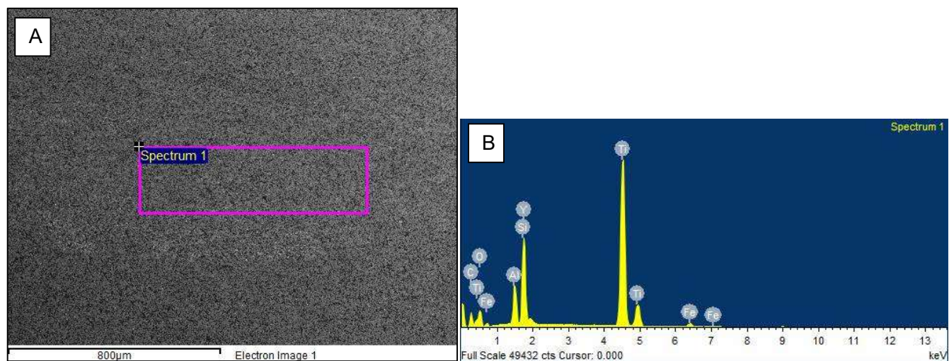
Figure 7.15 A: Spectrum 1 Area on the wear track scanned by EDS for composition B: Results of EDS qualitative analysis on Spectrum 1.
