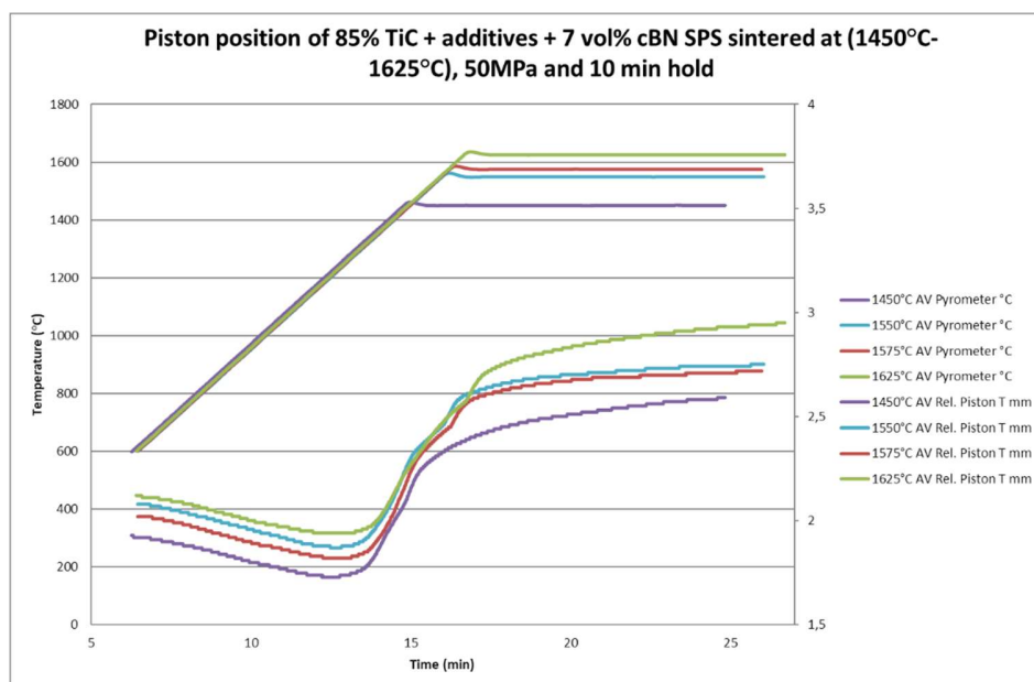
Figure 1 a) Temperature profile, piston position
