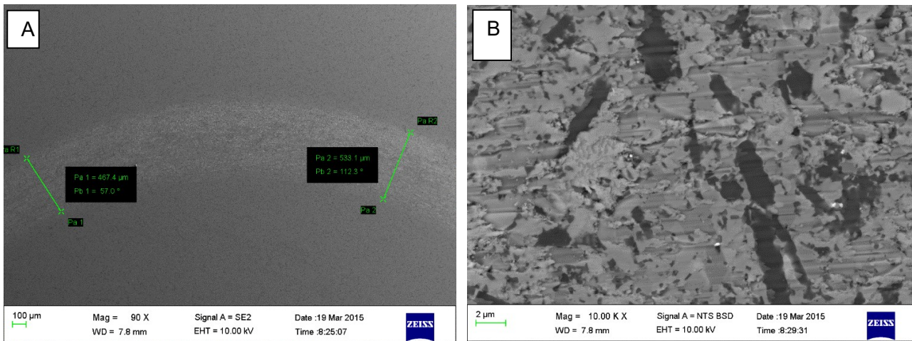
Figure 7.7 A: wear track on the surface of the 79TiC-11Al 2 O 3 -3Y 2 O 3 -7(10 vol.%) SiCw sample disc. B: High magnification image of the wear track on the 79TiC-11Al 2 O 3 -3Y 2 O 3 -7(10 vol.%) SiCw sample disc.
