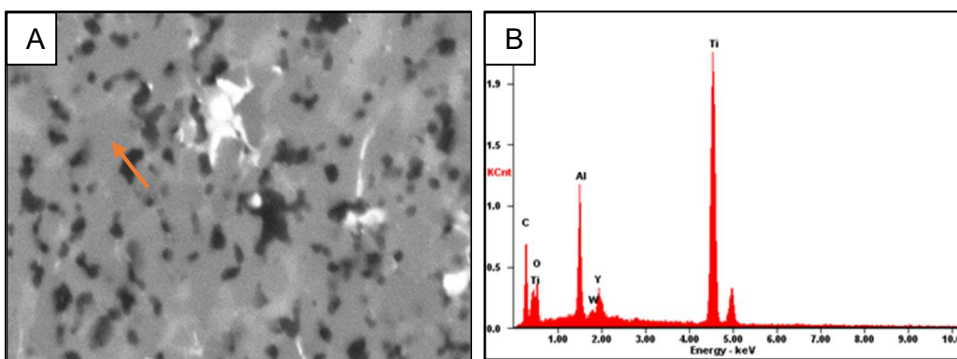
Figure 4.11 A: Image of the area of sintered 85TiC-12Al 2 O 3 -3Y 2 O 3 SPS'd at 1550 °C, 50MPa and 10 min hold scanned by EDS for composition B: Results of EDS qualitative analysis on the area highlighted in Fig. 4.11 A.
