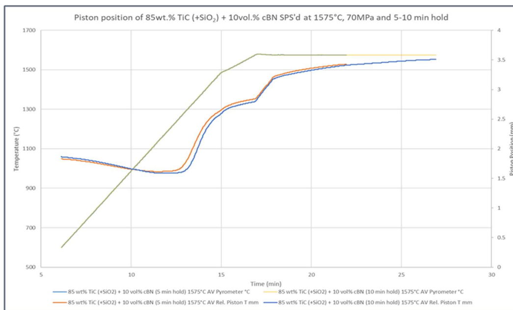
Figure 1 a) Piston position
