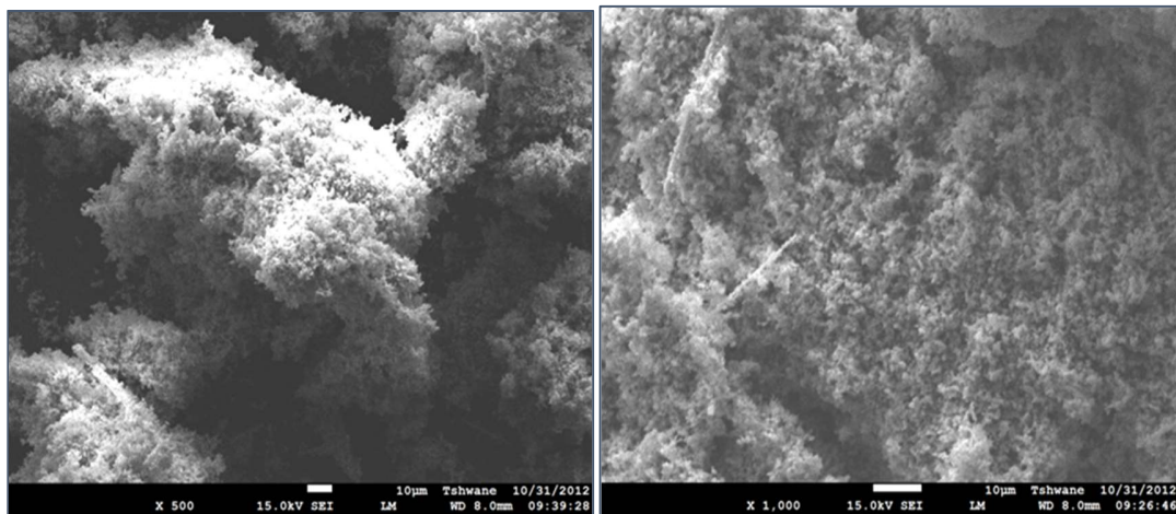
Figure 5.2 SEM images of 83.8 wt.% TiC-7.45 wt.% Al 2 O 3 -1.86 wt. %Y 2 O 3 matrix powder after the addition of 6.89 wt.% (10 vol.%) SiC whiskers
