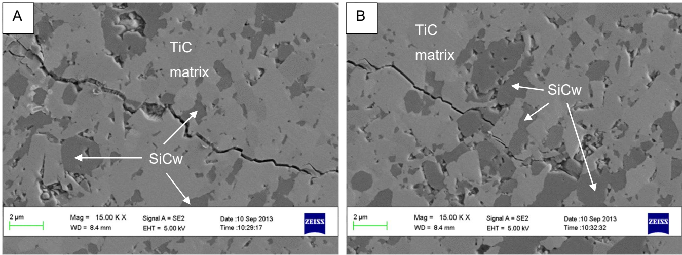
Figure 5.9 SEM micrographs of A – 77.2TiC-6.9Al 2 O 3 -1.7Y 2 O 3 -14.2 (20 vol.%) SiCw SPS'd at 1625°C, 70MPa and 20 min hold time and B - crack path from Vickers Hardness indentation in 77.2TiC-6.9Al 2 O 3 -1.7Y 2 O 3 -14.2 (20 vol.%) SiCw SPS'd at 1625°C, 70MPa and 20 min hold time magnified by 15 K X.
