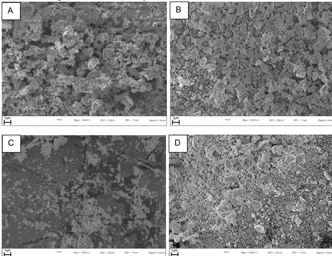
Figure 4.3A Micrograph of 95% TiC mix, Figure 4.3B Micrograph of 90% TiC mix, Figure 4.3C Micrograph of 85% TiC mix and Figure 4.3D Micrograph of 80% TiC mix
