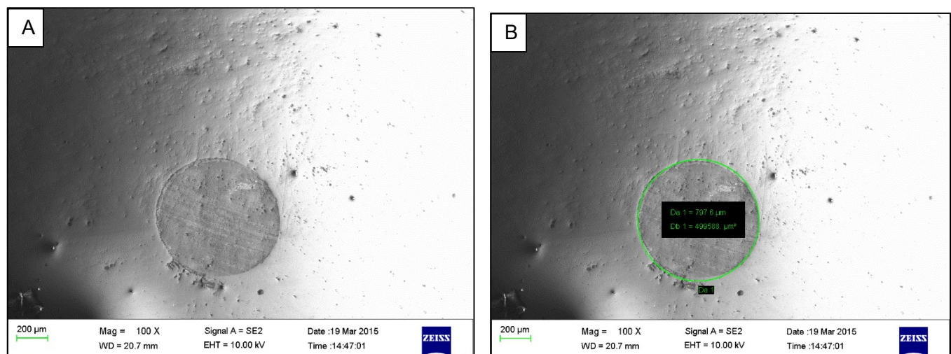
Figure 7.22 A: Wear scar on the surface of the worn AISI 52100 steel ball bearing. B: Diameter and area of the wear scar on the worn AISI 52100 steel ball bearing. (Diameter: 0.798mm and Area: 0.500mm 2 )
