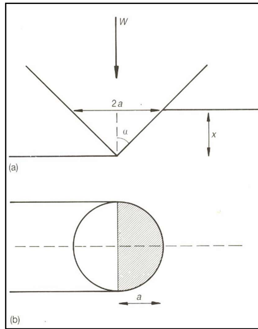
Figure 2.14 Geometry of contact between an idealised conical abrasive particle and a surface: (a) in elevation; (b) in the plane view (K.-H. Zum Gahr, 1987)
