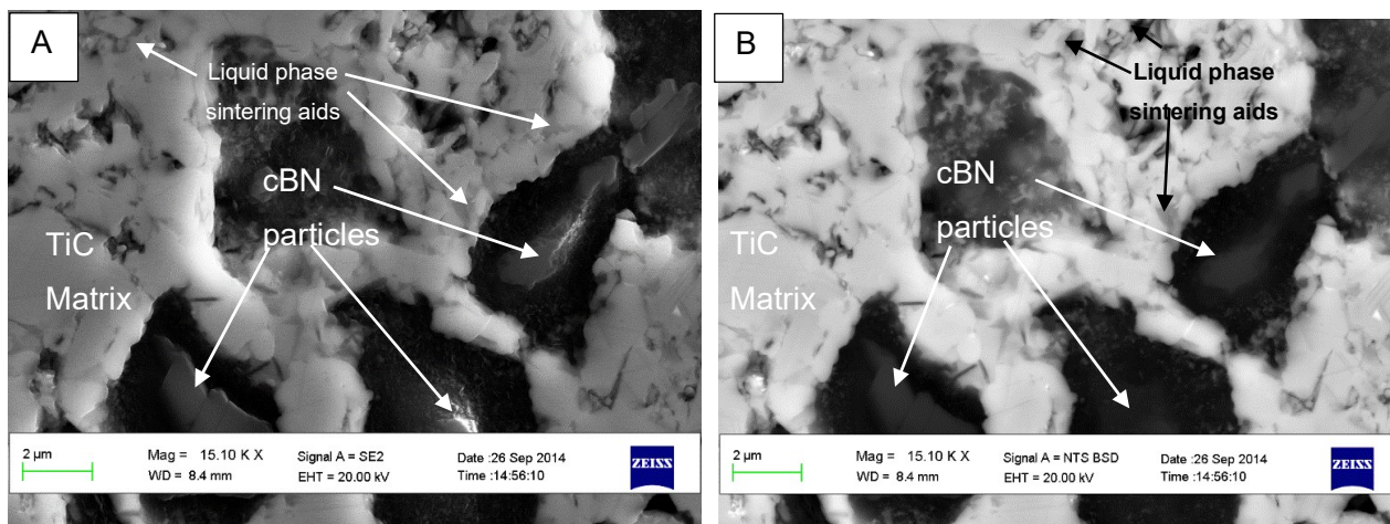
Figure 5.14 SEM micrographs of A – 83.3TiC-2.3Al 2 O 3 -3.7Y 2 O 3 -3.2SiO 2 -7.5 (10 vol.%) cBN SPS'd at 1575°C, 70MPa and 10 min hold time viewed with the Secondary electron detector magnified at 15.1 K X and B - 83.3TiC-2.3Al 2 O 3 -3.7Y 2 O 3 -3.2SiO 2 -7.5 (10 vol.%) cBN SPS'd at 1575°C, 70MPa and 10 min hold time viewed via Backscatter electron detector magnified by 15.1 K X.
