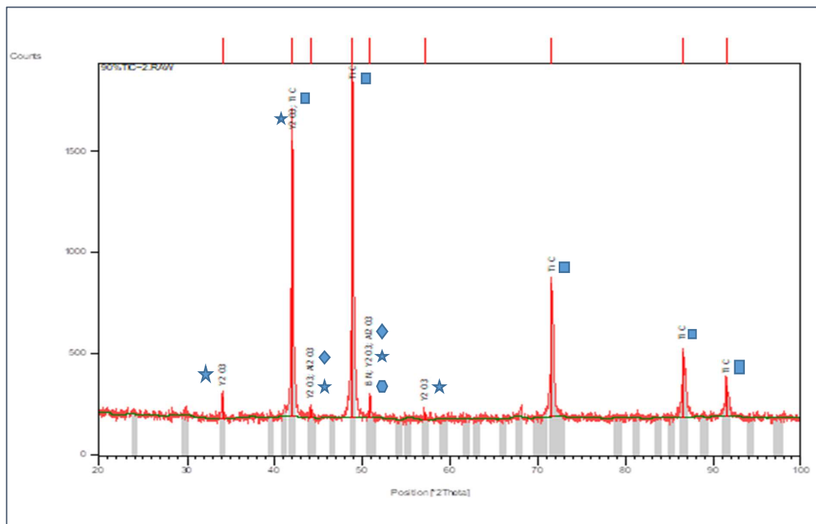
Figure 5.1 b) 90 wt.% TiC (2µm) + 7 vol.% cBN powder (■TiC, ♦ Al 2 O 3 , ●BN, ★Y 2 O 3 )
