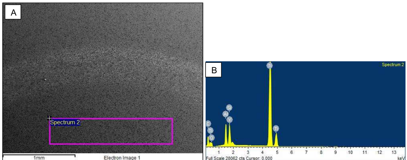
Figure 7.8 A: Spectrum 2 Area alongside the wear track scanned by EDS for composition B: Results of EDS qualitative analysis on Spectrum 2
