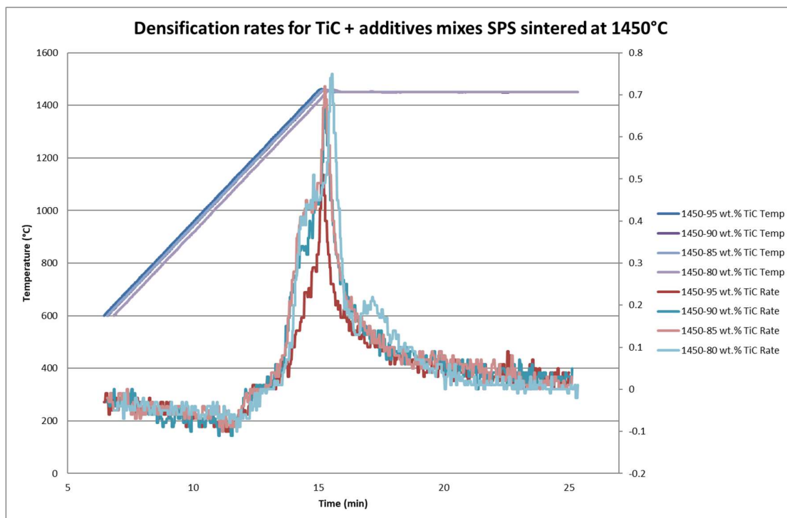
Figure 1 b) Densification rate
