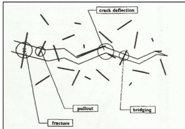
Figure 2.6 Typical processes occurring during crack propagation in whisker reinforced ceramics (Bengisu et al., 1991).
