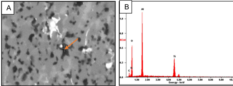
Figure 4.9 A: Image of the area of sintered 85TiC-12Al 2 O 3 -3Y 2 O 3 SPS'd at 1550 °C, 50MPa and 10 min hold scanned by EDS for composition B: Results of EDS qualitative analysis on the area highlighted in Fig. 4.9 A.
