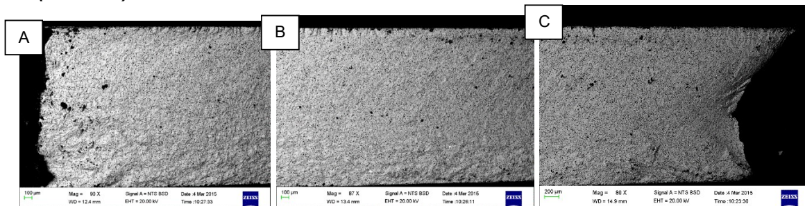
Figure 6.18 A- Outer limit of fractured edge (outside circumference of sample furthest from the site of loading), B- mid-length of fractured edge and C-inner edge of fracture of edge (centre of sample directly under the site of loading)
