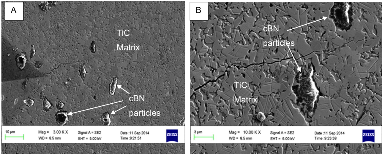
Figure 5.11 SEM micrographs of A – 78.6TiC-3.5Al 2 O 3 -5.6Y 2 O 3 -4.9SiO 2 -7.5 (10 vol.%) cBN SPS'd at 1625°C, 70MPa and 10 min hold time and B - crack path from Vickers Hardness indentation in 78.6TiC-3.5Al 2 O 3 -5.6Y 2 O 3 -4.9SiO 2 -7.5 (10 vol.%) cBN SPS'd at 1625°C, 70MPa and 10 min hold time magnified by 10 K X.
