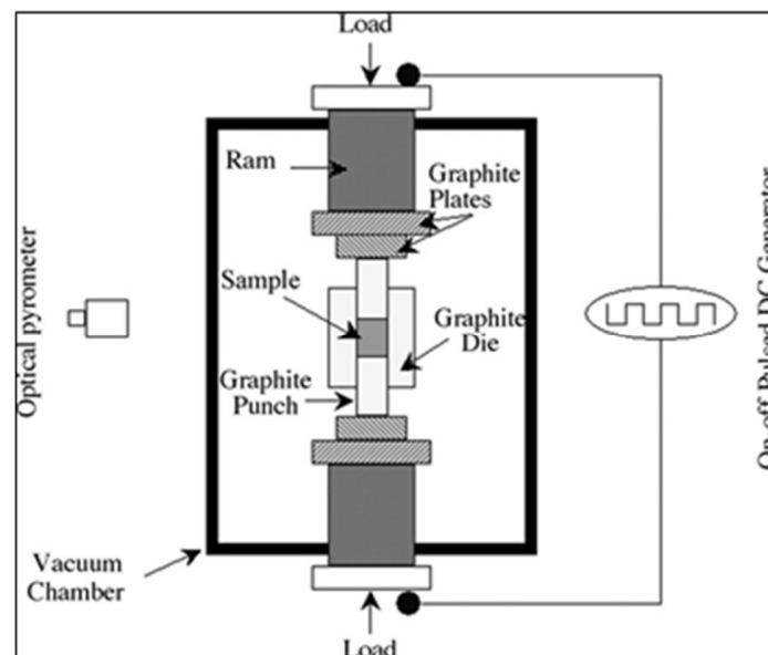
Figure 2.7 Schematic representation of the spark plasma sintering apparatus (Zhao & Wang, 2009)
