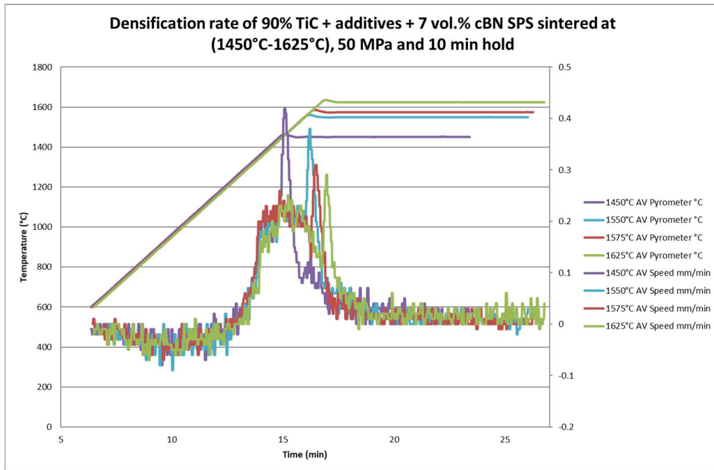
Figure 2 b) Densification rate
