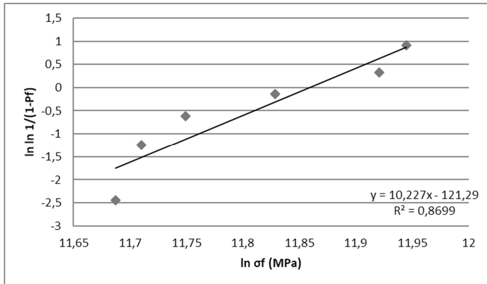
Figure 6.20 Graph of the regression line used to determine the Weibull modulus for 78.6TiC-3.5Al 2 O 3 -5.6Y 2 O 3 -4.9SiO 2 -7.5 (10 vol.%) cBN
