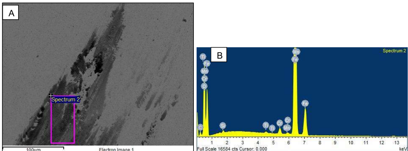
Figure 7.12 A: Spectrum 2 Area inside the wear scar on the worn AISI 52100 steel ball bearing scanned by EDS for composition B: Results of EDS qualitative analysis on Spectrum 2.
