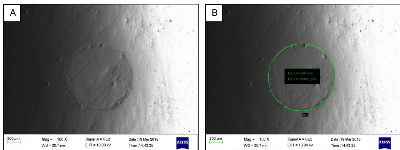
Figure 7.4 A: Wear scar on the surface of the worn AISI 52100 steel ball bearing. B: Diameter and area of the wear scar on the worn AISI 52100 steel ball bearing. (Diameter: 1.041mm and Area: 0.850mm 2 )
