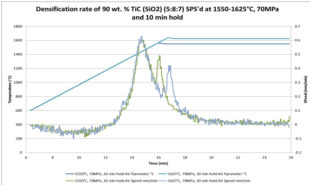
Figure 2 b) Densification rate
