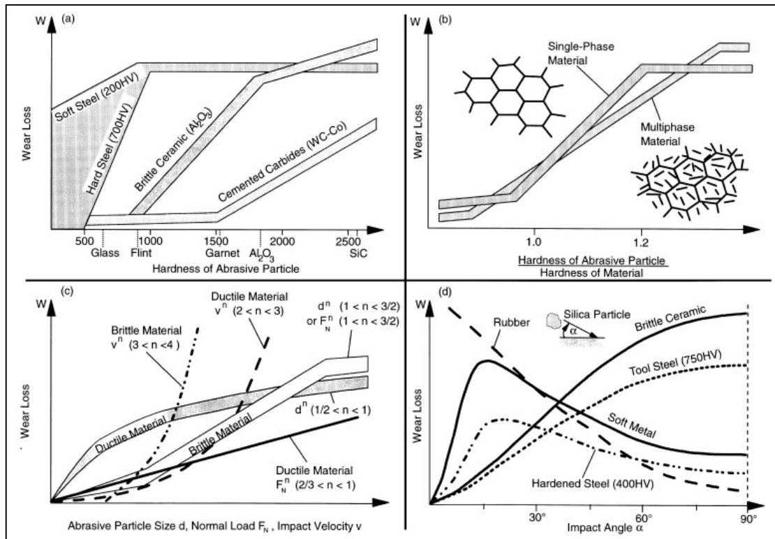
Figure 2.13 Graphs of wear loss by hard particles as a function of material properties and operating parameters such as: a) hardness of the abrasive particle, b) ratio of hardness of the abrasive particle and hardness of the wearing material, c) abrasive particle size, normal load and impact velocity and d) impact angle without considering lubrication (K.-H. Z. Gahr, 1998).
