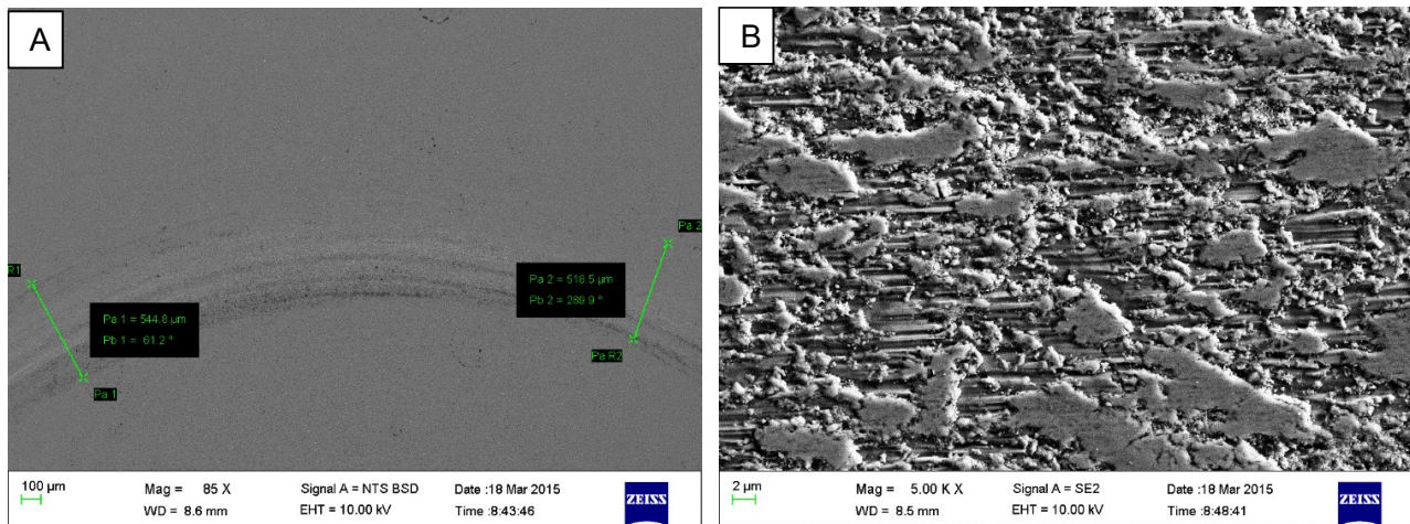
Figure 7.1 A: wear track on the surface of the 85TiC-12Al 2 O 3 -3Y 2 O 3 matrix only sample disc. B: High magnification image of the wear track on the 85TiC-12Al 2 O 3 -3Y 2 O 3 matrix only sample disc.
