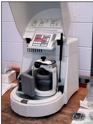
Figure 3.6 Fritsch Pulverisette 6 planetary ball mill
