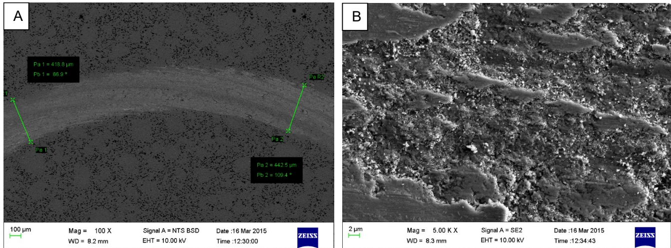
Figure 7.25 A: wear track on the surface of the 78.6TiC-3.5Al 2 O 3 -5.6Y 2 O 3 -4.9SiO 2 -7.5 (10 vol.%) cBN sample disc SPS'd at 1575°C, 70MPa and 5 min hold . B: High magnification image of the wear track on the 78.6TiC-3.5Al 2 O 3 -5.6Y 2 O 3 -4.9SiO 2 -7.5 (10 vol.%) cBN sample disc.
