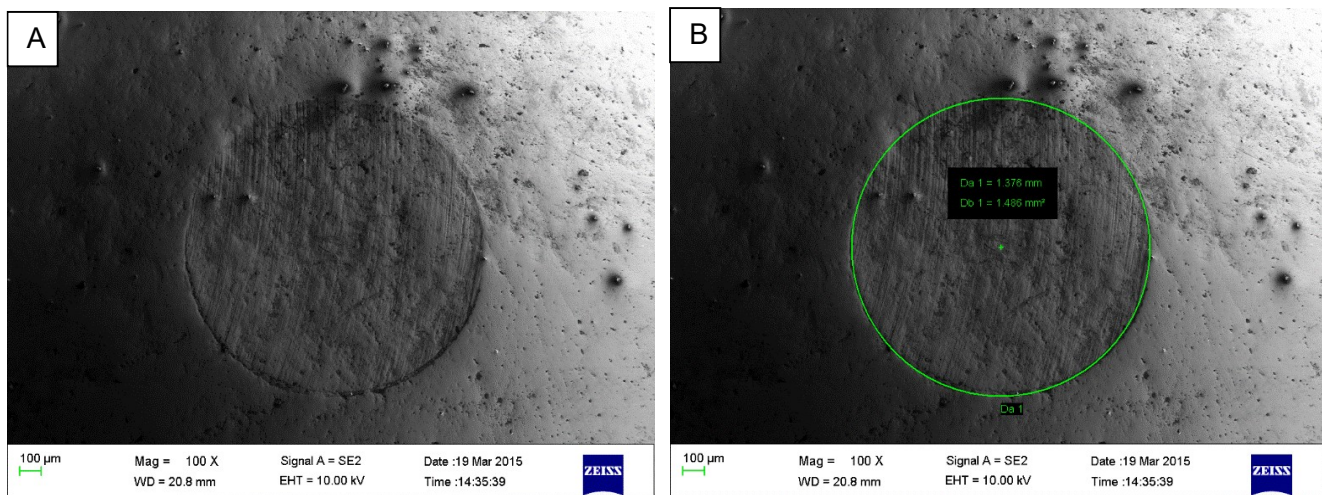
Figure 7.28 A: Wear scar on the surface of the worn AISI 52100 steel ball bearing. B: Diameter and area of the wear scar on the worn AISI 52100 steel ball bearing. (Diameter: 1.376mm and Area: 1.486mm 2 )
