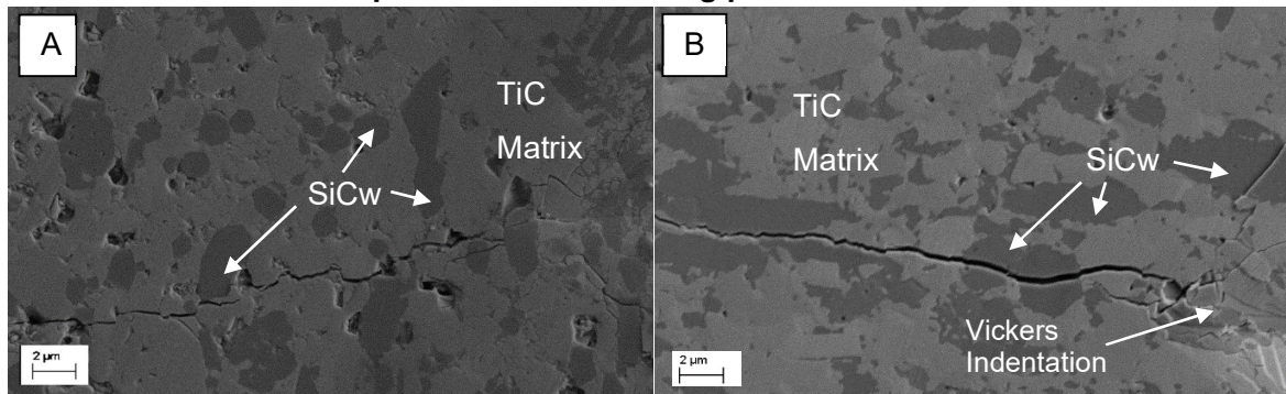
Figure 5.7 SEM micrographs of A - crack path from Vickers Hardness indentation in a sample with the composition 79TiC-11 \text{Al}_2\text{O}_3 -3 \text{Y}_2\text{O}_3 -7 (10 vol.%) SiCw SPS'd at 1600°C, 70MPa and 10 min hold time and B - crack path from Vickers Hardness indentation in a sample with the composition 73TiC-10 \text{Al}_2\text{O}_3 -3 \text{Y}_2\text{O}_3 -14 (20 vol.%) SiCw SPS'd at 1625°C, 70MPa and 10 min hold.
