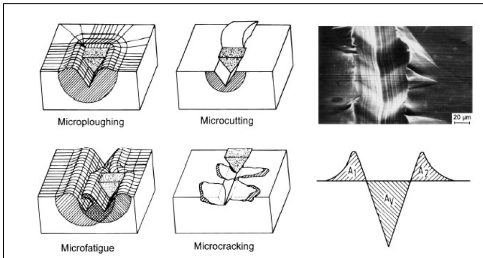
Figure 2.16 Schematic representation of different interactions between sliding abrasive particles and the surface of materials, scanning electron micrograph of a wear groove on an austenitic steel and a draft of a taper section through the wear groove (K.-H. Z. Gahr, 1998).
