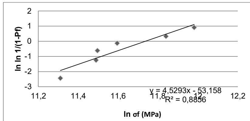
Figure 6.4 Graph of the regression line used to determine the Weibull modulus for 85TiC-12Al 2 O 3 -3Y 2 O 3
