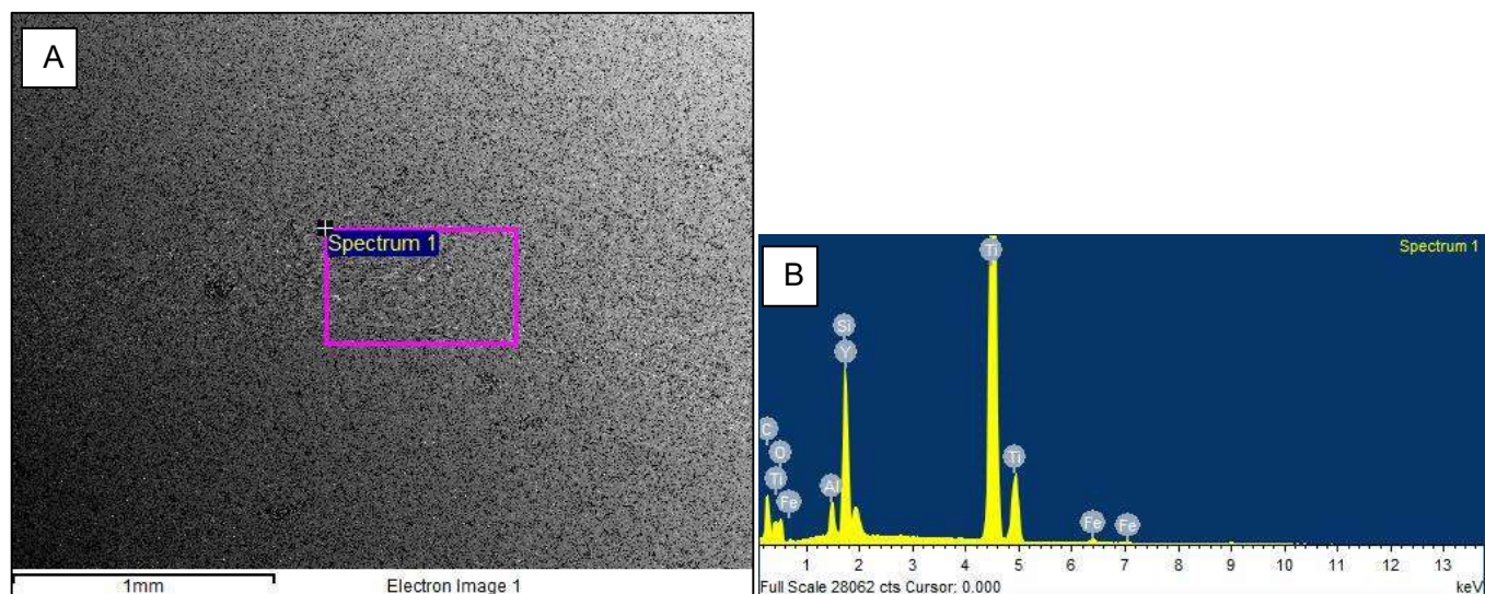
Figure 7.21 A: Spectrum 1 Area on the wear track scanned by EDS for composition B: Results of EDS qualitative analysis on Spectrum 1.
