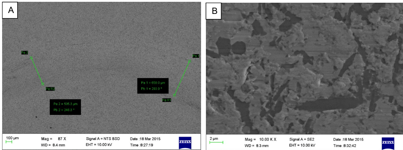
Figure 7.31 A: wear track on the surface of the 77.8TiC-6.9Al 2 O 3 -1.7Y 2 O 3 -14(20 vol.%) SiCw sample disc. B: High magnification image of the wear track on the 77.8TiC-6.9Al 2 O 3 -1.7Y 2 O 3 -14(20 vol.%) SiCw sample disc.
