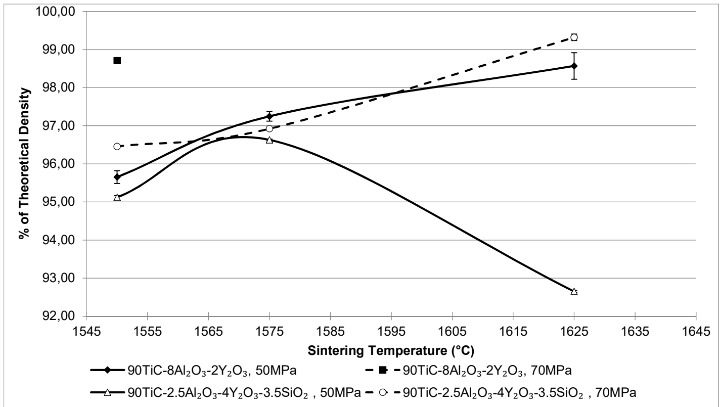
Figure 4.5 Graph of the trends in the density of SPS sintered samples with 90 wt. % TiC and liquid phase sintering aids
