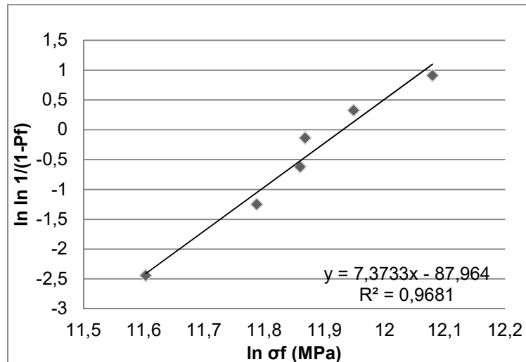
Figure 6.12 Graph of the regression line used to determine the Weibull modulus for 73TiC-10Al 2 O 3 -3Y 2 O 3 -14(20 vol.%) SiCw
