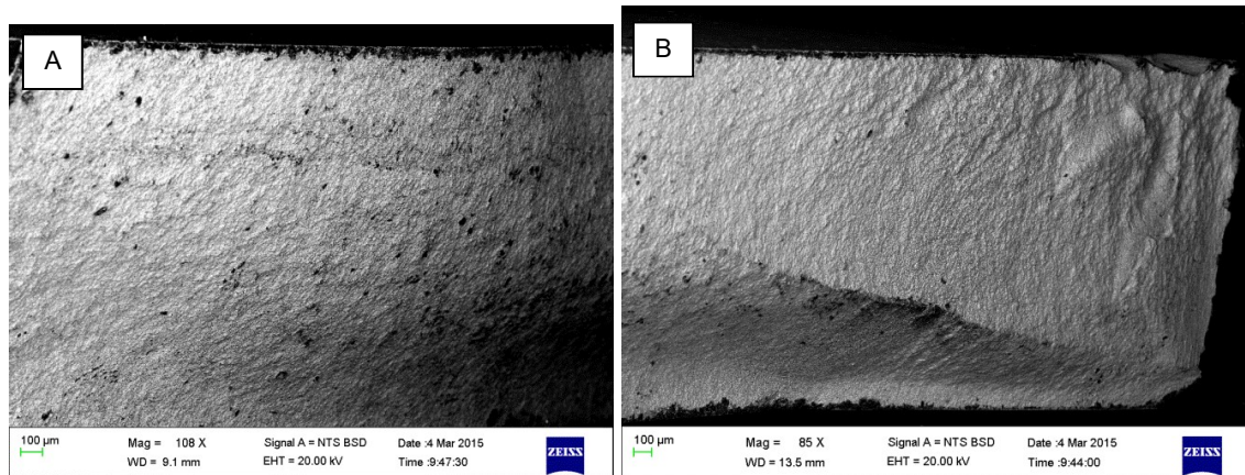
Figure 6.22 A- mid-length of fractured edge and B- inner edge of fracture of edge (centre of sample directly under the site of loading)
