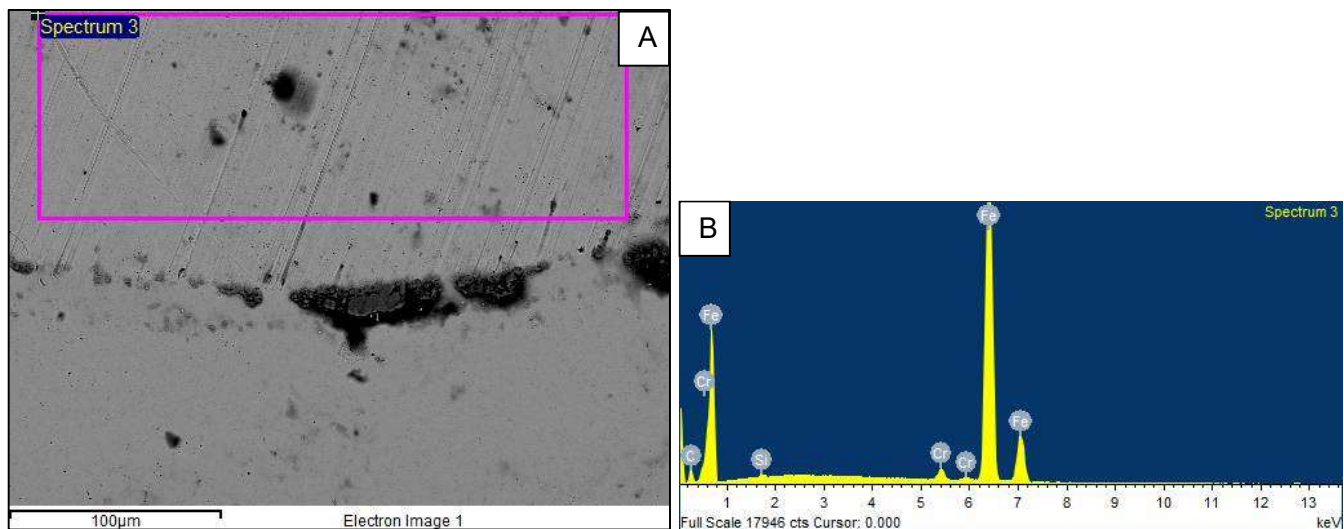
Figure 7.30 A: Spectrum 3 Area inside the wear scar on the worn AISI 52100 steel ball bearing scanned by EDS for composition B: Results of EDS qualitative analysis on Spectrum 3.
