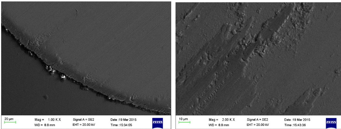
Figure 7.5 A: High magnification image of the edge of the wear scar on the worn AISI 52100 steel ball bearing. B: Higher magnification image of the centre of the wear scar on the worn AISI 52100 steel ball bearing.
