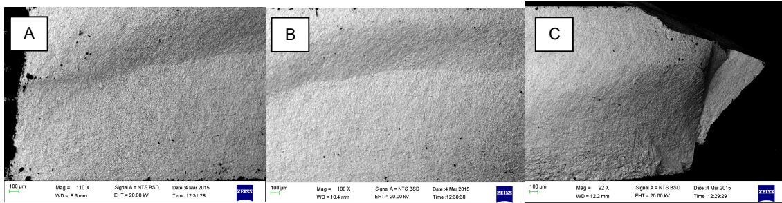
Figure 6.14 A- Outer limit of fractured edge (outside circumference of sample furthest from the site of loading), B- mid-length of fractured edge and C-inner edge of fracture of edge (centre of sample directly under the site of loading)
