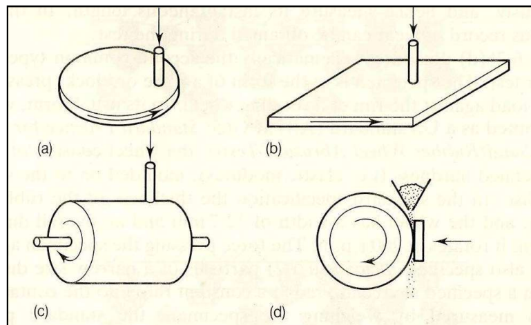
Figure 2.18 Schematic illustrations of four common methods used to measure abrasive wear rates of materials: (a) Pin on abrasive disc; (b) pin on abrasive plate; (c) pin on abrasive drum; (d) rubber wheel abrasion test (Axén et al., 2001)
