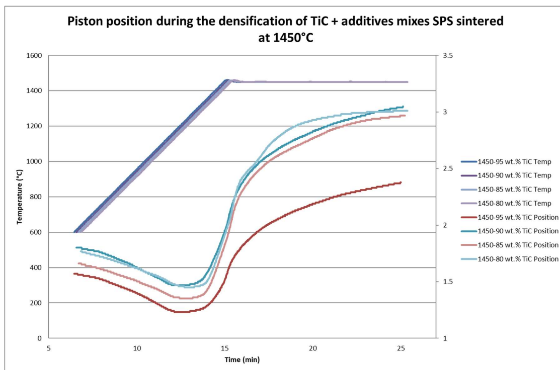
Figure 1 a) Piston position
