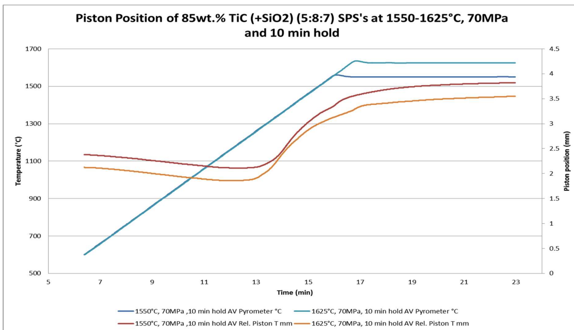
Figure 1 a) Piston position
