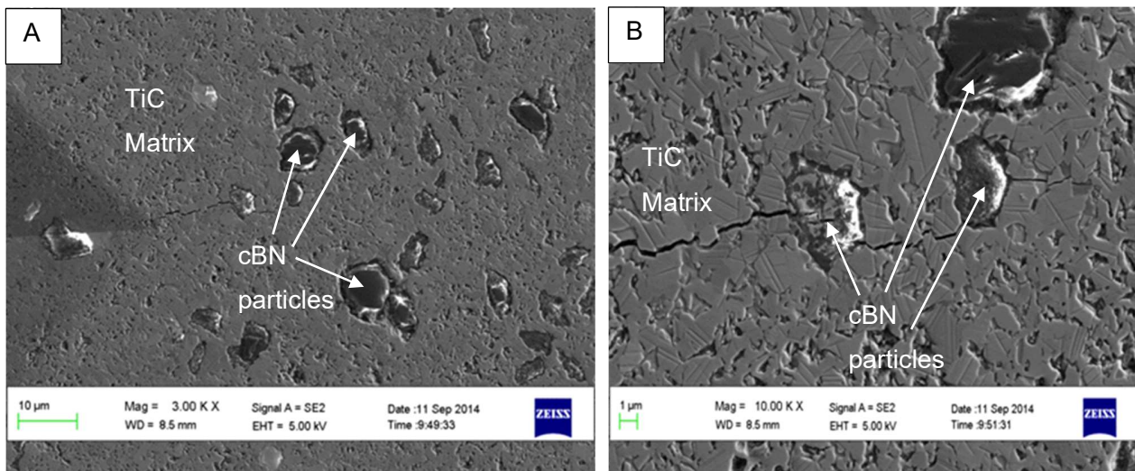
Figure 5.13 SEM micrographs of A – 83.3TiC-2.3Al 2 O 3 -3.7Y 2 O 3 -3.2SiO 2 -7.5 (10 vol.%) cBN SPS'd at 1575°C, 70MPa and 10 min hold time and B - crack path from Vickers Hardness indentation in 83.3TiC-2.3Al 2 O 3 -3.7Y 2 O 3 -3.2SiO 2 -7.5
