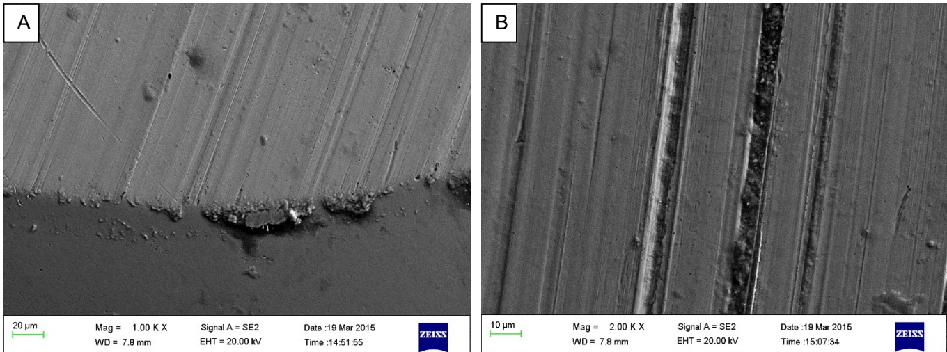
Figure 7.29 A: High magnification image of the edge of the wear scar on the worn AISI 52100 steel ball bearing. B: Higher magnification image of the centre of the wear scar on the worn AISI 52100 steel ball bearing.
