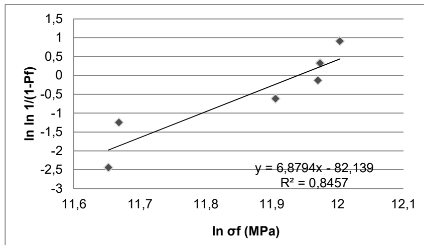
Figure 6.8 Graph of the regression line used to determine the Weibull modulus for 79TiC-11Al 2 O 3 -3Y 2 O 3 -7(10 vol.%) SiCw
