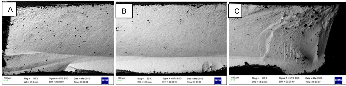
Figure 6.2 A- Outer limit of fractured edge (outside circumference of sample furthest from the site of loading), B- mid-length of fractured edge and C-inner edge of fracture of edge (centre of sample directly under the site of loading)
