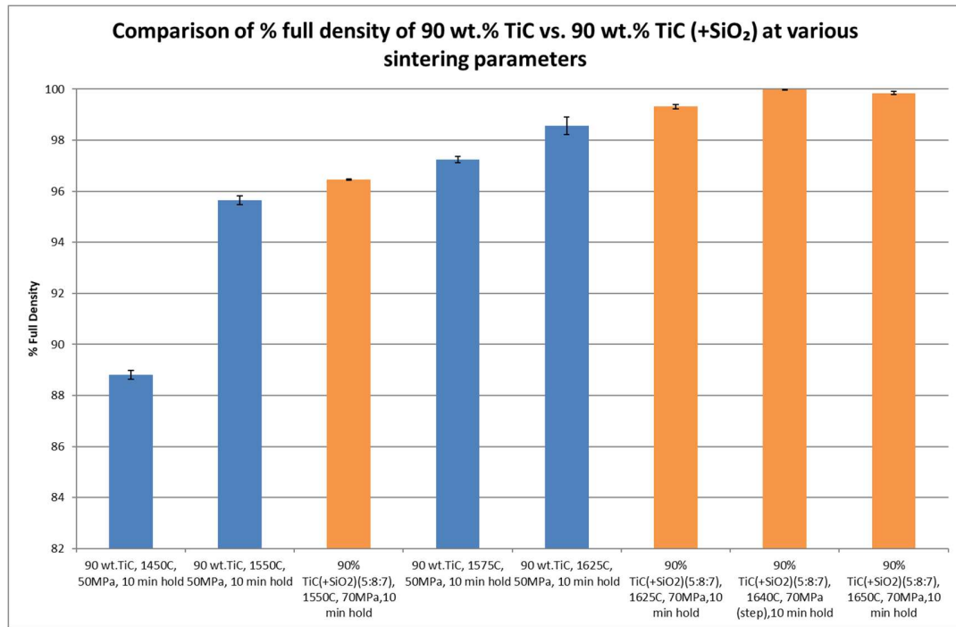
Figure 4.16 Comparison of % of full density of 90 wt.% TiC vs. 90 wt.% TiC(SiO 2 ) at various sintering parameters
