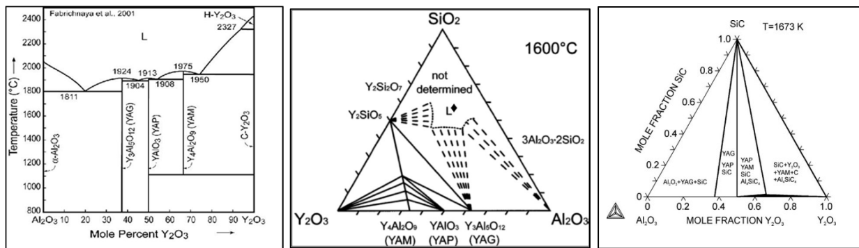
Figure 5.4 \text{Y}_2\text{O}_3 - \text{Al}_2\text{O}_3 phase diagram (Fabrichnaya & Seifert, 2001), Figure 5.5 Isothermal section of the system \text{Y}_2\text{O}_3 - \text{Al}_2\text{O}_3 - \text{SiO}_2 at 1600°C in air (in mol %) (Kolitsch et al., 1999) ♦ - Represents liquid phase sintering aid composition used and Figure 5.6 Phase relation in the ternary system SiC- \text{Al}_2\text{O}_3 - \text{Y}_2\text{O}_3 at 1400°C (Neher et al., 2011)
