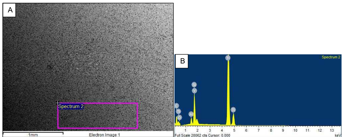
Figure 7.20 A: Spectrum 2 Area alongside the wear track scanned by EDS for composition B: Results of EDS qualitative analysis on Spectrum 2.
