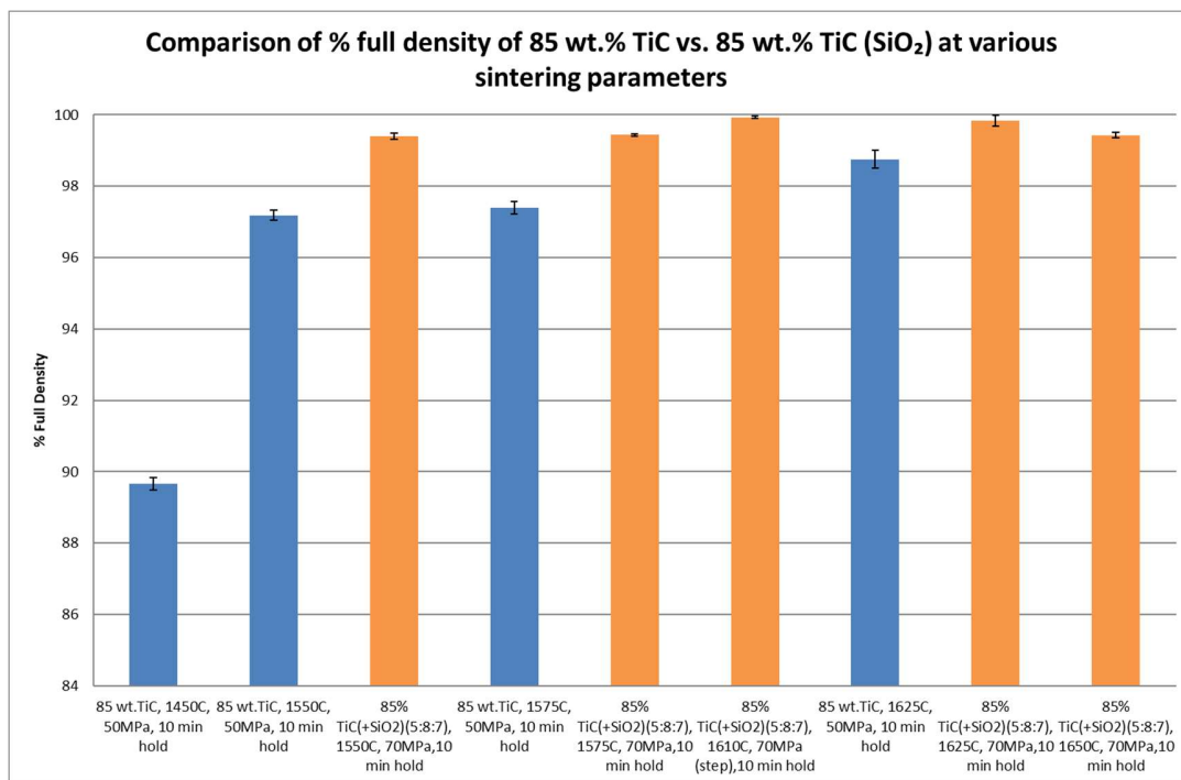
Figure 4.15 Comparison of % of full density of 85 wt.% TiC vs. 85 wt.% TiC(SiO 2 ) at various sintering parameters
