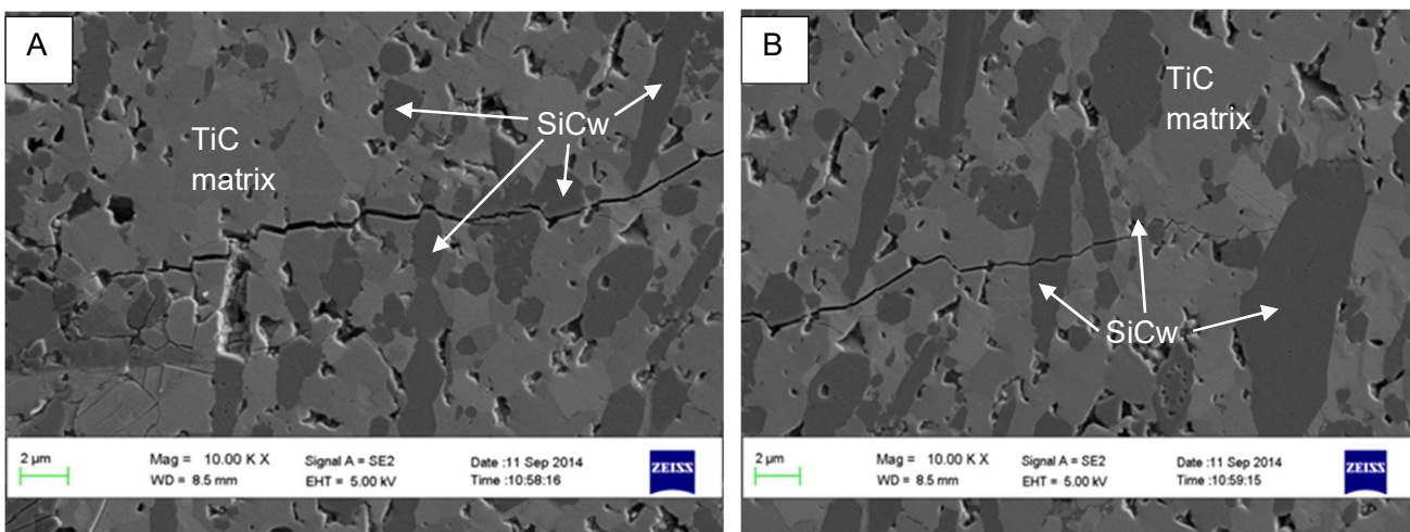
Figure 5.10 SEM micrographs of A – 77TiC-2.1Al 2 O 3 -3.4Y 2 O 3 -3SiO 2 -14.5 (20 vol.%) SiCw SPS'd at 1640°C, 70MPa and 10 min hold time and B - crack path from Vickers Hardness indentation in 77TiC-2.1Al 2 O 3 -3.4Y 2 O 3 -3SiO 2 -14.5 (20 vol.%) SiCw SPS'd at 1640°C, 70MPa and 10 min hold time magnified by 10 K X.
