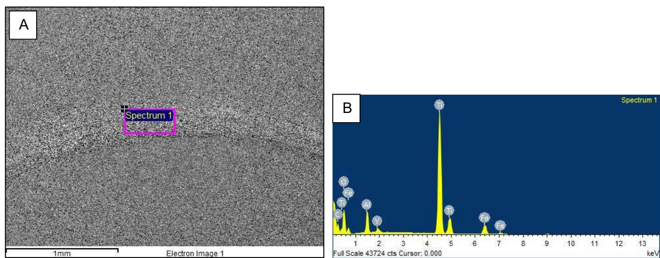
Figure 7.3 A: Spectrum 1 Area on the wear track scanned by EDS for composition B: Results of EDS qualitative analysis on Spectrum 1.
