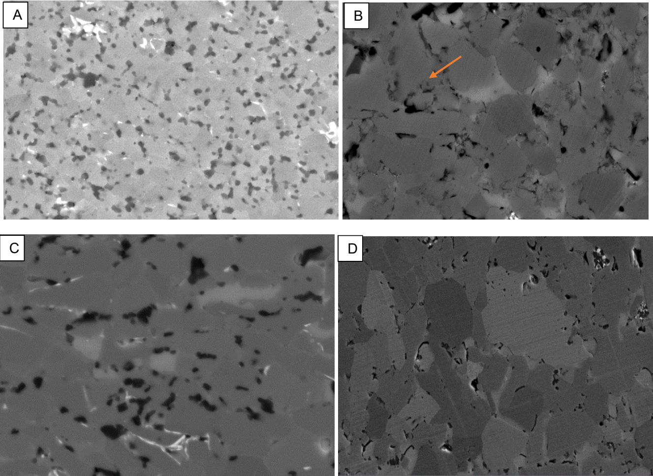
Figure 4.8A: SEM image of the microstructure of 85TiC-12Al 2 O 3 -3Y 2 O 3 SPS'd at 1550 °C, 50MPa and 10 min hold. 4.8B: SEM image of 85TiC-3.75Al 2 O 3 -6Y 2 O 3 -5.25SiO 2 SPS'd at 1610°C, 70MPa and 10 min hold. 4.8C: SEM image of 90TiC-8Al 2 O 3 -2Y 2 O 3 SPS'd at 1550°C, 50MPa and 10 min hold. 4.8D: SEM image of 90TiC-2.5Al 2 O 3 -4Y 2 O 3 -3.5SiO 2 SPS'd at 1625°C, 70MPa and 10 min hold
