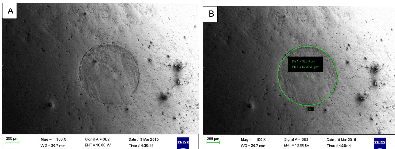
Figure 7.16 A: Wear scar on the surface of the worn AISI 52100 steel ball bearing. B: Diameter and area of the wear scar on the worn AISI 52100 steel ball bearing. (Diameter: 0.929mm and Area: 0.678mm 2 )
