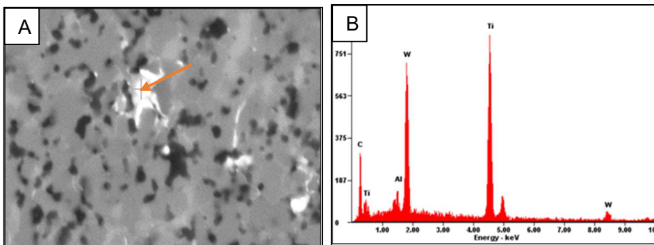
Figure 4.10 A: Image of the area of sintered 85TiC-12Al 2 O 3 -3Y 2 O 3 SPS'd at 1550 °C, 50MPa and 10 min hold scanned by EDS for composition B: Results of EDS qualitative analysis on the area highlighted in Fig. 4.10 A.
