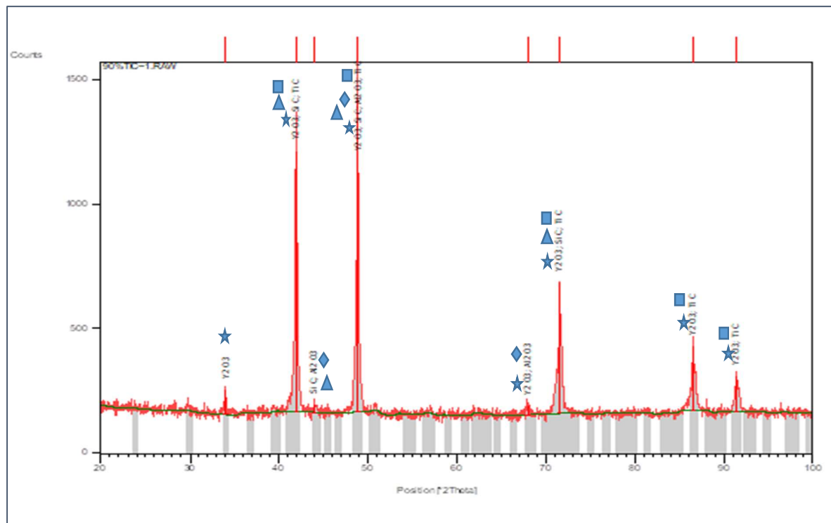
Figure 5.1 a) 90 wt.% TiC (2µm) + 10 vol.% SiCw powder (■TiC, ♦ Al 2 O 3 , ▲SiC, ★Y 2 O 3 )
