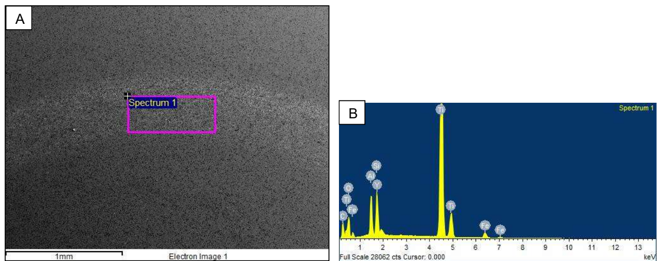
Figure 7.9 A: Spectrum 1 Area on the wear track scanned by EDS for composition B: Results of EDS qualitative analysis on Spectrum 1.
