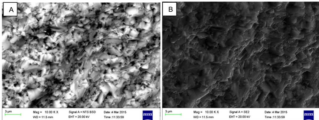
Figure 6.3 A - Fracture surface analysed under high magnification (10.0 K X) using Backscatter Detector and B- same surface analysed under high magnification using Secondary Electron Detector
