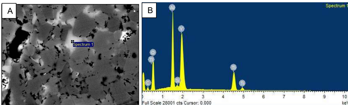
Figure 4.12 A: Image of the area of sintered 90\text{TiC}-2.5\text{Al}_2\text{O}_3-4\text{Y}_2\text{O}_3-3.5\text{SiO}_2 SPS'd at 1625^\circ\text{C} , 70MPa and 10 min hold scanned by EDS for composition B: Results of EDS qualitative analysis on the area highlighted in Fig. 4.12 A.
