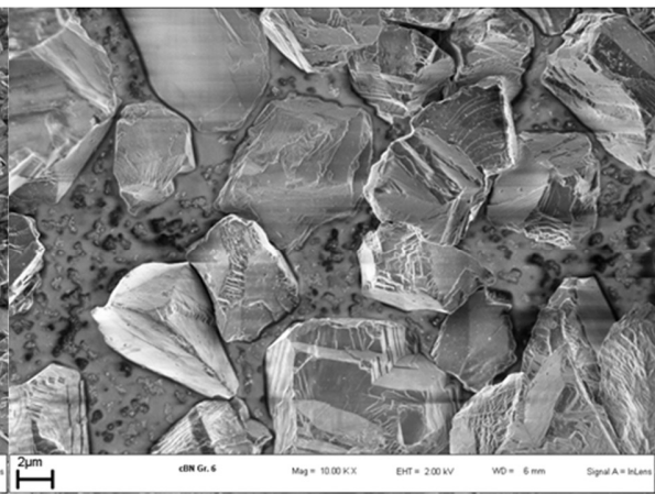
Figure 3.5 SEM image of cBN crush grade 6 (higher magnification)
