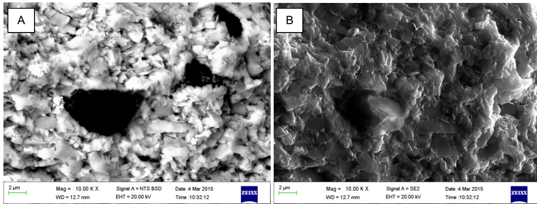
Figure 6.19 A - Fracture surface analysed under high magnification (10.0 K X) using Backscatter Detector and B- same surfaced analysed under high magnification using Secondary Electron Detector
