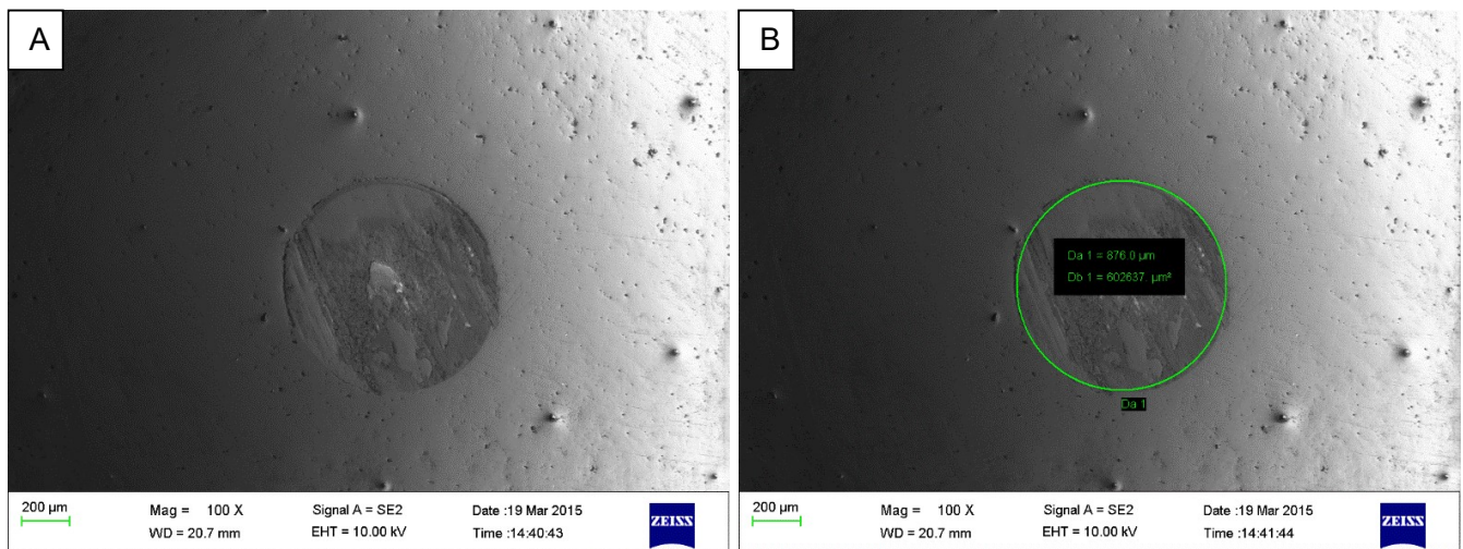
Figure 7.34 A: Wear scar on the surface of the worn AISI 52100 steel ball bearing. B: Diameter and area of the wear scar on the worn AISI 52100 steel ball bearing. (Diameter: 0.876mm and Area: 0.603mm 2 )
