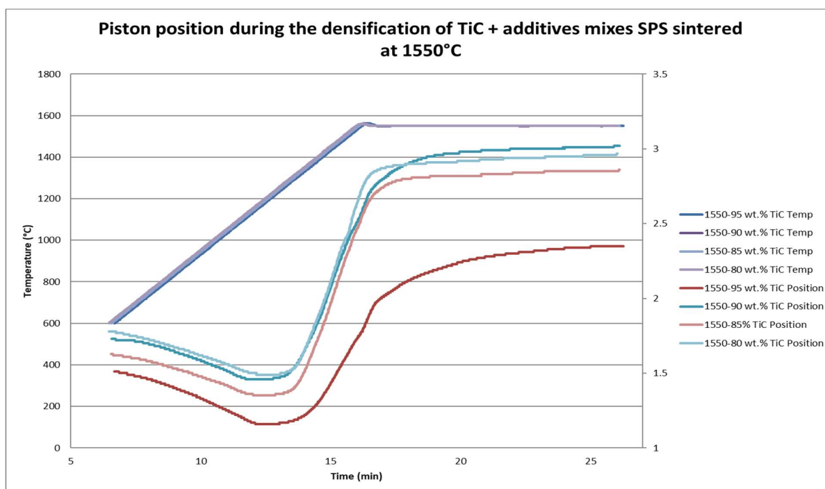
Figure 2 a) Piston position
