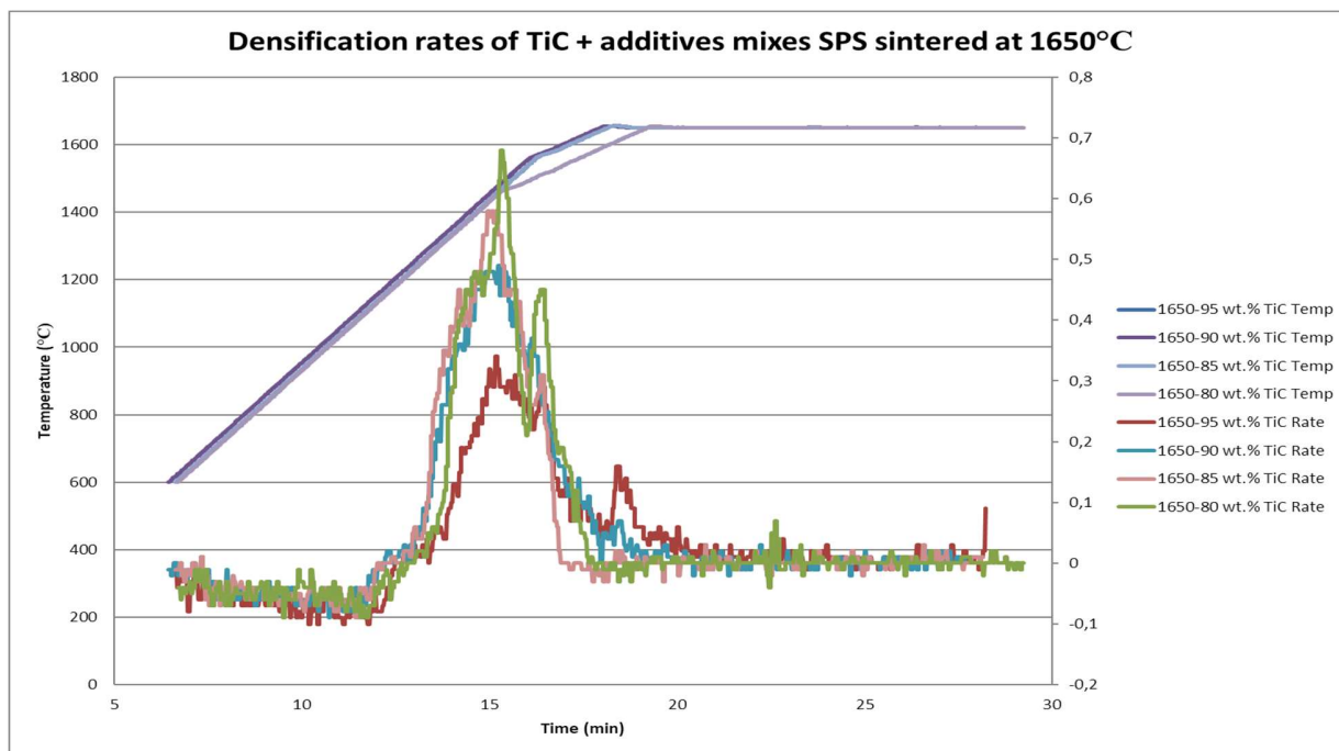
Figure 3 b) Densification rate
