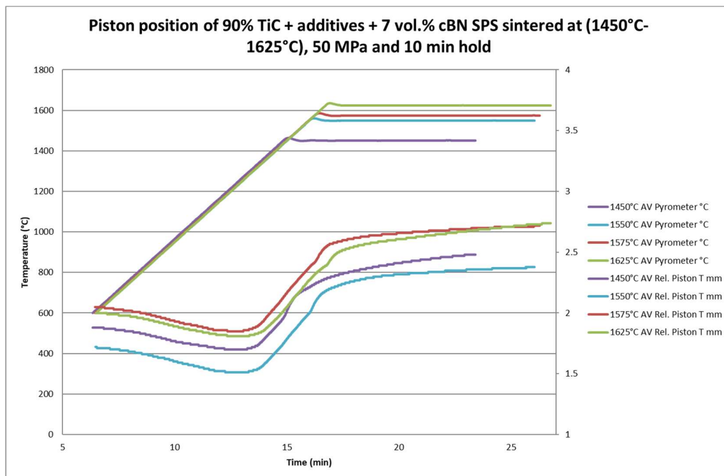
Figure 2 a) Piston position
