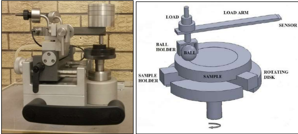
Figure 3.9 Ball on disc sliding wear testing rig. Figure 3.10 Diagram of the positioning of the sample disc and wear ball in a ball on disc sliding wear testing rig (ALEMDAG1* et al., 2015).
