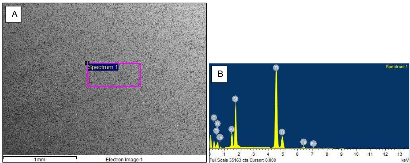
Figure 7.33 A: Spectrum 1 Area on the wear track scanned by EDS for composition B: Results of EDS qualitative analysis on Spectrum 1.
