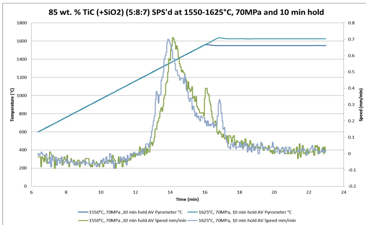
Figure 1 b) Densification rate
