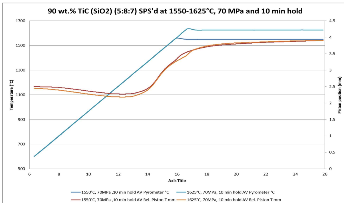
Figure 2 a) Piston position
