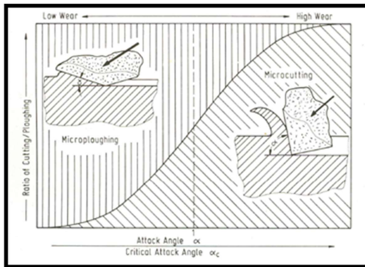
Figure 2.17 Ratio of microcutting to microploughing as a function of the ratio of the attack angle to the critical attack angle (K.-H. Zum Gahr, 1987).
