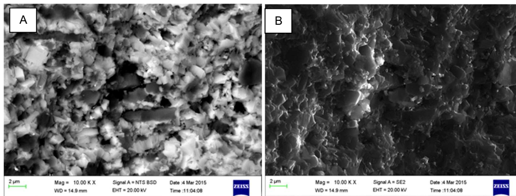
Figure 6.11 A - Fracture surface analysed under high magnification (10.0 K X) using Backscatter Detector and B- same surfaced analysed under high magnification using Secondary Electron Detector
