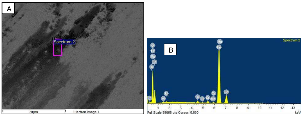
Figure 7.6 A: Spectrum 2 Area inside the wear scar on the worn AISI 52100 steel ball bearing scanned by EDS for composition B: Results of EDS qualitative analysis on Spectrum 2.
