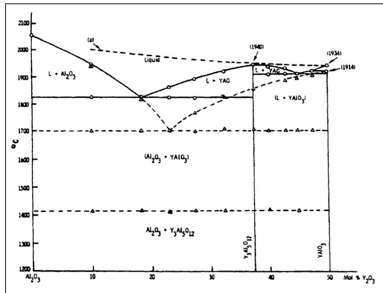
Figure 2.4 Alumina-Yttria phase diagram of the Alumina rich portion of the \text{Al}_2\text{O}_3\text{-Y}_2\text{O}_3 system. The metastable phase diagram is superimposed with dashed lines and the phase fields are labelled (Caslavsky & Viechnicki, 1980).
