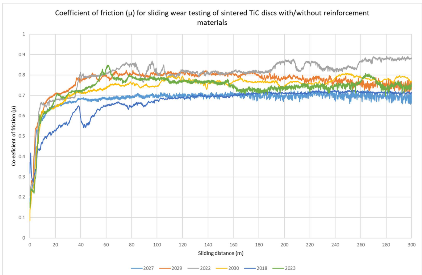
Figure 7.37 Graphs for results given by the CSM Tribometer for the sliding wear tests of the sintered TiC discs with/without reinforcements
