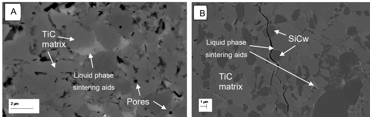
Figure 5.8 SEM micrographs of A - 85TiC-3.75Al 2 O 3 -6Y 2 O 3 -5.25SiO 2 SPS'd at 1610°C, 70MPa and 10 min hold time and B - crack path from Vickers Hardness indentation in 73TiC-3Al 2 O 3 -5Y 2 O 3 -4SiO 2 -15 (20 vol.%) SiCw SPS'd at 1625°C, 70MPa and 10 min hold.
