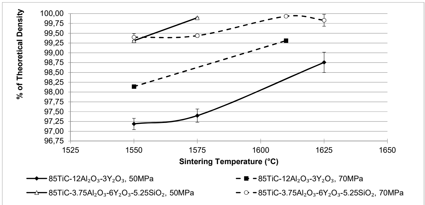
Figure 4.4 Graph of the trends in the density of SPS sintered samples with 85 wt. % TiC and liquid phase sintering aids
