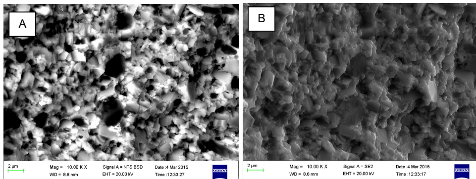
Figure 6.15 A - Fracture surface analysed under high magnification (10.0 K X) using Backscatter Detector and B- same surfaced analysed under high magnification using Secondary Electron Detector
