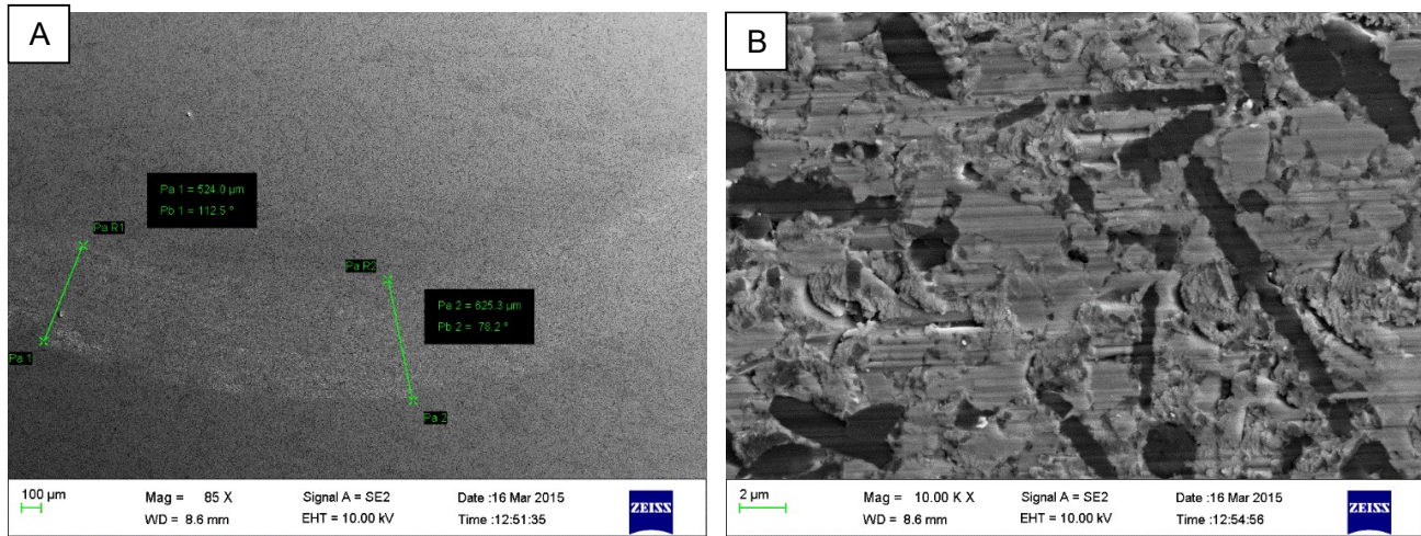
Figure 7.13 A: wear track on the surface of the 73TiC-10Al 2 O 3 -3Y 2 O 3 -14(20 vol.%) SiCw sample disc. B: High magnification image of the wear track on the 73TiC-10Al 2 O 3 -3Y 2 O 3 -14(20 vol.%) SiCw sample disc.
