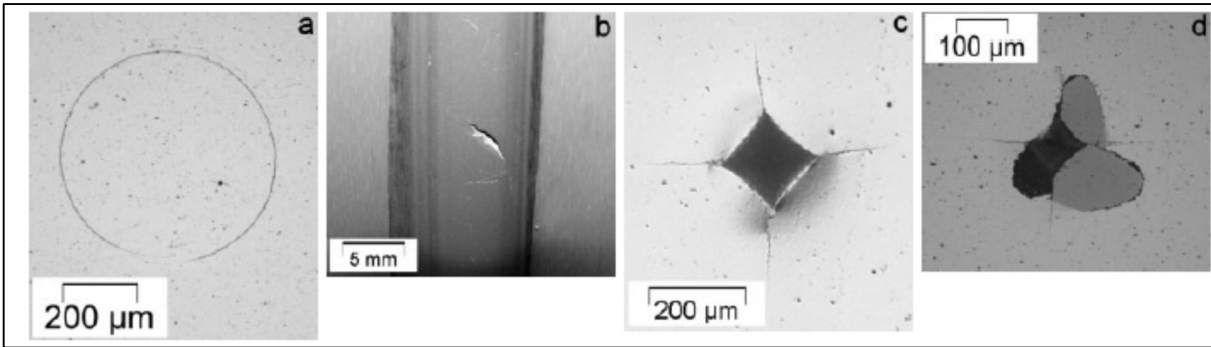
Figure 2.11 Contact damage/cracks on the surface of ceramics: a) Hertzian ring crack in silicon nitride and b) crack caused in operation by the rolling of high alloyed steel wires. These cracks were caused by blunt contact. c) Radial cracks in the corners of a Vickers indent in silicon nitride and d) breakout due to lateral crack under a Vickers indent in silicon carbide. These cracks were caused by a sharp indenter (Danzer et al., 2008).
