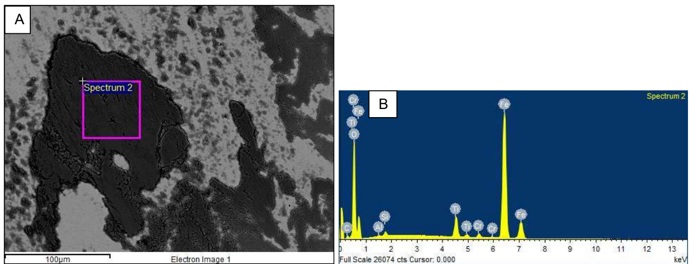
Figure 7.36 A: Spectrum 2 Area inside the wear scar on the worn AISI 52100 steel ball bearing scanned by EDS for composition B: Results of EDS qualitative analysis on Spectrum 2.
