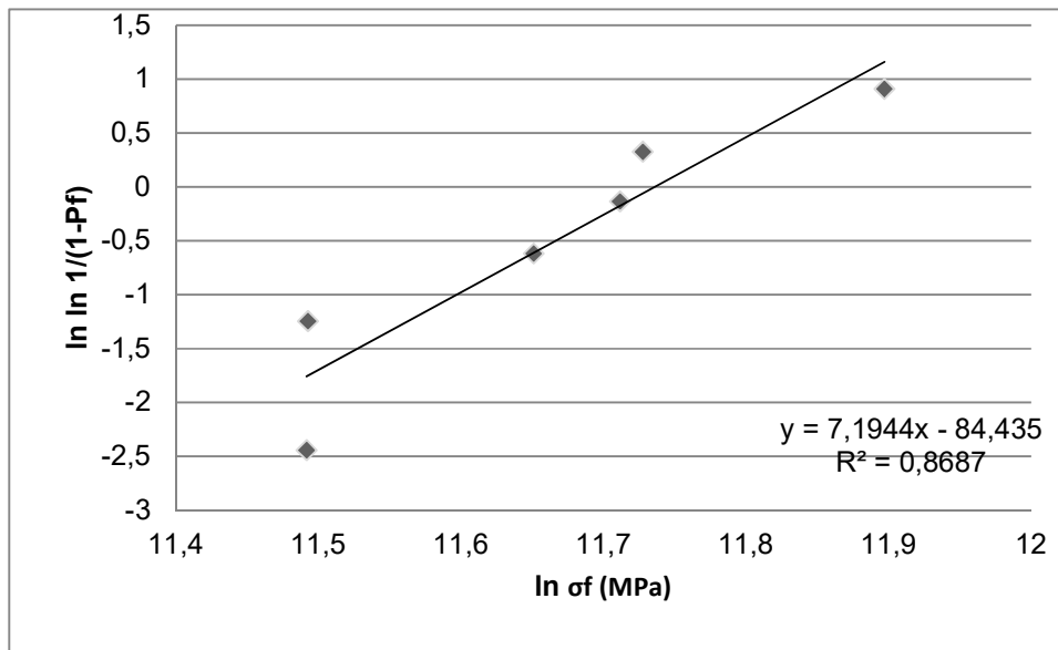
Figure 6.16 Graph of the regression line used to determine the Weibull modulus for 79TiC-4.5Al 2 O 3 -5.6Y 2 O 3 -4.9SiO 2 -7.1(10 vol.%) SiCw
