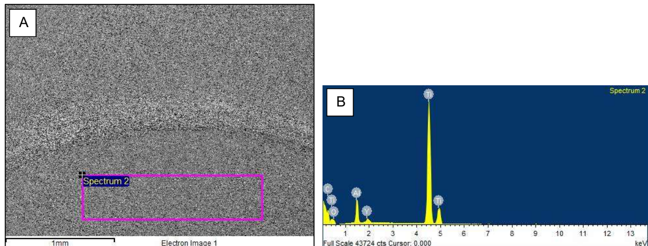
Figure 7.2 A: Spectrum 2 Area alongside the wear track scanned by EDS for composition B: Results of EDS qualitative analysis on Spectrum 2.
