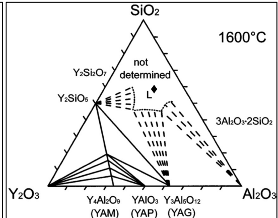
Figure 4.7 Isothermal section of the system \text{Y}_2\text{O}_3 - \text{Al}_2\text{O}_3 - \text{SiO}_2 at 1600°C in air (in mol %). (Kolitsch et al., 1999) ♦ - Represents liquid phase sintering aid composition used.
