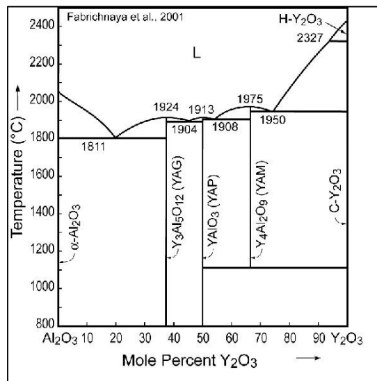
Figure 2.3 Alumina-Yttria phase diagram (Fabrichnaya & Seifert, 2001)
