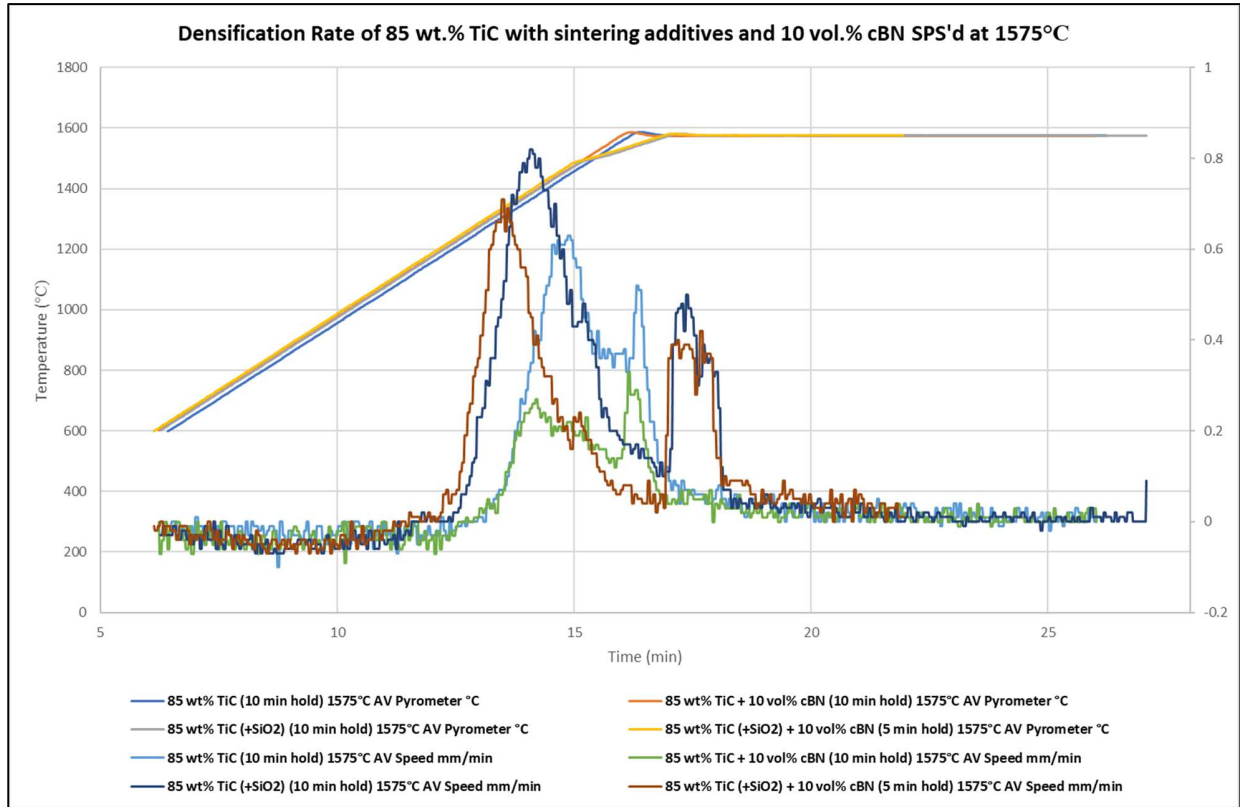
Figure 5.3 Densification rate of 85 wt.% TiC matrices with/without SiO 2 and 10 vol.% cBN SPS'd at 1575°C
