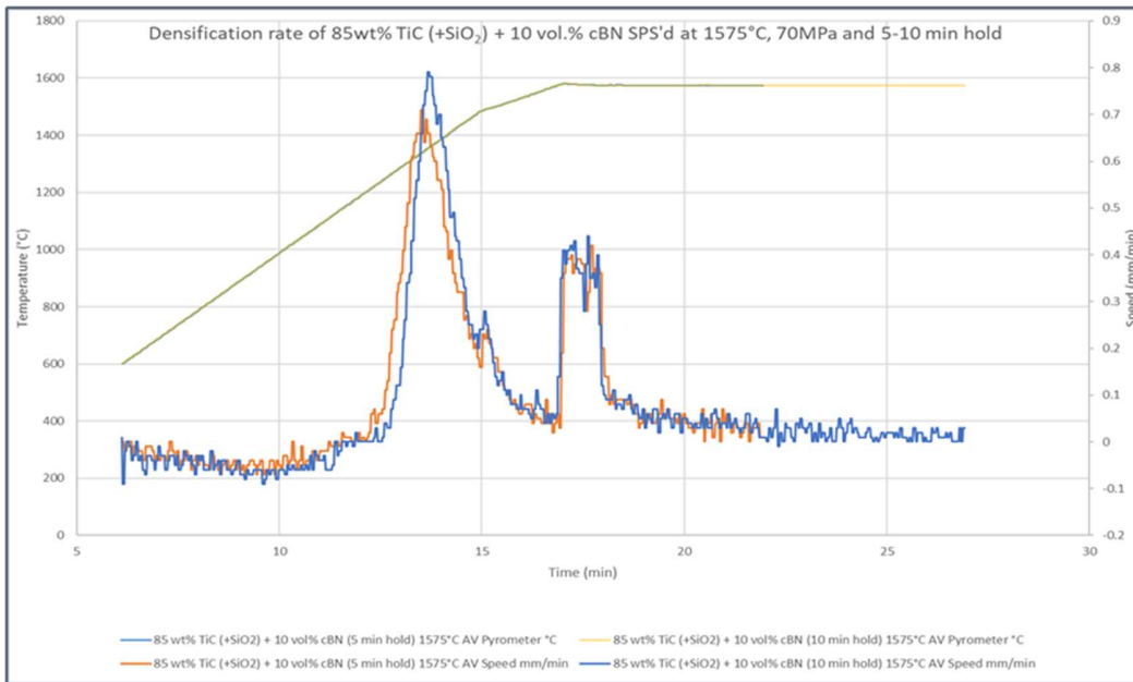
Figure 1 b) Densification rate
