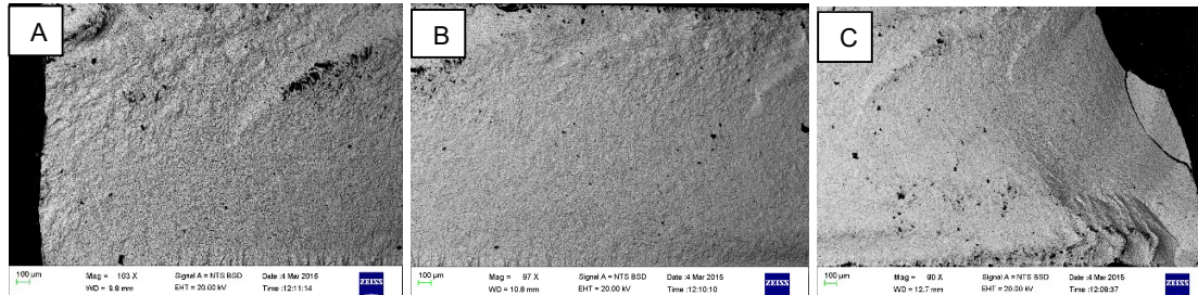
Figure 6.6 A- Outer limit of fractured edge (outside circumference of sample furthest from the site of loading), B- mid-length of fractured edge and C-inner edge of fracture of edge (centre of sample directly under the site of loading)
