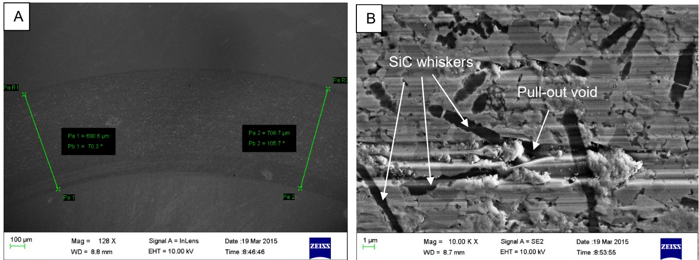
Figure 7.19 A: wear track on the surface of 79TiC-4.5Al 2 O 3 -5.6Y 2 O 3 -4.9SiO 2 -7.1(10 vol.%) SiCw sample disc. B: High magnification image of the wear track on the 79TiC-4.5Al 2 O 3 -5.6Y 2 O 3 -4.9SiO 2 -7.1(10 vol.%) SiCw sample disc.
