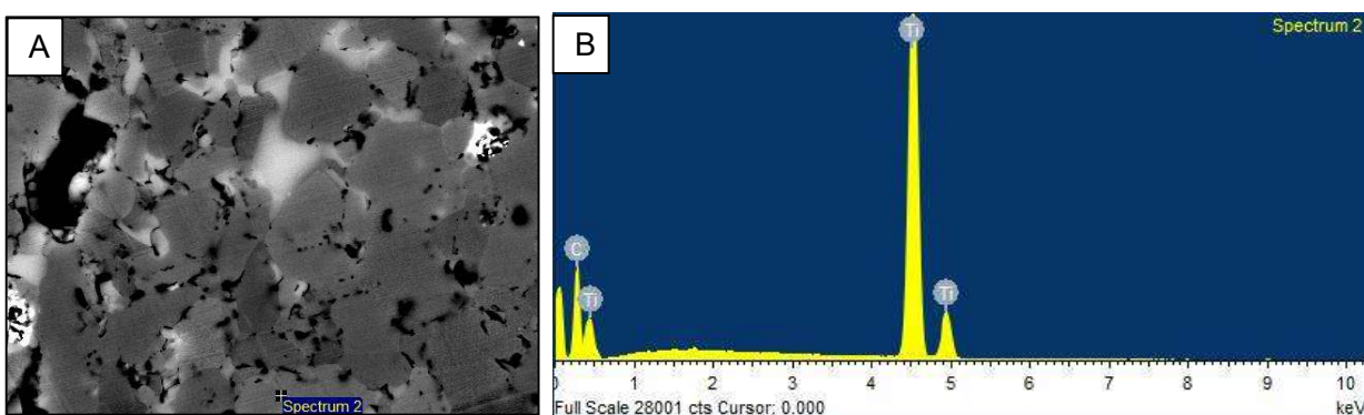
Figure 4.13 A: Image of the area of sintered 90\text{TiC}-2.5\text{Al}_2\text{O}_3-4\text{Y}_2\text{O}_3-3.5\text{SiO}_2 SPS'd at 1625^\circ\text{C} , 70MPa and 10 min hold scanned by EDS for composition B: Results of EDS qualitative analysis on the area highlighted in Fig. 4.13 A.
