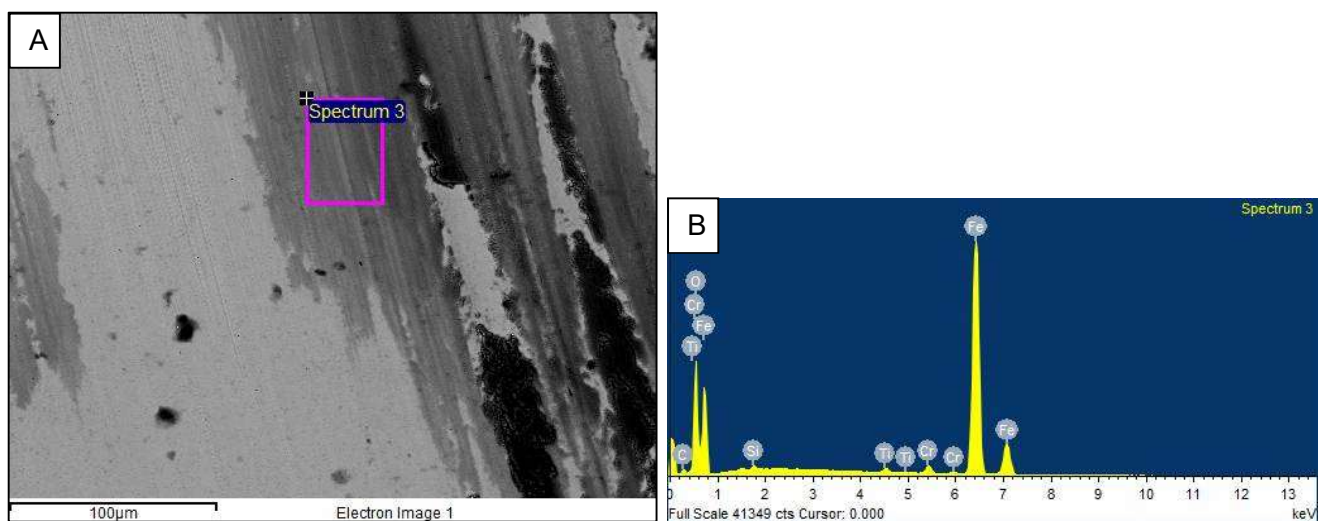
Figure 7.18 A: Spectrum 3 Area inside the wear scar on the worn AISI 52100 steel ball bearing scanned by EDS for composition B: Results of EDS qualitative analysis on Spectrum 3.
