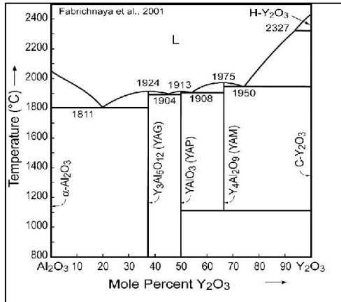
Figure 4.6 \text{Y}_2\text{O}_3 - \text{Al}_2\text{O}_3 phase diagram (Fabrichnaya & Seifert, 2001)
