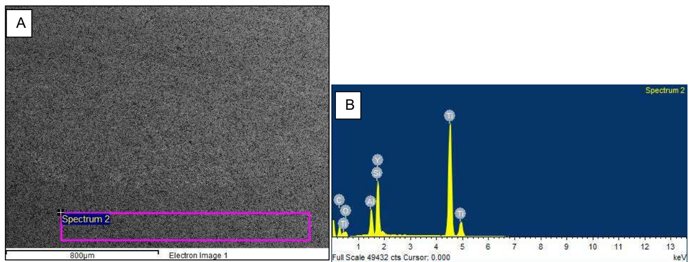
Figure 7.14 A: Spectrum 2 Area alongside the wear track scanned by EDS for composition B: Results of EDS qualitative analysis on Spectrum 2.
