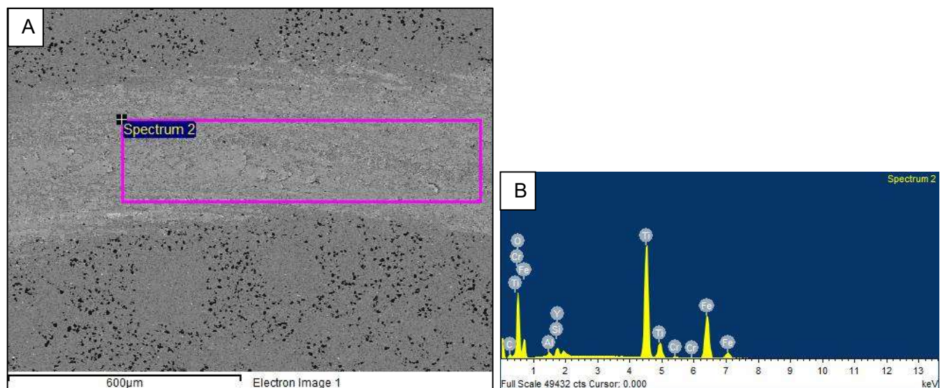
Figure 7.27 A: Spectrum 2 Area on the wear track scanned by EDS for composition B: Results of EDS qualitative analysis on Spectrum 2.
