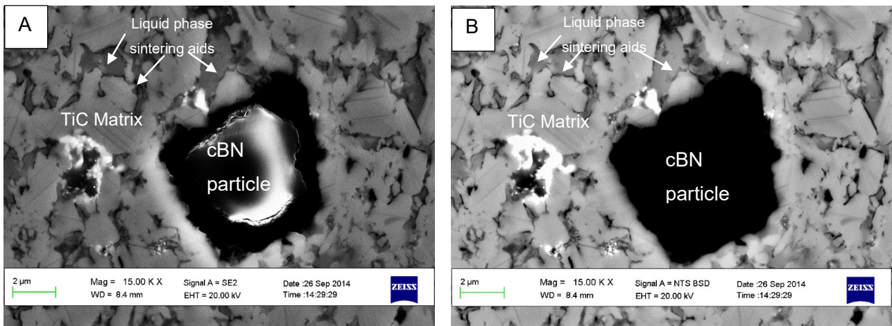
Figure 5.12 SEM micrographs of A – 78.6TiC-3.5Al 2 O 3 -5.6Y 2 O 3 -4.9SiO 2 -7.5 (10 vol.%) cBN SPS'd at 1575°C, 70MPa and 10 min hold time viewed with the Secondary detector magnified by 15 K X and B - 78.6TiC-3.5Al 2 O 3 -5.6Y 2 O 3 -4.9SiO 2 -7.5 (10 vol.%) cBN SPS'd at 1575°C, 70MPa and 10 min hold time viewed via Backscatter detector magnified by 15 K X.
