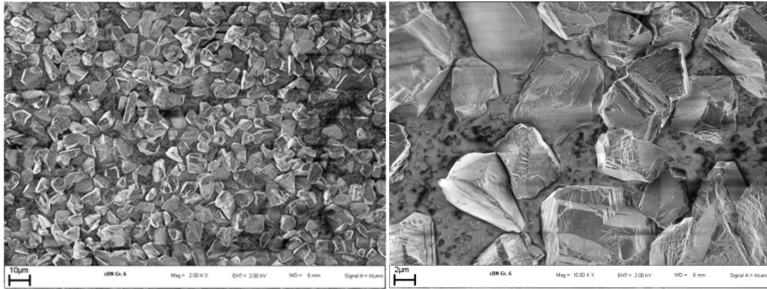
Figure 2.10 SEM morphologies of cBN powders
