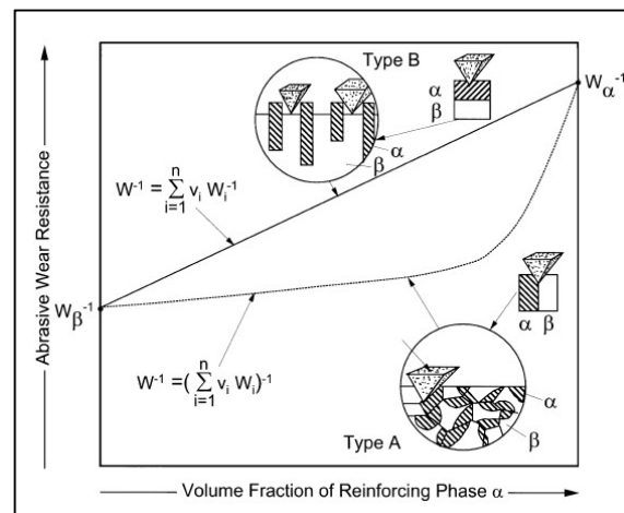
Figure 2.19 Schematic representation of abrasive wear resistance of two-phase structures as a function of volume fraction of a reinforcing phase (K.-H. Z. Gahr, 1998).
