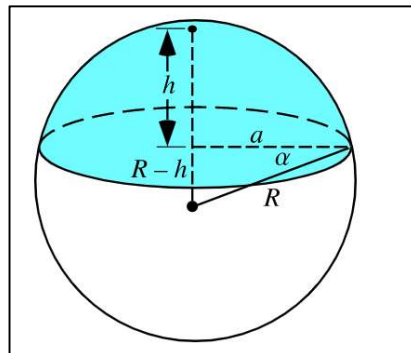
Figure 3.11 Diagram of a spherical cap region of a sphere (Weisstein, n.d.).
