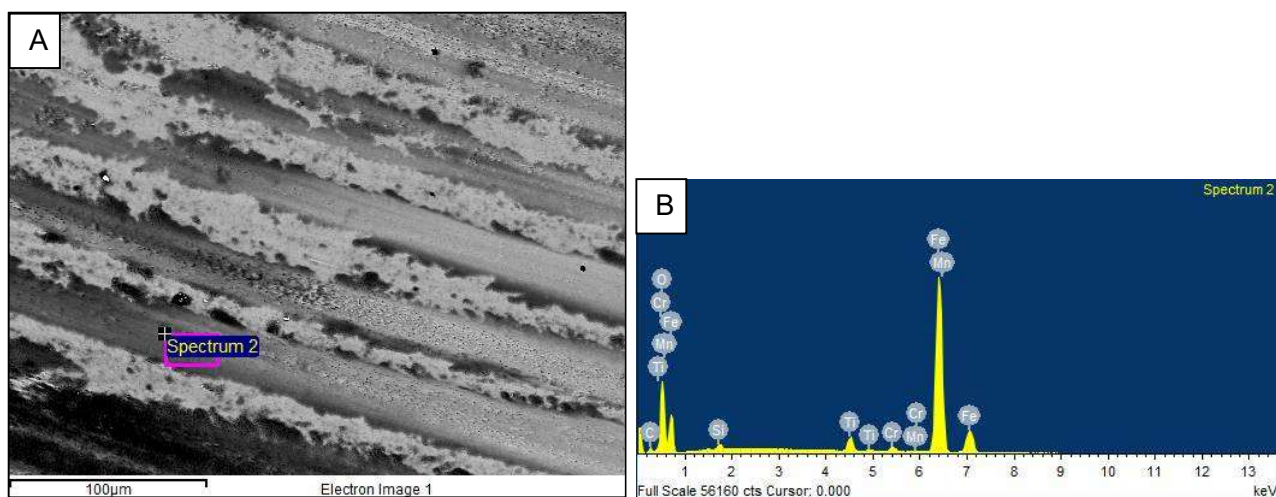
Figure 7.24 A: Spectrum 2 Area inside the wear scar on the worn AISI 52100 steel ball bearing scanned by EDS for composition B: Results of EDS qualitative analysis on Spectrum 2.
