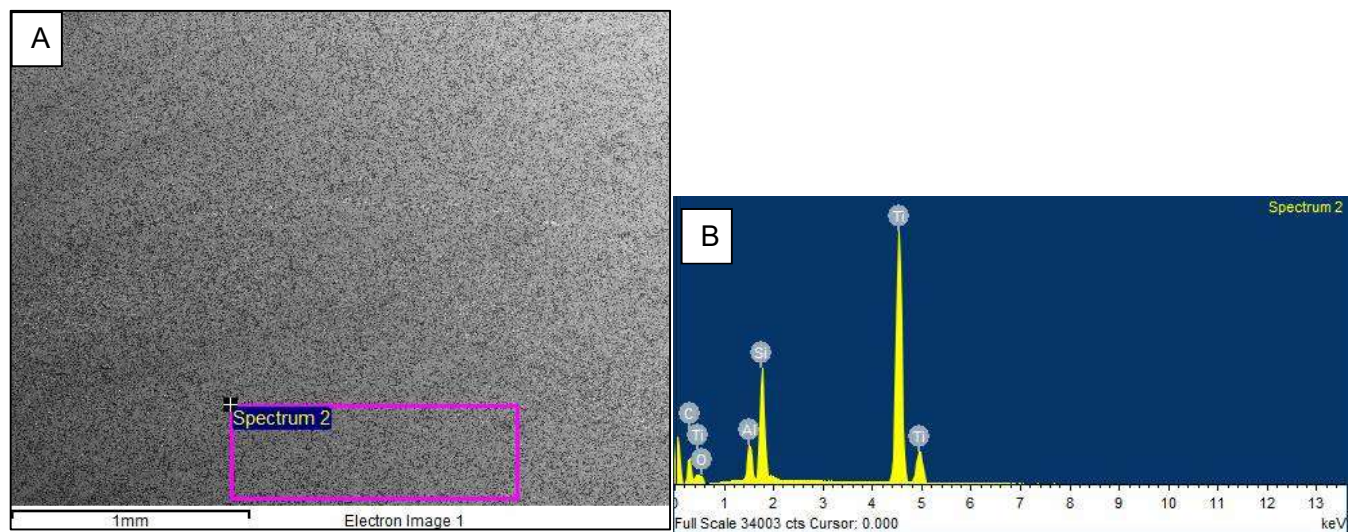
Figure 7.32 A: Spectrum 2 Area alongside the wear track scanned by EDS for composition B: Results of EDS qualitative analysis on Spectrum 2.
