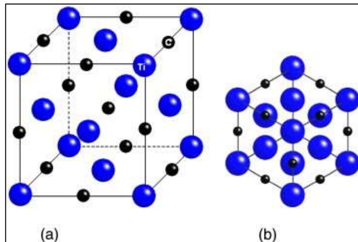
Figure 2.1 (a) Crystal structure of TiC and (b) Projection of TiC atoms along [111] direction. The blue atoms are Ti and the black atoms are C atoms (Li et al., 2008).
