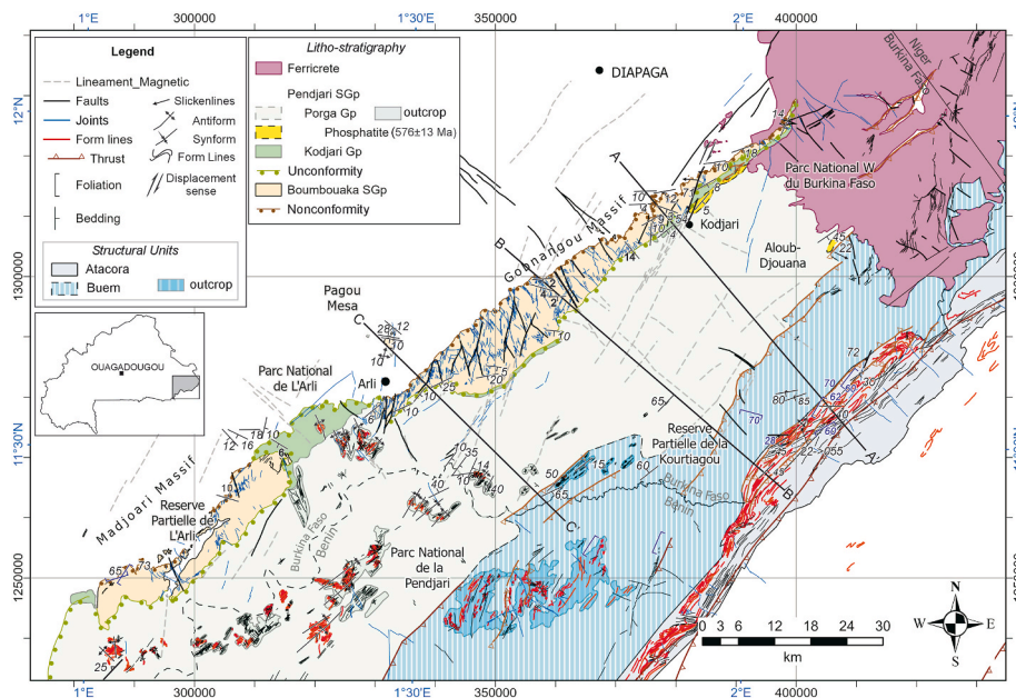
Fig. 8. Litho-stratigraphic map for the Volta Basin in Burkina Faso from this study in WGS84 UTM31N and latitude/longitude. The map presents generalized (1) lithological and structural data collected during field missions, (2) relevant lithologies from the 1:200 000 Parga geological map by the Office Beninois de Mines for northwest Benin and (3) Remote sensing interpretations completed during this study. Magnetic lineaments were extracted from magnetic images of the Volta basin in Burkina Faso. The location of three NW-SE section lines (A-A', B-B', C-C') are marked.
