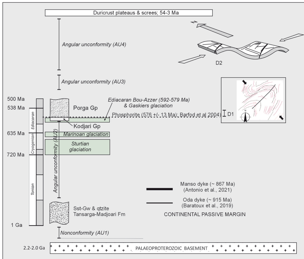
Fig. 12. Schematic event diagram that incorporates stratigraphic and tectonics elements for the Volta Basin in Burkina Faso. D1 deformation is constrained by the Boumbouaka and Pendjari Groups because the rocks are comprehensively folded and faulted along NE-striking axes. D2 deformation event crosscuts D1. The Oda and Manso dyke swarms crosscut the equivalent of the Tansarga-Madjoari Formation (Boumbouaka Group) in Ghana and the age constraint applies to the Volta basin in Burkina Faso by Baratoux et al. (2019) and Antonio et al. (2021) . The age of Sturtian, Marinoan and Ediacaran Bou-Azzer and Gaskiers glaciations are by Williams et al. (2008) , Pu et al. (2016) , Letsch et al. (2018) , Wang et al. (2023) . Age constraints for the Pendjari Group are by Bozhko et al. (1971, 1974) , Clauer (1976) , Clauer and Deynoux (1987) , Barfod et al. (2004) , Kalsbeek et al. (2008) , Ganade et al. (2016) , and Antonio et al. (2021) .
