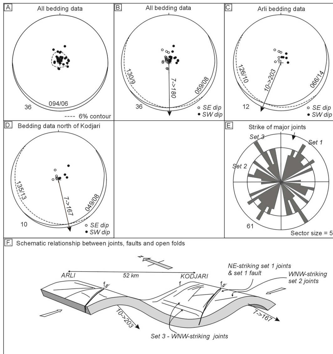
Fig. 11. Equal area stereographic projections, rose and schematic block model for the Boumbouaka Supergroup along the Madjoari and Gobjangou massifs. Bedding data with calculated mean at 094/06, 36 measurements. Bedding data divided into southwest and southeast calculated means. Mean calculated fold plunge is 7->180. Bedding data divided into southwest and southeast calculated means for the region close to the village of Arli. Mean calculated fold plunge is 10->203. Bedding data divided into southwest and southeast calculated means for the region north of the village of Kodjari. Mean calculated fold plunge is 7->167. Rose plot of the strike of single Master Joints, which are near vertical. Sets 1–3 are consistent across the massifs. Block diagram for the Gobjangou Massif over 52 km resolves gentle folding of the sandstone-greywacke and quartzite beds of the Tansarga-Madjoari Formation. Master joints and faults are interpreted to have formed during folding and progressive deformation in D2.
