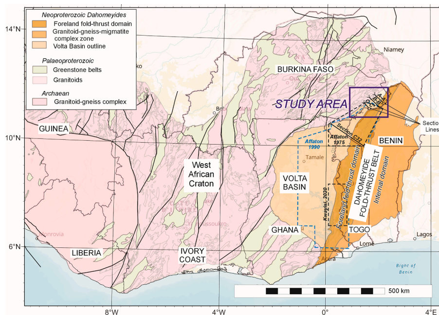
Fig. 1. Location map of the Volta Basin in the West African craton (modified after Markwitz et al., 2016). Studies areas of Affaton (1975, 1990), and Kwayisi et al. (2020) are shown in dashed lines. The study area and location of three NW-SE section lines (A-A', B-B', C-C') are given for this study. The NW-SE section line C32 of Affaton (1975) extends for 190 km from the village of Dapango in Togo to Perma in Benin.
