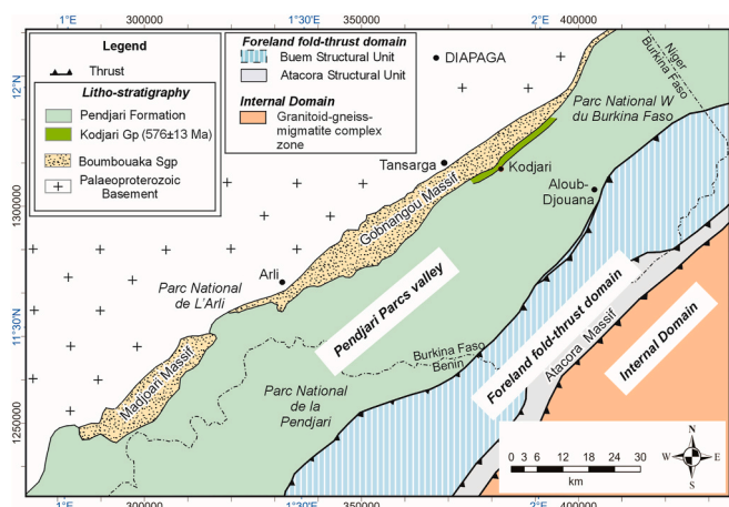
Fig. 3. Schematic structural geology map presented by Affaton (1975 & 1990, Fig. 31) and Kabore and Ouedraogo (2006) of the Volta Basin in Burkina Faso, gridded for WGS84 UTM31N and latitude/longitude. The map broadly locates the position of the Dahomeyide foreland fold thrust domain and Internal Domain in Benin and Burkina Faso. The fold thrust domain was broadly divided into the Buem and Atacora structural units as interpreted by Affaton (1975) from photogrammetry.
