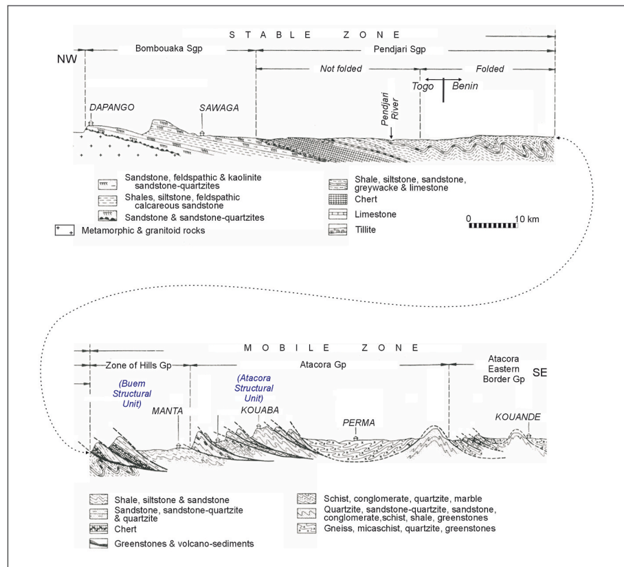
Fig. 2. A modified version of the schematic NW-SE section C32 from Affaton (1975) with a stable domain of undeformed geology and mobile zone representing the Dahomeyide foreland fold-thrust belt, with Buem and Atacora structural units. The distance between the town of Perma in Benin at Lat/Long 10.123052° and 1.439382° and Dapango in Togo at Lat/Long 10.873542° and 0.200808° is approximately 160 km.
