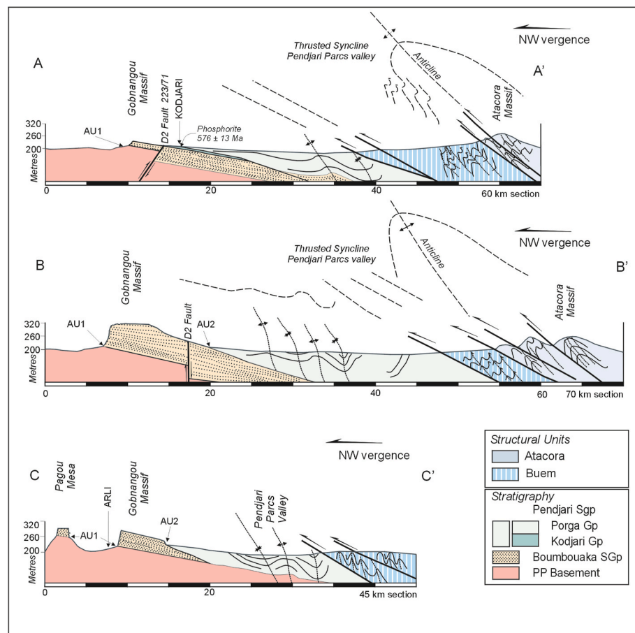
Fig. 10. Schematic cross-sections A-A', B-B' and C-C' for the Volta Basin in Burkina Faso. The cross-sections present the interpreted trace of beds, thrusts and the form of folds in the Pendjari Parc valley, Buem and Atacora structural units. The Atacora Structural Unit is defined by a macroscopic anticline. The Buem Structural Unit is interpreted as the overturned northwestern limb of the anticline. It is important to note that the felspathic sandstone-greywacke beds of the Boumbouaka Supergroup in the Gobnangou massif and Palaeoproterozoic basement are unconformably overlain by siltstone-shale sequences of the Pendjari Supergroup that are folded, thrust-faulted and sheared.
