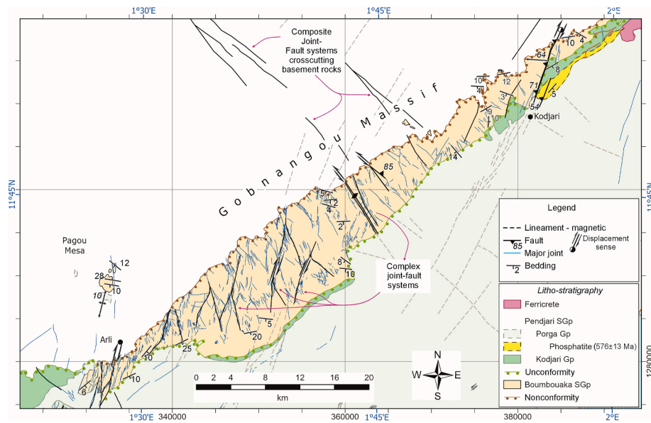
Fig. 9. Map of joints, fracture corridors, and fracture-faults that are evident from remote sensing images across the Gobnangou Massif in WGS84 UTM. Certain fracture corridors and faults coincide and crosscut the Palaeoproterozoic basement in several locations. Magnetic lineaments extracted as linear attributes from magnetic imagery coincide with fracture corridors suggesting that the corridors could be up to 50 km in strike length.
